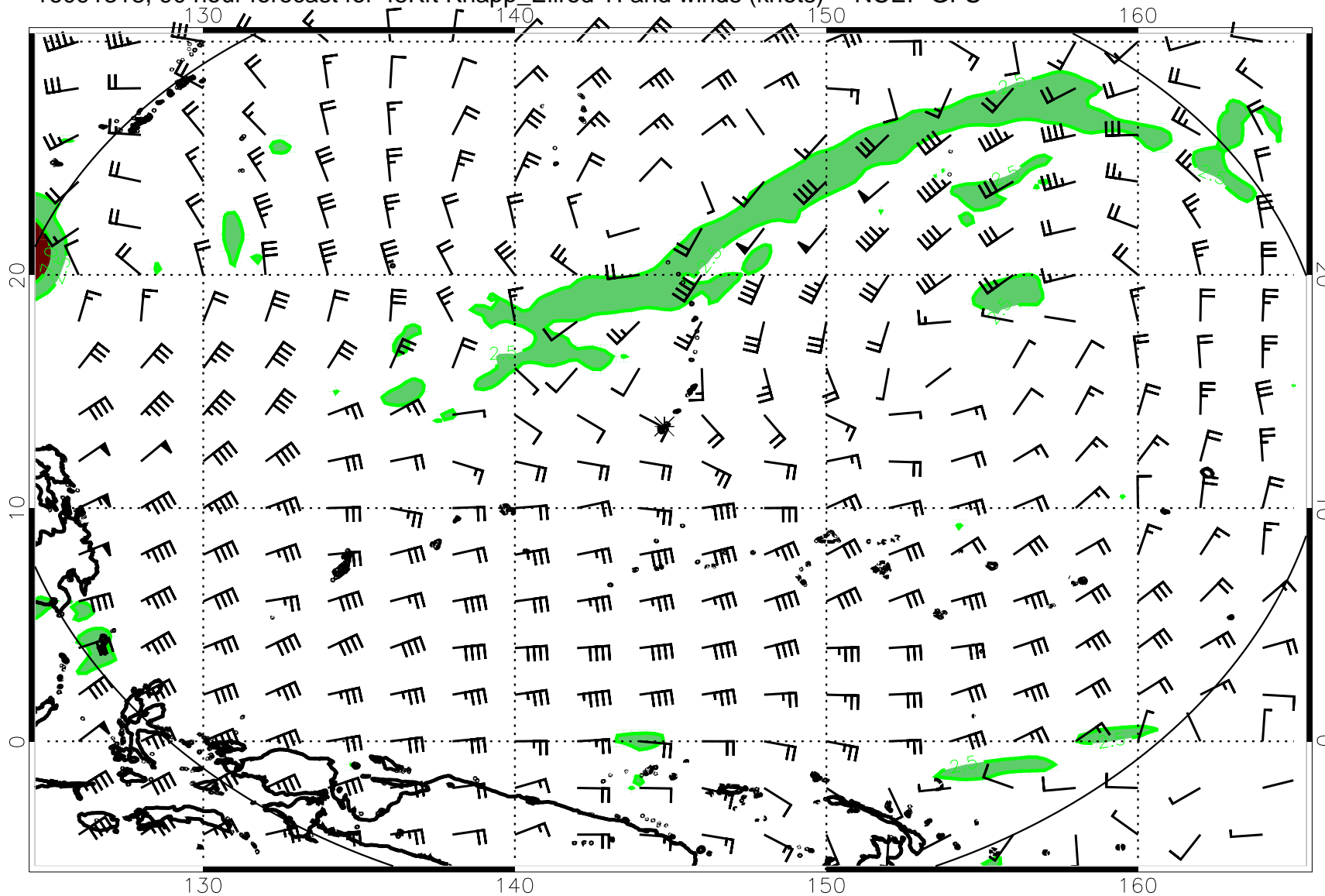
16091318, 90 hour forecast for 45Kft Knapp_Ellrod TI and winds (knots) -- NCEP GFS
