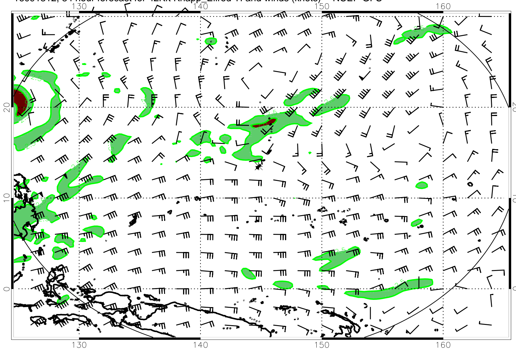
16091312, 84 hour forecast for 42Kft Knapp_Ellrod TI and winds (knots) -- NCEP GFS
