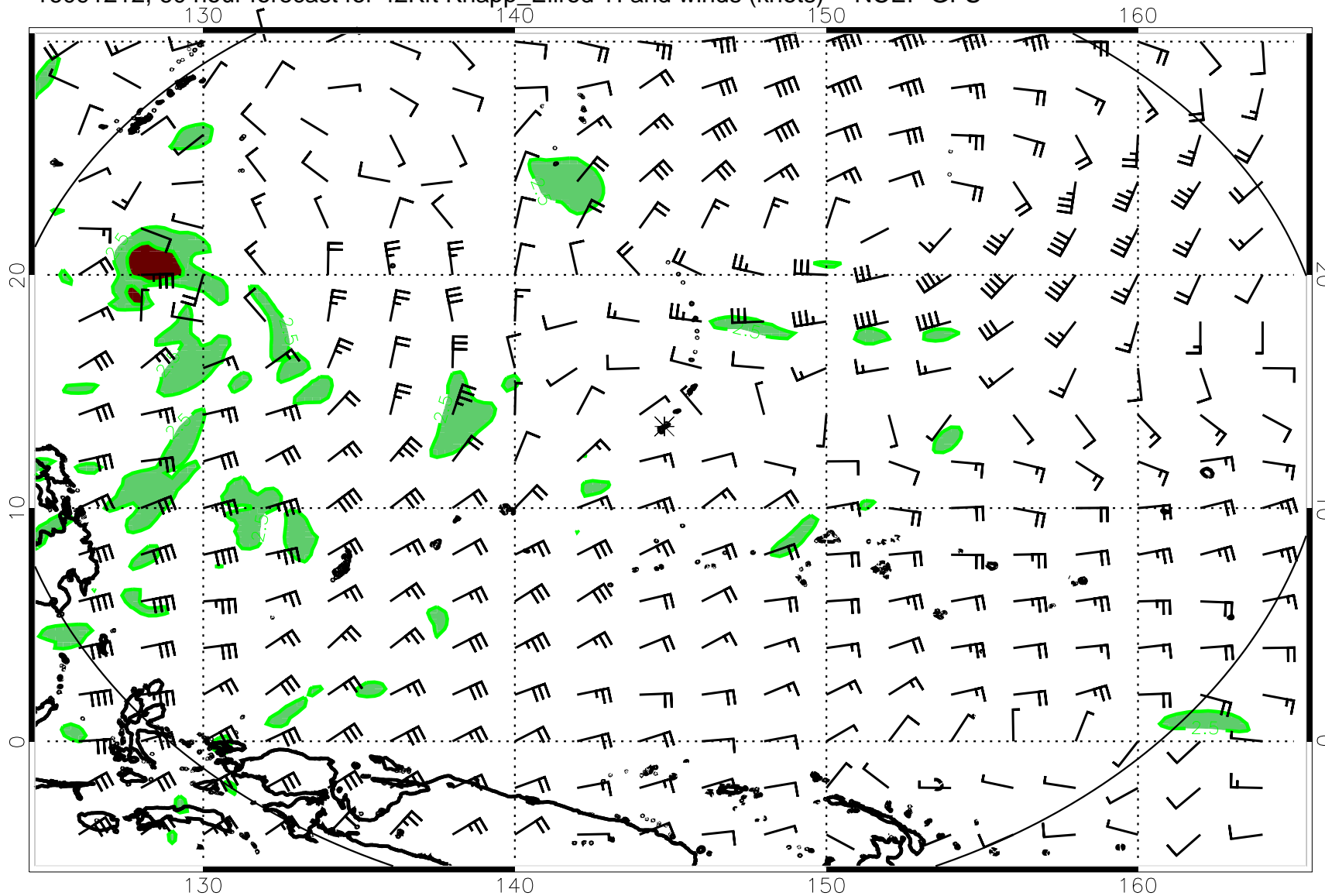
16091212, 60 hour forecast for 42Kft Knapp_Ellrod TI and winds (knots) -- NCEP GFS
