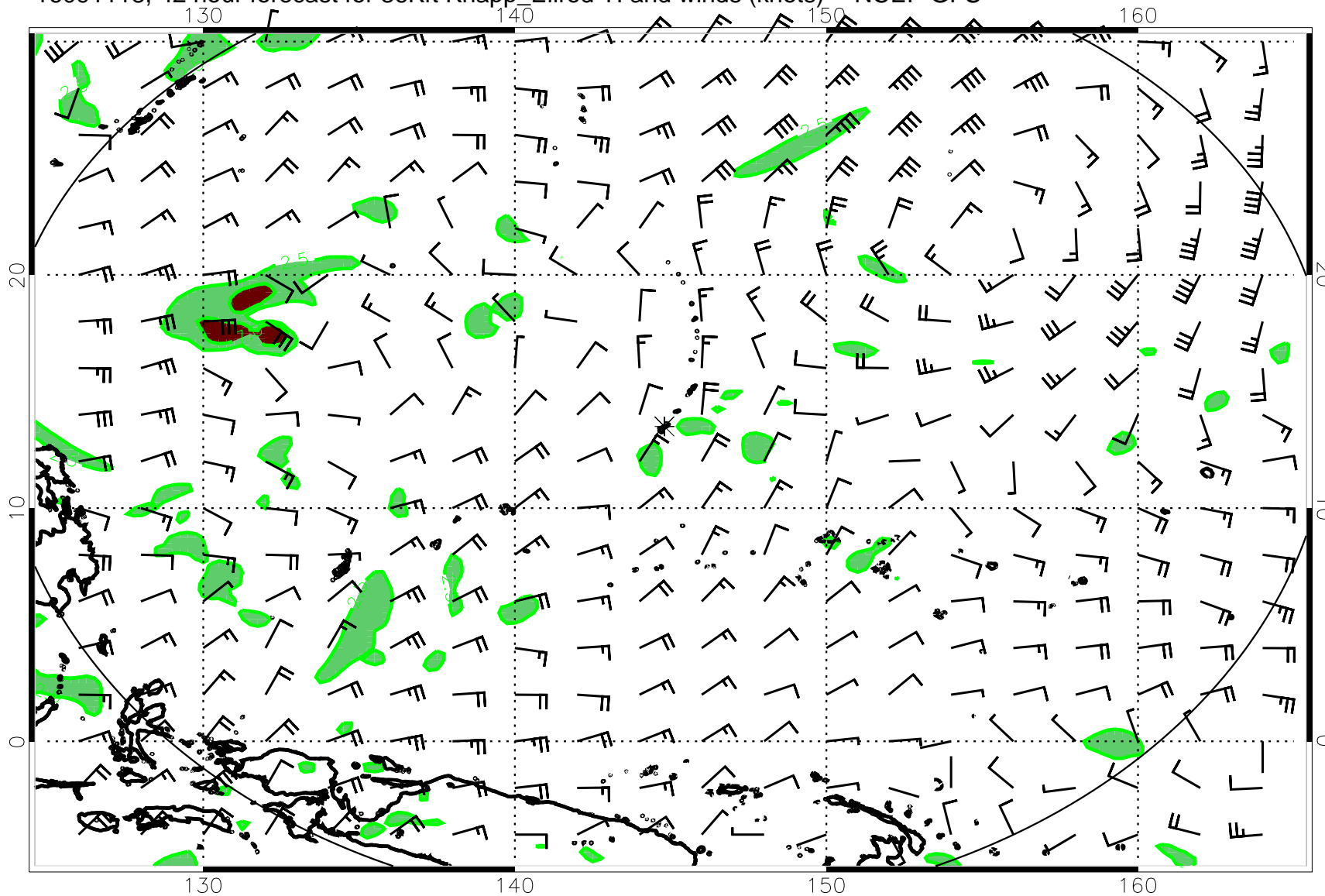
16091118, 42 hour forecast for 36Kft Knapp_Ellrod TI and winds (knots) -- NCEP GFS
