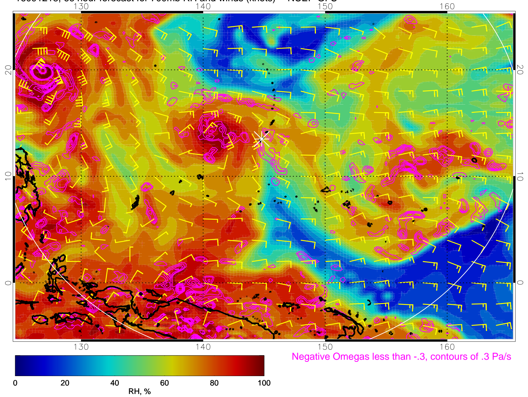
16091218, 66 hour forecast for 700mb RH and winds (knots) -- NCEP GFS
