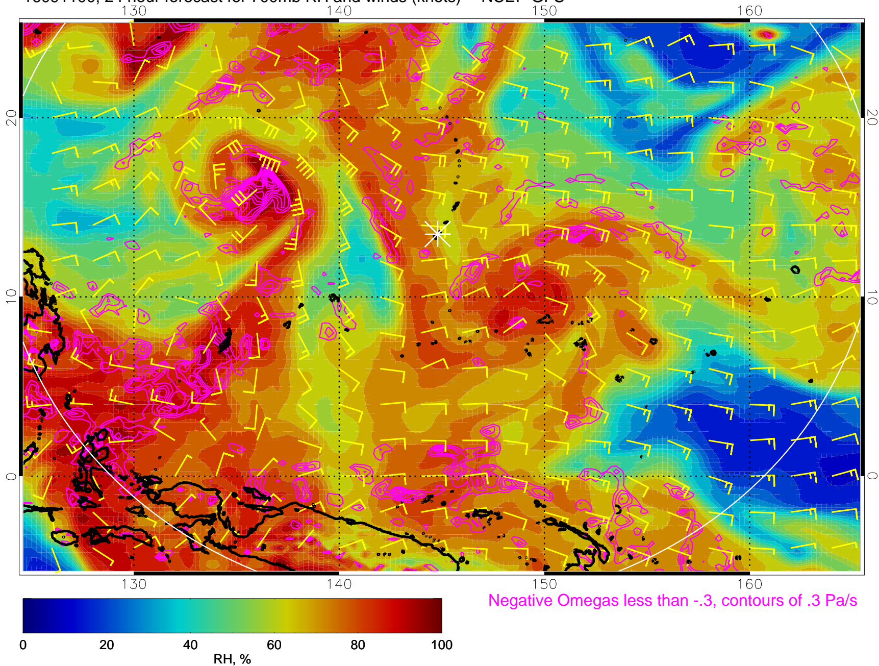
16091100, 24 hour forecast for 700mb RH and winds (knots) -- NCEP GFS
