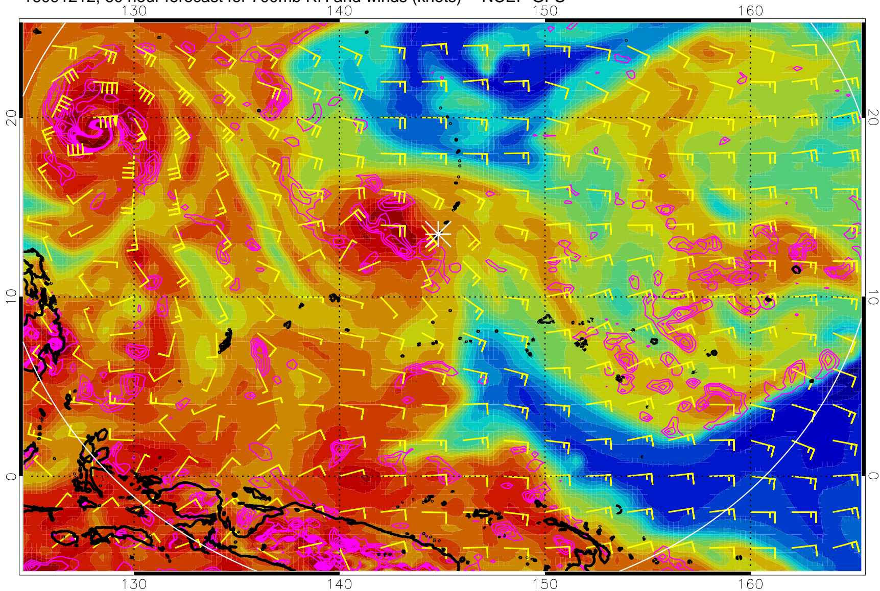
16091212, 60 hour forecast for 700mb RH and winds (knots) -- NCEP GFS
