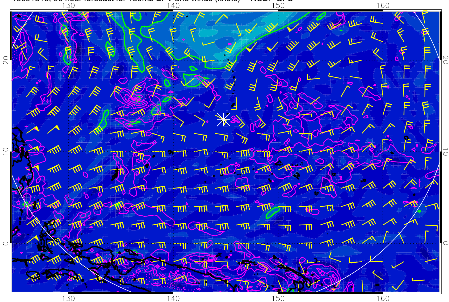
16091318, 90 hour forecast for 150mb EPV and winds (knots) -- NCEP GFS
