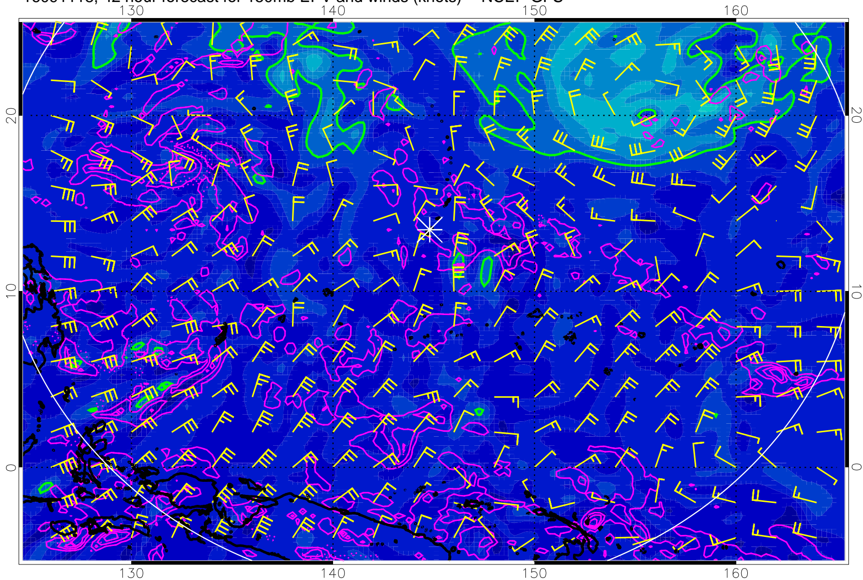
16091118, 42 hour forecast for 150mb EPV and winds (knots) -- NCEP GFS
