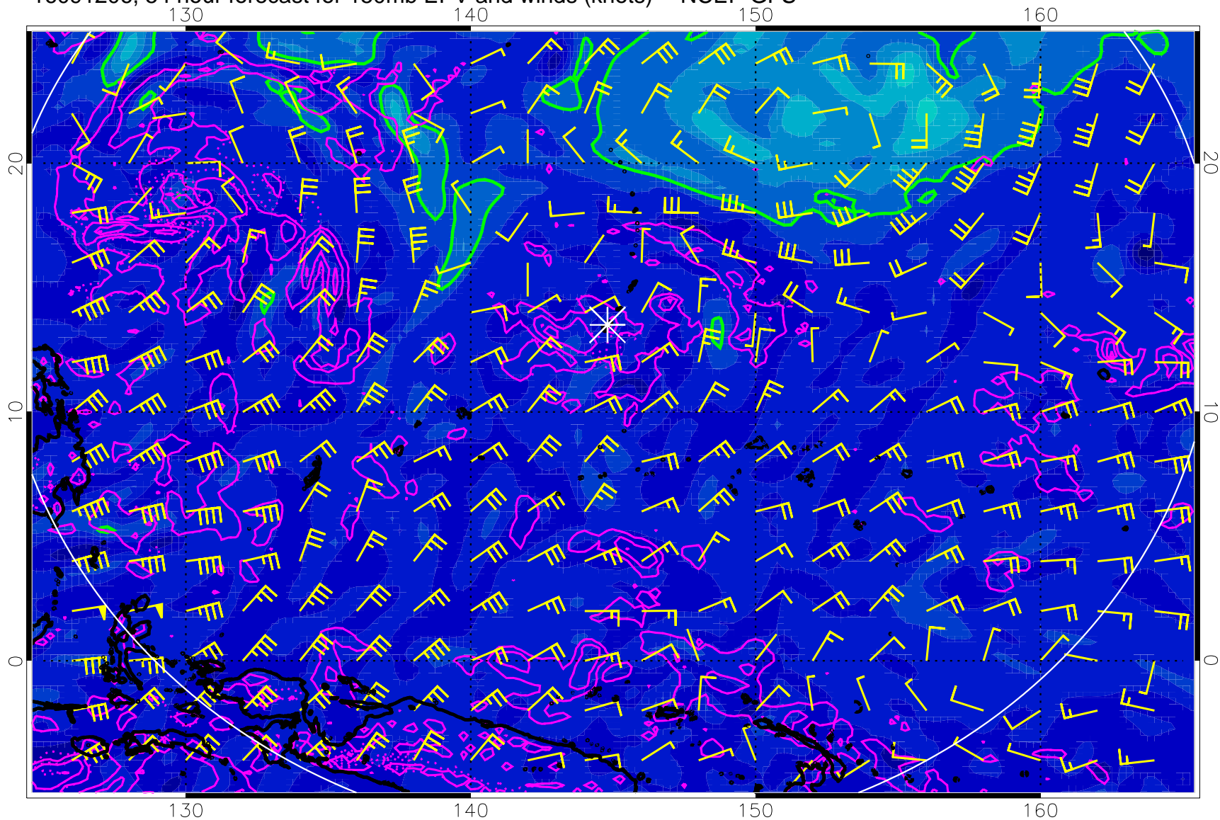
16091206, 54 hour forecast for 150mb EPV and winds (knots) -- NCEP GFS
