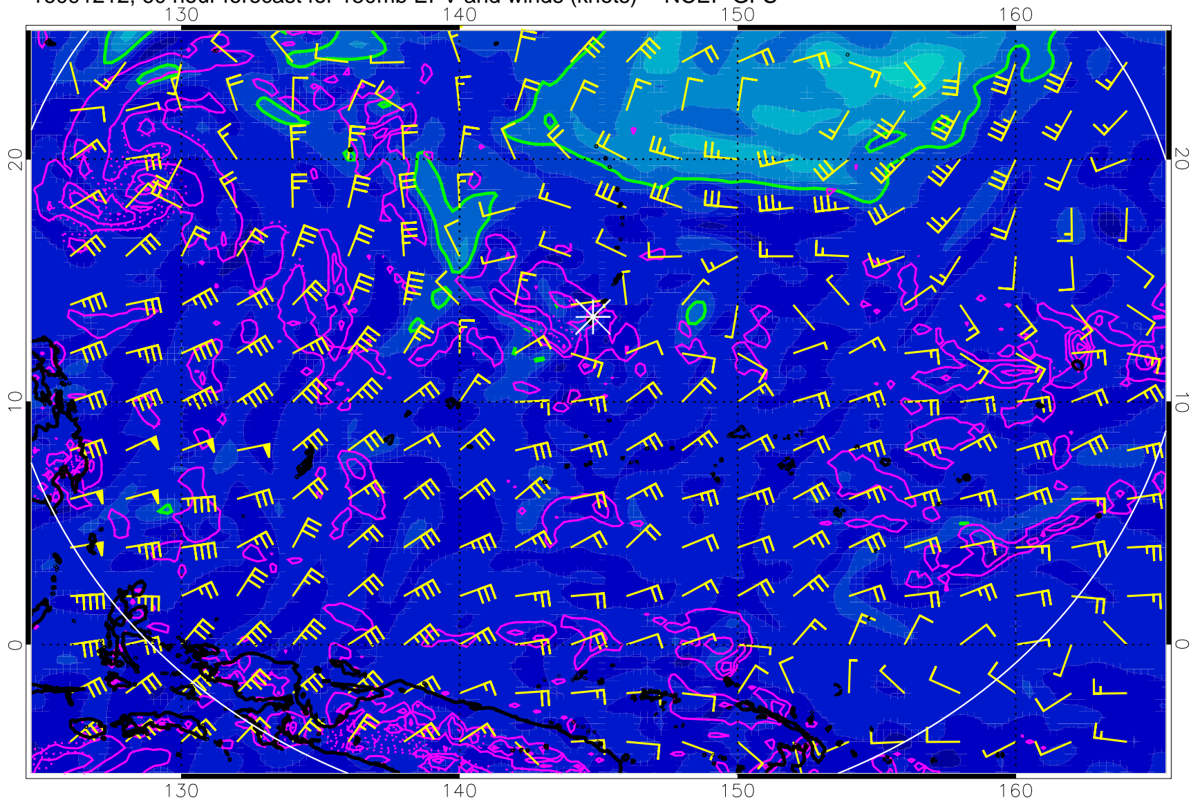
16091212, 60 hour forecast for 150mb EPV and winds (knots) -- NCEP GFS
