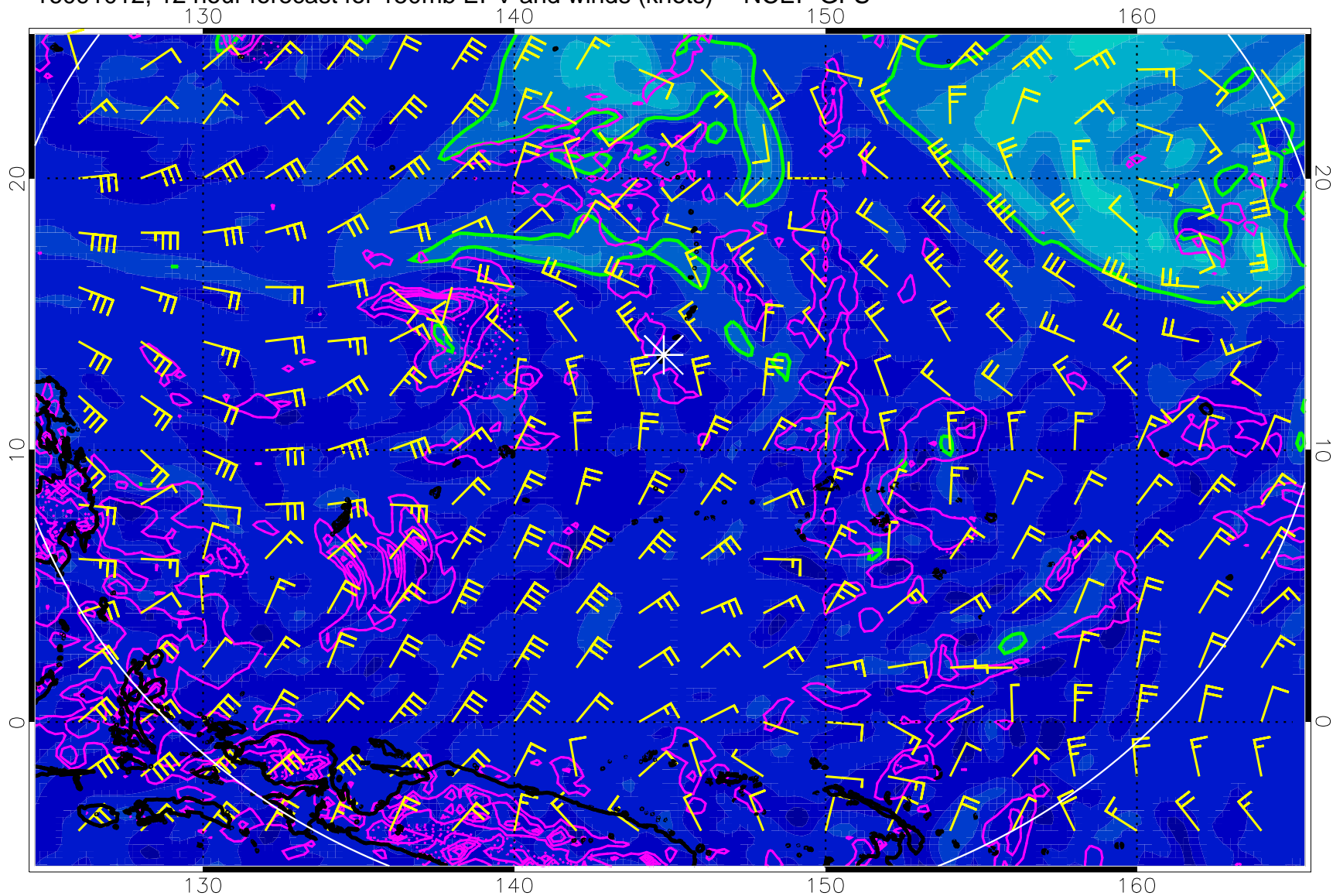
16091012, 12 hour forecast for 150mb EPV and winds (knots) -- NCEP GFS
