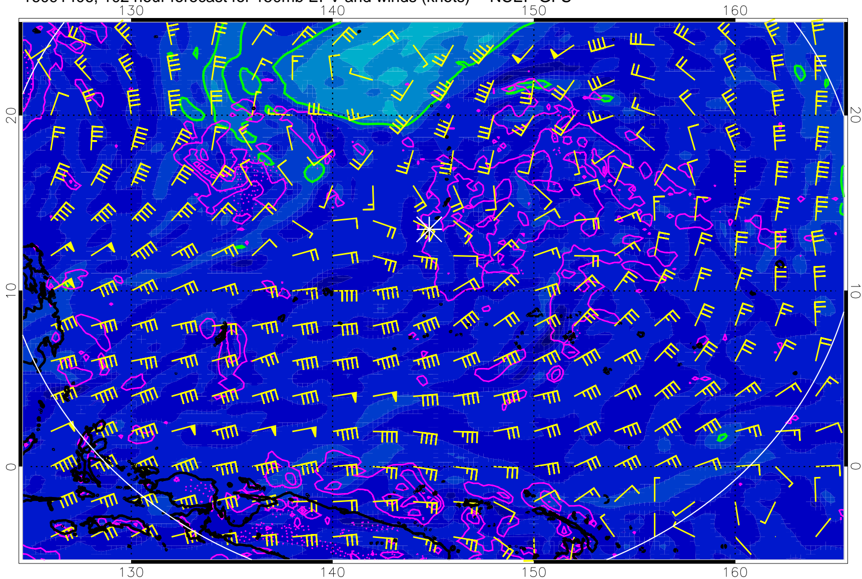
16091406, 102 hour forecast for 150mb EPV and winds (knots) -- NCEP GFS
