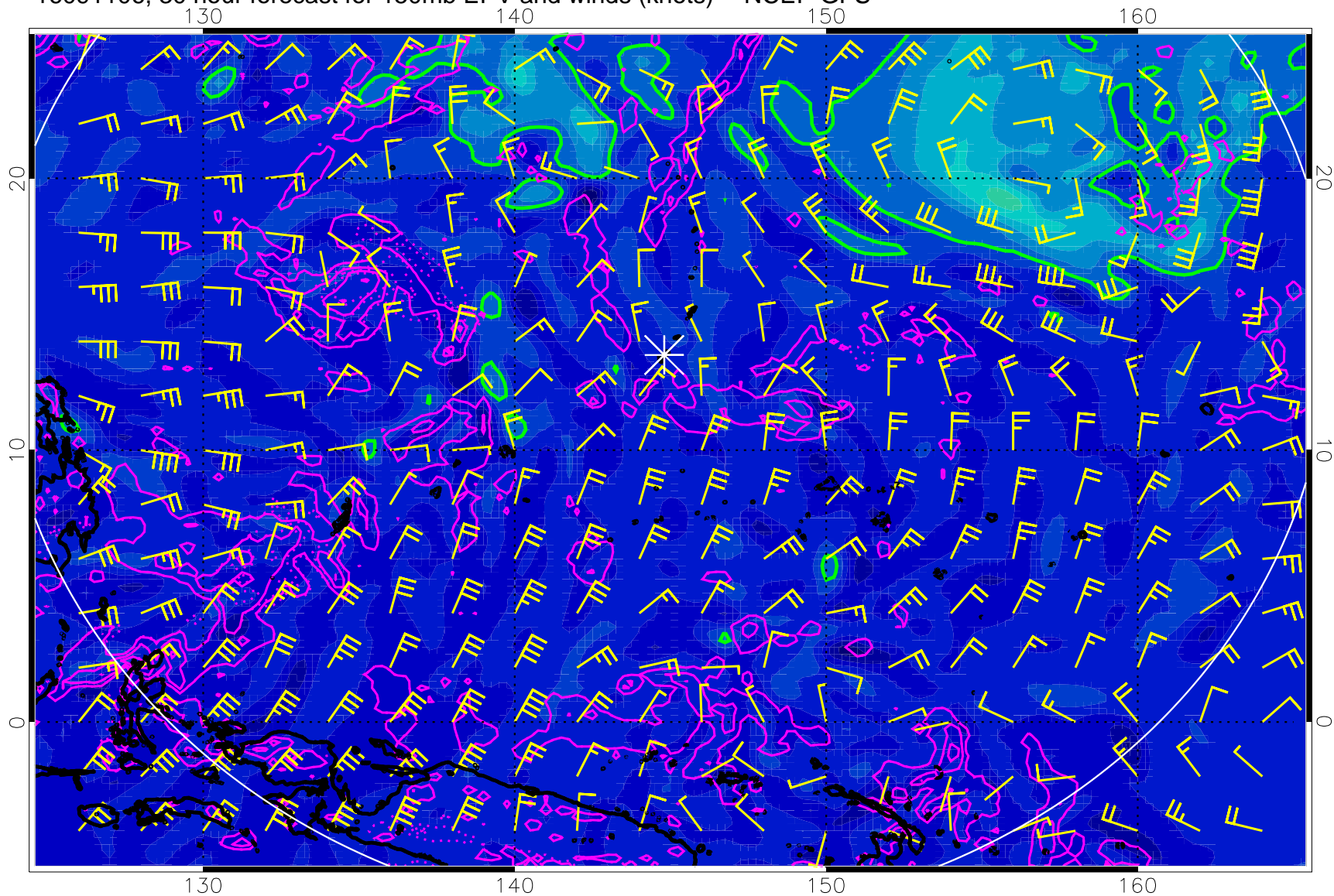
16091106, 30 hour forecast for 150mb EPV and winds (knots) -- NCEP GFS
