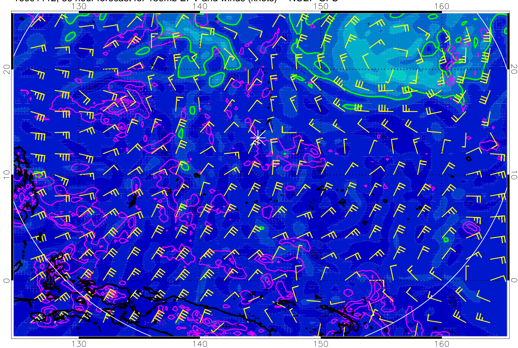
16091112, 36 hour forecast for 150mb EPV and winds (knots) -- NCEP GFS
