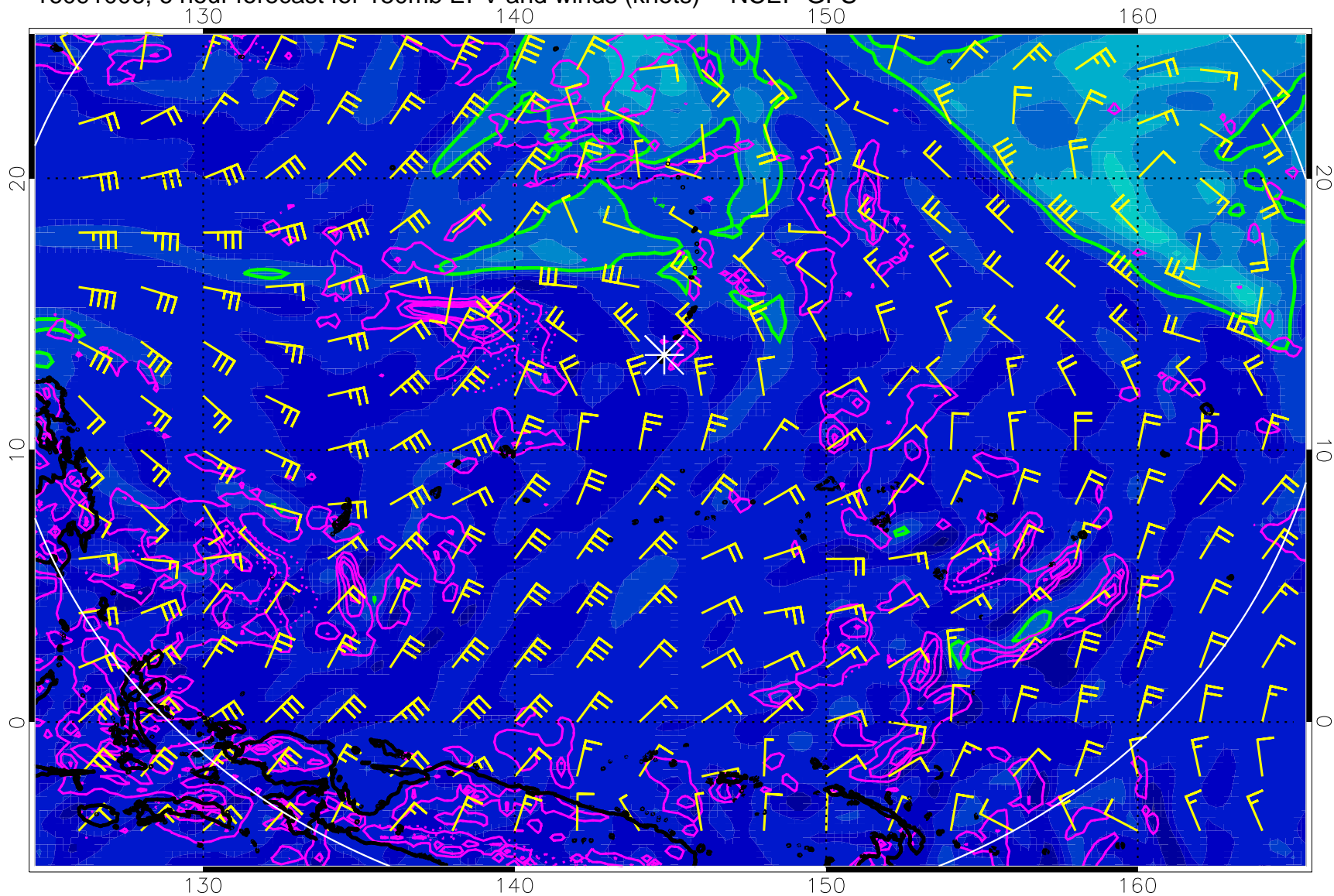
16091006, 6 hour forecast for 150mb EPV and winds (knots) -- NCEP GFS
