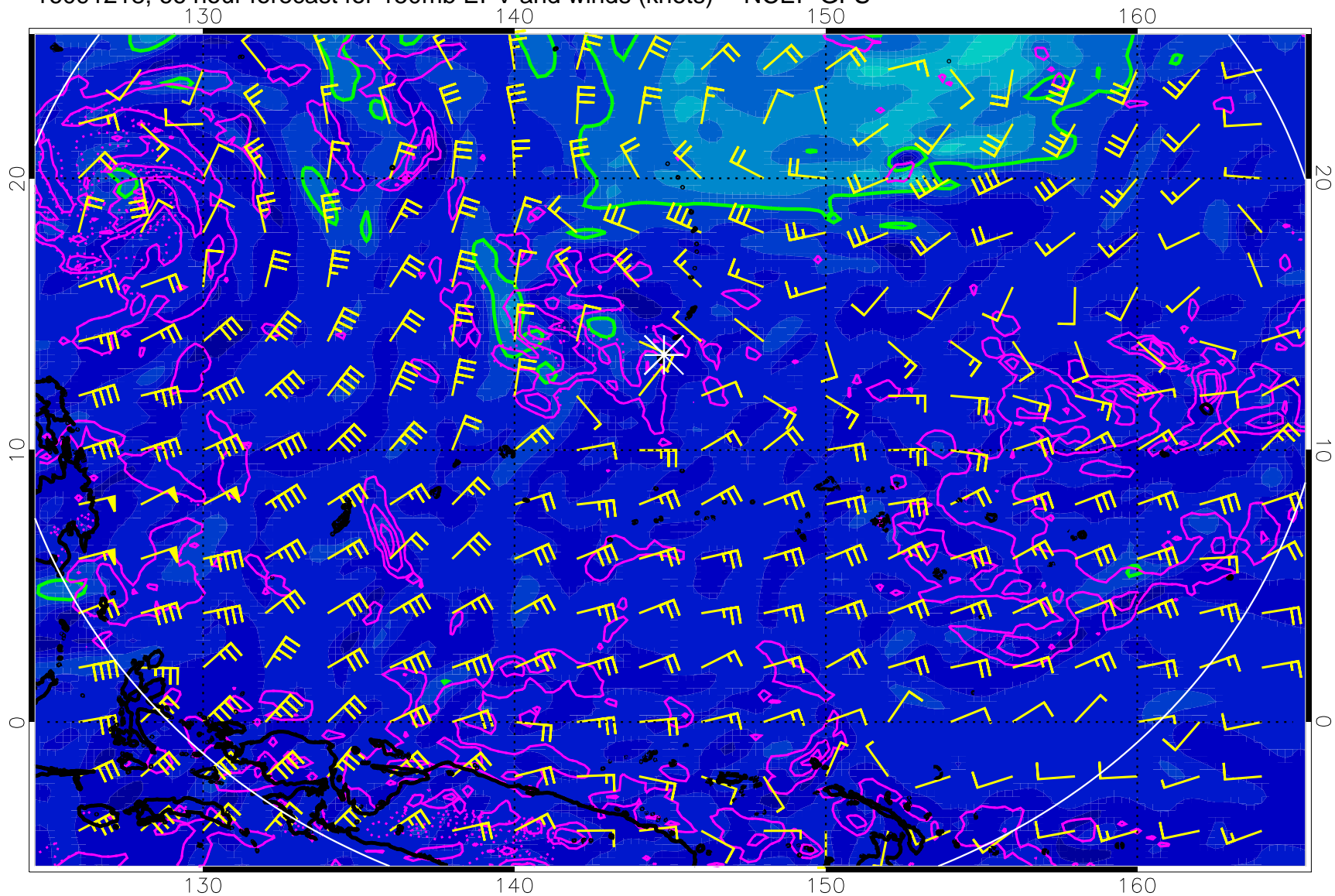
16091218, 66 hour forecast for 150mb EPV and winds (knots) -- NCEP GFS
