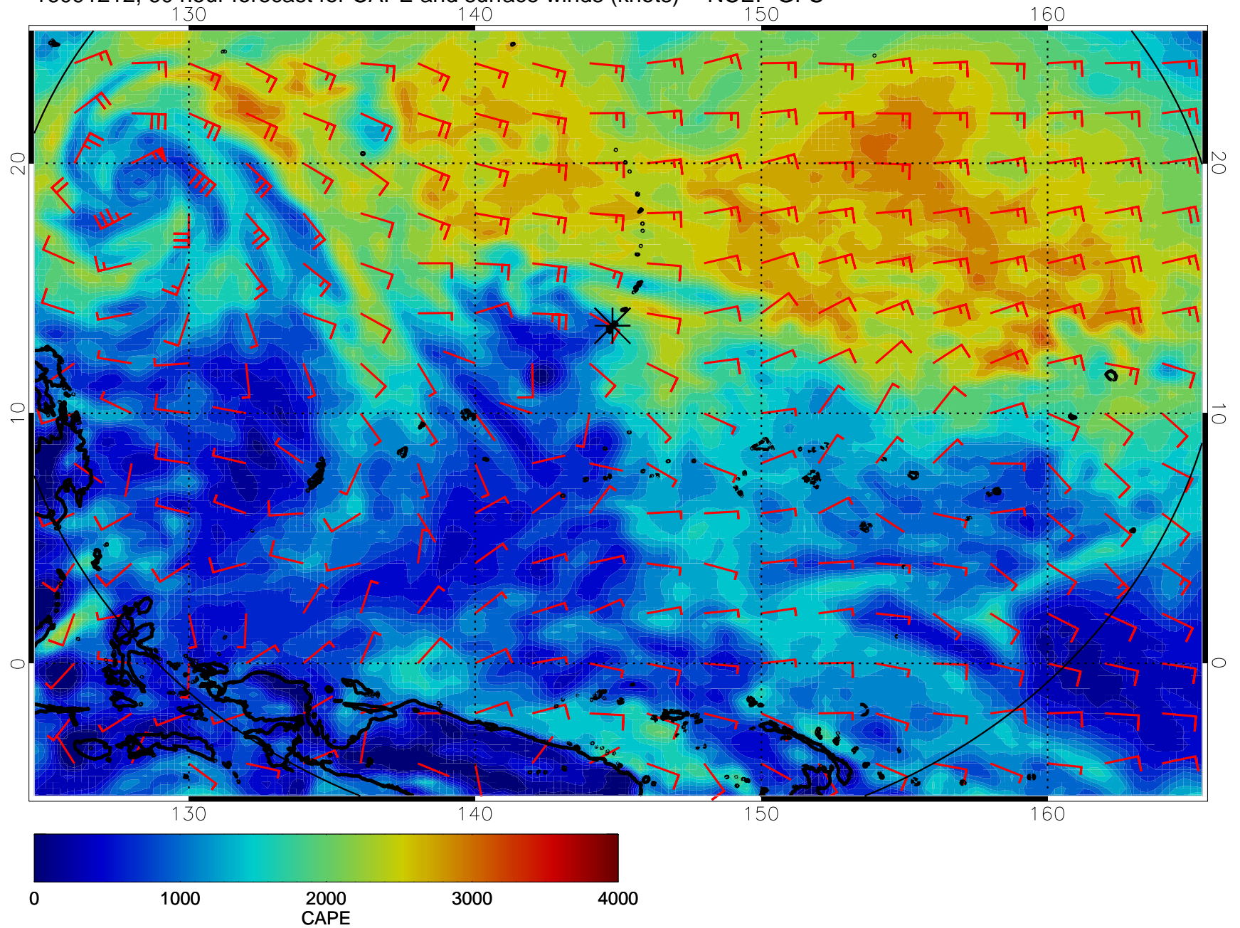
16091212, 60 hour forecast for CAPE and surface winds (knots) -- NCEP GFS
