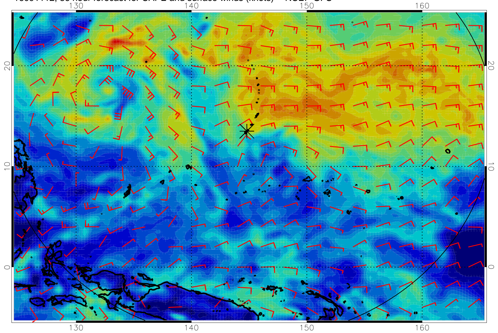
16091112, 36 hour forecast for CAPE and surface winds (knots) -- NCEP GFS
