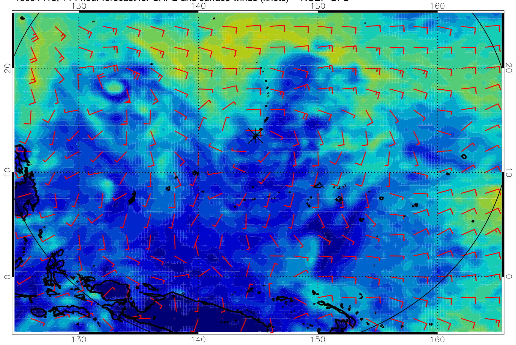
16091418, 114 hour forecast for CAPE and surface winds (knots) -- NCEP GFS
