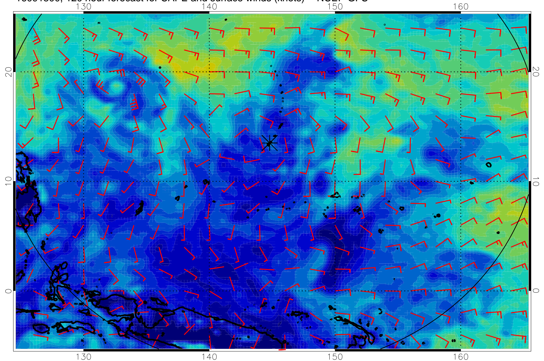
16091500, 120 hour forecast for CAPE and surface winds (knots) -- NCEP GFS
