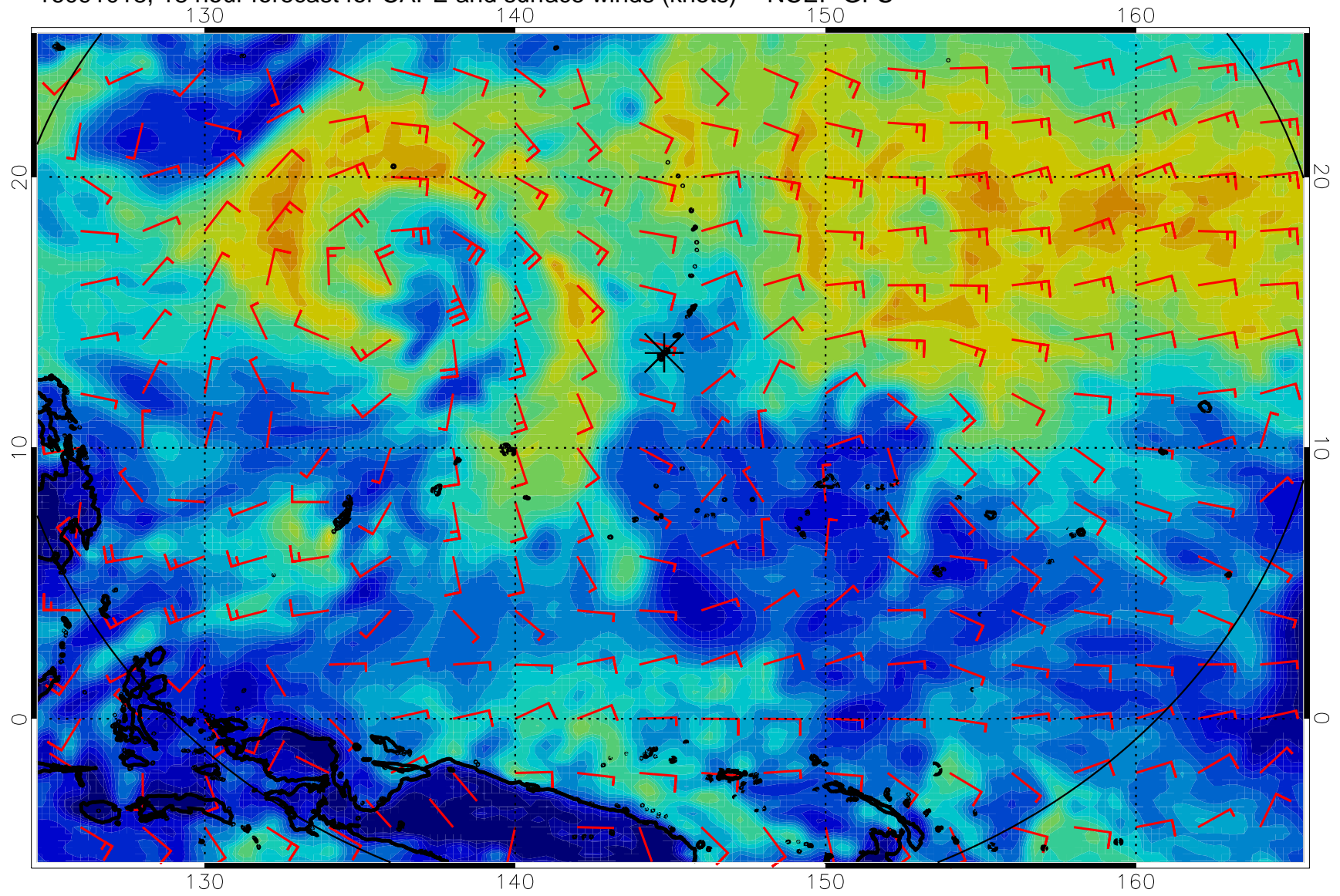
16091018, 18 hour forecast for CAPE and surface winds (knots) -- NCEP GFS
