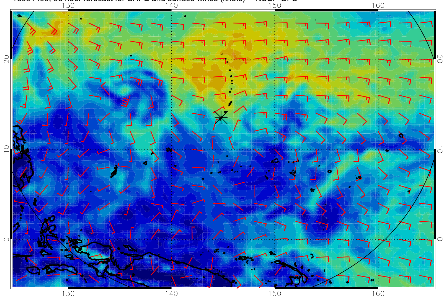
16091400, 96 hour forecast for CAPE and surface winds (knots) -- NCEP GFS
