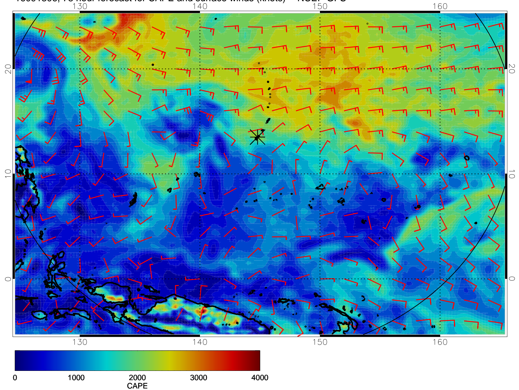
16091306, 78 hour forecast for CAPE and surface winds (knots) -- NCEP GFS
