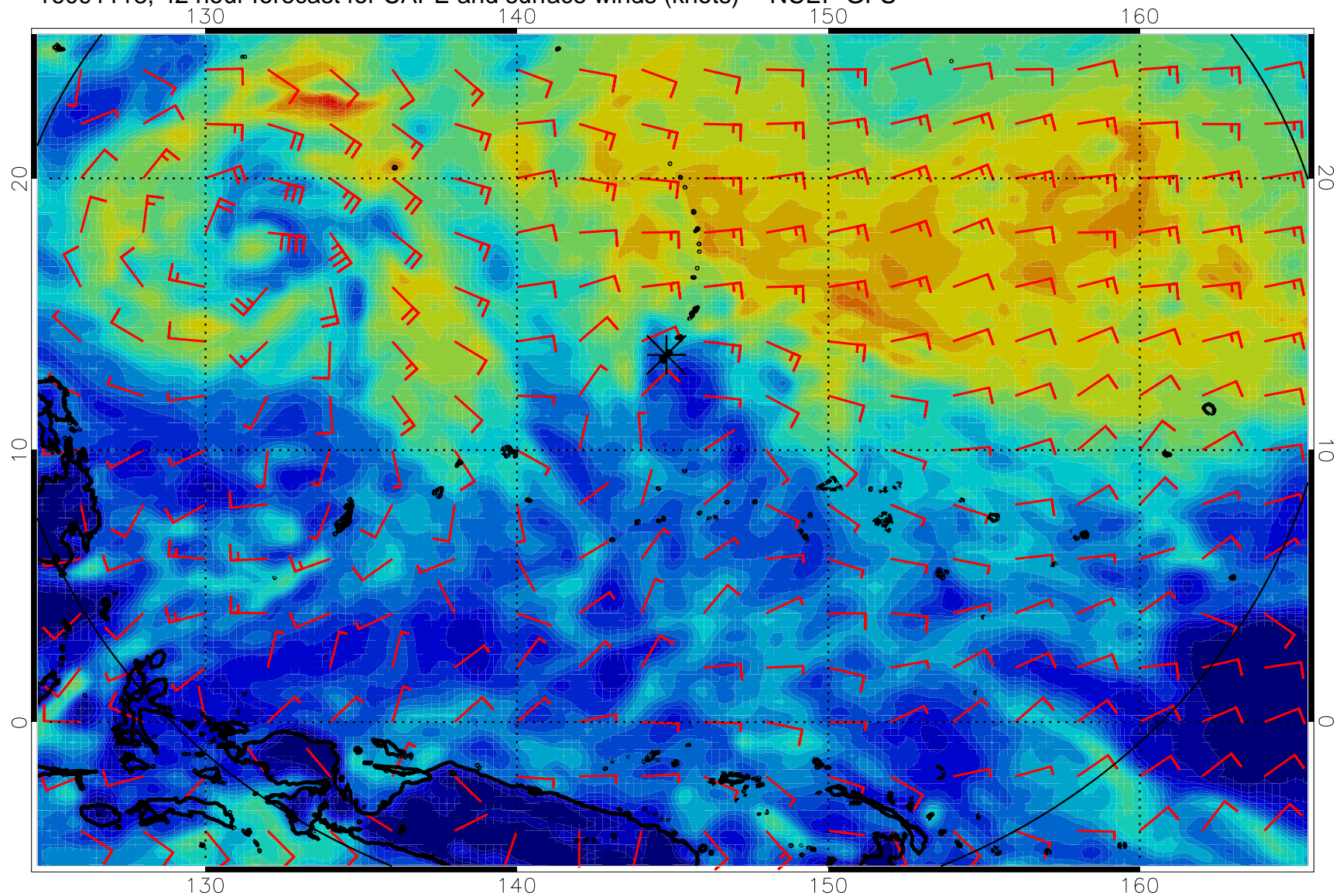
16091118, 42 hour forecast for CAPE and surface winds (knots) -- NCEP GFS
