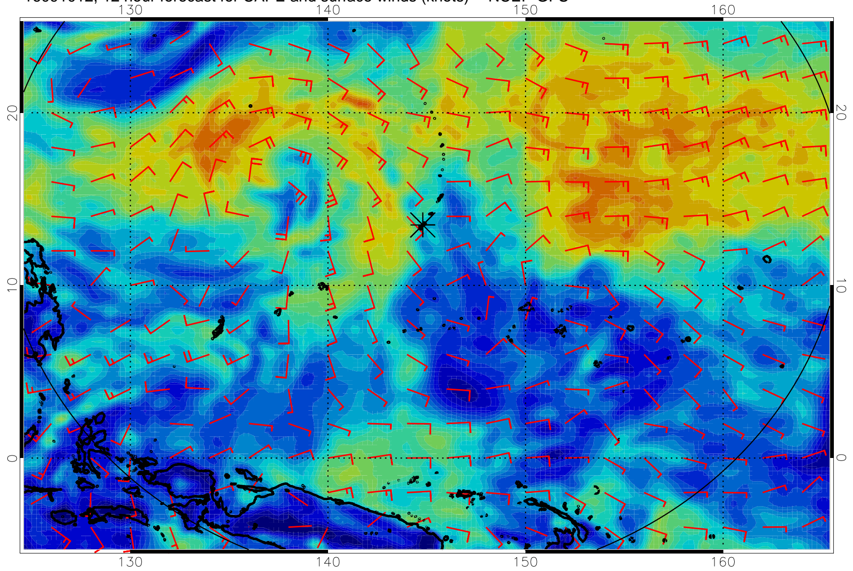
16091012, 12 hour forecast for CAPE and surface winds (knots) -- NCEP GFS
