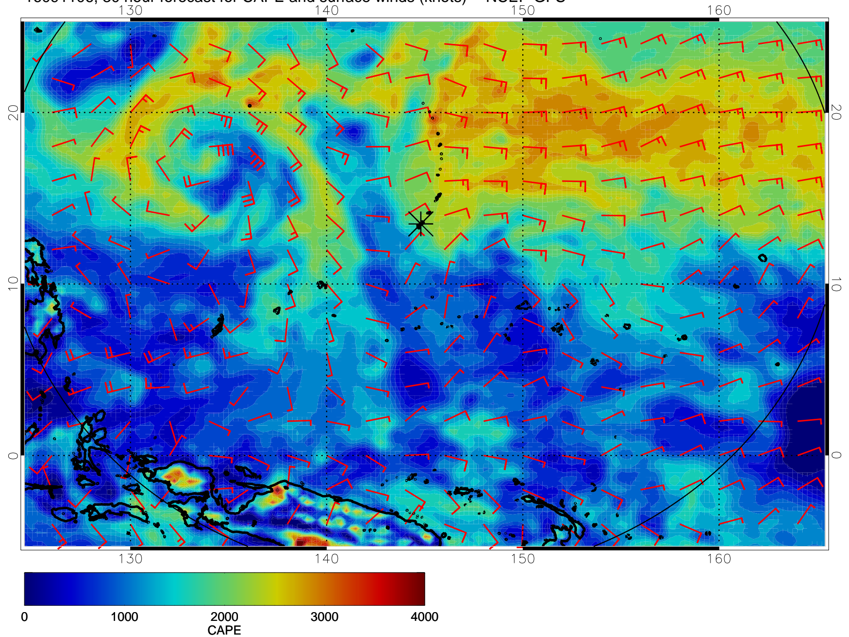
16091106, 30 hour forecast for CAPE and surface winds (knots) -- NCEP GFS
