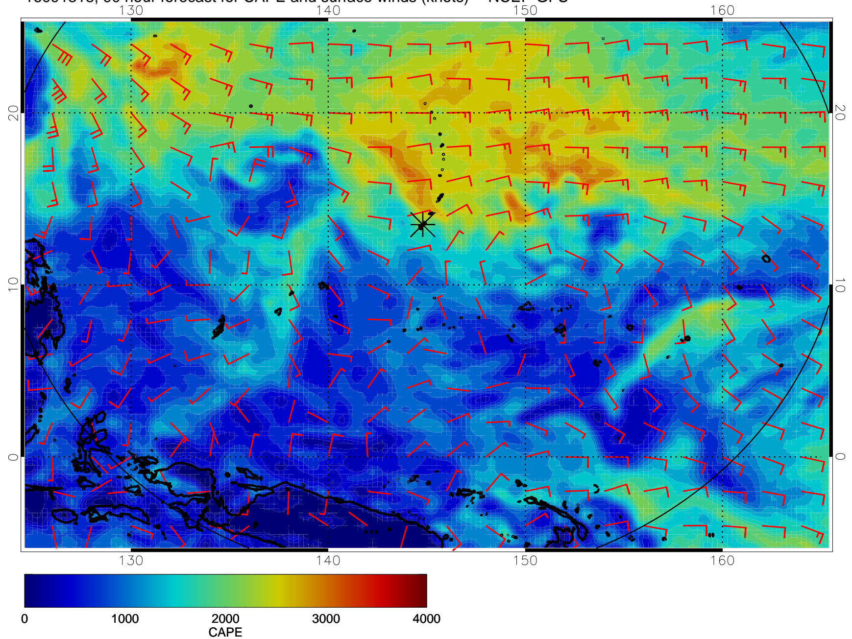
16091318, 90 hour forecast for CAPE and surface winds (knots) -- NCEP GFS
