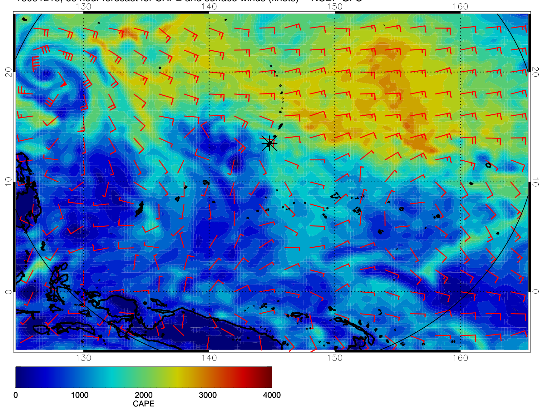
16091218, 66 hour forecast for CAPE and surface winds (knots) -- NCEP GFS
