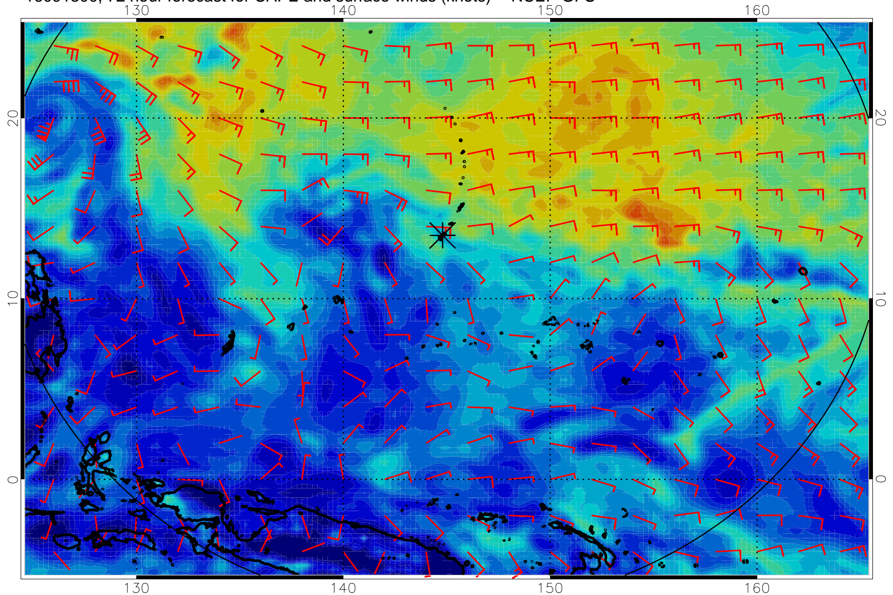
16091300, 72 hour forecast for CAPE and surface winds (knots) -- NCEP GFS
