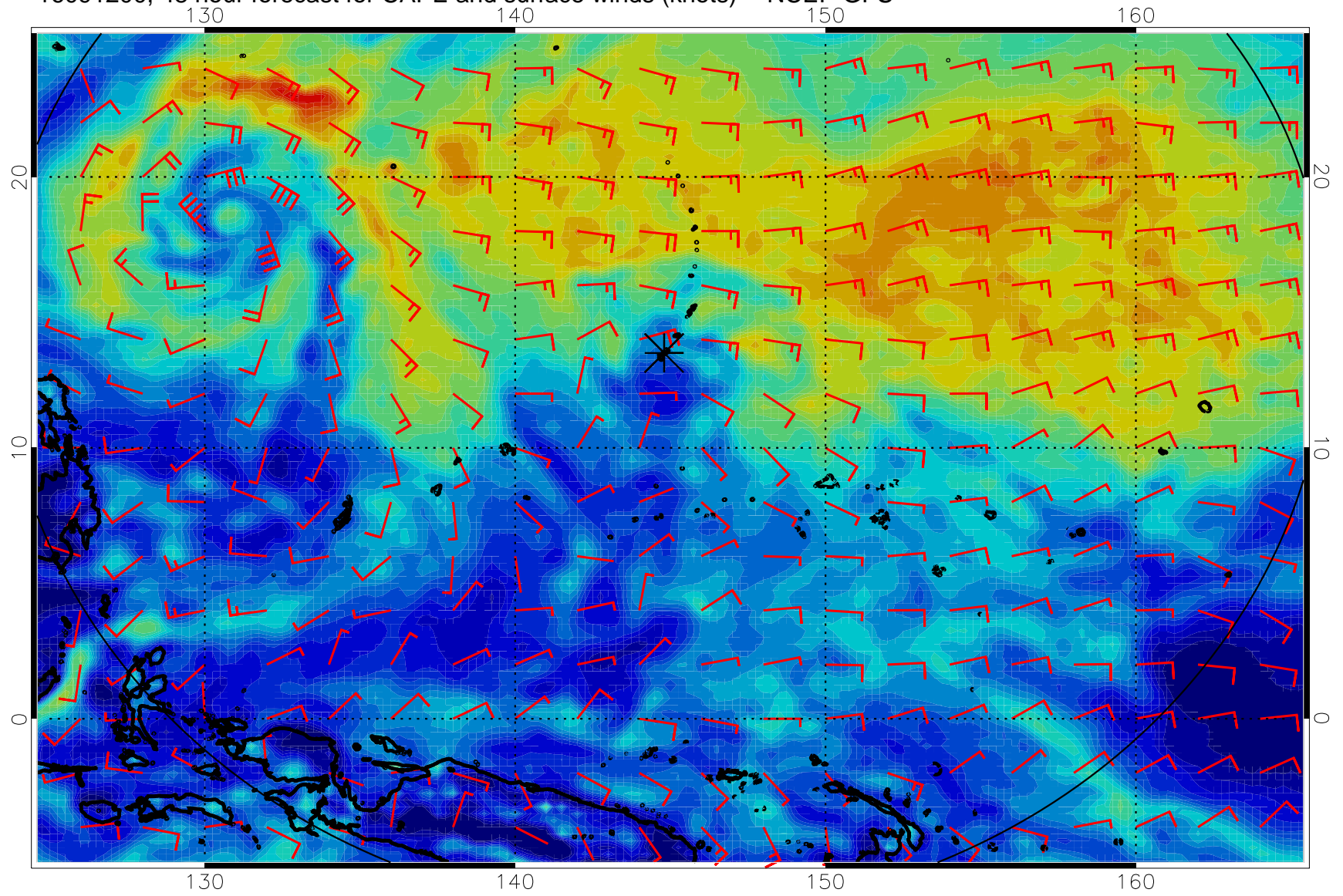
16091200, 48 hour forecast for CAPE and surface winds (knots) -- NCEP GFS
