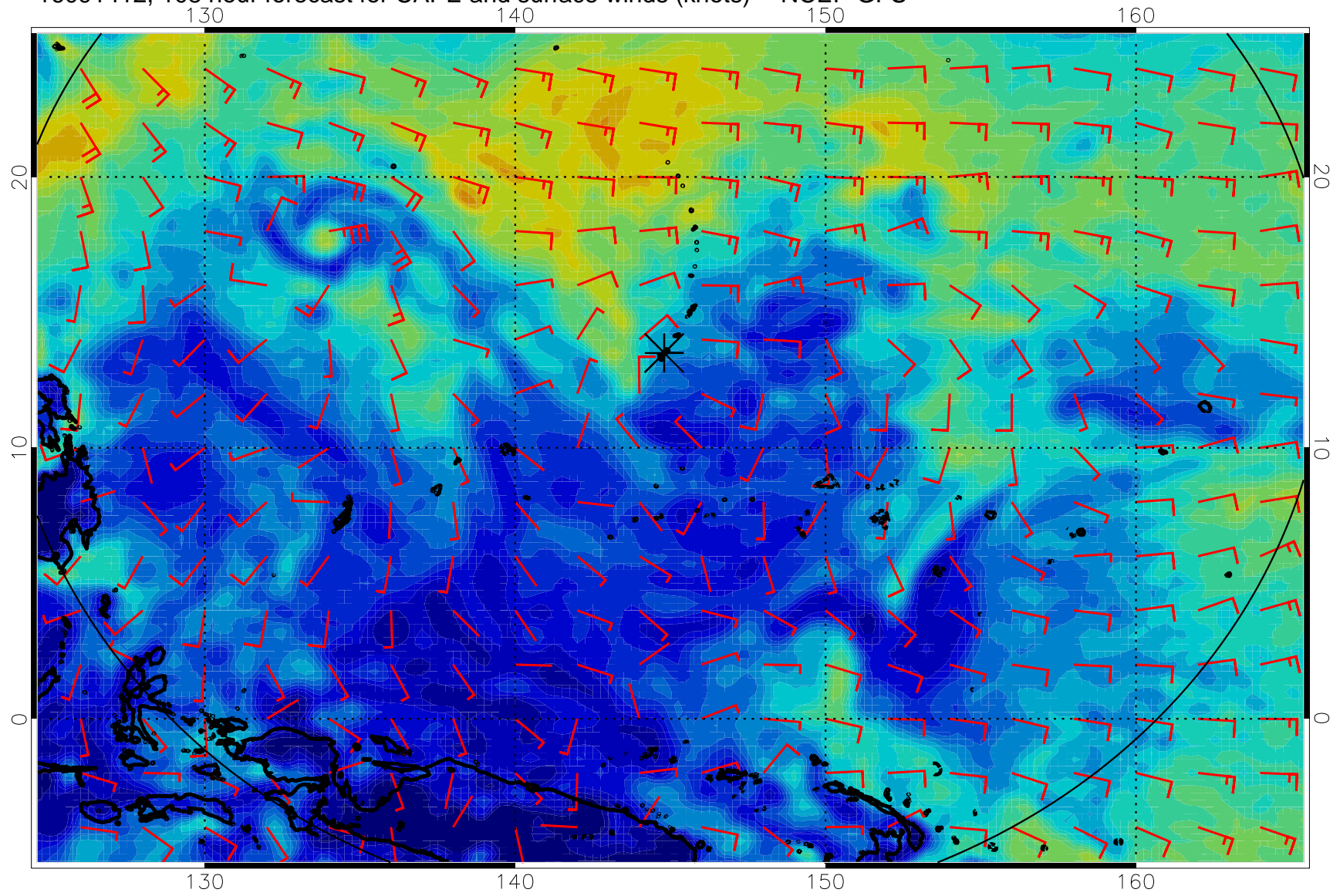
16091412, 108 hour forecast for CAPE and surface winds (knots) -- NCEP GFS
