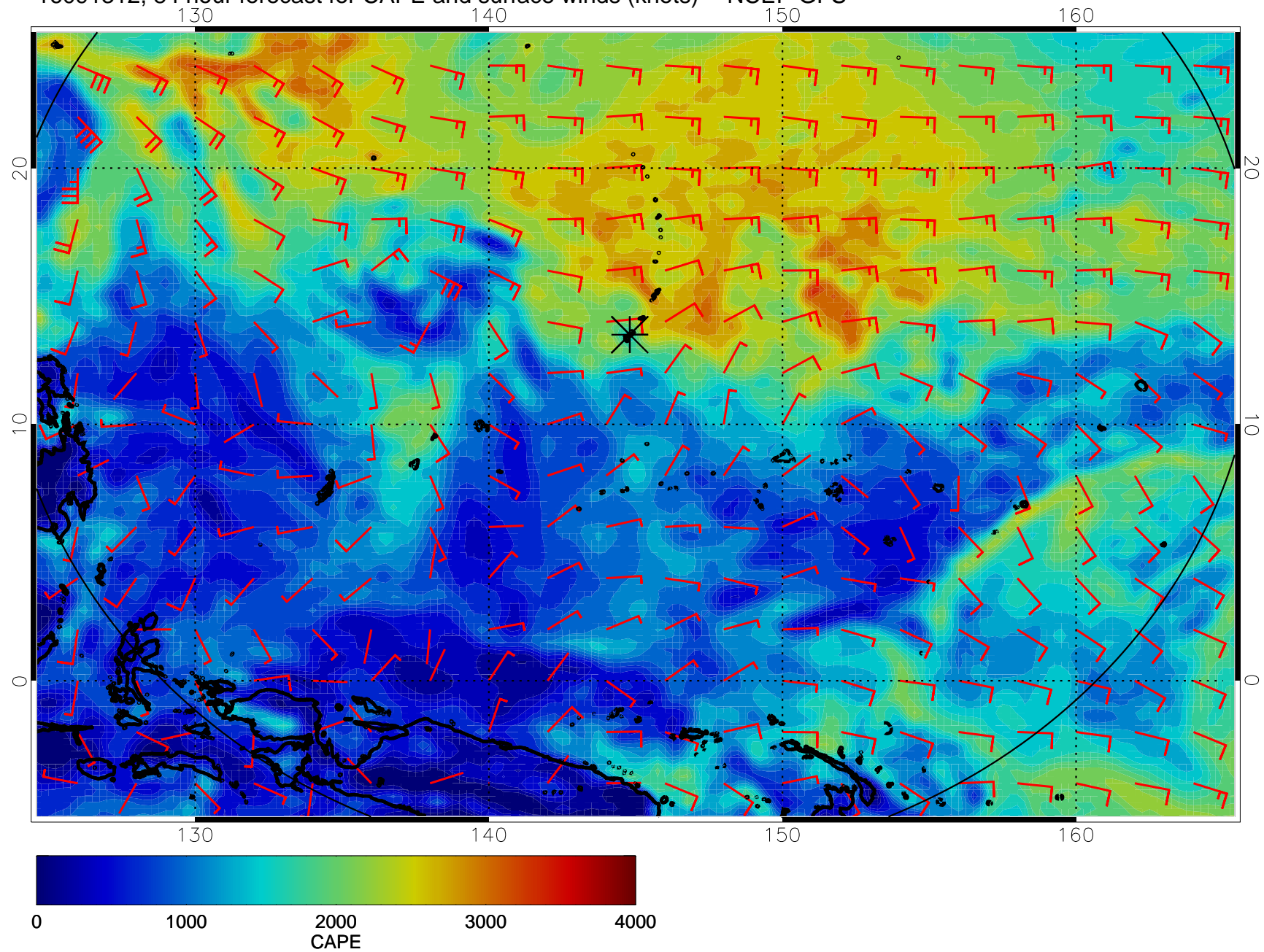
16091312, 84 hour forecast for CAPE and surface winds (knots) -- NCEP GFS
