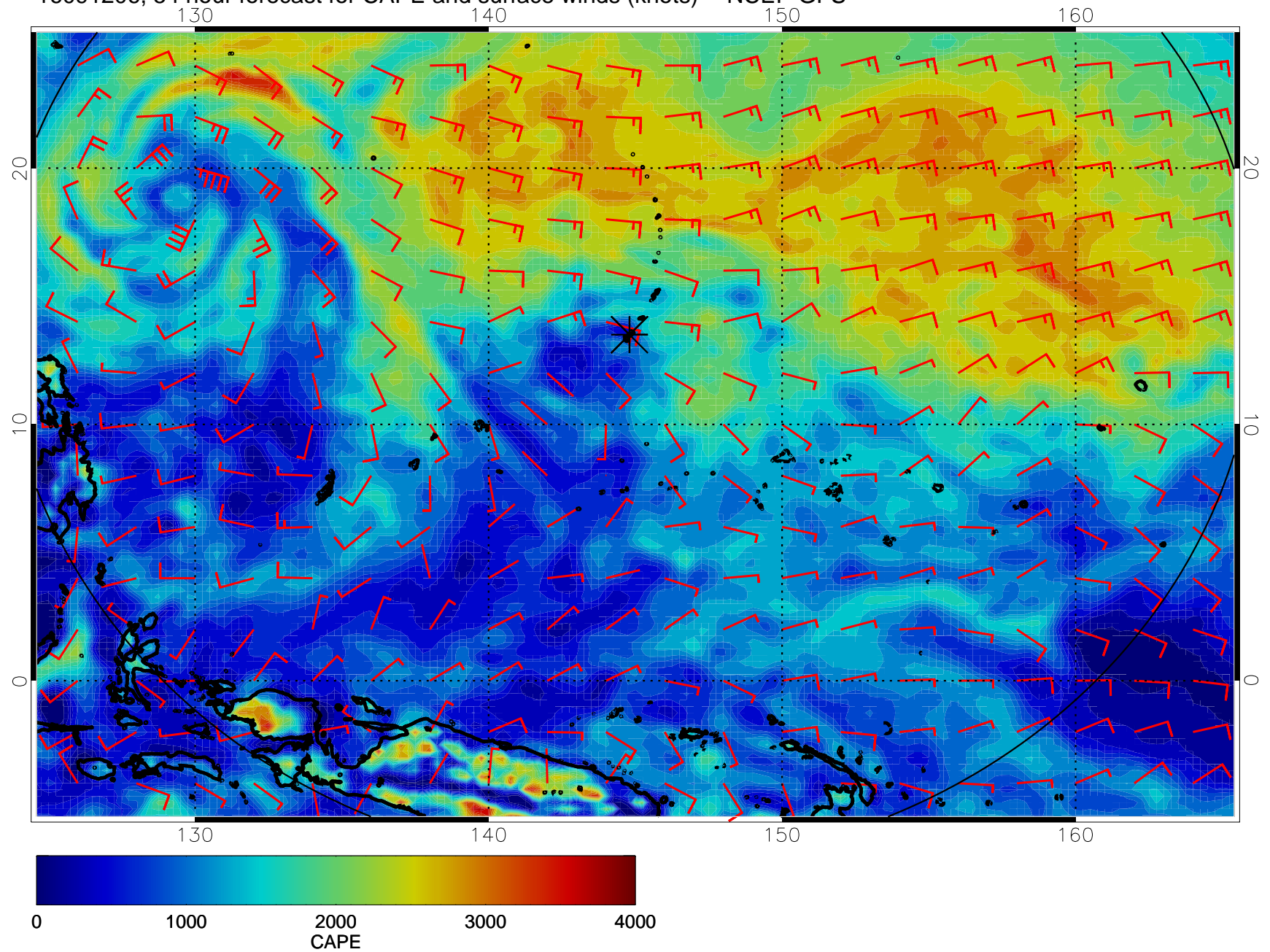
16091206, 54 hour forecast for CAPE and surface winds (knots) -- NCEP GFS
