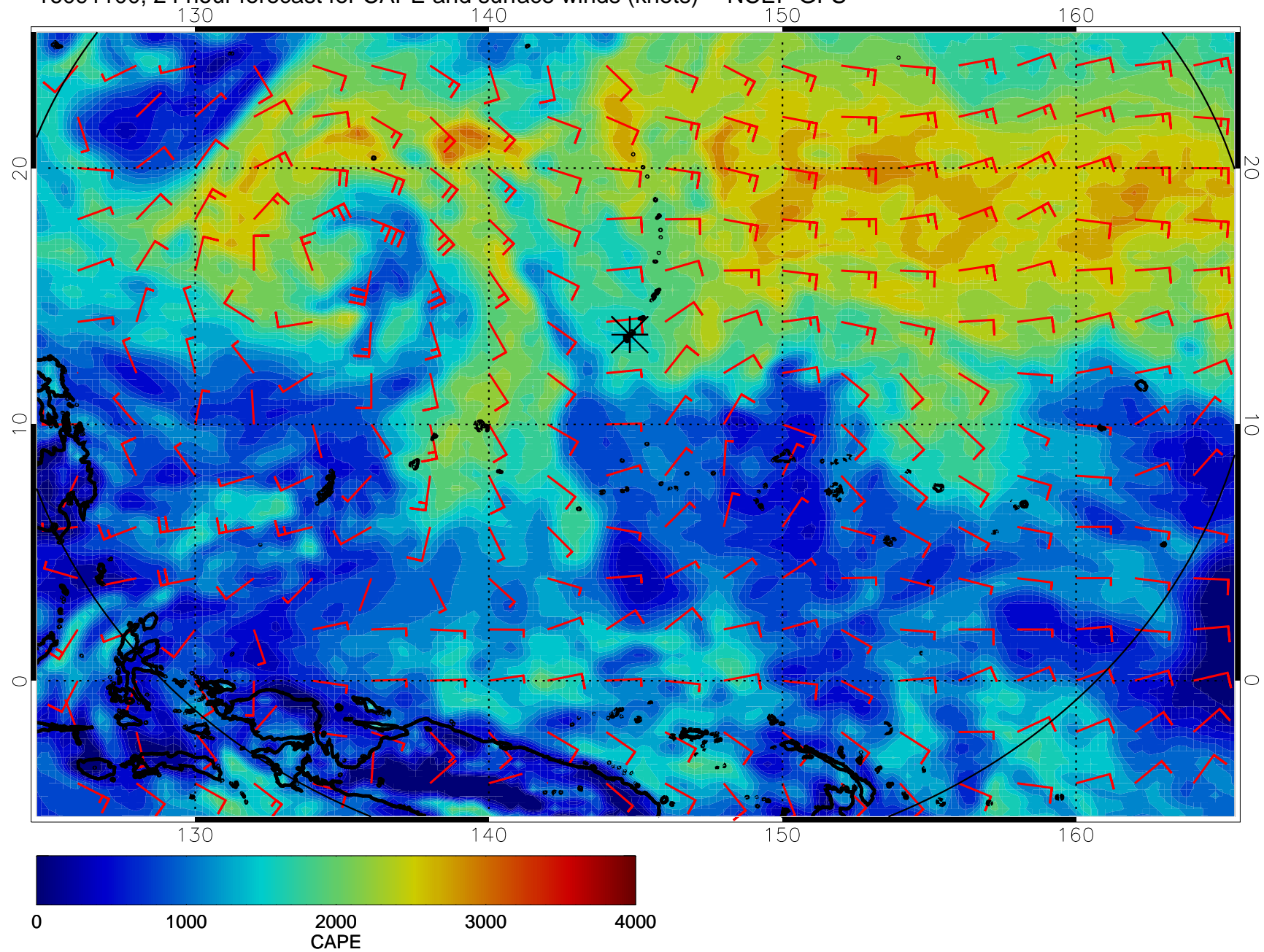
16091100, 24 hour forecast for CAPE and surface winds (knots) -- NCEP GFS
