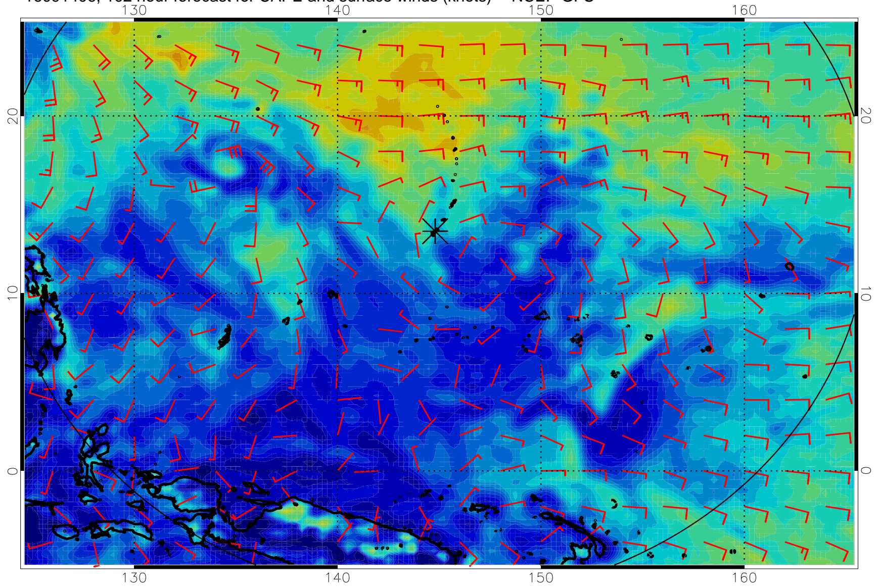
16091406, 102 hour forecast for CAPE and surface winds (knots) -- NCEP GFS
