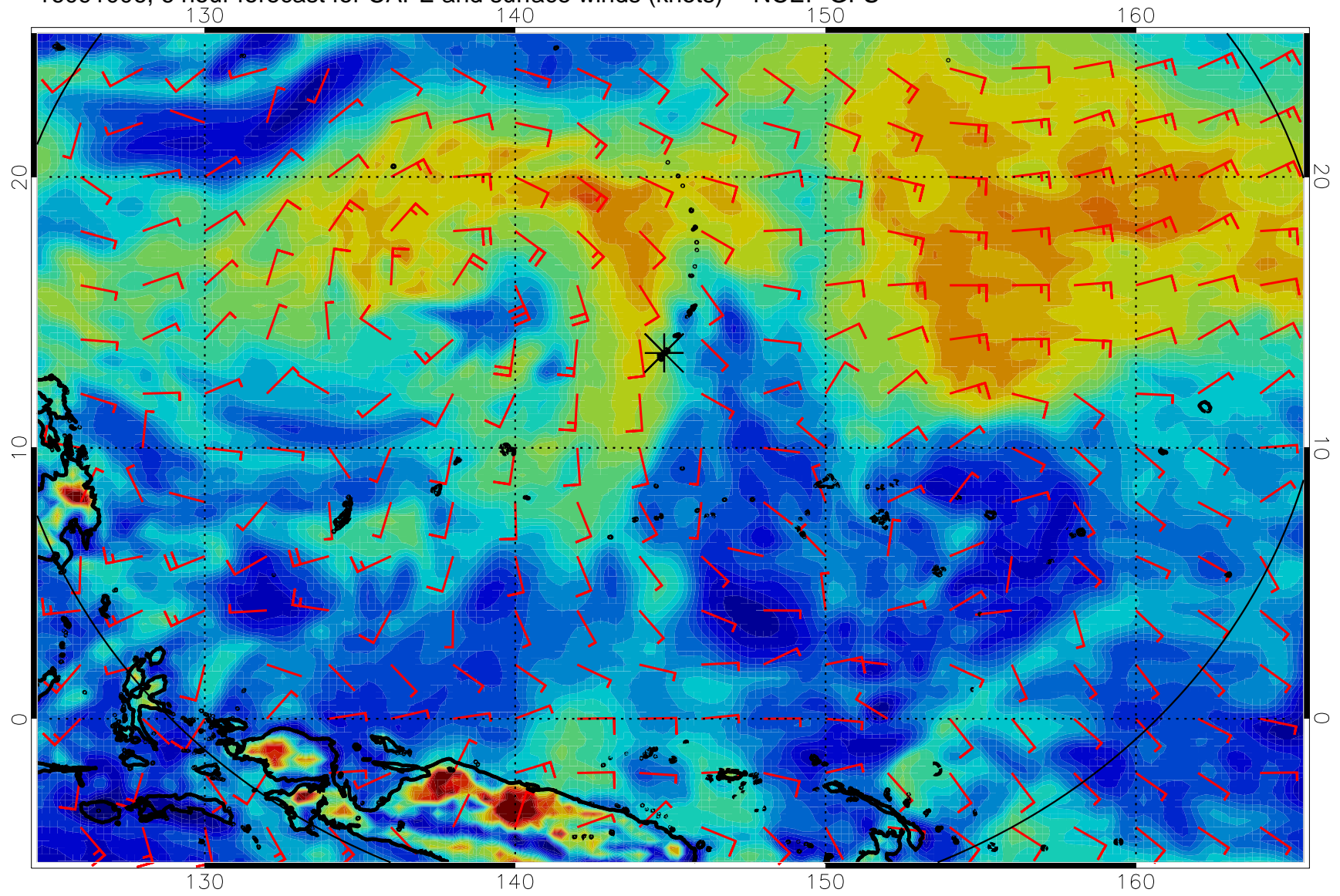
16091006, 6 hour forecast for CAPE and surface winds (knots) -- NCEP GFS
