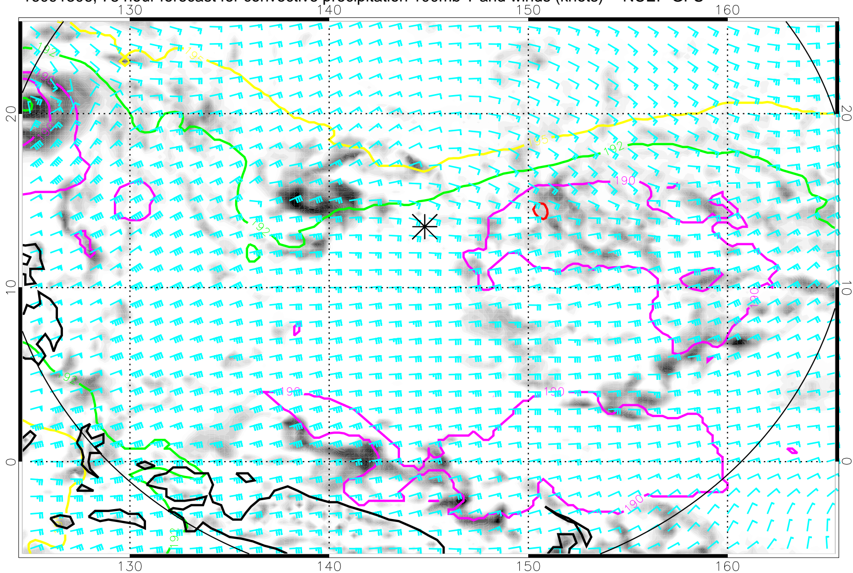
16091306, 78 hour forecast for convective precipitation 100mb T and winds (knots) -- NCEP GFS
