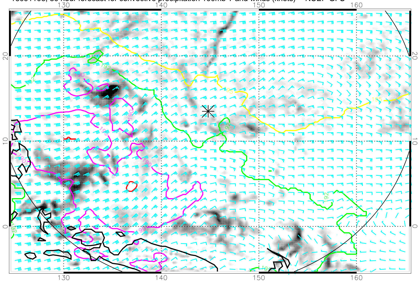
16091106, 30 hour forecast for convective precipitation 100mb T and winds (knots) -- NCEP GFS
