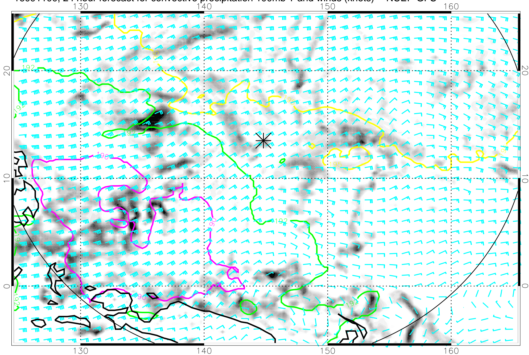
16091100, 24 hour forecast for convective precipitation 100mb T and winds (knots) -- NCEP GFS
