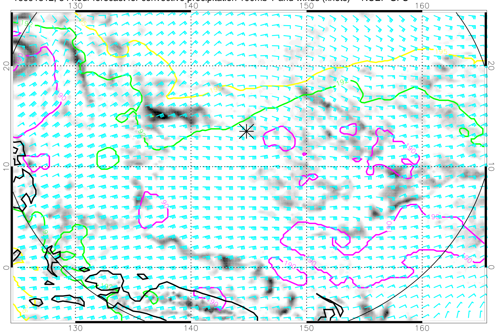
16091312, 84 hour forecast for convective precipitation 100mb T and winds (knots) -- NCEP GFS
