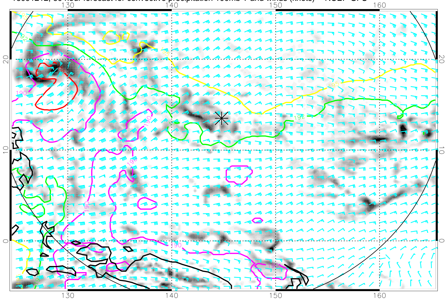
16091212, 60 hour forecast for convective precipitation 100mb T and winds (knots) -- NCEP GFS
