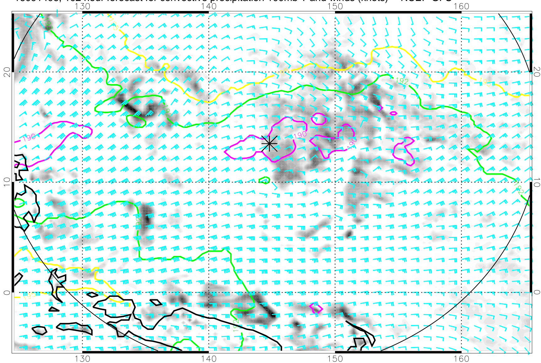
16091406, 102 hour forecast for convective precipitation 100mb T and winds (knots) -- NCEP GFS
