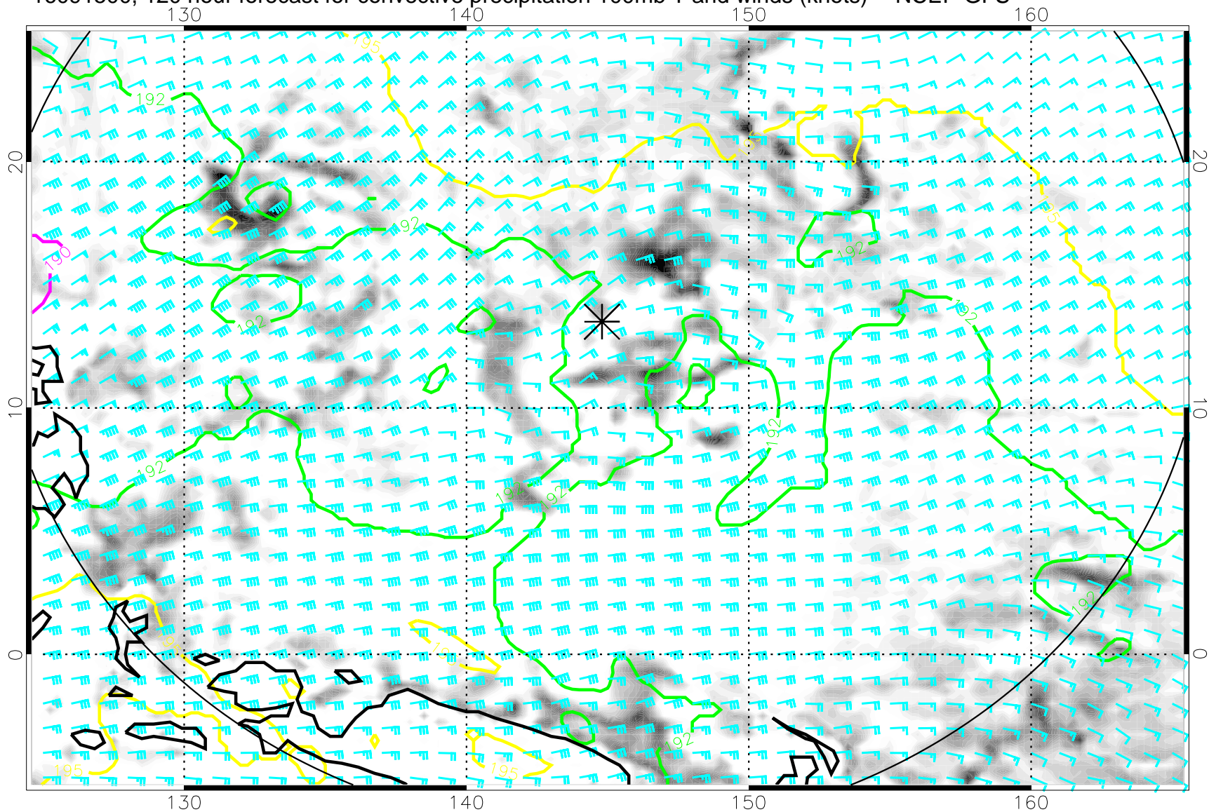
16091500, 120 hour forecast for convective precipitation 100mb T and winds (knots) -- NCEP GFS
