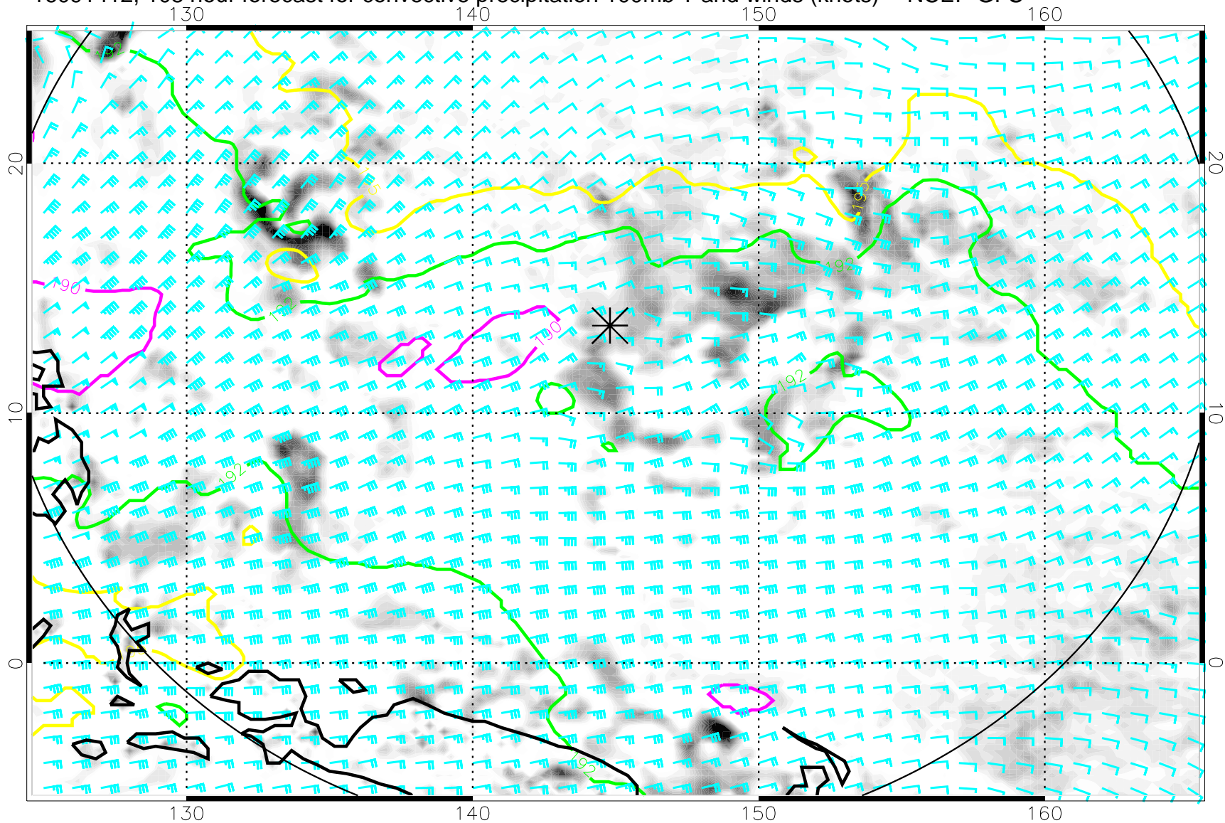
16091412, 108 hour forecast for convective precipitation 100mb T and winds (knots) -- NCEP GFS
