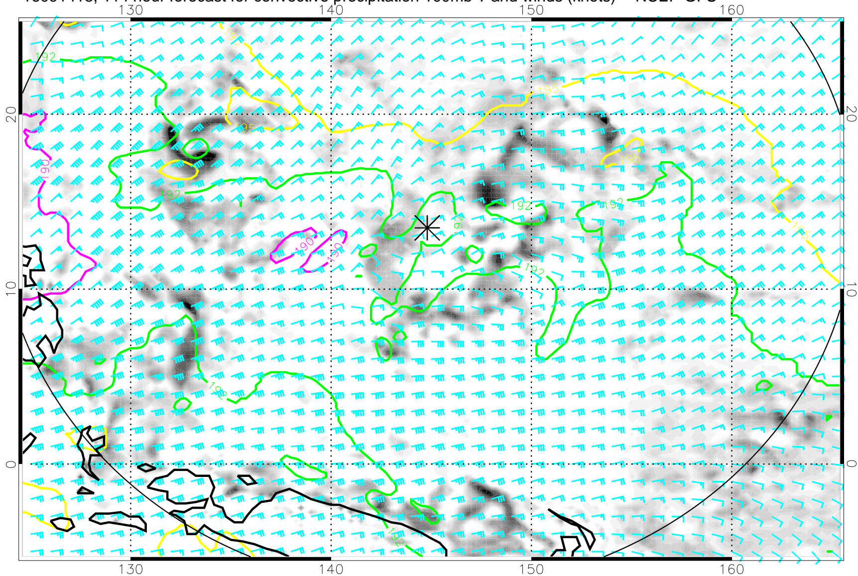
16091418, 114 hour forecast for convective precipitation 100mb T and winds (knots) -- NCEP GFS
