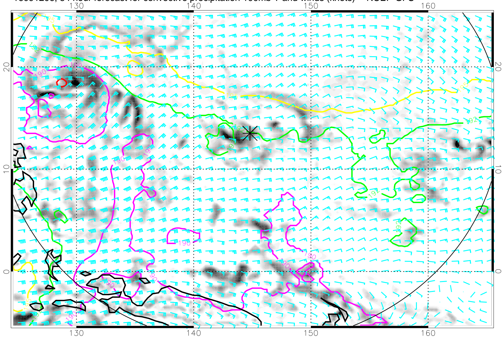
16091206, 54 hour forecast for convective precipitation 100mb T and winds (knots) -- NCEP GFS
