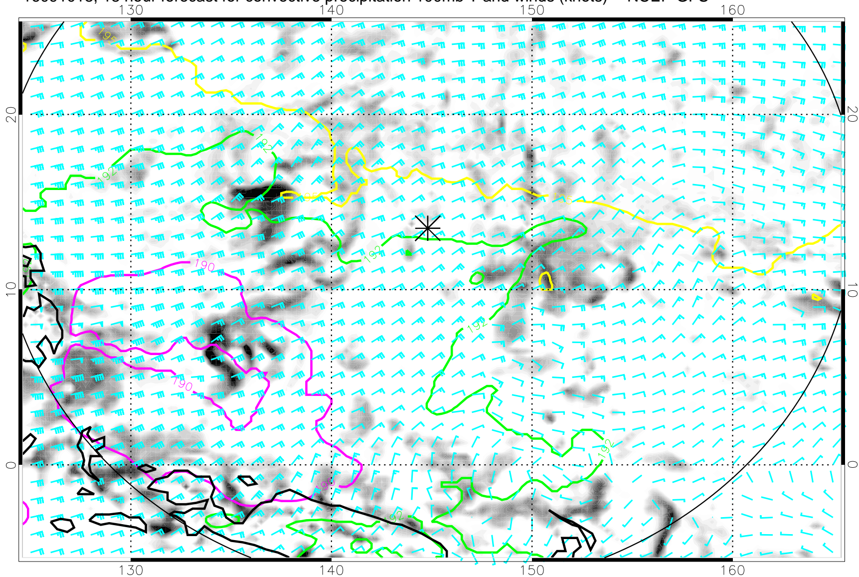
16091018, 18 hour forecast for convective precipitation 100mb T and winds (knots) -- NCEP GFS
