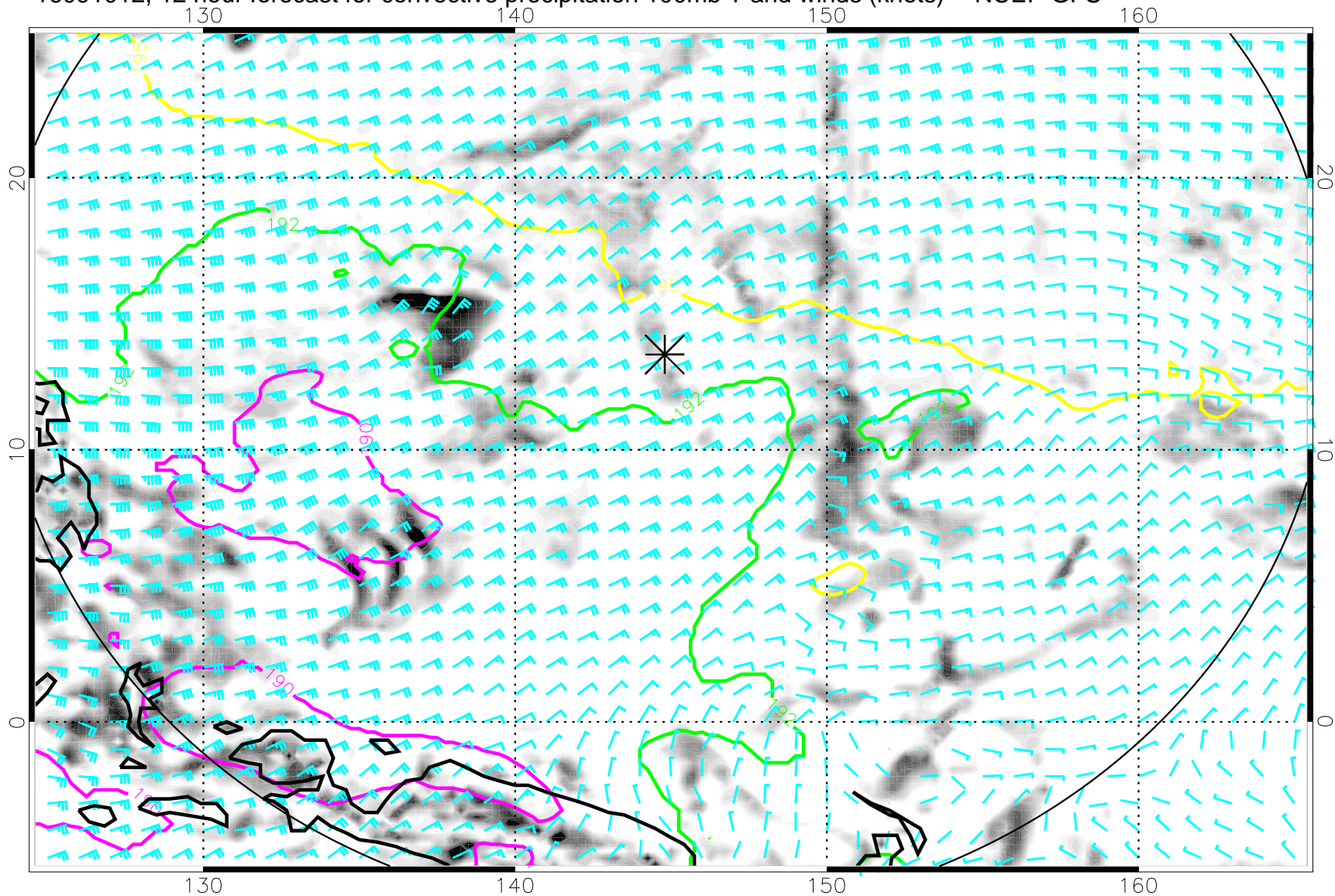
16091012, 12 hour forecast for convective precipitation 100mb T and winds (knots) -- NCEP GFS
