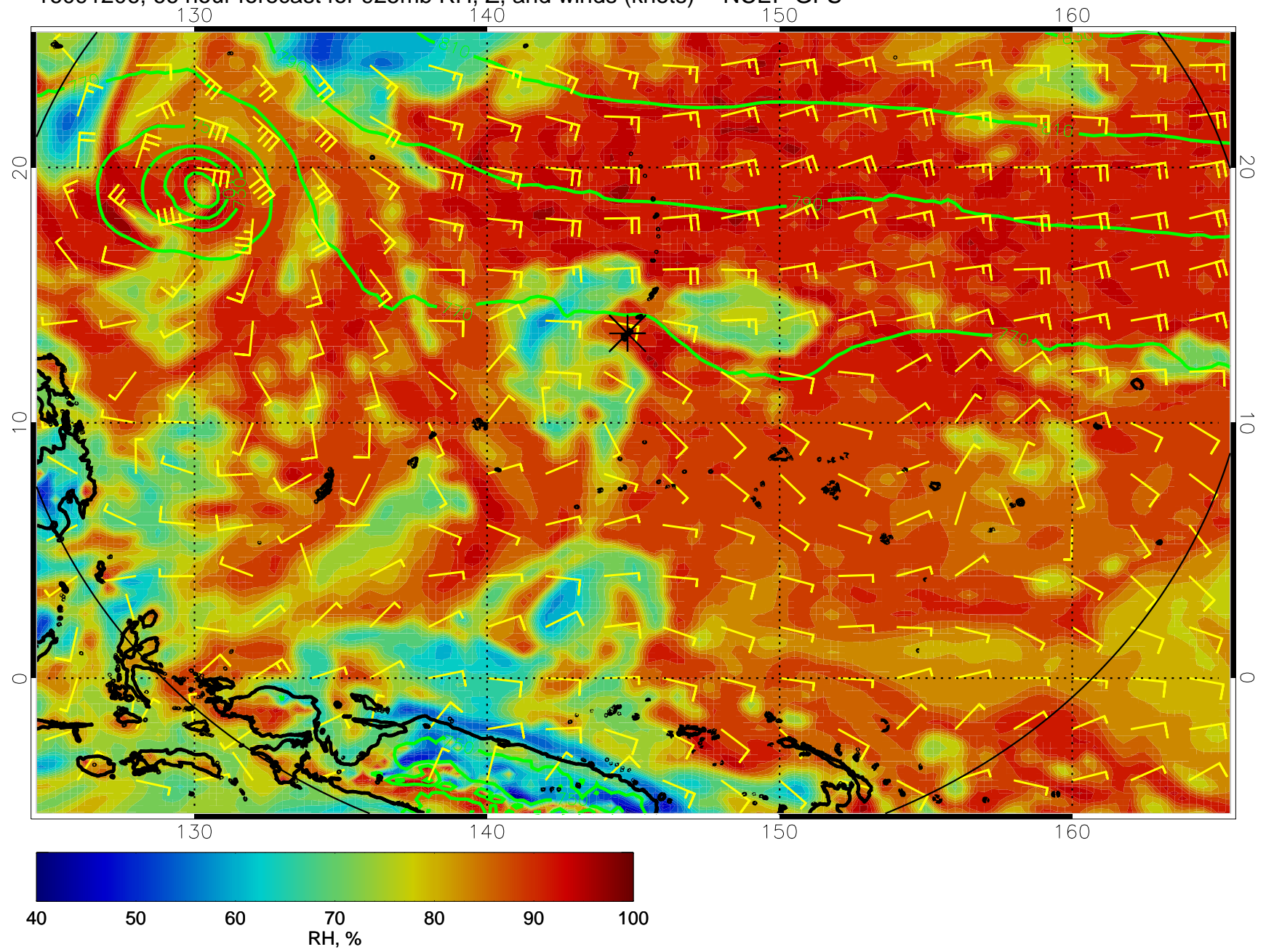
16091206, 66 hour forecast for 925mb RH, Z, and winds (knots) -- NCEP GFS
