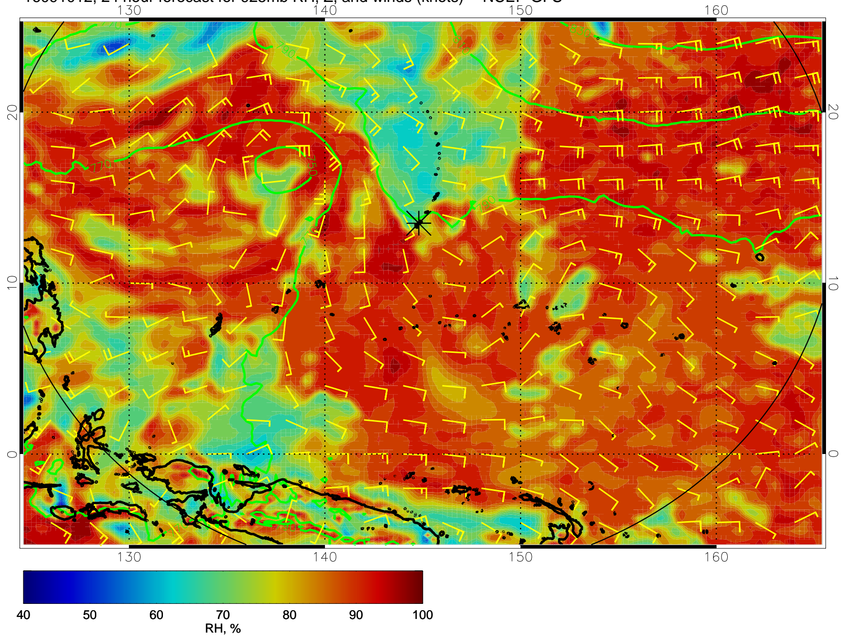
16091012, 24 hour forecast for 925mb RH, Z, and winds (knots) -- NCEP GFS
