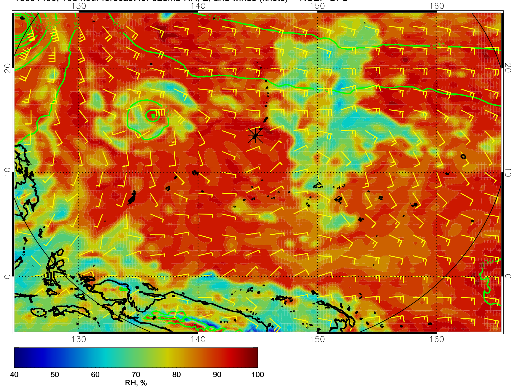
16091400, 108 hour forecast for 925mb RH, Z, and winds (knots) -- NCEP GFS
