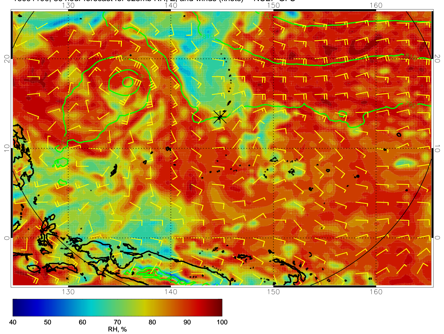
16091100, 36 hour forecast for 925mb RH, Z, and winds (knots) -- NCEP GFS
