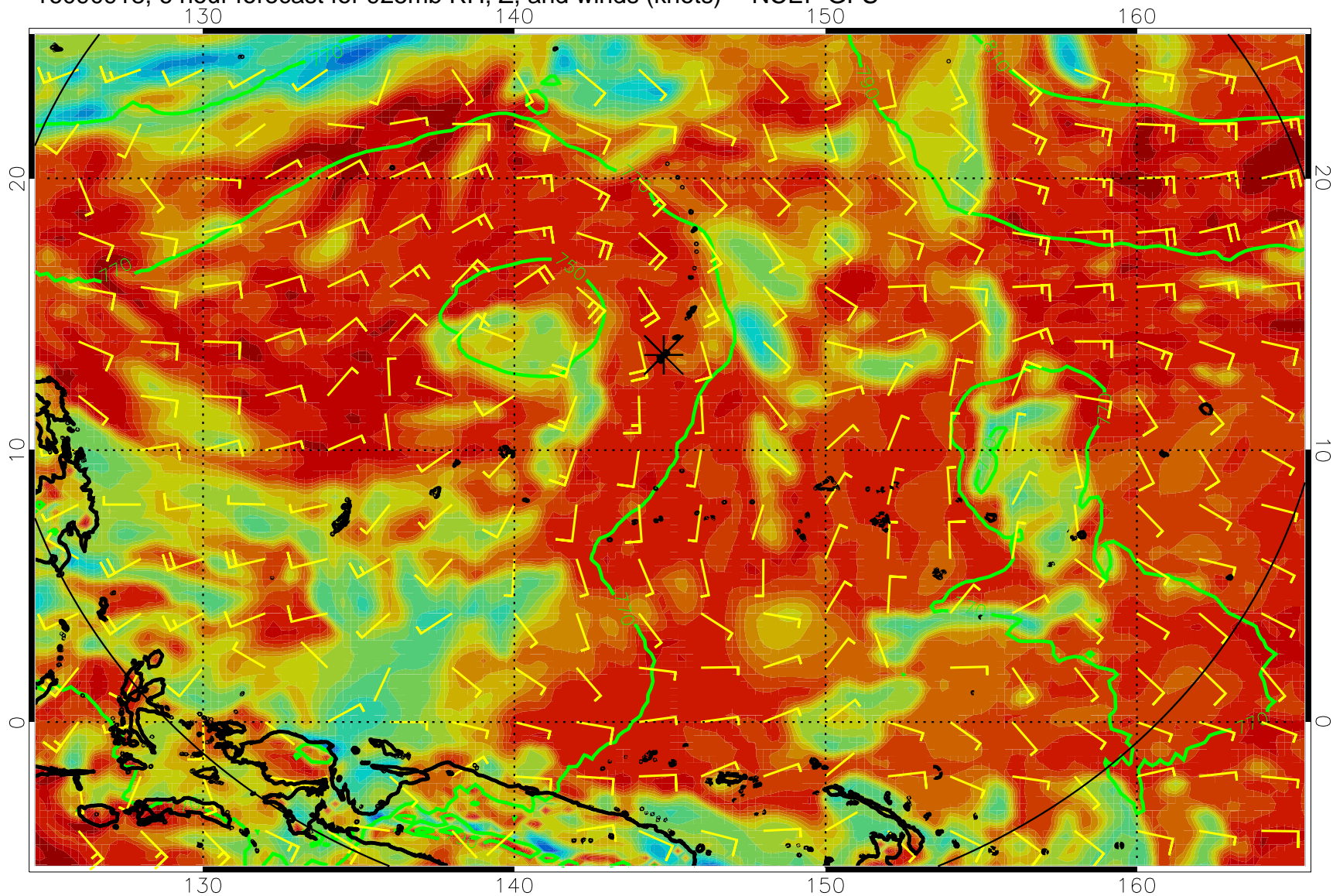
16090918, 6 hour forecast for 925mb RH, Z, and winds (knots) -- NCEP GFS
