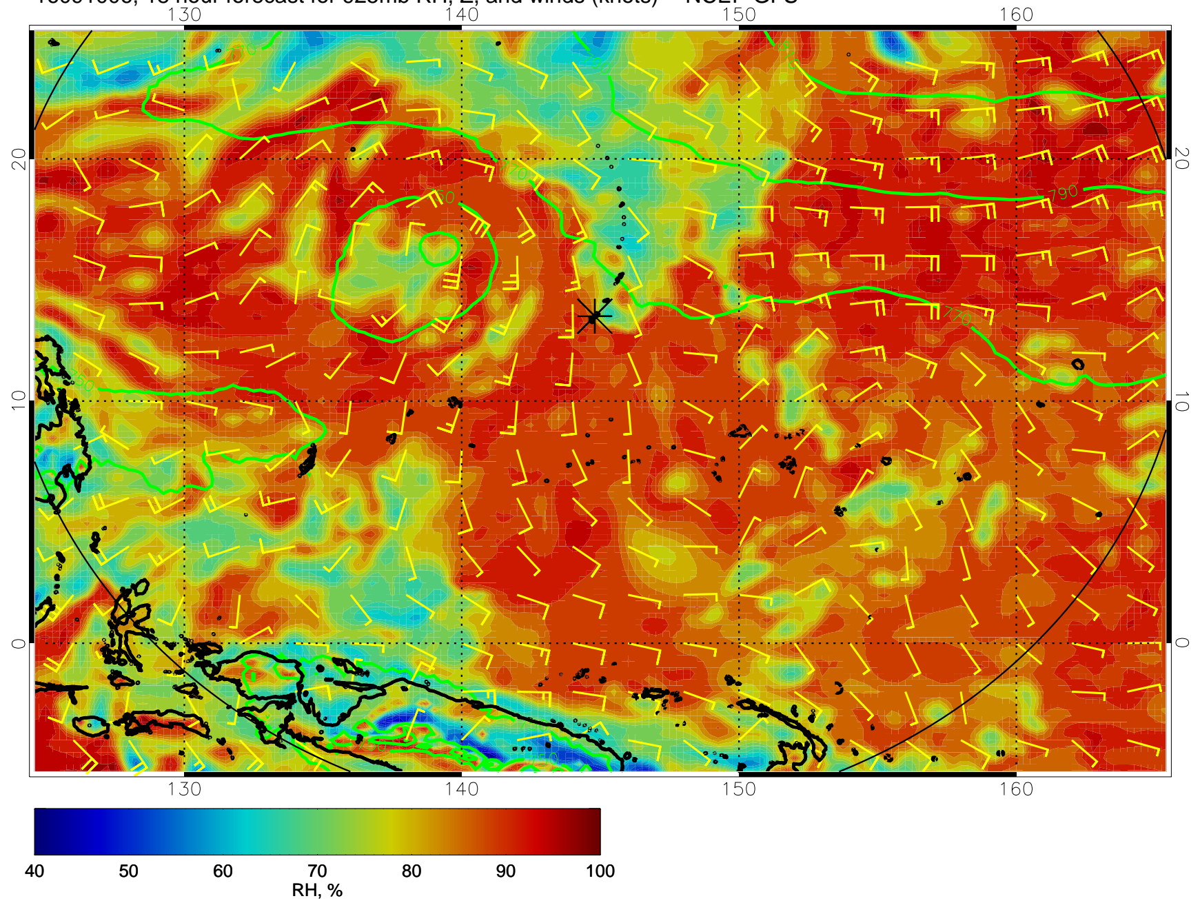
16091006, 18 hour forecast for 925mb RH, Z, and winds (knots) -- NCEP GFS
