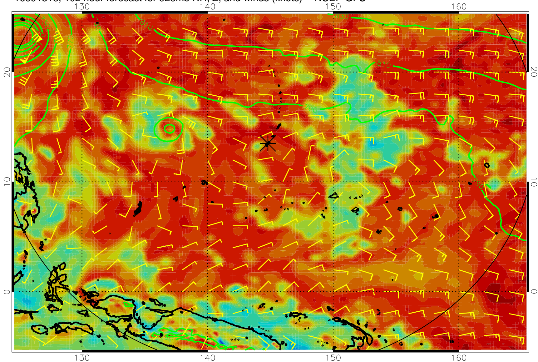
16091318, 102 hour forecast for 925mb RH, Z, and winds (knots) -- NCEP GFS
