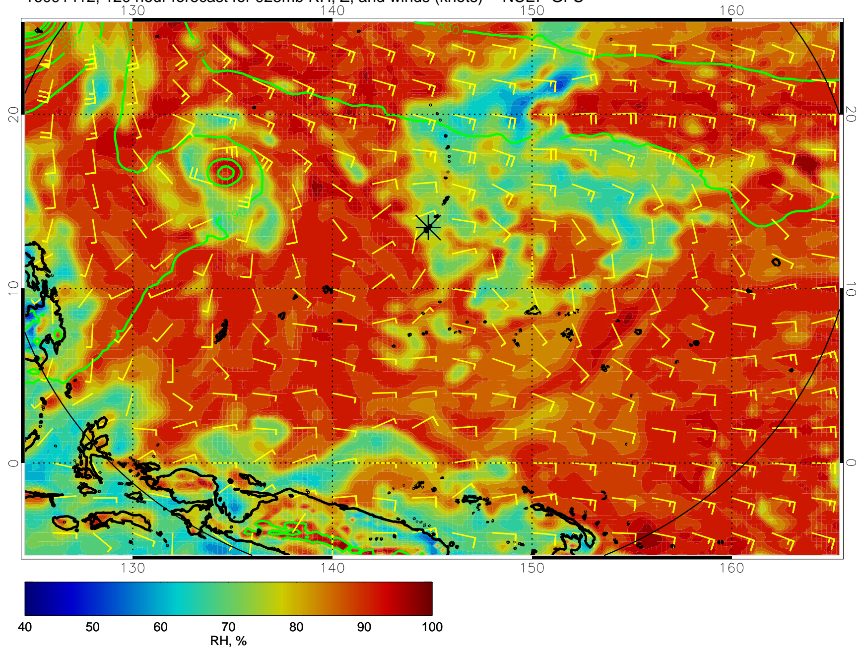
16091412, 120 hour forecast for 925mb RH, Z, and winds (knots) -- NCEP GFS
