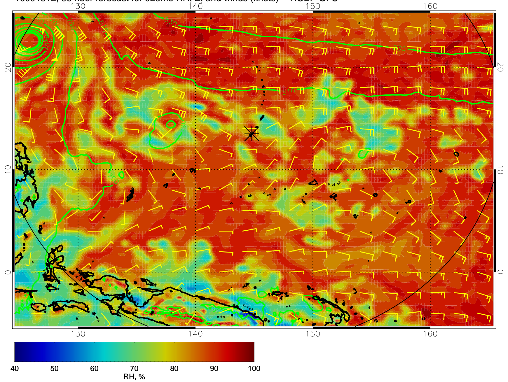
16091312, 96 hour forecast for 925mb RH, Z, and winds (knots) -- NCEP GFS
