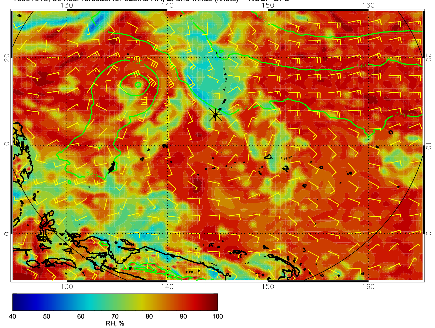
16091018, 30 hour forecast for 925mb RH, Z, and winds (knots) -- NCEP GFS
