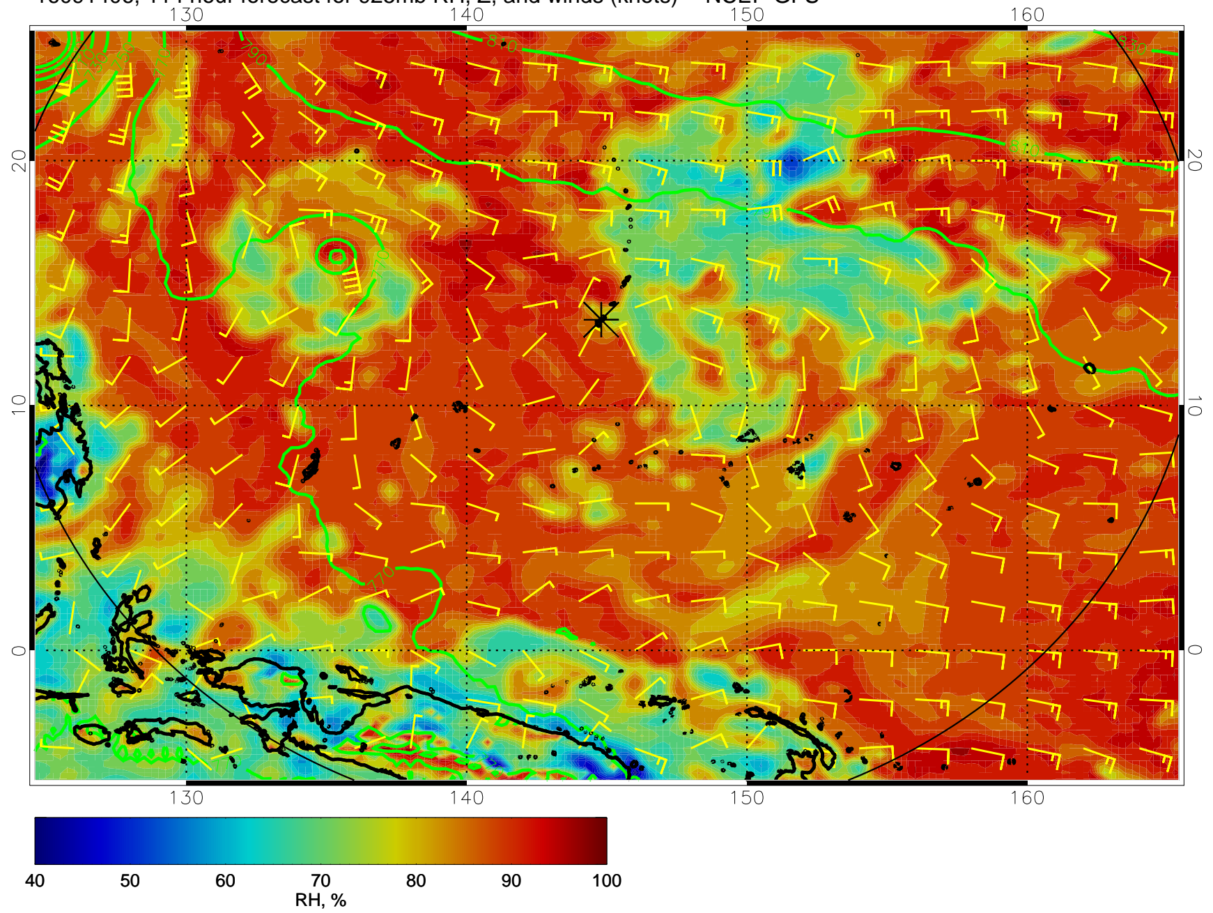
16091406, 114 hour forecast for 925mb RH, Z, and winds (knots) -- NCEP GFS
