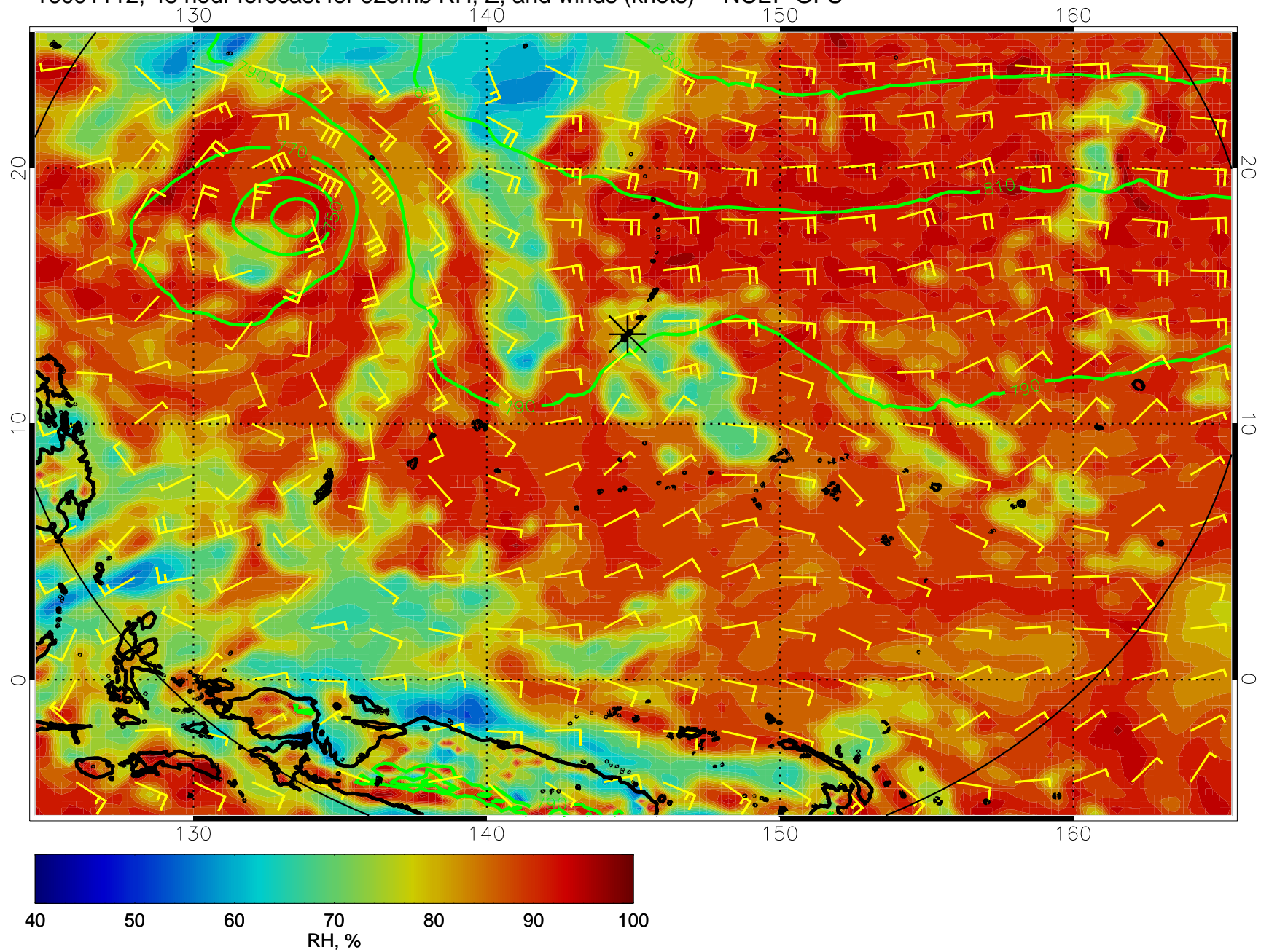
16091112, 48 hour forecast for 925mb RH, Z, and winds (knots) -- NCEP GFS
