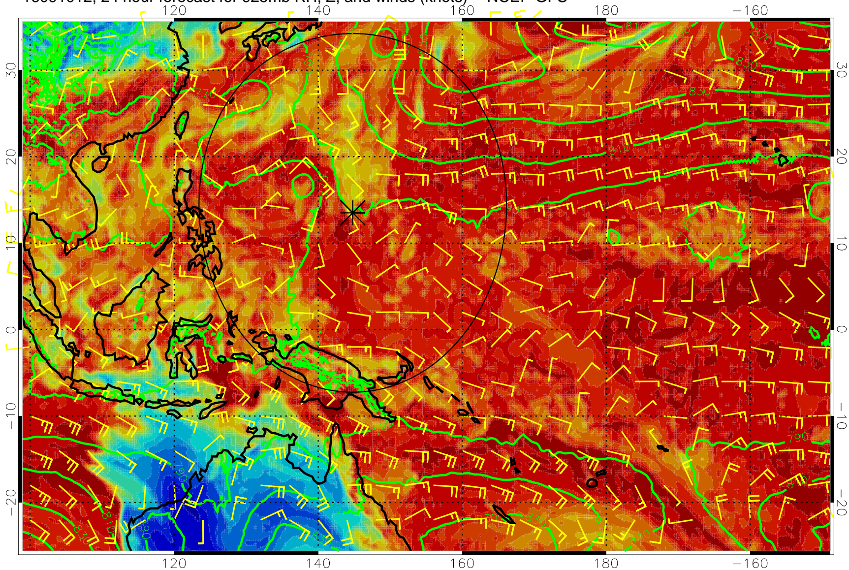
16091012, 24 hour forecast for 925mb RH, Z, and winds (knots) -- NCEP GFS
