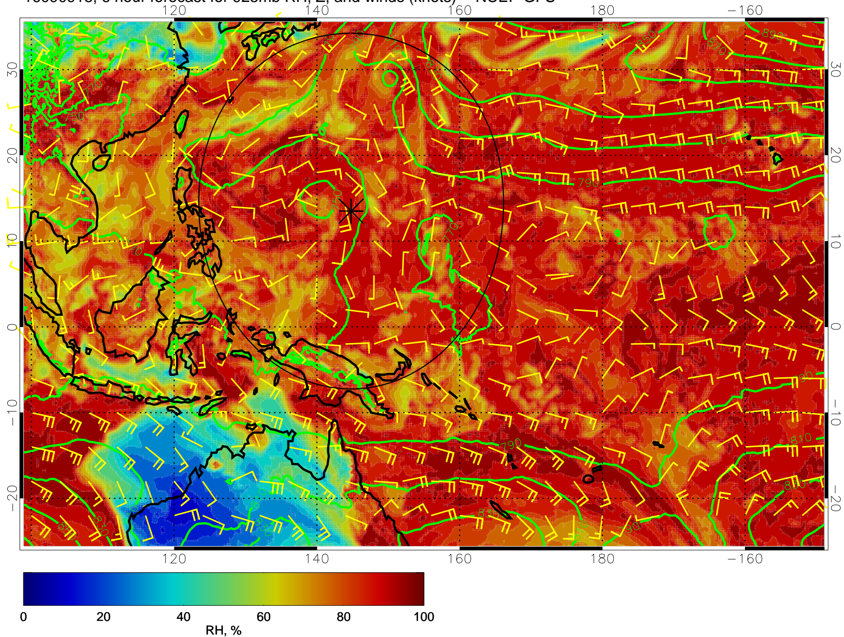
16090918, 6 hour forecast for 925mb RH, Z, and winds (knots) -- NCEP GFS
