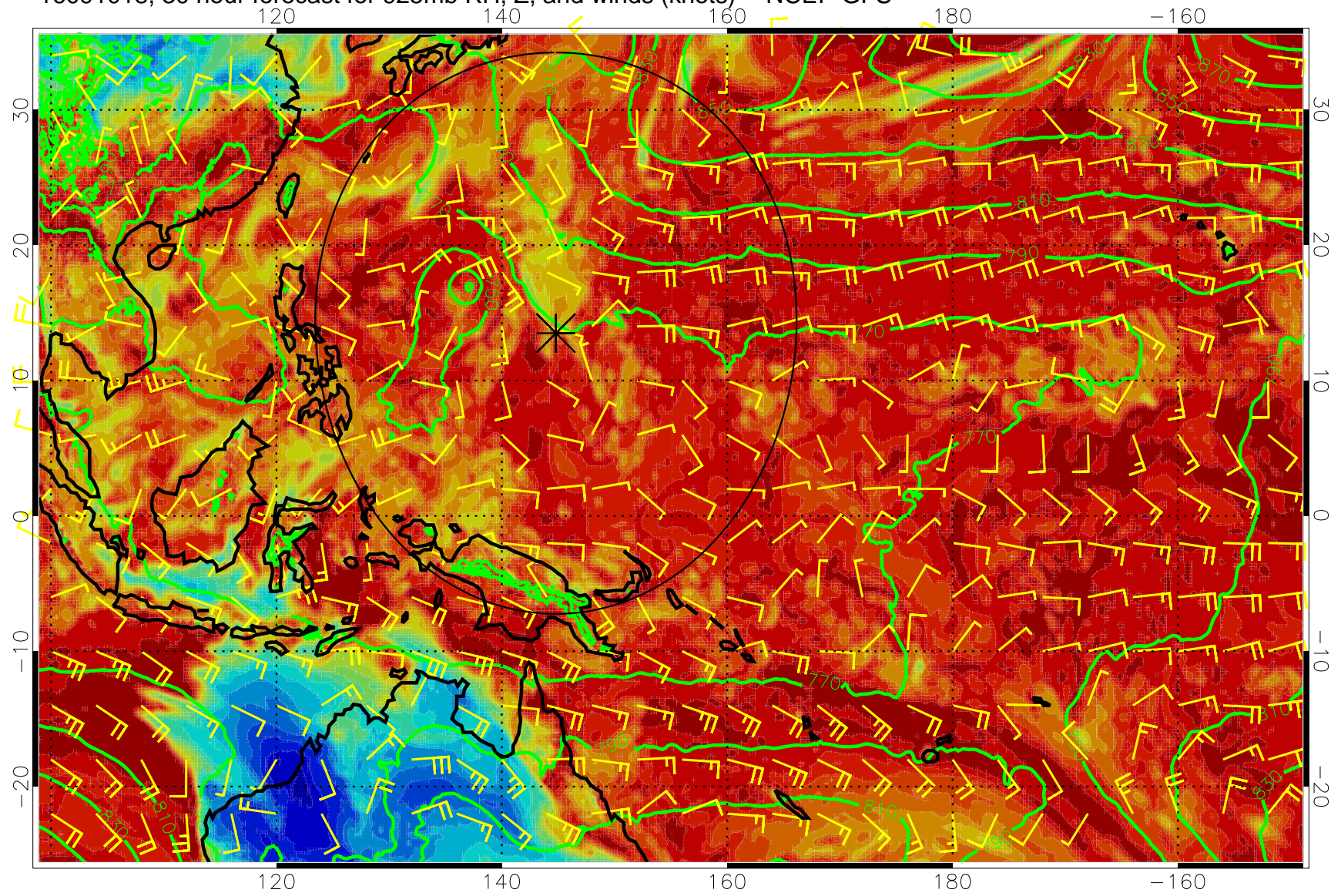
16091018, 30 hour forecast for 925mb RH, Z, and winds (knots) -- NCEP GFS
