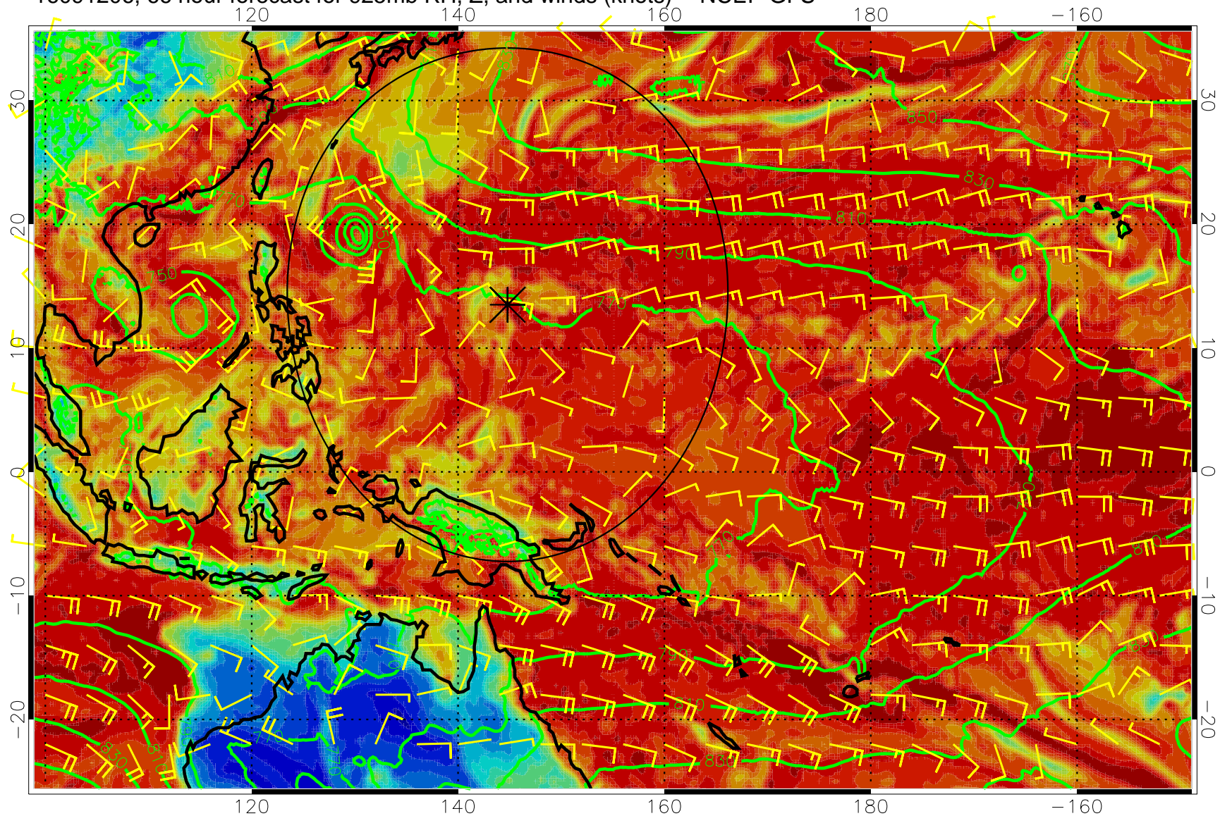
16091206, 66 hour forecast for 925mb RH, Z, and winds (knots) -- NCEP GFS
