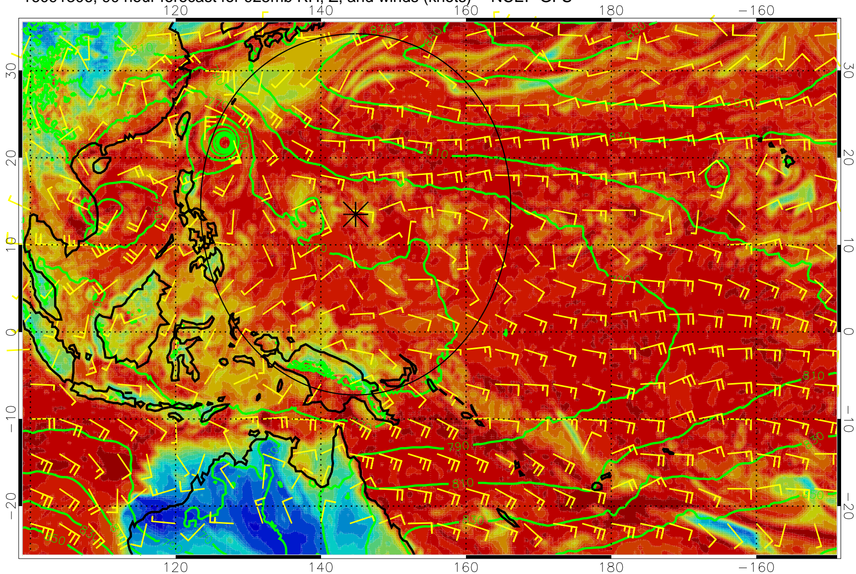
16091306, 90 hour forecast for 925mb RH, Z, and winds (knots) -- NCEP GFS
