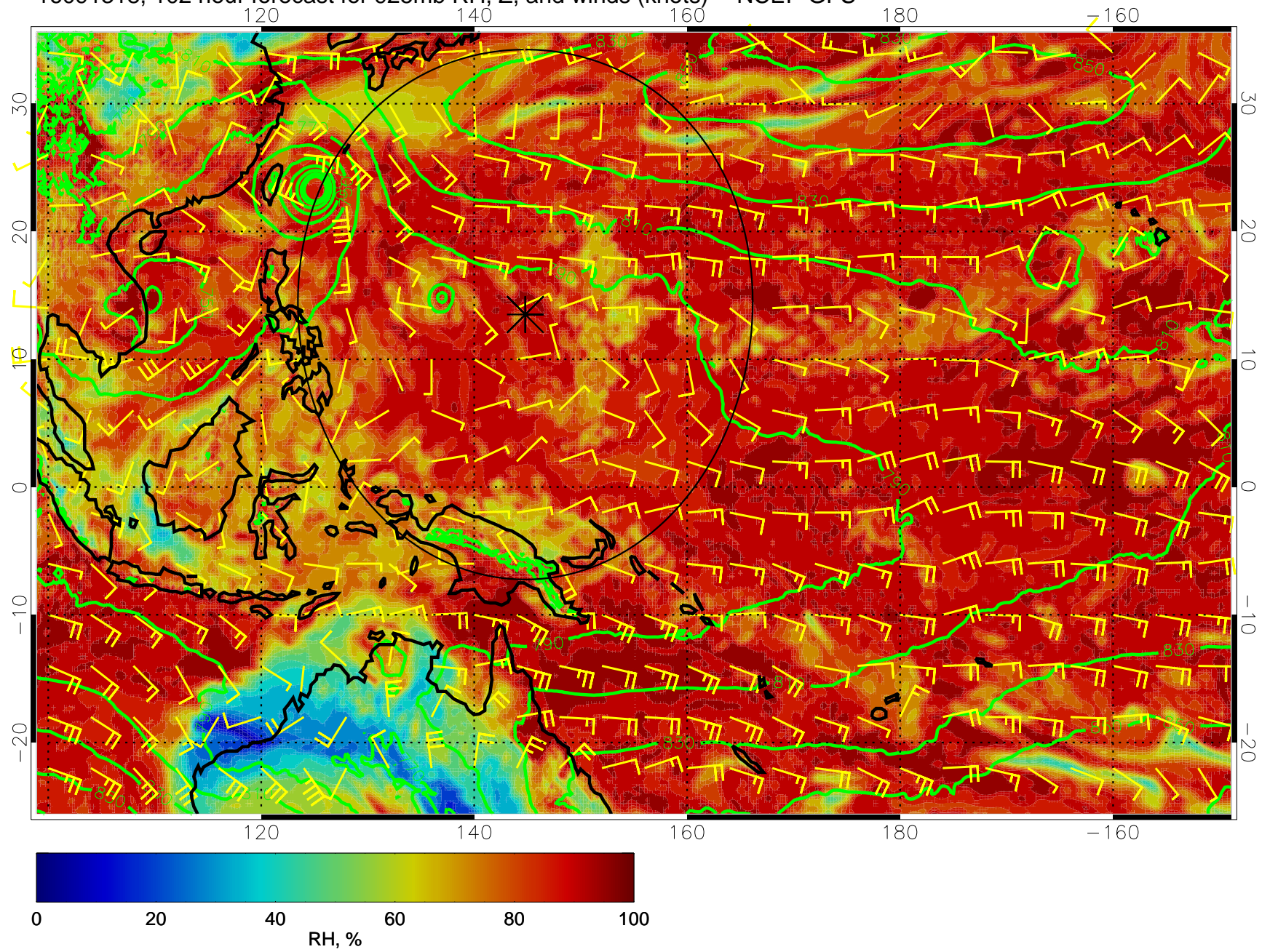
16091318, 102 hour forecast for 925mb RH, Z, and winds (knots) -- NCEP GFS
