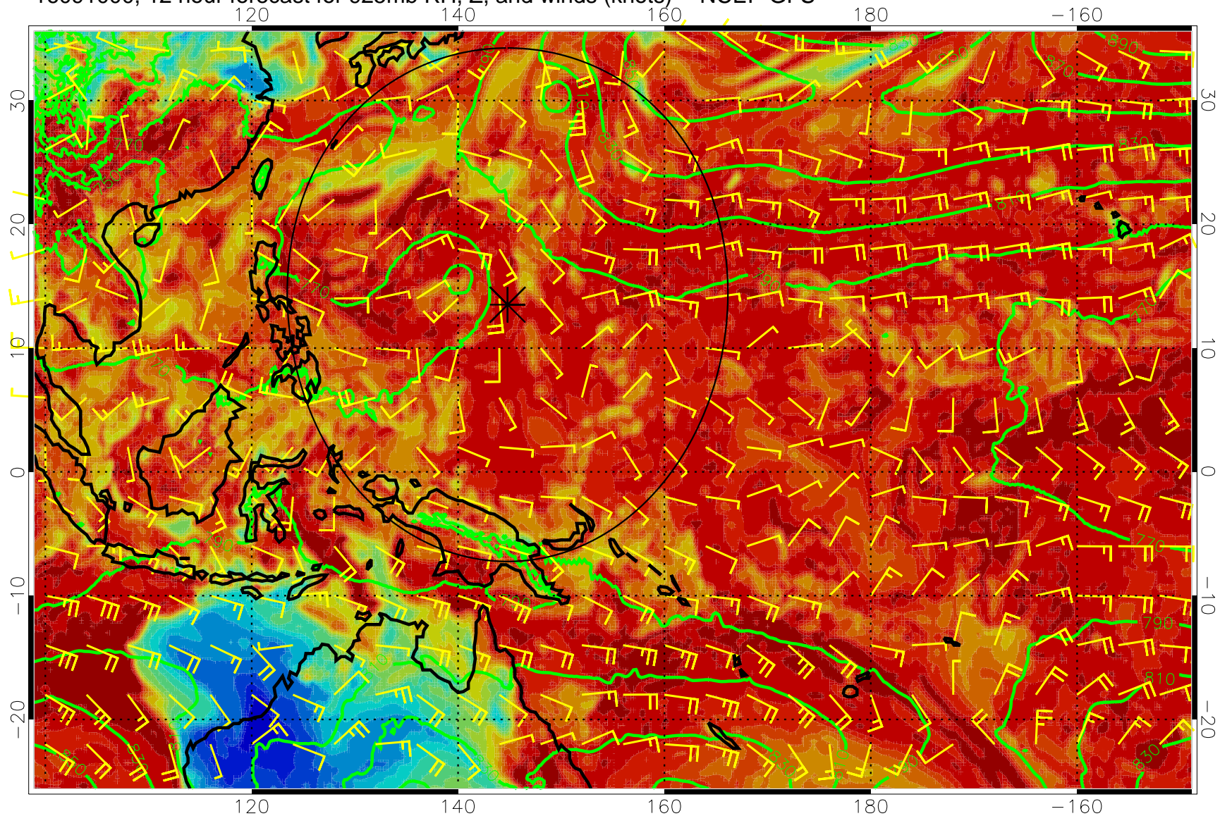
16091000, 12 hour forecast for 925mb RH, Z, and winds (knots) -- NCEP GFS
