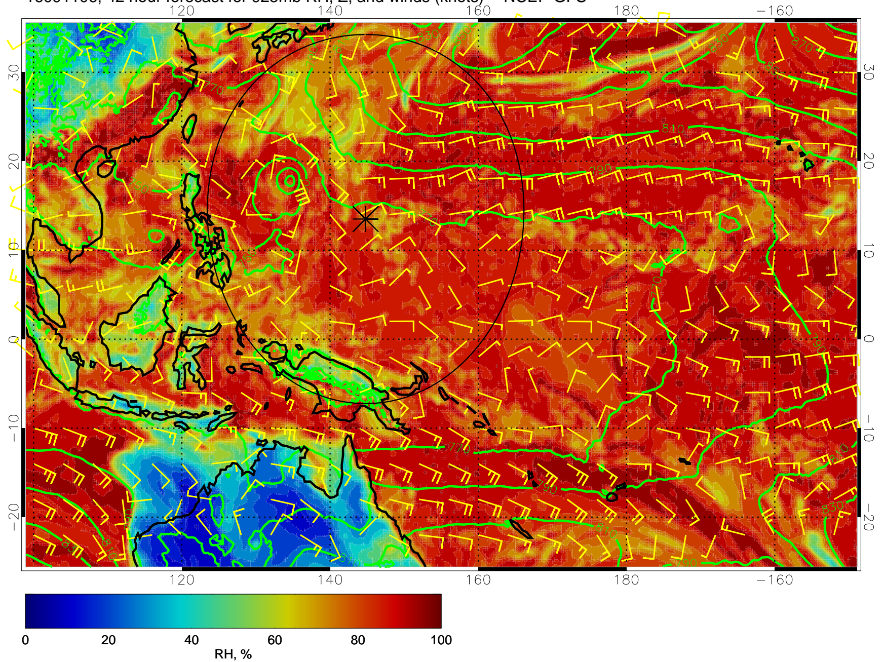
16091106, 42 hour forecast for 925mb RH, Z, and winds (knots) -- NCEP GFS
