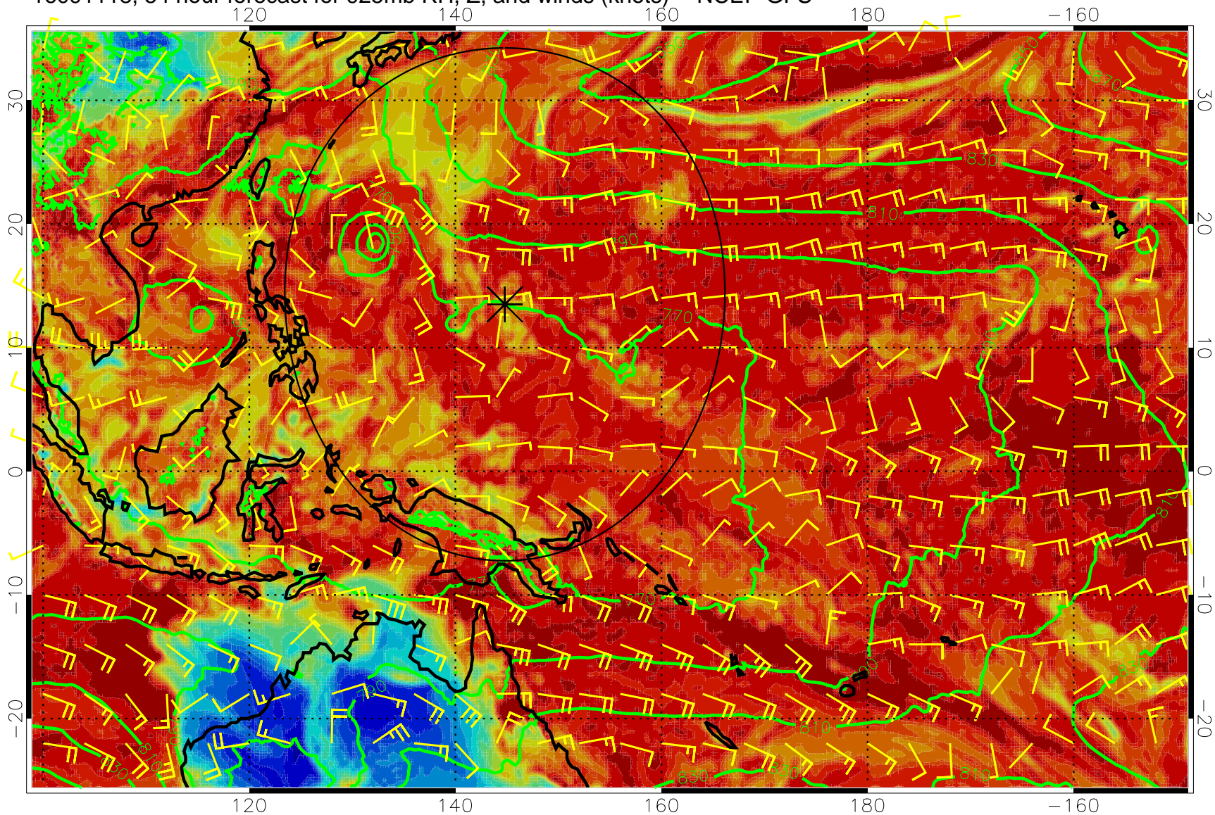
16091118, 54 hour forecast for 925mb RH, Z, and winds (knots) -- NCEP GFS
