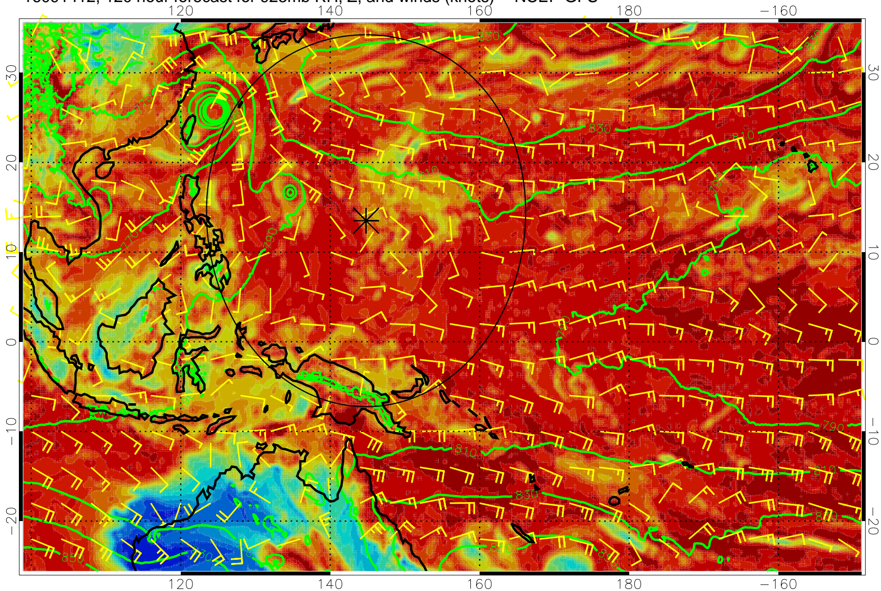
16091412, 120 hour forecast for 925mb RH, Z, and winds (knots) -- NCEP GFS
