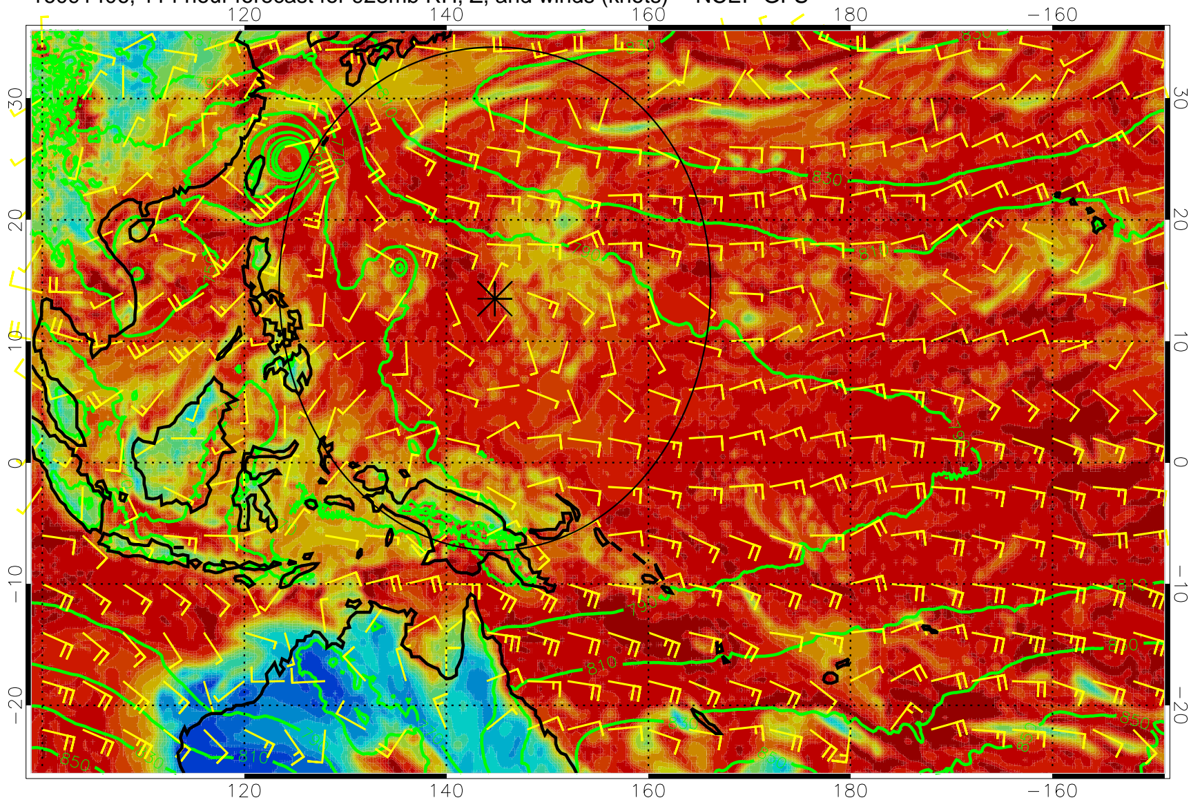
16091406, 114 hour forecast for 925mb RH, Z, and winds (knots) -- NCEP GFS
