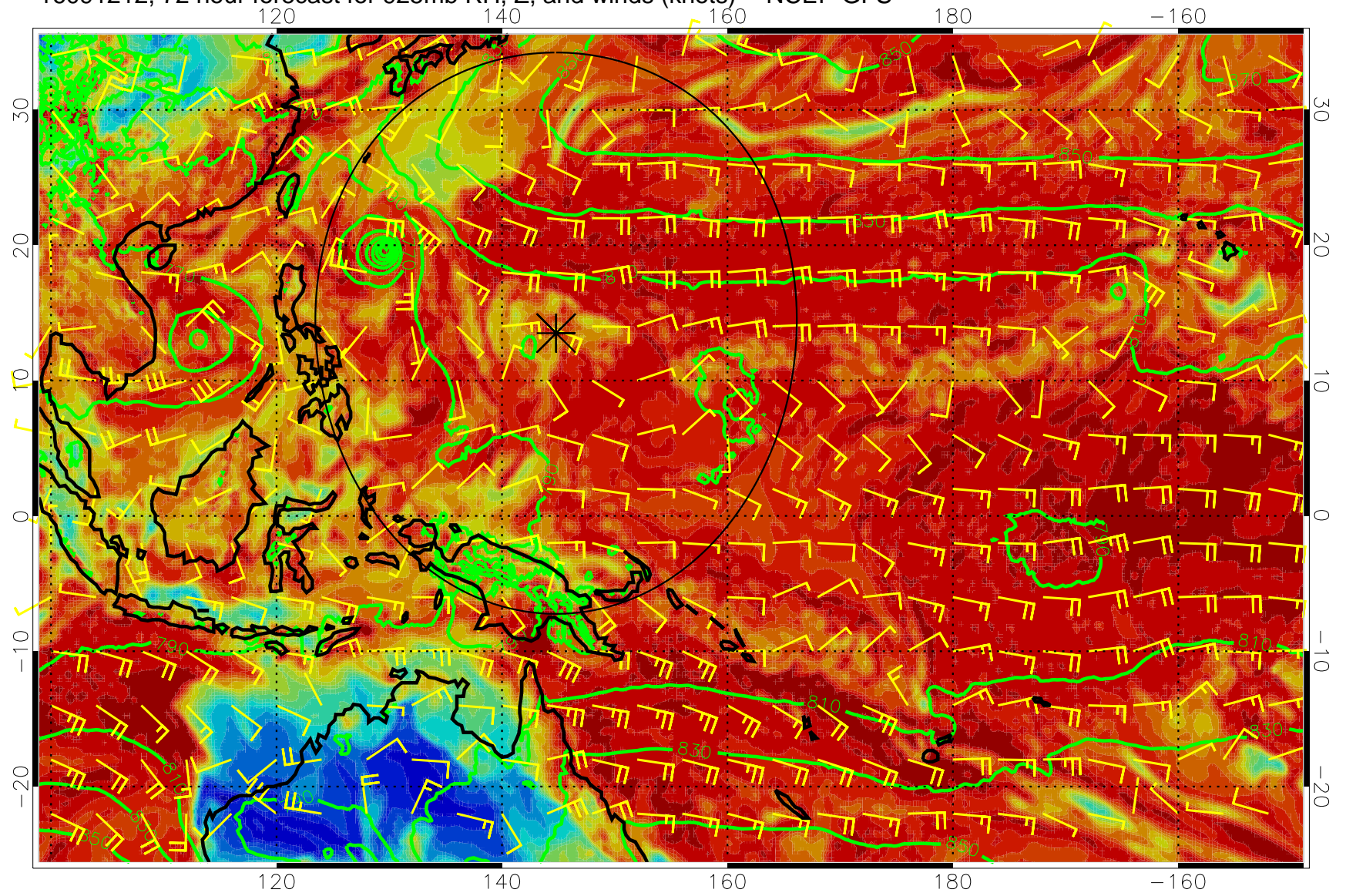
16091212, 72 hour forecast for 925mb RH, Z, and winds (knots) -- NCEP GFS
