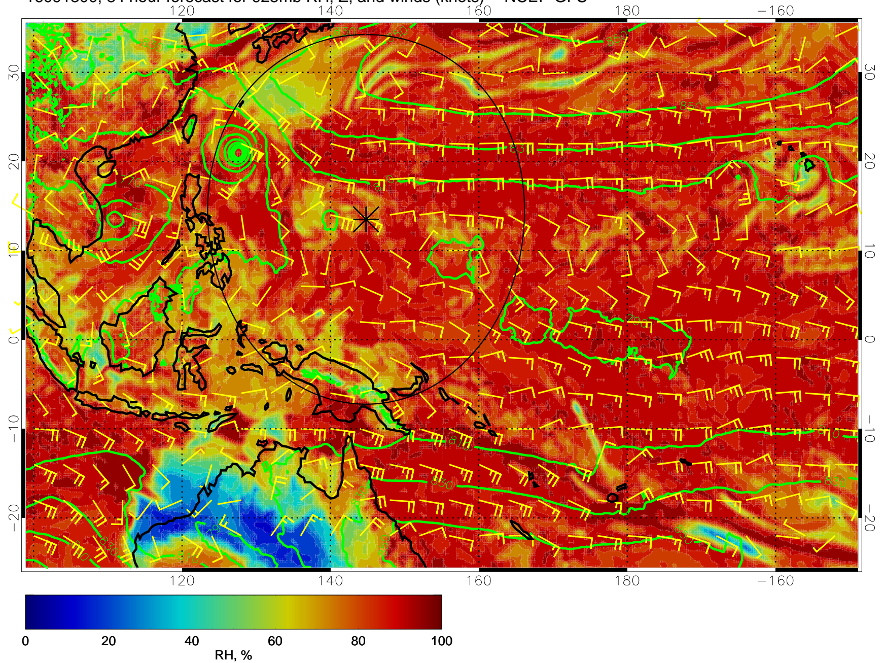
16091300, 84 hour forecast for 925mb RH, Z, and winds (knots) -- NCEP GFS
