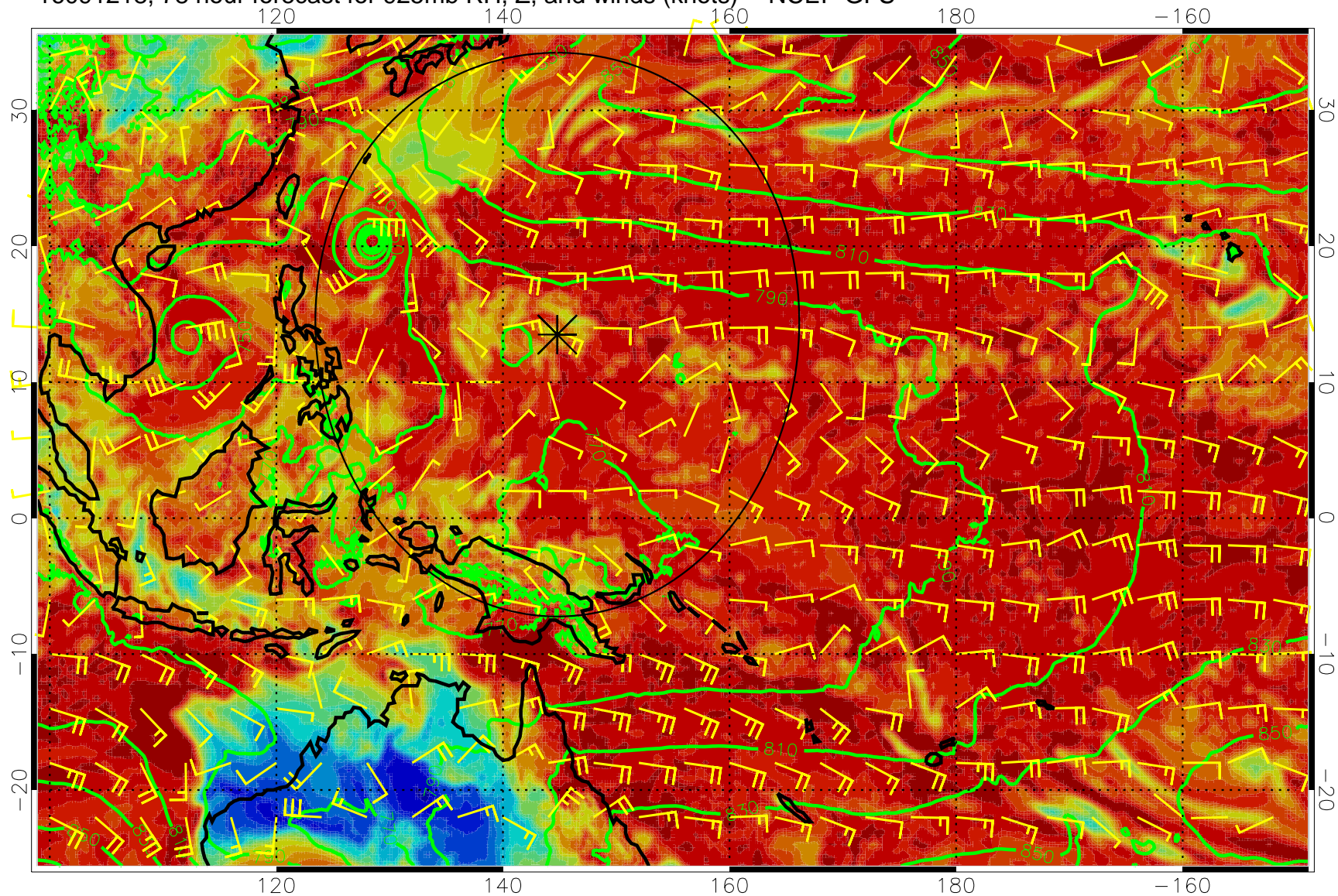
16091218, 78 hour forecast for 925mb RH, Z, and winds (knots) -- NCEP GFS
