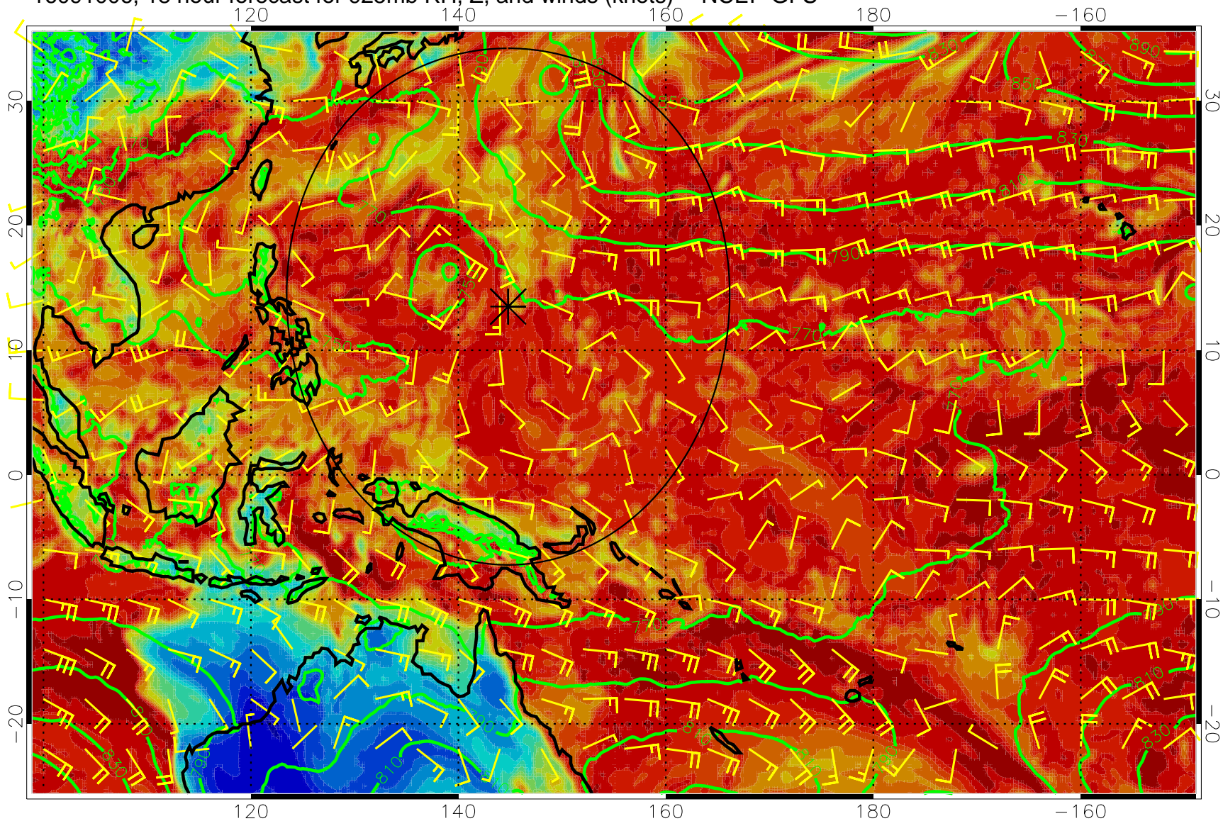
16091006, 18 hour forecast for 925mb RH, Z, and winds (knots) -- NCEP GFS
