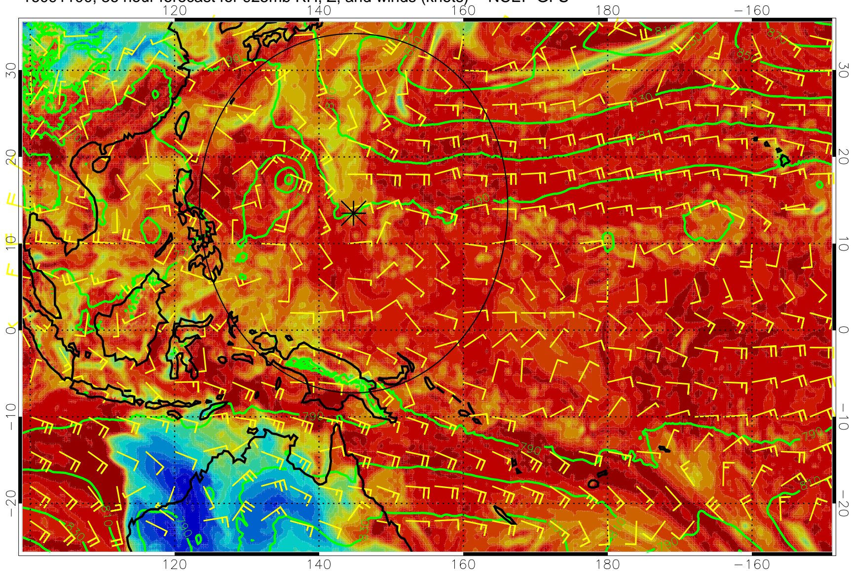
16091100, 36 hour forecast for 925mb RH, Z, and winds (knots) -- NCEP GFS
