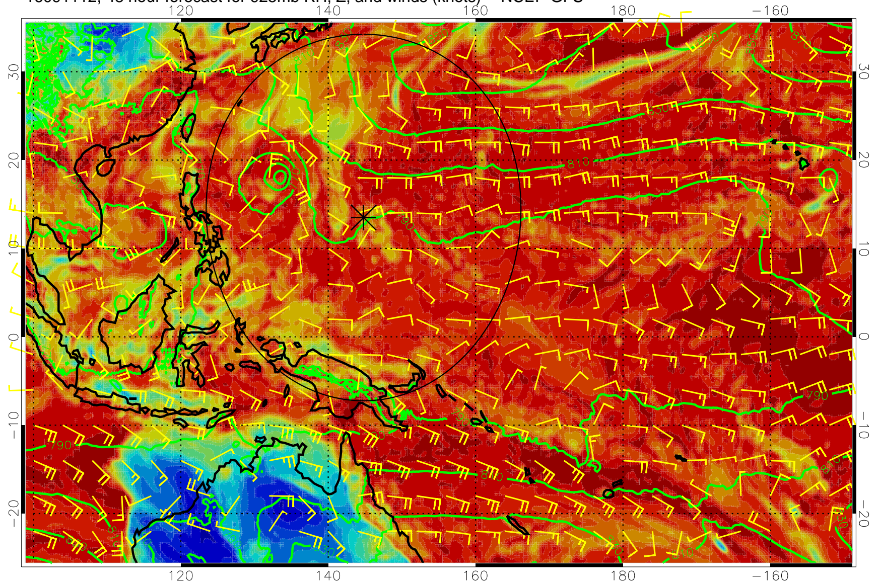
16091112, 48 hour forecast for 925mb RH, Z, and winds (knots) -- NCEP GFS
