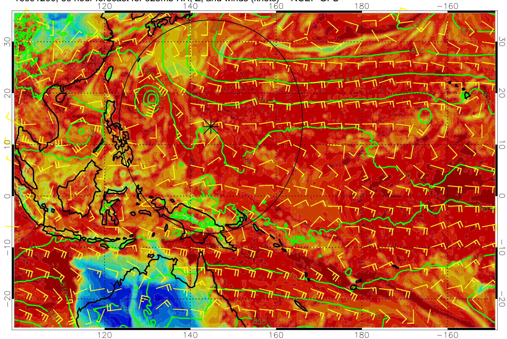
16091200, 60 hour forecast for 925mb RH, Z, and winds (knots) -- NCEP GFS
