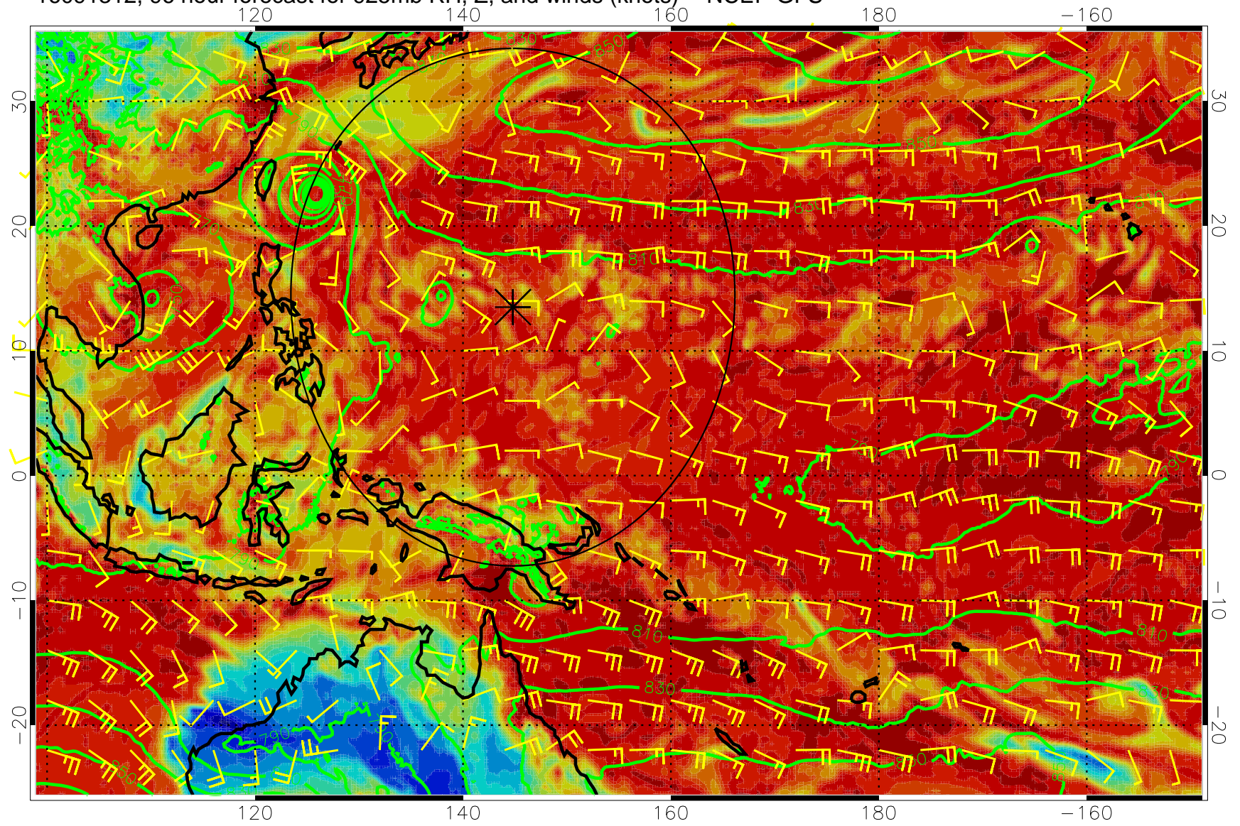
16091312, 96 hour forecast for 925mb RH, Z, and winds (knots) -- NCEP GFS
