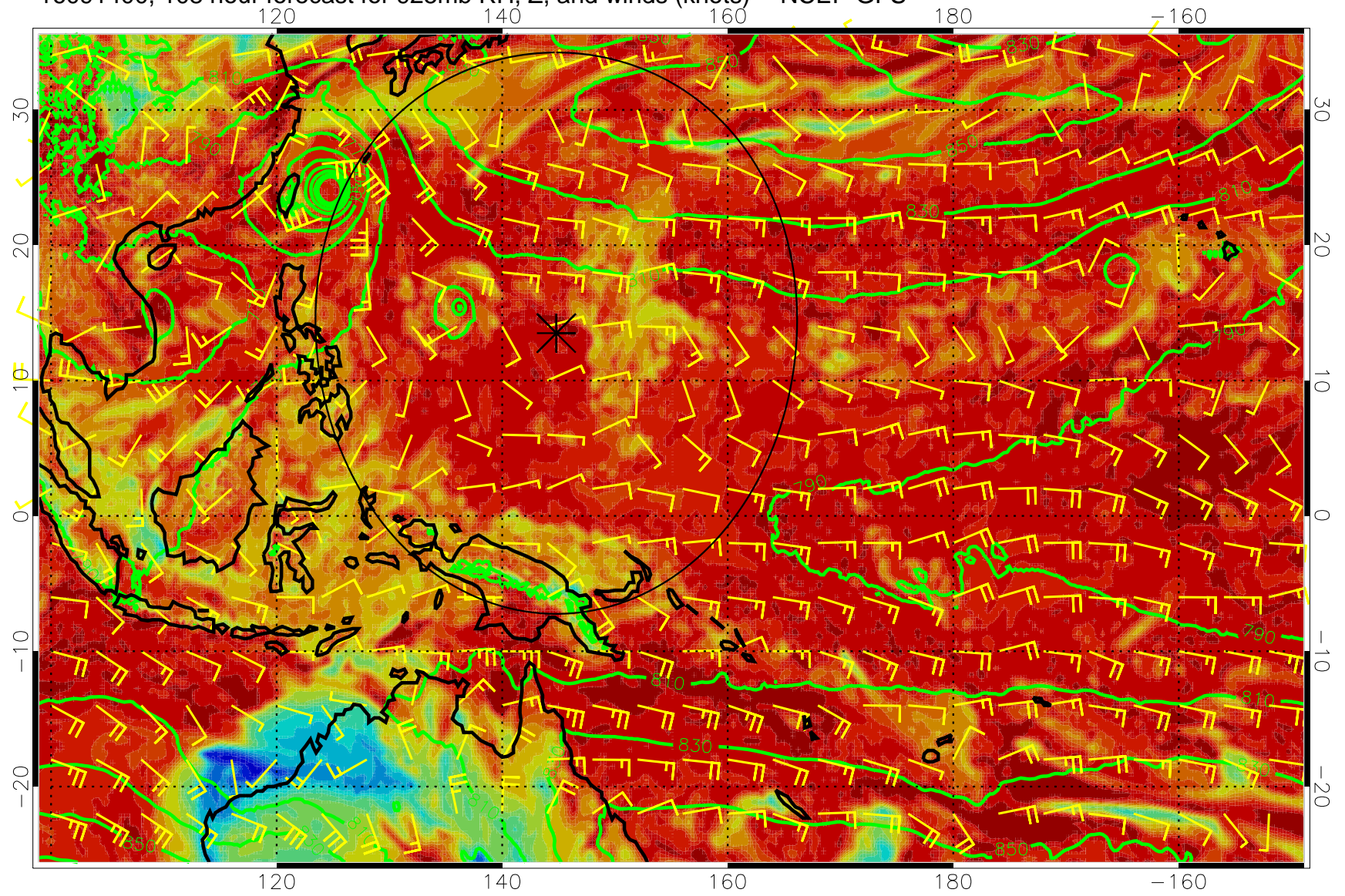
16091400, 108 hour forecast for 925mb RH, Z, and winds (knots) -- NCEP GFS
