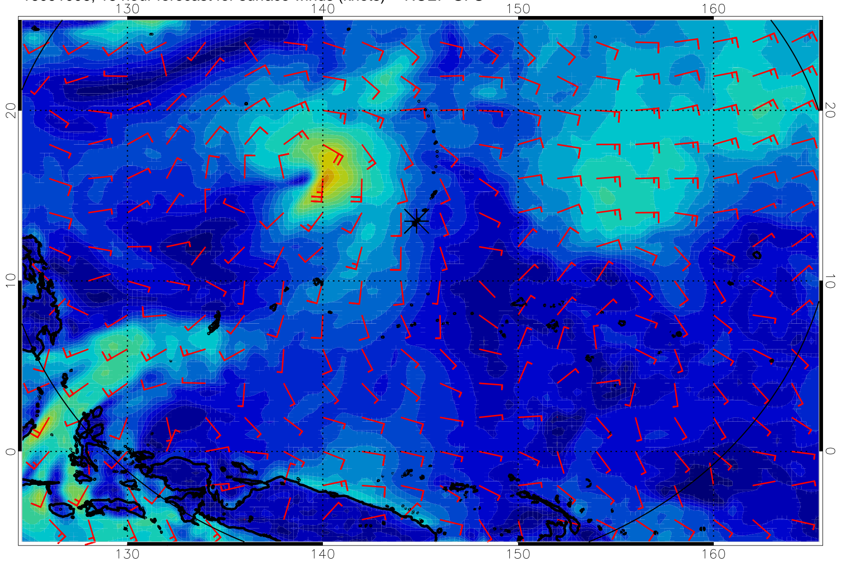
16091006, 18 hour forecast for surface winds (knots) -- NCEP GFS
