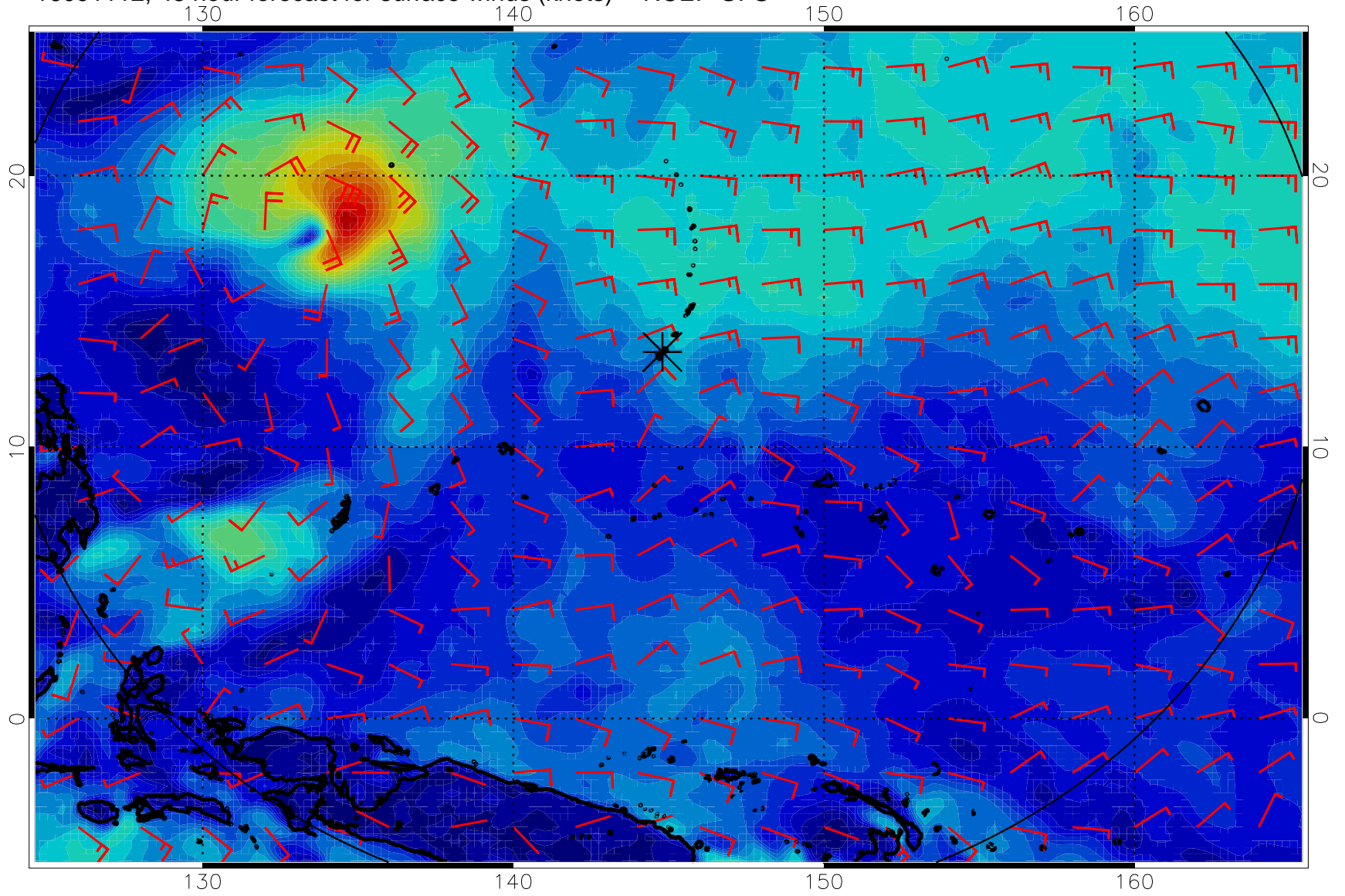
16091112, 48 hour forecast for surface winds (knots) -- NCEP GFS
