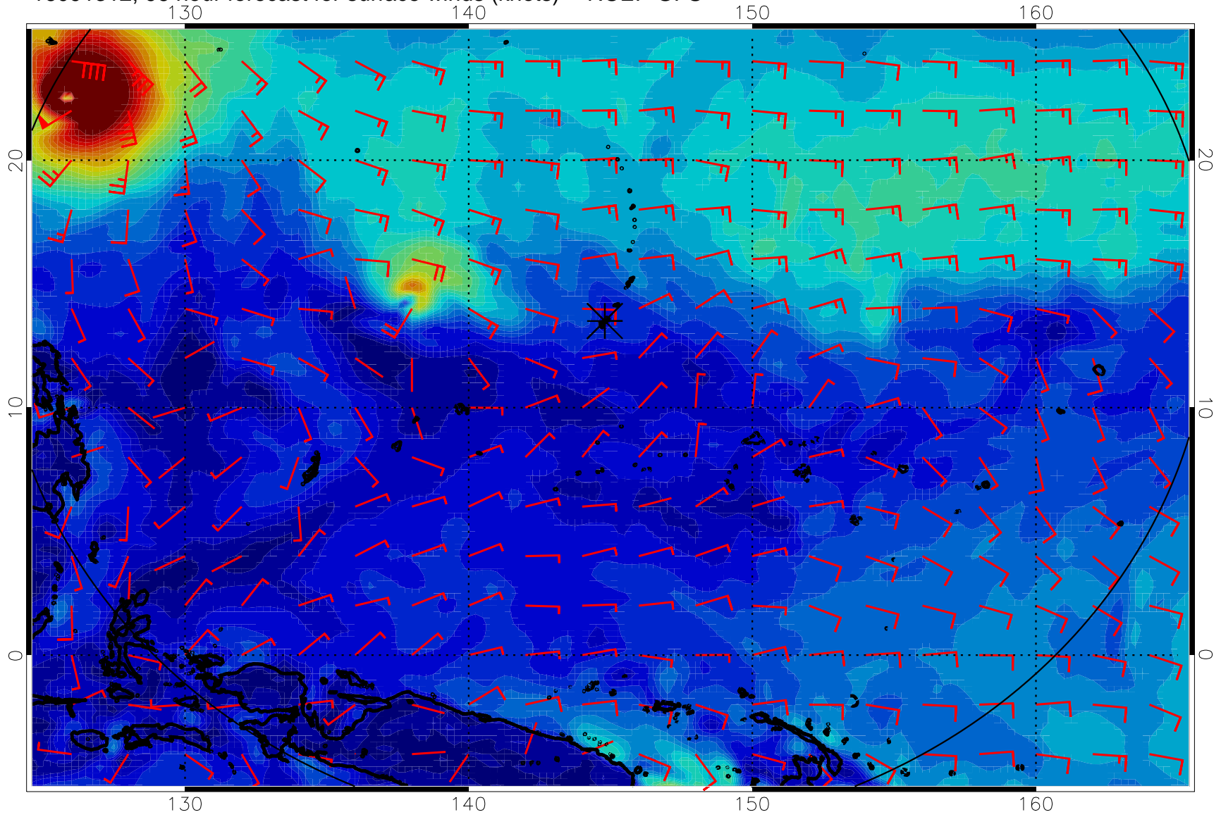
16091312, 96 hour forecast for surface winds (knots) -- NCEP GFS
