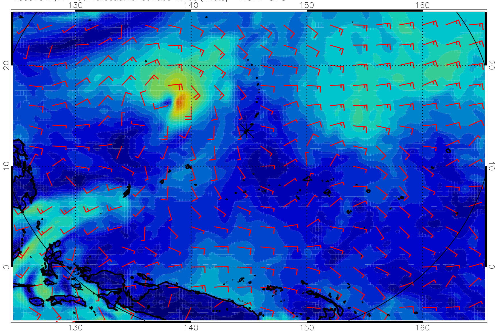
16091012, 24 hour forecast for surface winds (knots) -- NCEP GFS
