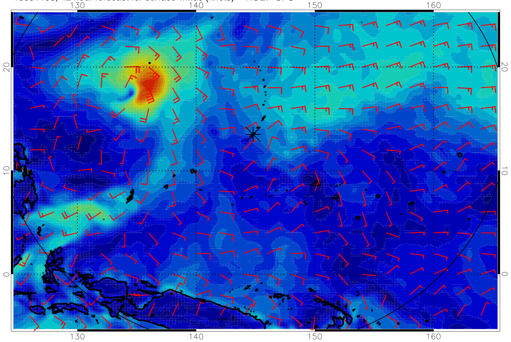
16091106, 42 hour forecast for surface winds (knots) -- NCEP GFS
