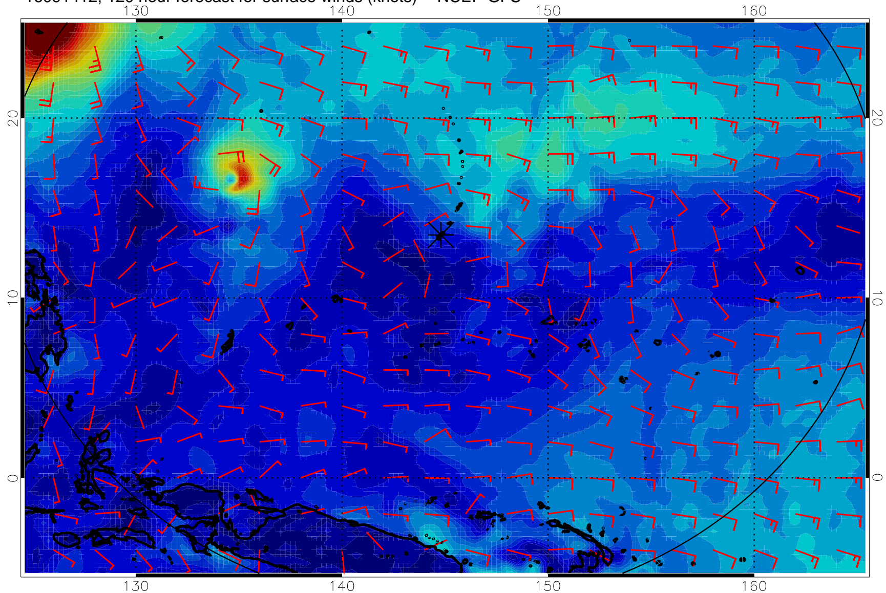
16091412, 120 hour forecast for surface winds (knots) -- NCEP GFS
