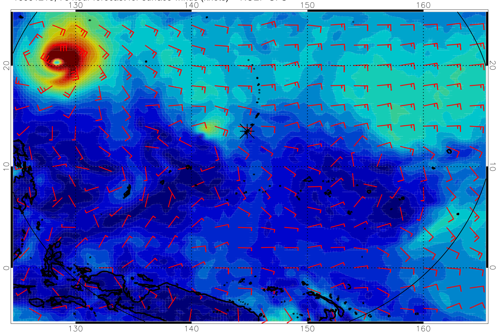
16091218, 78 hour forecast for surface winds (knots) -- NCEP GFS
