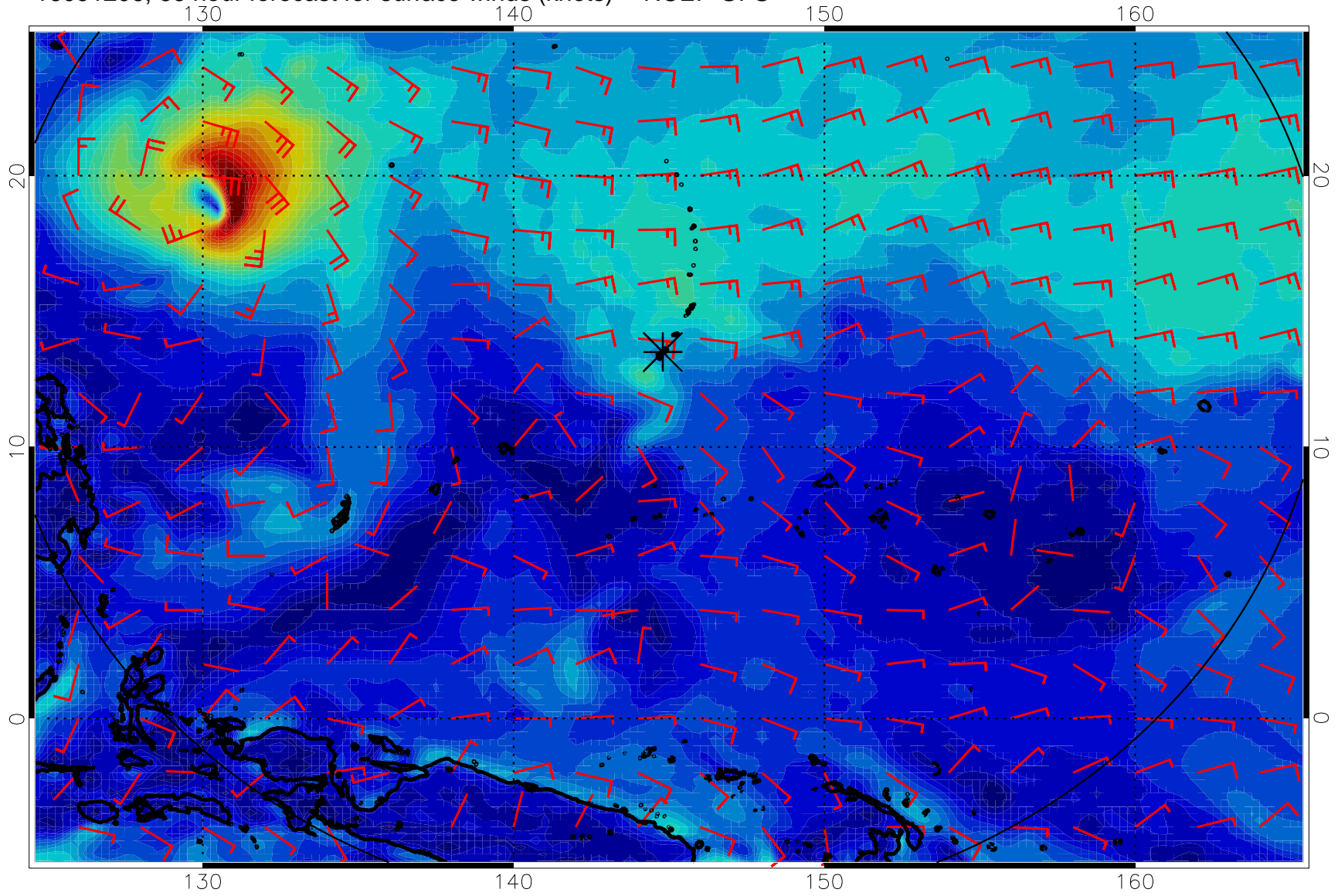
16091206, 66 hour forecast for surface winds (knots) -- NCEP GFS
