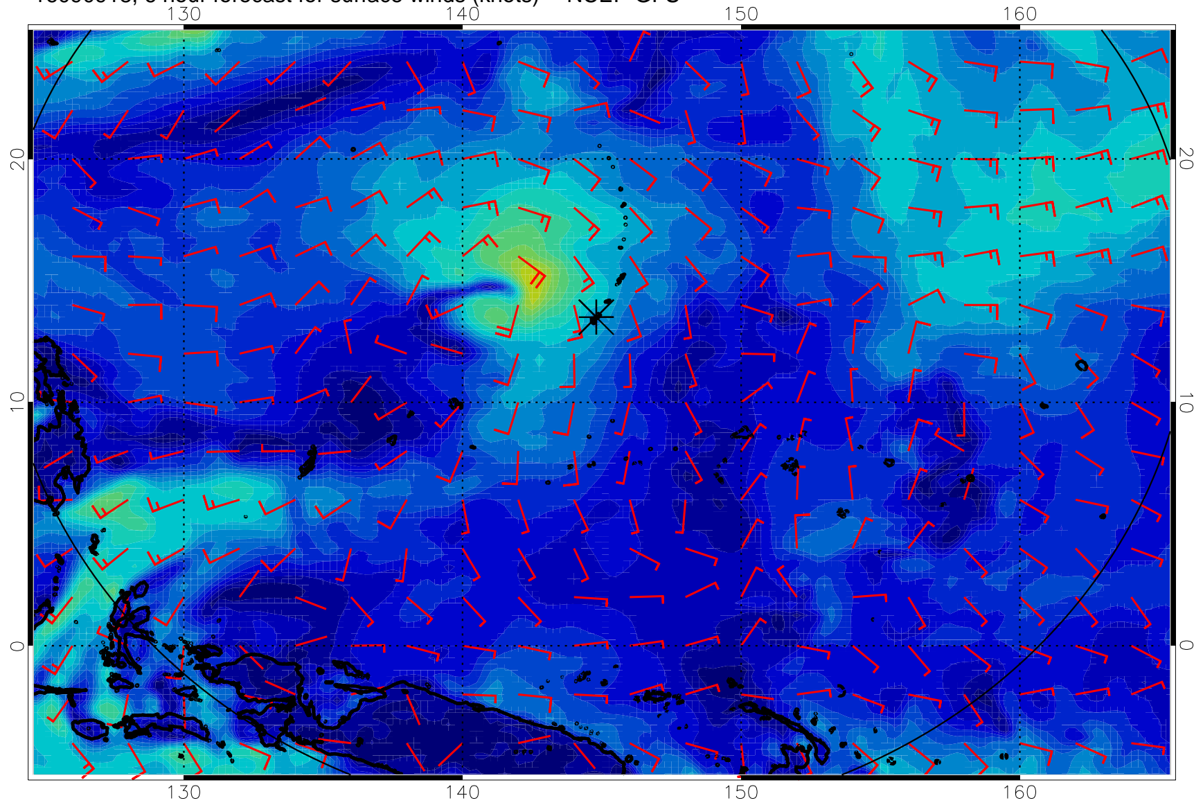
16090918, 6 hour forecast for surface winds (knots) -- NCEP GFS
