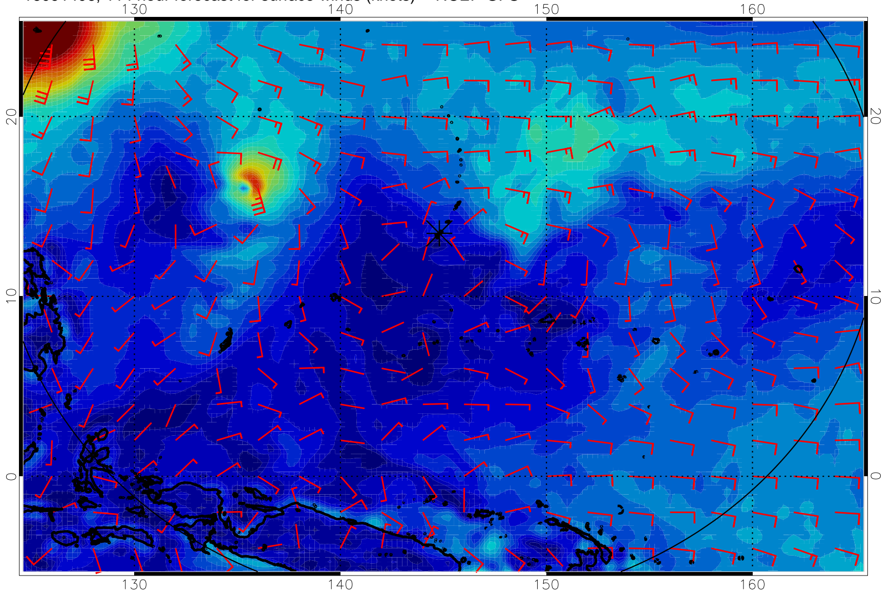
16091406, 114 hour forecast for surface winds (knots) -- NCEP GFS
