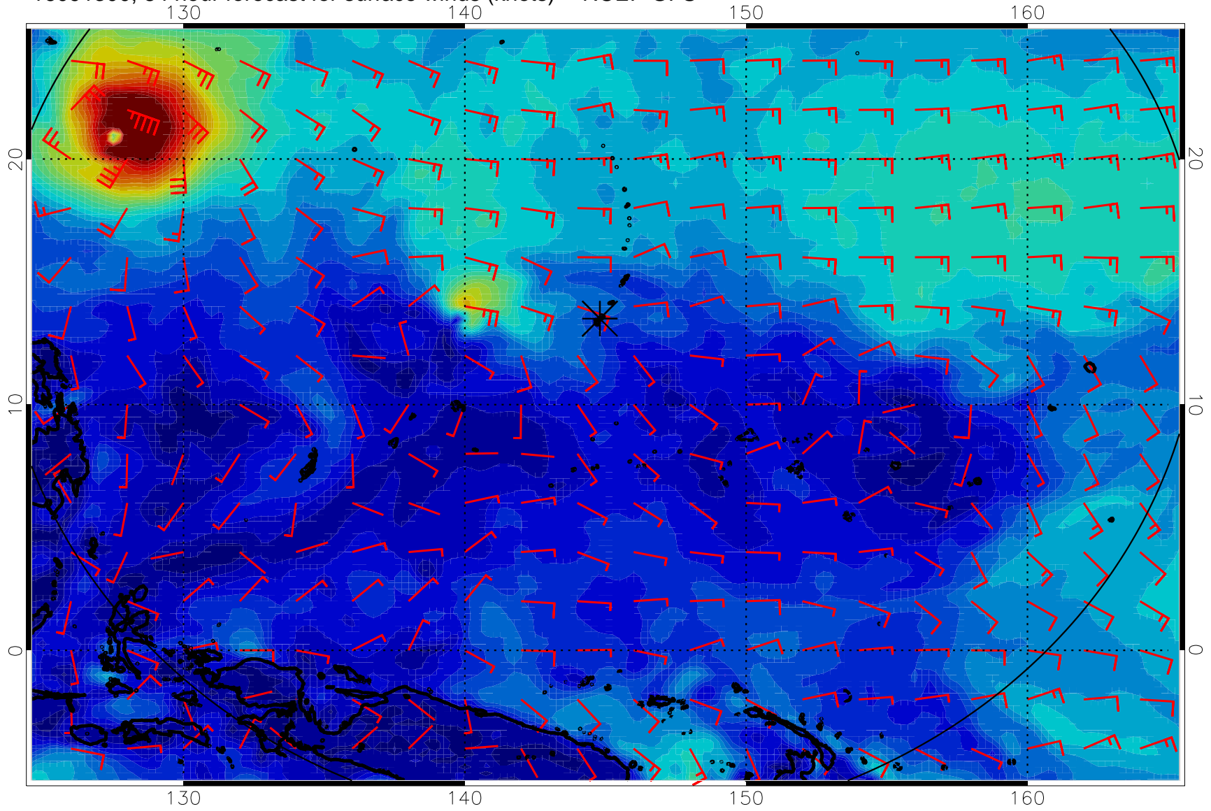
16091300, 84 hour forecast for surface winds (knots) -- NCEP GFS
