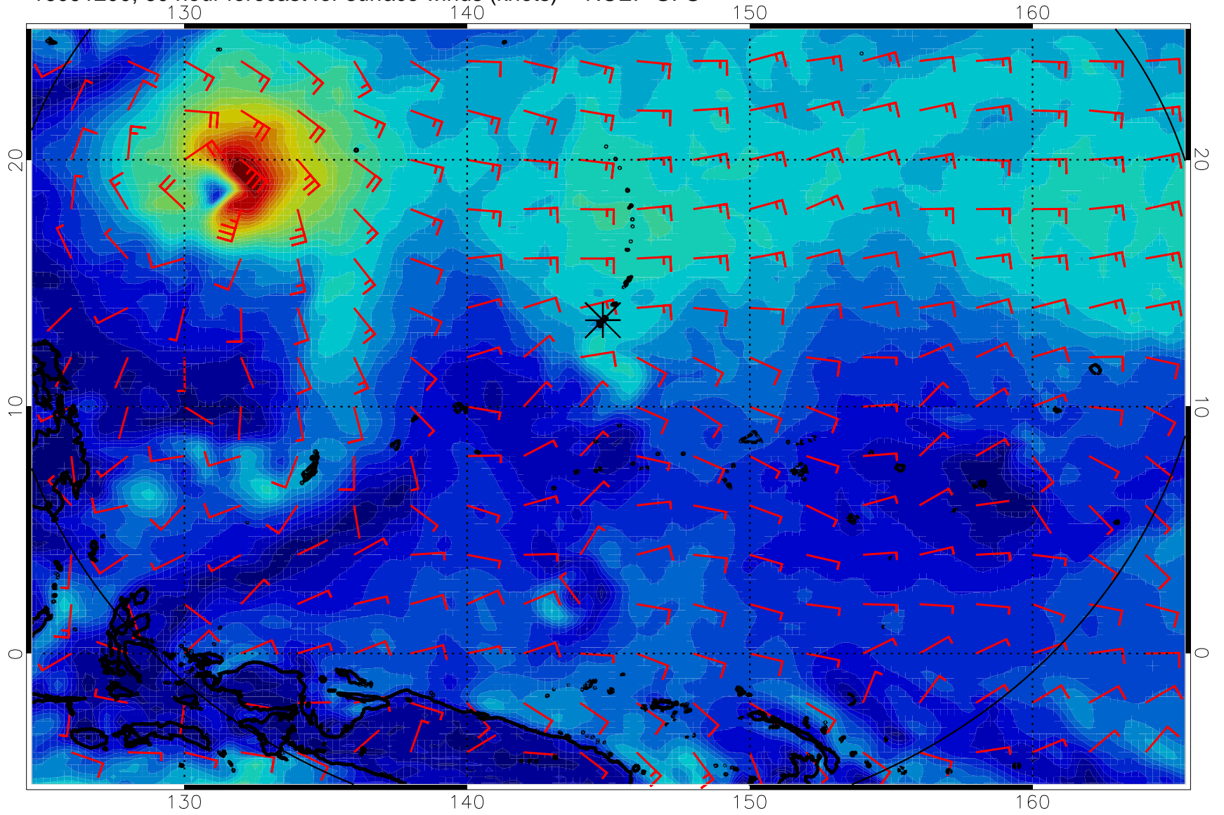
16091200, 60 hour forecast for surface winds (knots) -- NCEP GFS
