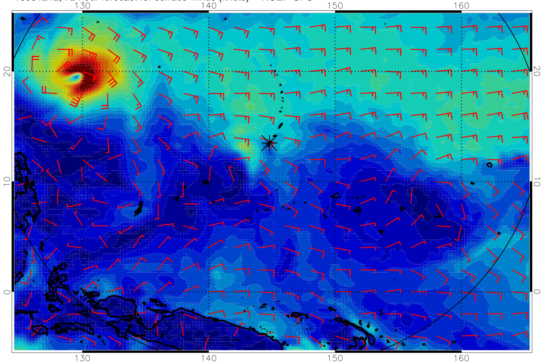
16091212, 72 hour forecast for surface winds (knots) -- NCEP GFS
