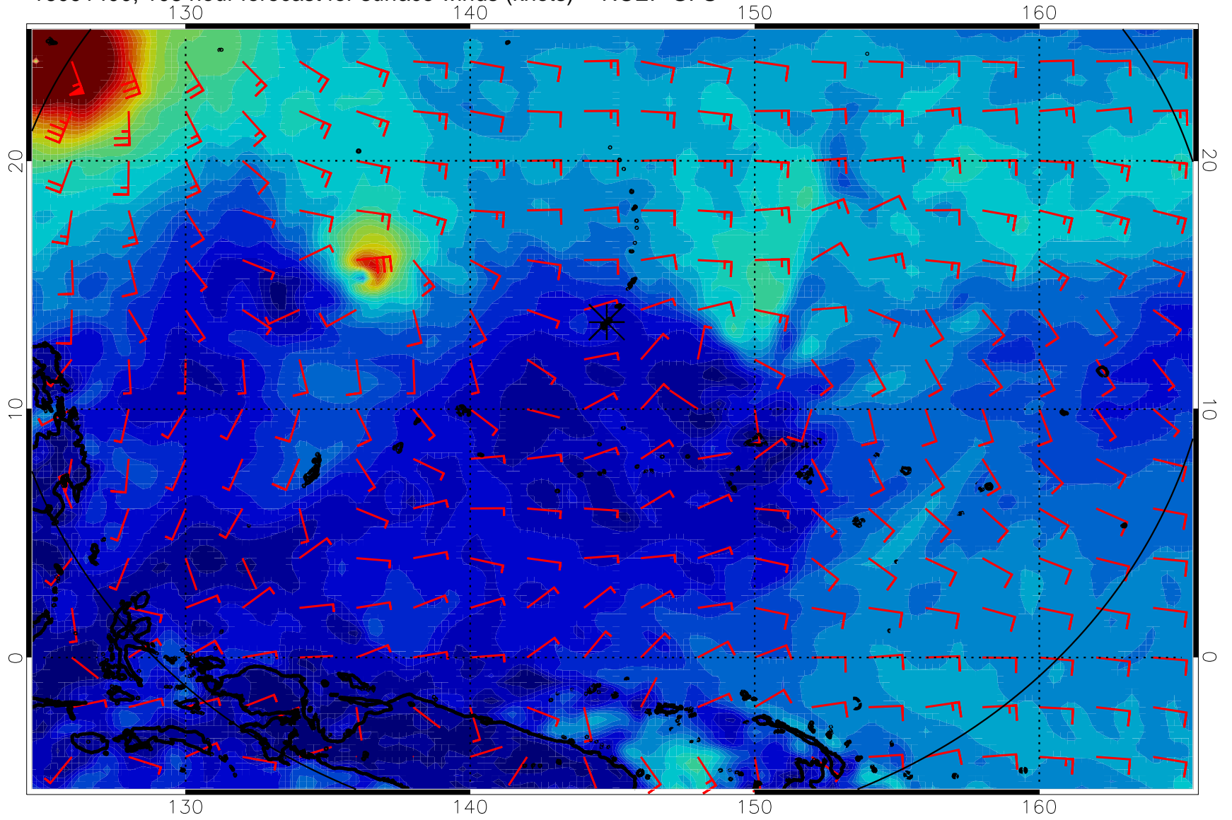
16091400, 108 hour forecast for surface winds (knots) -- NCEP GFS
