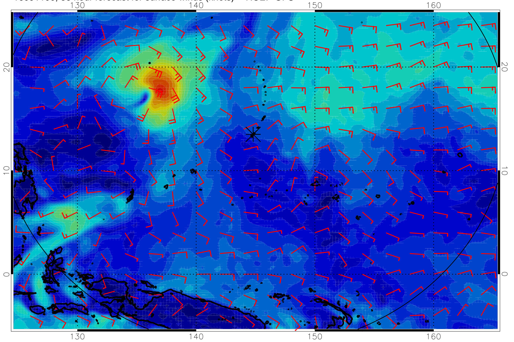
16091100, 36 hour forecast for surface winds (knots) -- NCEP GFS
