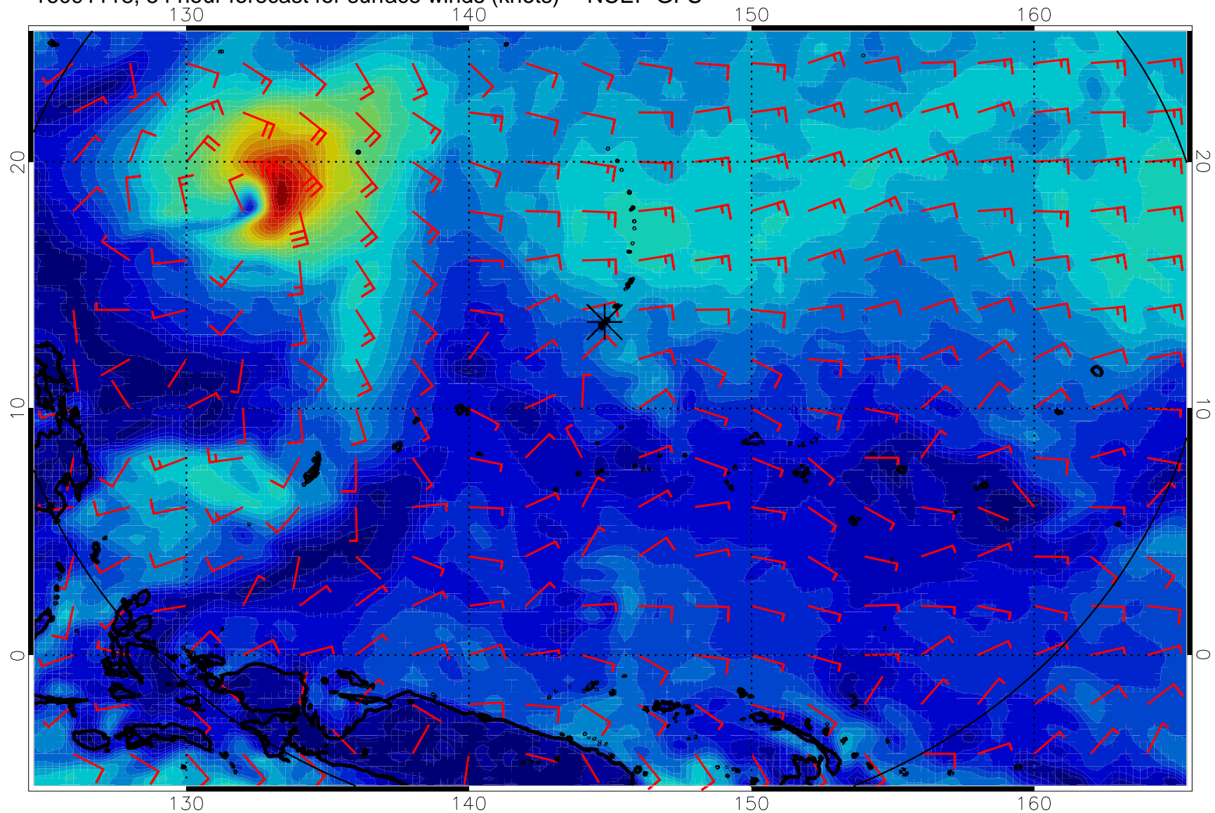
16091118, 54 hour forecast for surface winds (knots) -- NCEP GFS
