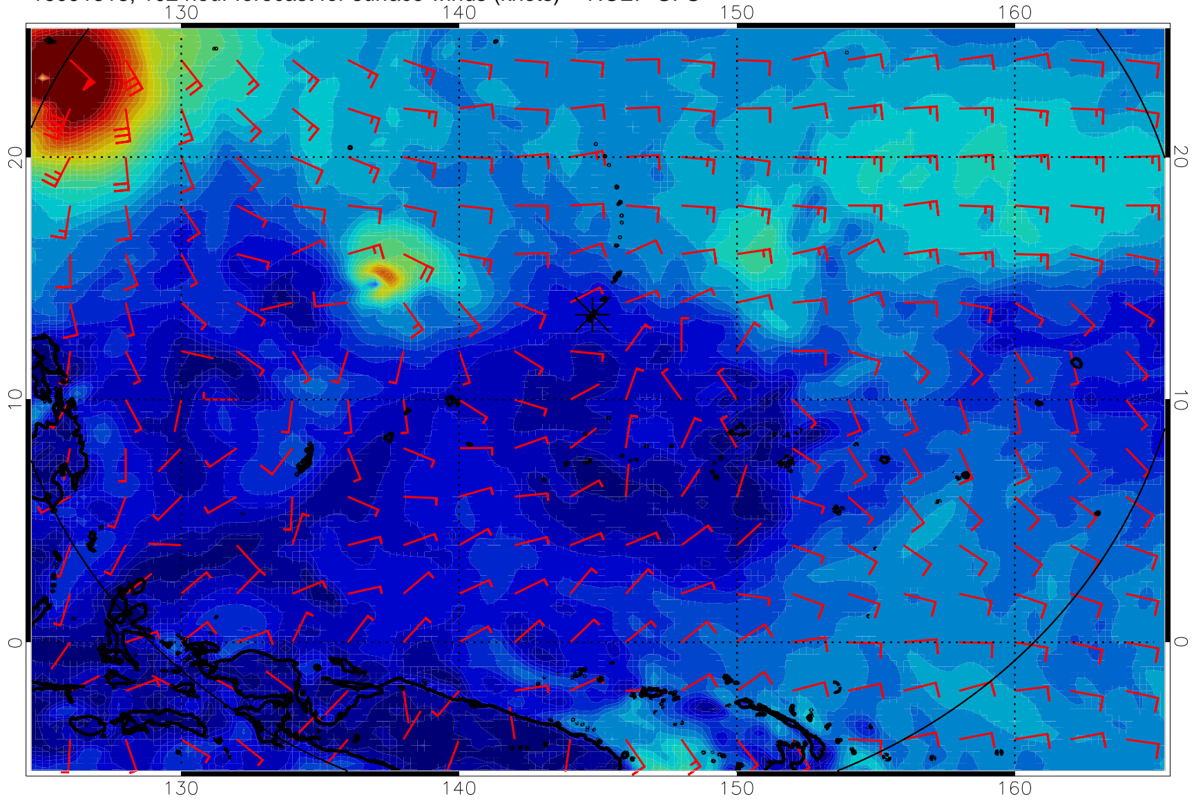
16091318, 102 hour forecast for surface winds (knots) -- NCEP GFS
