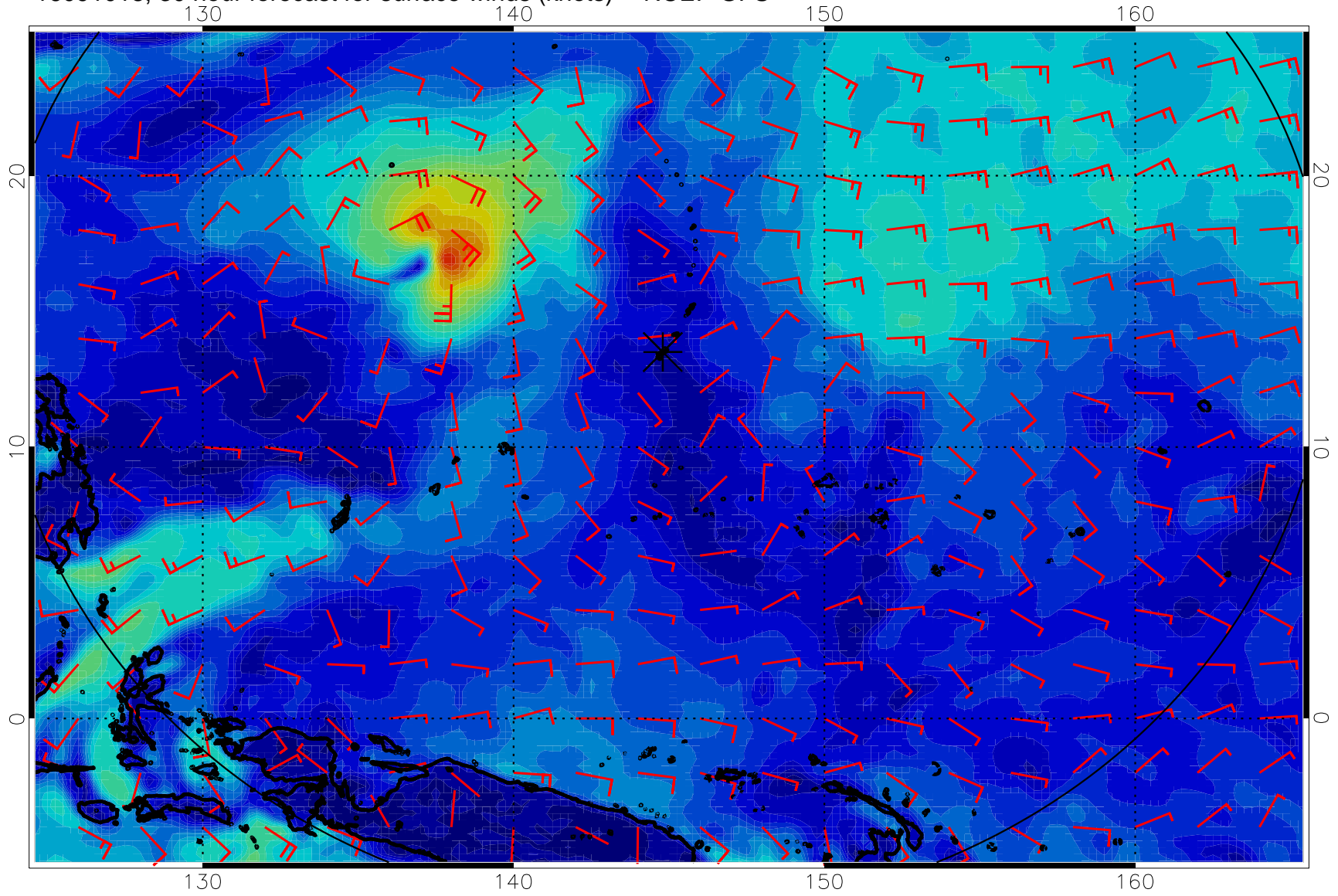
16091018, 30 hour forecast for surface winds (knots) -- NCEP GFS
