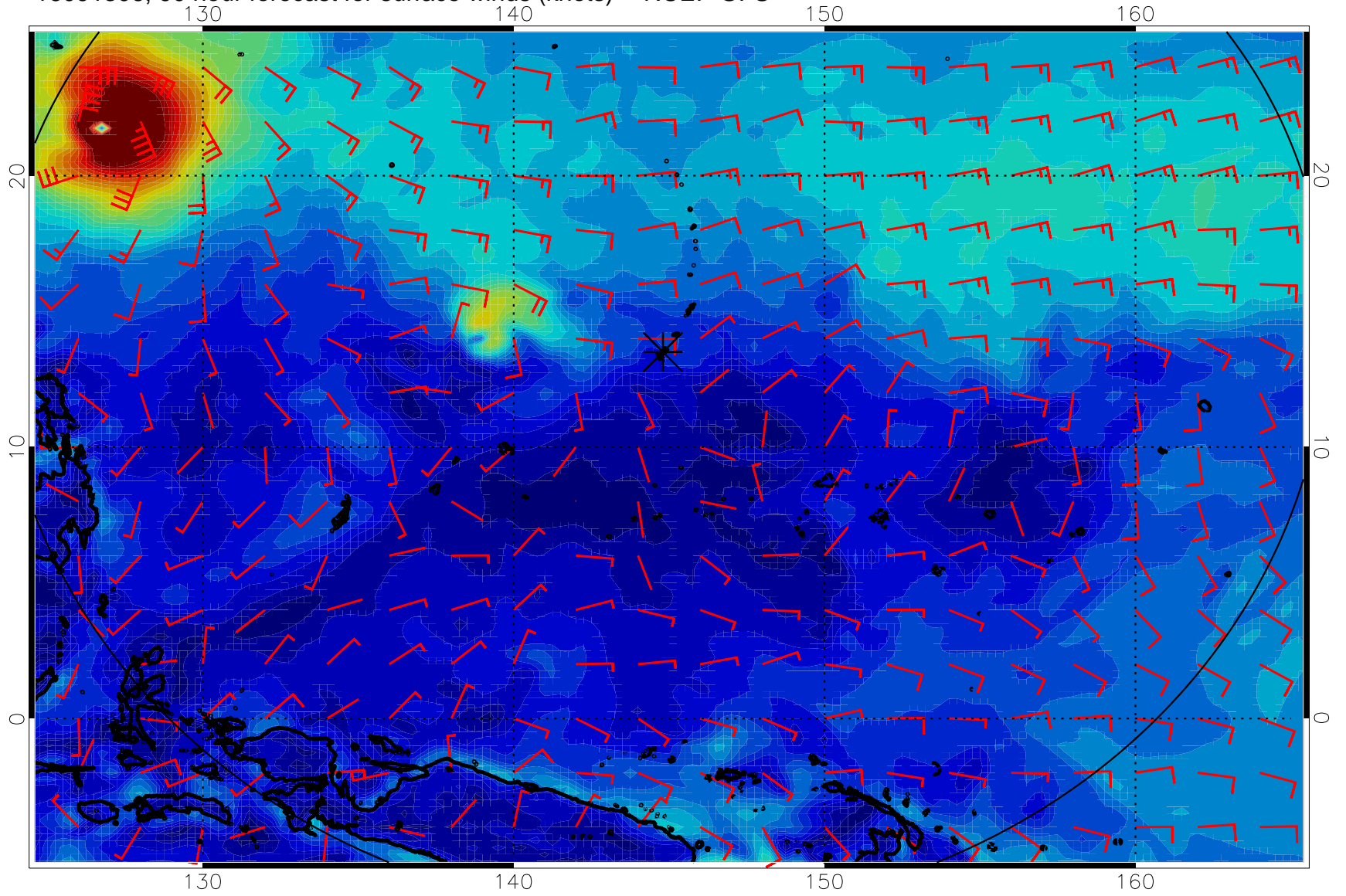
16091306, 90 hour forecast for surface winds (knots) -- NCEP GFS
