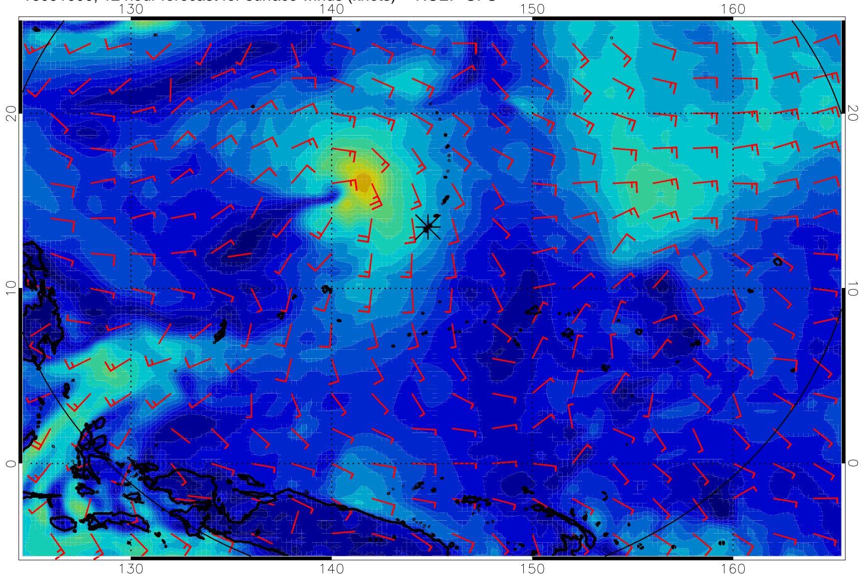
16091000, 12 hour forecast for surface winds (knots) -- NCEP GFS
