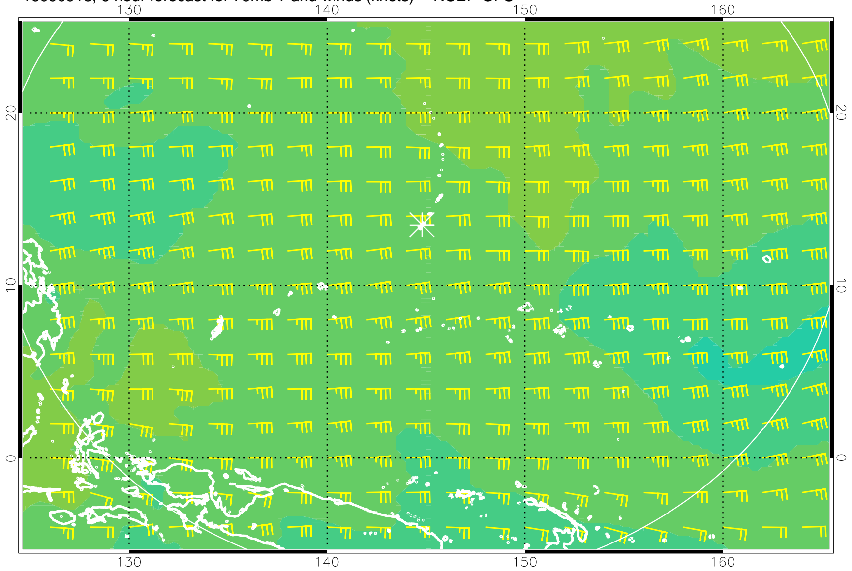
16090918, 6 hour forecast for 70mb T and winds (knots) -- NCEP GFS
