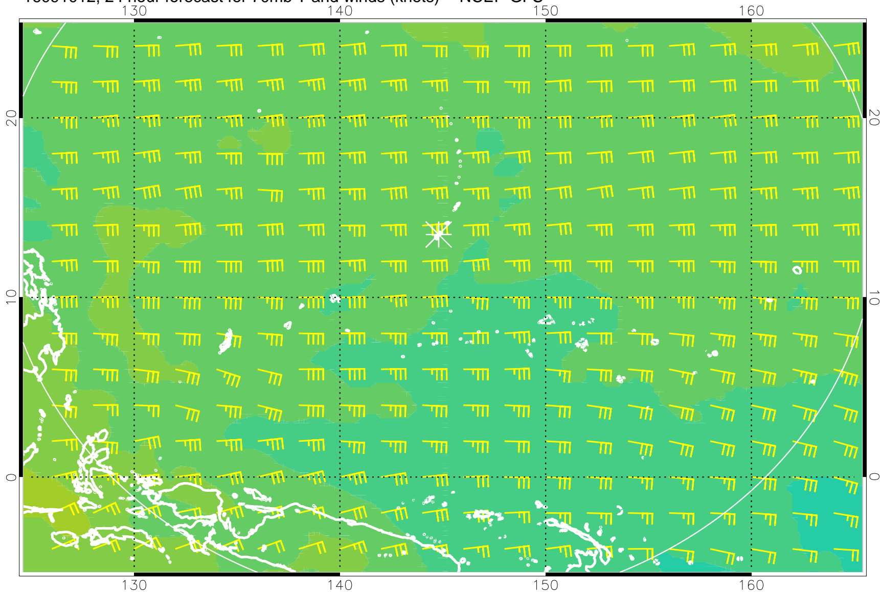
16091012, 24 hour forecast for 70mb T and winds (knots) -- NCEP GFS
