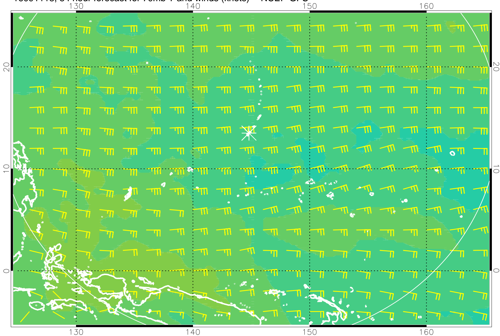
16091118, 54 hour forecast for 70mb T and winds (knots) -- NCEP GFS
