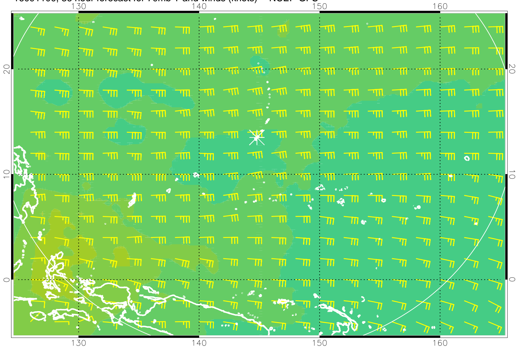
16091100, 36 hour forecast for 70mb T and winds (knots) -- NCEP GFS
