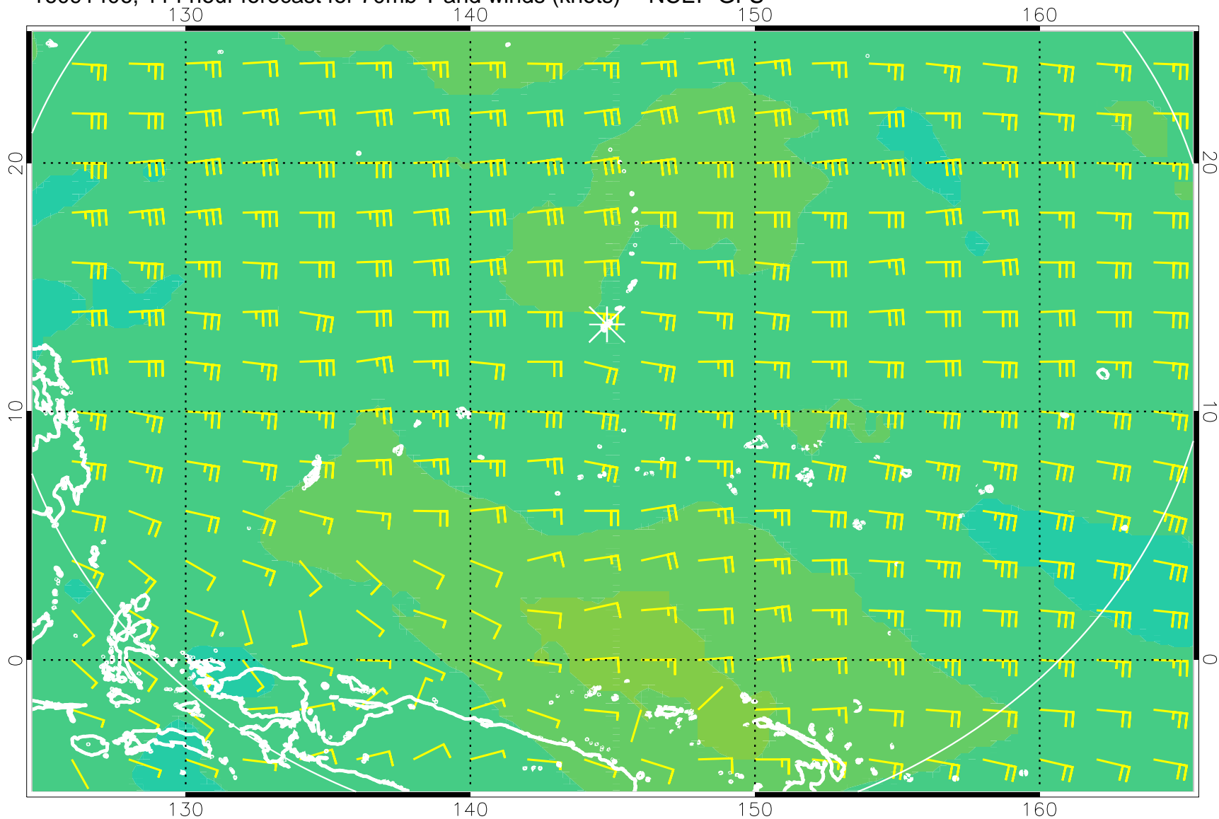
16091406, 114 hour forecast for 70mb T and winds (knots) -- NCEP GFS
