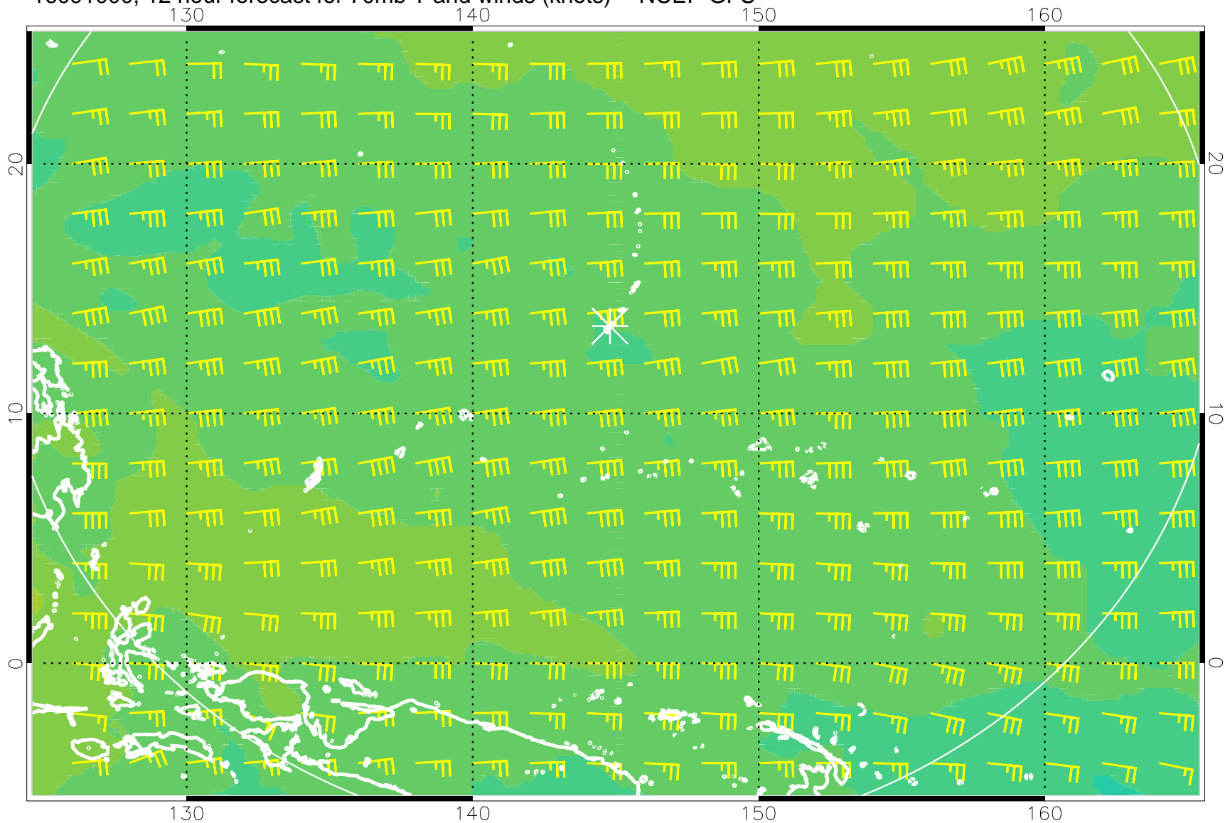
16091000, 12 hour forecast for 70mb T and winds (knots) -- NCEP GFS
