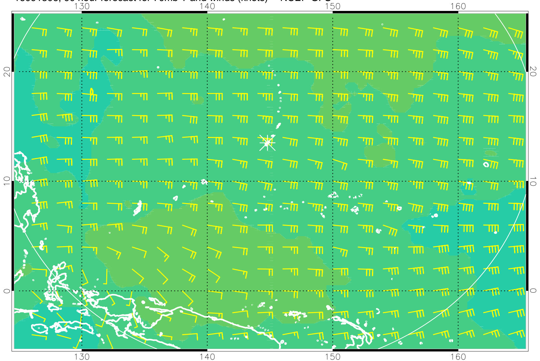
16091306, 90 hour forecast for 70mb T and winds (knots) -- NCEP GFS
