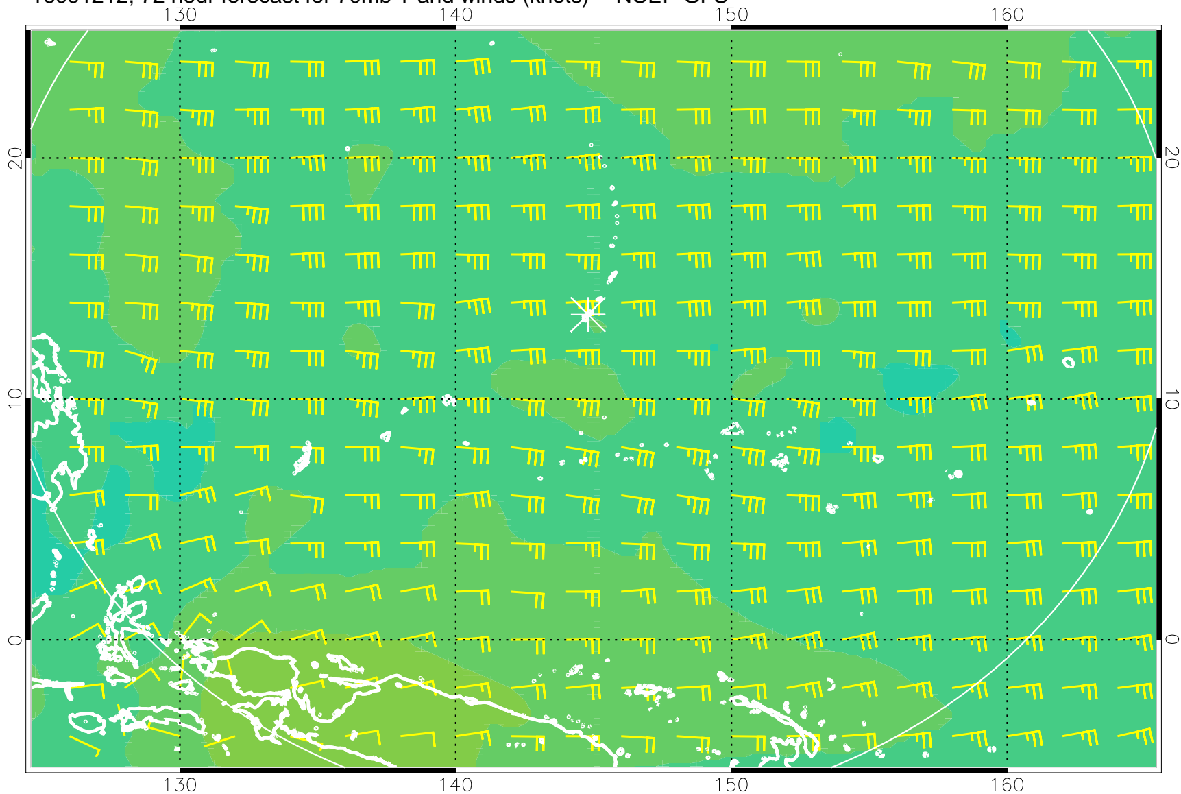
16091212, 72 hour forecast for 70mb T and winds (knots) -- NCEP GFS
