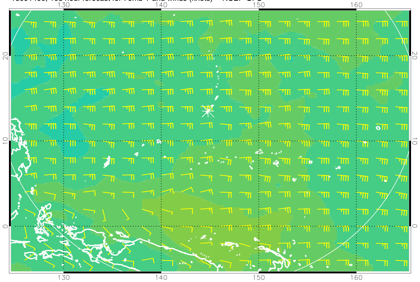
16091400, 108 hour forecast for 70mb T and winds (knots) -- NCEP GFS
