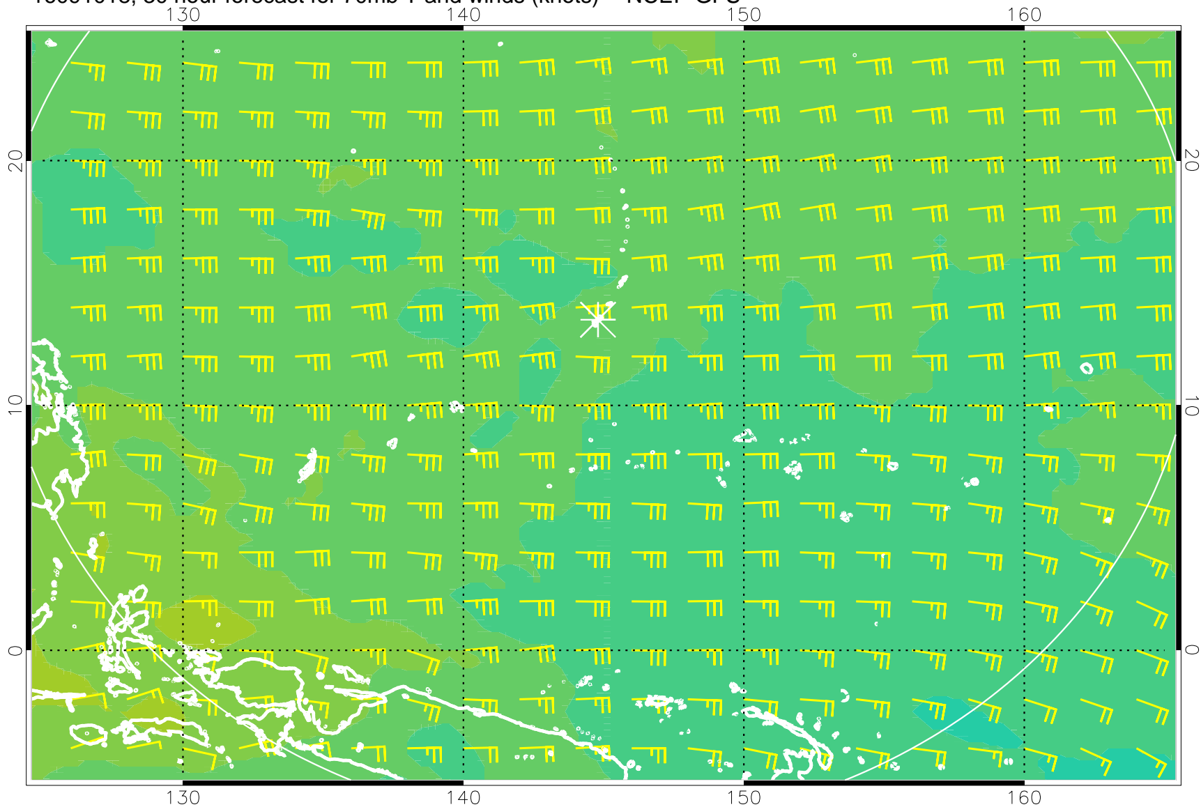
16091018, 30 hour forecast for 70mb T and winds (knots) -- NCEP GFS
