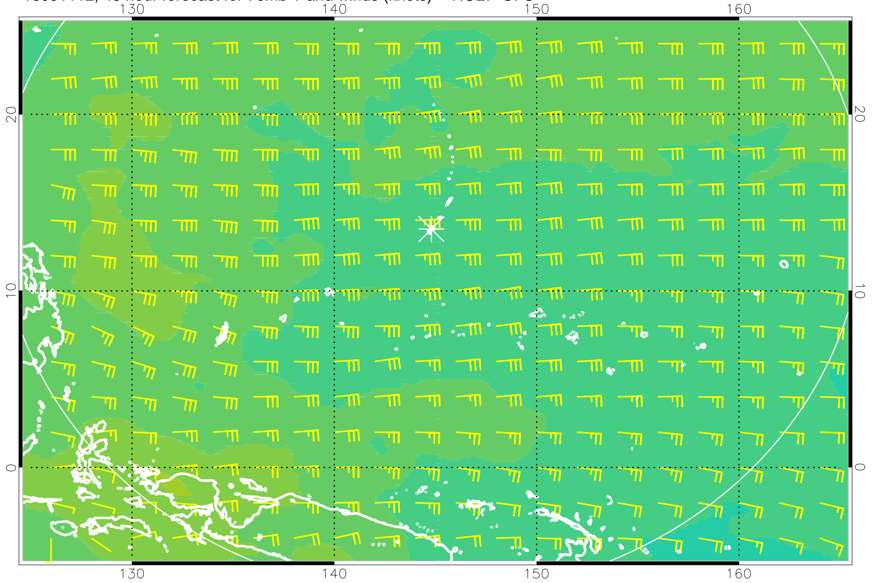
16091112, 48 hour forecast for 70mb T and winds (knots) -- NCEP GFS
