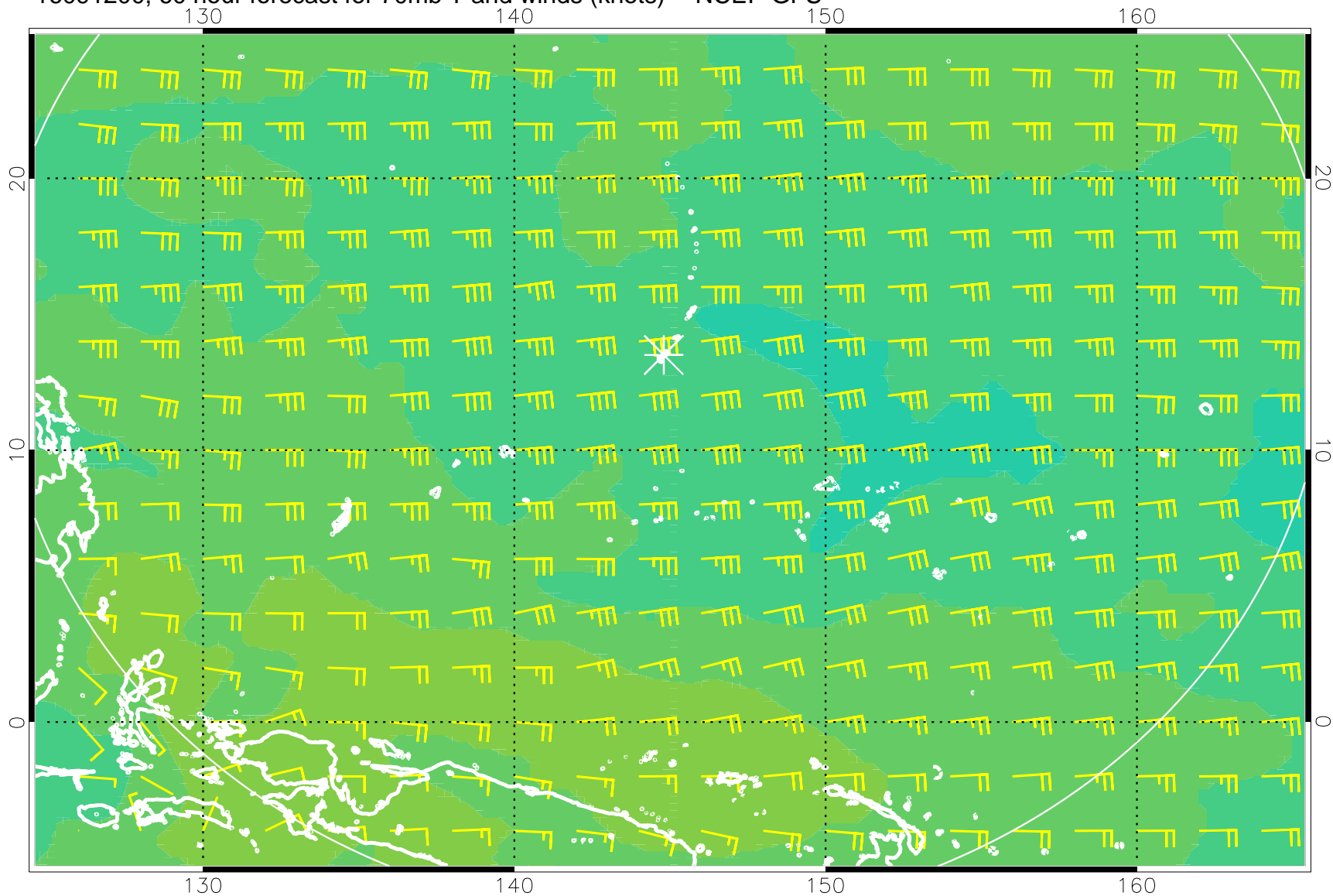
16091200, 60 hour forecast for 70mb T and winds (knots) -- NCEP GFS
