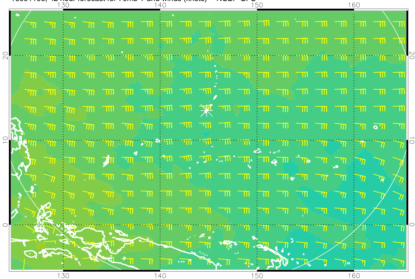
16091106, 42 hour forecast for 70mb T and winds (knots) -- NCEP GFS
