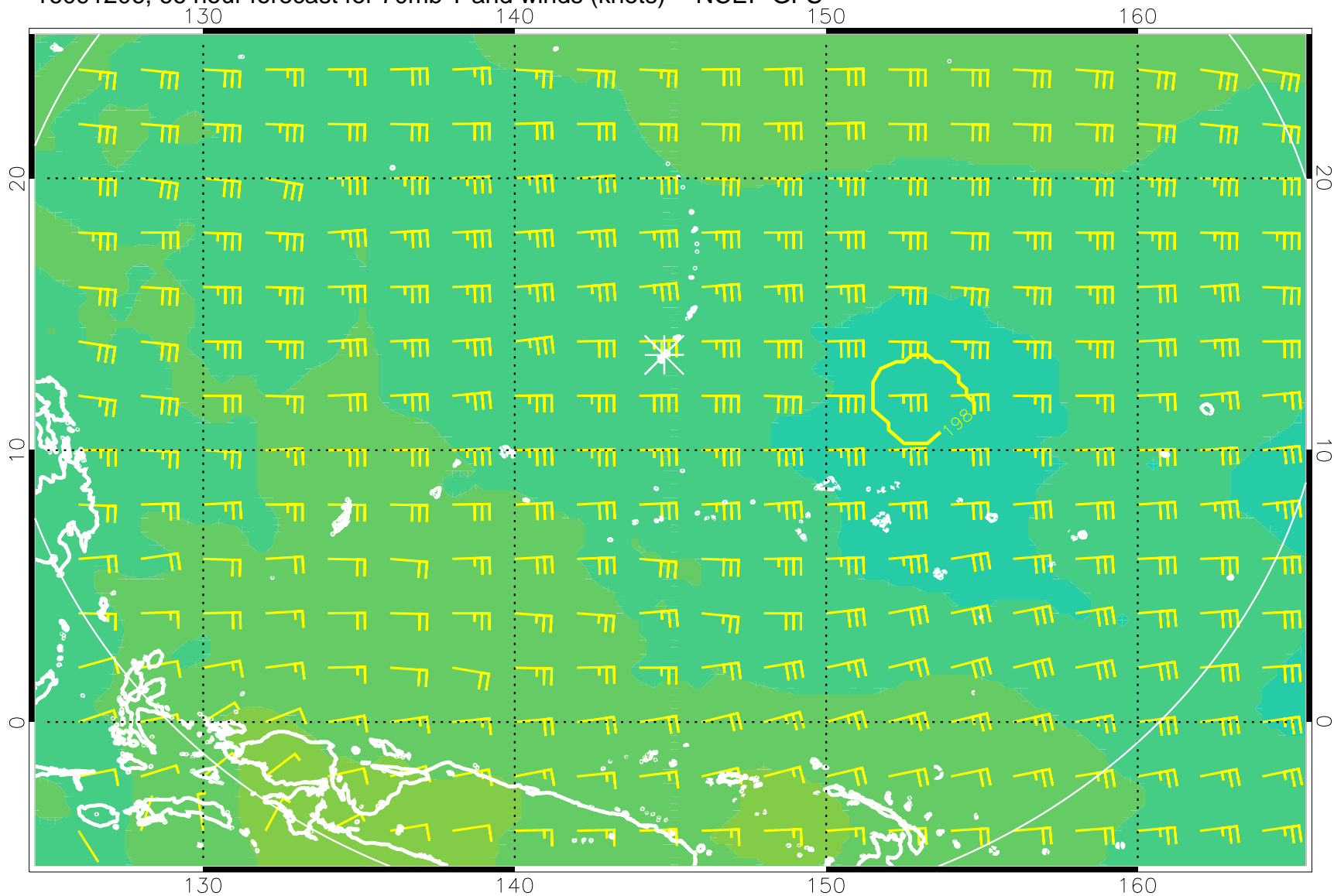
16091206, 66 hour forecast for 70mb T and winds (knots) -- NCEP GFS
