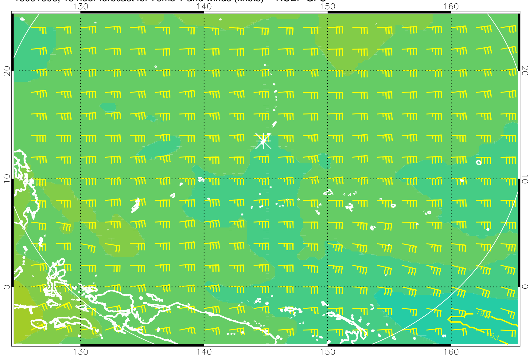
16091006, 18 hour forecast for 70mb T and winds (knots) -- NCEP GFS
