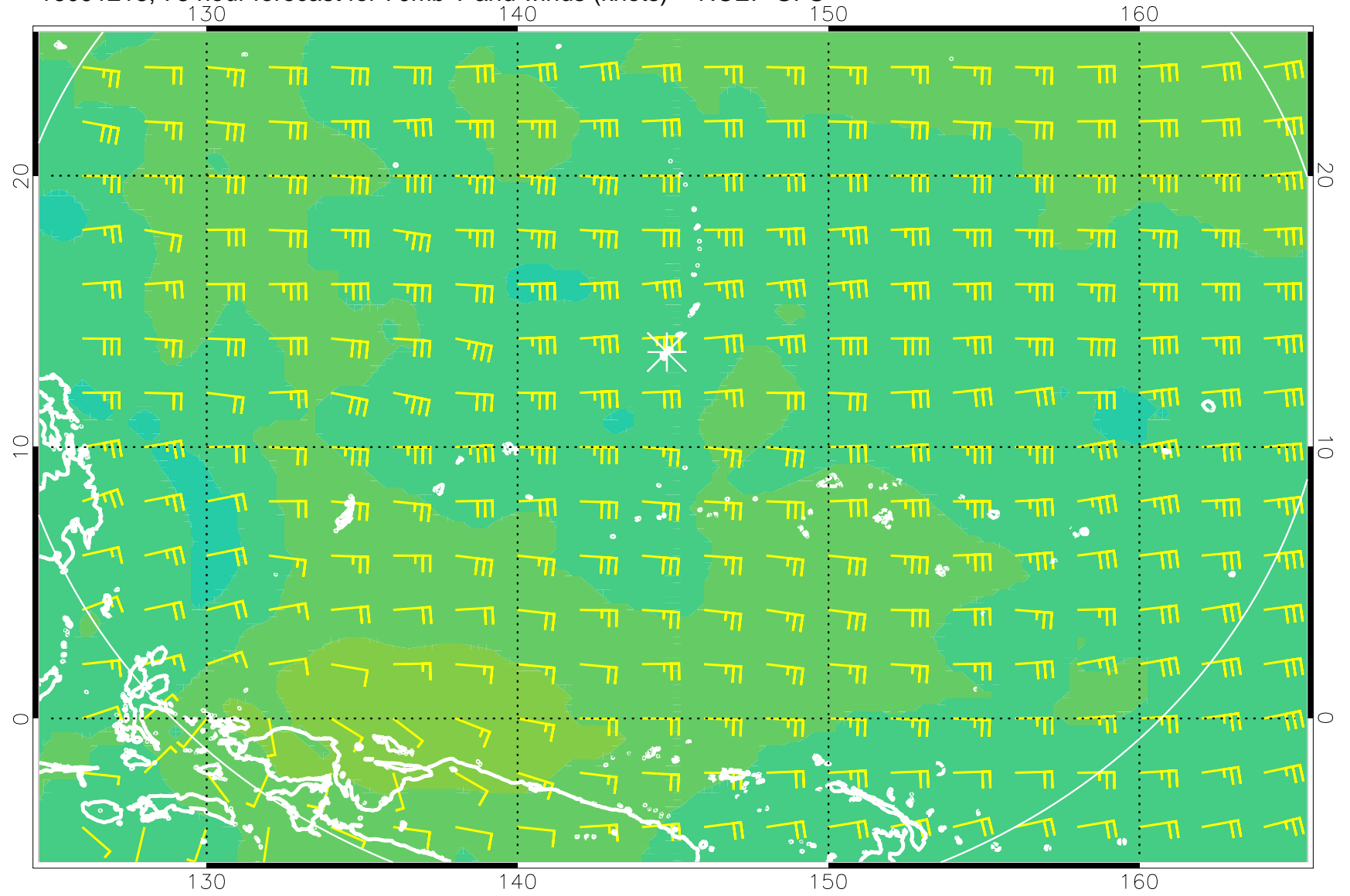
16091218, 78 hour forecast for 70mb T and winds (knots) -- NCEP GFS
