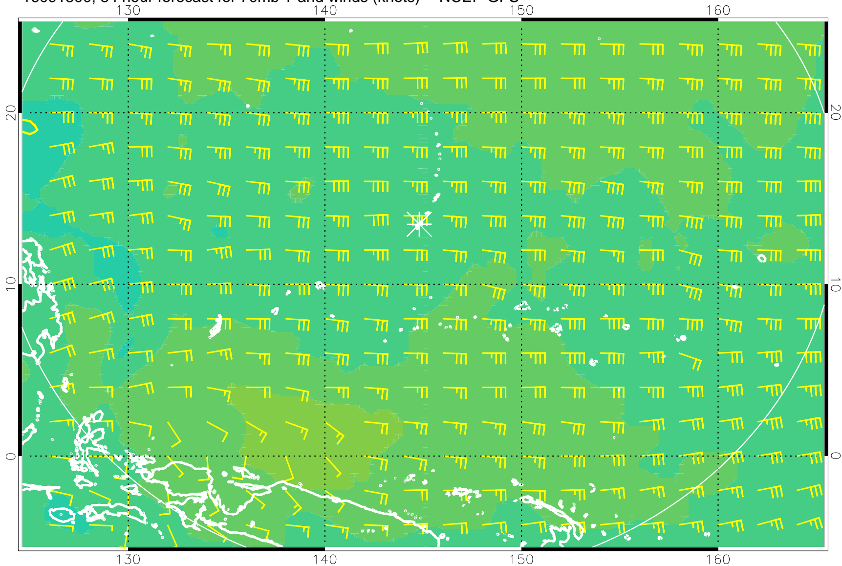
16091300, 84 hour forecast for 70mb T and winds (knots) -- NCEP GFS
