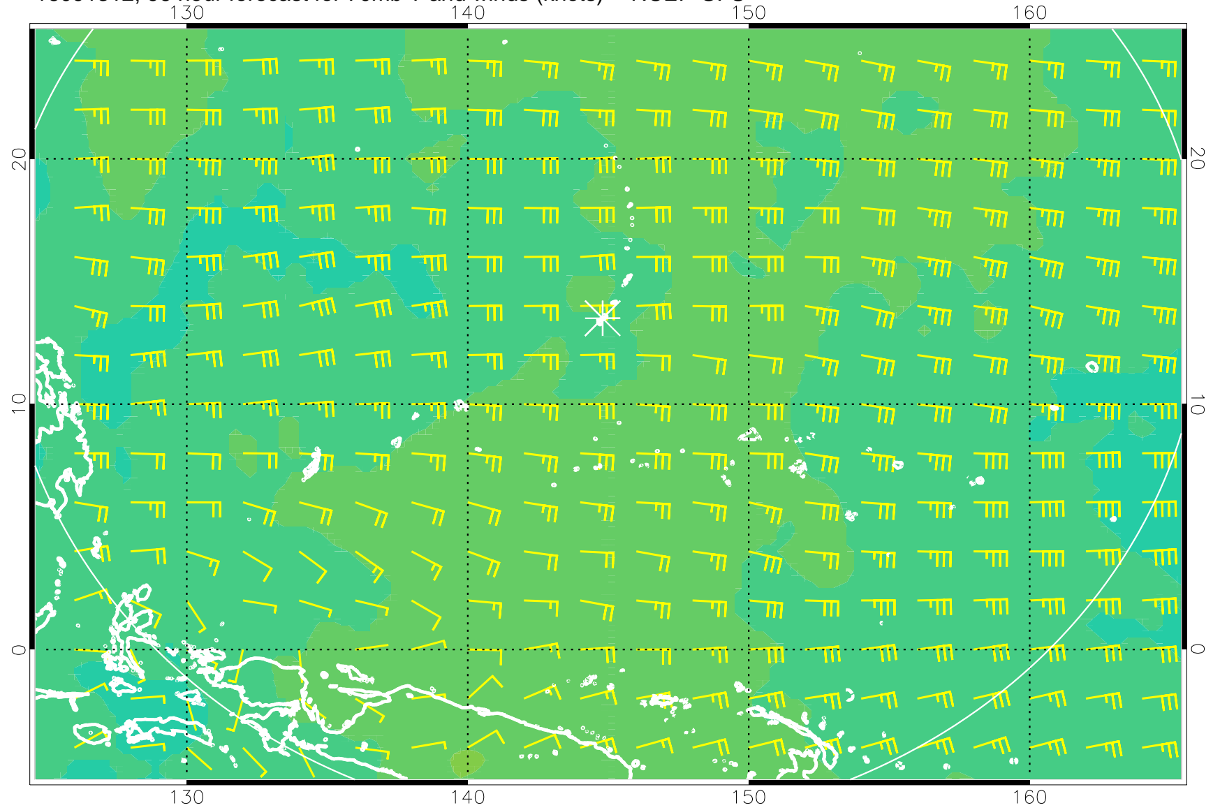
16091312, 96 hour forecast for 70mb T and winds (knots) -- NCEP GFS
