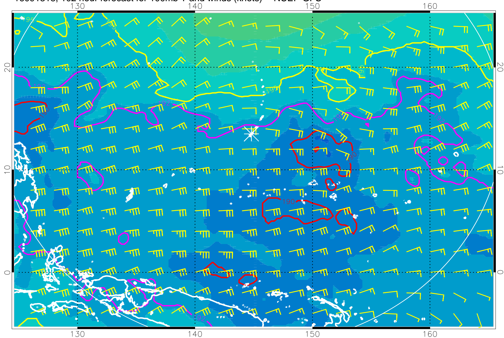
16091318, 102 hour forecast for 100mb T and winds (knots) -- NCEP GFS
