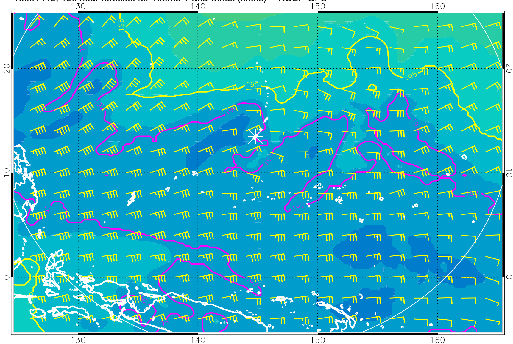
16091412, 120 hour forecast for 100mb T and winds (knots) -- NCEP GFS
