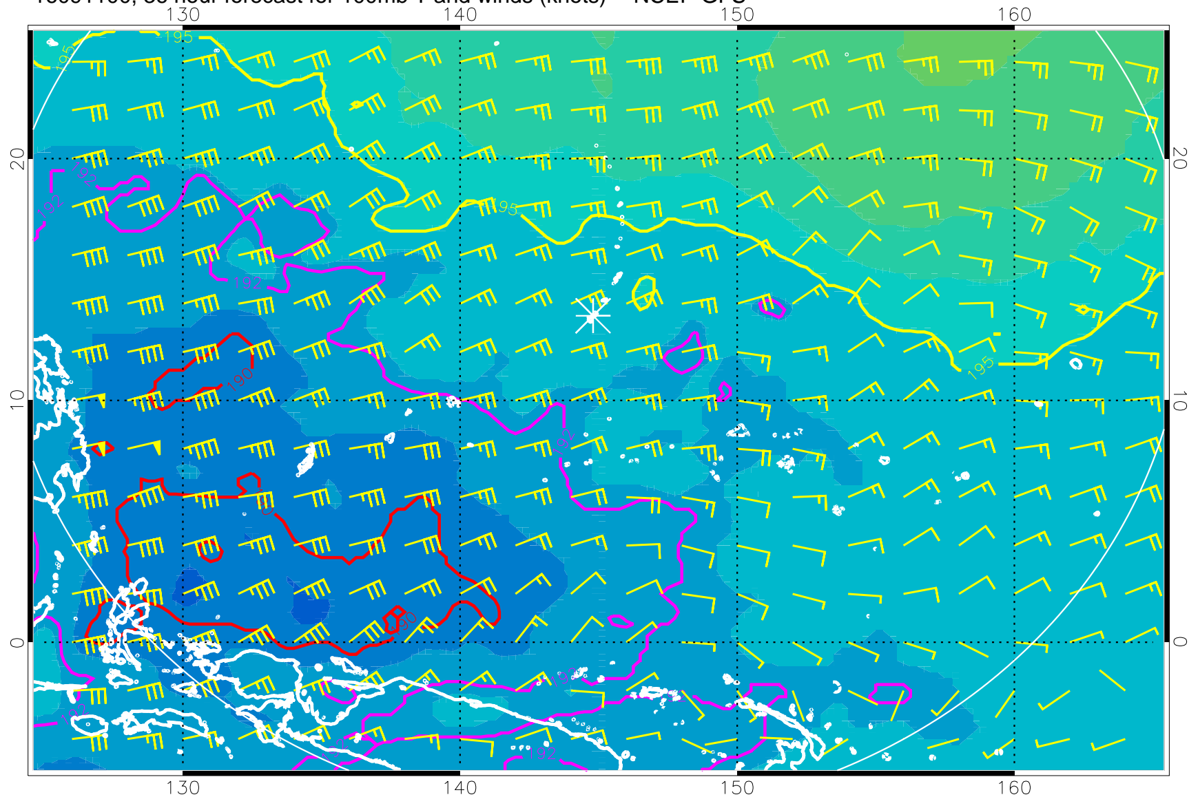
16091100, 36 hour forecast for 100mb T and winds (knots) -- NCEP GFS
