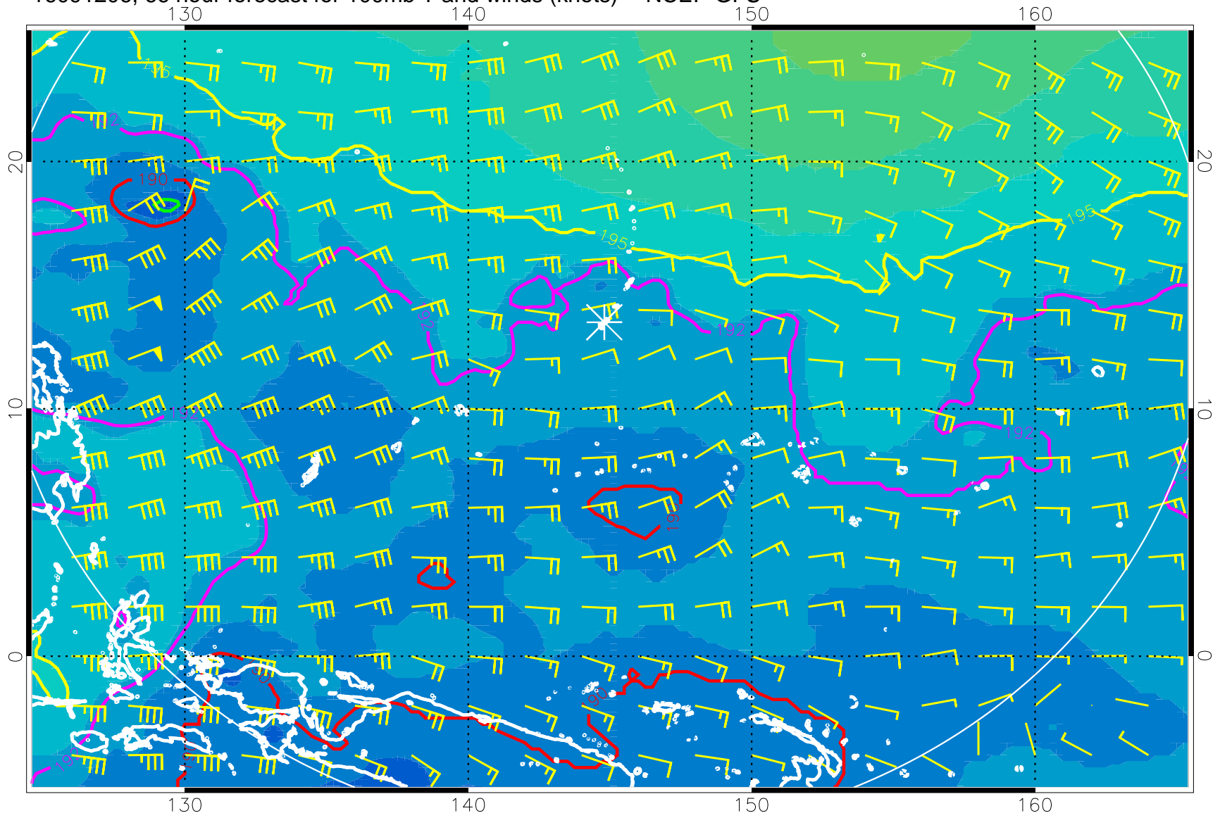
16091206, 66 hour forecast for 100mb T and winds (knots) -- NCEP GFS
