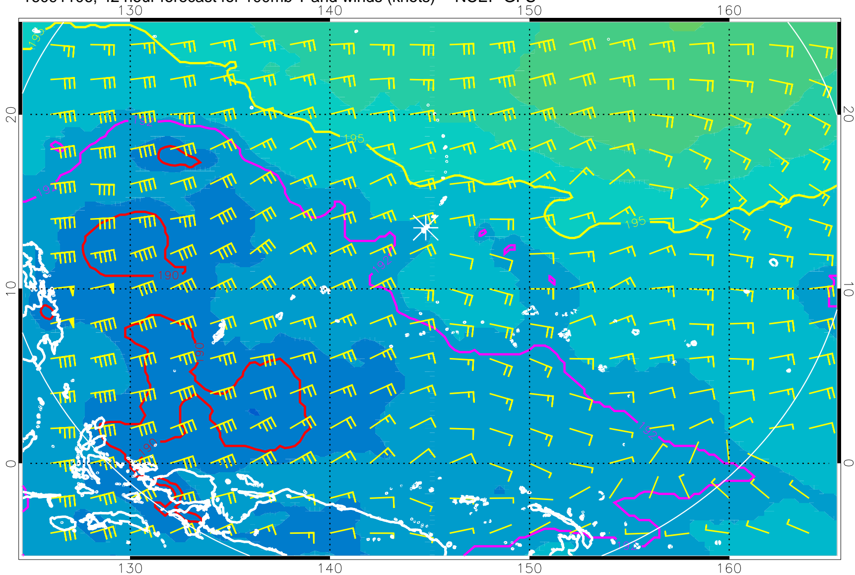
16091106, 42 hour forecast for 100mb T and winds (knots) -- NCEP GFS
