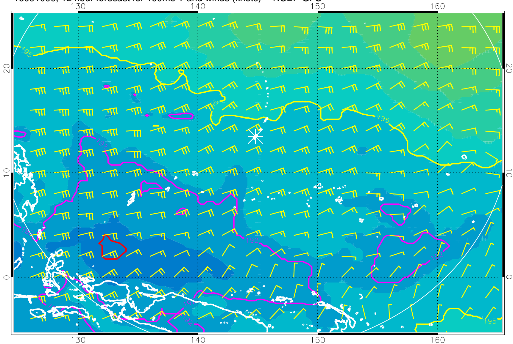
16091000, 12 hour forecast for 100mb T and winds (knots) -- NCEP GFS
