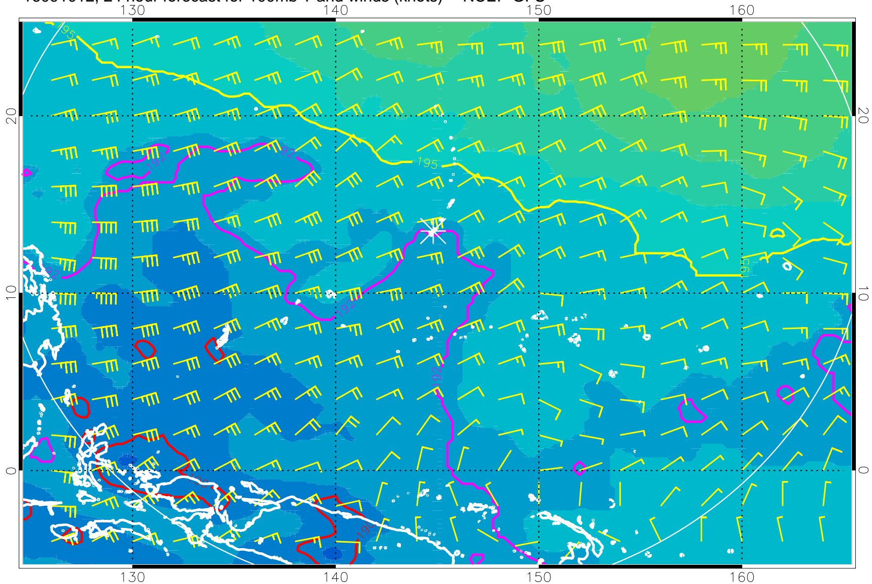
16091012, 24 hour forecast for 100mb T and winds (knots) -- NCEP GFS
