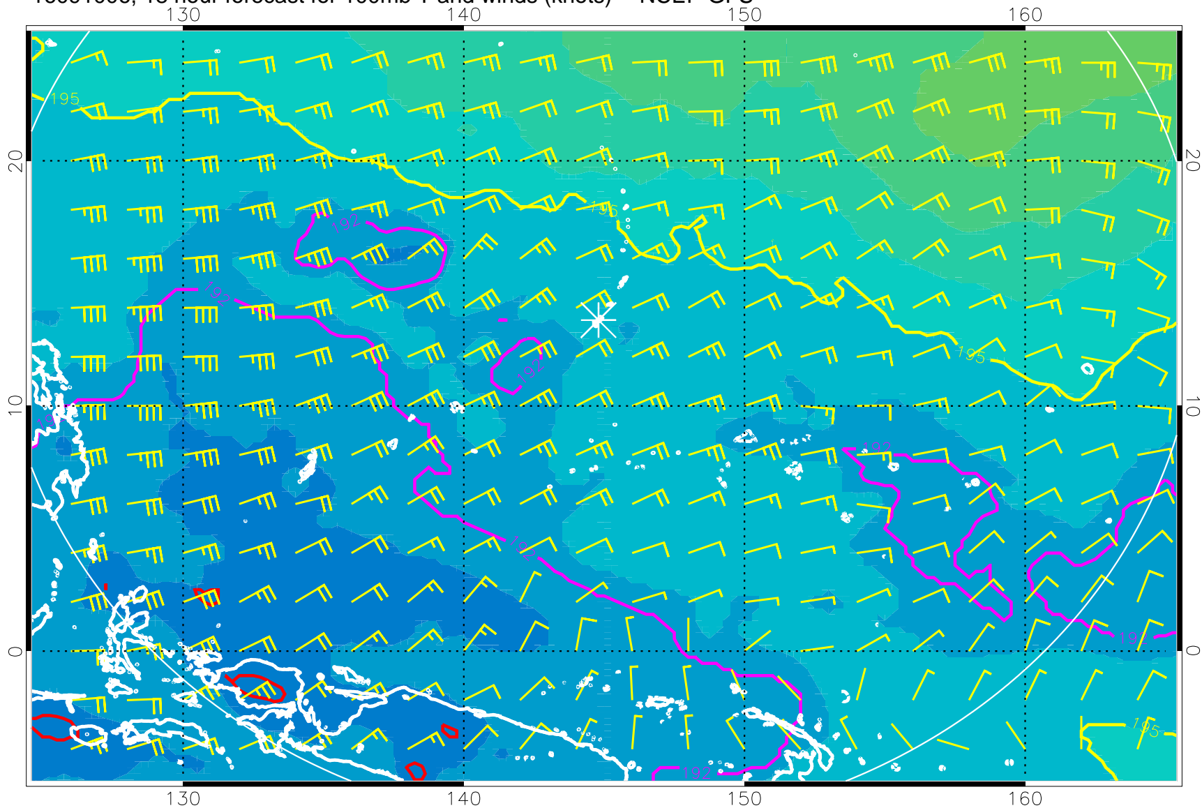
16091006, 18 hour forecast for 100mb T and winds (knots) -- NCEP GFS
