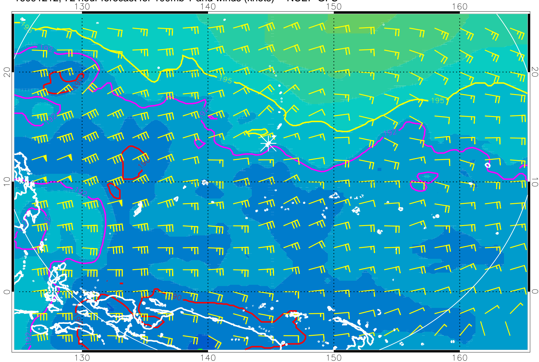
16091212, 72 hour forecast for 100mb T and winds (knots) -- NCEP GFS
