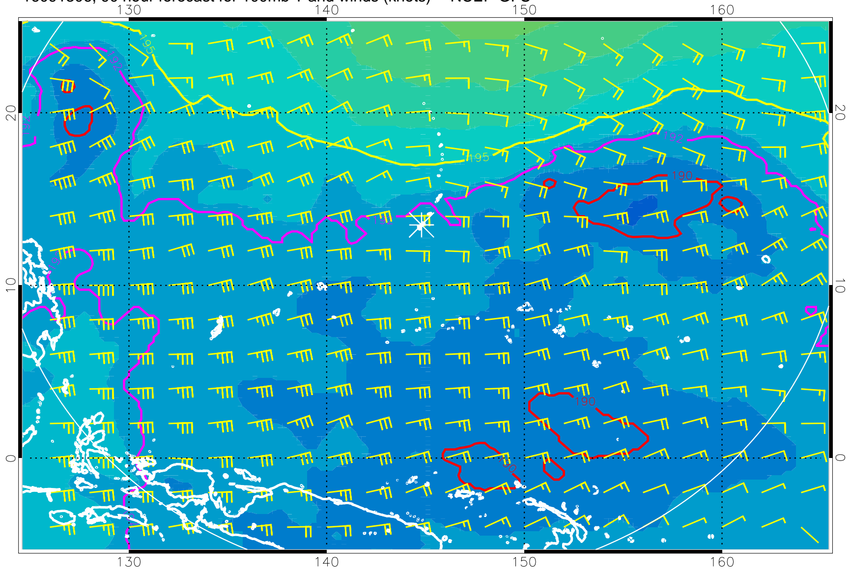
16091306, 90 hour forecast for 100mb T and winds (knots) -- NCEP GFS
