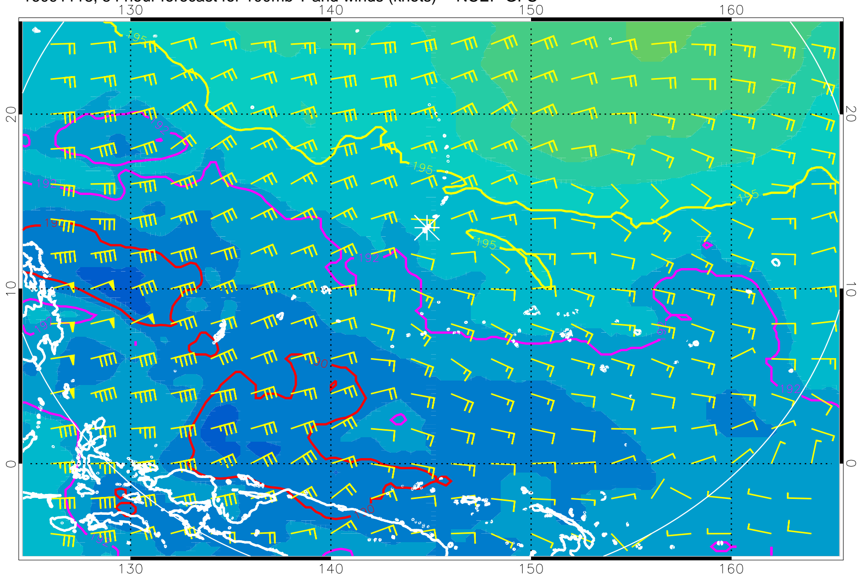
16091118, 54 hour forecast for 100mb T and winds (knots) -- NCEP GFS
