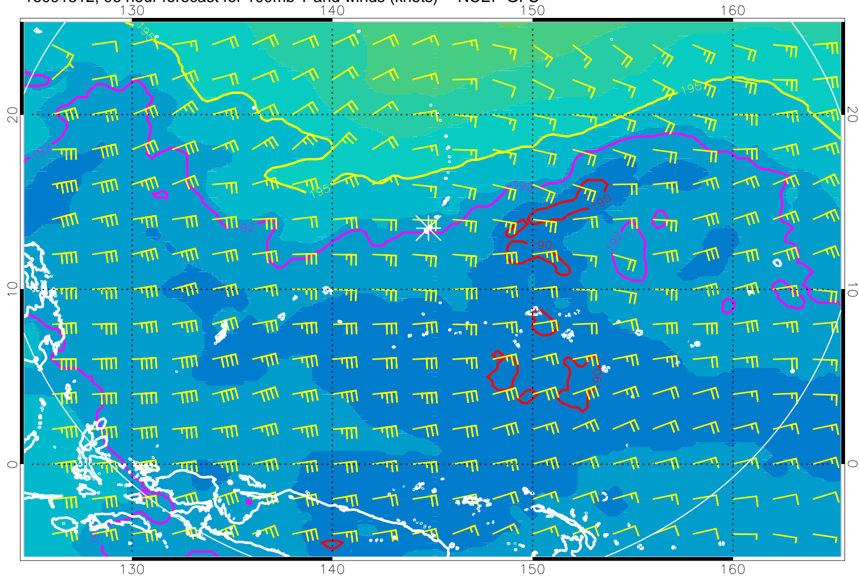
16091312, 96 hour forecast for 100mb T and winds (knots) -- NCEP GFS
