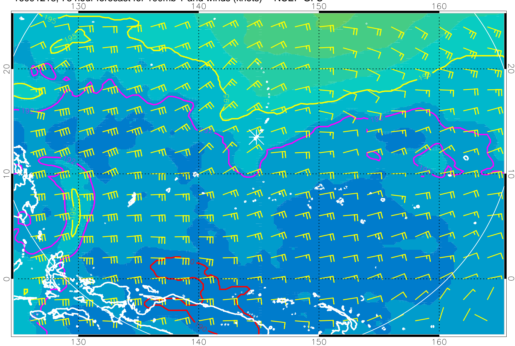
16091218, 78 hour forecast for 100mb T and winds (knots) -- NCEP GFS
