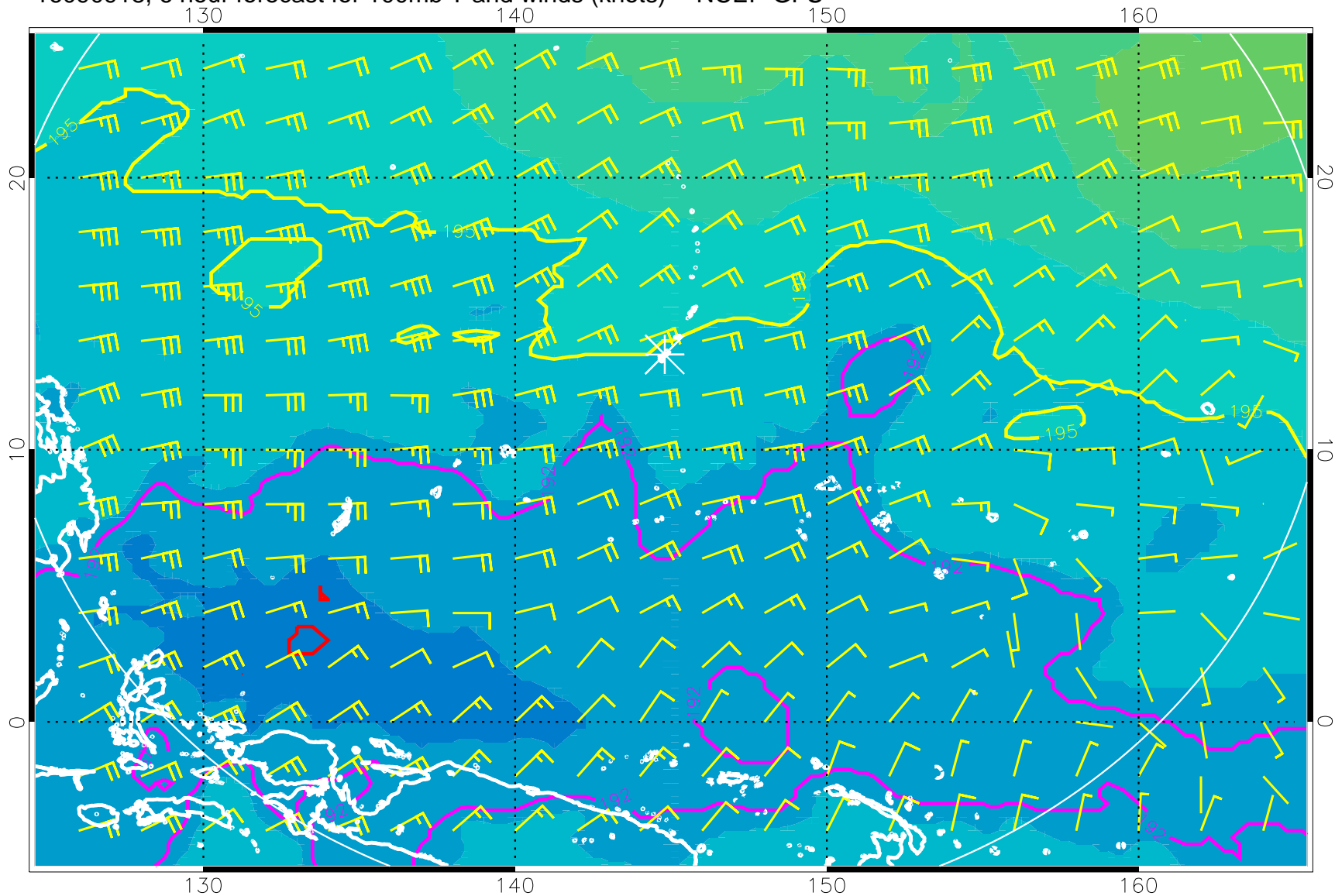
16090918, 6 hour forecast for 100mb T and winds (knots) -- NCEP GFS
