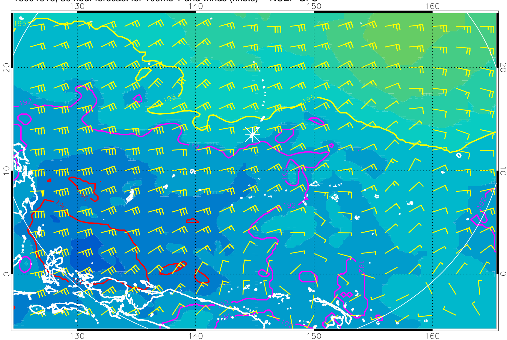
16091018, 30 hour forecast for 100mb T and winds (knots) -- NCEP GFS
