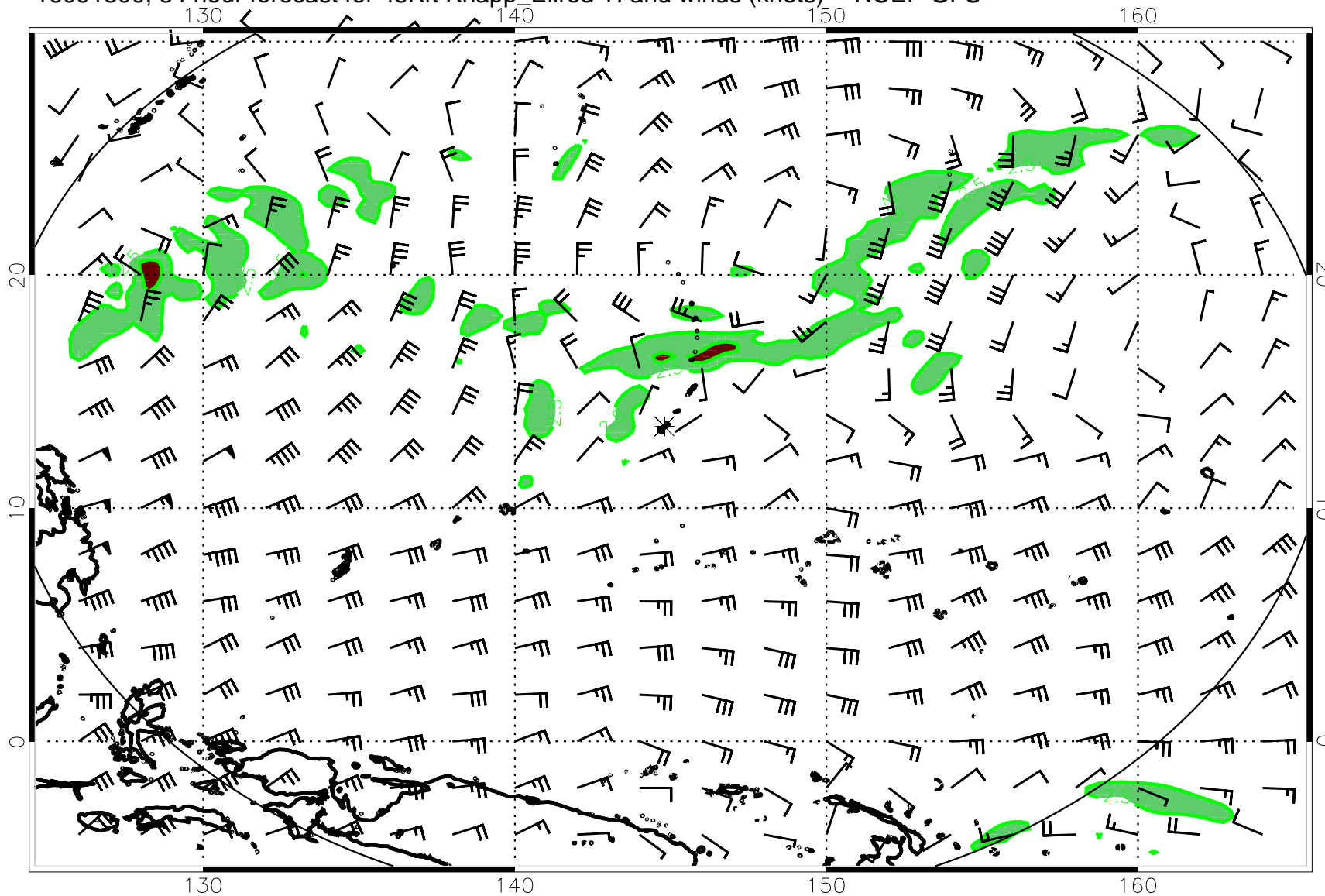
16091300, 84 hour forecast for 45Kft Knapp_Ellrod TI and winds (knots) -- NCEP GFS
