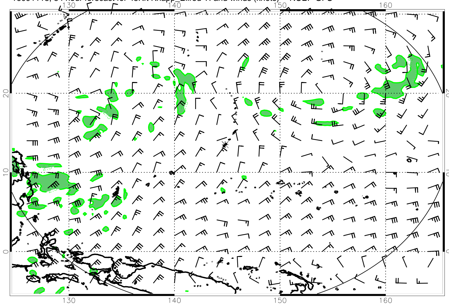
16091118, 54 hour forecast for 45Kft Knapp_Ellrod TI and winds (knots) -- NCEP GFS
