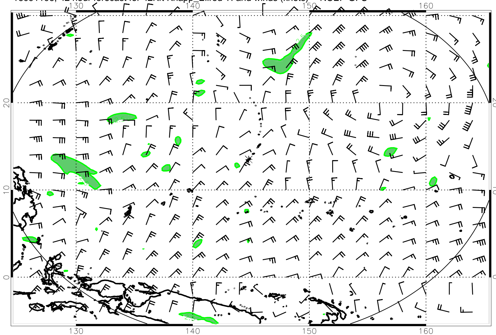
16091106, 42 hour forecast for 42Kft Knapp_Ellrod TI and winds (knots) -- NCEP GFS
