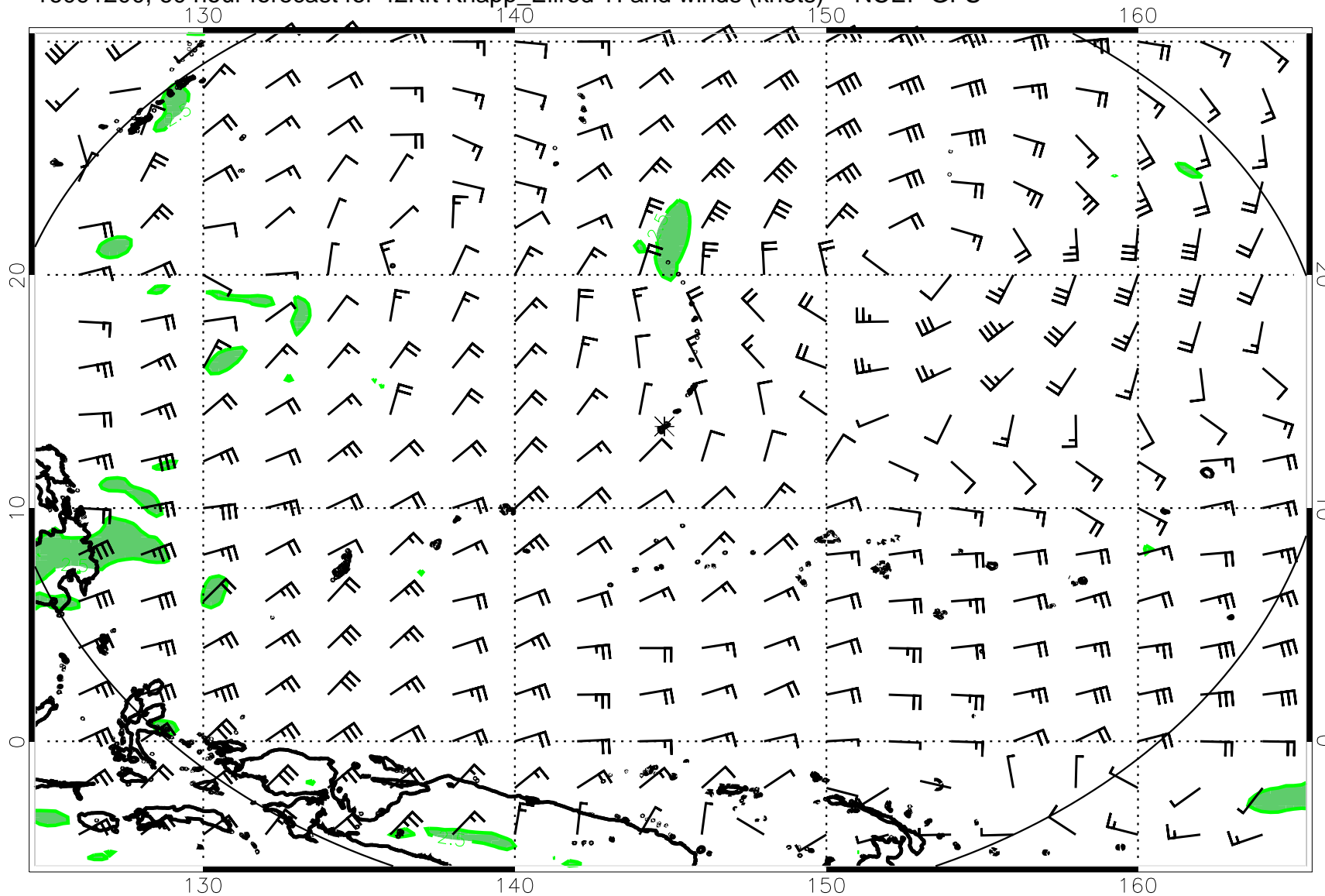
16091200, 60 hour forecast for 42Kft Knapp_Ellrod TI and winds (knots) -- NCEP GFS
