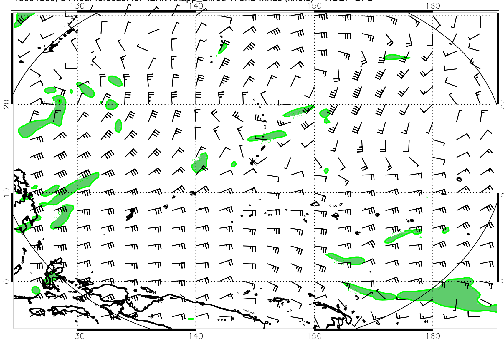
16091300, 84 hour forecast for 42Kft Knapp_Ellrod TI and winds (knots) -- NCEP GFS
