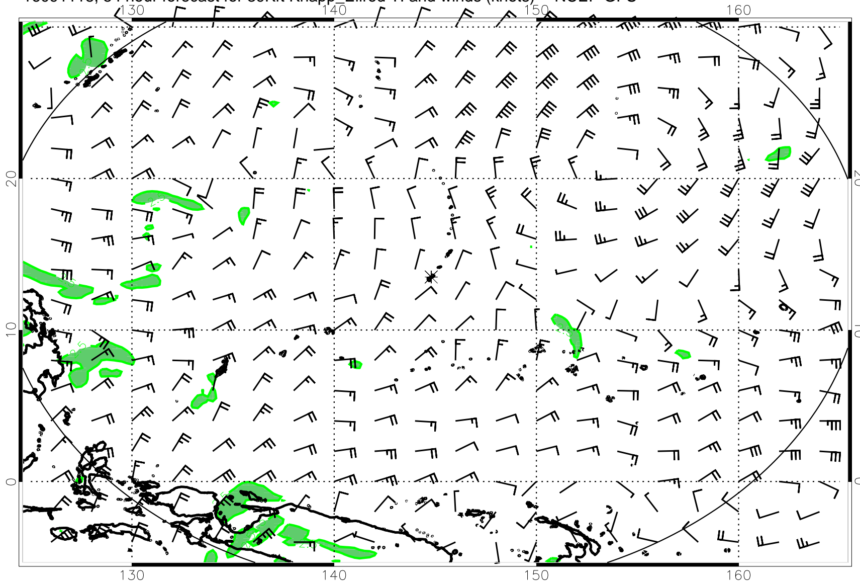
16091118, 54 hour forecast for 39Kft Knapp_Ellrod TI and winds (knots) -- NCEP GFS
