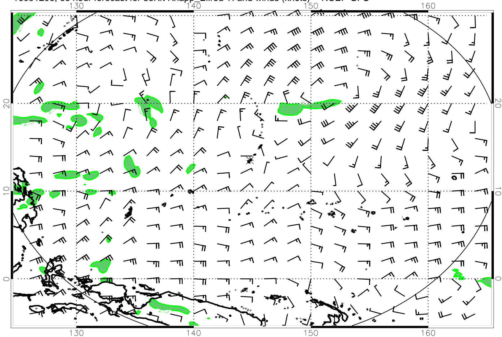
16091206, 66 hour forecast for 36Kft Knapp_Ellrod TI and winds (knots) -- NCEP GFS
