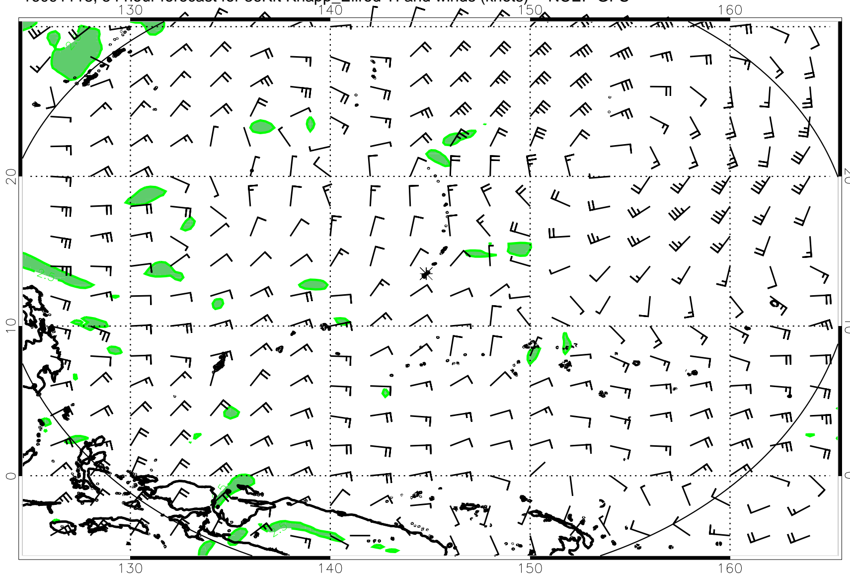
16091118, 54 hour forecast for 36Kft Knapp_Ellrod TI and winds (knots) -- NCEP GFS
