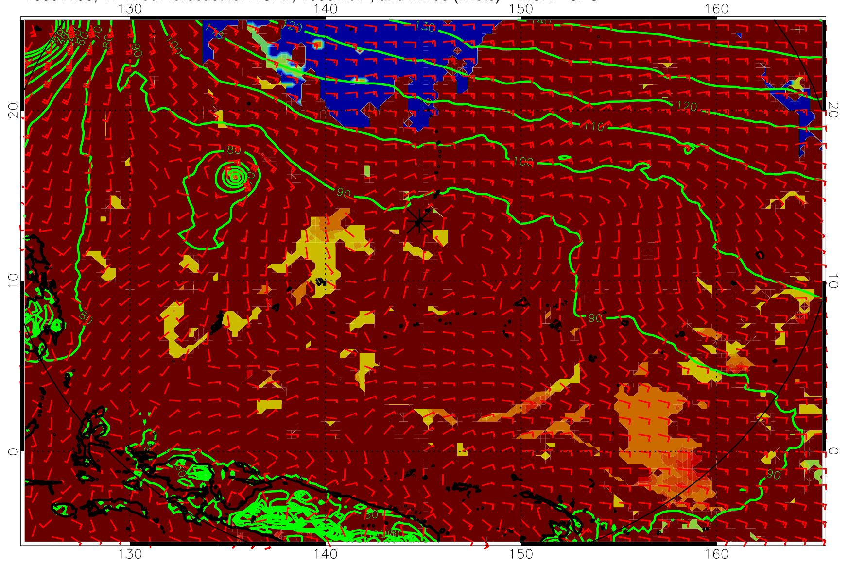
16091406, 114 hour forecast for HCAL, 1000mb Z, and winds (knots) -- NCEP GFS
