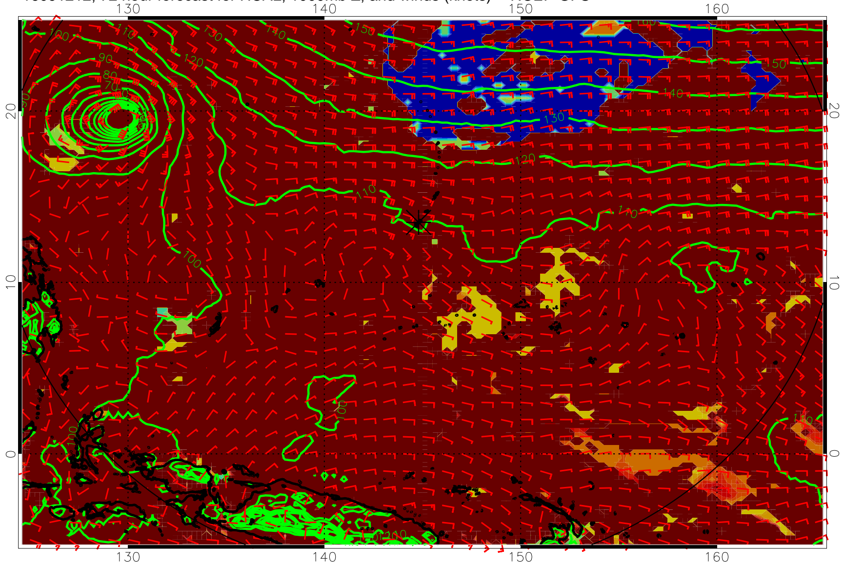
16091212, 72 hour forecast for HCAL, 1000mb Z, and winds (knots) -- NCEP GFS
