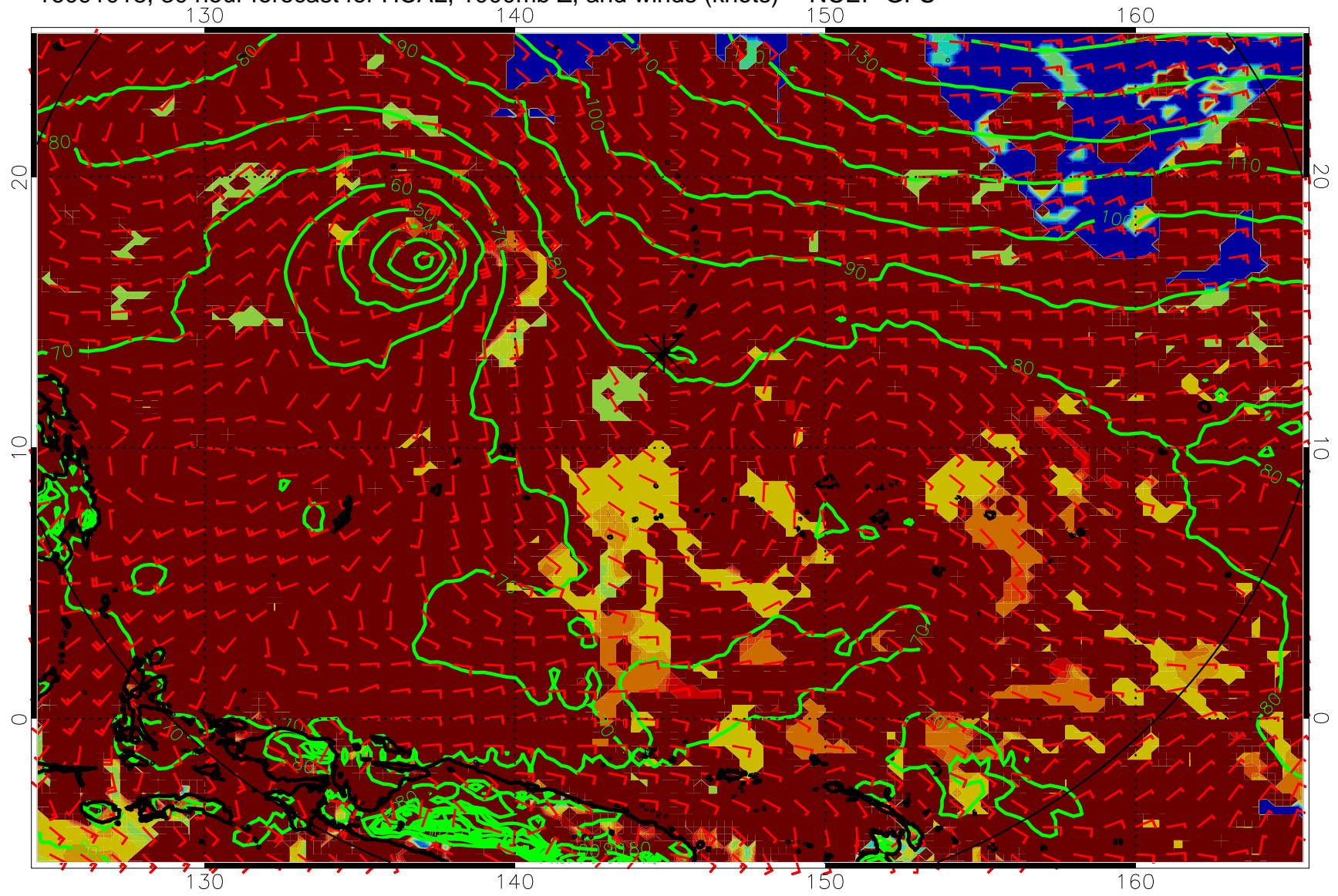
16091018, 30 hour forecast for HCAL, 1000mb Z, and winds (knots) -- NCEP GFS
