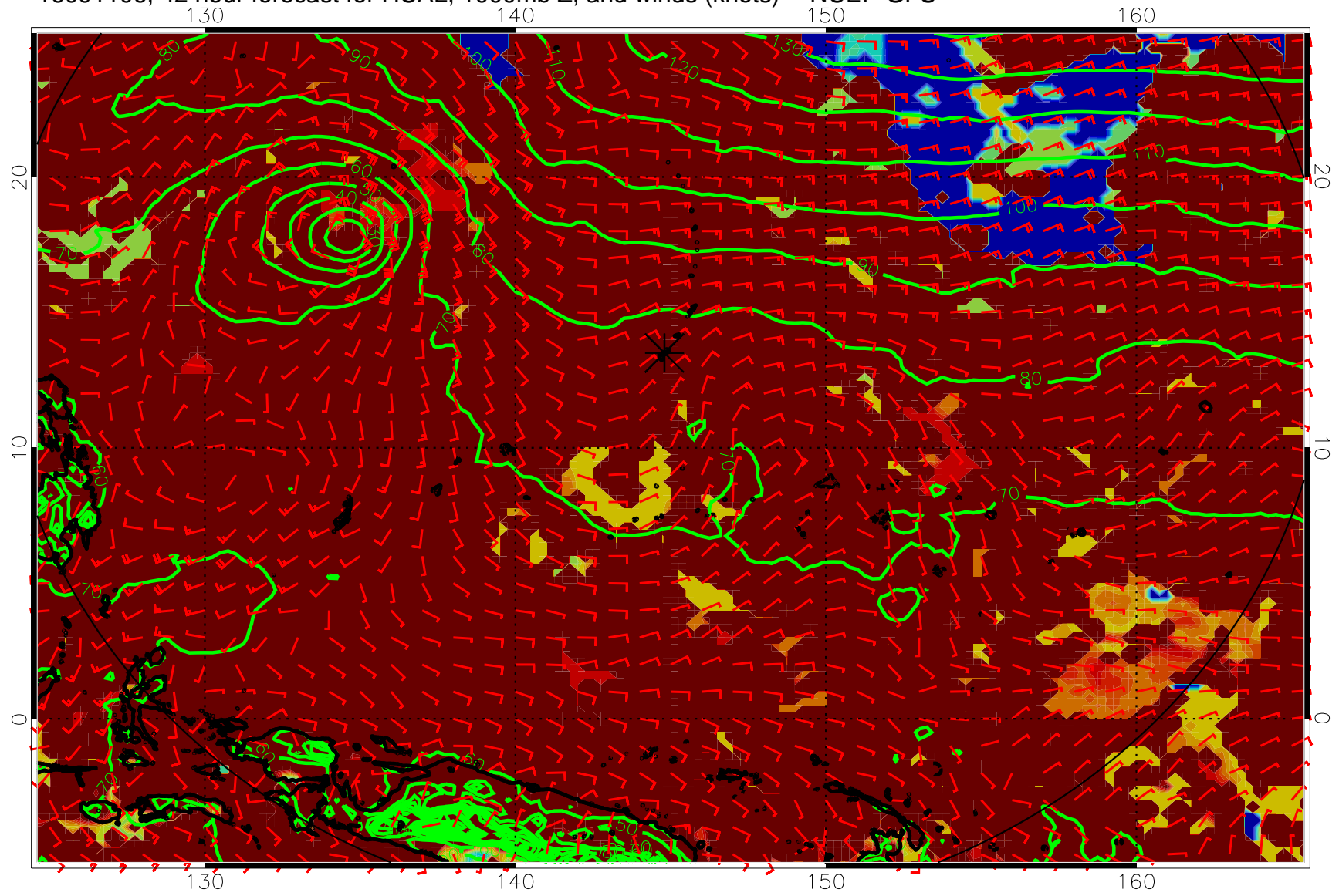
16091106, 42 hour forecast for HCAL, 1000mb Z, and winds (knots) -- NCEP GFS
