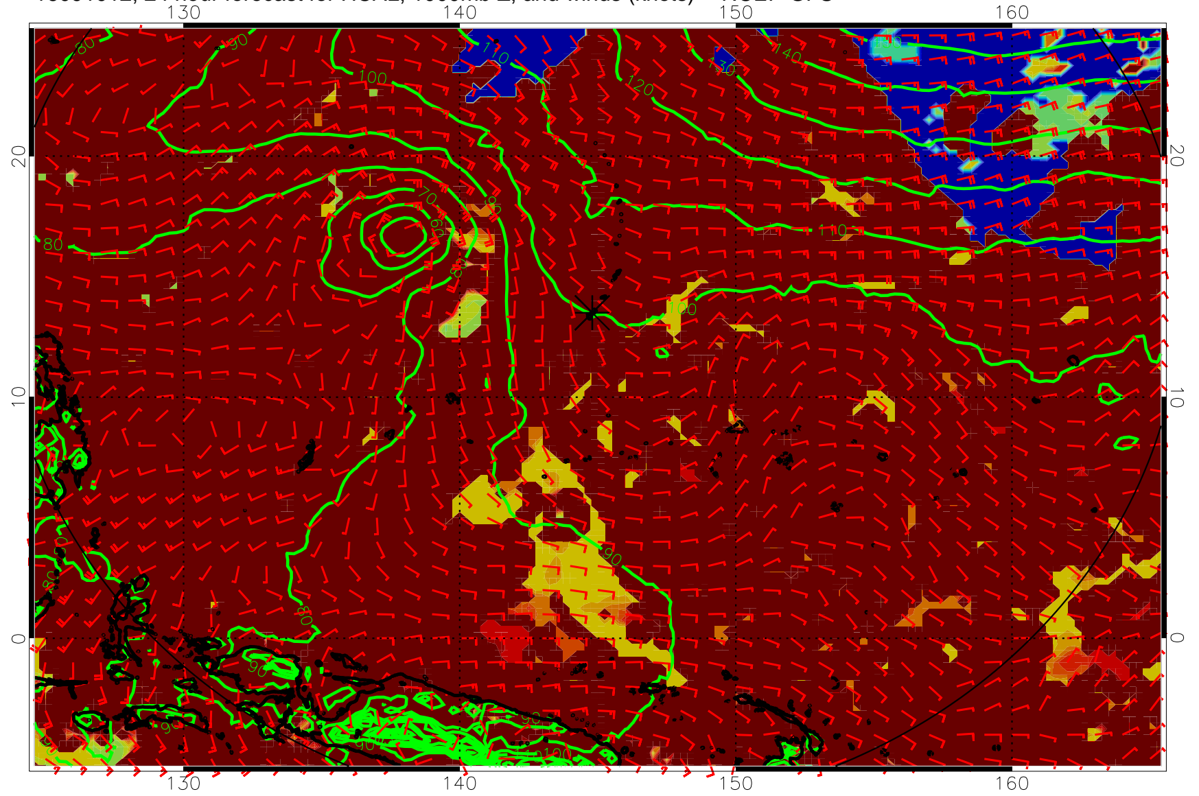
16091012, 24 hour forecast for HCAL, 1000mb Z, and winds (knots) -- NCEP GFS
