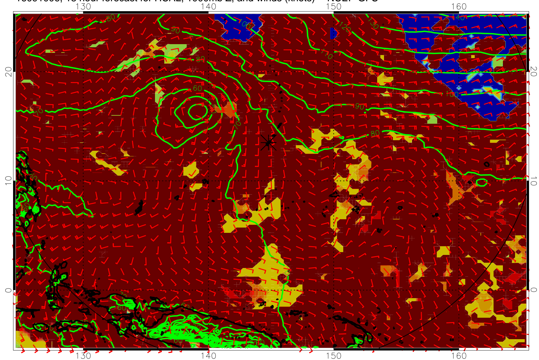
16091006, 18 hour forecast for HCAL, 1000mb Z, and winds (knots) -- NCEP GFS
