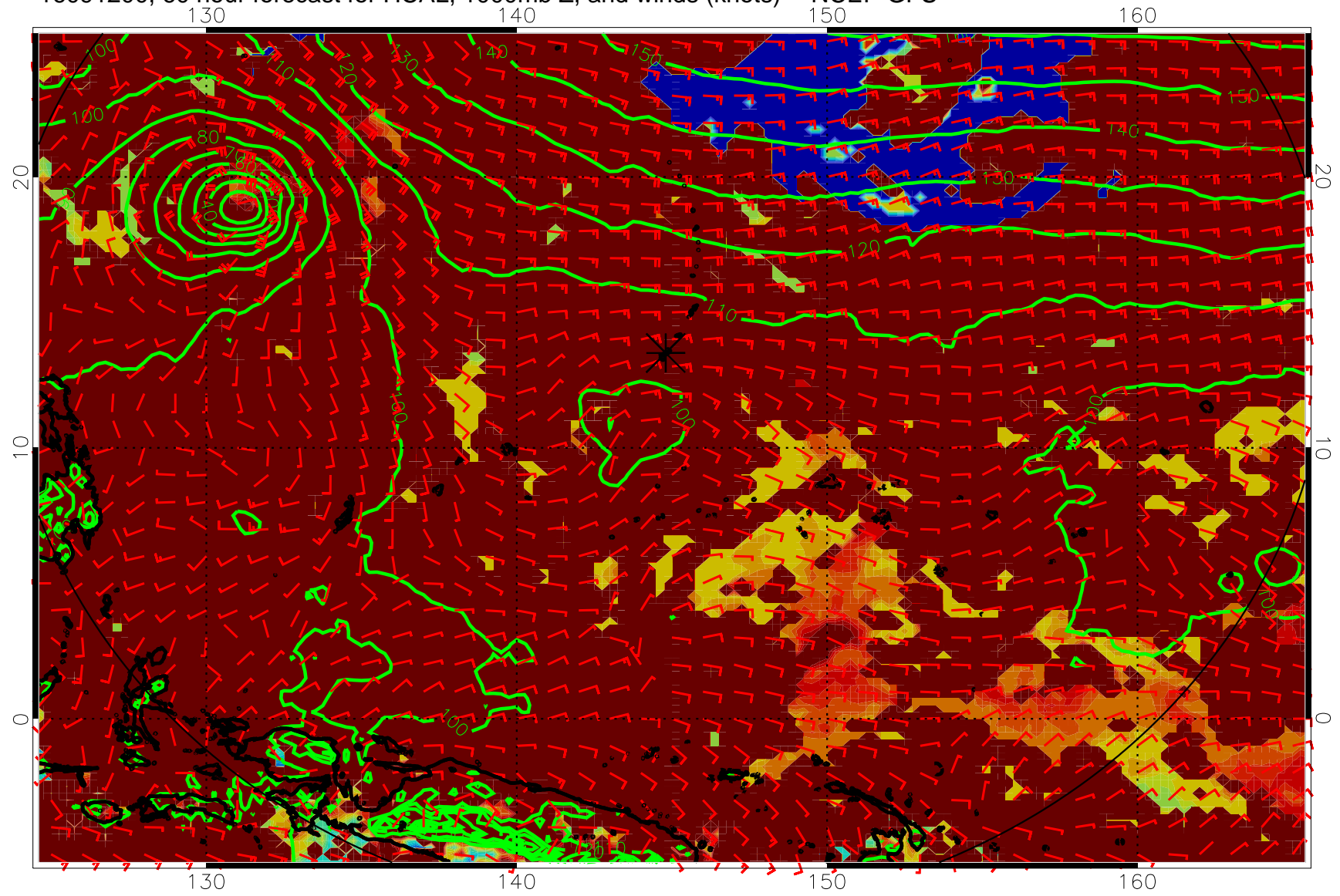
16091200, 60 hour forecast for HCAL, 1000mb Z, and winds (knots) -- NCEP GFS
