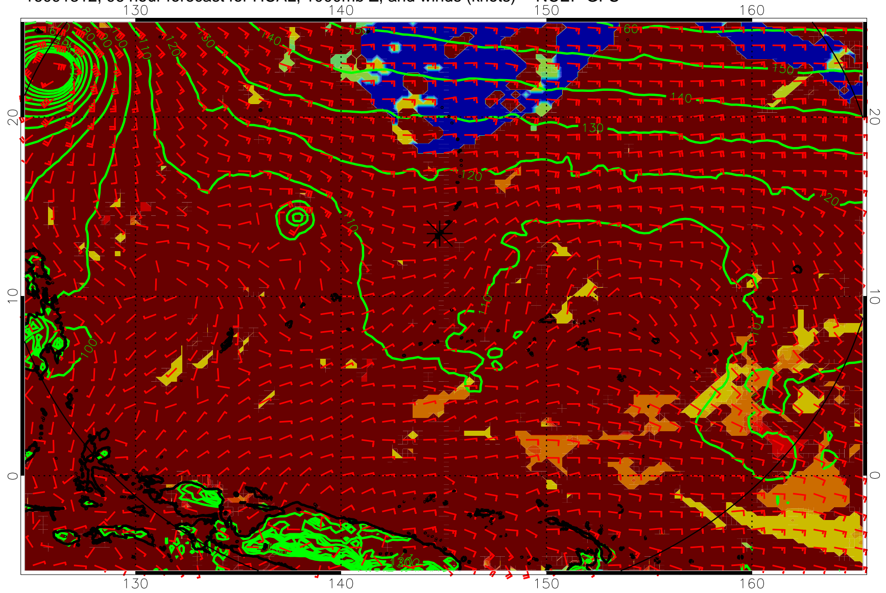
16091312, 96 hour forecast for HCAL, 1000mb Z, and winds (knots) -- NCEP GFS
