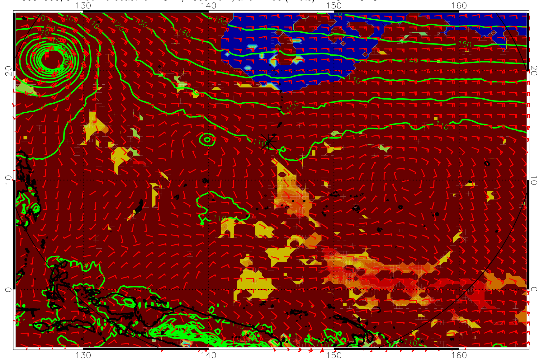
16091300, 84 hour forecast for HCAL, 1000mb Z, and winds (knots) -- NCEP GFS
