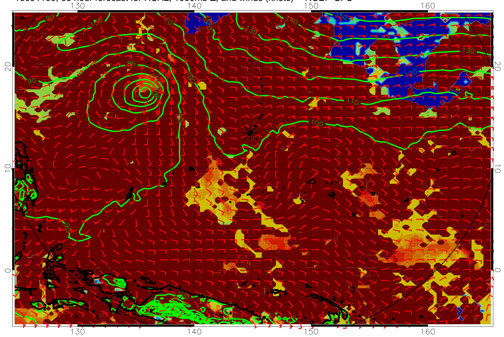
16091100, 36 hour forecast for HCAL, 1000mb Z, and winds (knots) -- NCEP GFS
