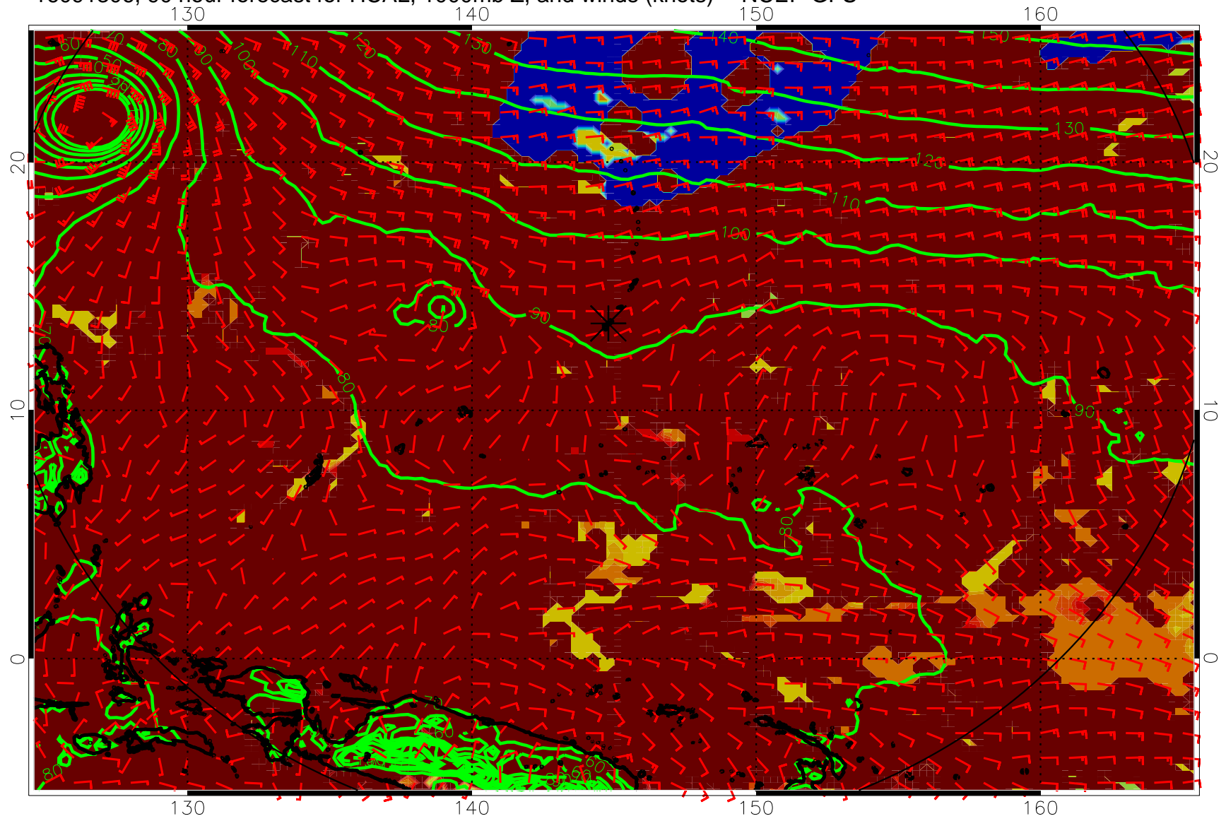
16091306, 90 hour forecast for HCAL, 1000mb Z, and winds (knots) -- NCEP GFS
