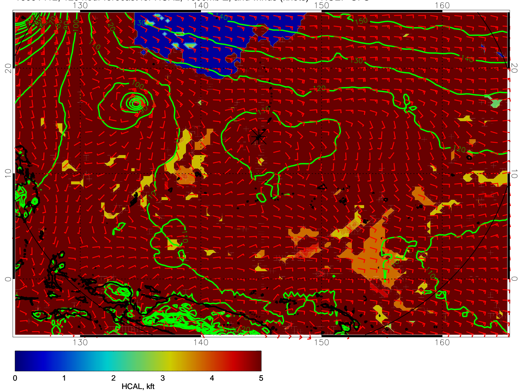
16091412, 120 hour forecast for HCAL, 1000mb Z, and winds (knots) -- NCEP GFS
