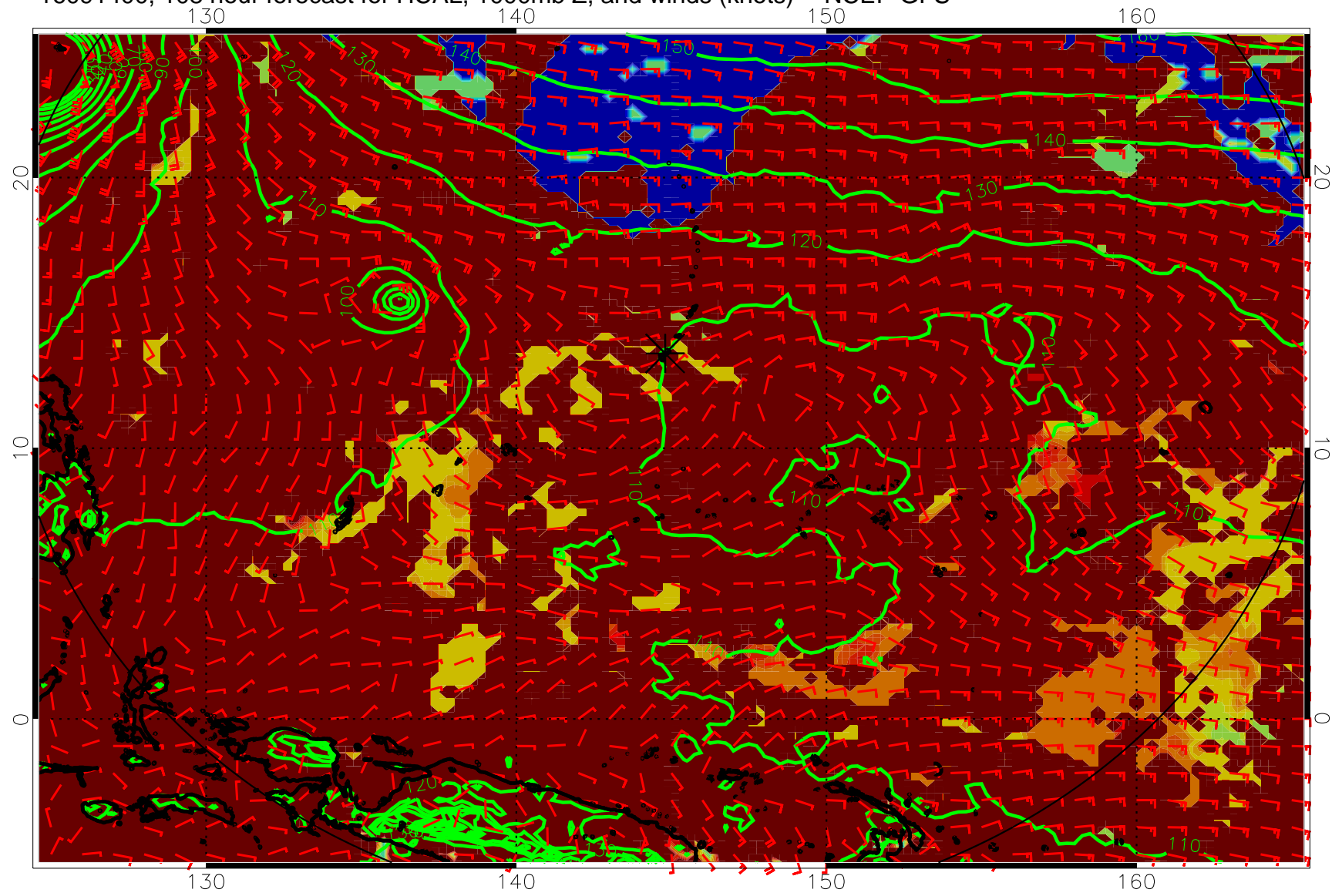
16091400, 108 hour forecast for HCAL, 1000mb Z, and winds (knots) -- NCEP GFS
