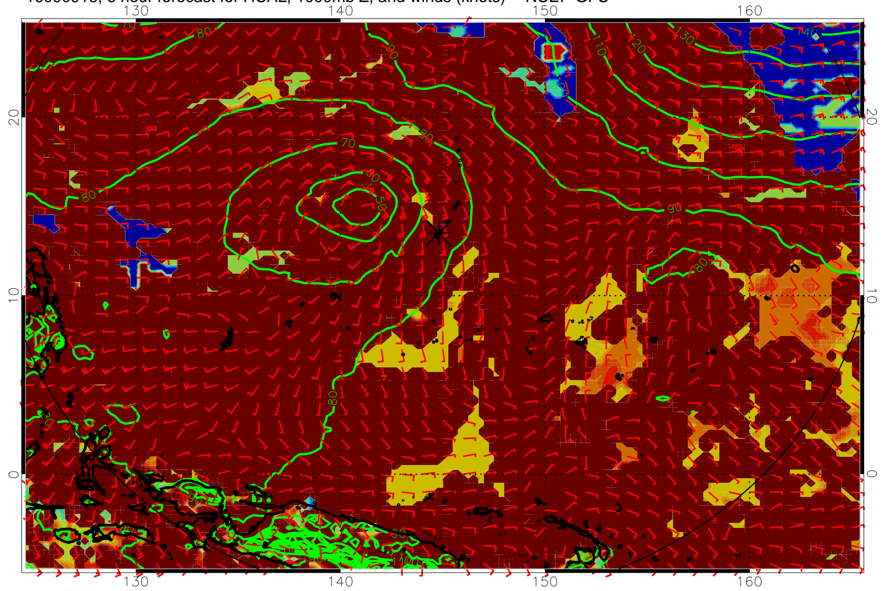
16090918, 6 hour forecast for HCAL, 1000mb Z, and winds (knots) -- NCEP GFS
