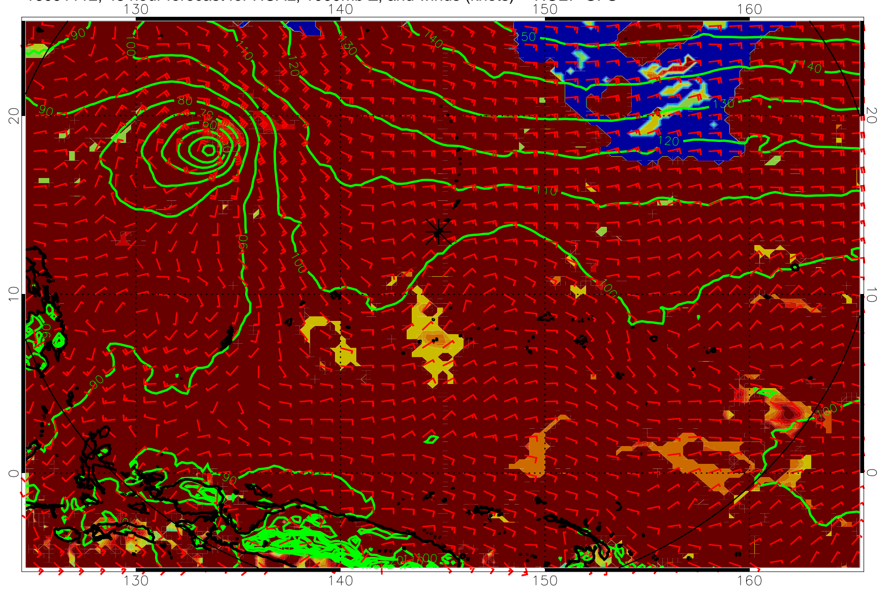
16091112, 48 hour forecast for HCAL, 1000mb Z, and winds (knots) -- NCEP GFS
