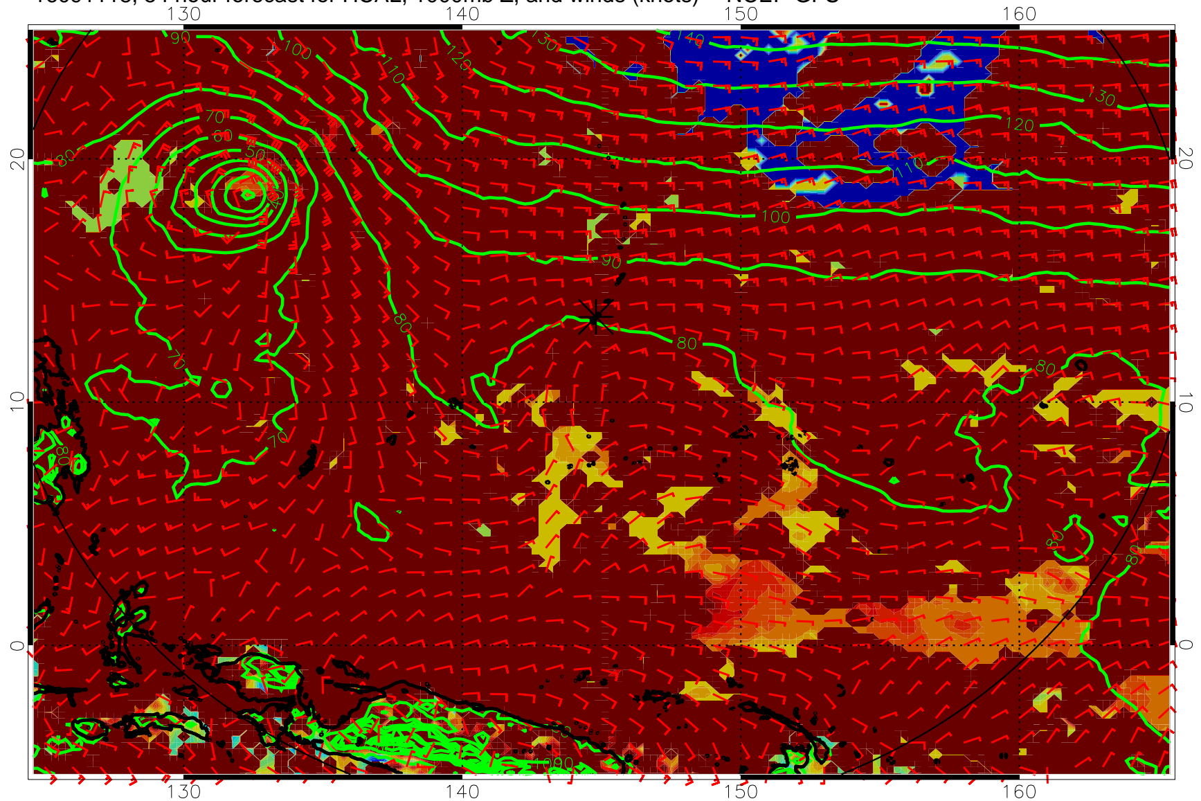
16091118, 54 hour forecast for HCAL, 1000mb Z, and winds (knots) -- NCEP GFS
