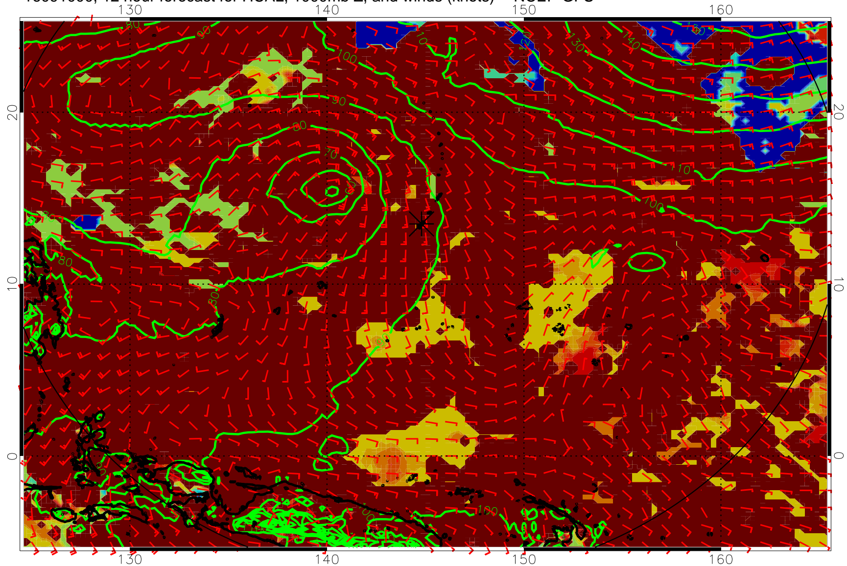
16091000, 12 hour forecast for HCAL, 1000mb Z, and winds (knots) -- NCEP GFS
