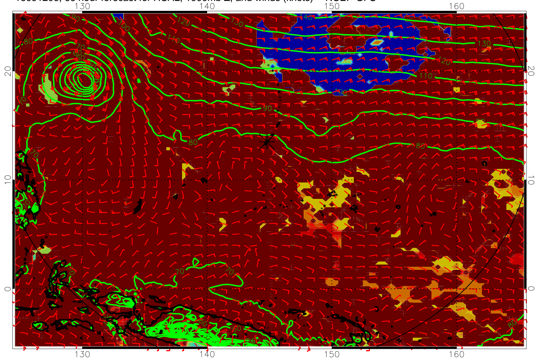
16091206, 66 hour forecast for HCAL, 1000mb Z, and winds (knots) -- NCEP GFS
