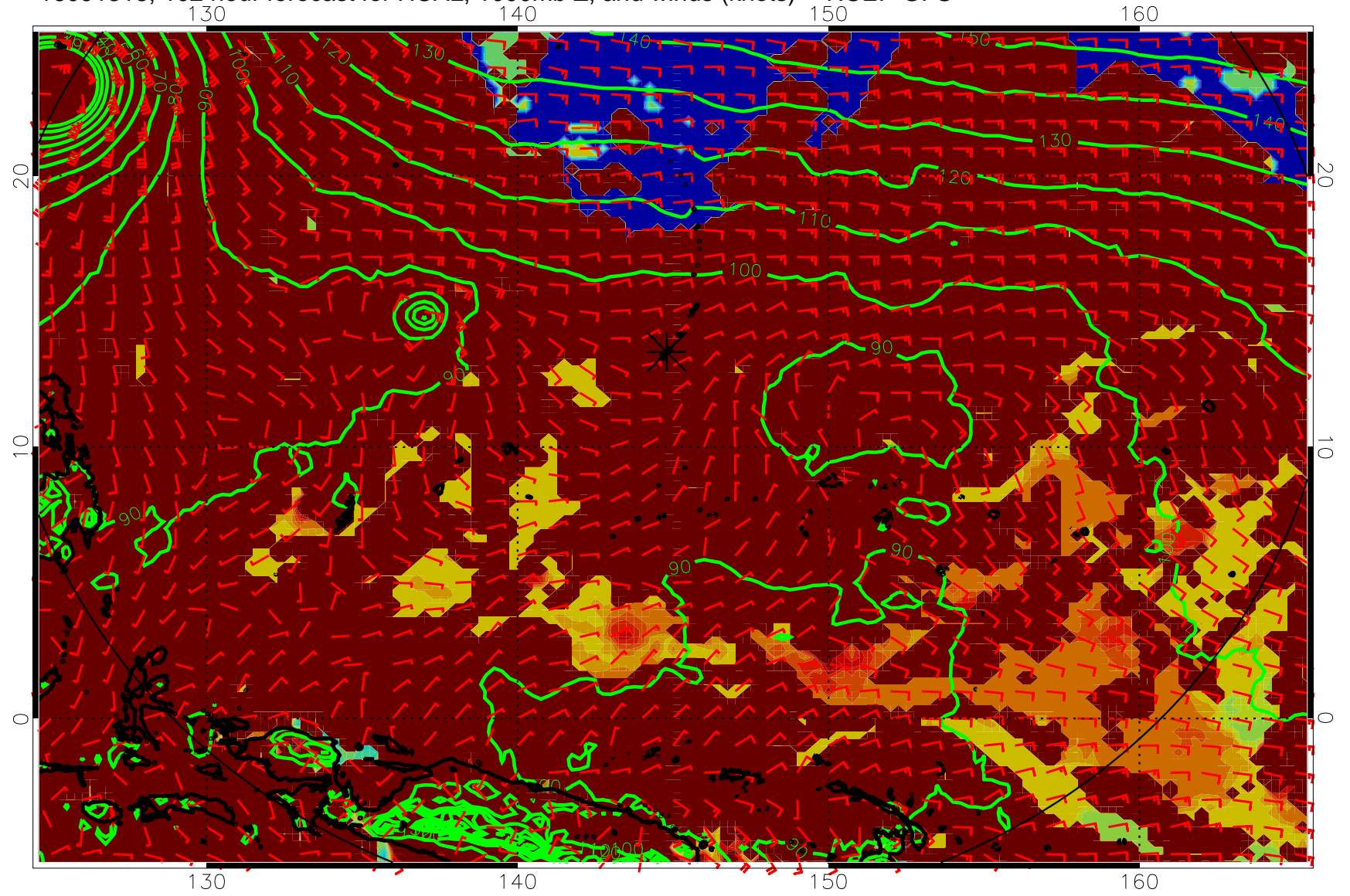
16091318, 102 hour forecast for HCAL, 1000mb Z, and winds (knots) -- NCEP GFS
