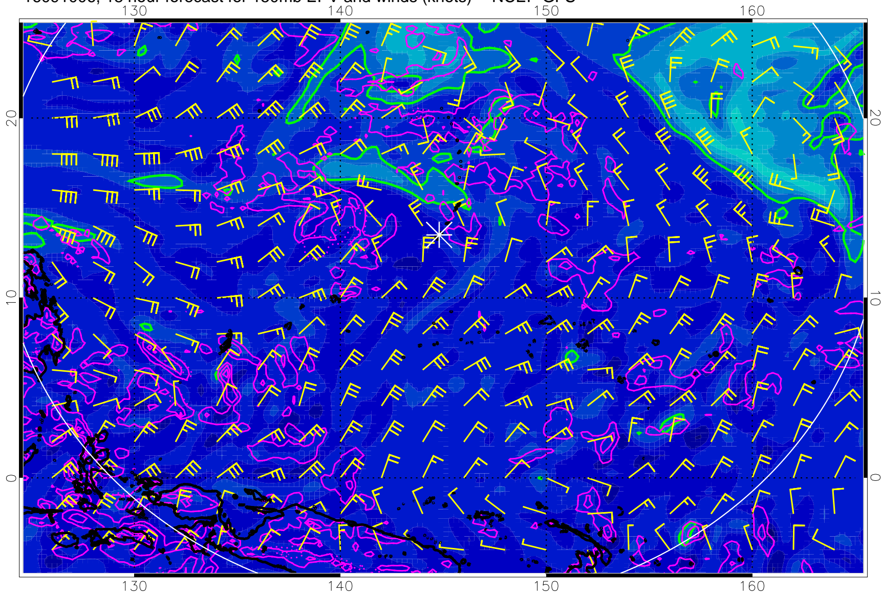
16091006, 18 hour forecast for 150mb EPV and winds (knots) -- NCEP GFS
