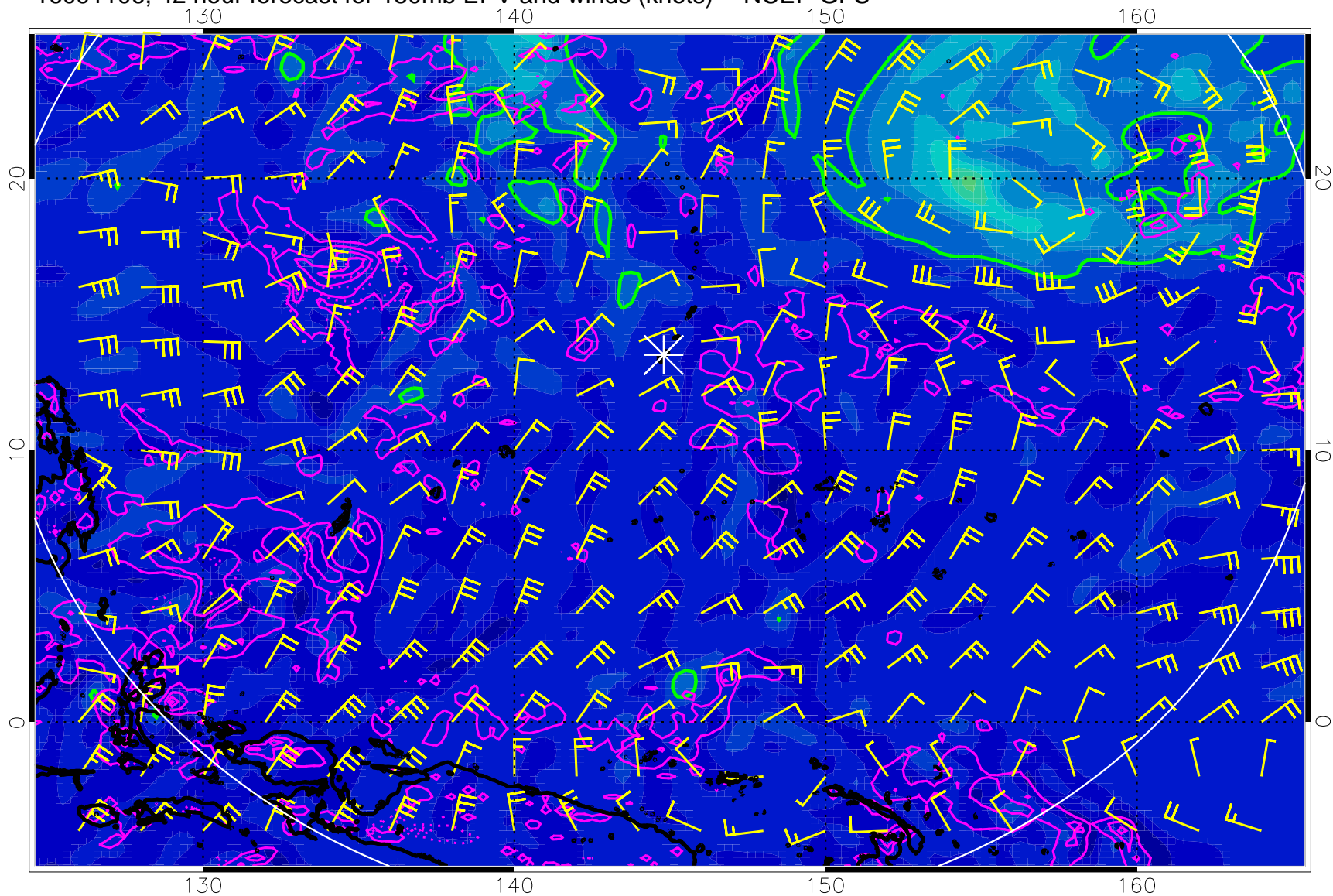
16091106, 42 hour forecast for 150mb EPV and winds (knots) -- NCEP GFS
