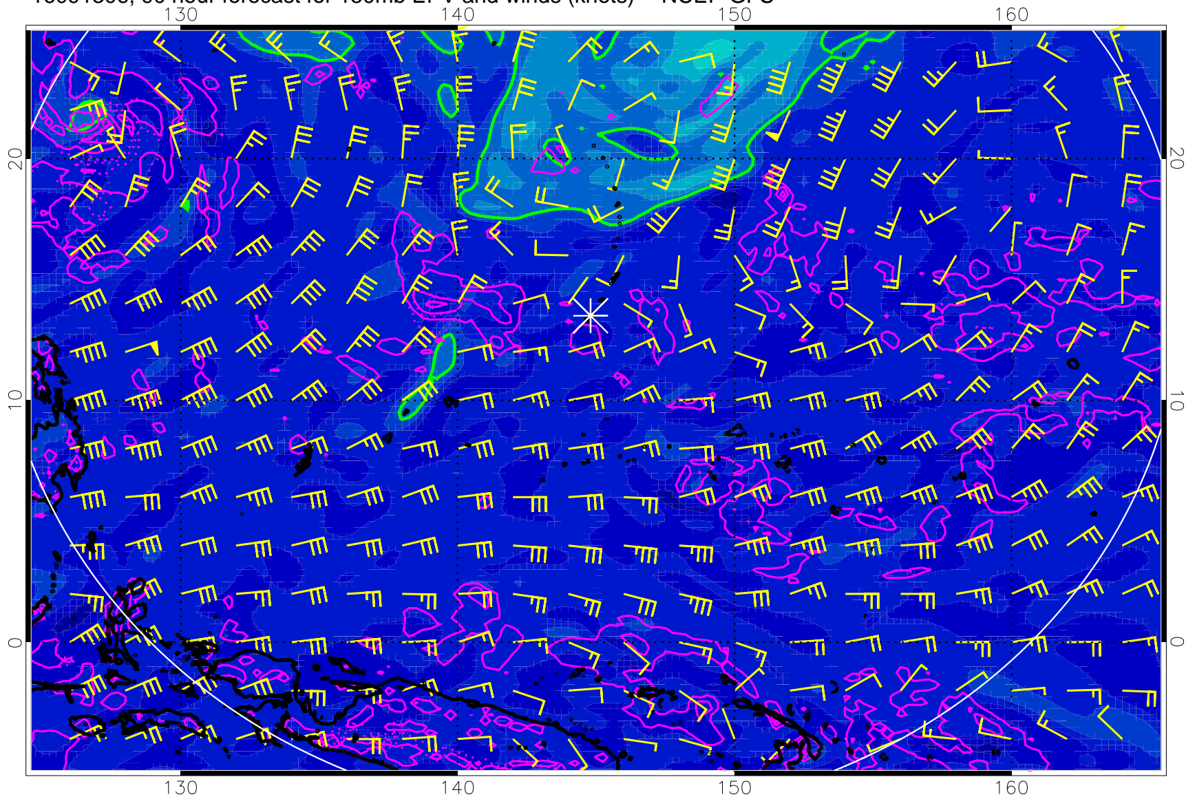
16091306, 90 hour forecast for 150mb EPV and winds (knots) -- NCEP GFS
