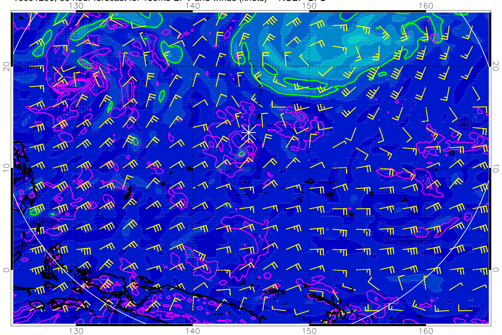
16091206, 66 hour forecast for 150mb EPV and winds (knots) -- NCEP GFS
