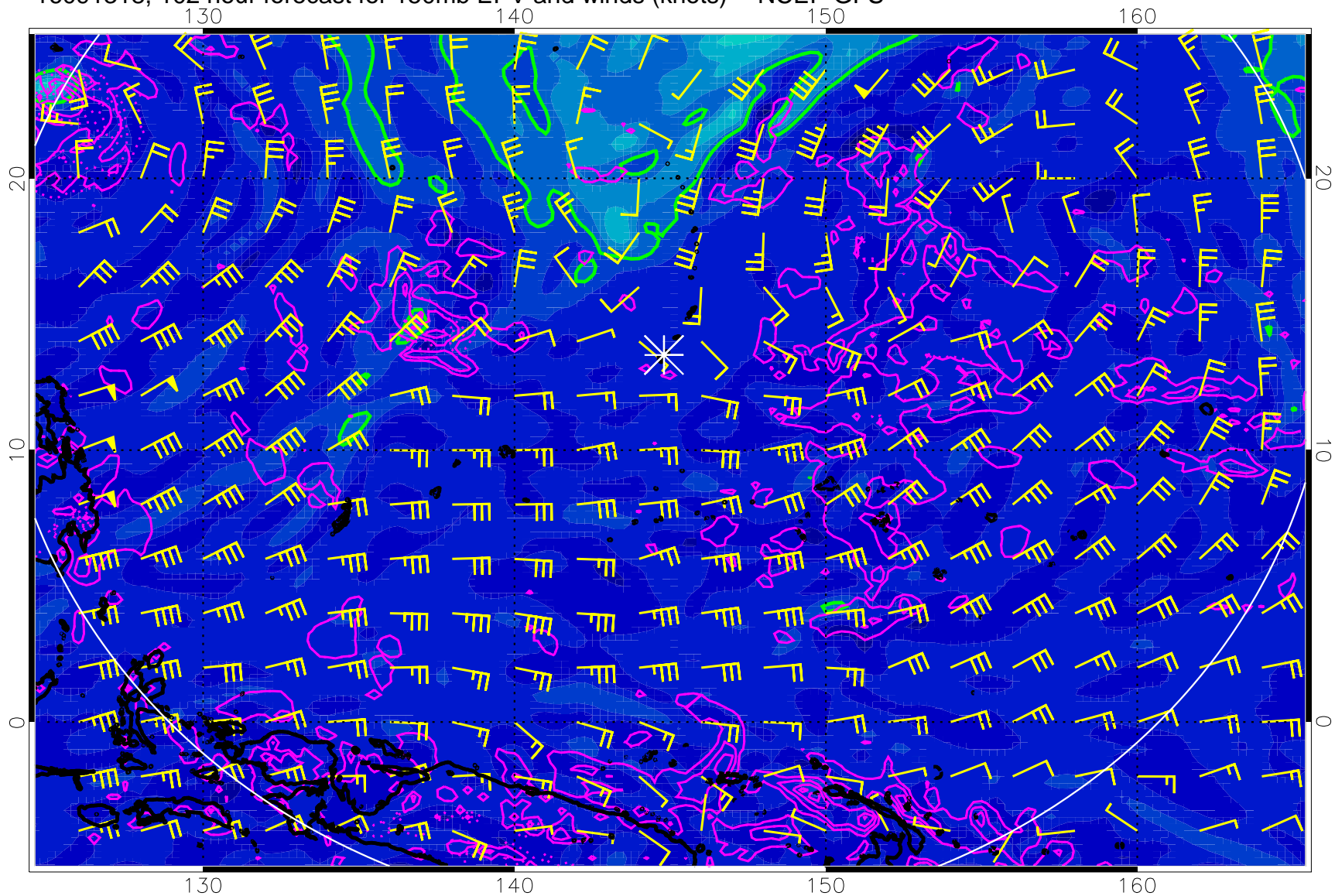
16091318, 102 hour forecast for 150mb EPV and winds (knots) -- NCEP GFS
