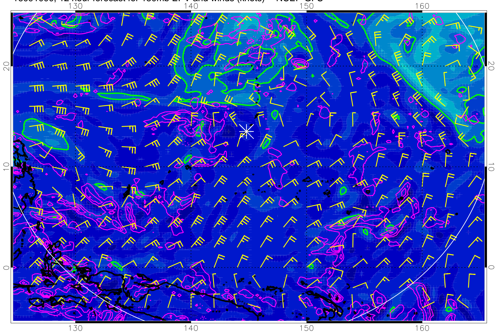
16091000, 12 hour forecast for 150mb EPV and winds (knots) -- NCEP GFS
