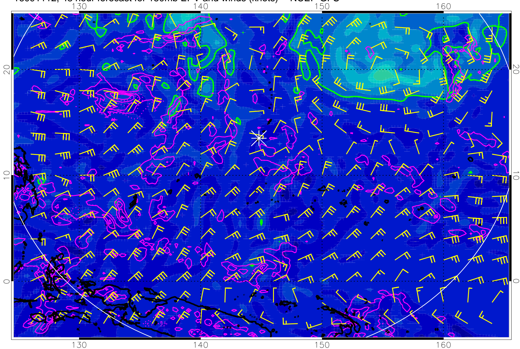
16091112, 48 hour forecast for 150mb EPV and winds (knots) -- NCEP GFS
