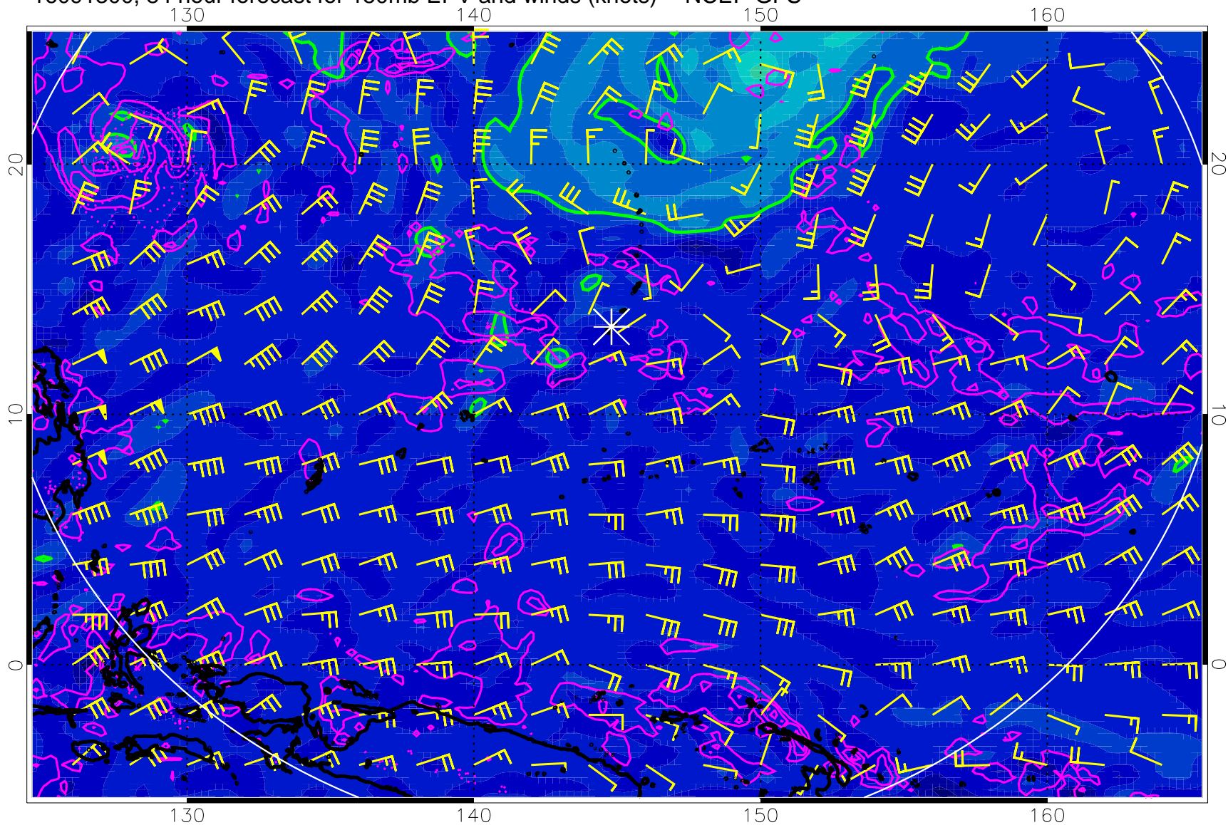
16091300, 84 hour forecast for 150mb EPV and winds (knots) -- NCEP GFS
