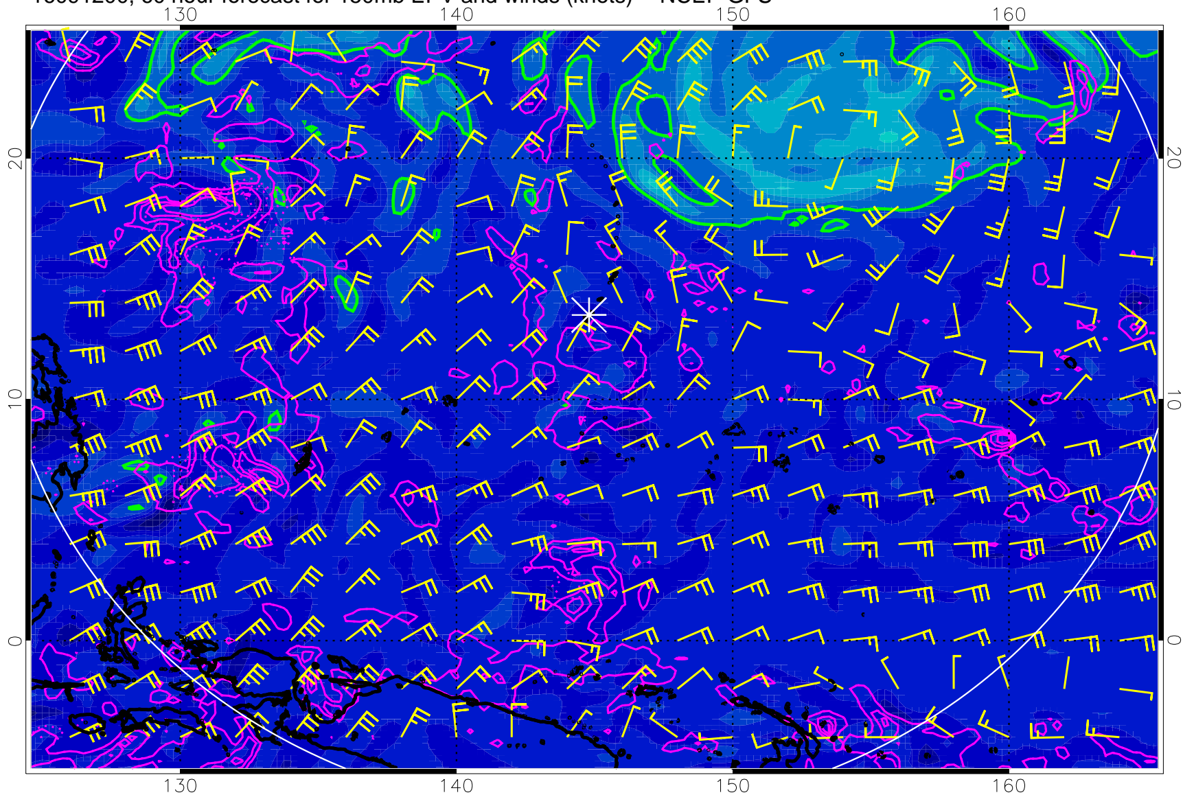
16091200, 60 hour forecast for 150mb EPV and winds (knots) -- NCEP GFS
