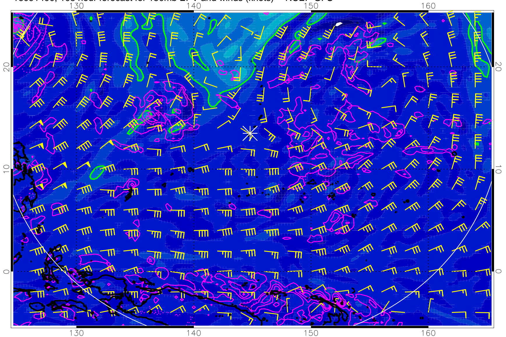
16091400, 108 hour forecast for 150mb EPV and winds (knots) -- NCEP GFS
