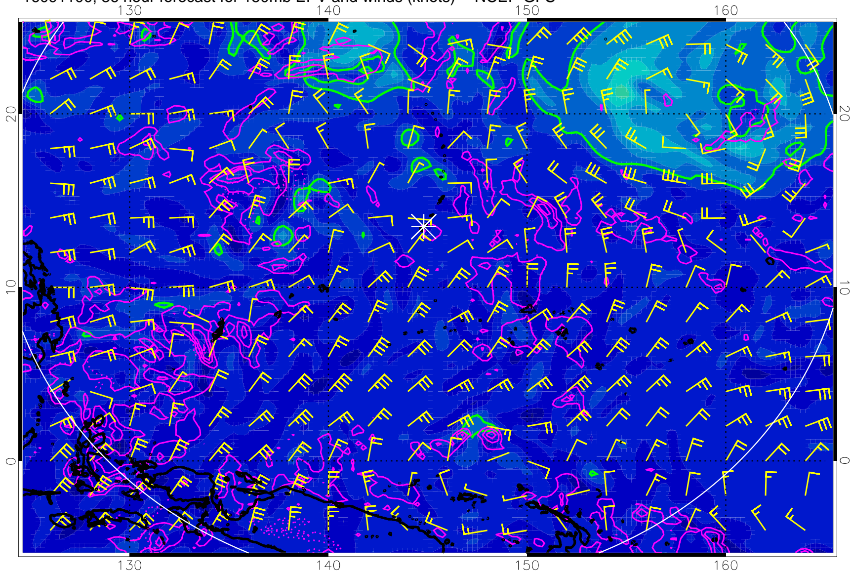
16091100, 36 hour forecast for 150mb EPV and winds (knots) -- NCEP GFS
