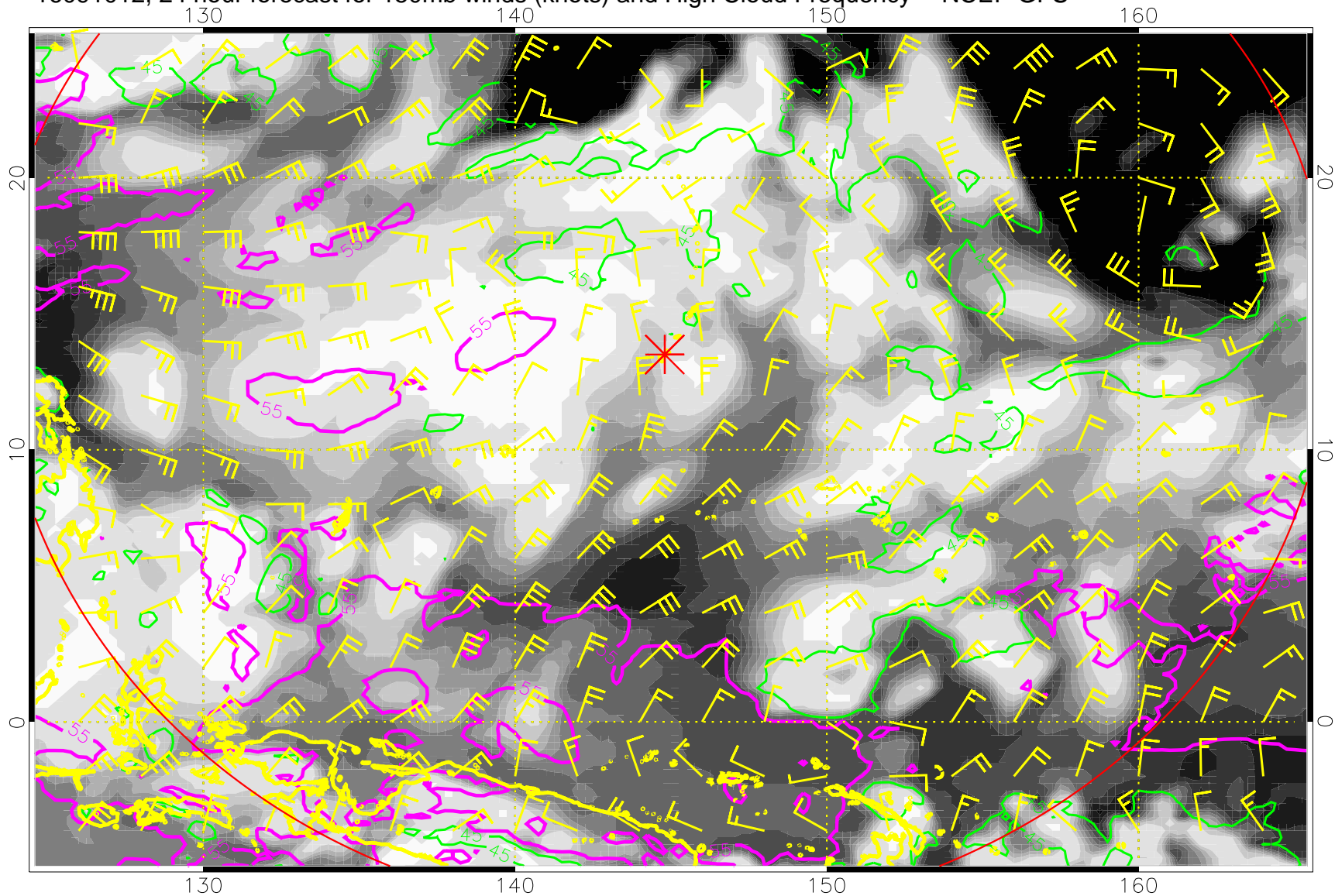
16091012, 24 hour forecast for 150mb winds (knots) and High Cloud Frequency -- NCEP GFS
