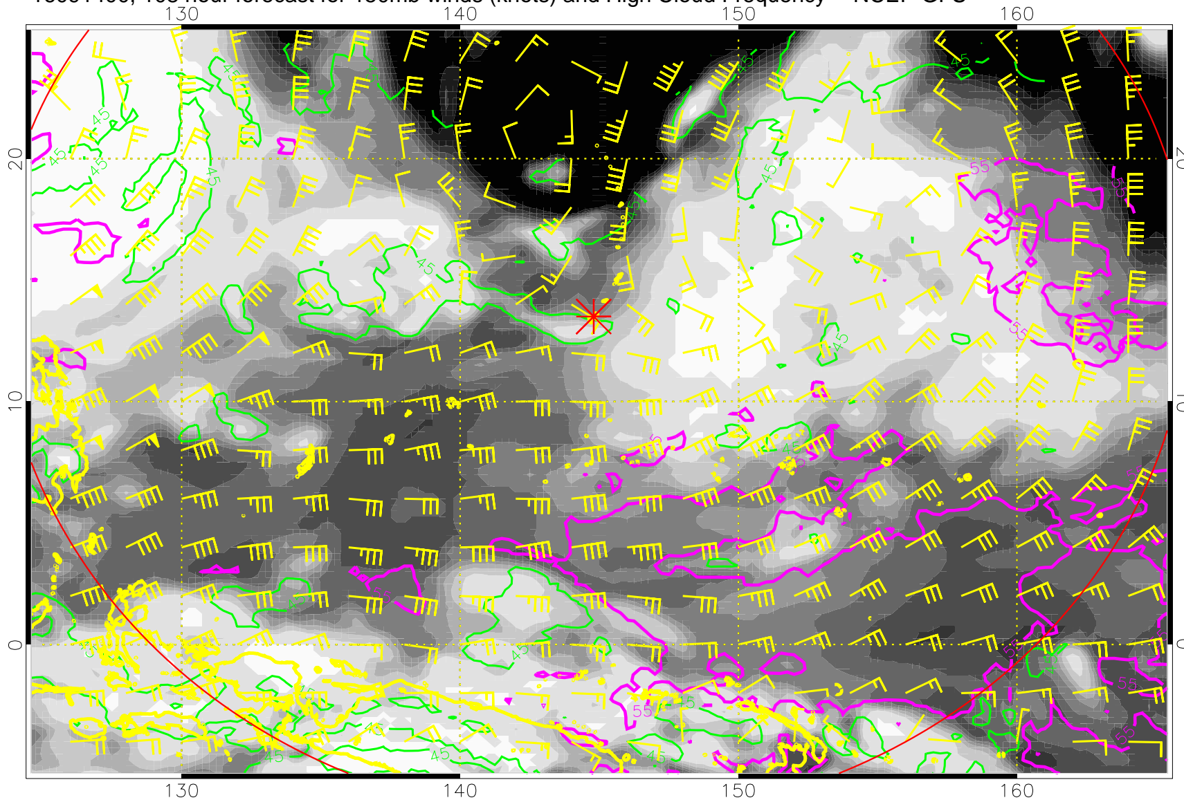
16091400, 108 hour forecast for 150mb winds (knots) and High Cloud Frequency -- NCEP GFS
