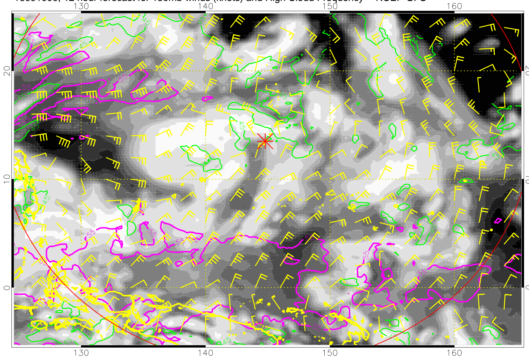
16091000, 12 hour forecast for 150mb winds (knots) and High Cloud Frequency -- NCEP GFS
