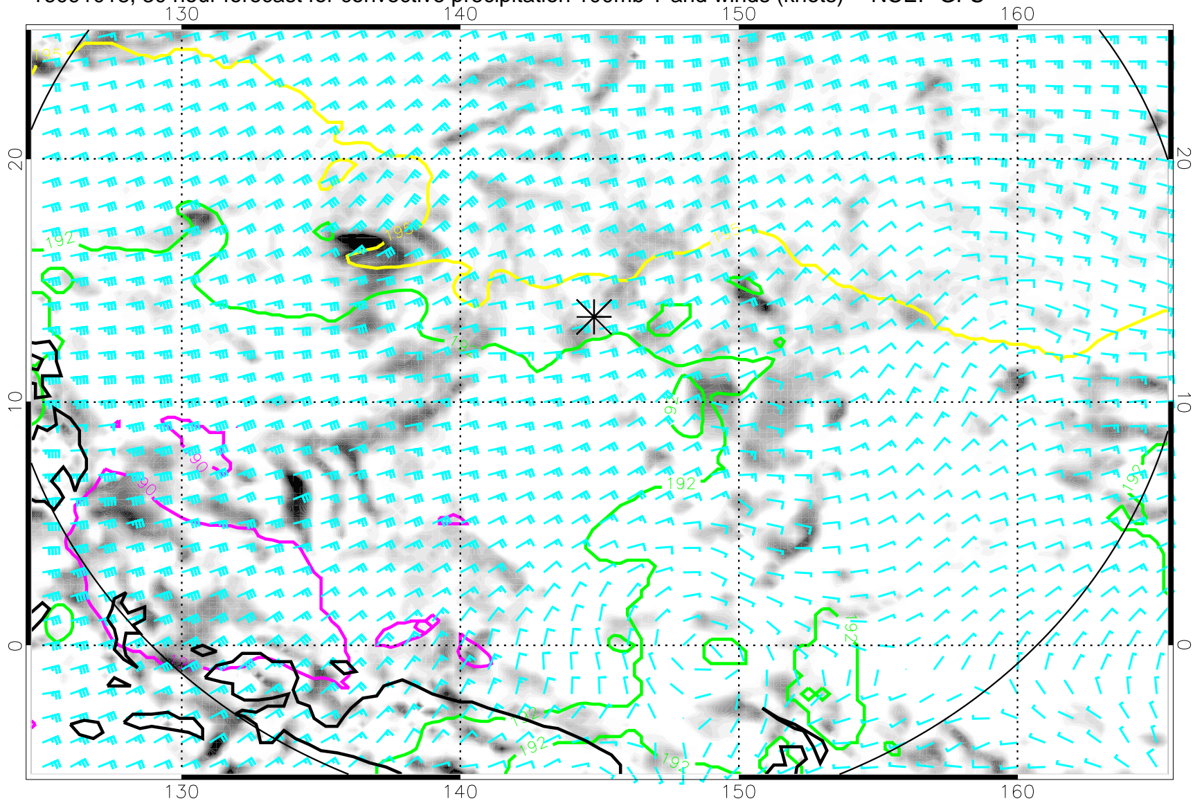
16091018, 30 hour forecast for convective precipitation 100mb T and winds (knots) -- NCEP GFS
