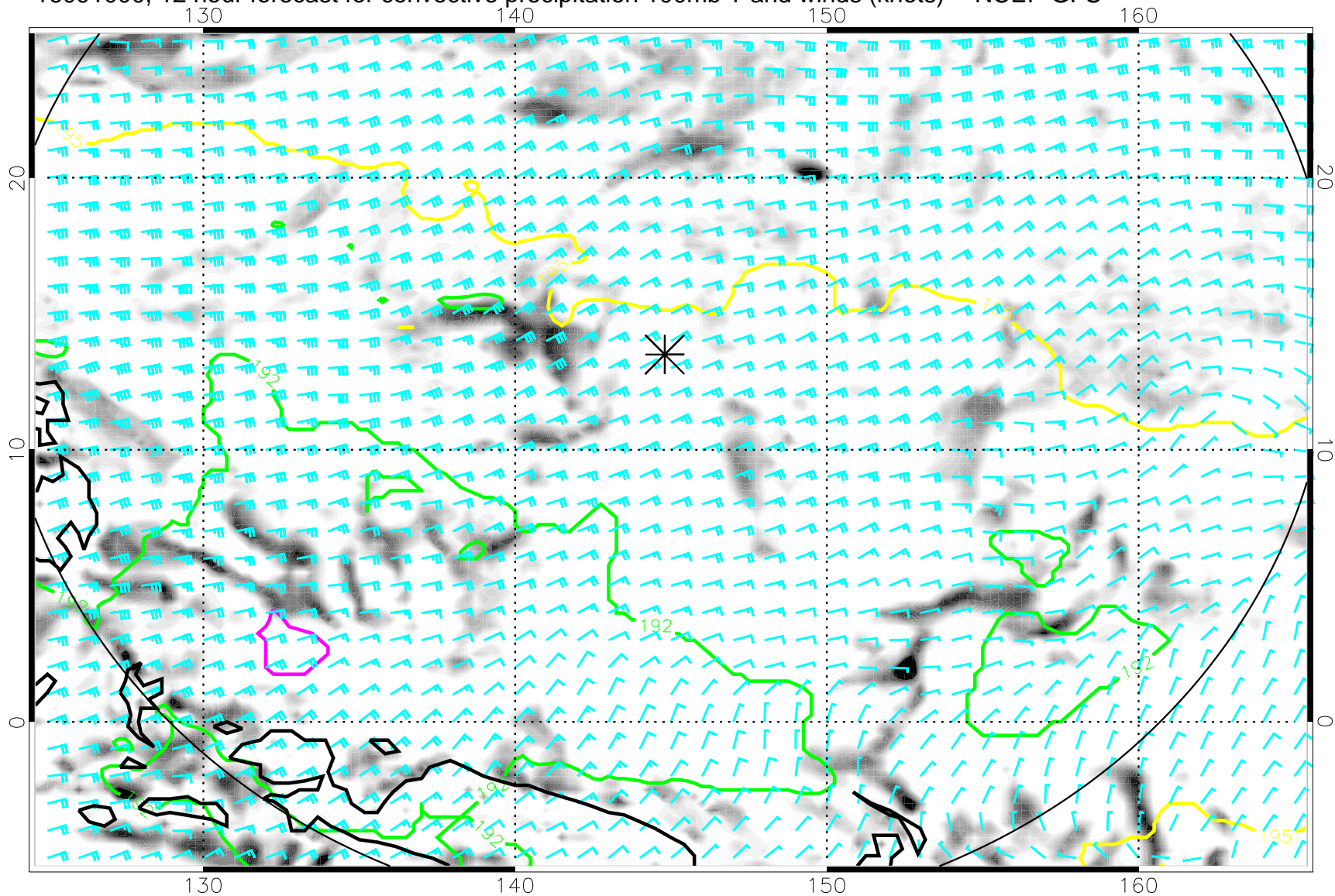
16091000, 12 hour forecast for convective precipitation 100mb T and winds (knots) -- NCEP GFS
