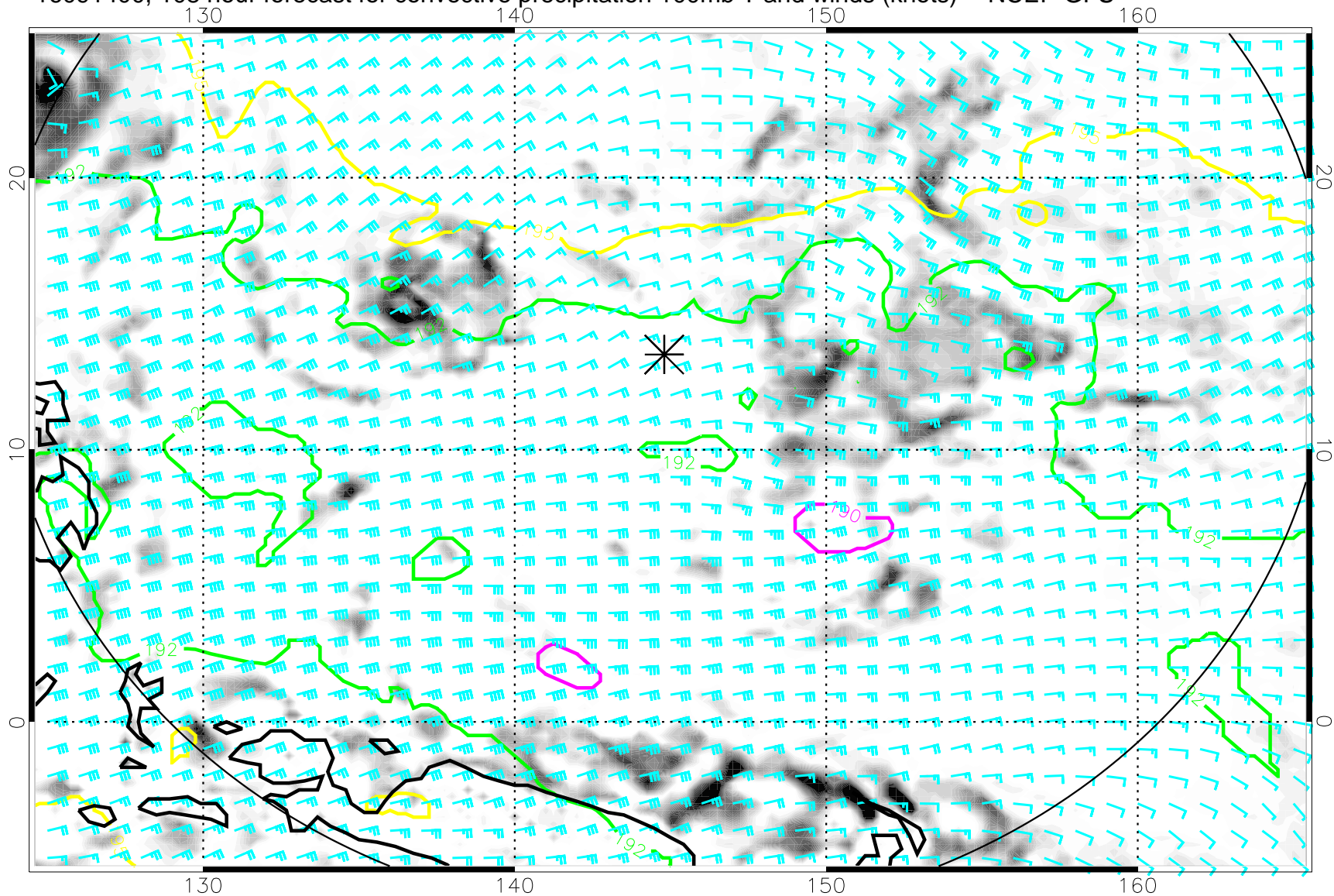
16091400, 108 hour forecast for convective precipitation 100mb T and winds (knots) -- NCEP GFS
