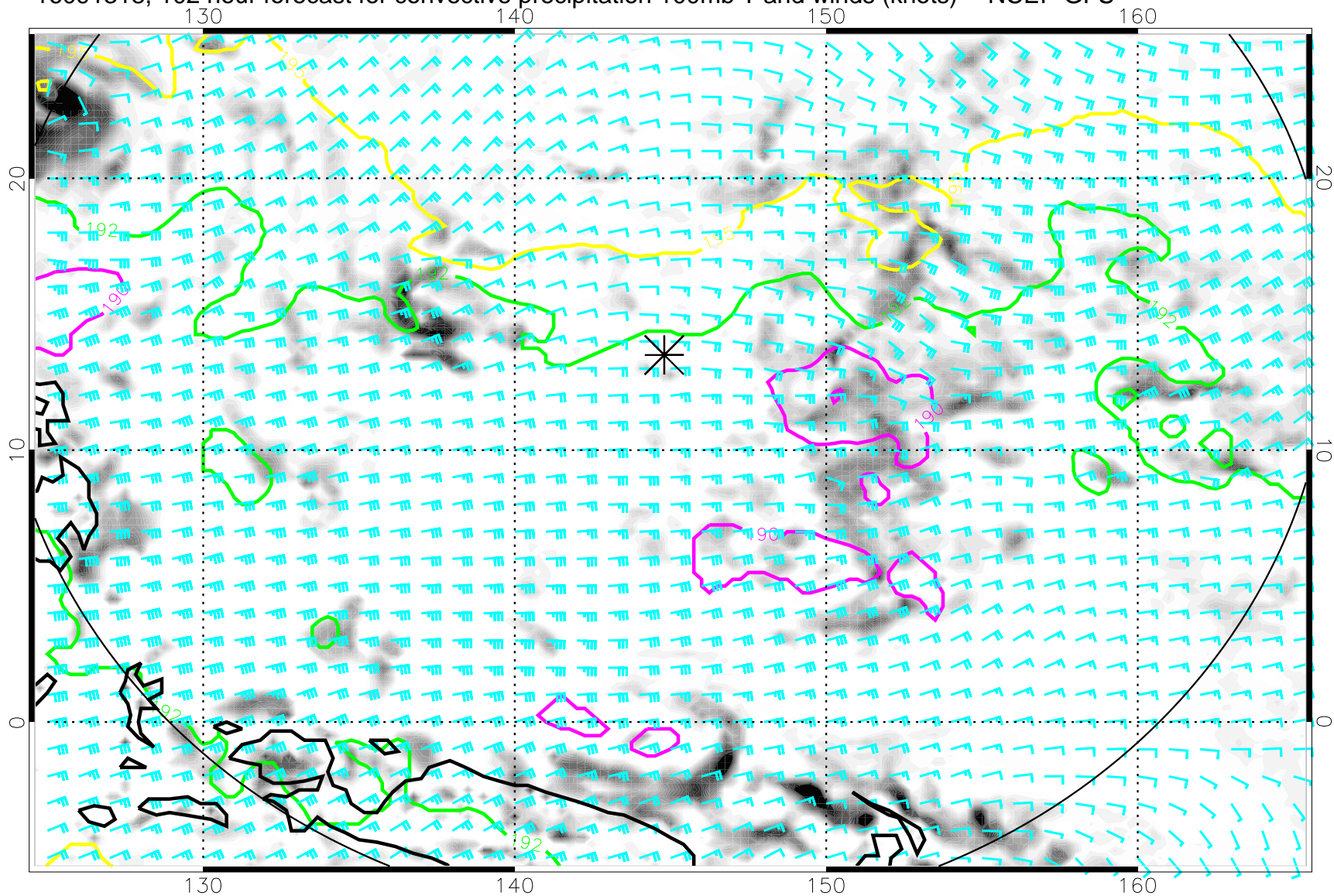
16091318, 102 hour forecast for convective precipitation 100mb T and winds (knots) -- NCEP GFS
