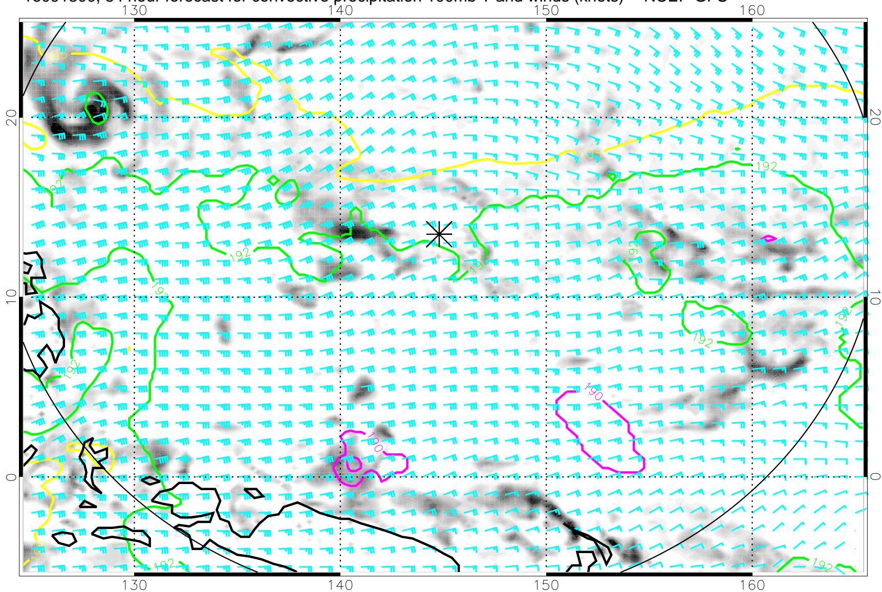
16091300, 84 hour forecast for convective precipitation 100mb T and winds (knots) -- NCEP GFS
