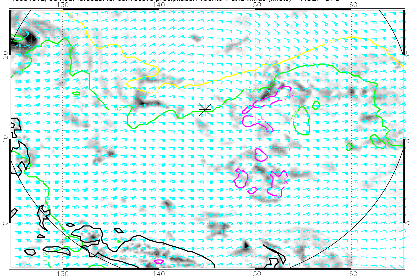
16091312, 96 hour forecast for convective precipitation 100mb T and winds (knots) -- NCEP GFS
