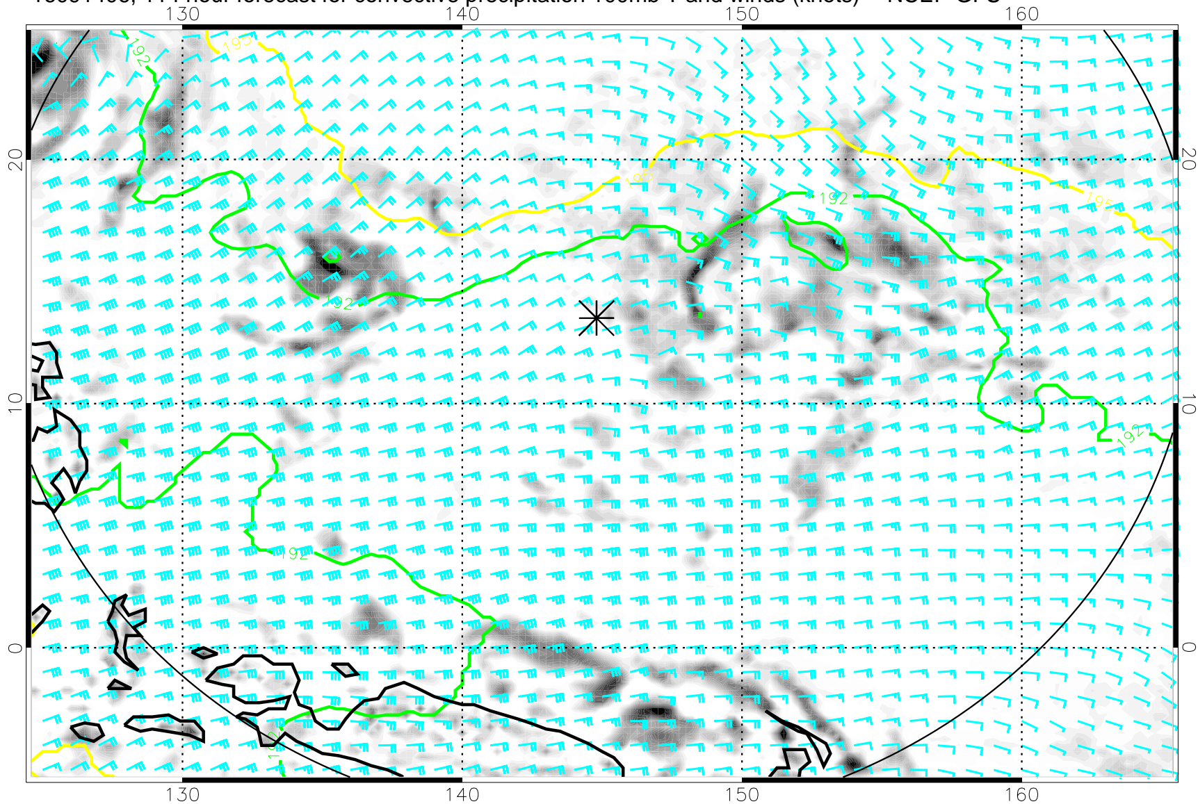
16091406, 114 hour forecast for convective precipitation 100mb T and winds (knots) -- NCEP GFS
