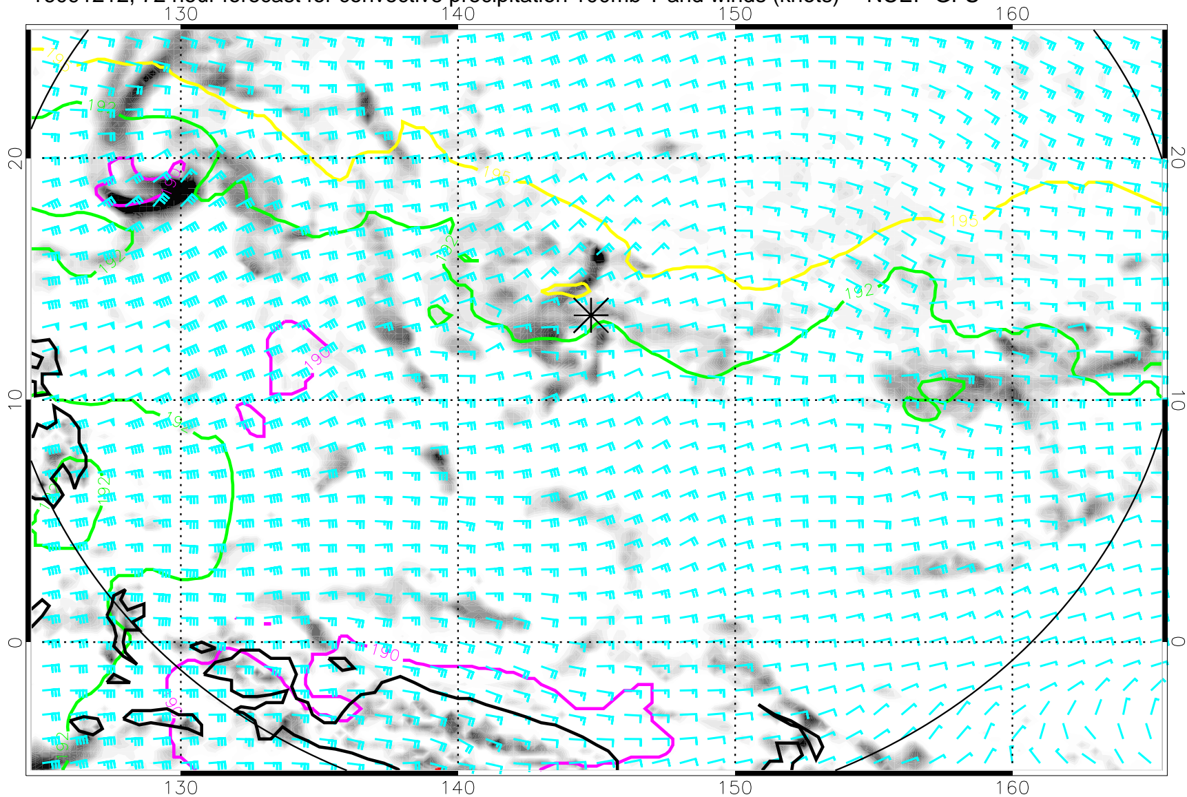
16091212, 72 hour forecast for convective precipitation 100mb T and winds (knots) -- NCEP GFS
