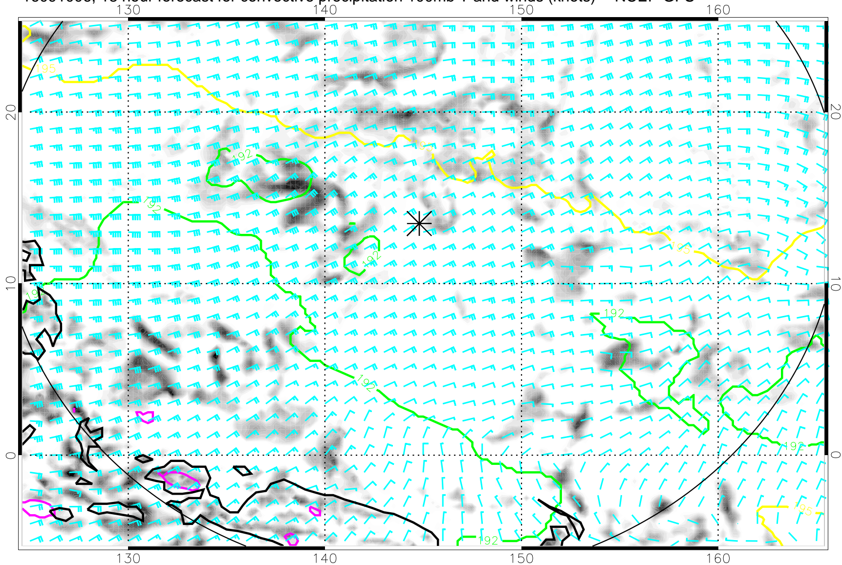
16091006, 18 hour forecast for convective precipitation 100mb T and winds (knots) -- NCEP GFS
