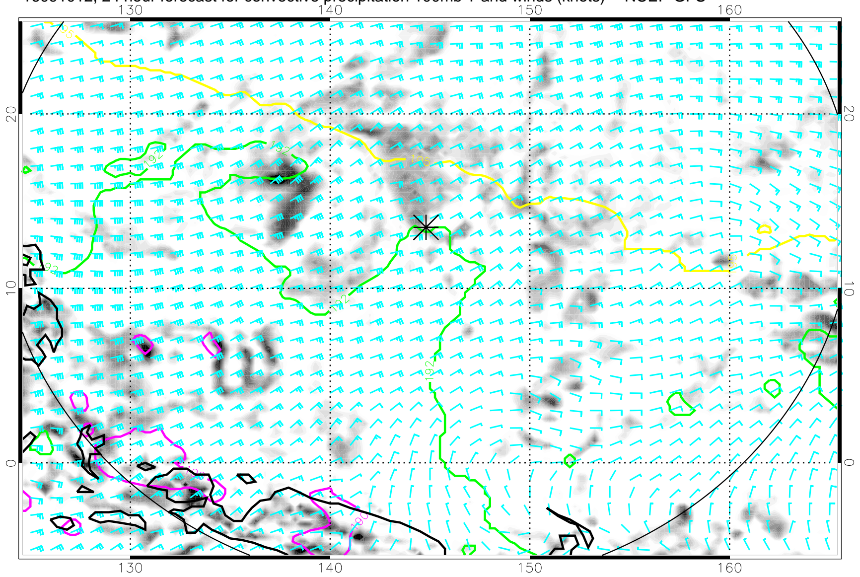
16091012, 24 hour forecast for convective precipitation 100mb T and winds (knots) -- NCEP GFS
