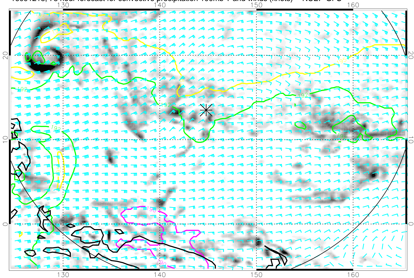
16091218, 78 hour forecast for convective precipitation 100mb T and winds (knots) -- NCEP GFS
