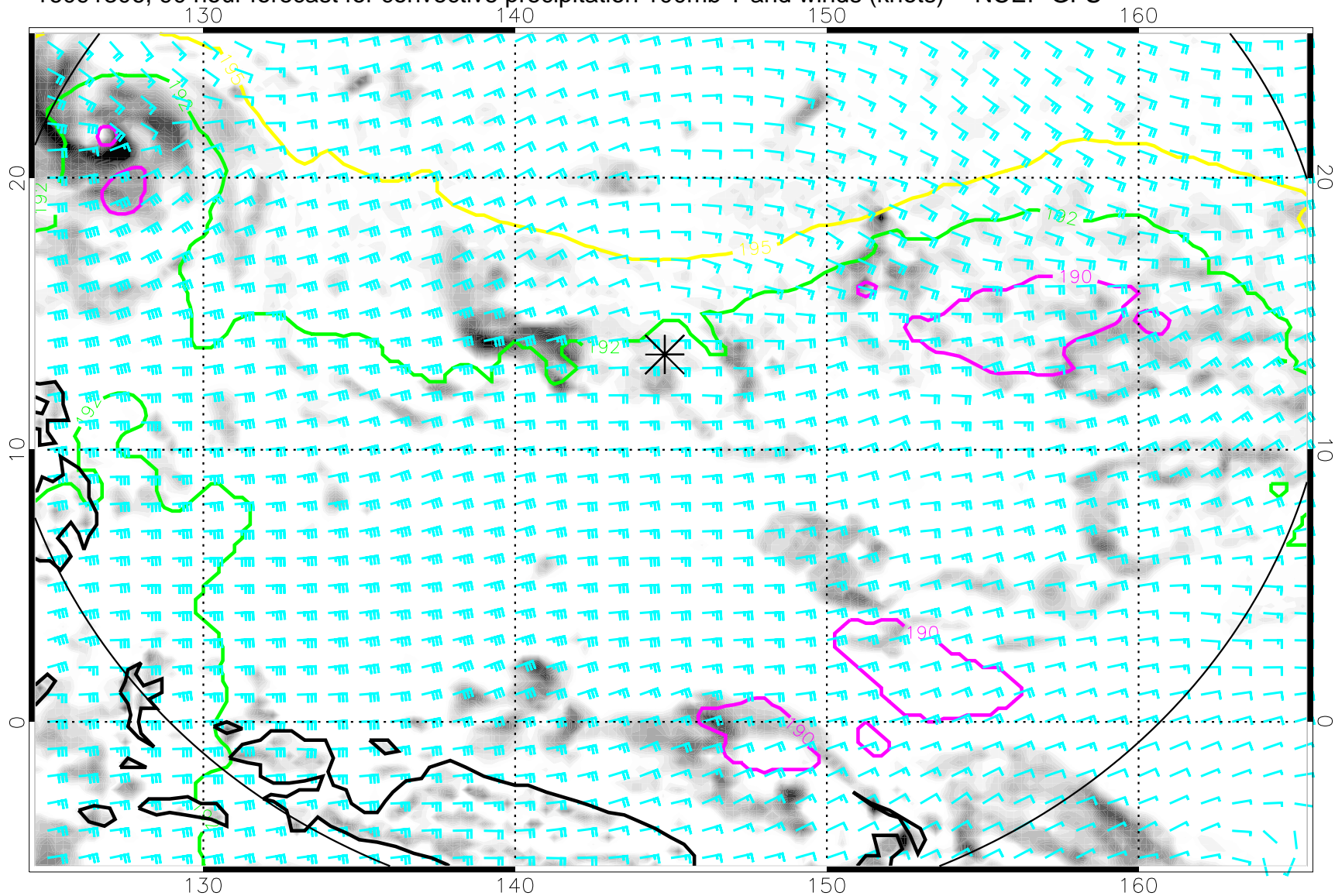
16091306, 90 hour forecast for convective precipitation 100mb T and winds (knots) -- NCEP GFS
