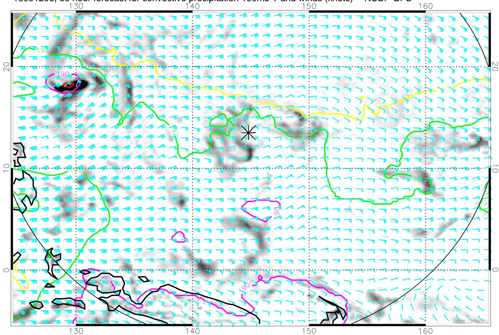
16091206, 66 hour forecast for convective precipitation 100mb T and winds (knots) -- NCEP GFS
