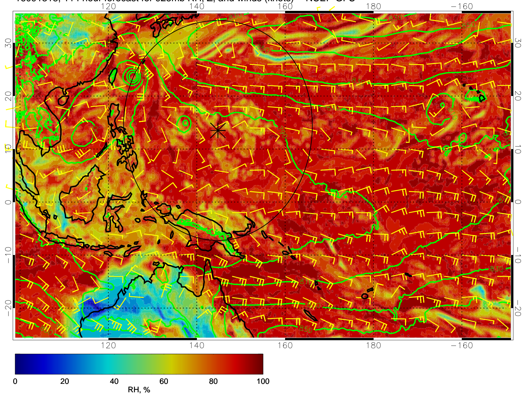
16091318, 114 hour forecast for 925mb RH, Z, and winds (knots) -- NCEP GFS
