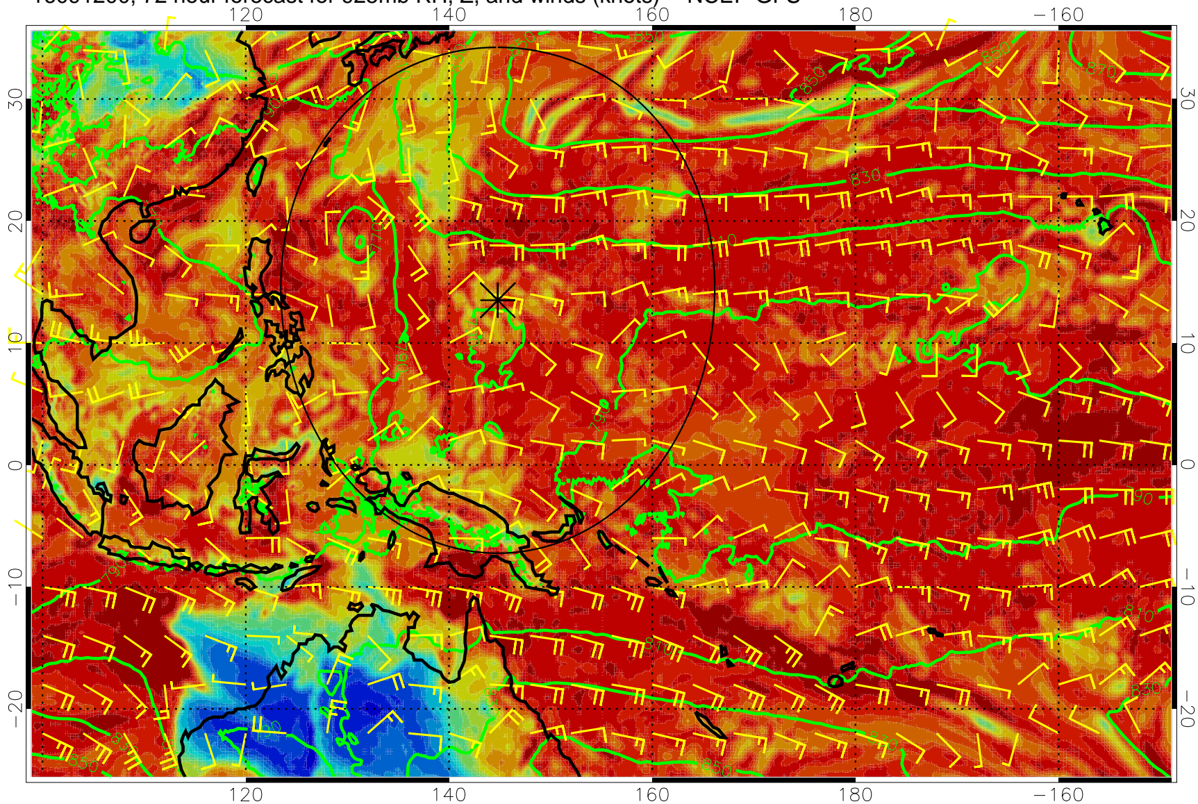
16091200, 72 hour forecast for 925mb RH, Z, and winds (knots) -- NCEP GFS
