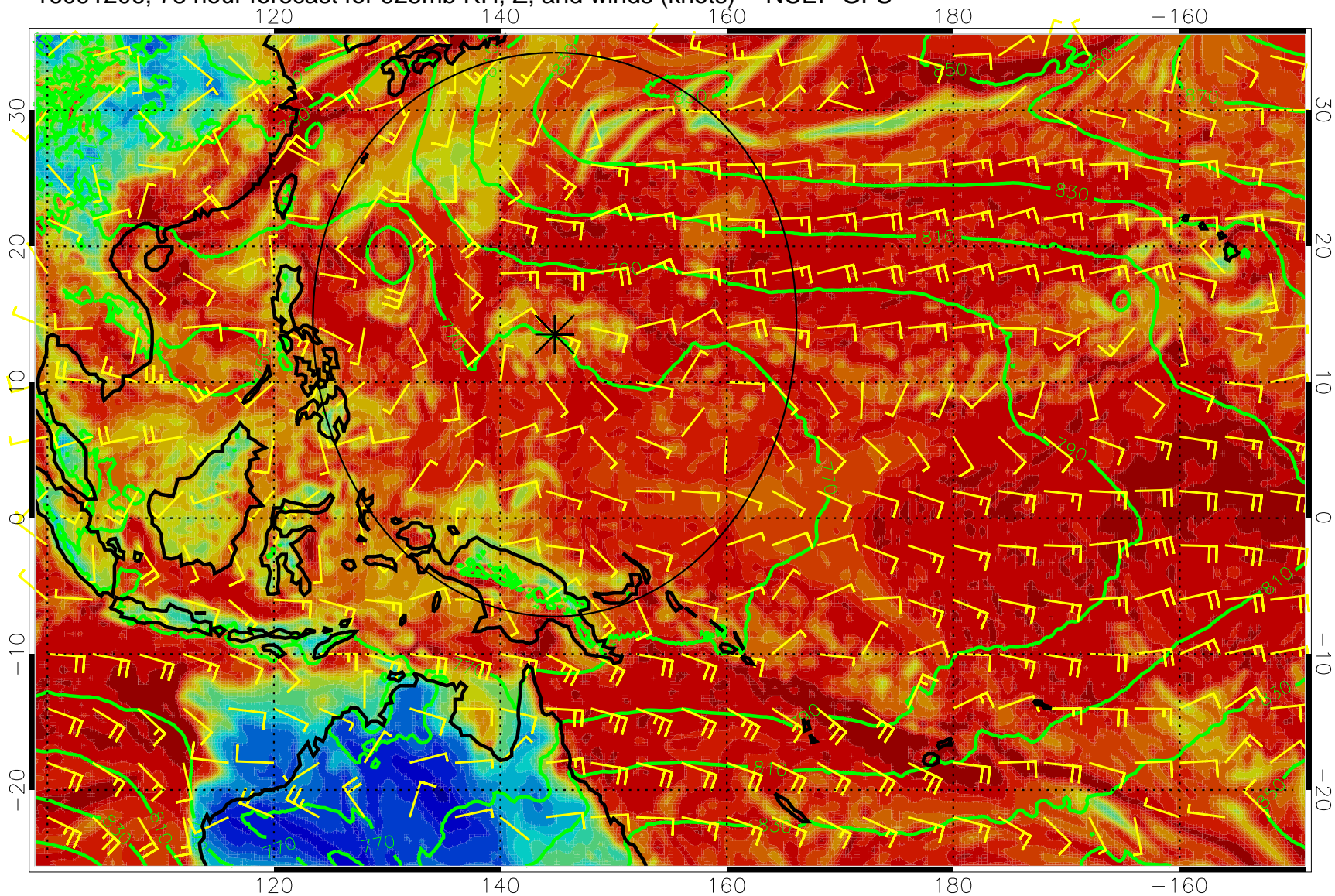
16091206, 78 hour forecast for 925mb RH, Z, and winds (knots) -- NCEP GFS
