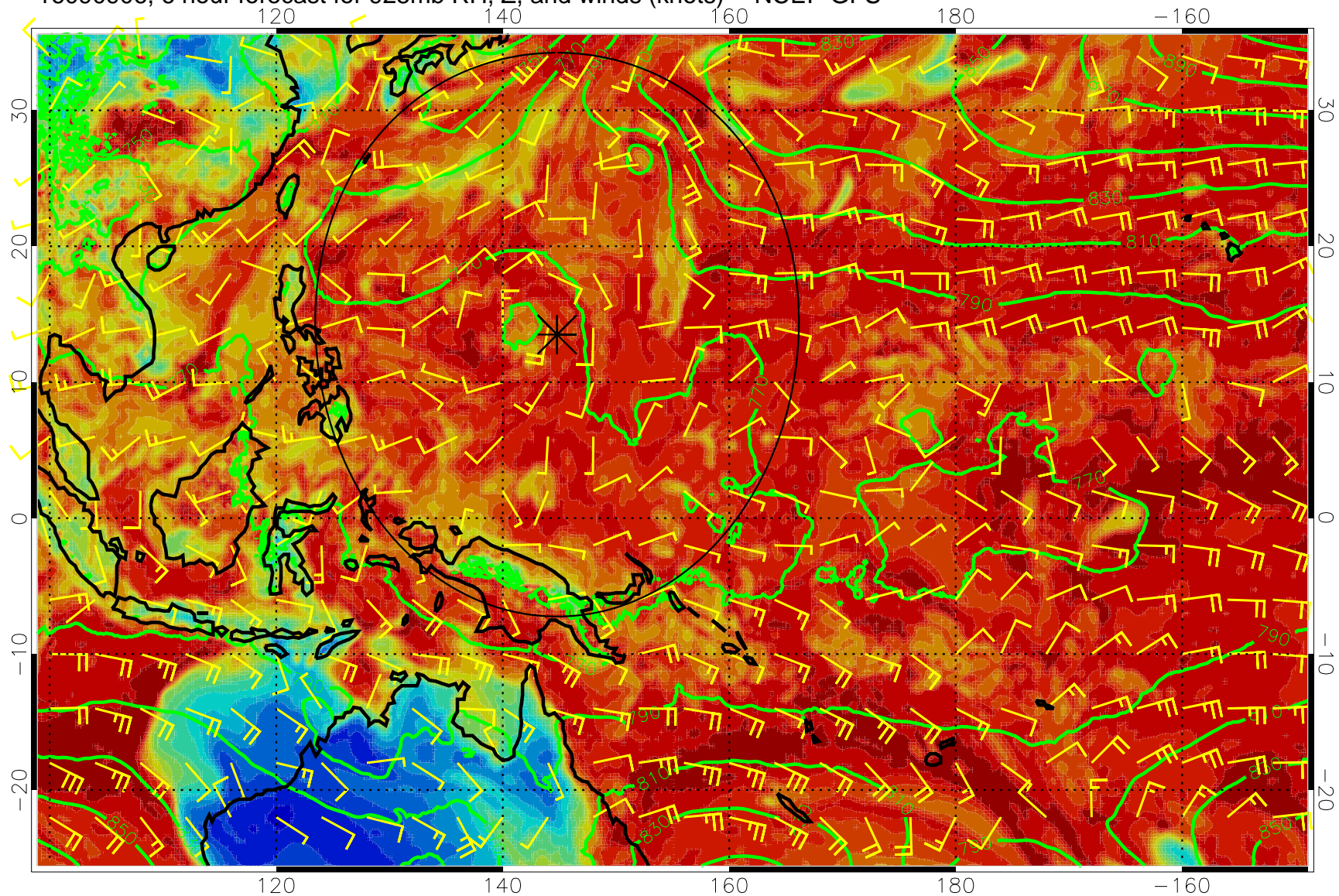
16090906, 6 hour forecast for 925mb RH, Z, and winds (knots) -- NCEP GFS
