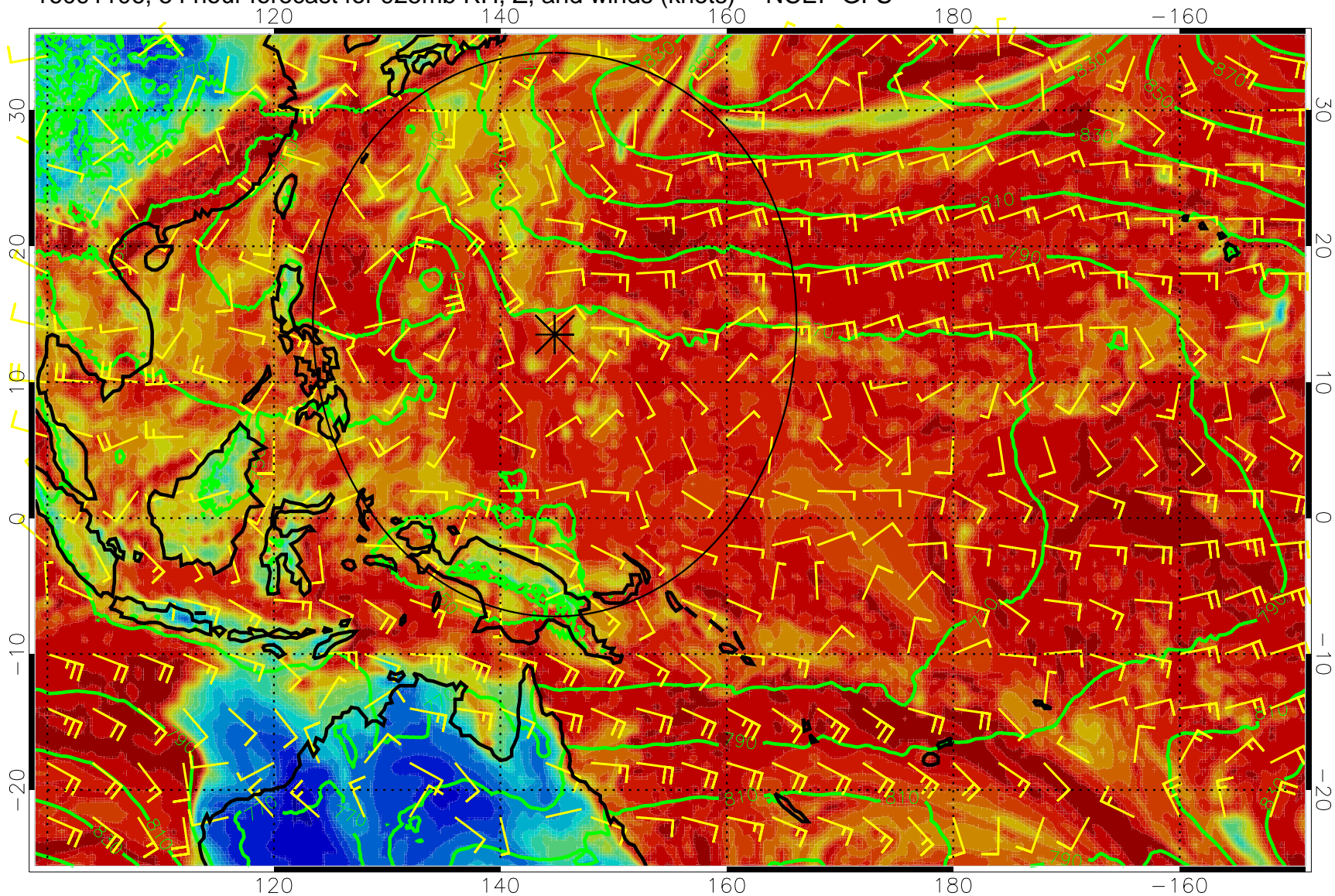
16091106, 54 hour forecast for 925mb RH, Z, and winds (knots) -- NCEP GFS
