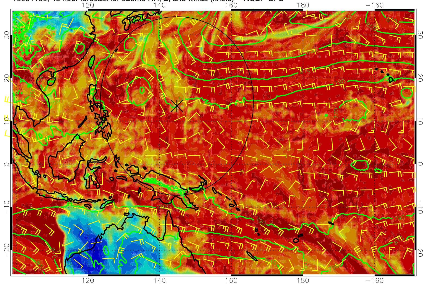
16091100, 48 hour forecast for 925mb RH, Z, and winds (knots) -- NCEP GFS
