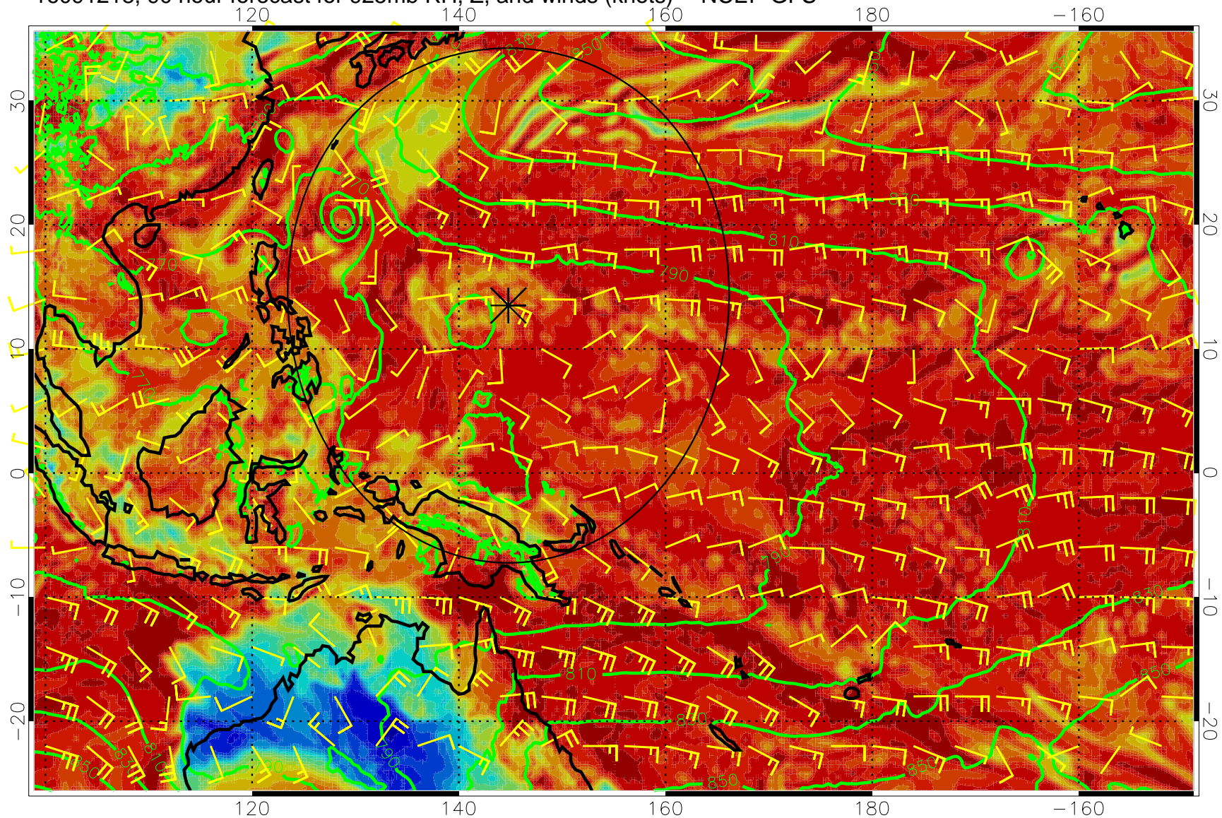
16091218, 90 hour forecast for 925mb RH, Z, and winds (knots) -- NCEP GFS
