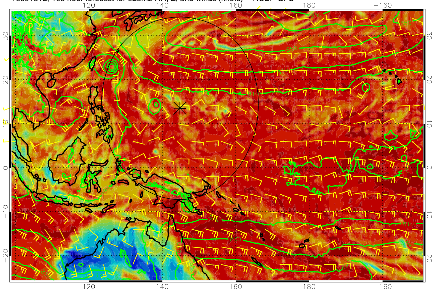
16091312, 108 hour forecast for 925mb RH, Z, and winds (knots) -- NCEP GFS
