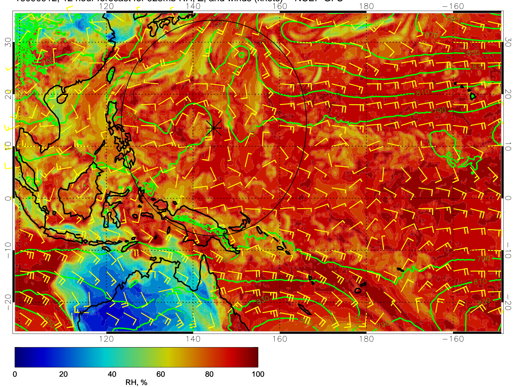
16090912, 12 hour forecast for 925mb RH, Z, and winds (knots) -- NCEP GFS
