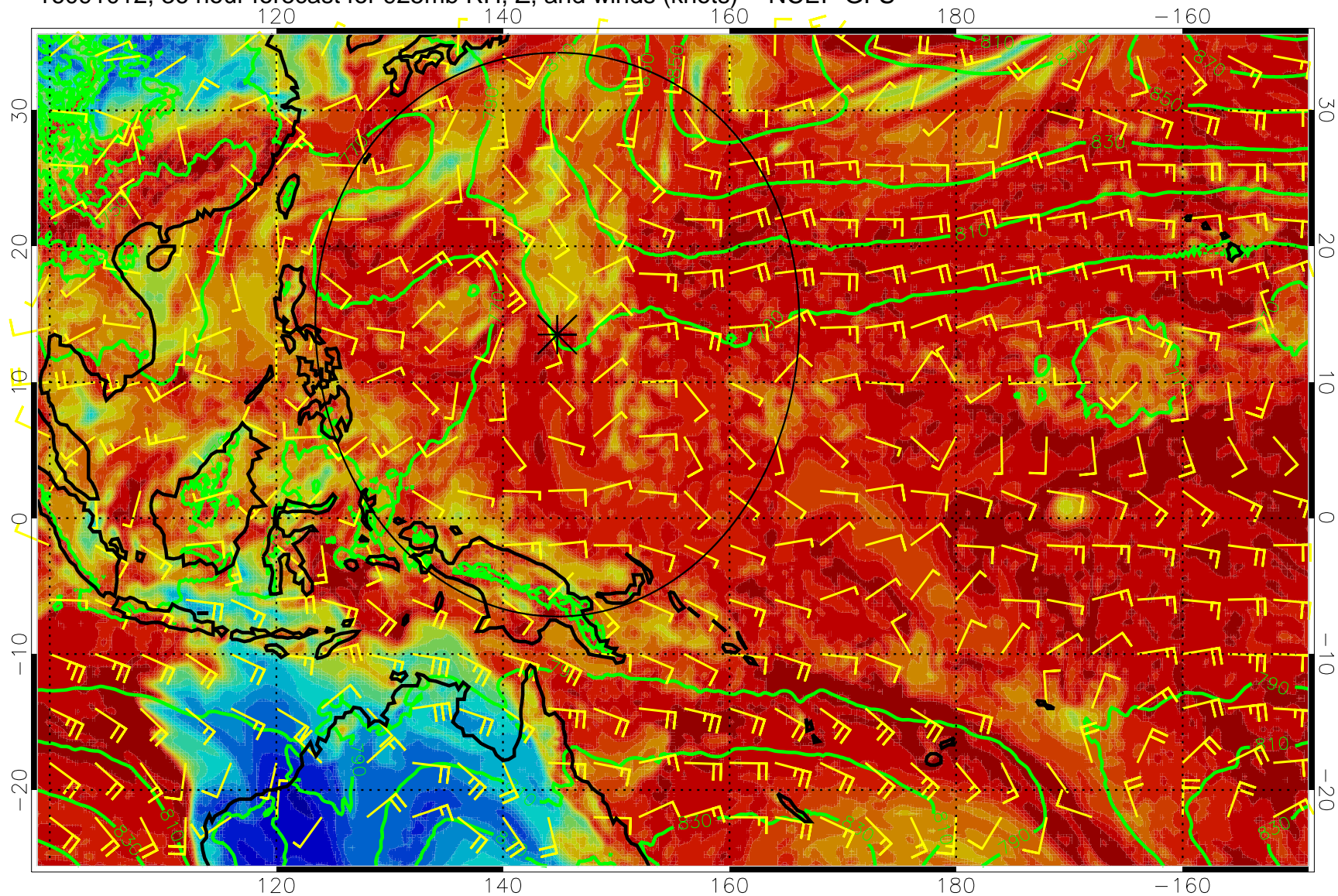
16091012, 36 hour forecast for 925mb RH, Z, and winds (knots) -- NCEP GFS
