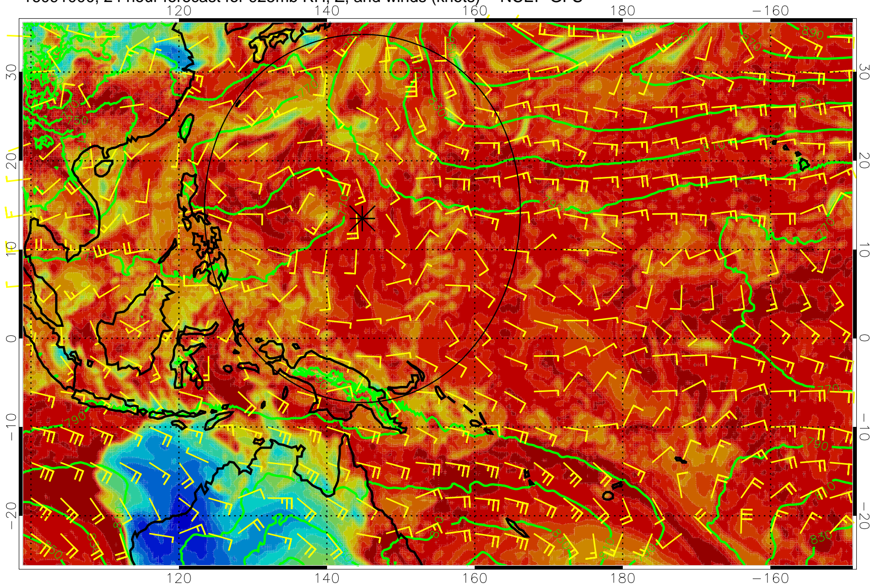
16091000, 24 hour forecast for 925mb RH, Z, and winds (knots) -- NCEP GFS
