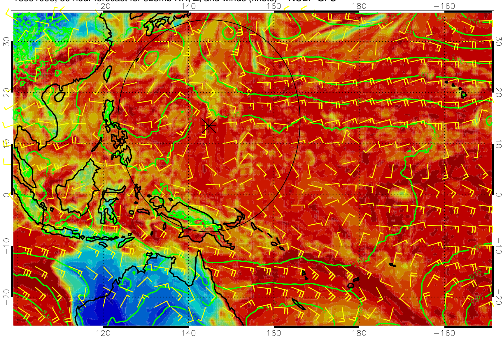
16091006, 30 hour forecast for 925mb RH, Z, and winds (knots) -- NCEP GFS
