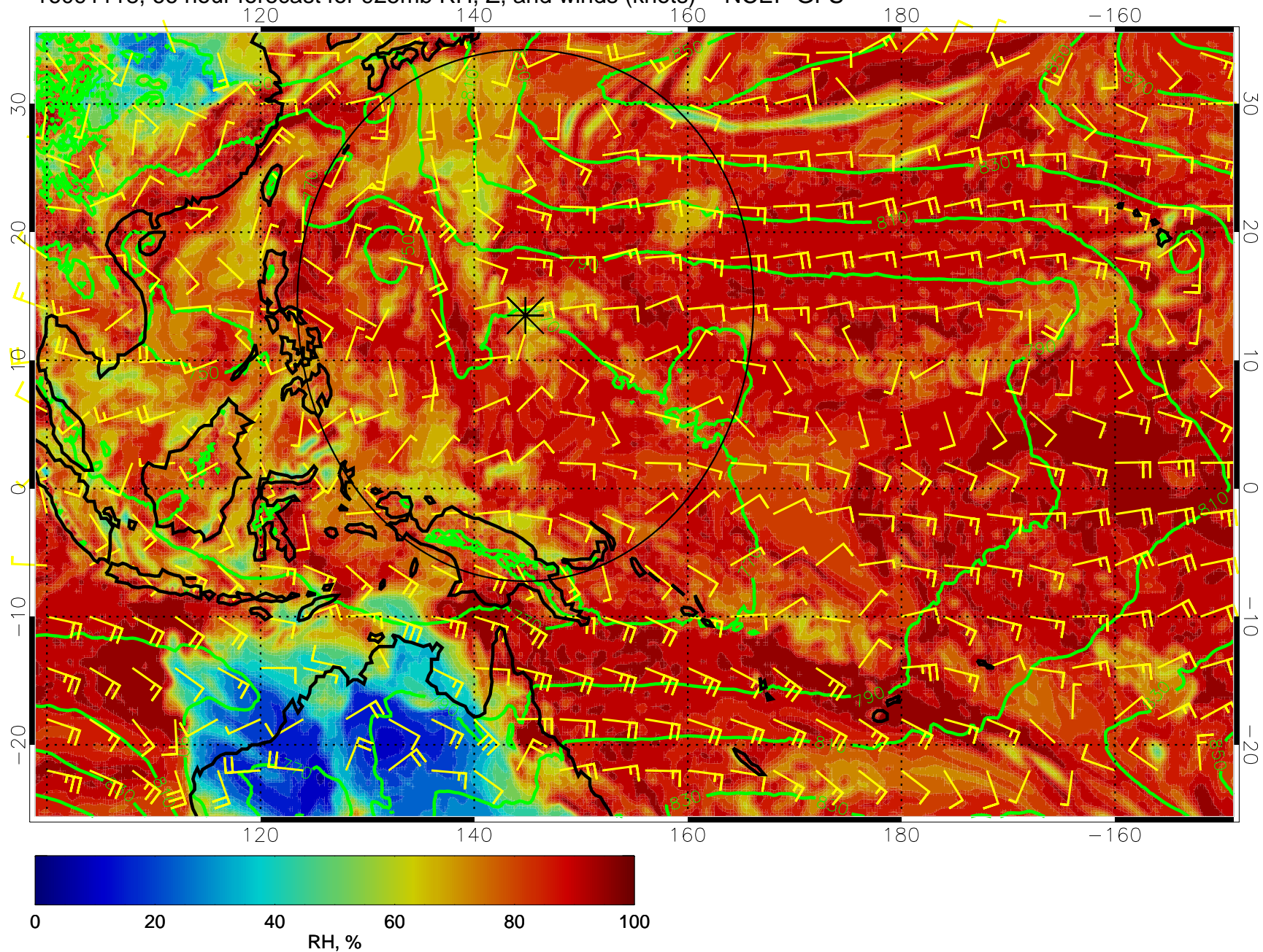
16091118, 66 hour forecast for 925mb RH, Z, and winds (knots) -- NCEP GFS
