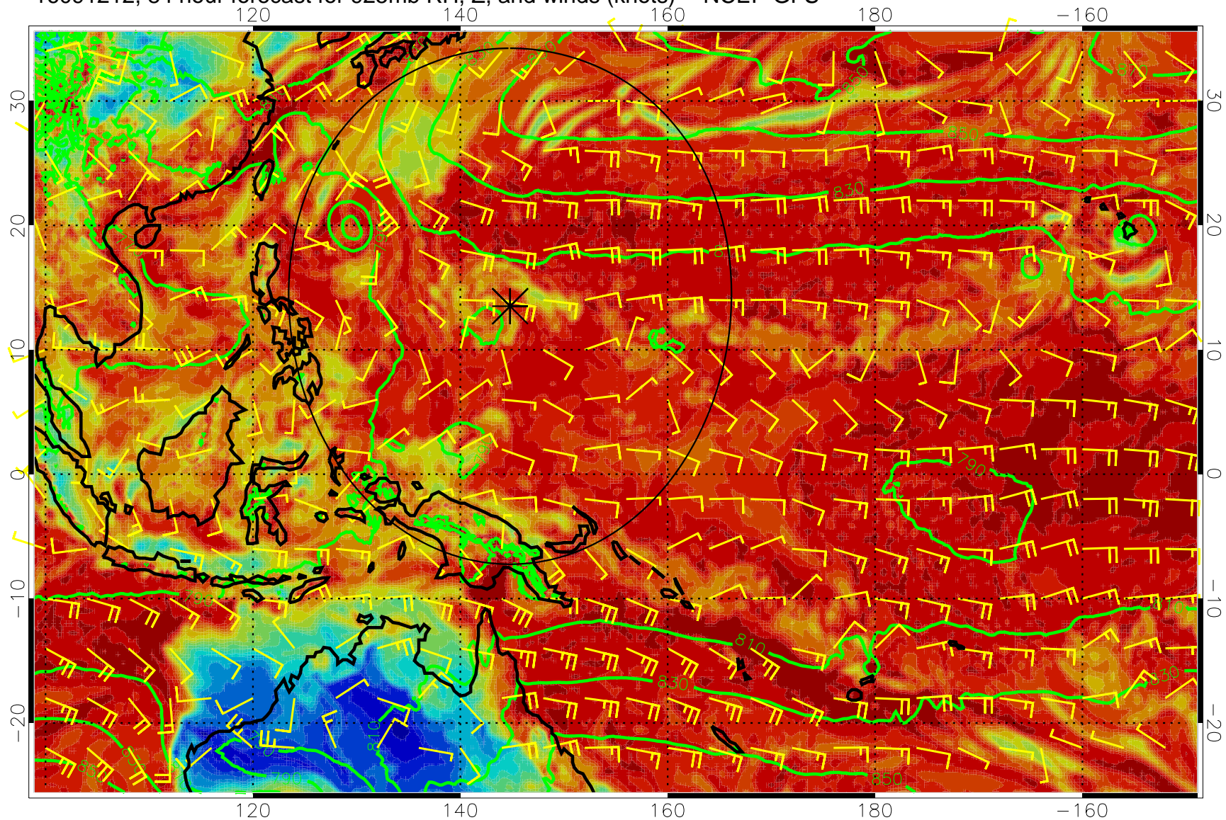
16091212, 84 hour forecast for 925mb RH, Z, and winds (knots) -- NCEP GFS
