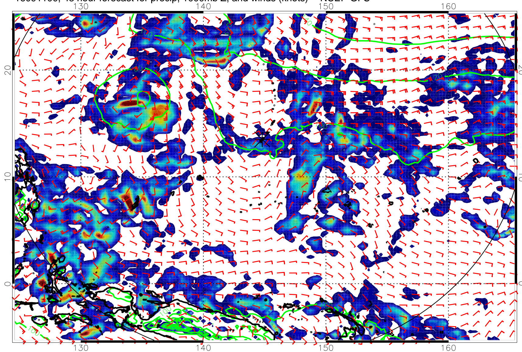
16091100, 48 hour forecast for precip, 1000mb Z, and winds (knots) -- NCEP GFS
