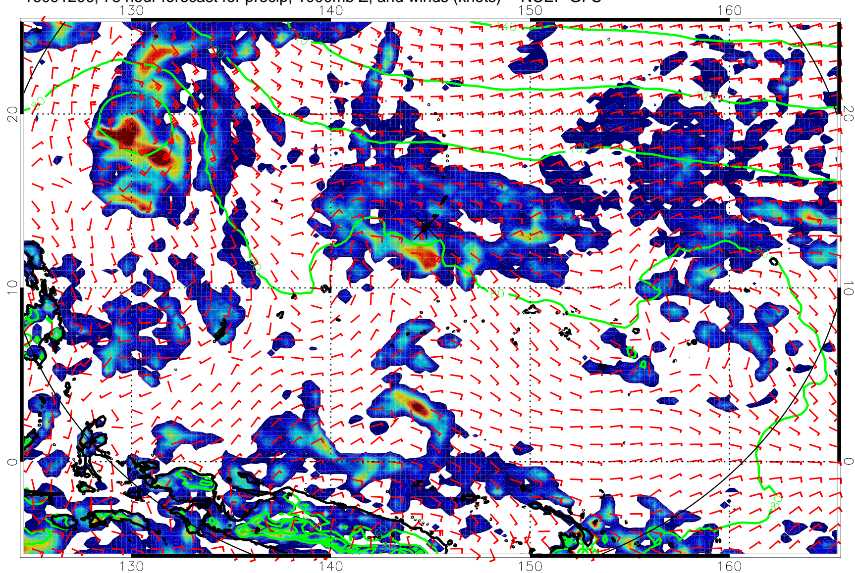
16091206, 78 hour forecast for precip, 1000mb Z, and winds (knots) -- NCEP GFS
