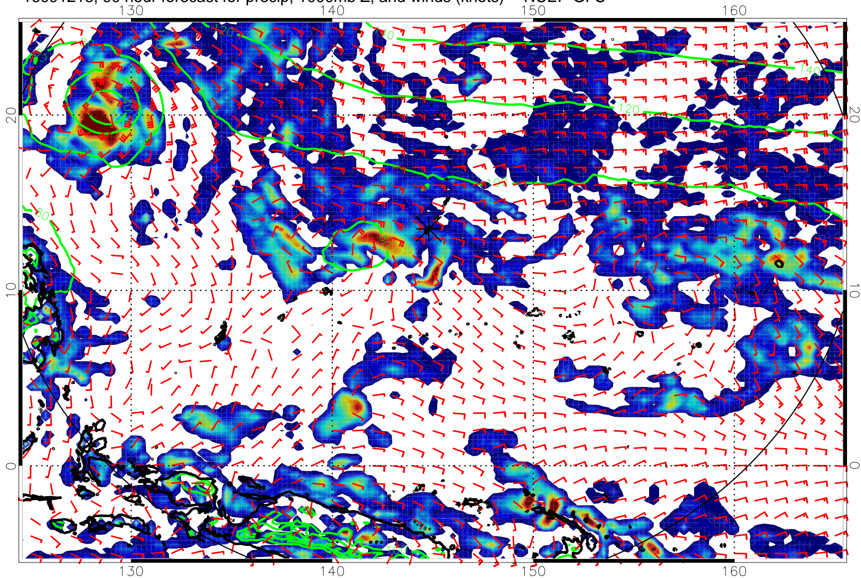
16091218, 90 hour forecast for precip, 1000mb Z, and winds (knots) -- NCEP GFS
