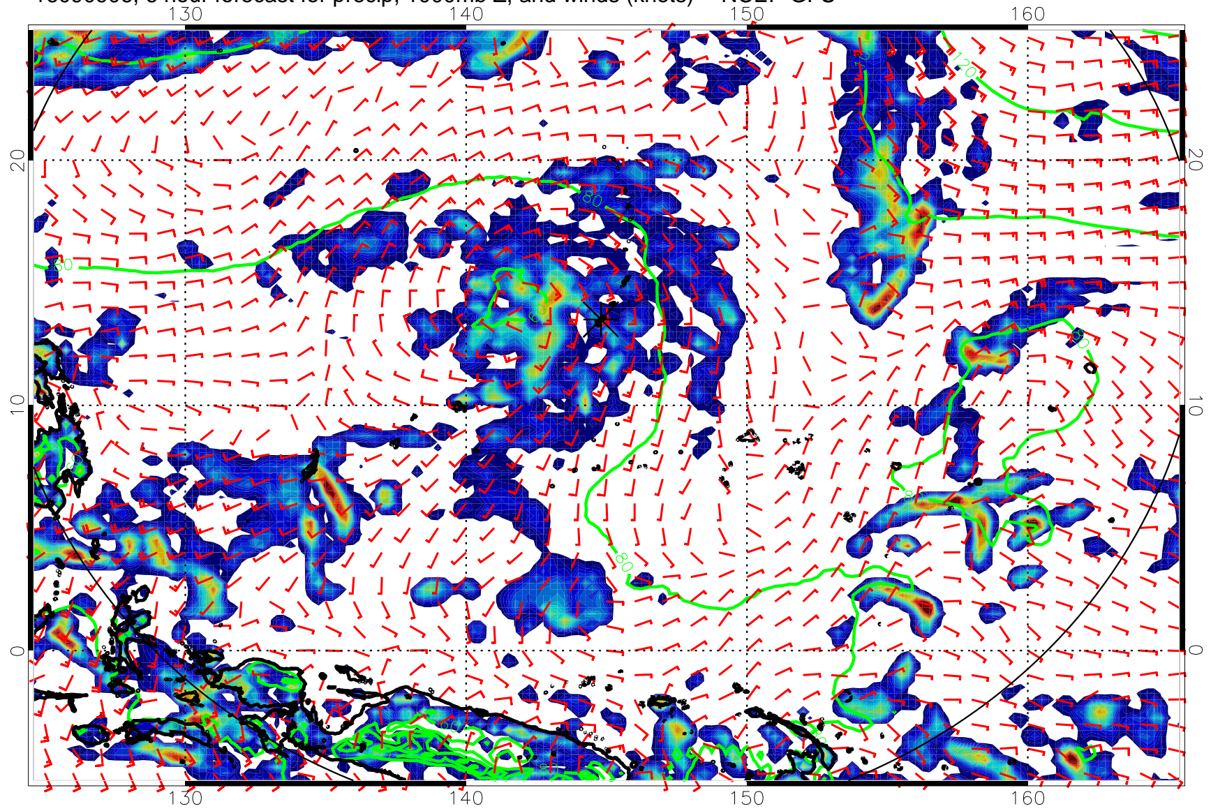
16090906, 6 hour forecast for precip, 1000mb Z, and winds (knots) -- NCEP GFS
