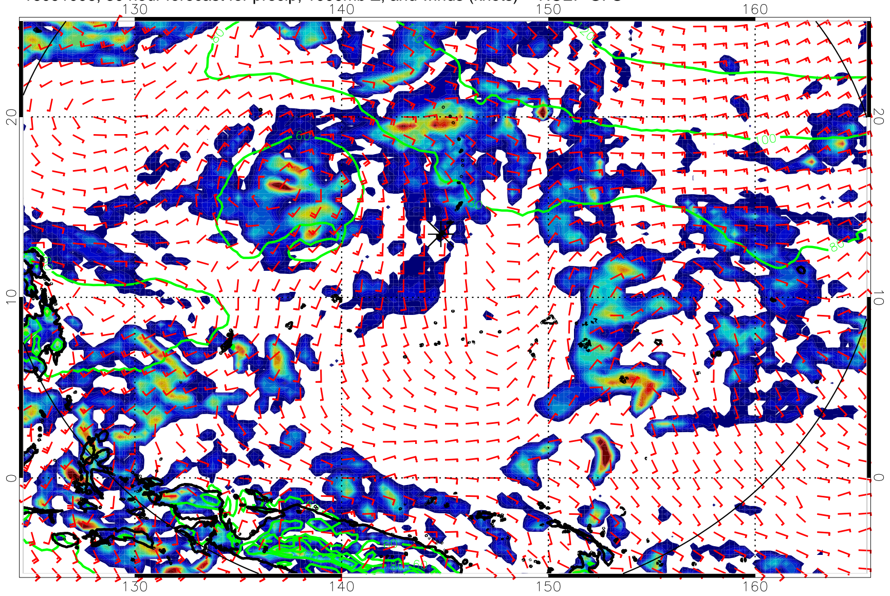
16091006, 30 hour forecast for precip, 1000mb Z, and winds (knots) -- NCEP GFS
