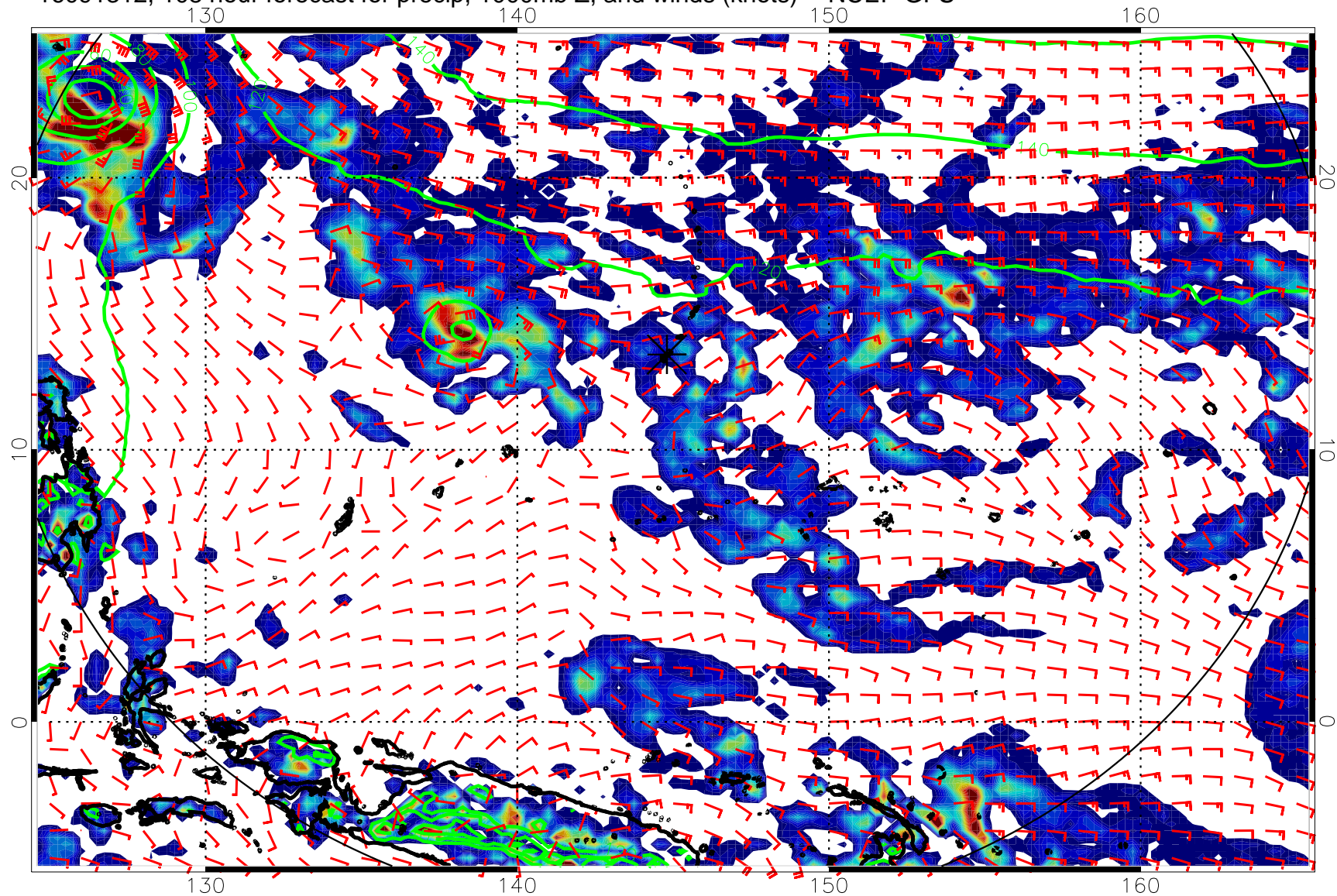
16091312, 108 hour forecast for precip, 1000mb Z, and winds (knots) -- NCEP GFS
