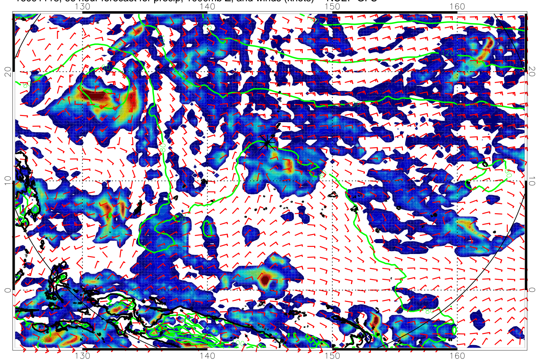
16091118, 66 hour forecast for precip, 1000mb Z, and winds (knots) -- NCEP GFS
