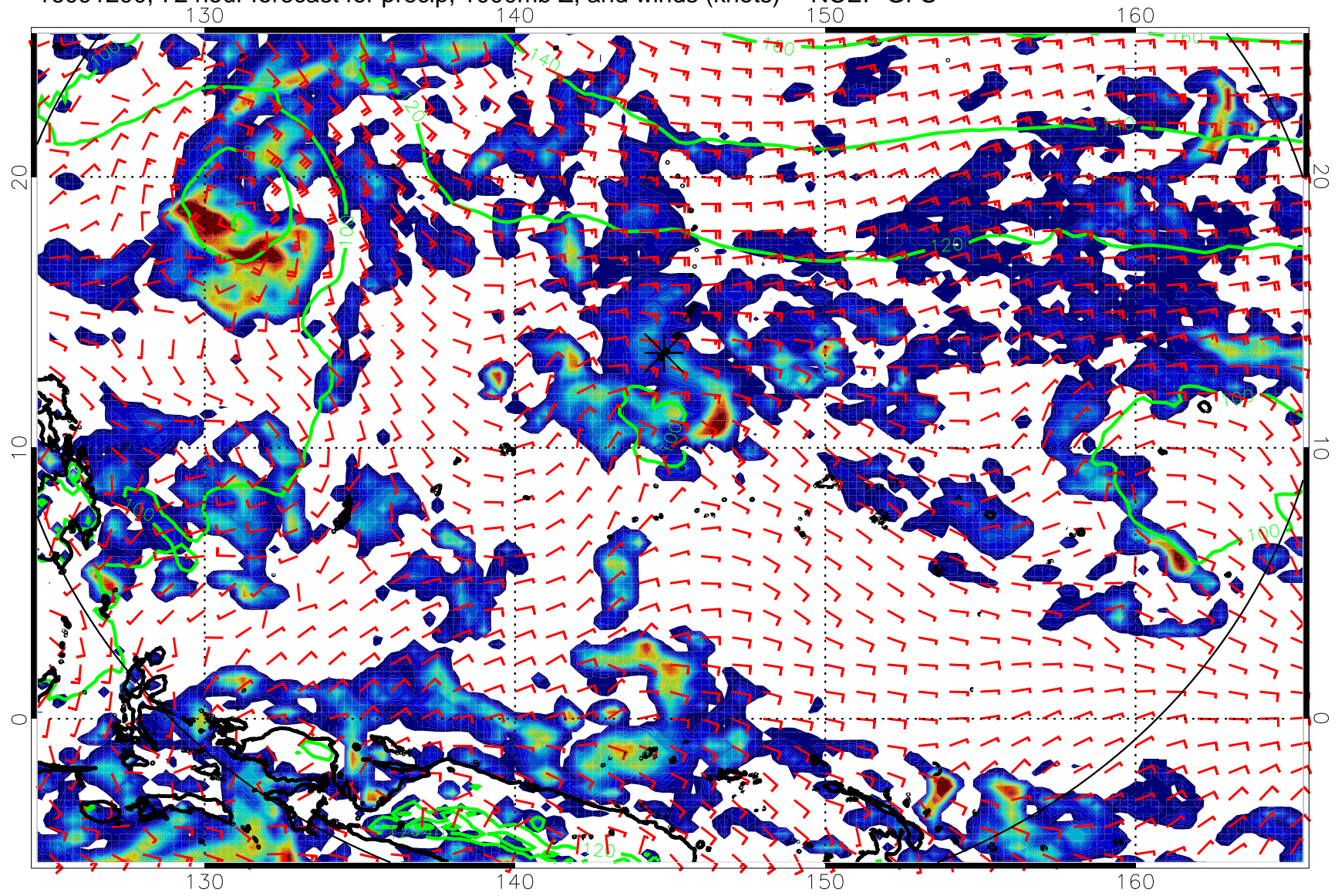
16091200, 72 hour forecast for precip, 1000mb Z, and winds (knots) -- NCEP GFS
