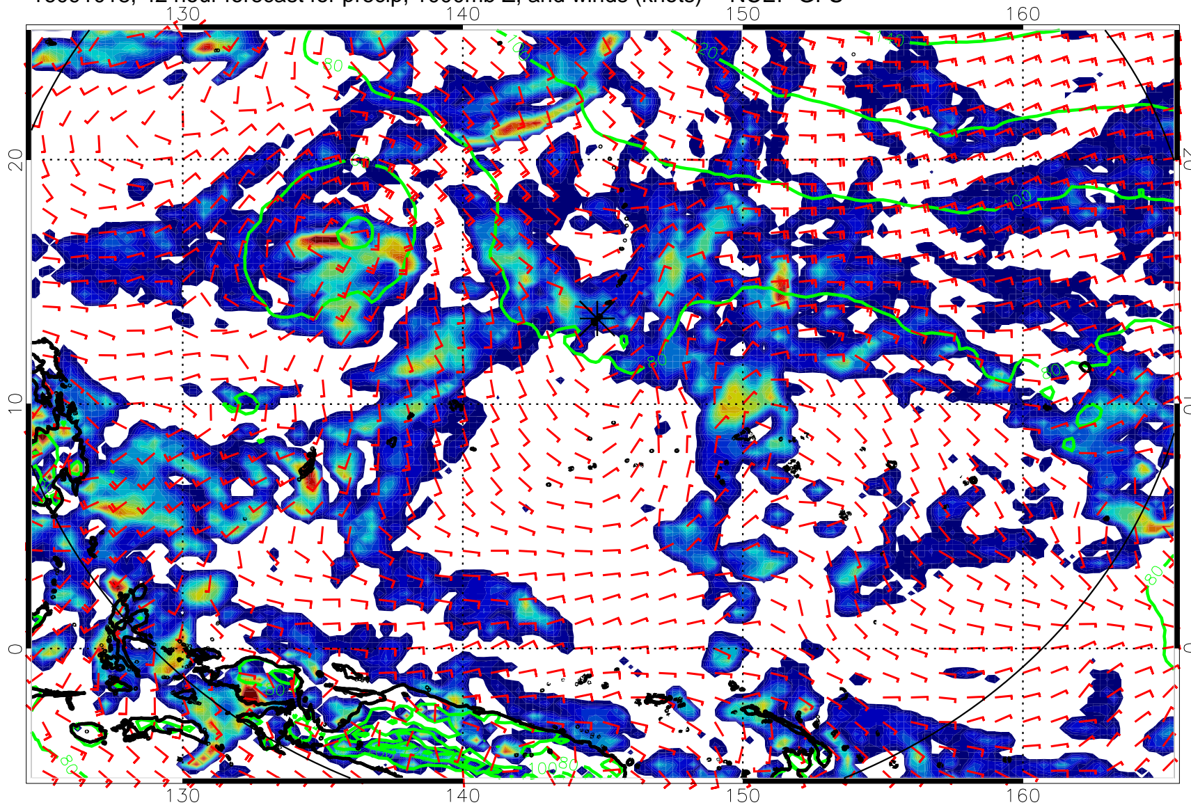
16091018, 42 hour forecast for precip, 1000mb Z, and winds (knots) -- NCEP GFS
