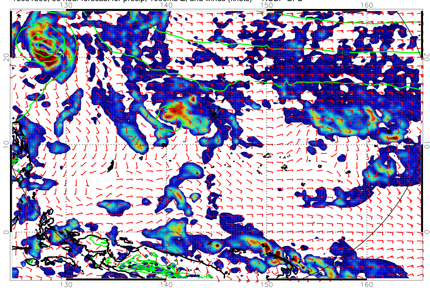
16091300, 96 hour forecast for precip, 1000mb Z, and winds (knots) -- NCEP GFS
