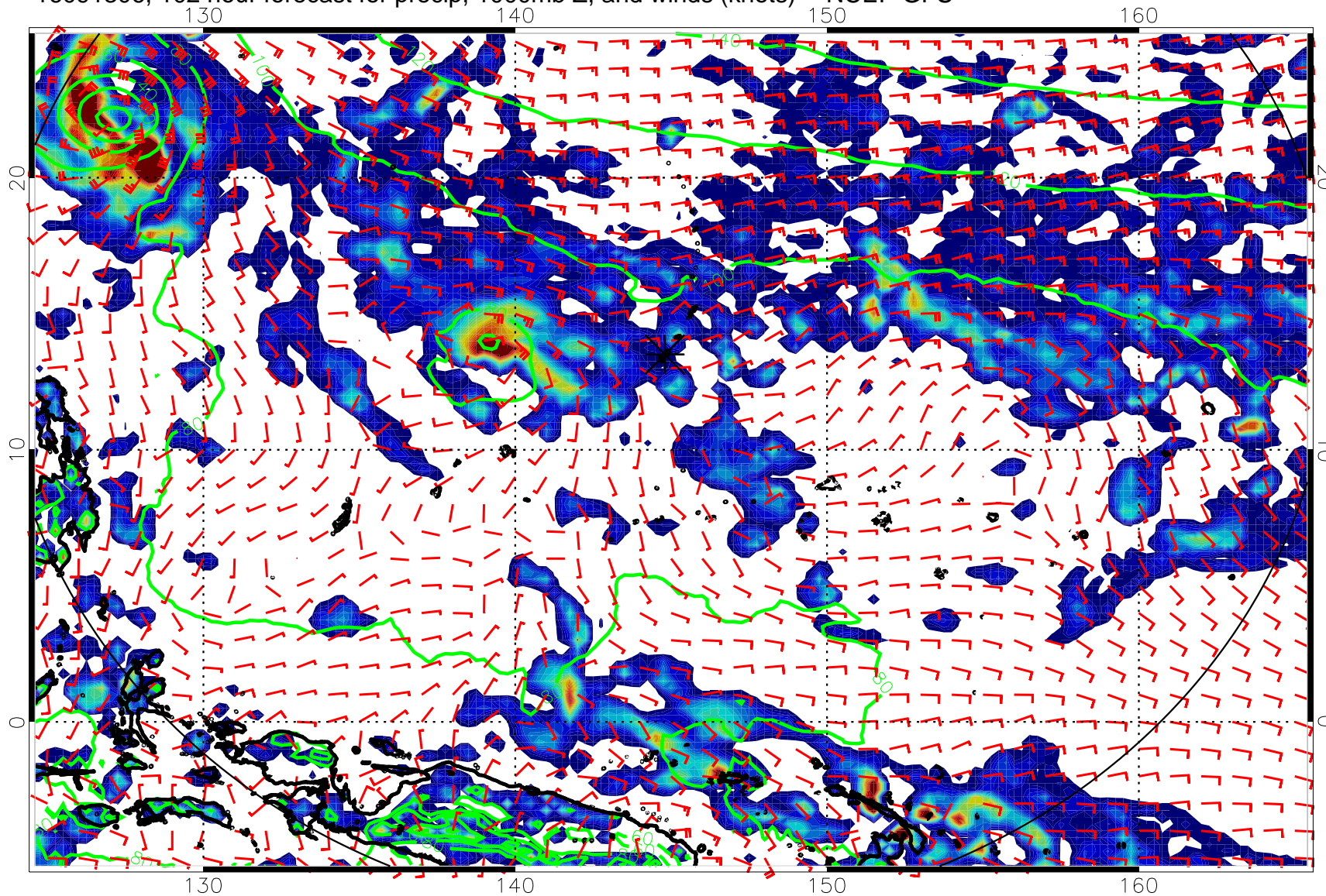
16091306, 102 hour forecast for precip, 1000mb Z, and winds (knots) -- NCEP GFS
