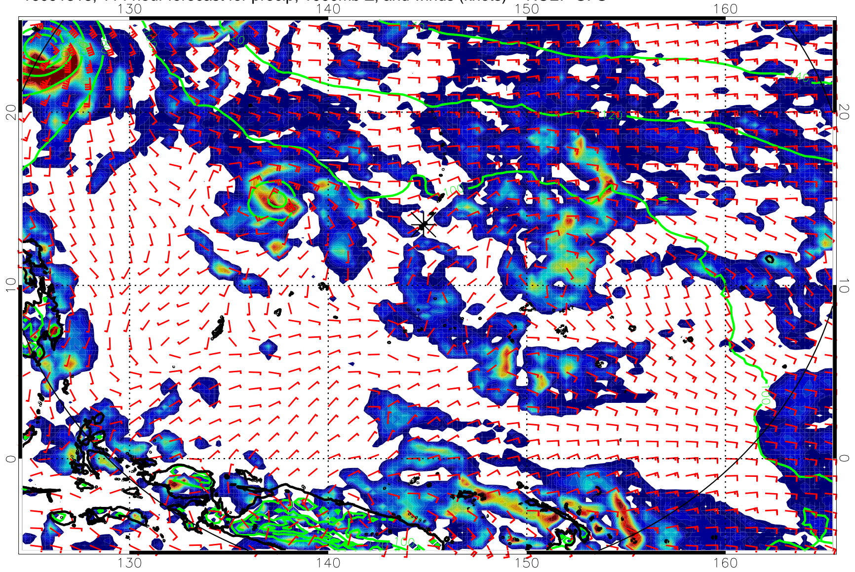
16091318, 114 hour forecast for precip, 1000mb Z, and winds (knots) -- NCEP GFS
