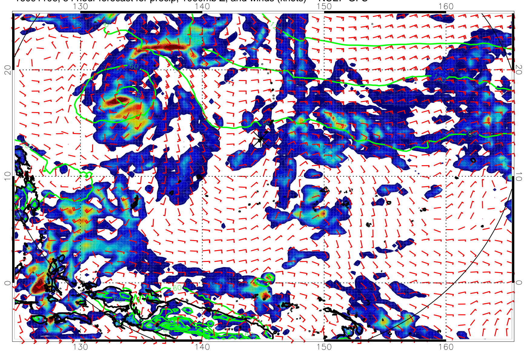
16091106, 54 hour forecast for precip, 1000mb Z, and winds (knots) -- NCEP GFS
