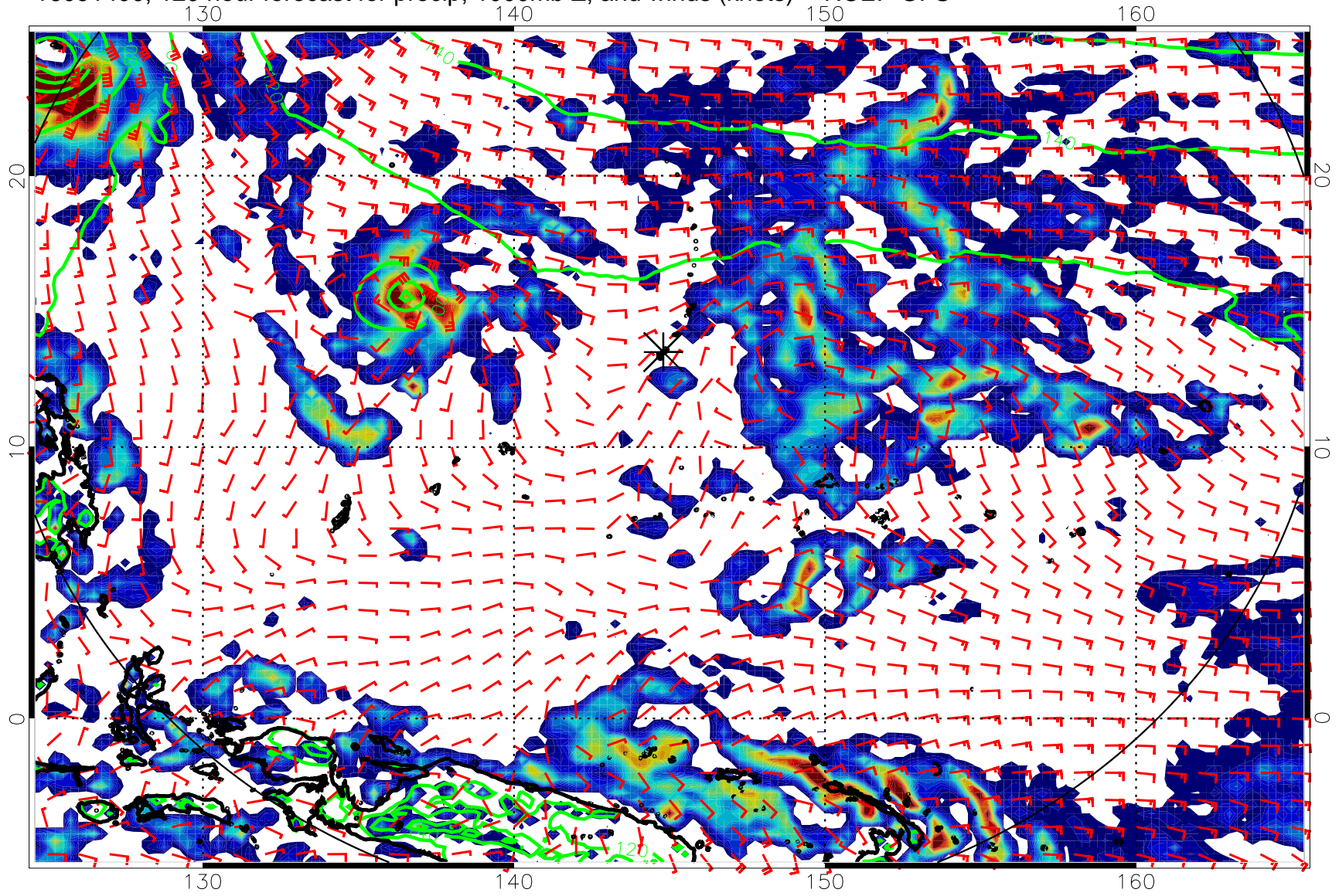
16091400, 120 hour forecast for precip, 1000mb Z, and winds (knots) -- NCEP GFS
