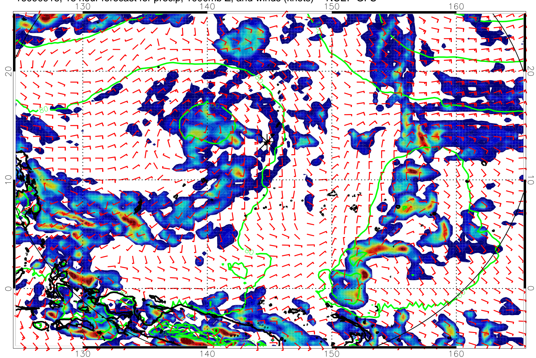
16090918, 18 hour forecast for precip, 1000mb Z, and winds (knots) -- NCEP GFS
