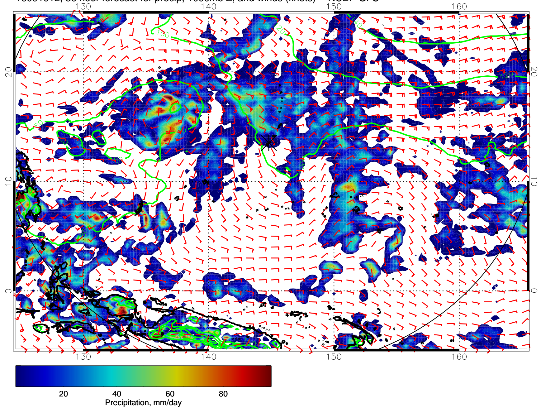
16091012, 36 hour forecast for precip, 1000mb Z, and winds (knots) -- NCEP GFS
