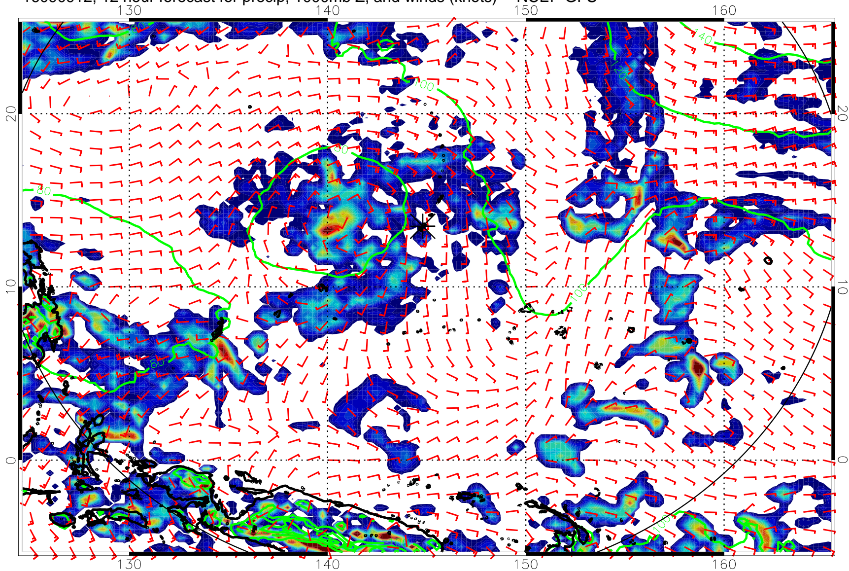
16090912, 12 hour forecast for precip, 1000mb Z, and winds (knots) -- NCEP GFS
