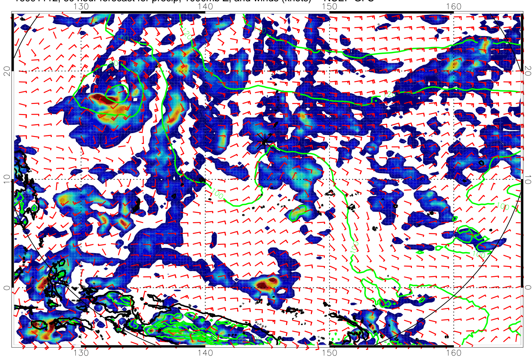
16091112, 60 hour forecast for precip, 1000mb Z, and winds (knots) -- NCEP GFS
