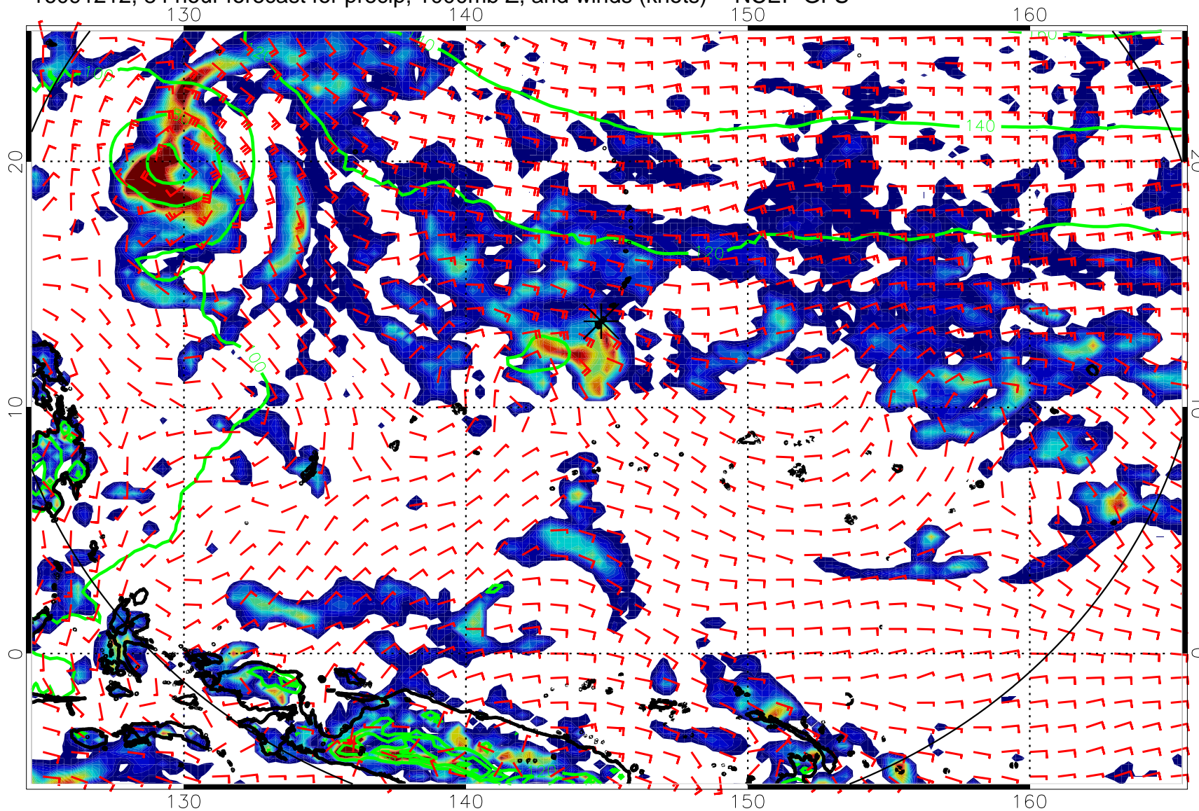
16091212, 84 hour forecast for precip, 1000mb Z, and winds (knots) -- NCEP GFS
