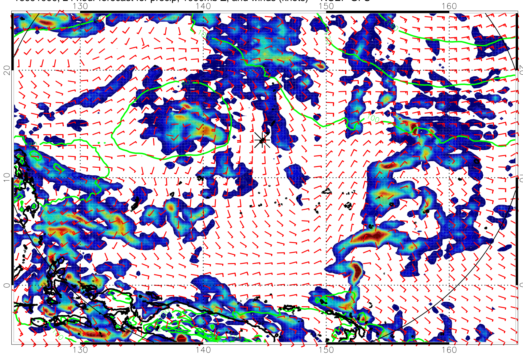
16091000, 24 hour forecast for precip, 1000mb Z, and winds (knots) -- NCEP GFS
