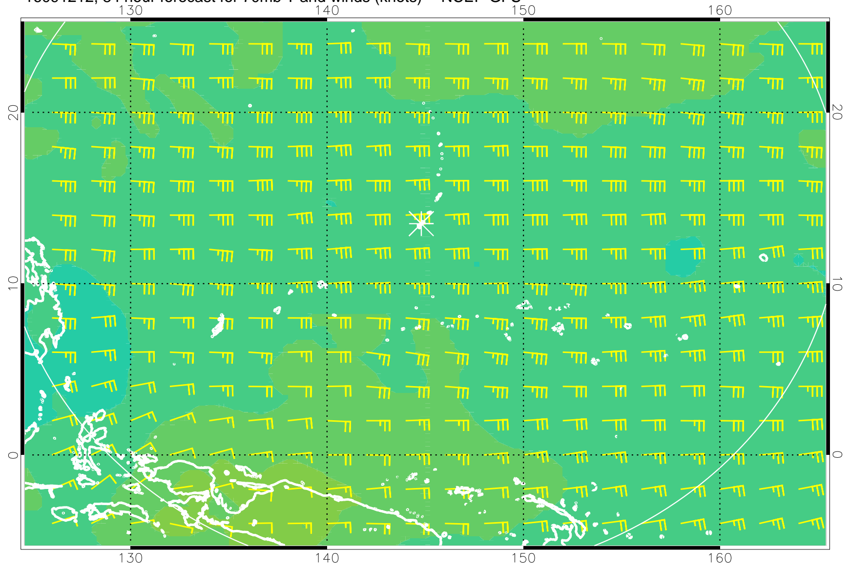
16091212, 84 hour forecast for 70mb T and winds (knots) -- NCEP GFS
