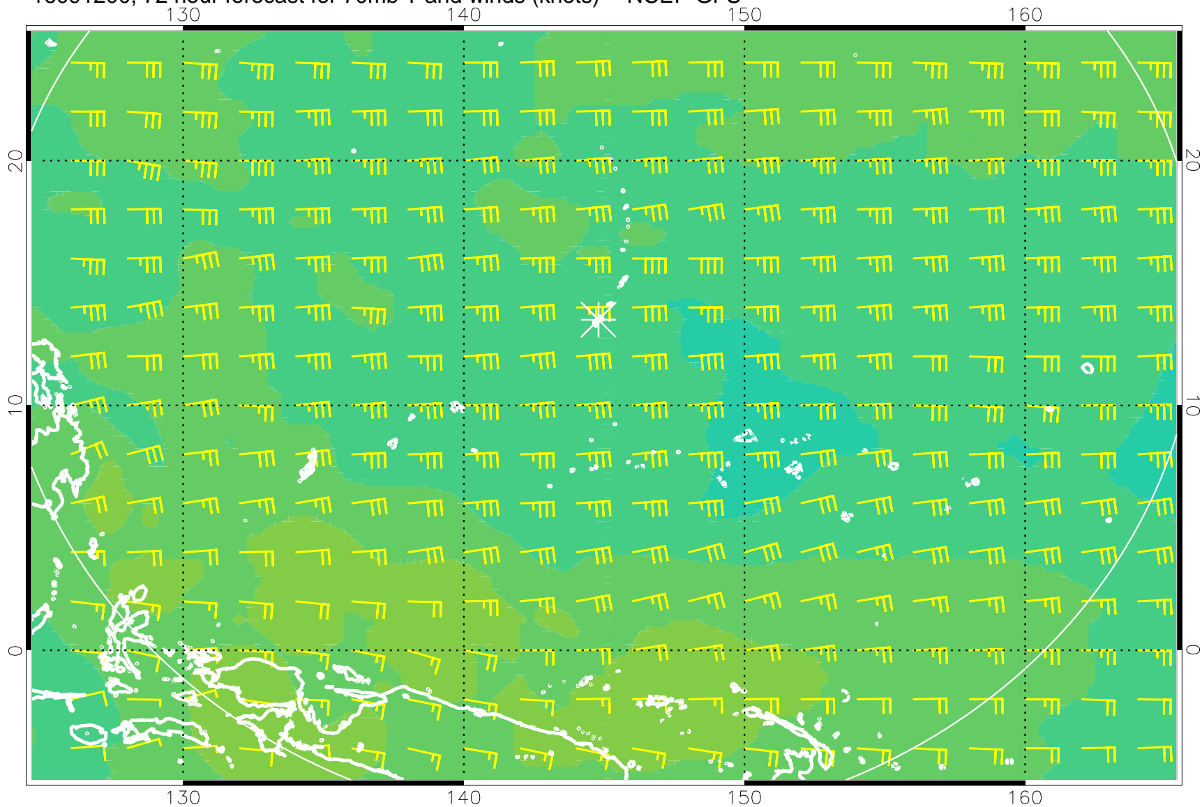
16091200, 72 hour forecast for 70mb T and winds (knots) -- NCEP GFS
