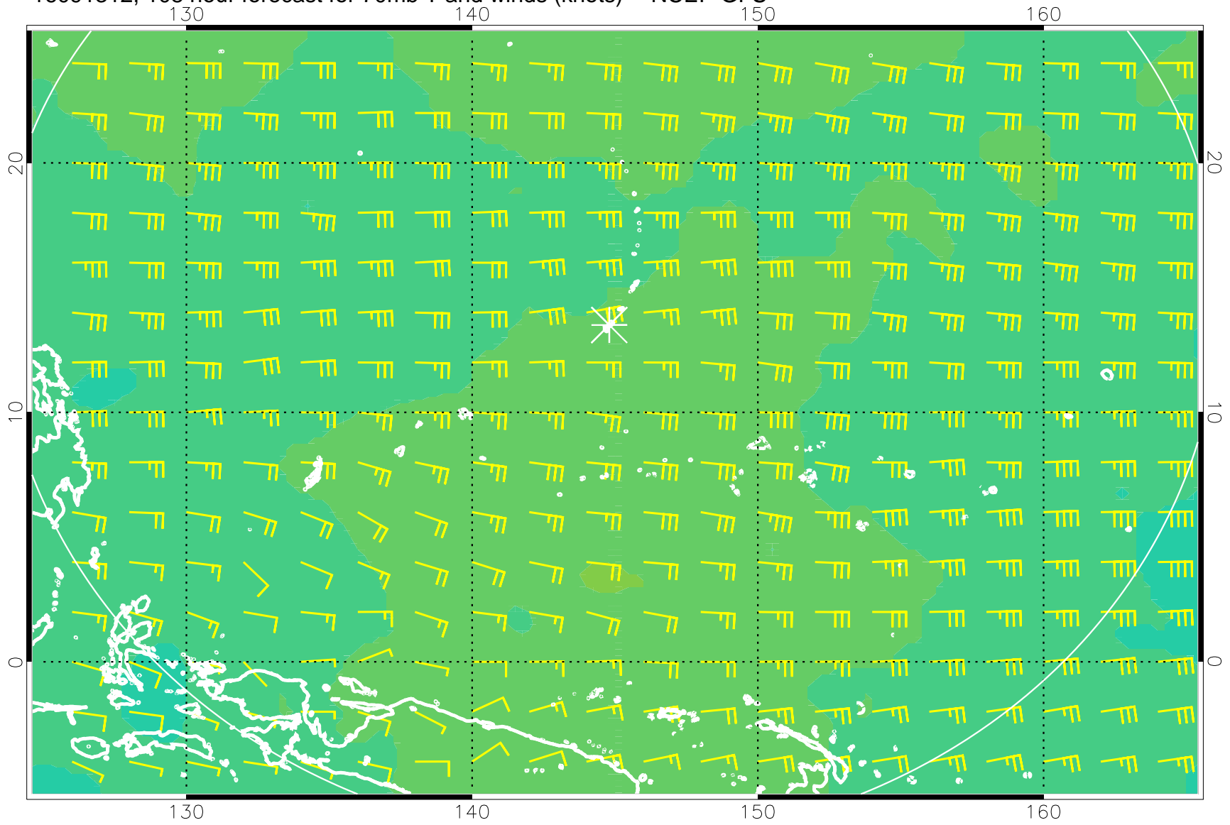
16091312, 108 hour forecast for 70mb T and winds (knots) -- NCEP GFS
