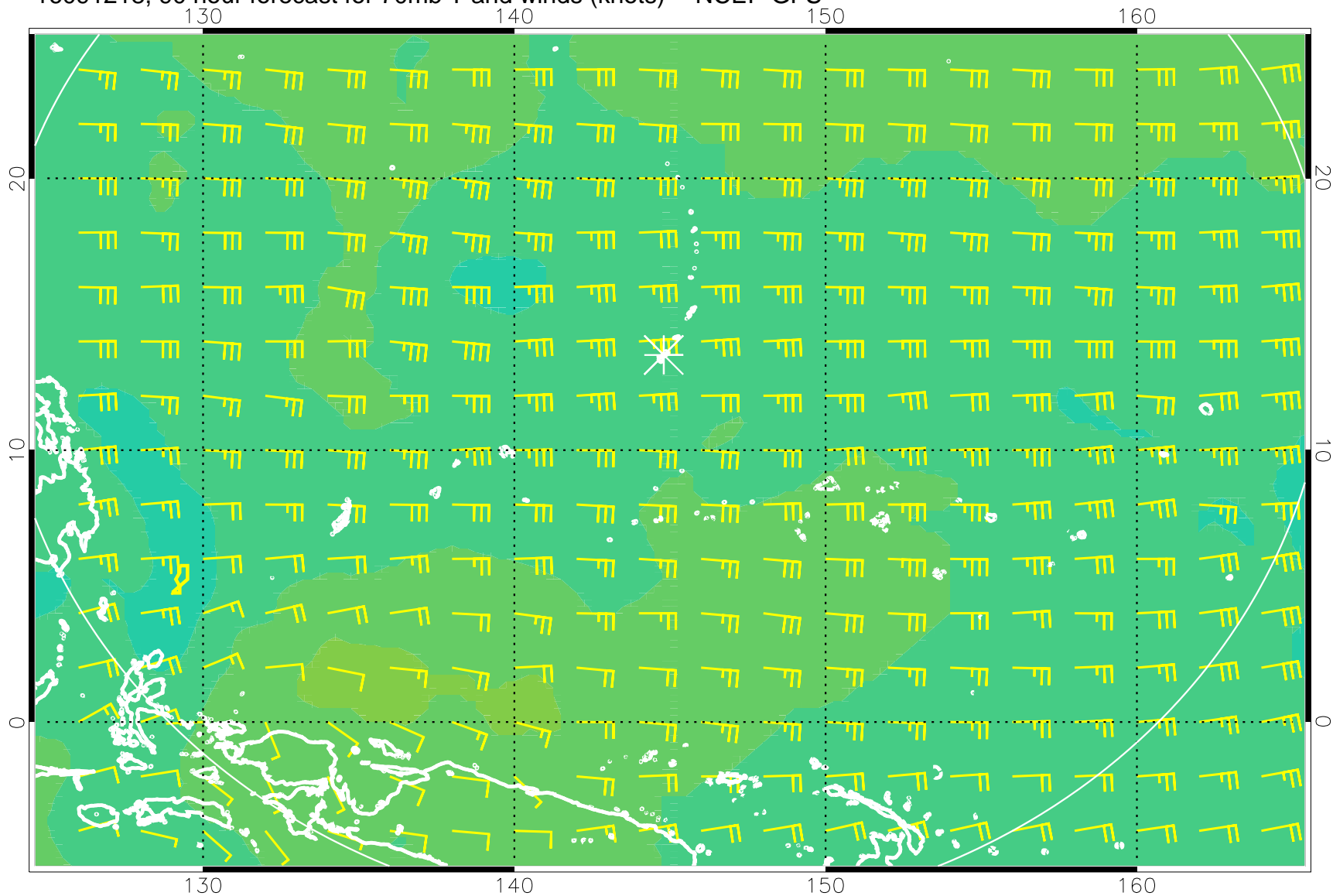
16091218, 90 hour forecast for 70mb T and winds (knots) -- NCEP GFS
