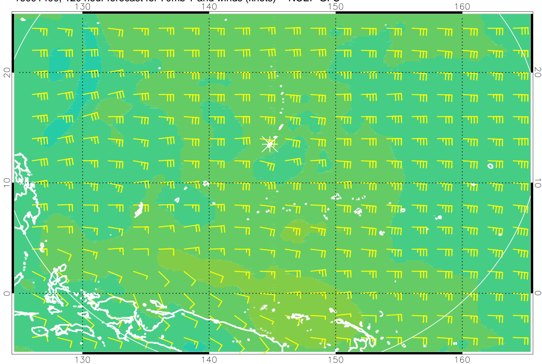
16091400, 120 hour forecast for 70mb T and winds (knots) -- NCEP GFS
