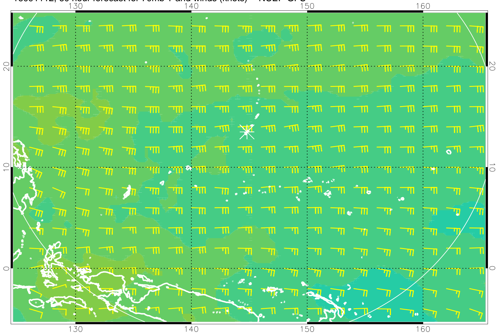
16091112, 60 hour forecast for 70mb T and winds (knots) -- NCEP GFS
