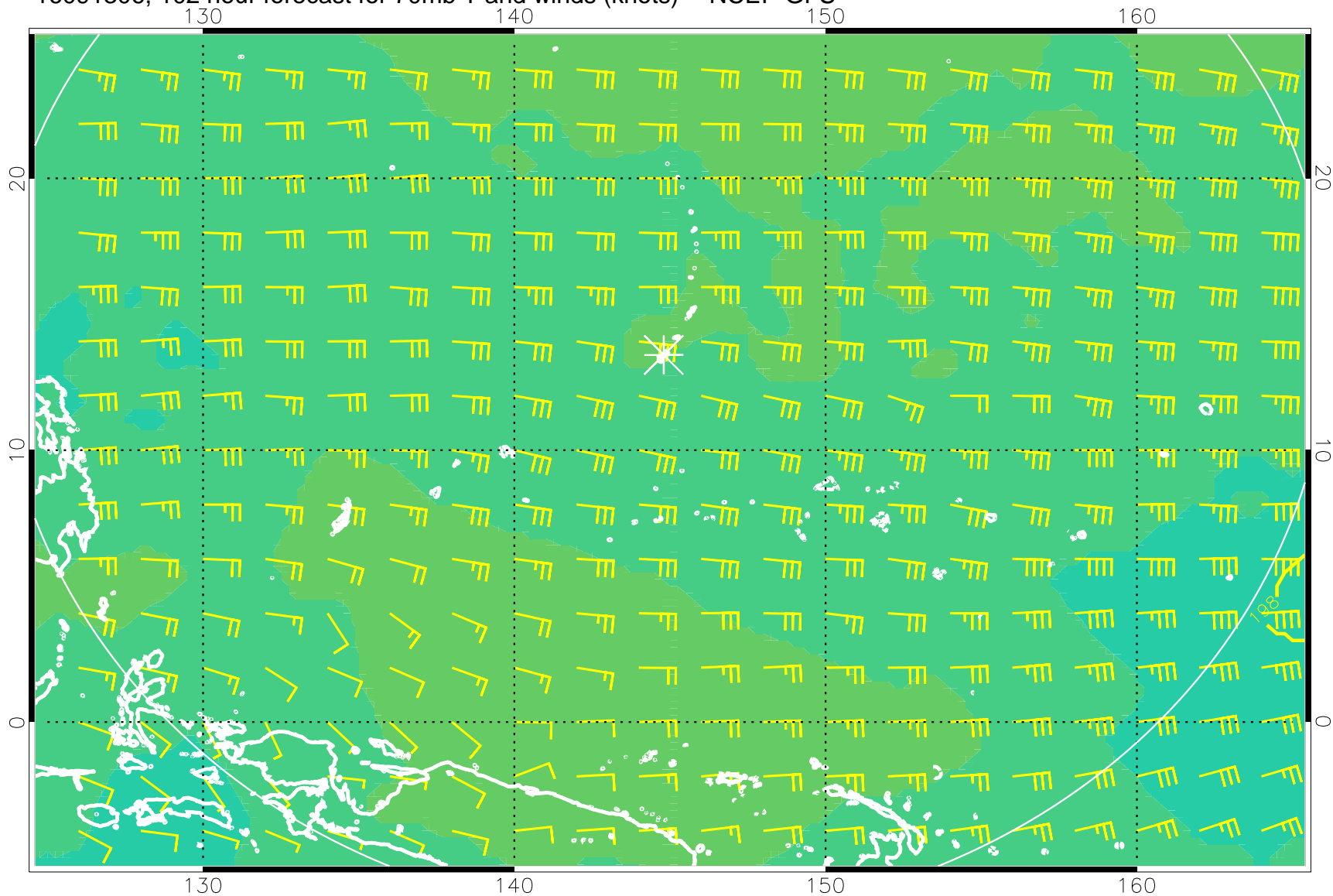
16091306, 102 hour forecast for 70mb T and winds (knots) -- NCEP GFS
