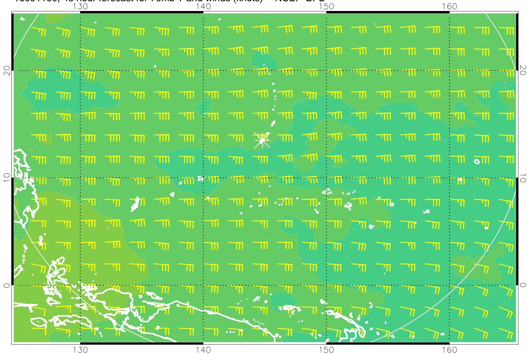
16091100, 48 hour forecast for 70mb T and winds (knots) -- NCEP GFS
