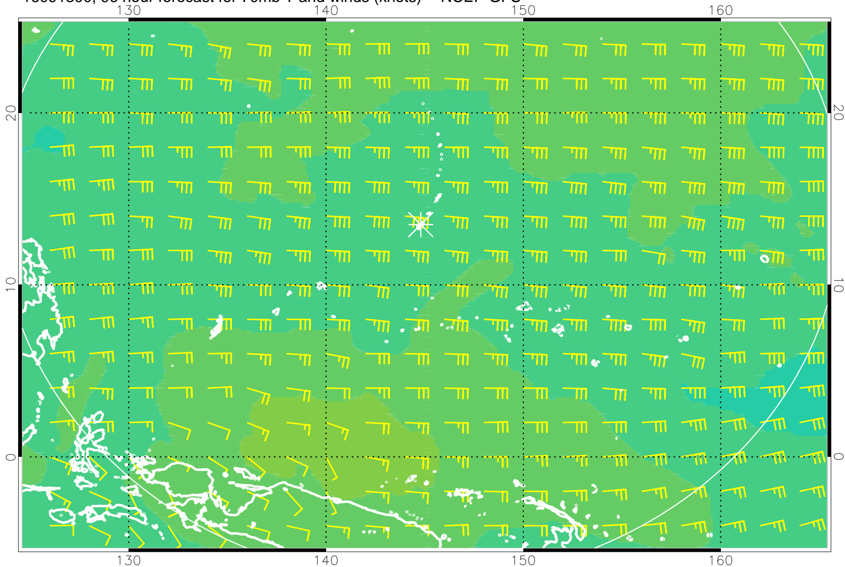
16091300, 96 hour forecast for 70mb T and winds (knots) -- NCEP GFS
