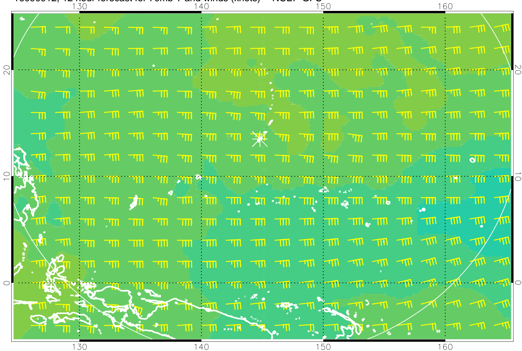
16090912, 12 hour forecast for 70mb T and winds (knots) -- NCEP GFS
