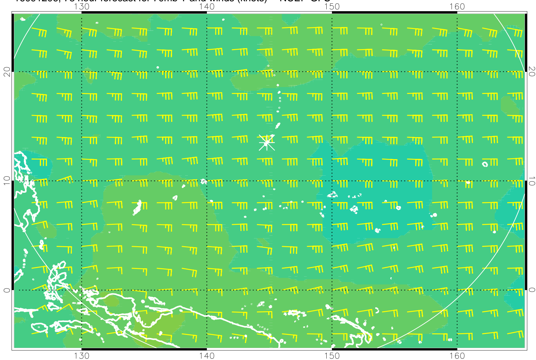
16091206, 78 hour forecast for 70mb T and winds (knots) -- NCEP GFS
