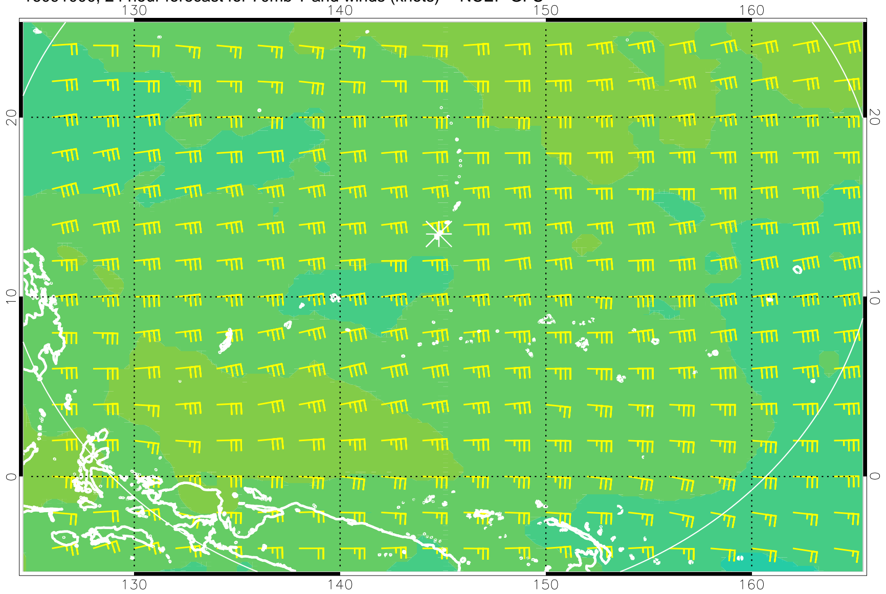
16091000, 24 hour forecast for 70mb T and winds (knots) -- NCEP GFS
