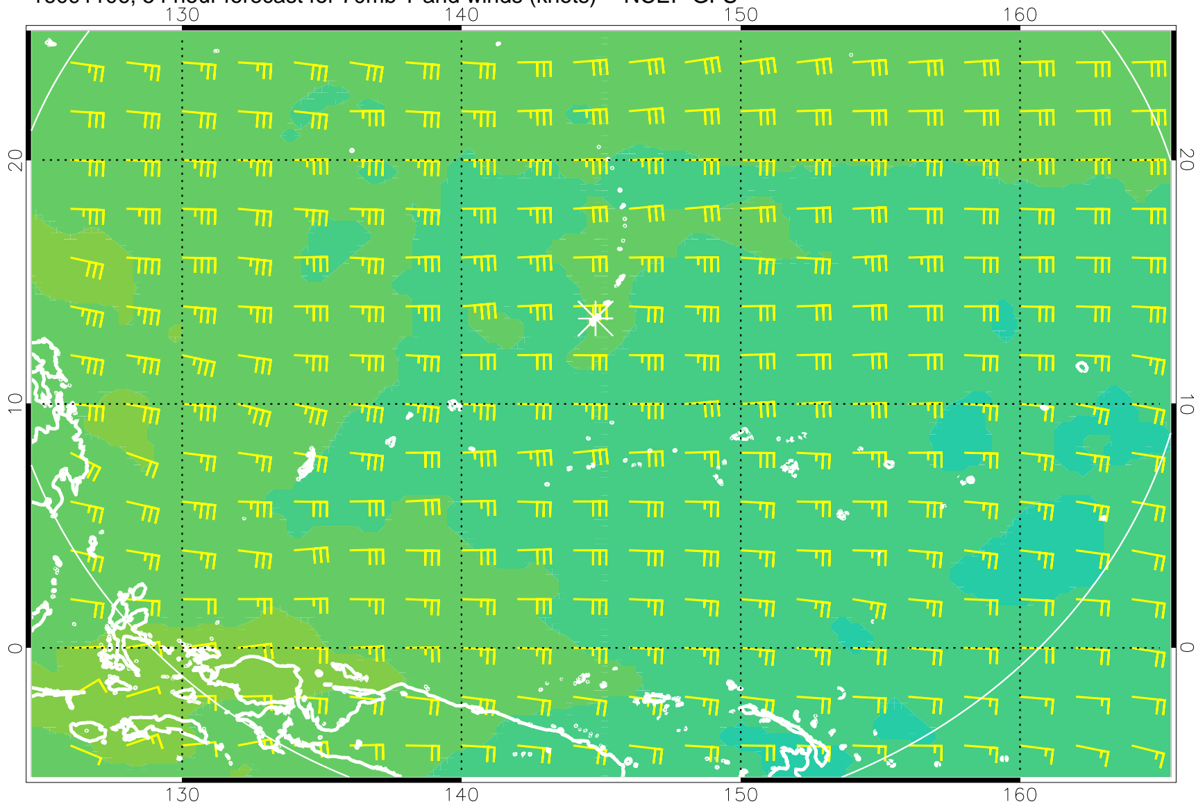
16091106, 54 hour forecast for 70mb T and winds (knots) -- NCEP GFS
