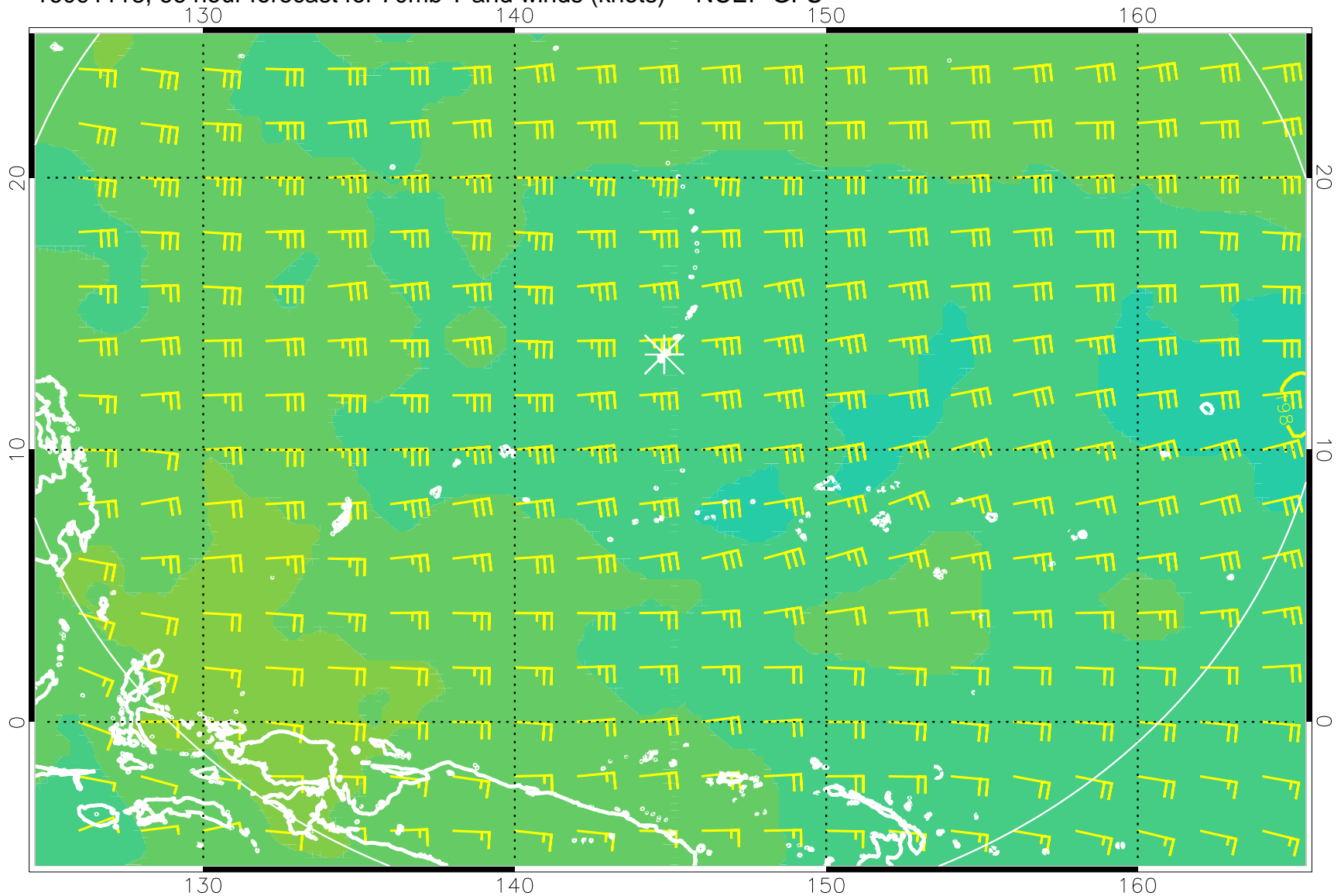
16091118, 66 hour forecast for 70mb T and winds (knots) -- NCEP GFS
