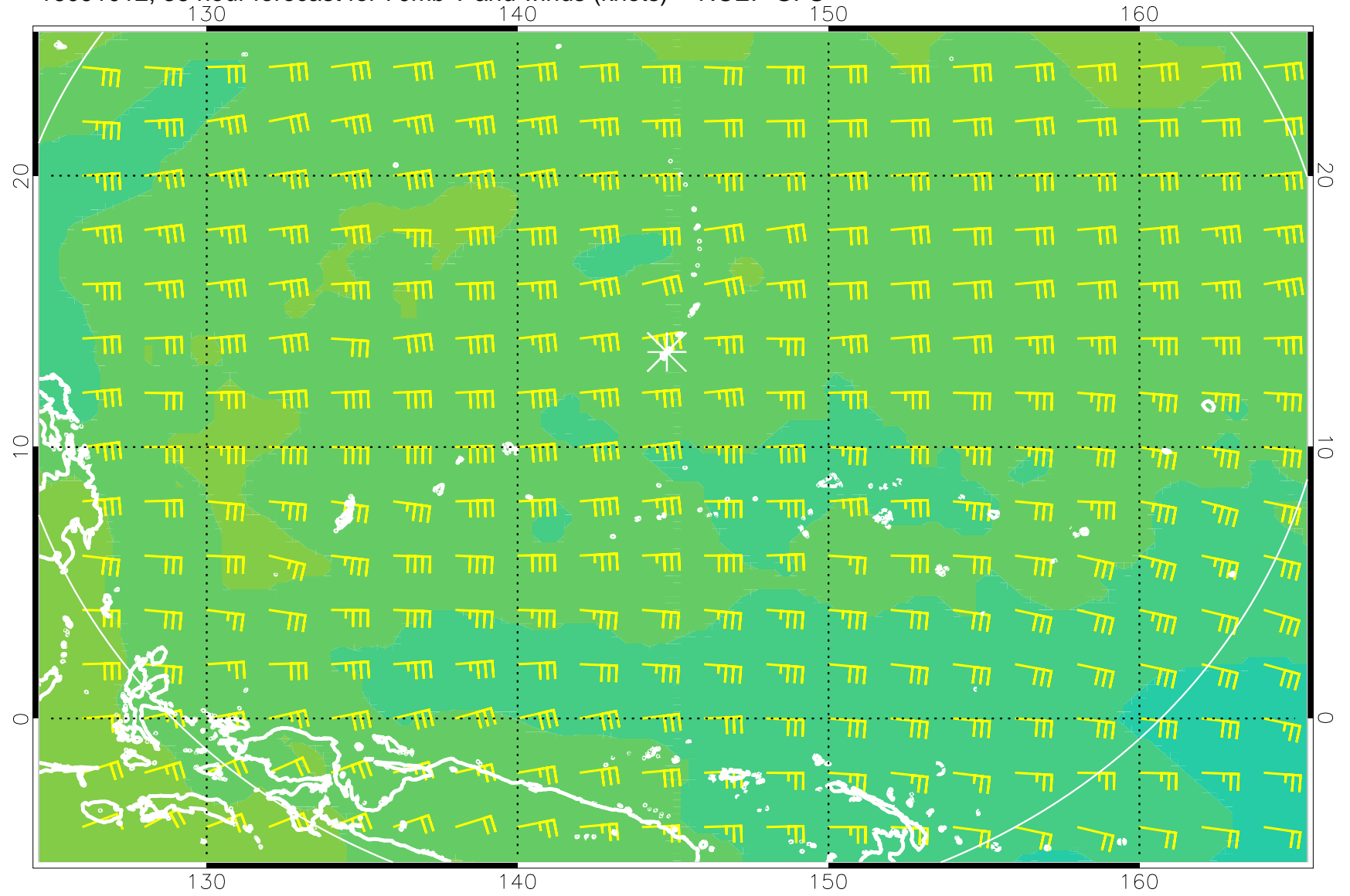
16091012, 36 hour forecast for 70mb T and winds (knots) -- NCEP GFS
