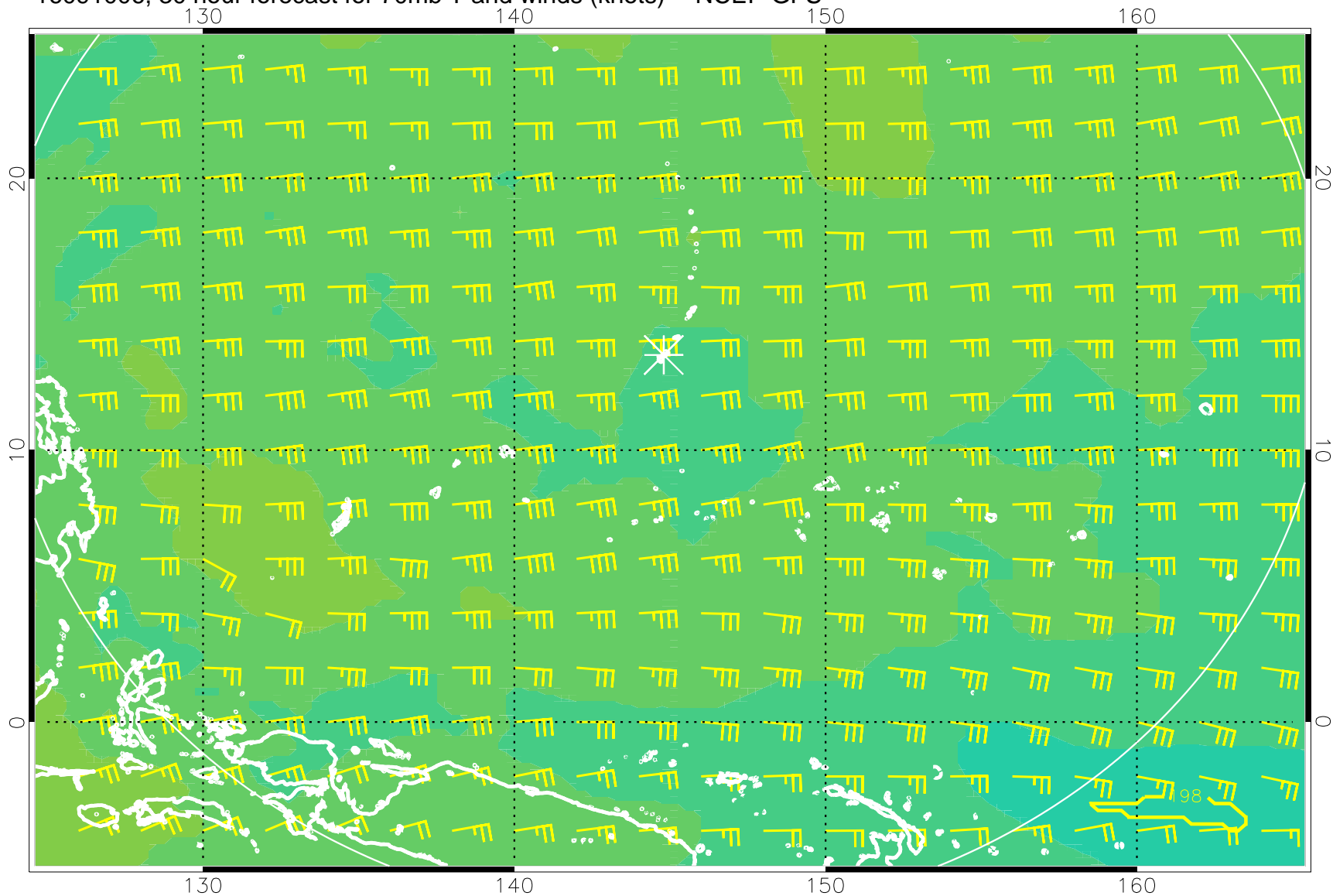
16091006, 30 hour forecast for 70mb T and winds (knots) -- NCEP GFS
