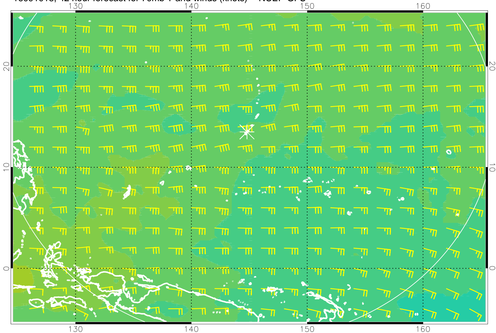
16091018, 42 hour forecast for 70mb T and winds (knots) -- NCEP GFS
