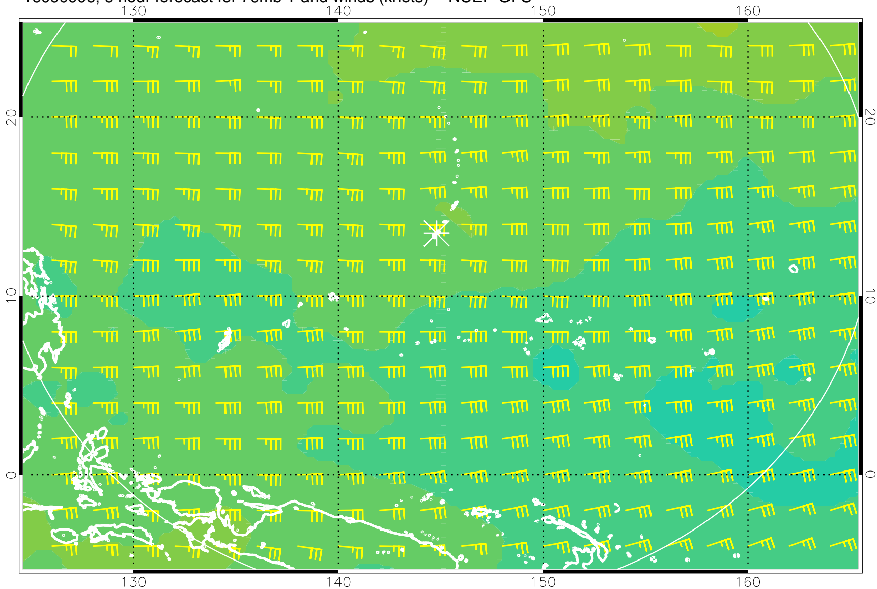
16090906, 6 hour forecast for 70mb T and winds (knots) -- NCEP GFS
