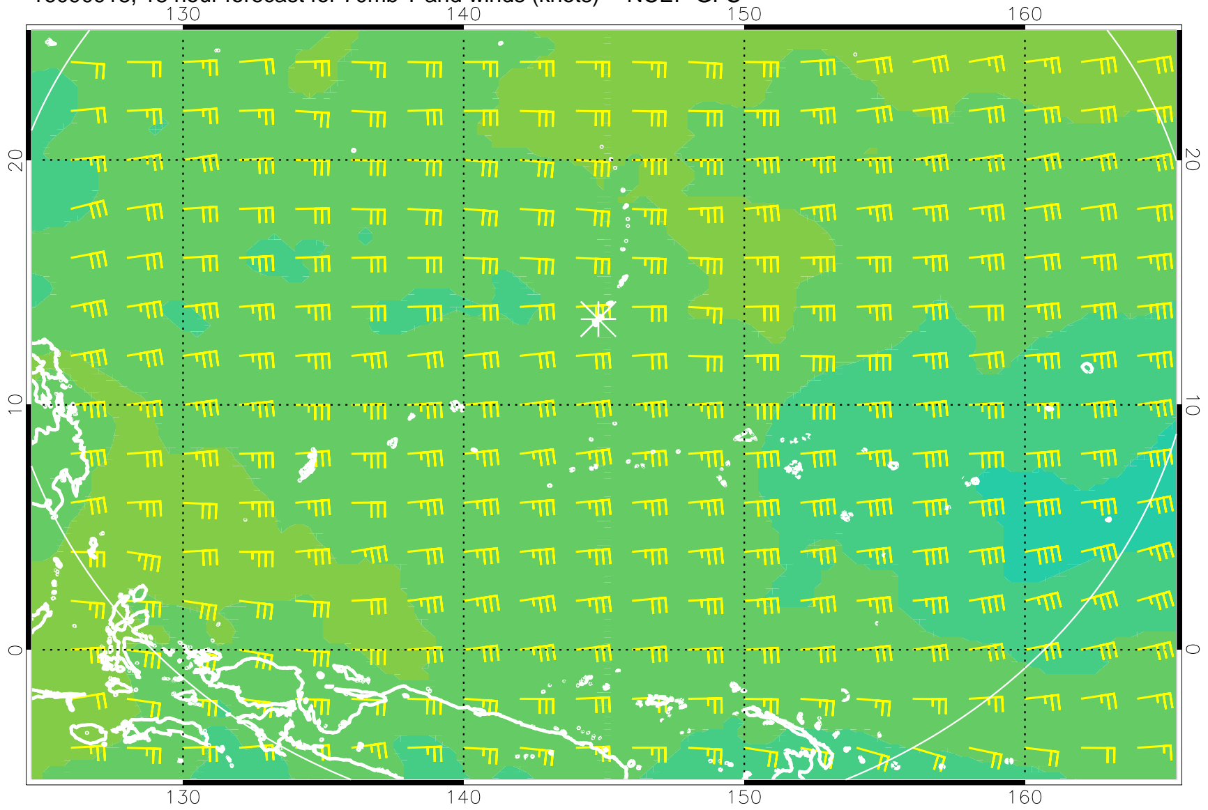
16090918, 18 hour forecast for 70mb T and winds (knots) -- NCEP GFS
