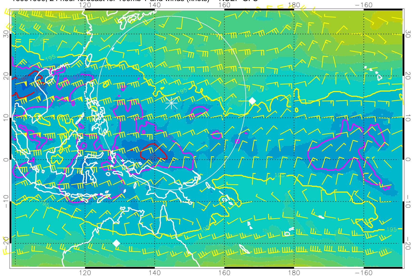
16091000, 24 hour forecast for 100mb T and winds (knots) -- NCEP GFS
