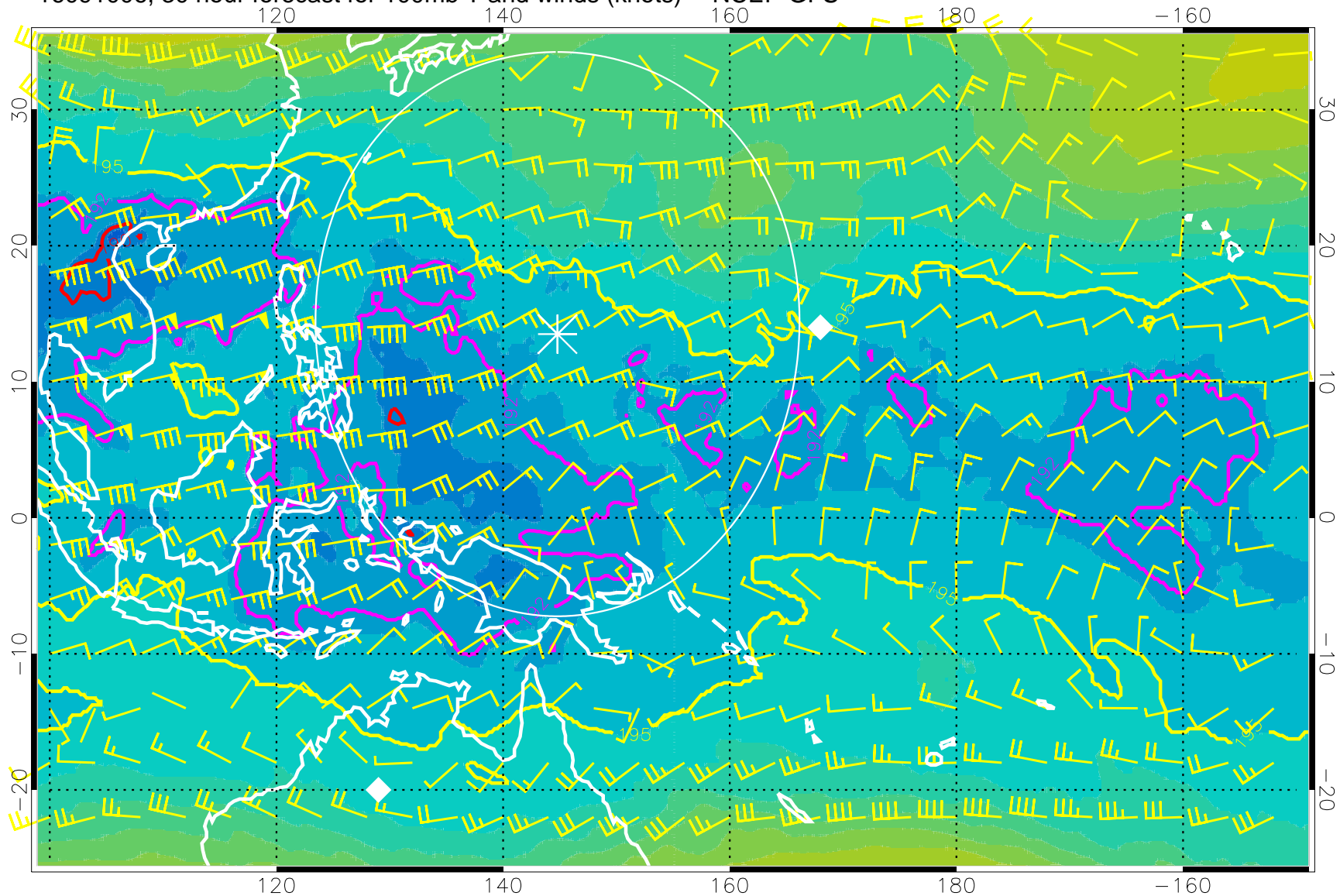
16091006, 30 hour forecast for 100mb T and winds (knots) -- NCEP GFS
