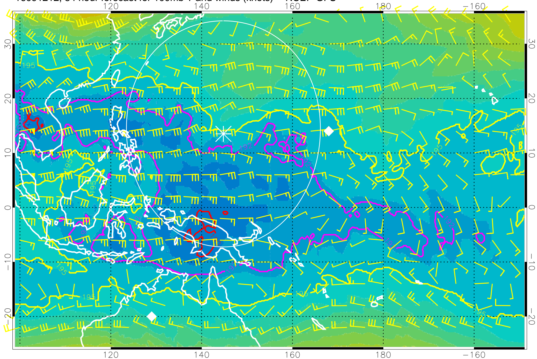
16091212, 84 hour forecast for 100mb T and winds (knots) -- NCEP GFS
