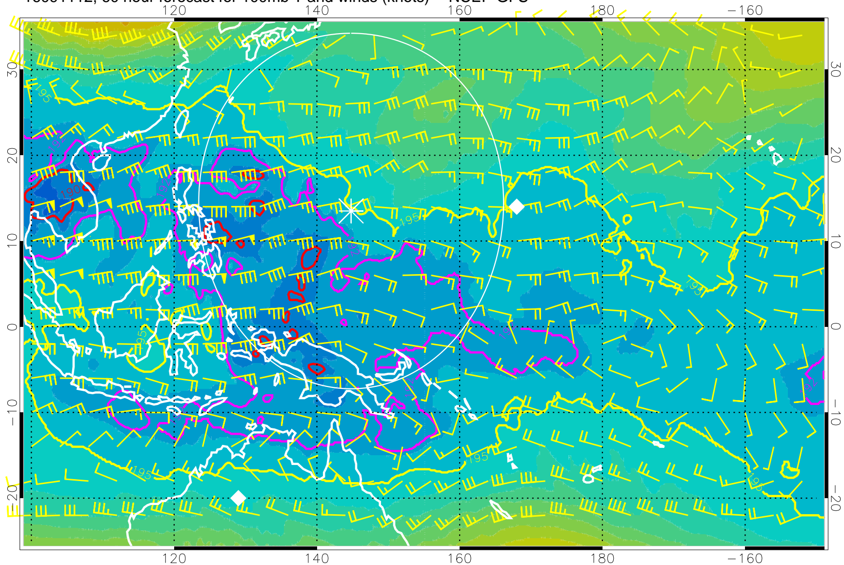
16091112, 60 hour forecast for 100mb T and winds (knots) -- NCEP GFS
