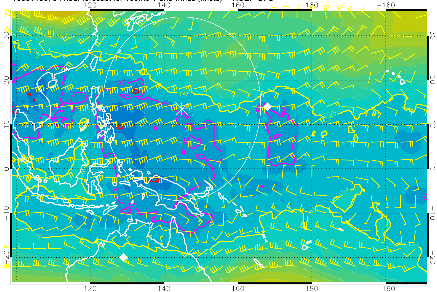
16091106, 54 hour forecast for 100mb T and winds (knots) -- NCEP GFS
