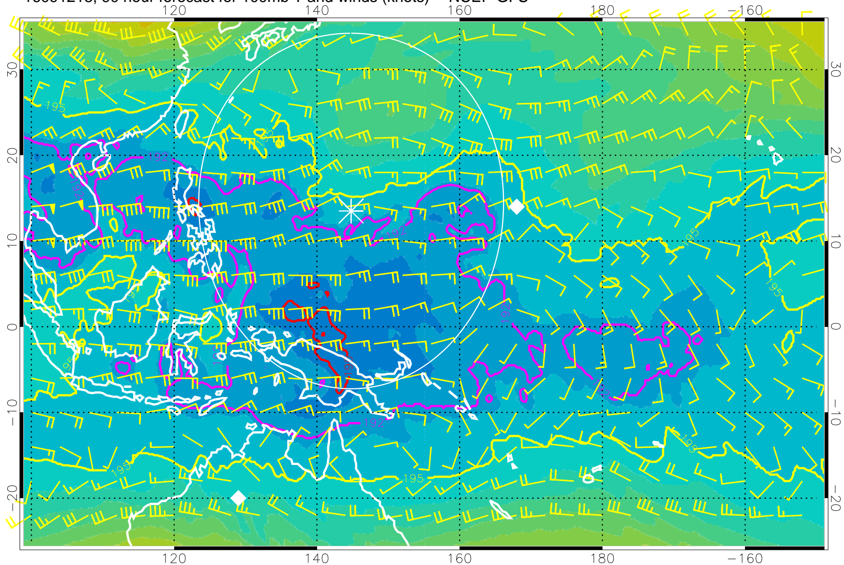
16091218, 90 hour forecast for 100mb T and winds (knots) -- NCEP GFS
