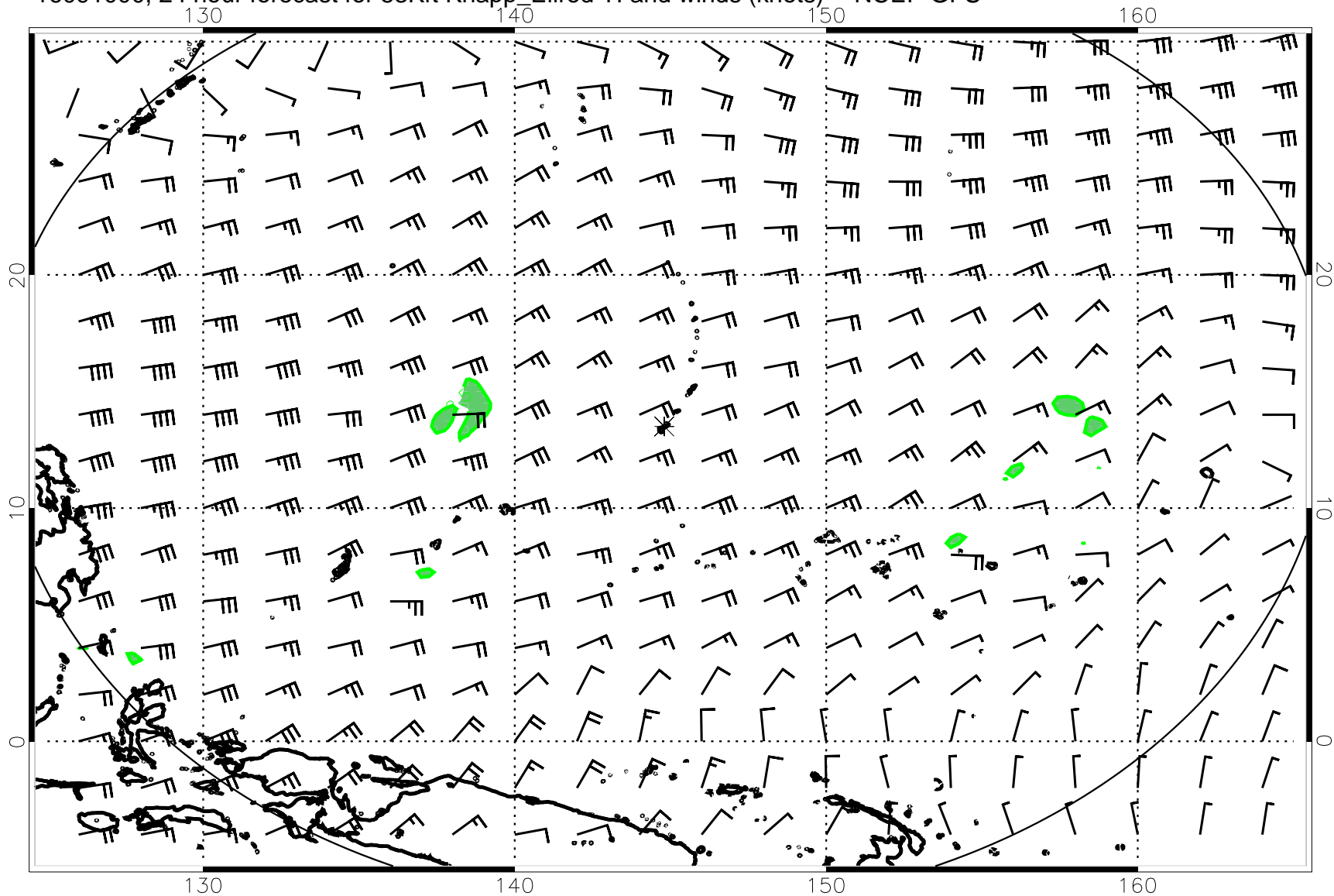
16091000, 24 hour forecast for 53Kft Knapp_Ellrod TI and winds (knots) -- NCEP GFS
