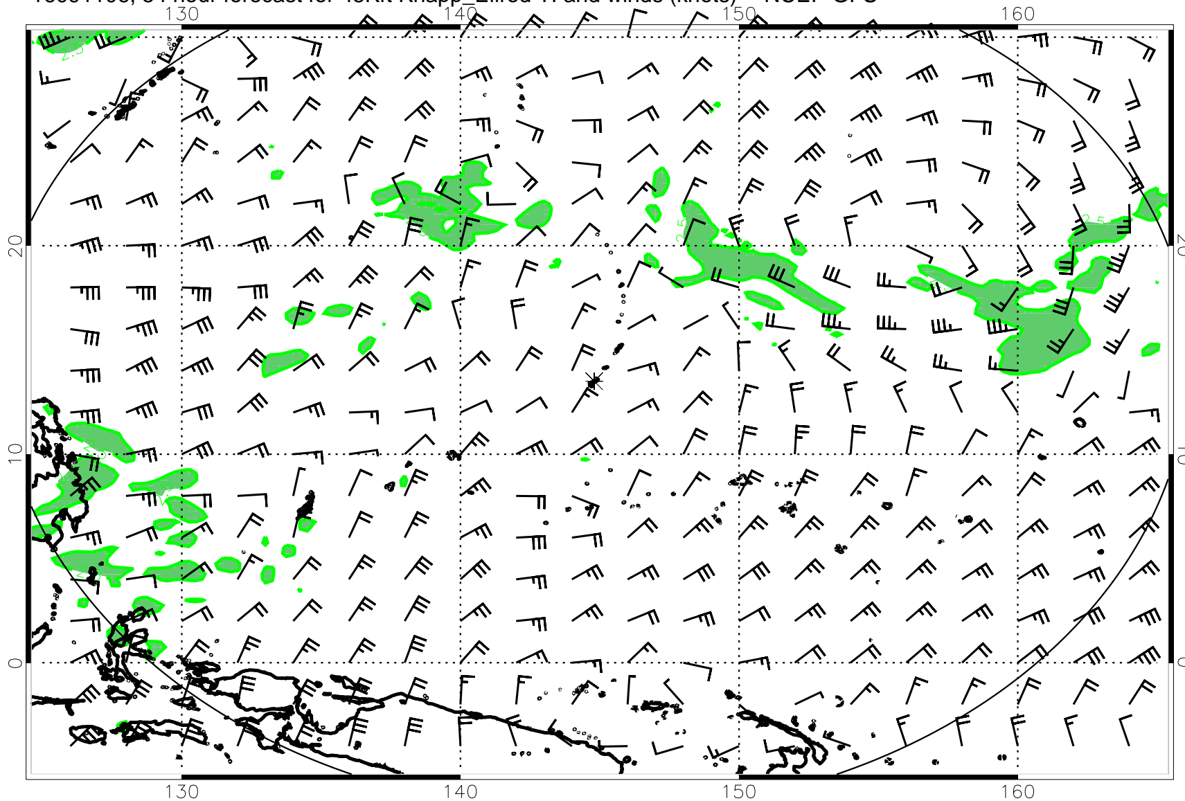
16091106, 54 hour forecast for 45Kft Knapp_Ellrod TI and winds (knots) -- NCEP GFS
