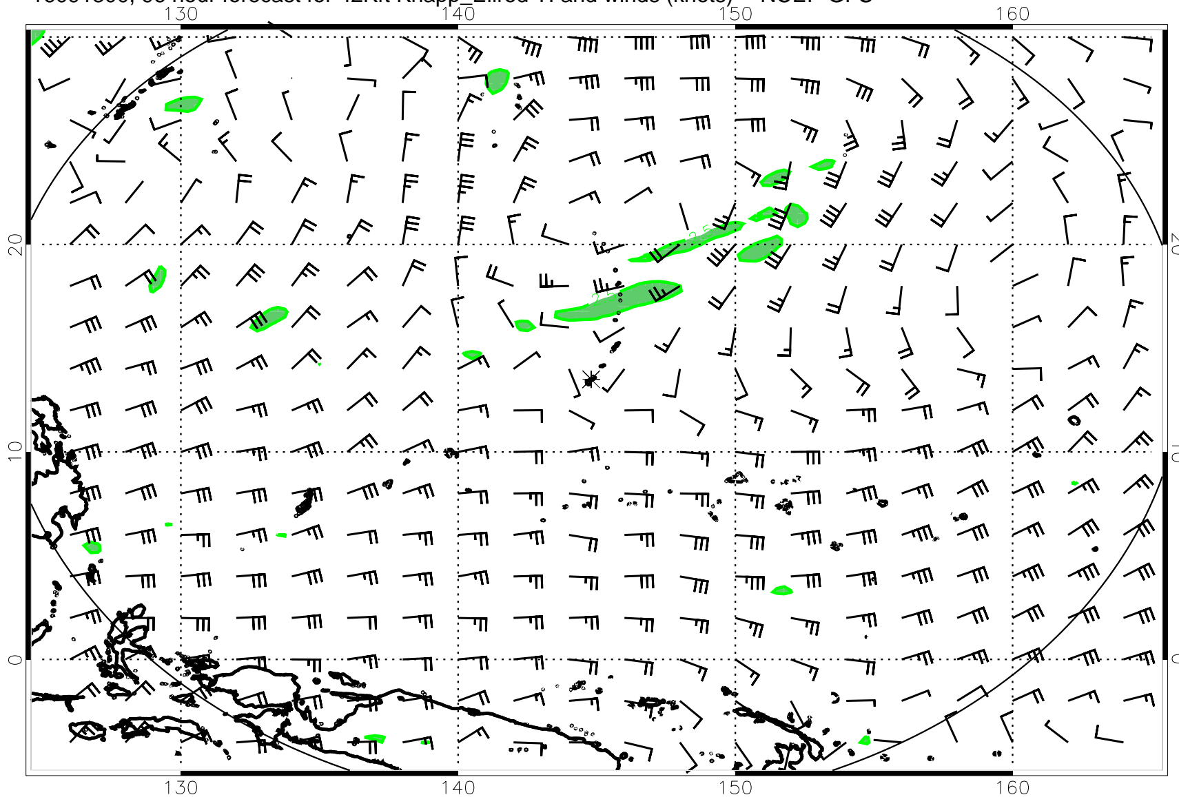
16091300, 96 hour forecast for 42Kft Knapp_Ellrod TI and winds (knots) -- NCEP GFS
