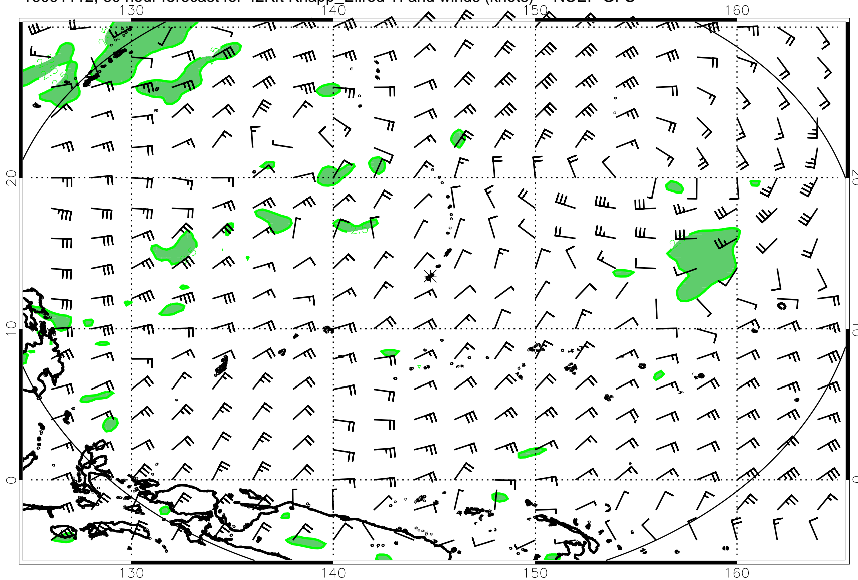
16091112, 60 hour forecast for 42Kft Knapp_Ellrod TI and winds (knots) -- NCEP GFS
