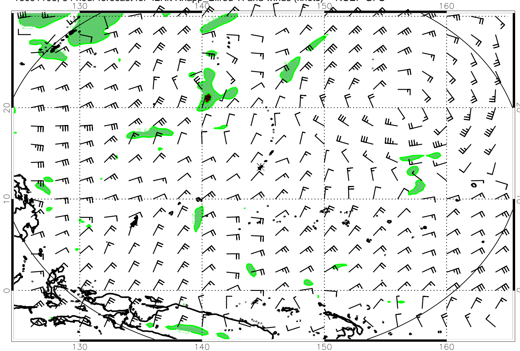
16091106, 54 hour forecast for 42Kft Knapp_Ellrod TI and winds (knots) -- NCEP GFS
