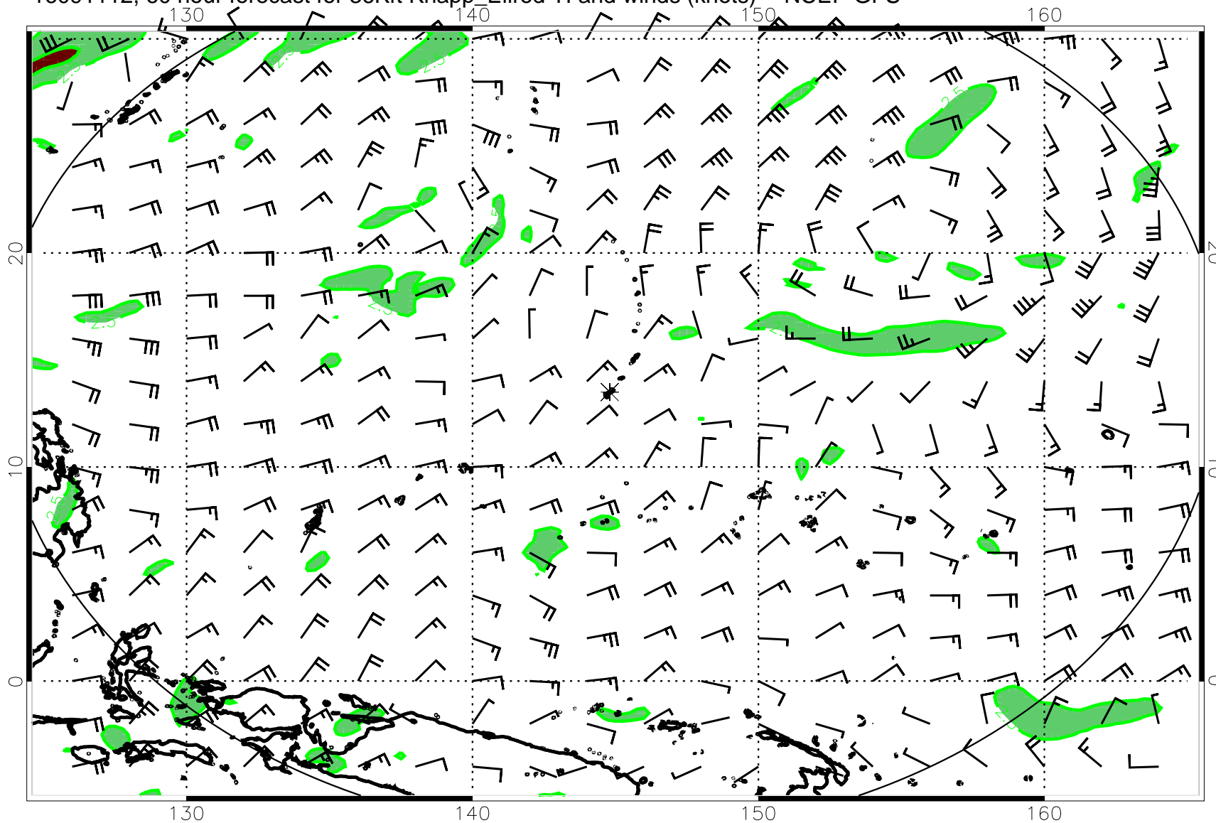
16091112, 60 hour forecast for 36Kft Knapp_Ellrod TI and winds (knots) -- NCEP GFS
