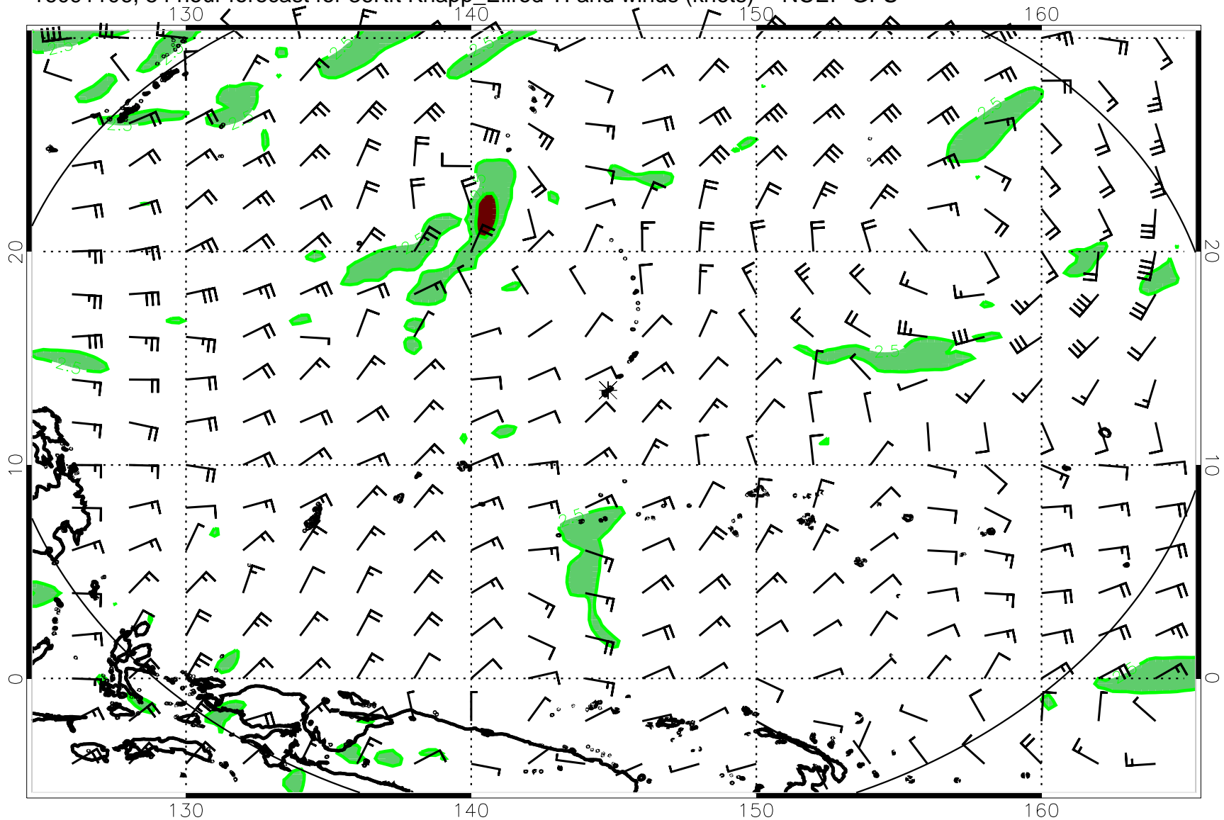
16091106, 54 hour forecast for 36Kft Knapp_Ellrod TI and winds (knots) -- NCEP GFS
