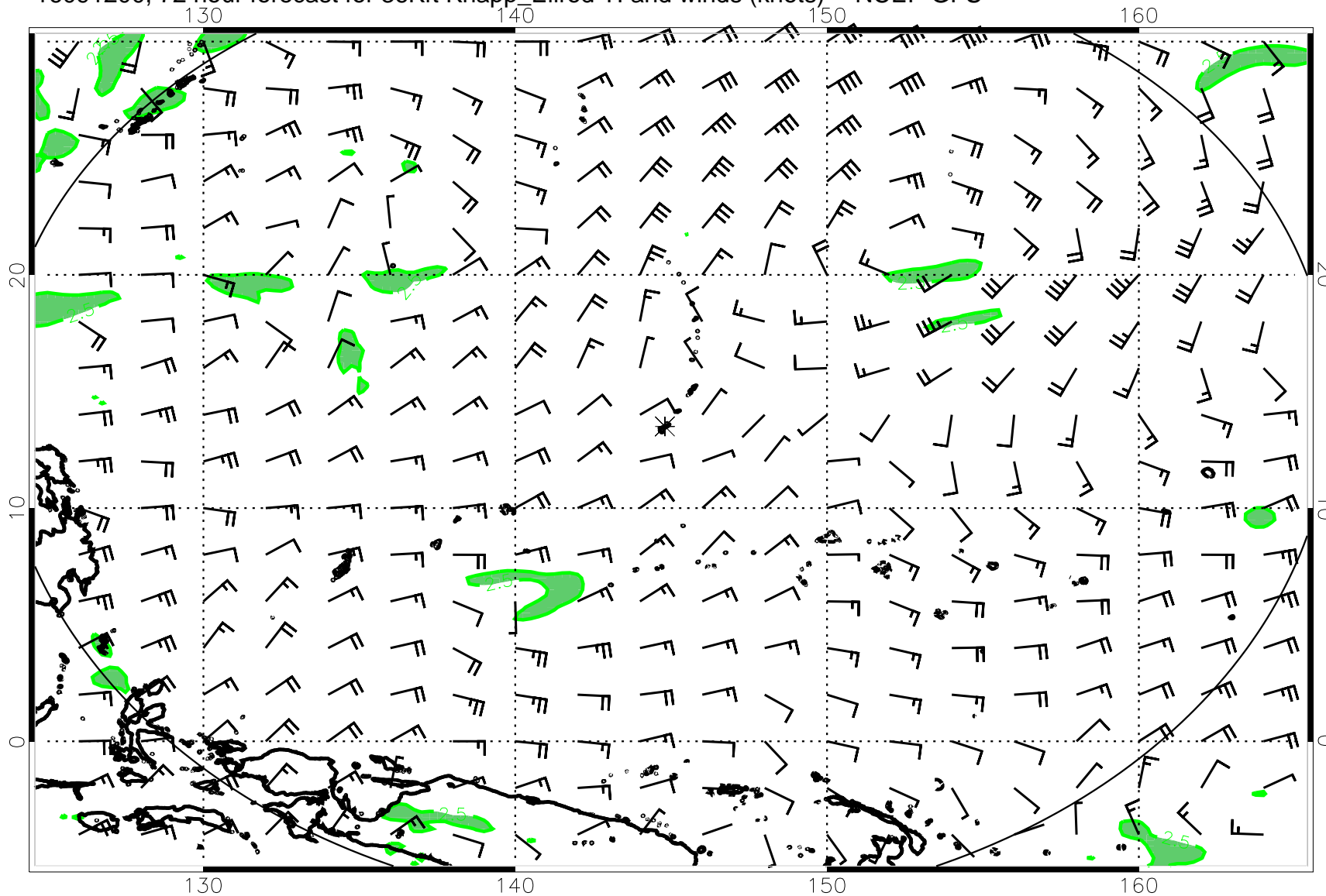
16091200, 72 hour forecast for 36Kft Knapp_Ellrod TI and winds (knots) -- NCEP GFS
