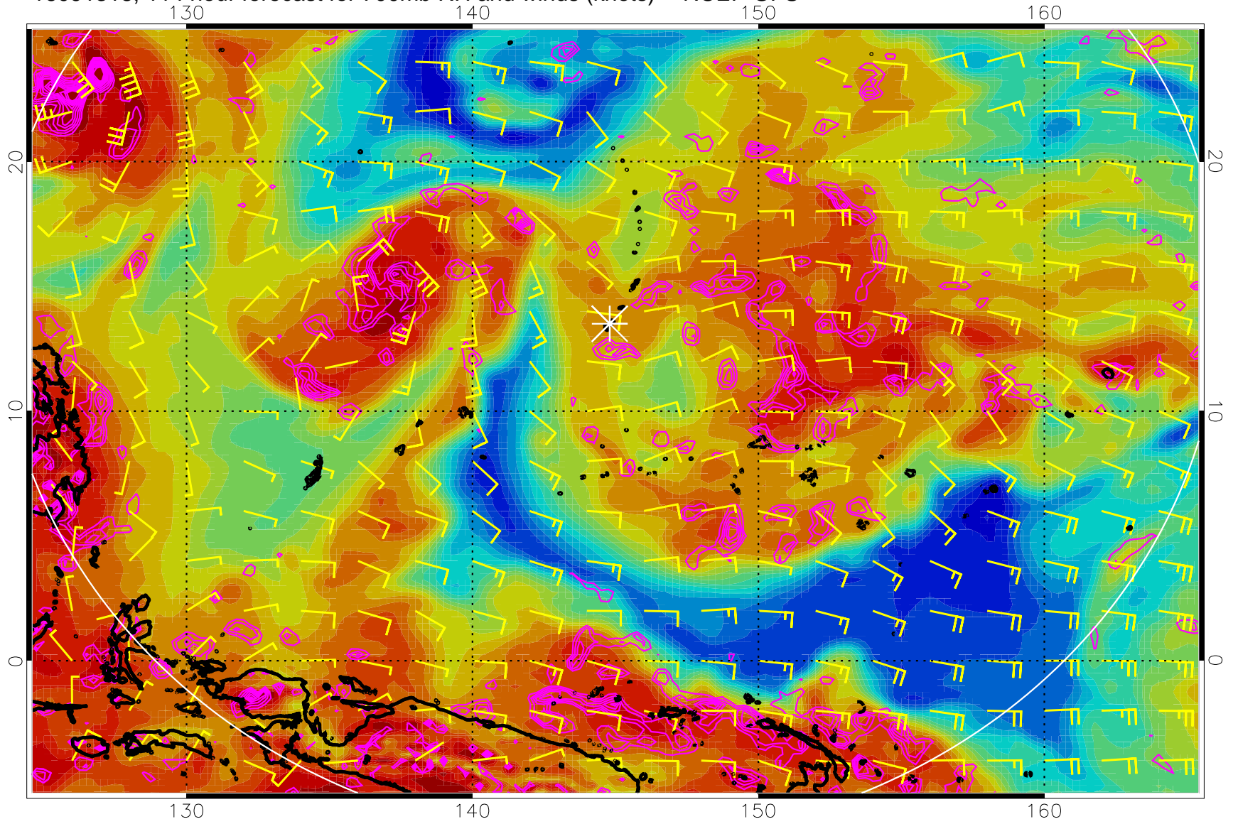
16091318, 114 hour forecast for 700mb RH and winds (knots) -- NCEP GFS
