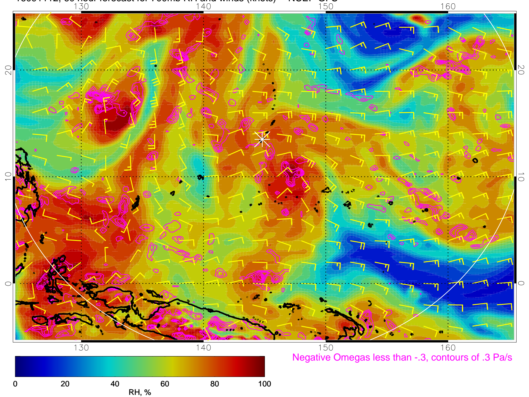
16091112, 60 hour forecast for 700mb RH and winds (knots) -- NCEP GFS
