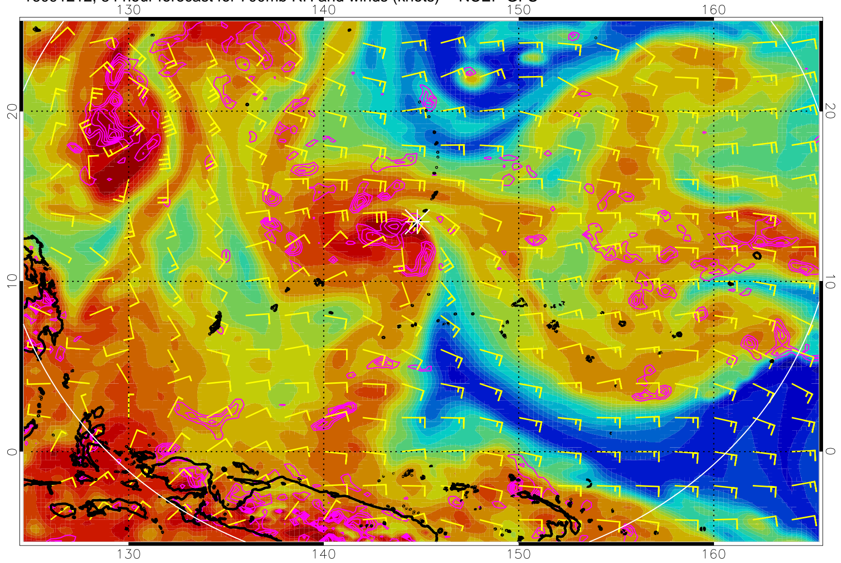
16091212, 84 hour forecast for 700mb RH and winds (knots) -- NCEP GFS
