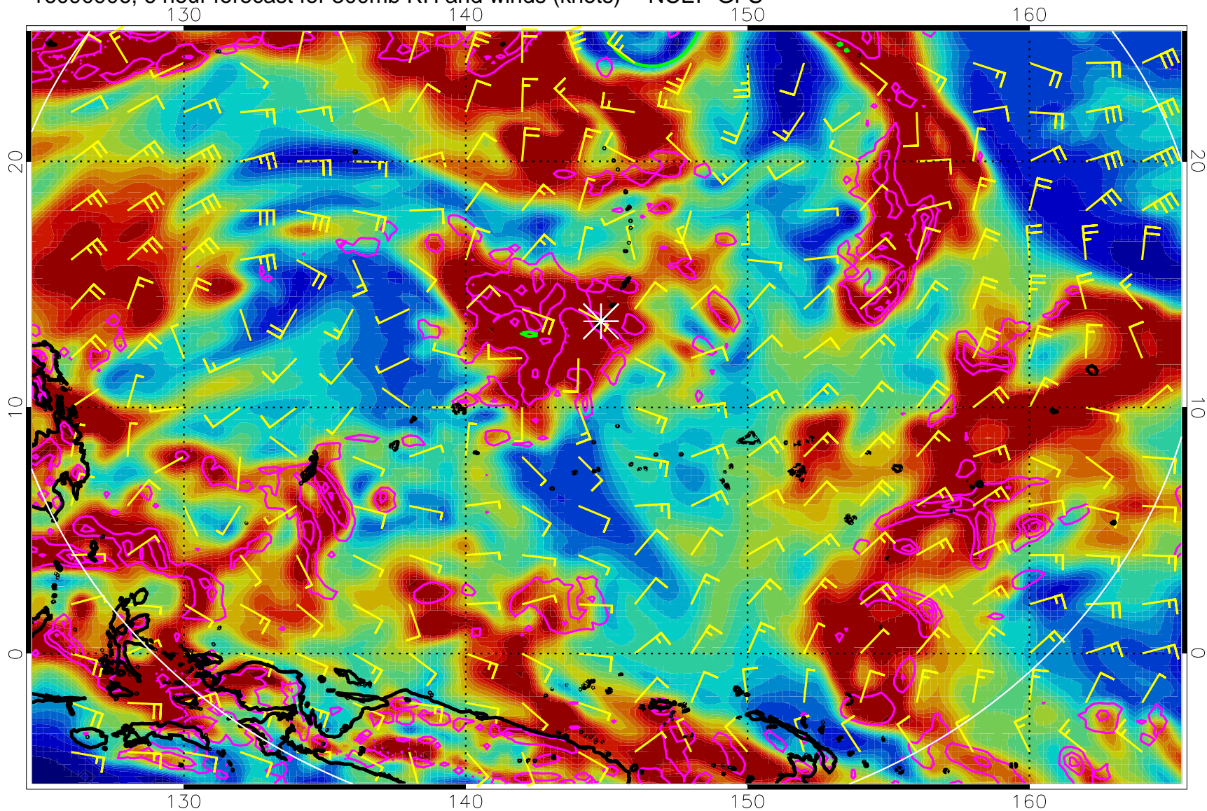
16090906, 6 hour forecast for 300mb RH and winds (knots) -- NCEP GFS
