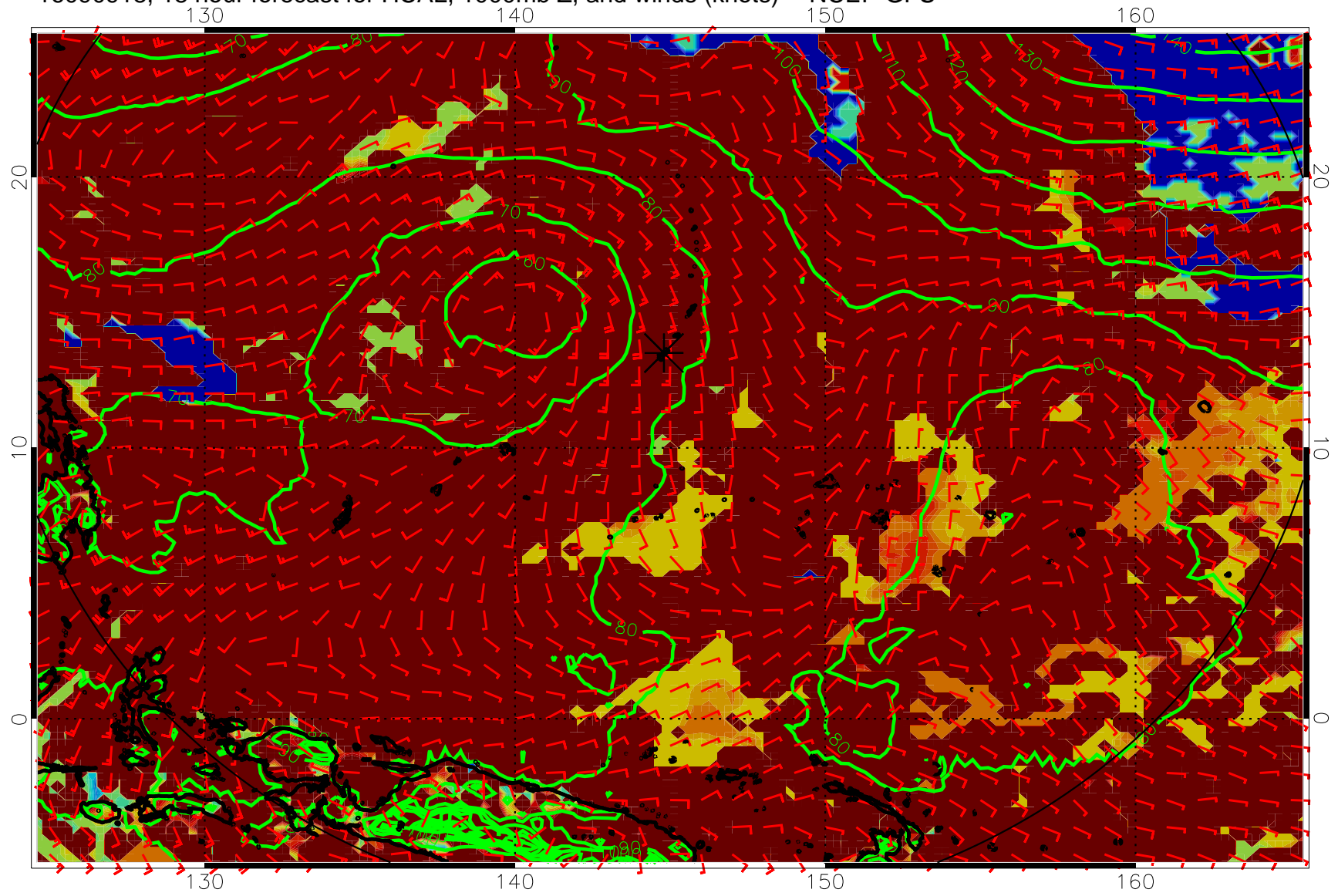
16090918, 18 hour forecast for HCAL, 1000mb Z, and winds (knots) -- NCEP GFS
