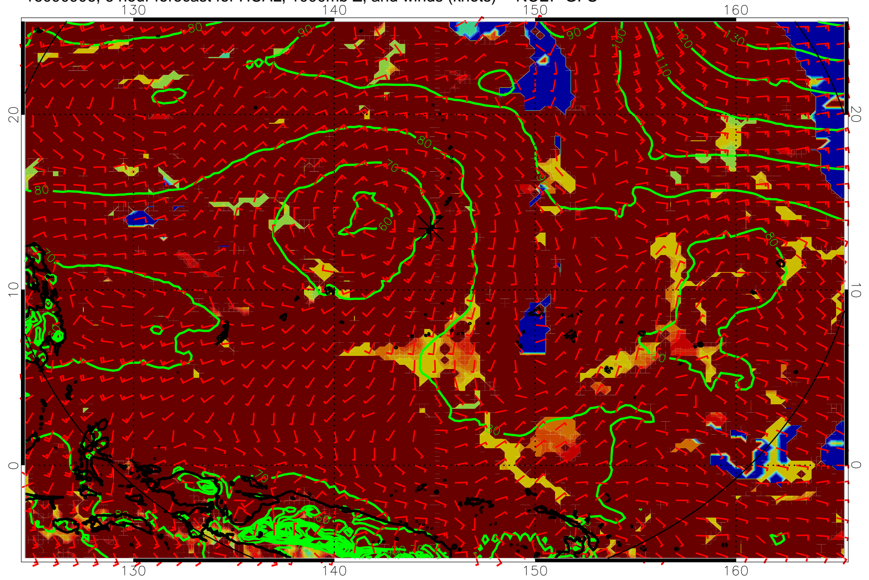
16090906, 6 hour forecast for HCAL, 1000mb Z, and winds (knots) -- NCEP GFS
