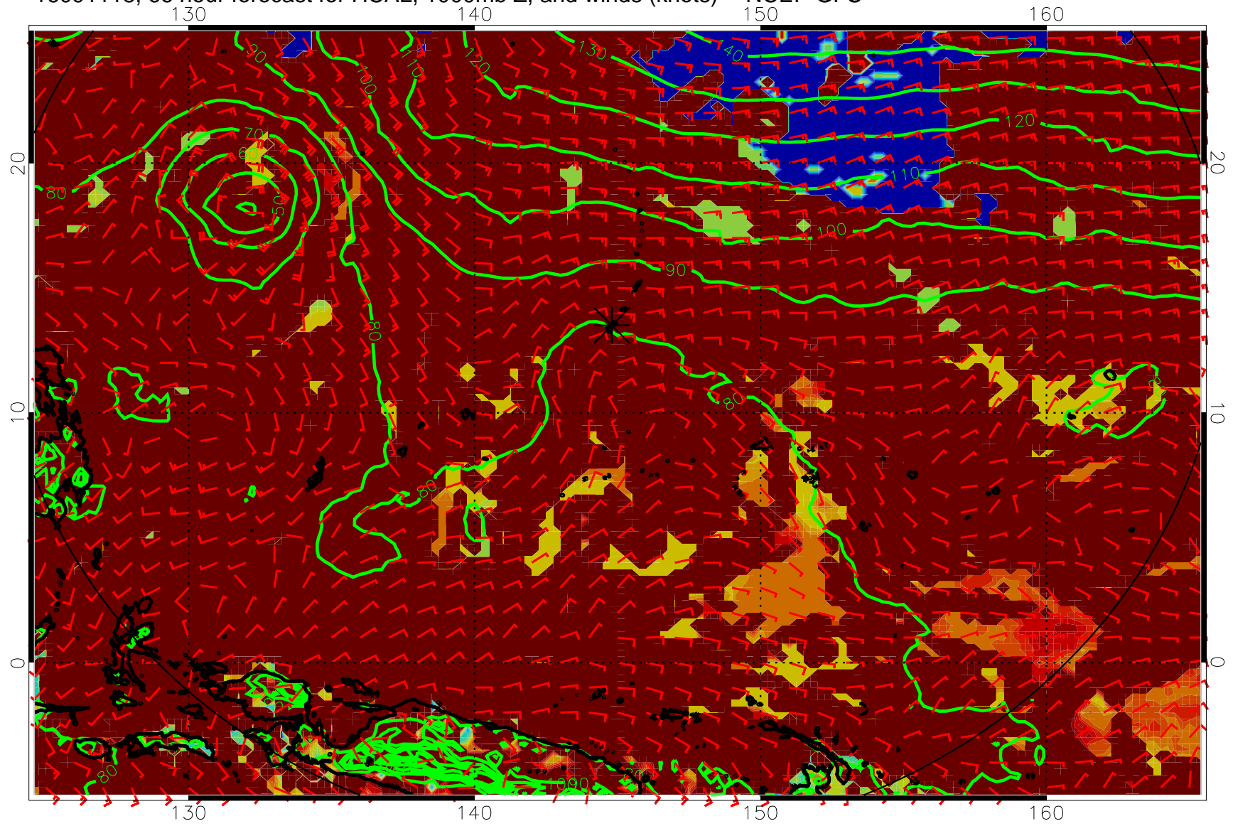
16091118, 66 hour forecast for HCAL, 1000mb Z, and winds (knots) -- NCEP GFS
