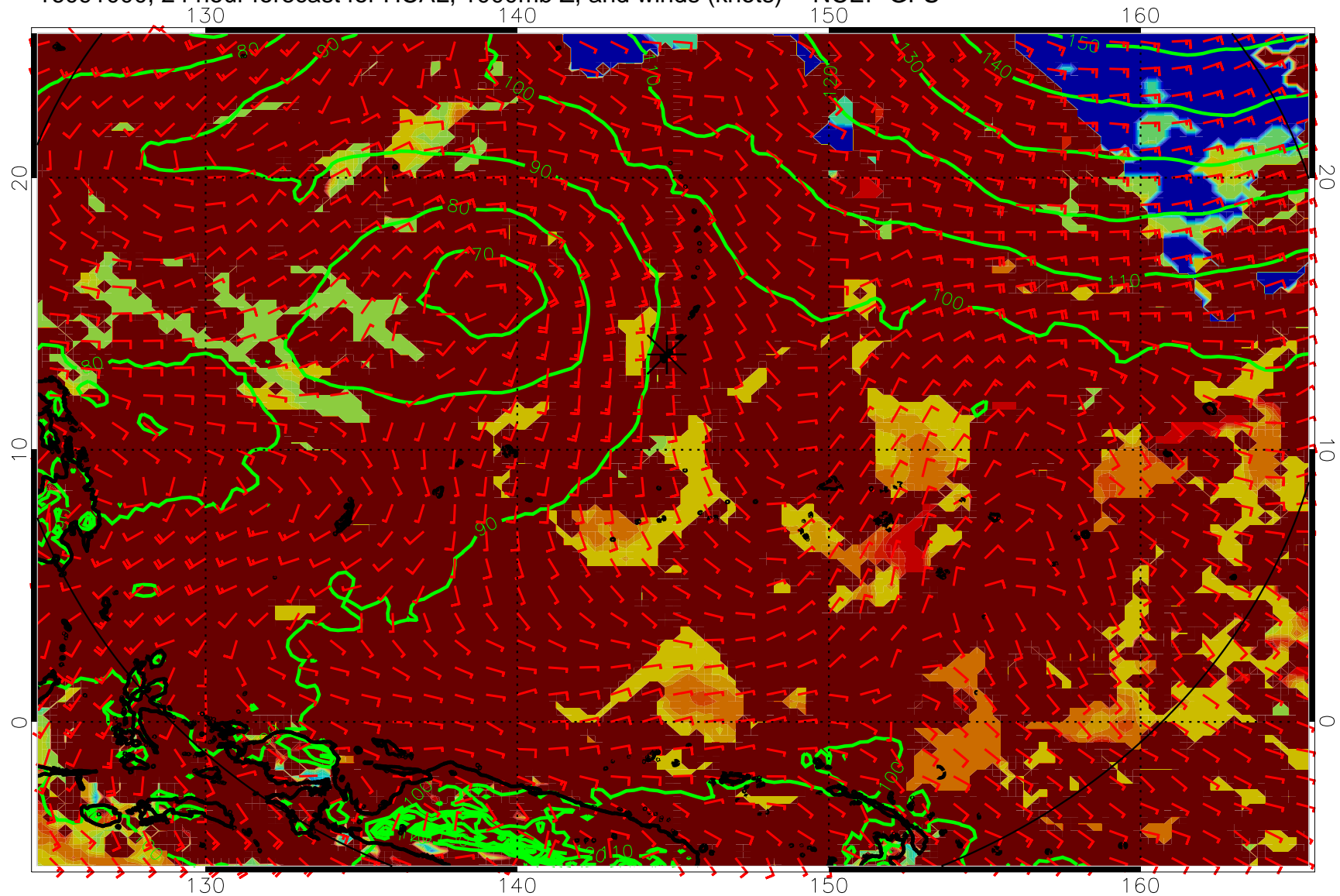
16091000, 24 hour forecast for HCAL, 1000mb Z, and winds (knots) -- NCEP GFS
