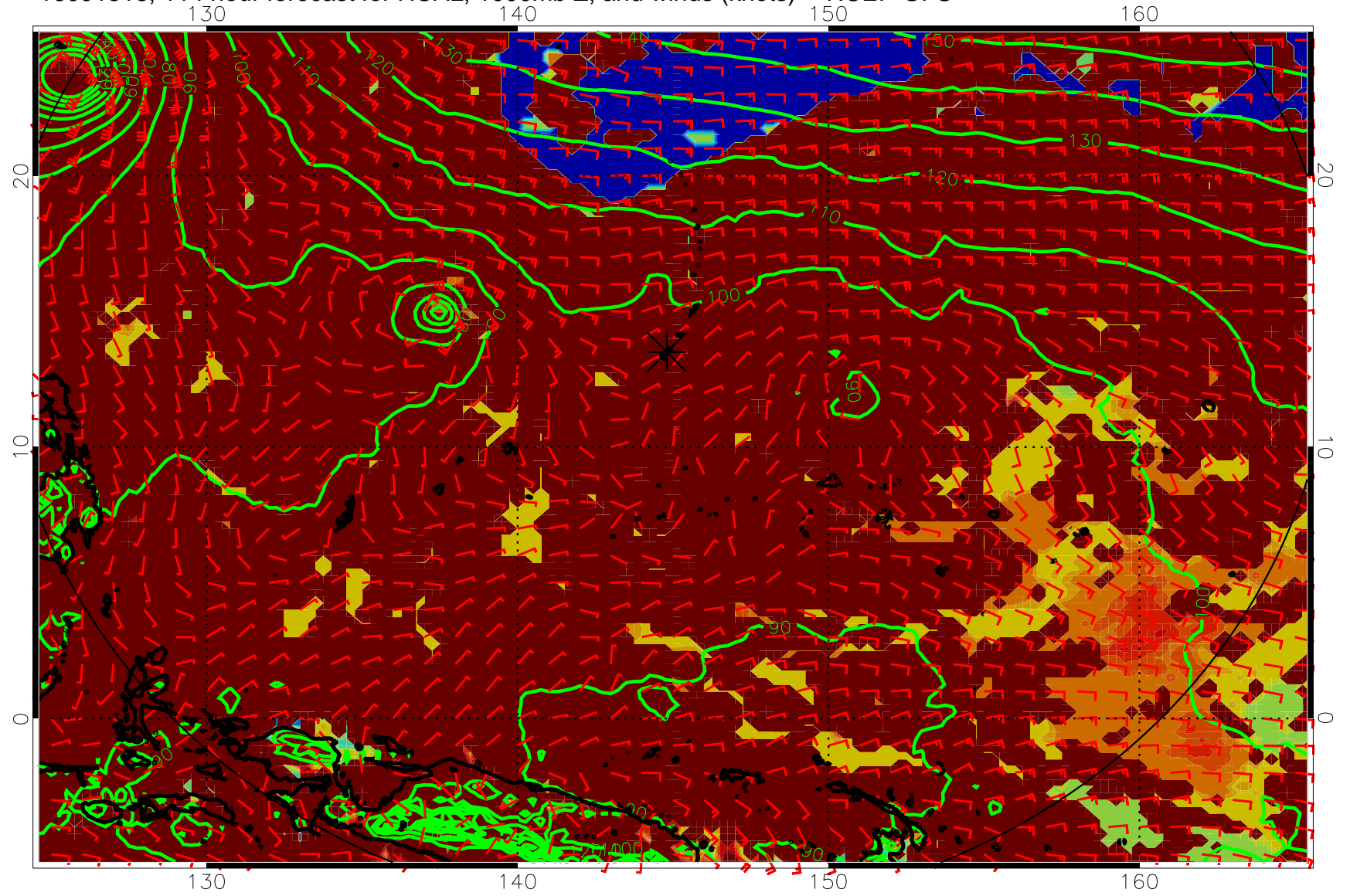
16091318, 114 hour forecast for HCAL, 1000mb Z, and winds (knots) -- NCEP GFS
