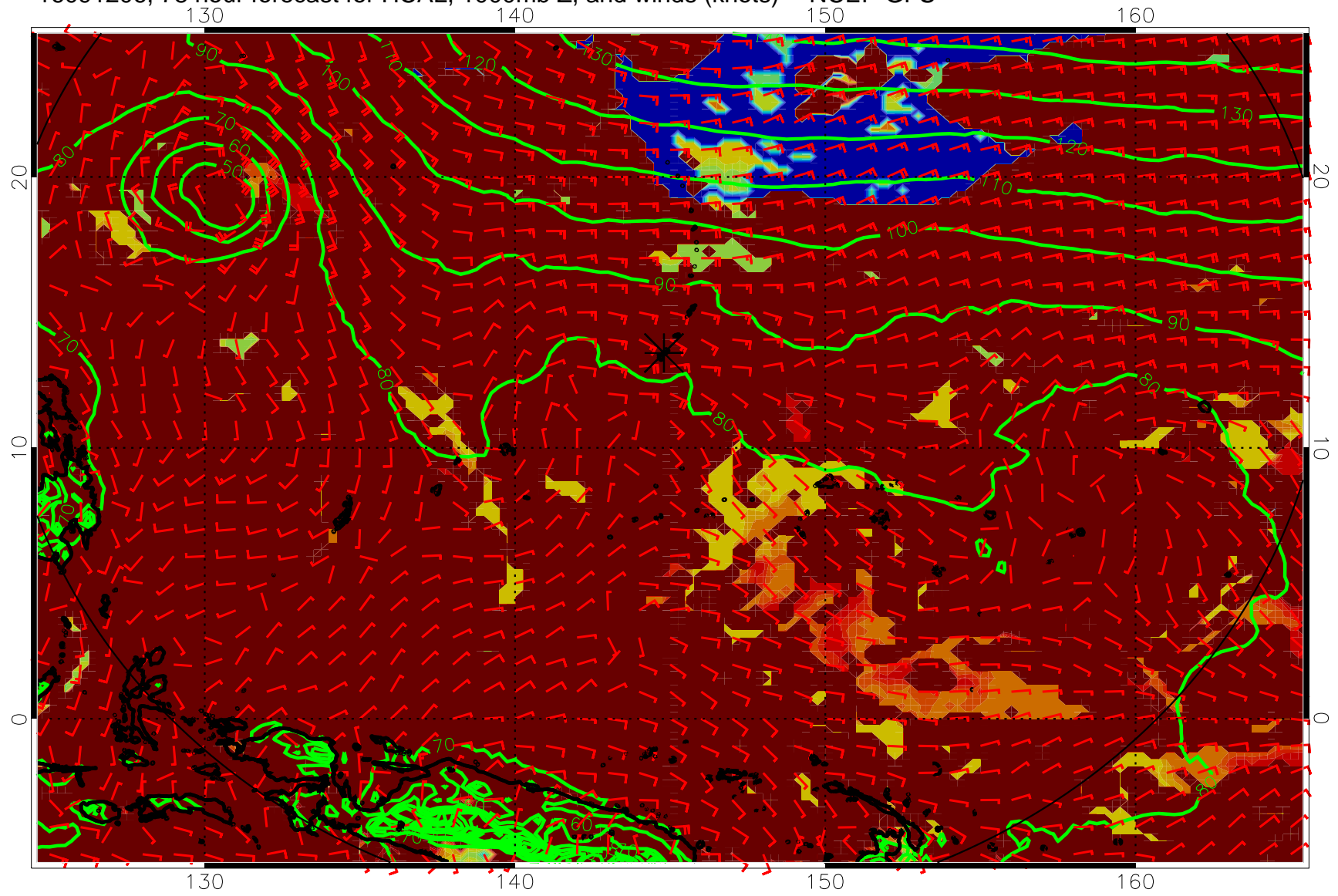
16091206, 78 hour forecast for HCAL, 1000mb Z, and winds (knots) -- NCEP GFS
