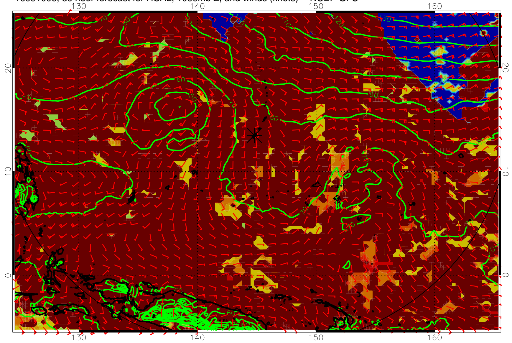
16091006, 30 hour forecast for HCAL, 1000mb Z, and winds (knots) -- NCEP GFS
