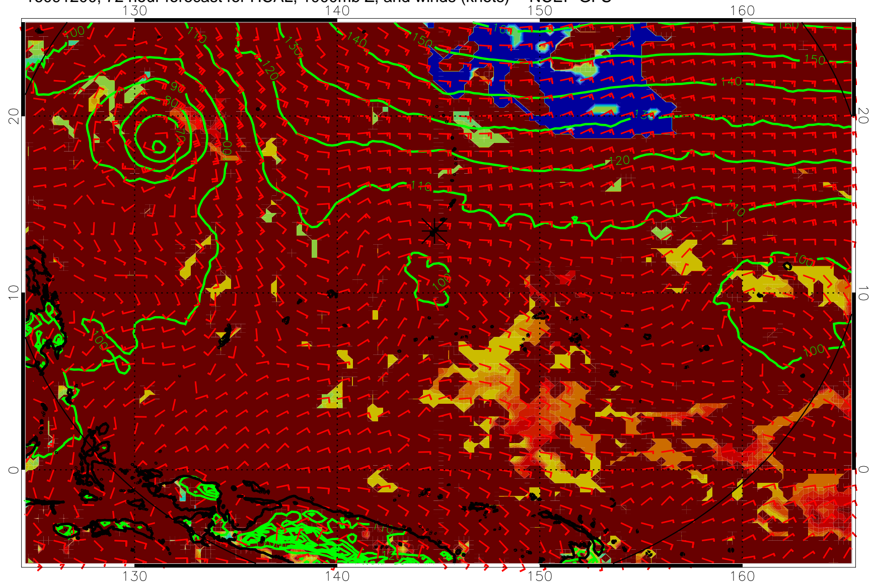
16091200, 72 hour forecast for HCAL, 1000mb Z, and winds (knots) -- NCEP GFS
