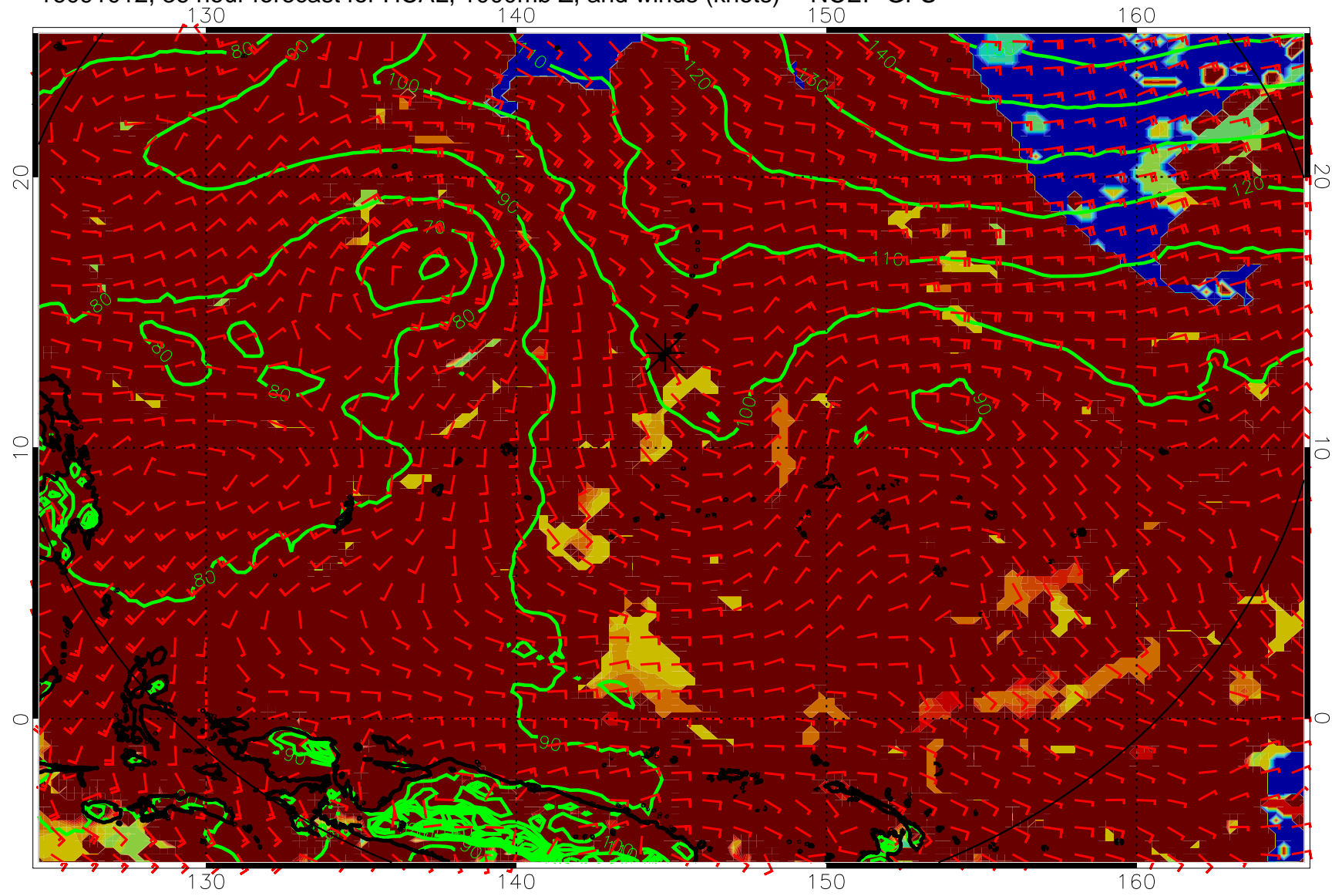
16091012, 36 hour forecast for HCAL, 1000mb Z, and winds (knots) -- NCEP GFS
