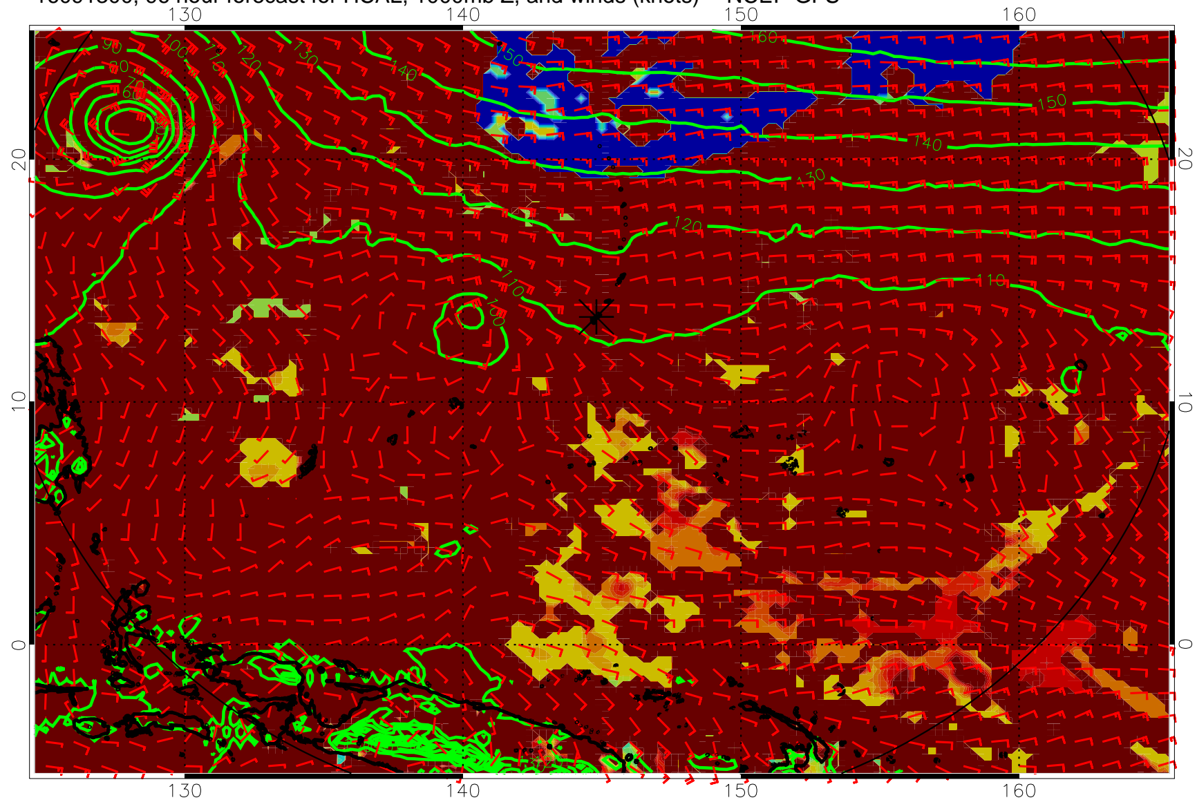
16091300, 96 hour forecast for HCAL, 1000mb Z, and winds (knots) -- NCEP GFS
