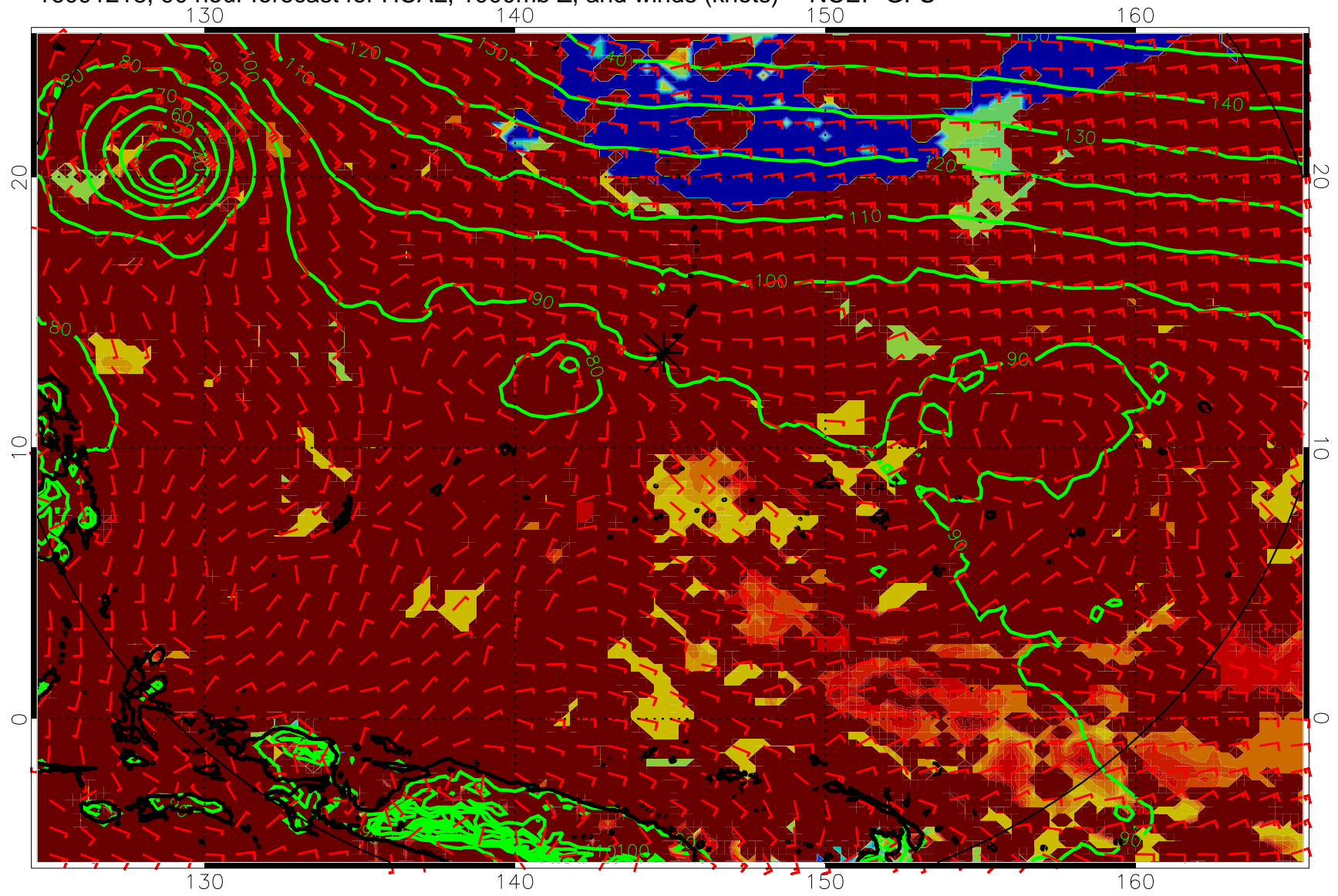
16091218, 90 hour forecast for HCAL, 1000mb Z, and winds (knots) -- NCEP GFS
