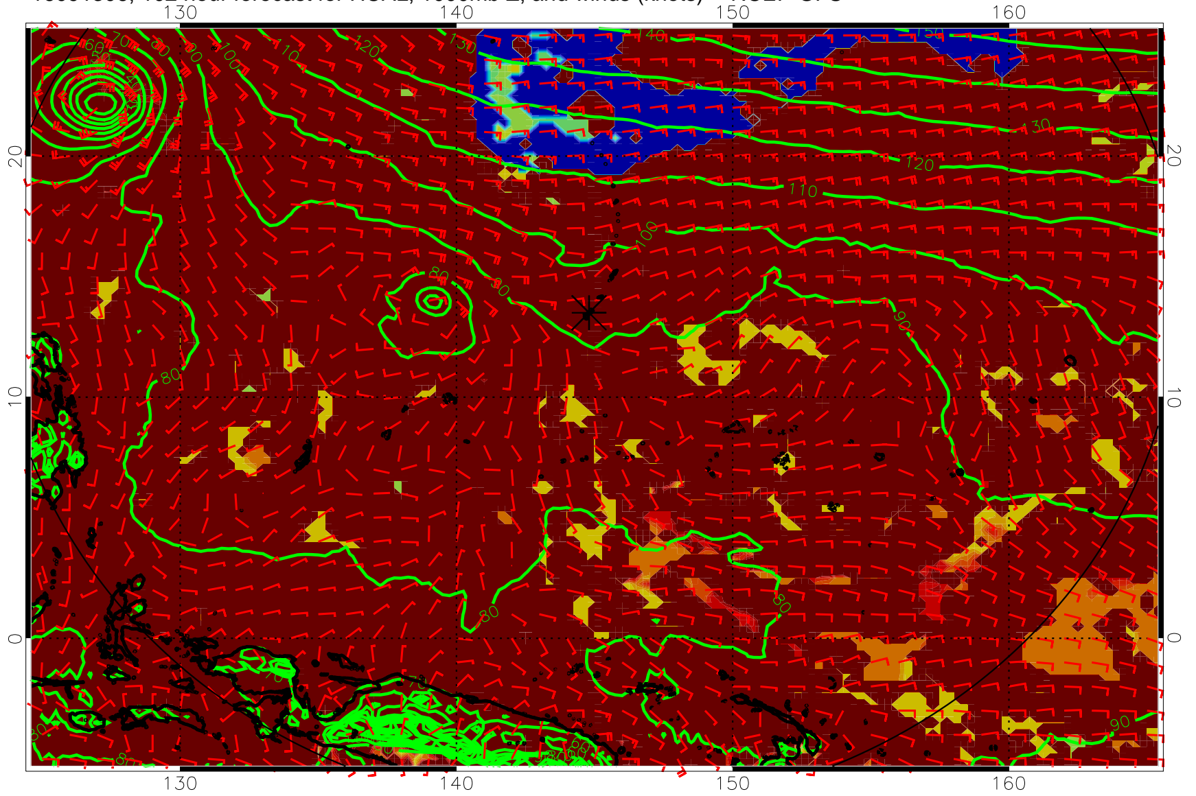
16091306, 102 hour forecast for HCAL, 1000mb Z, and winds (knots) -- NCEP GFS
