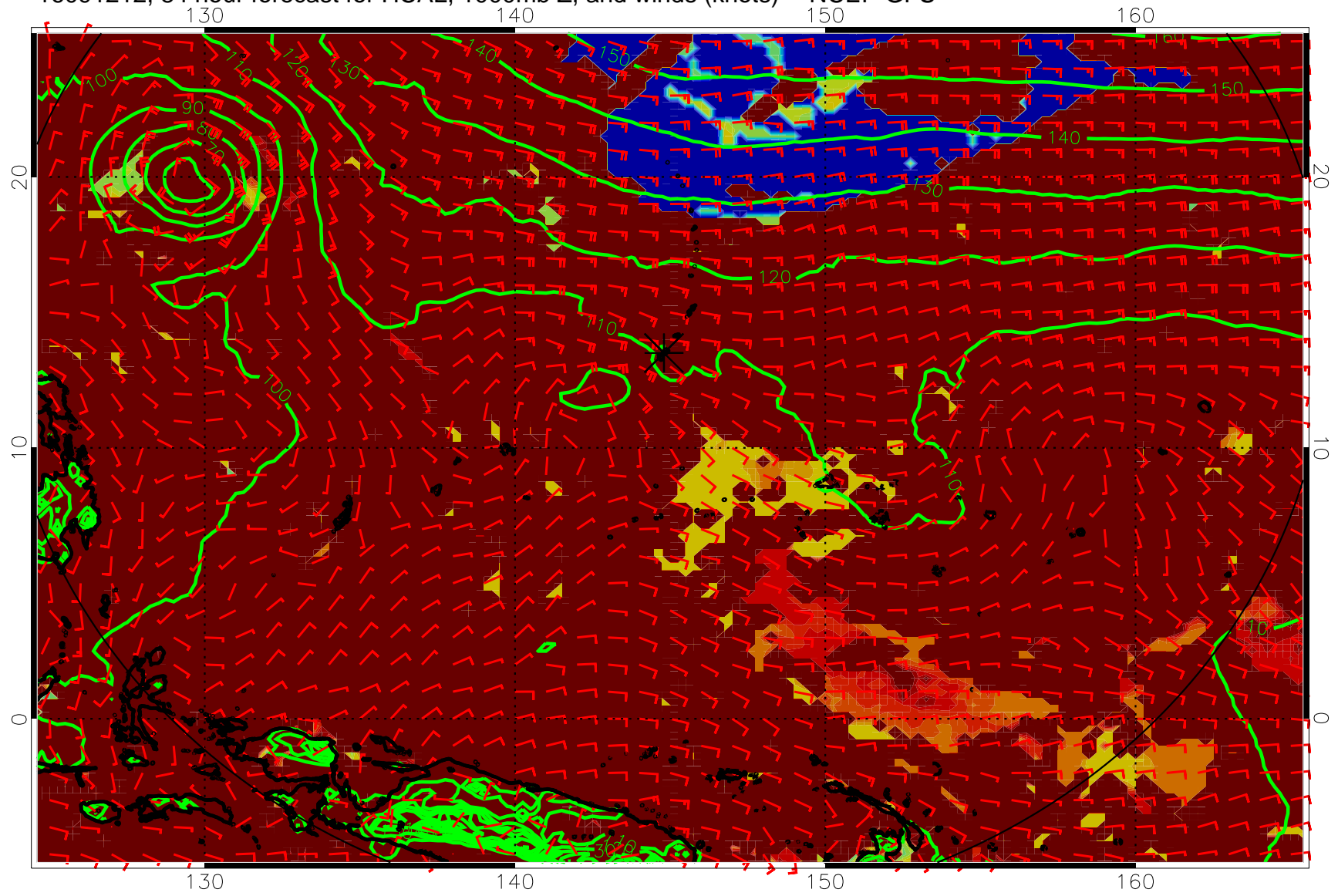
16091212, 84 hour forecast for HCAL, 1000mb Z, and winds (knots) -- NCEP GFS
