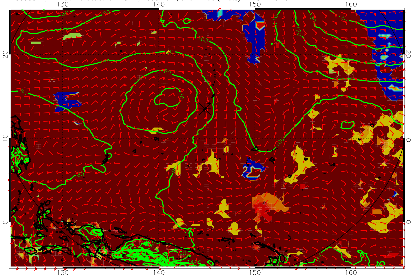
16090912, 12 hour forecast for HCAL, 1000mb Z, and winds (knots) -- NCEP GFS
