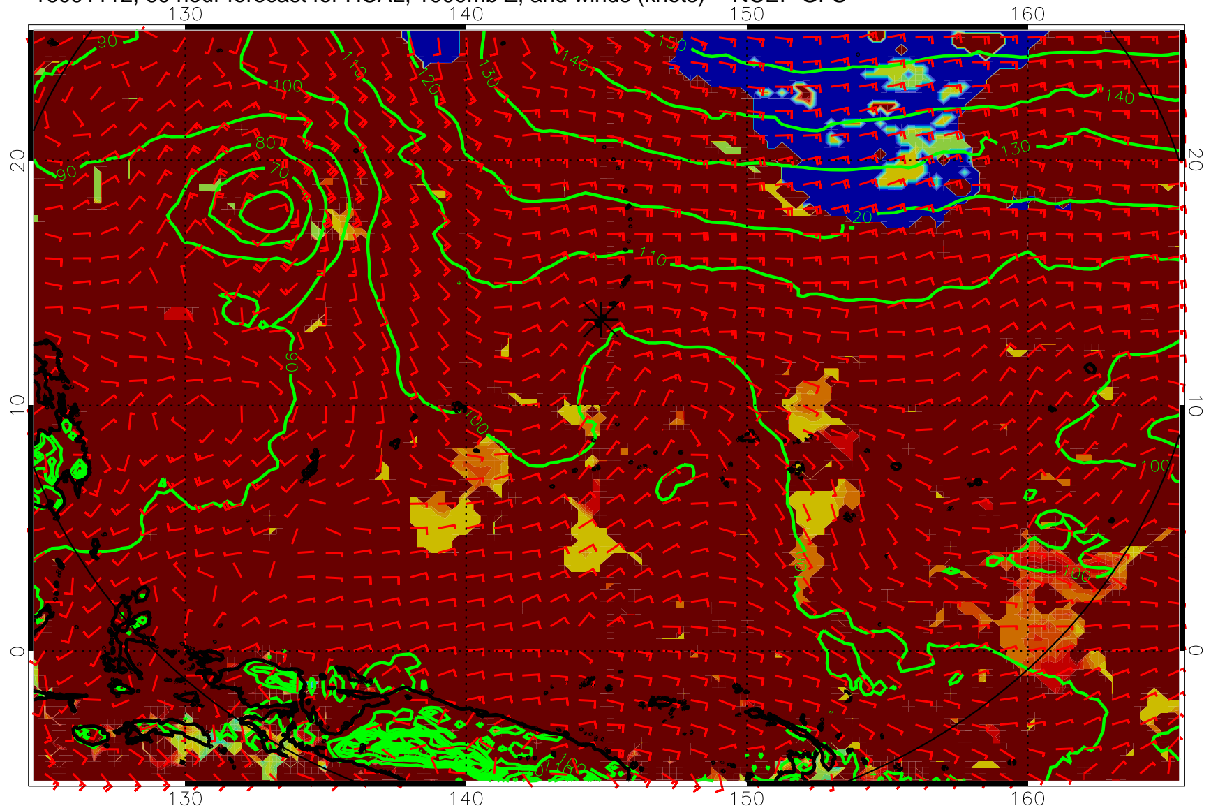
16091112, 60 hour forecast for HCAL, 1000mb Z, and winds (knots) -- NCEP GFS
