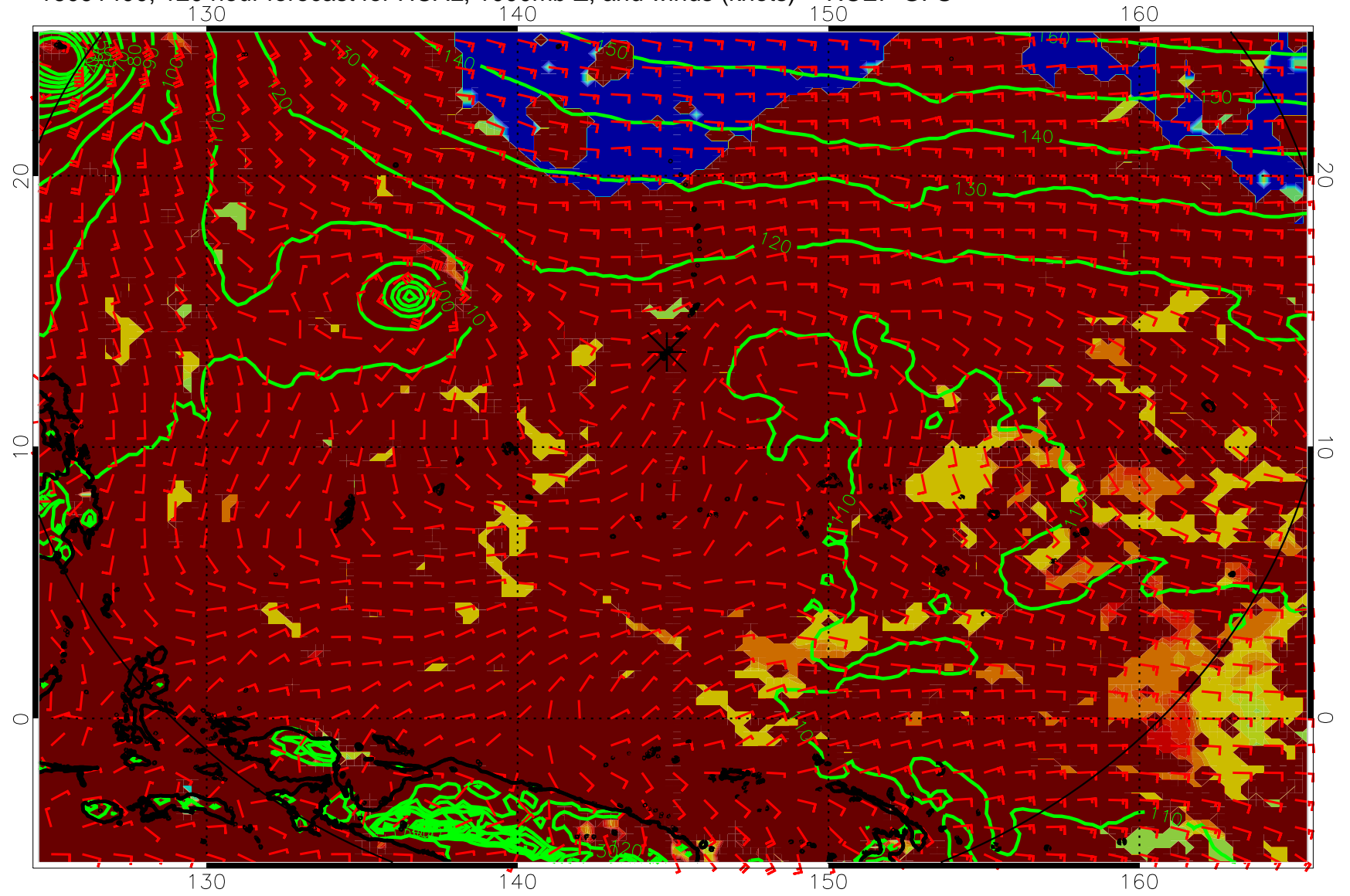
16091400, 120 hour forecast for HCAL, 1000mb Z, and winds (knots) -- NCEP GFS
