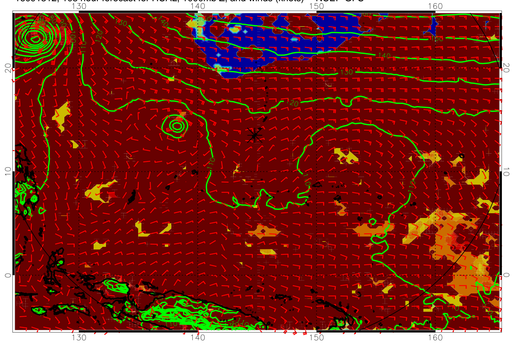
16091312, 108 hour forecast for HCAL, 1000mb Z, and winds (knots) -- NCEP GFS
