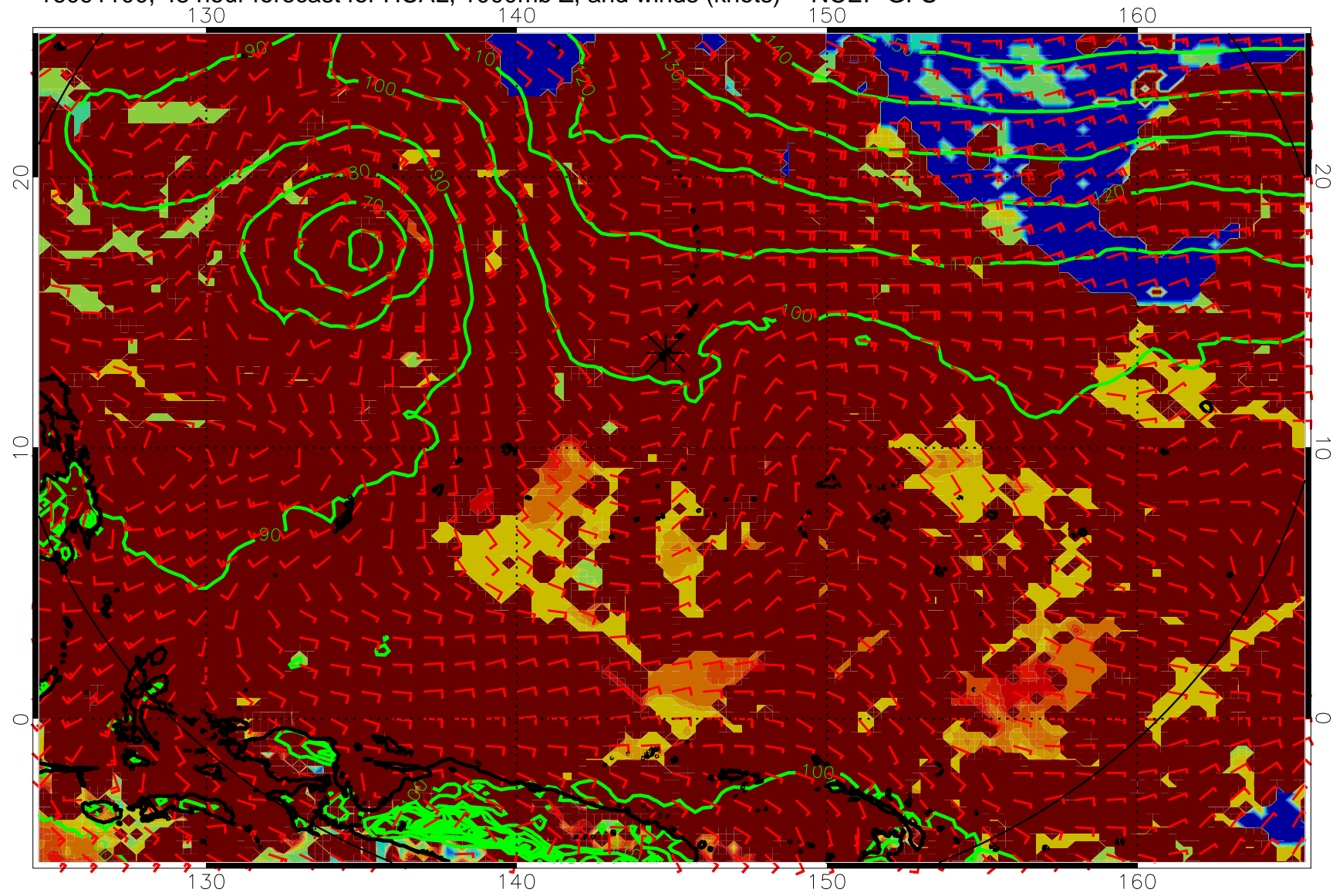
16091100, 48 hour forecast for HCAL, 1000mb Z, and winds (knots) -- NCEP GFS
