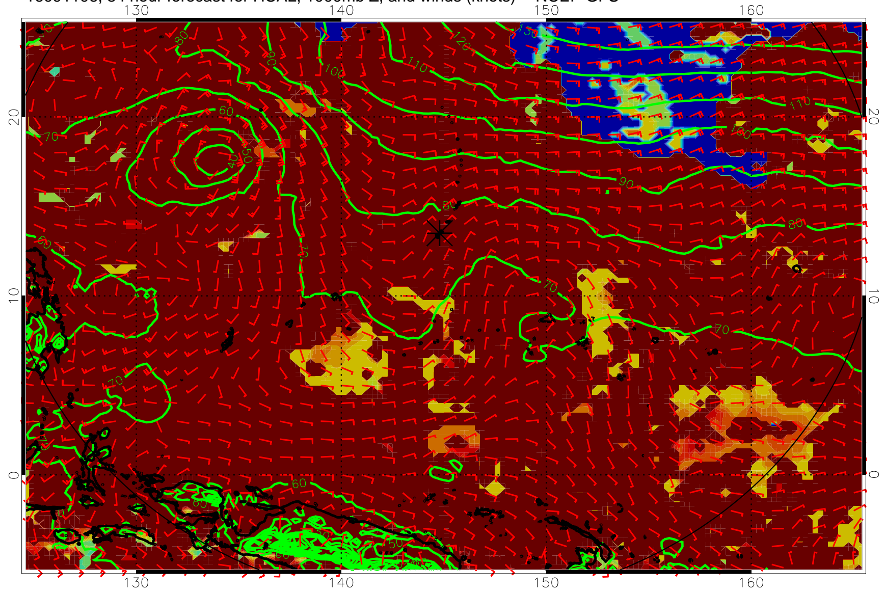
16091106, 54 hour forecast for HCAL, 1000mb Z, and winds (knots) -- NCEP GFS
