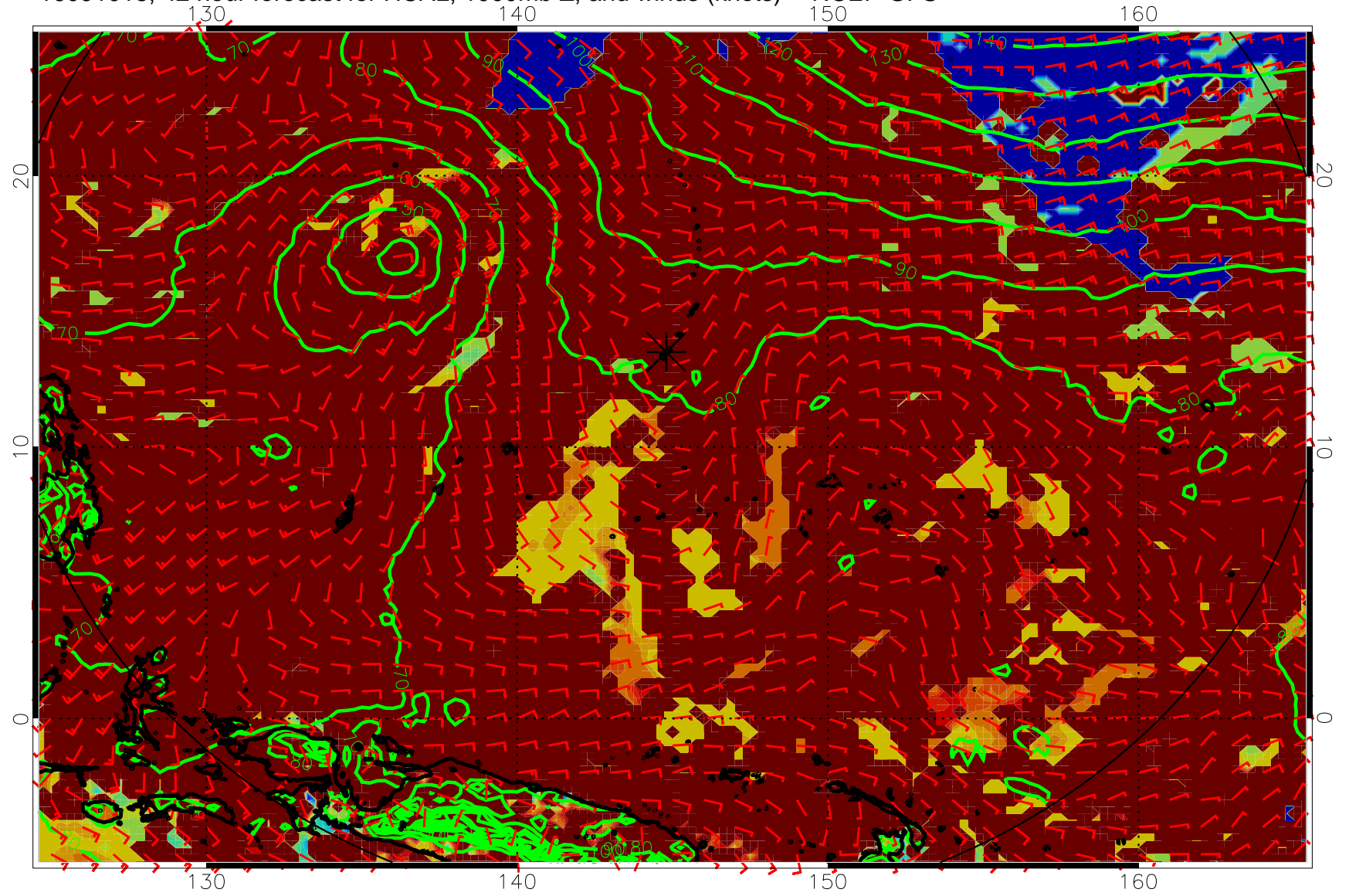
16091018, 42 hour forecast for HCAL, 1000mb Z, and winds (knots) -- NCEP GFS
