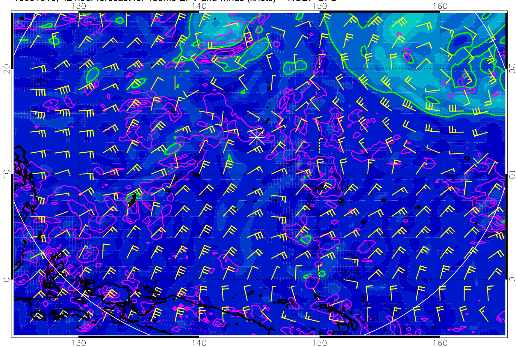
16091018, 42 hour forecast for 150mb EPV and winds (knots) -- NCEP GFS
