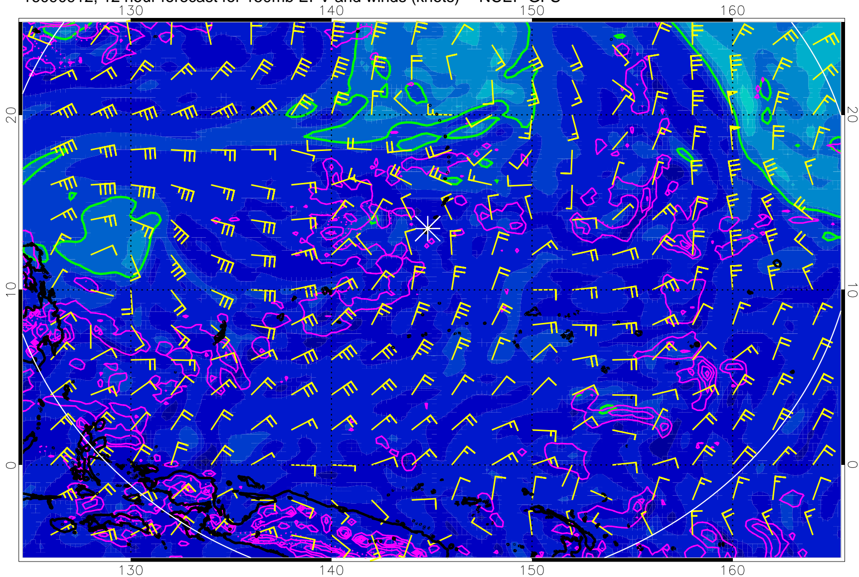
16090912, 12 hour forecast for 150mb EPV and winds (knots) -- NCEP GFS
