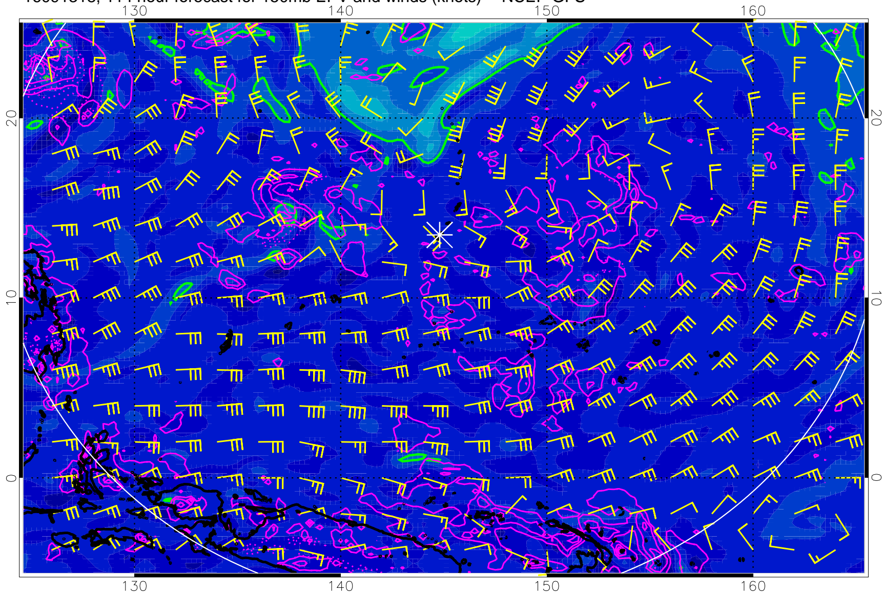
16091318, 114 hour forecast for 150mb EPV and winds (knots) -- NCEP GFS
