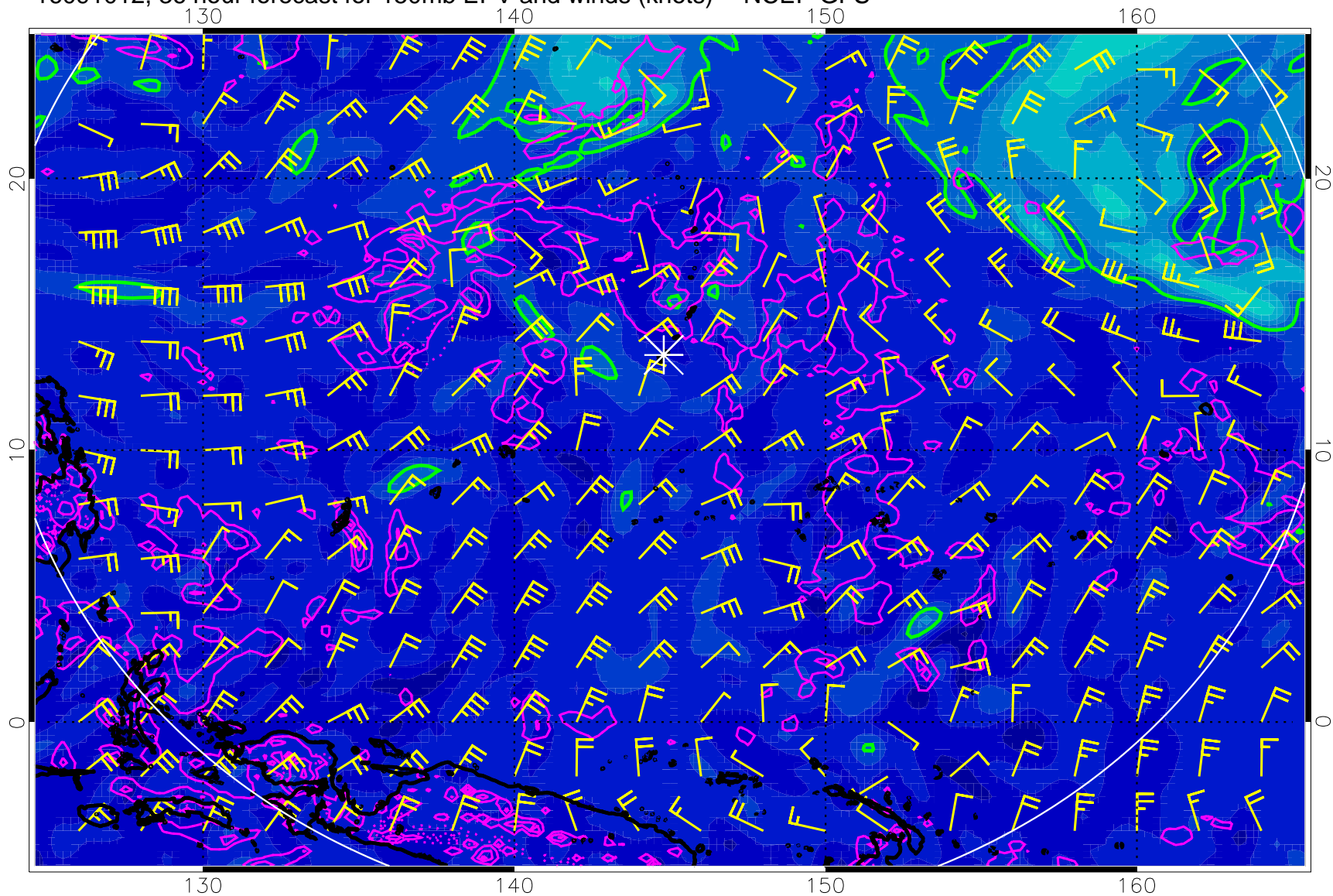
16091012, 36 hour forecast for 150mb EPV and winds (knots) -- NCEP GFS
