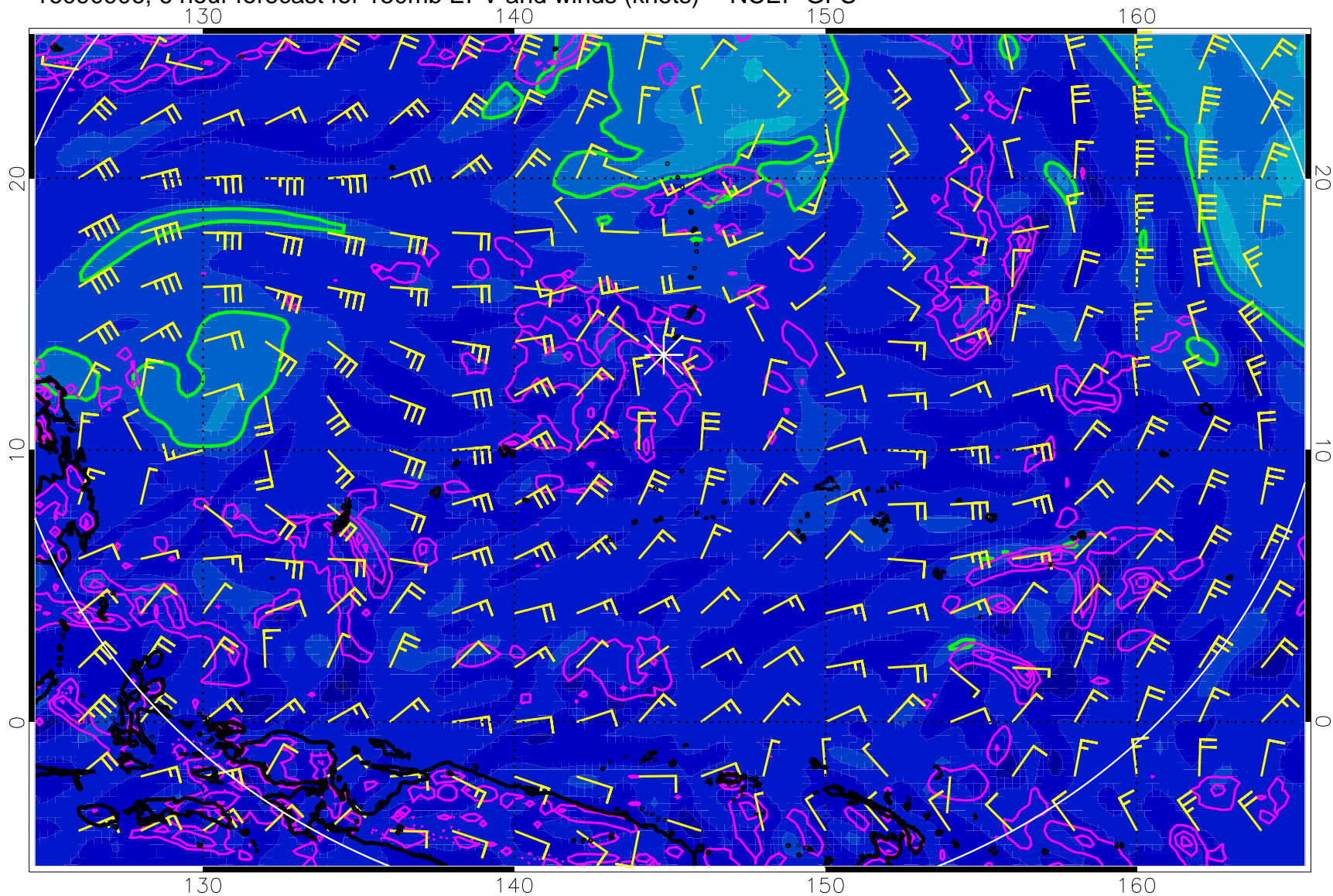
16090906, 6 hour forecast for 150mb EPV and winds (knots) -- NCEP GFS
