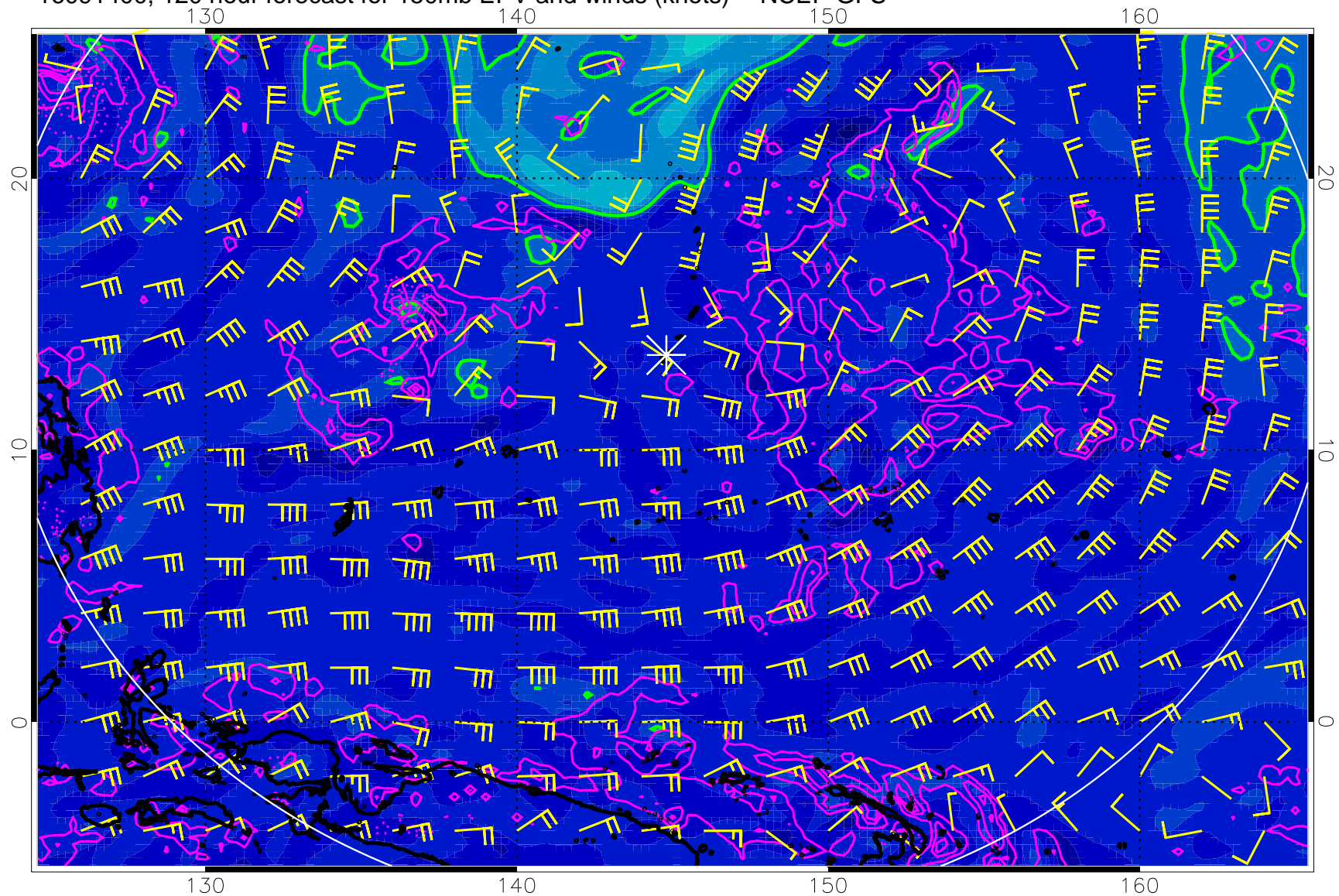
16091400, 120 hour forecast for 150mb EPV and winds (knots) -- NCEP GFS
