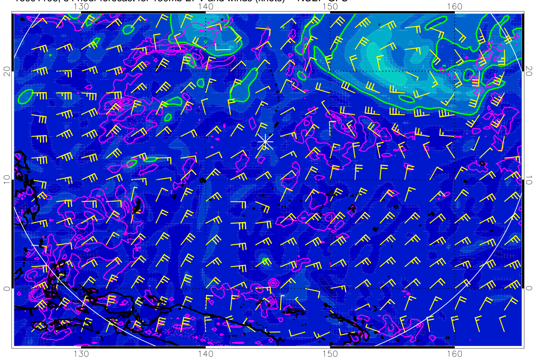
16091106, 54 hour forecast for 150mb EPV and winds (knots) -- NCEP GFS
