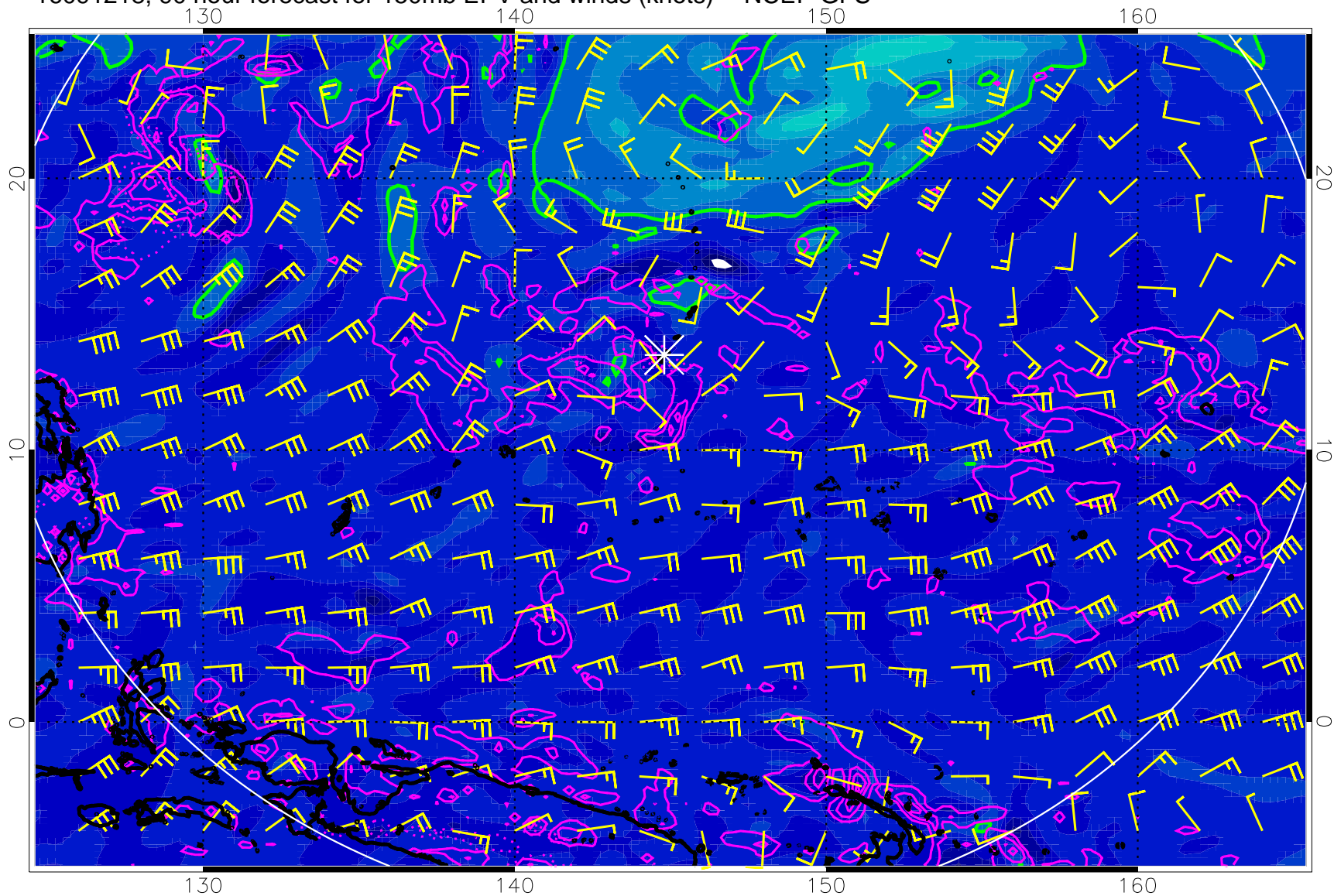
16091218, 90 hour forecast for 150mb EPV and winds (knots) -- NCEP GFS
