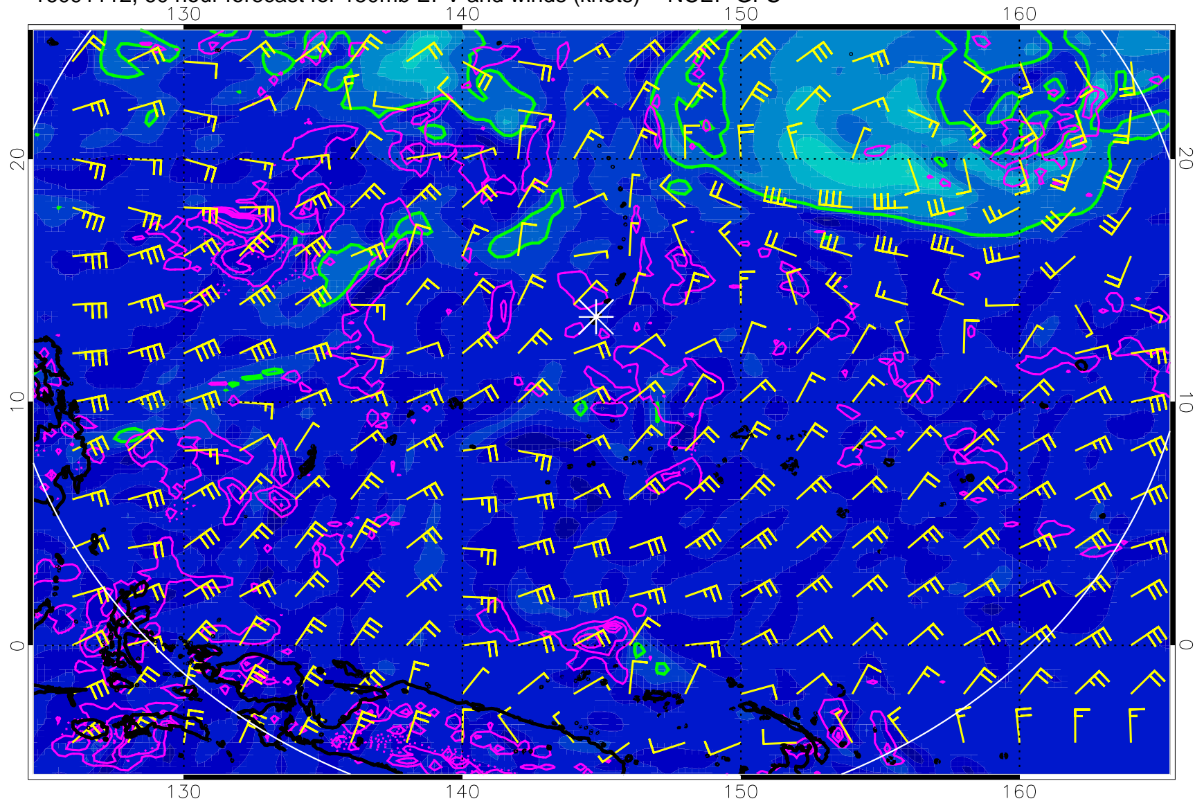
16091112, 60 hour forecast for 150mb EPV and winds (knots) -- NCEP GFS
