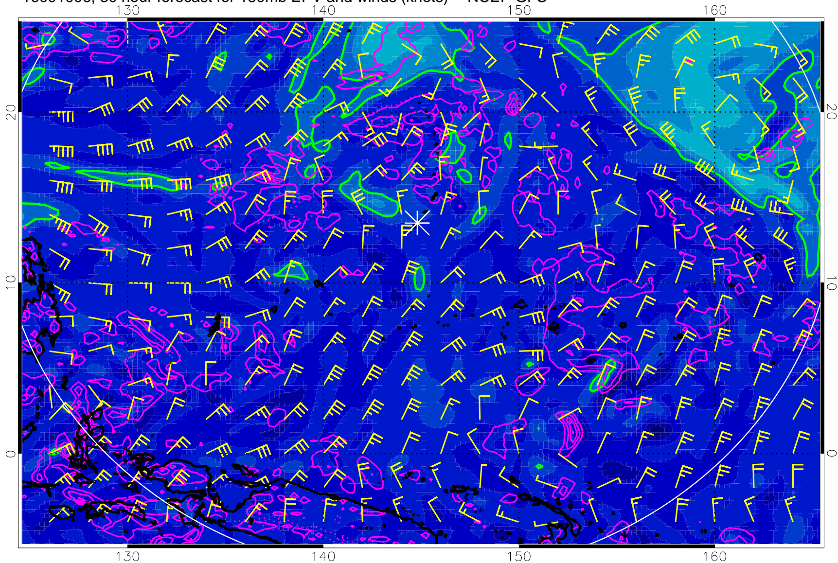
16091006, 30 hour forecast for 150mb EPV and winds (knots) -- NCEP GFS
