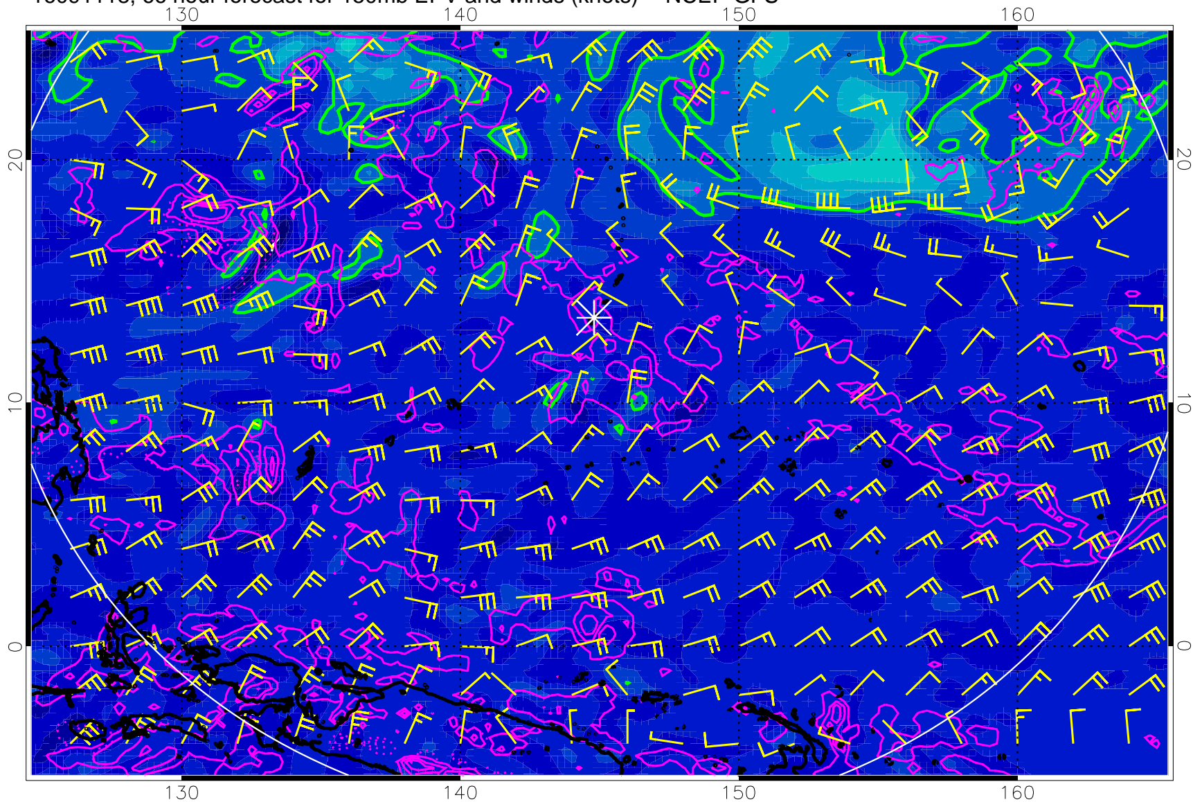
16091118, 66 hour forecast for 150mb EPV and winds (knots) -- NCEP GFS
