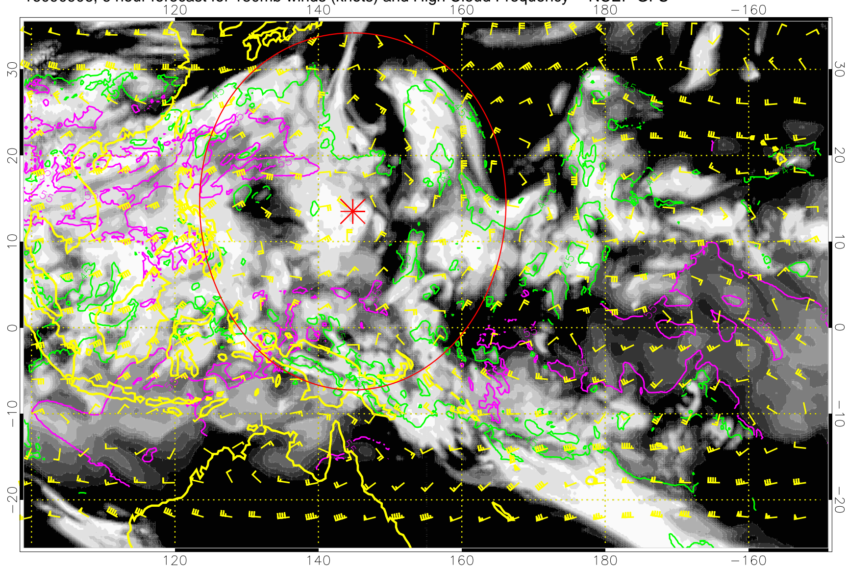
16090906, 6 hour forecast for 150mb winds (knots) and High Cloud Frequency -- NCEP GFS
