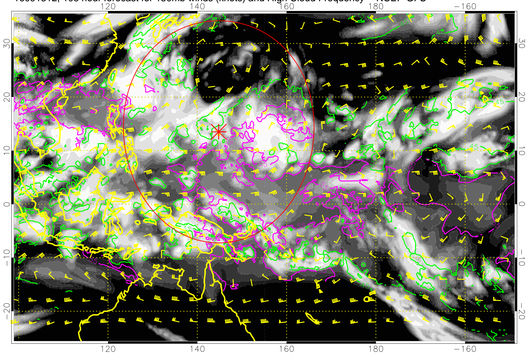
16091312, 108 hour forecast for 150mb winds (knots) and High Cloud Frequency -- NCEP GFS
