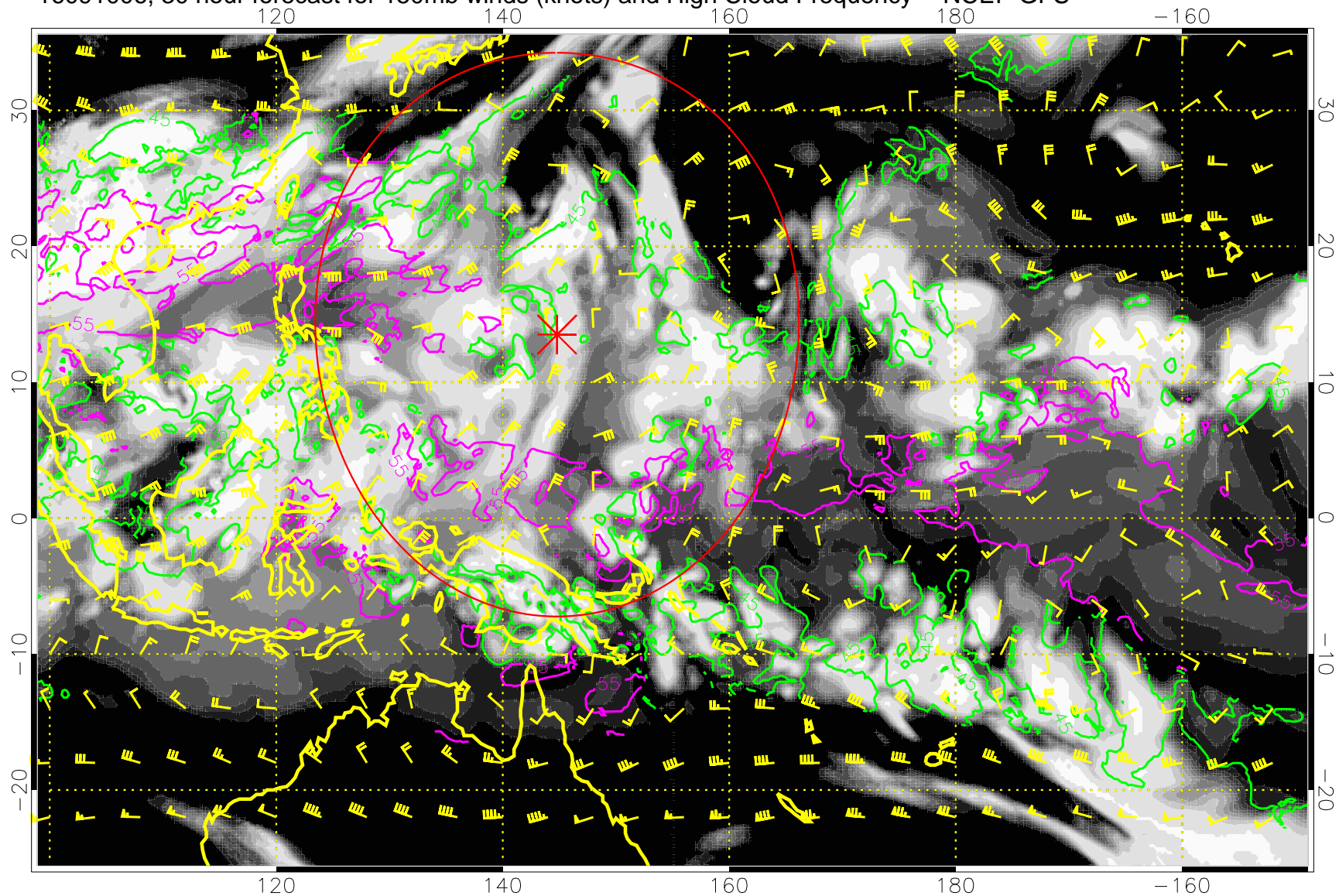
16091006, 30 hour forecast for 150mb winds (knots) and High Cloud Frequency -- NCEP GFS
