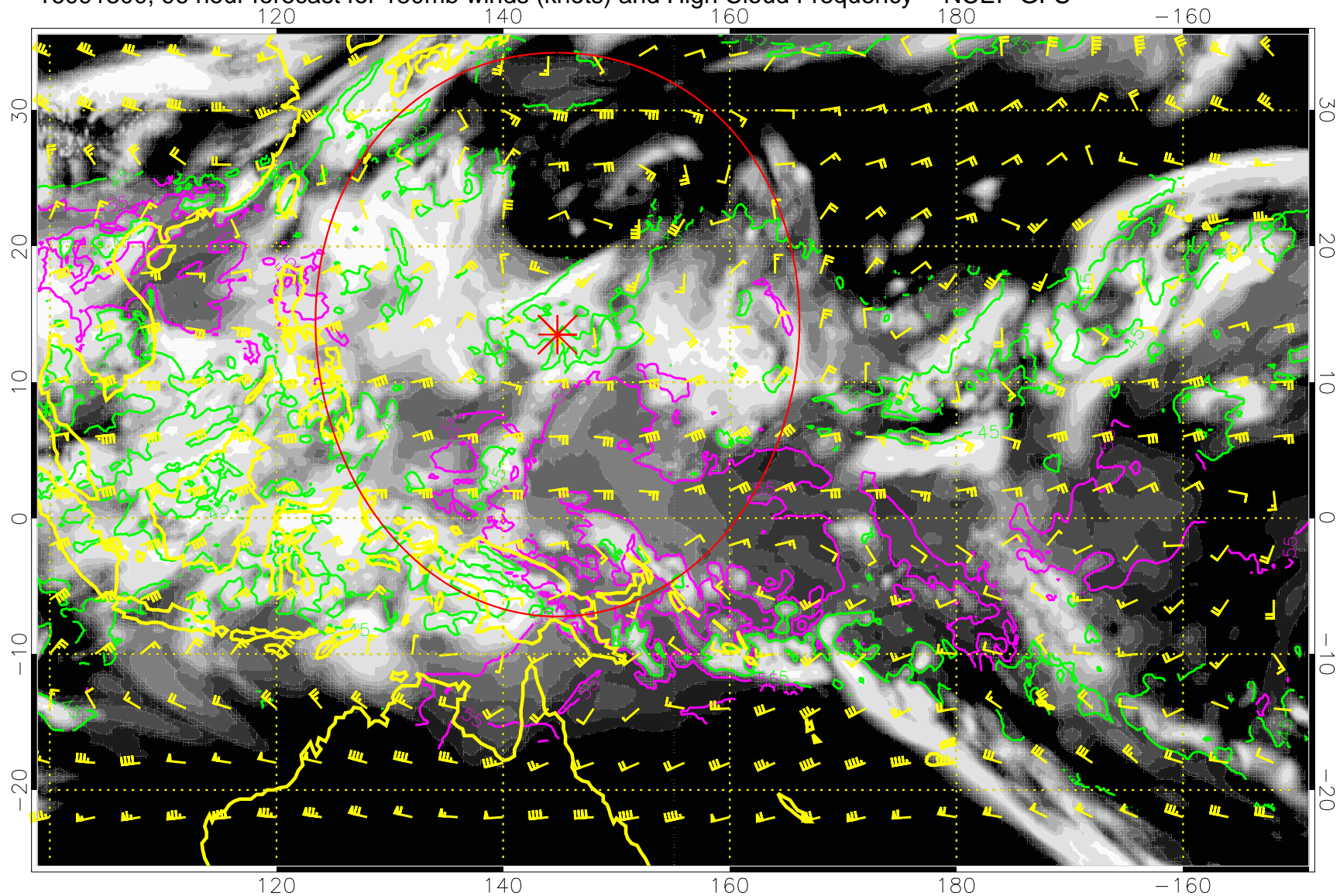
16091300, 96 hour forecast for 150mb winds (knots) and High Cloud Frequency -- NCEP GFS
