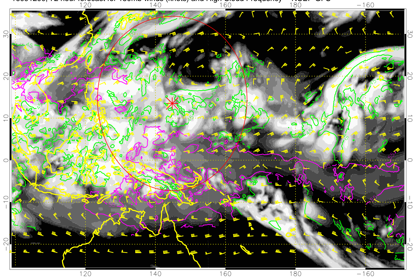
16091200, 72 hour forecast for 150mb winds (knots) and High Cloud Frequency -- NCEP GFS
