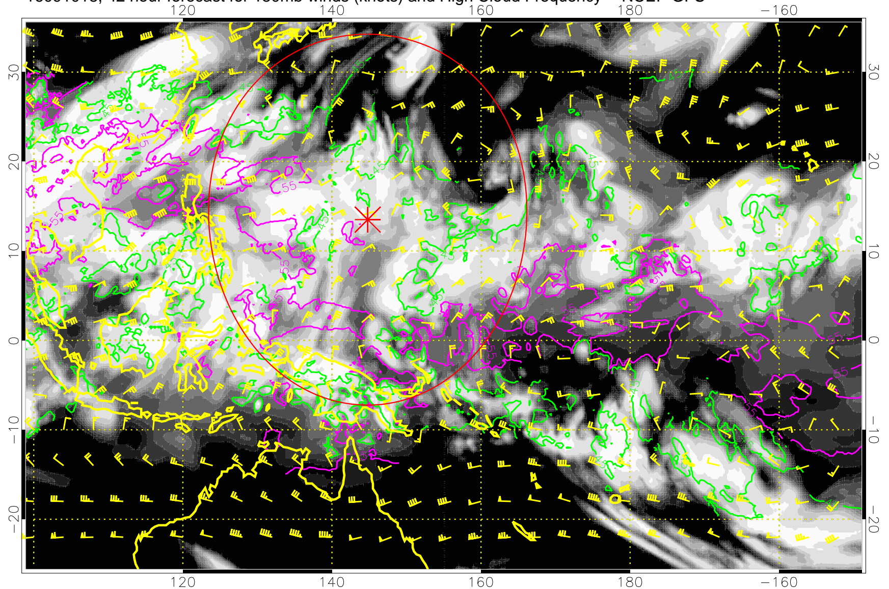
16091018, 42 hour forecast for 150mb winds (knots) and High Cloud Frequency -- NCEP GFS
