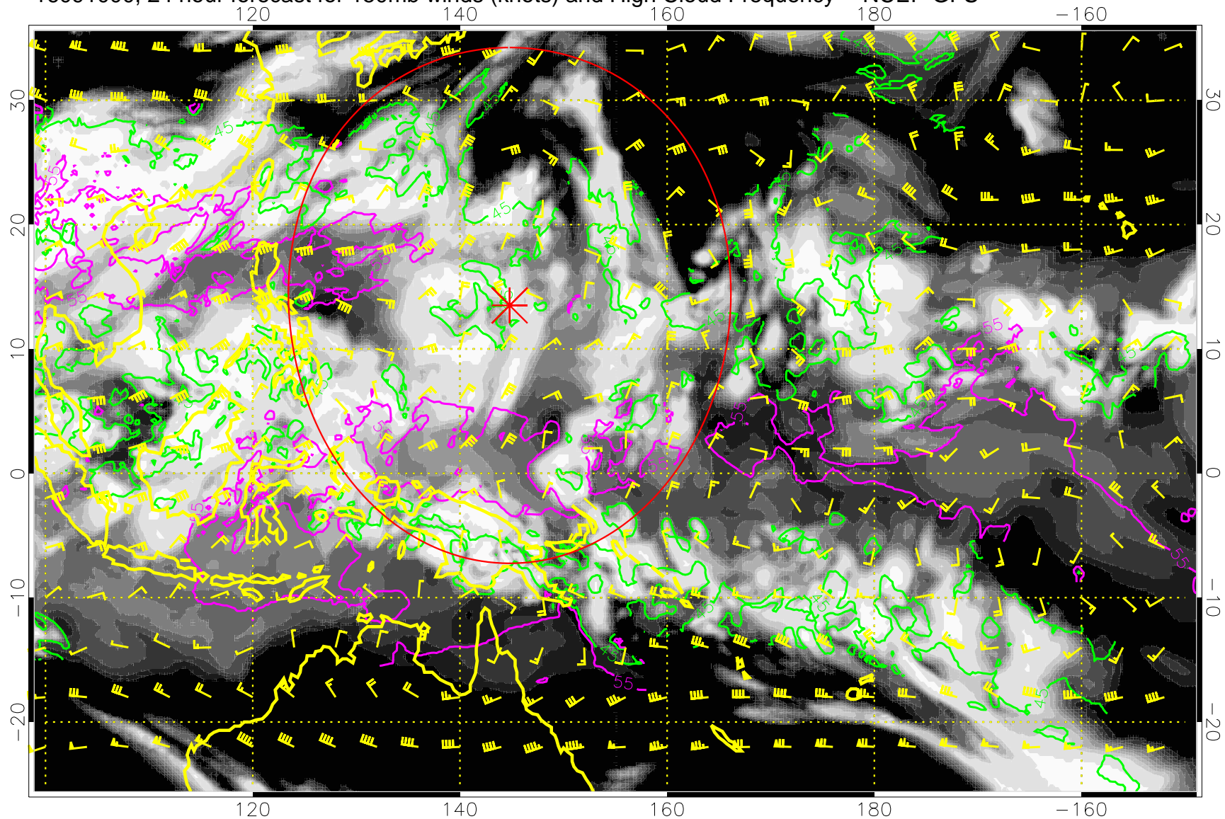
16091000, 24 hour forecast for 150mb winds (knots) and High Cloud Frequency -- NCEP GFS
