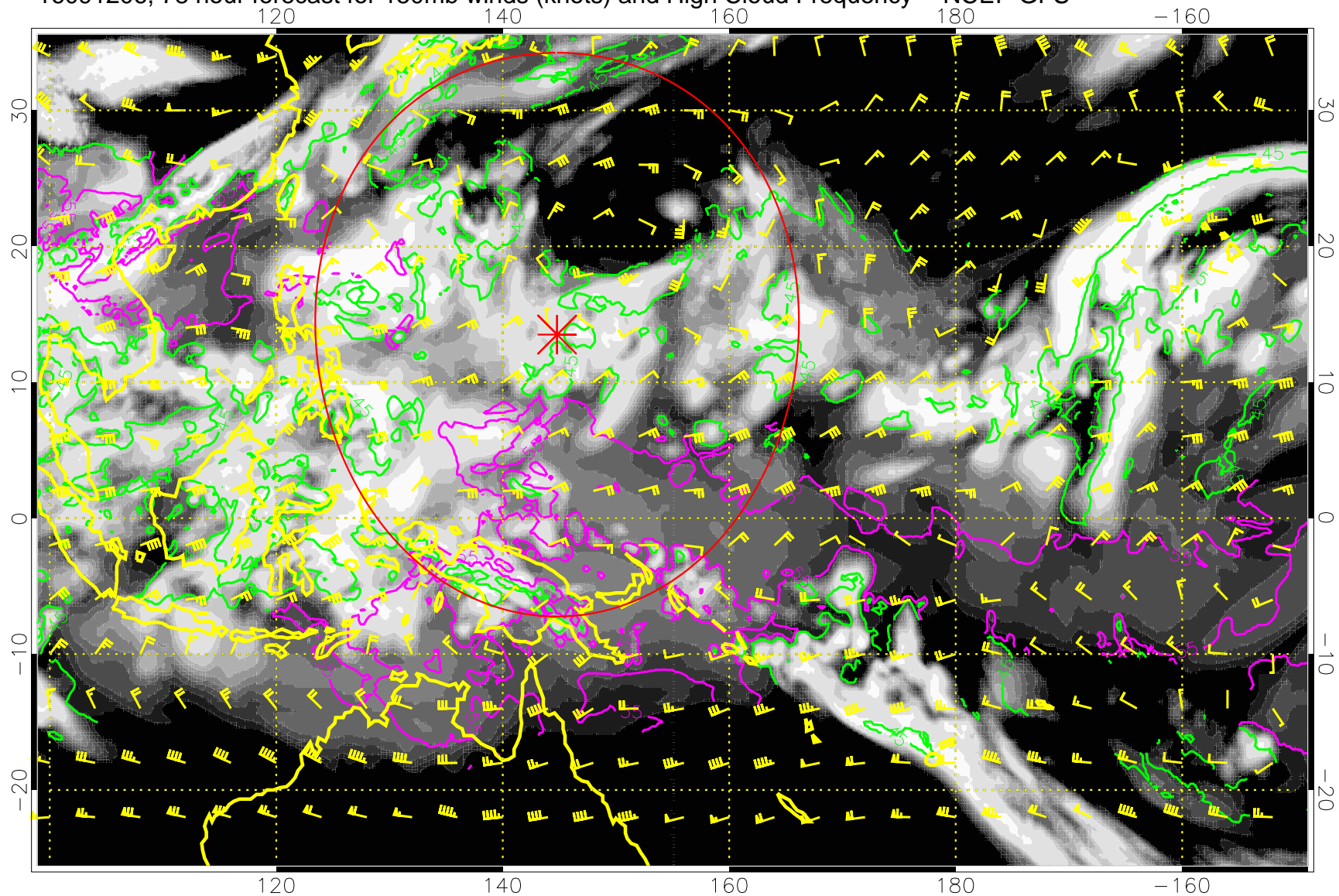
16091206, 78 hour forecast for 150mb winds (knots) and High Cloud Frequency -- NCEP GFS
