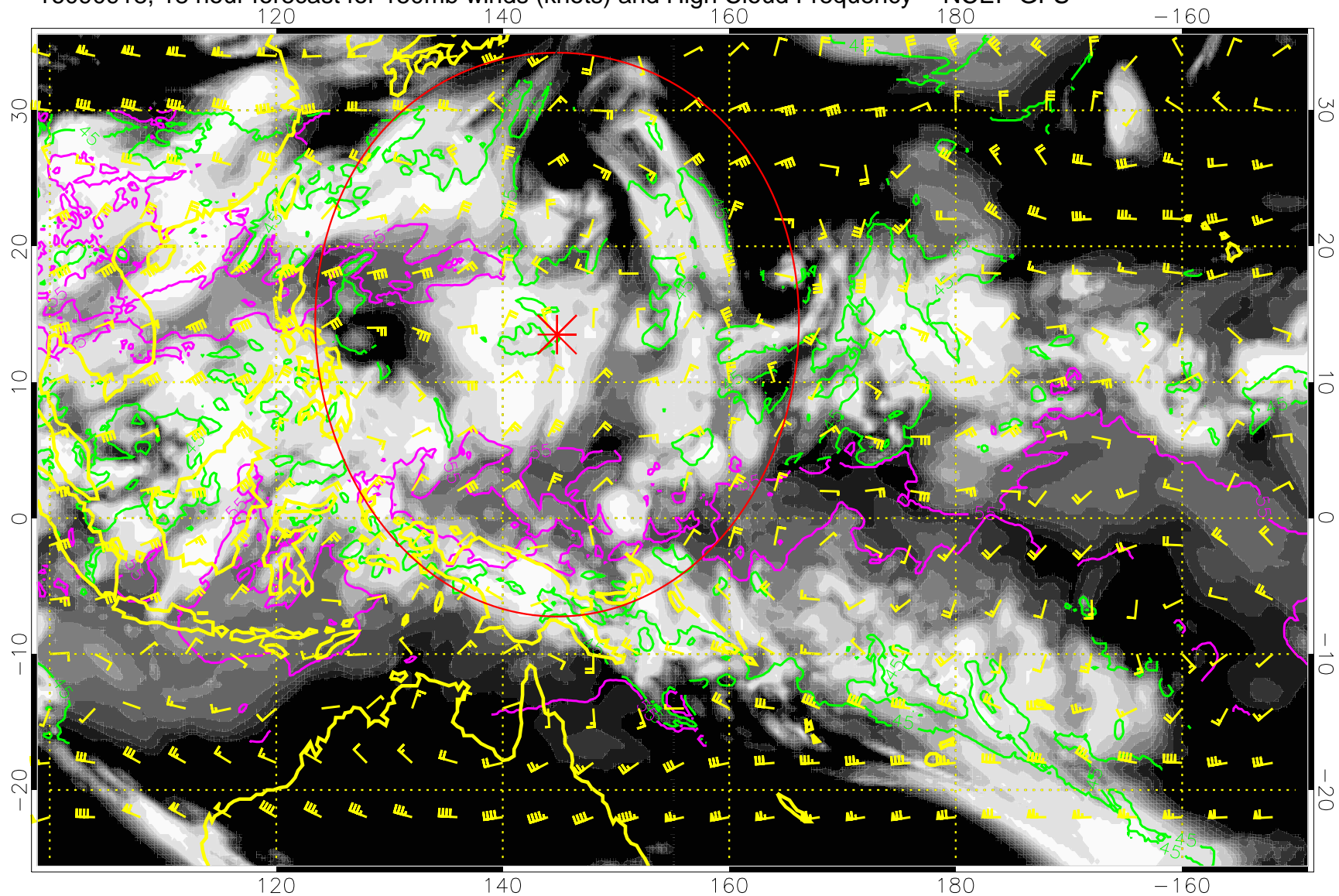
16090918, 18 hour forecast for 150mb winds (knots) and High Cloud Frequency -- NCEP GFS
