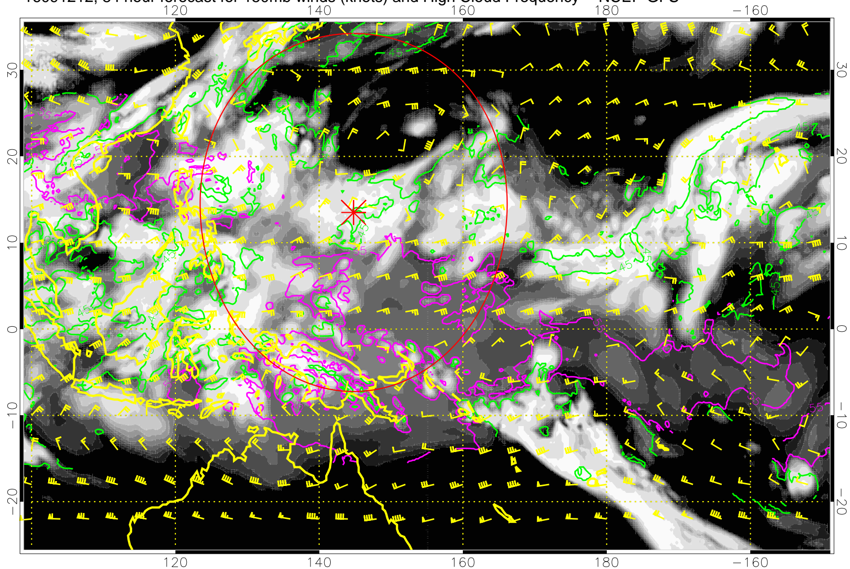
16091212, 84 hour forecast for 150mb winds (knots) and High Cloud Frequency -- NCEP GFS
