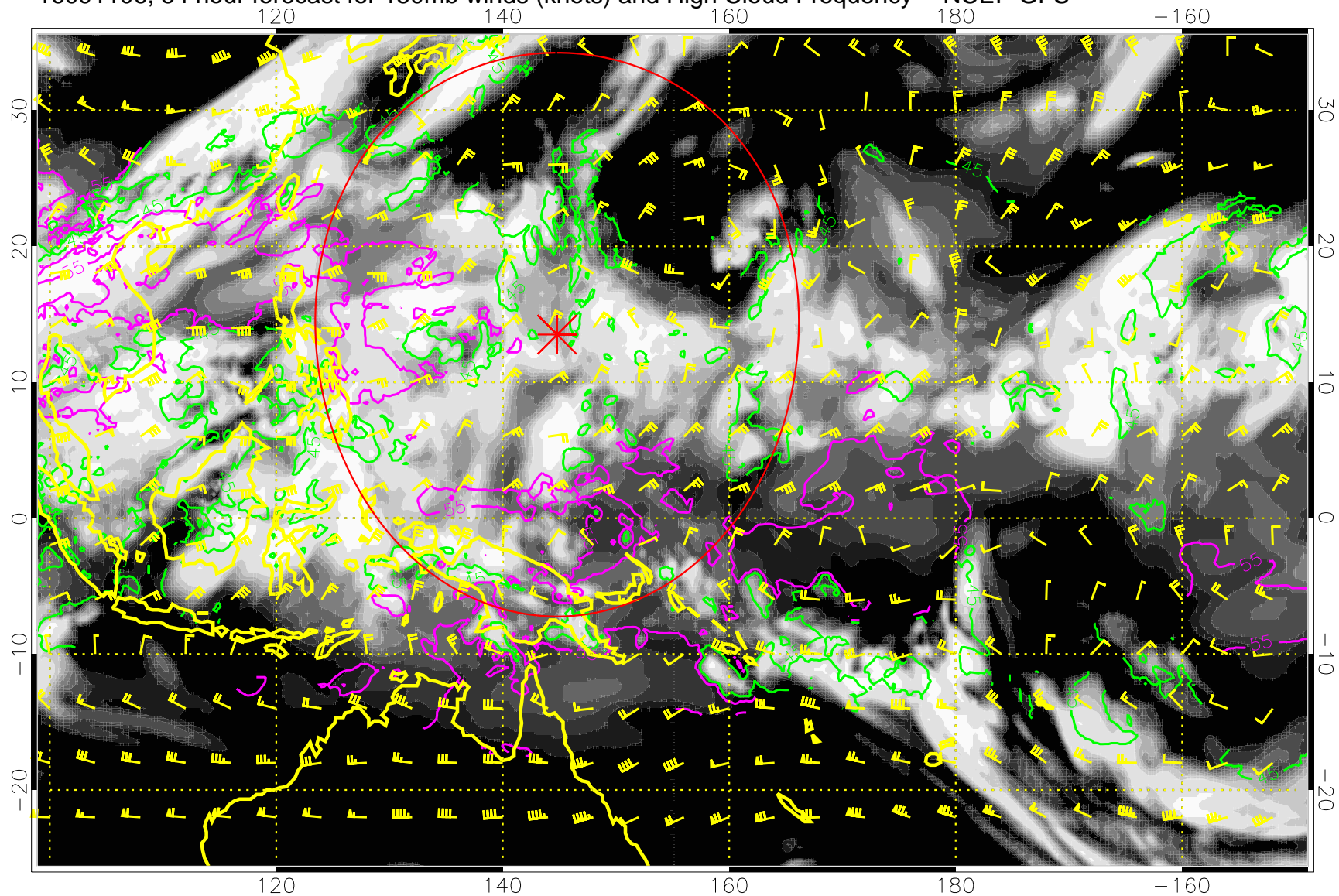
16091106, 54 hour forecast for 150mb winds (knots) and High Cloud Frequency -- NCEP GFS
