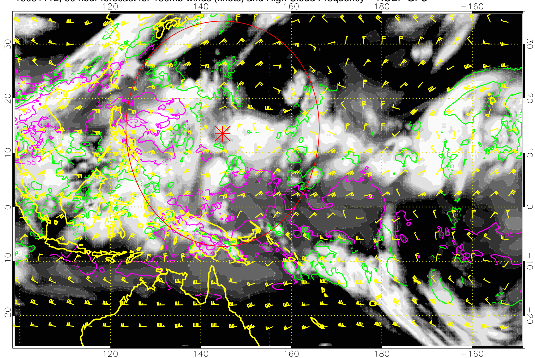
16091112, 60 hour forecast for 150mb winds (knots) and High Cloud Frequency -- NCEP GFS
