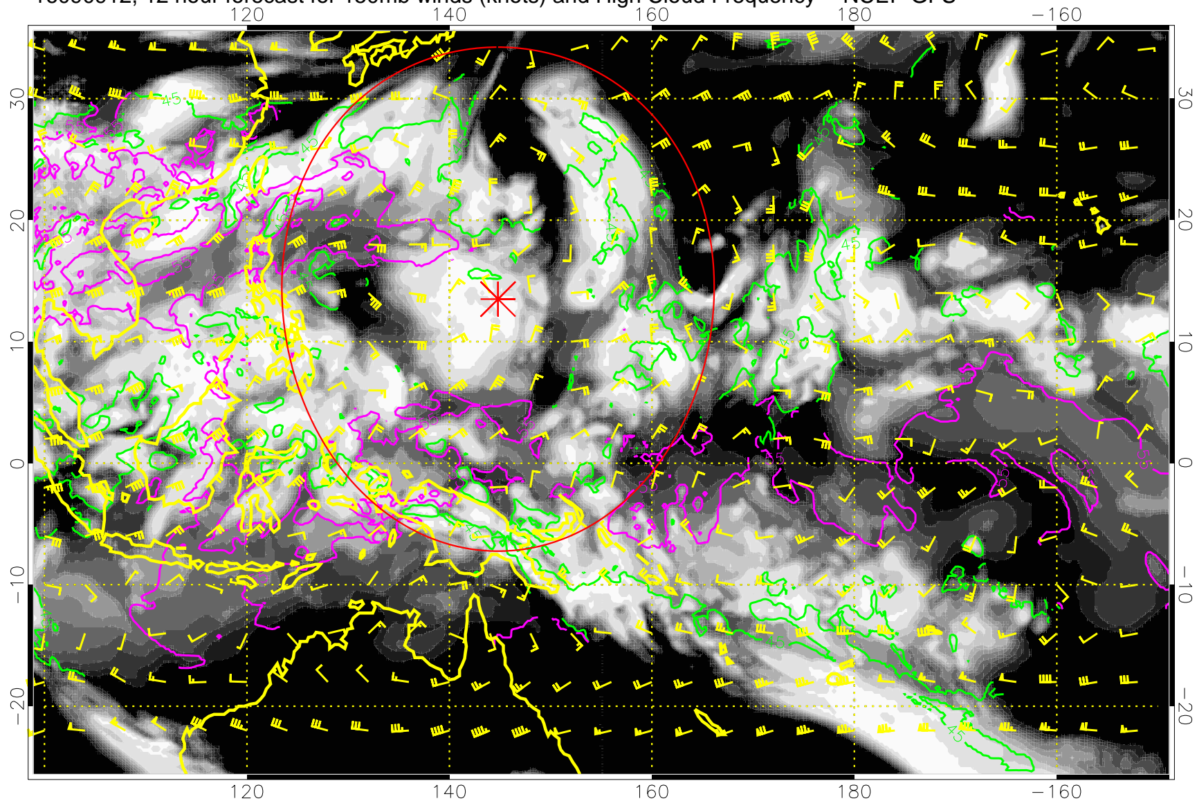
16090912, 12 hour forecast for 150mb winds (knots) and High Cloud Frequency -- NCEP GFS
