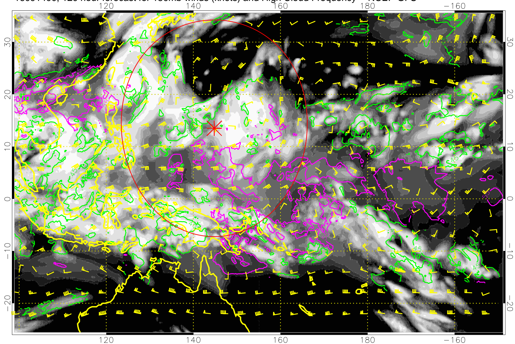
16091400, 120 hour forecast for 150mb winds (knots) and High Cloud Frequency -- NCEP GFS
