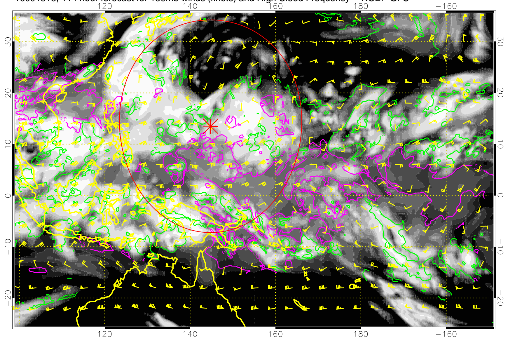
16091318, 114 hour forecast for 150mb winds (knots) and High Cloud Frequency -- NCEP GFS
