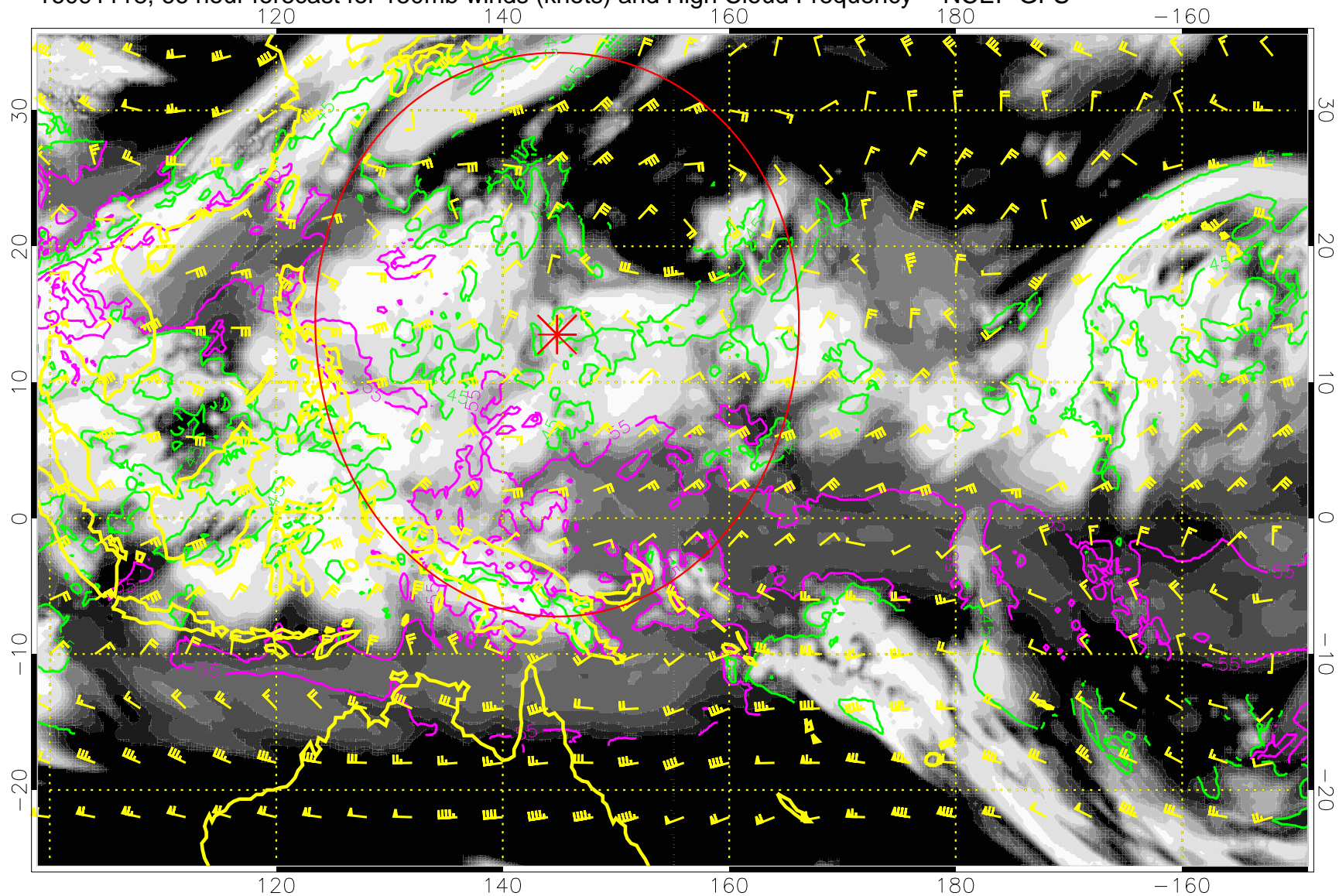
16091118, 66 hour forecast for 150mb winds (knots) and High Cloud Frequency -- NCEP GFS
