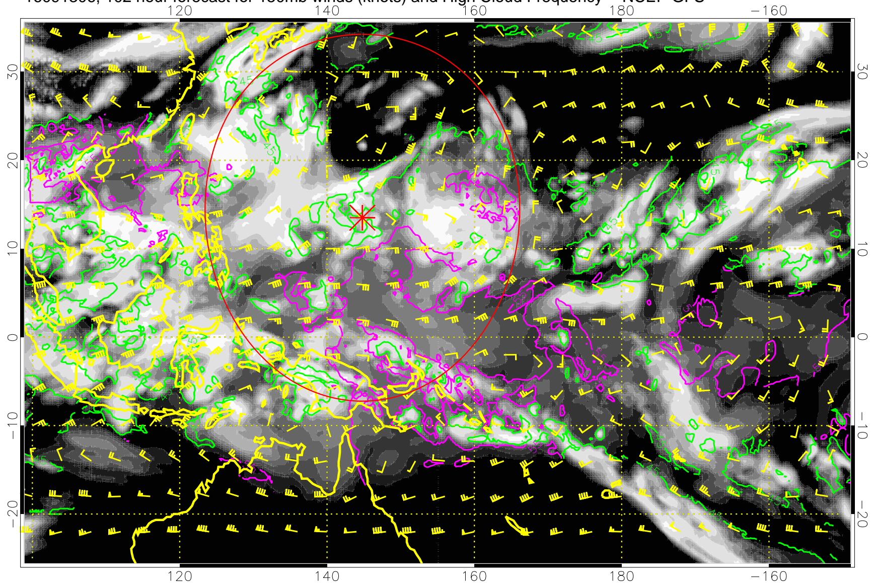
16091306, 102 hour forecast for 150mb winds (knots) and High Cloud Frequency -- NCEP GFS
