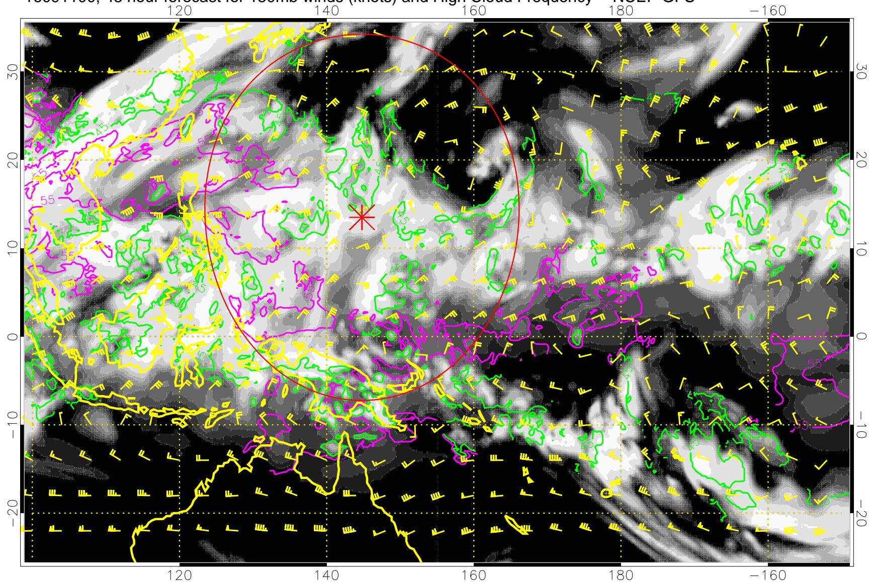
16091100, 48 hour forecast for 150mb winds (knots) and High Cloud Frequency -- NCEP GFS
