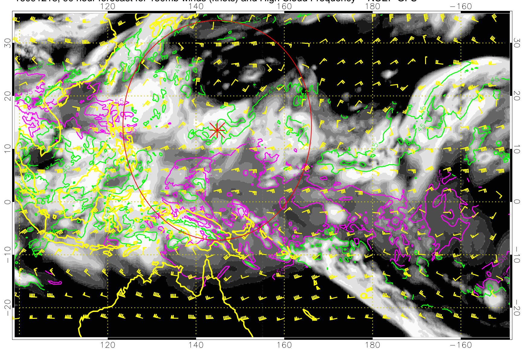
16091218, 90 hour forecast for 150mb winds (knots) and High Cloud Frequency -- NCEP GFS
