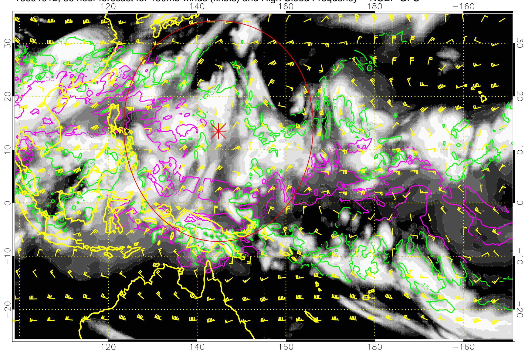
16091012, 36 hour forecast for 150mb winds (knots) and High Cloud Frequency -- NCEP GFS
