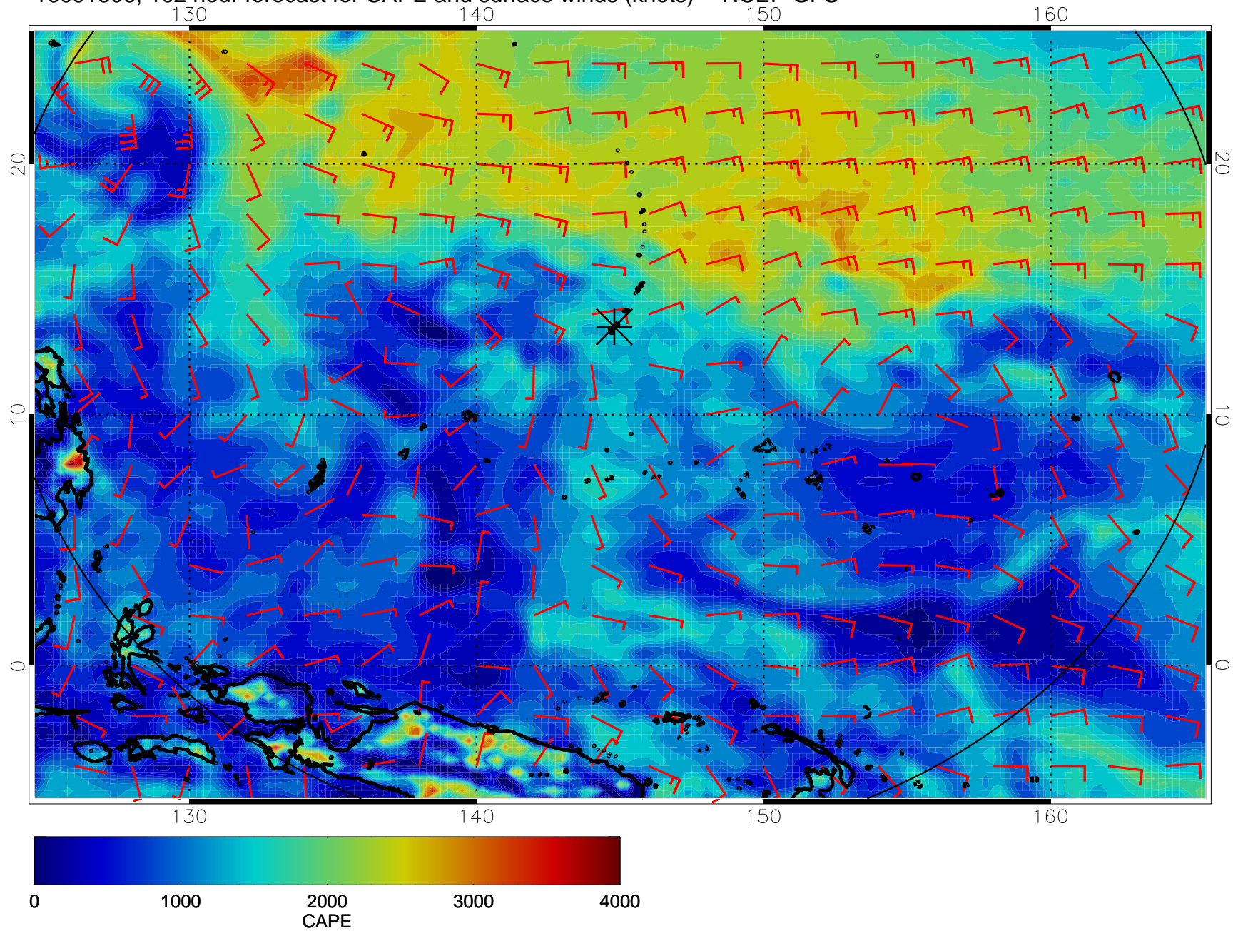
16091306, 102 hour forecast for CAPE and surface winds (knots) -- NCEP GFS
