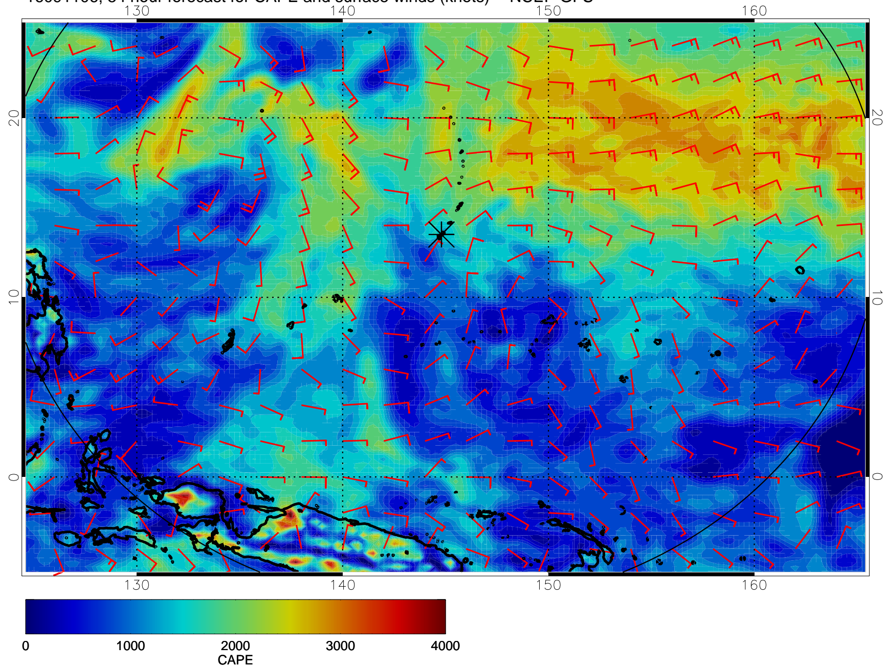
16091106, 54 hour forecast for CAPE and surface winds (knots) -- NCEP GFS
