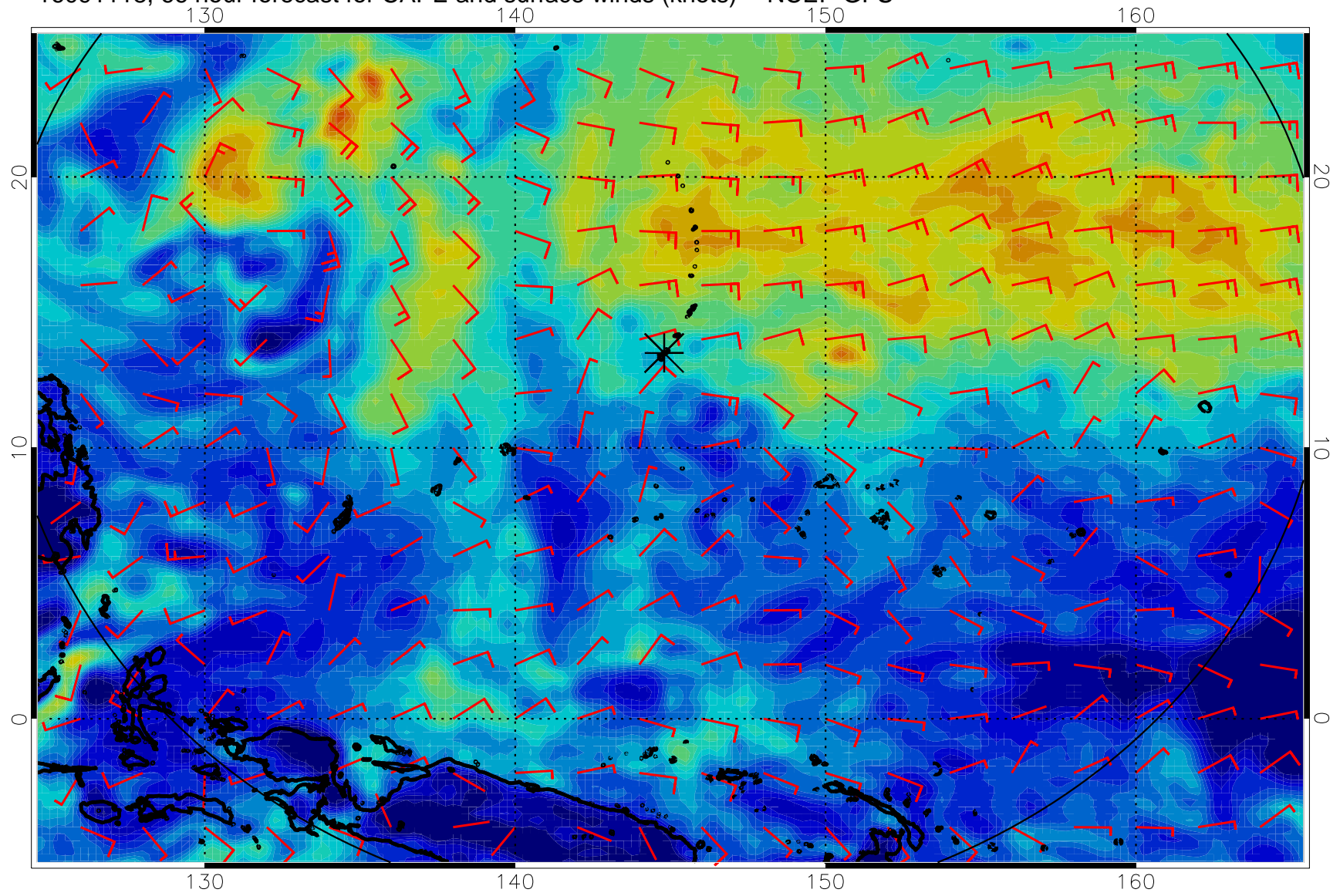
16091118, 66 hour forecast for CAPE and surface winds (knots) -- NCEP GFS
