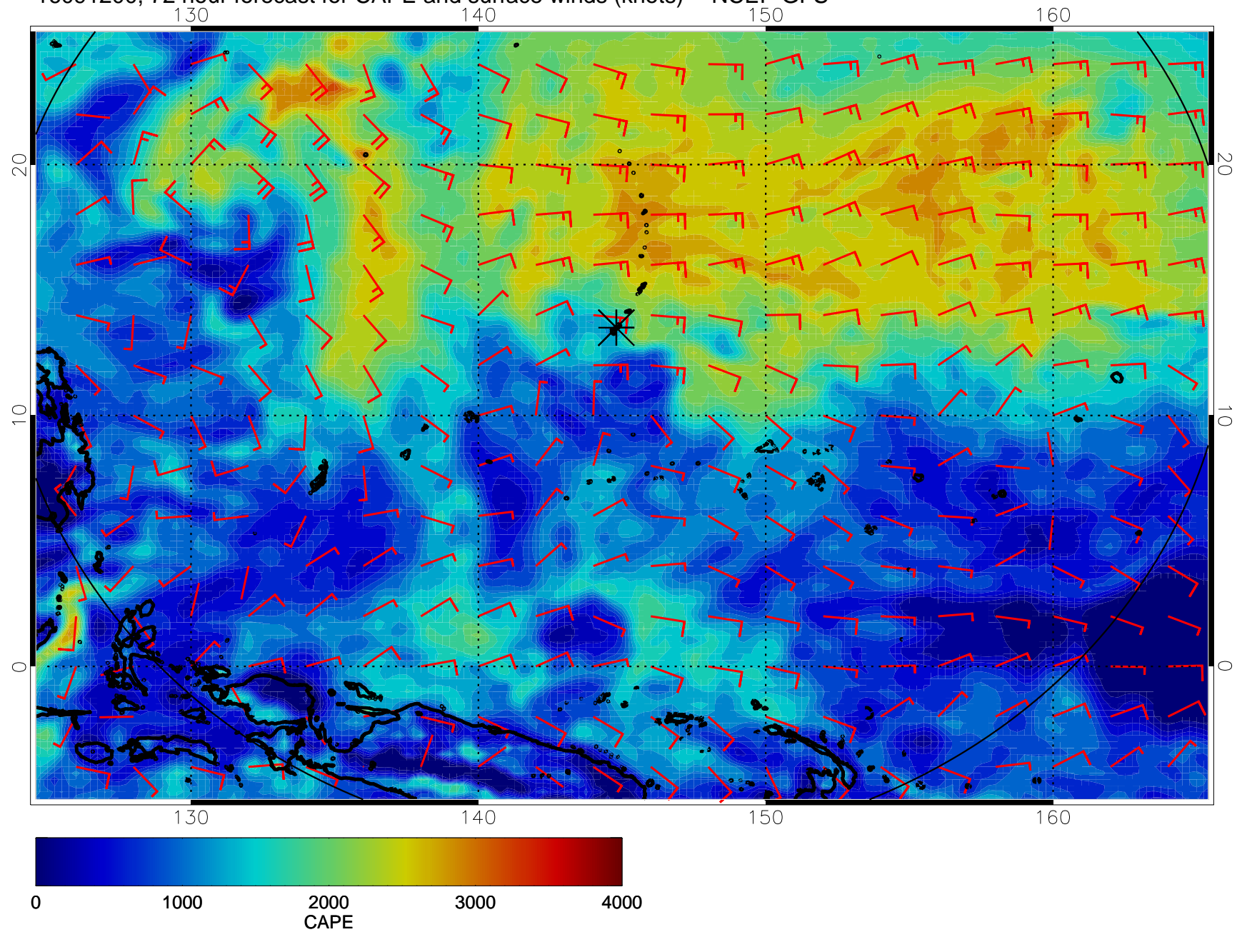
16091200, 72 hour forecast for CAPE and surface winds (knots) -- NCEP GFS
