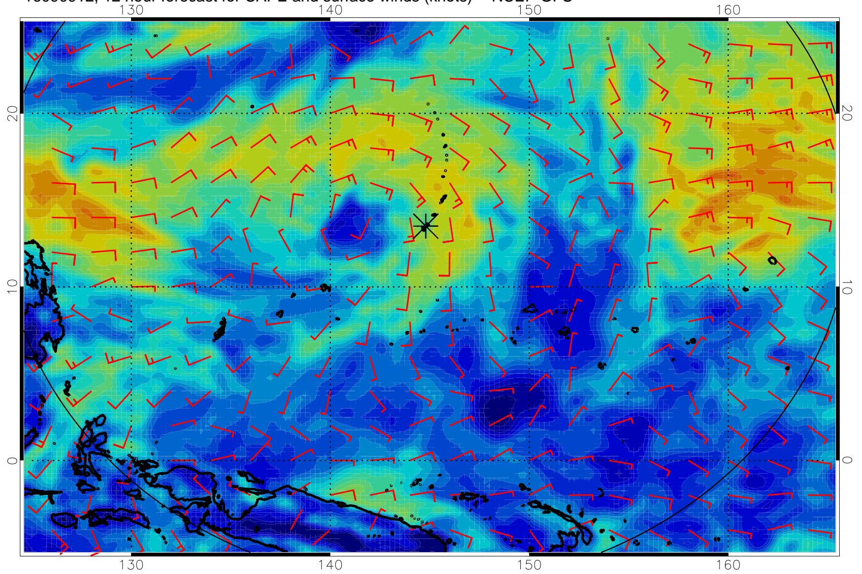
16090912, 12 hour forecast for CAPE and surface winds (knots) -- NCEP GFS
