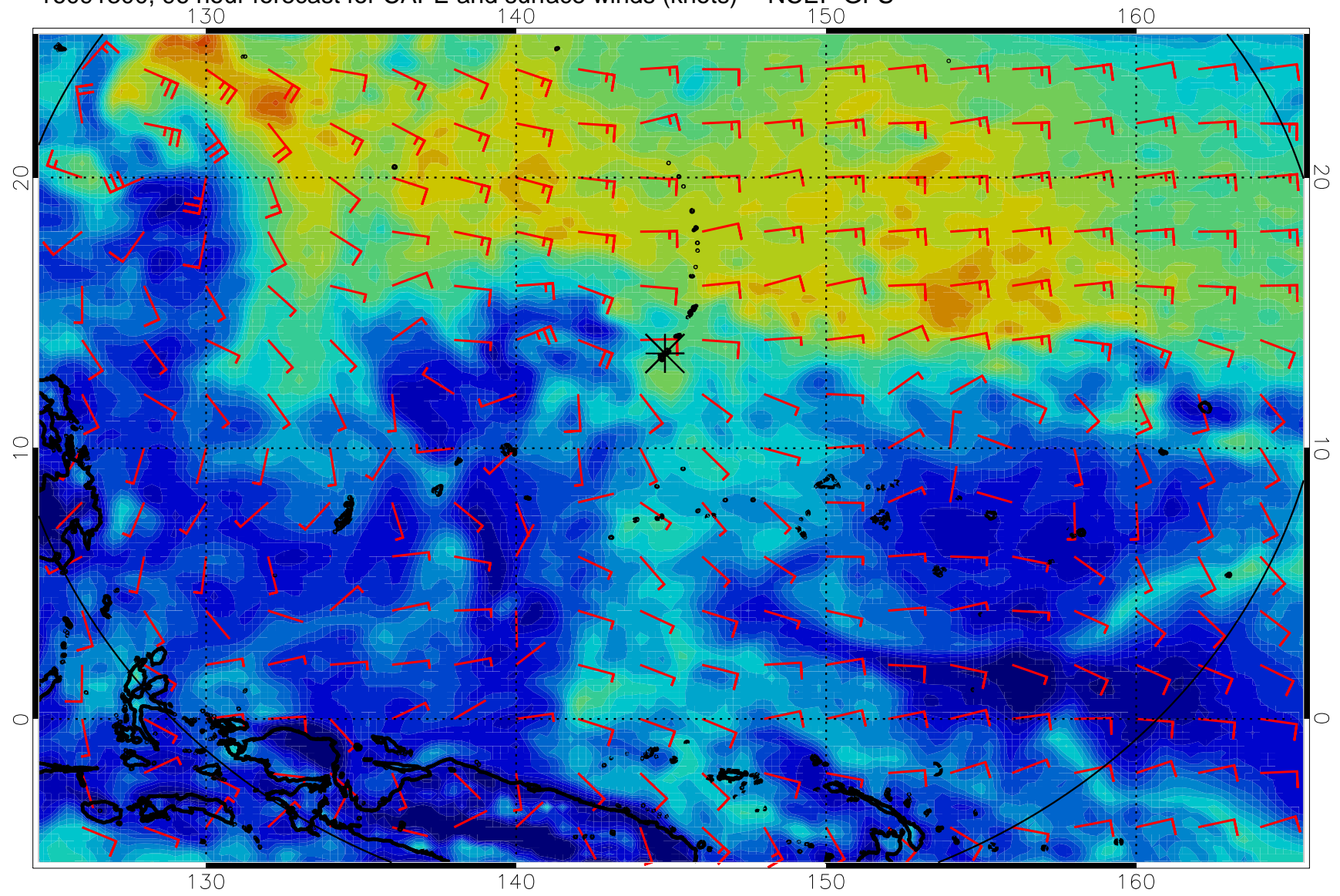
16091300, 96 hour forecast for CAPE and surface winds (knots) -- NCEP GFS
