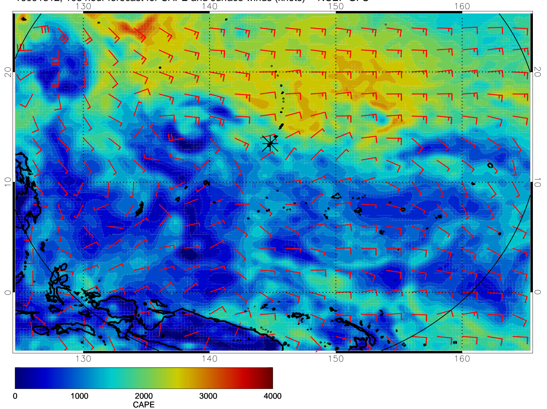
16091312, 108 hour forecast for CAPE and surface winds (knots) -- NCEP GFS
