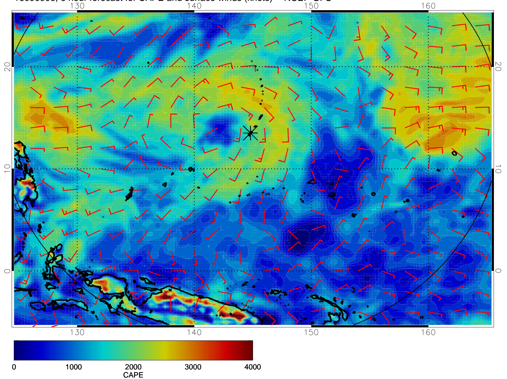
16090906, 6 hour forecast for CAPE and surface winds (knots) -- NCEP GFS
