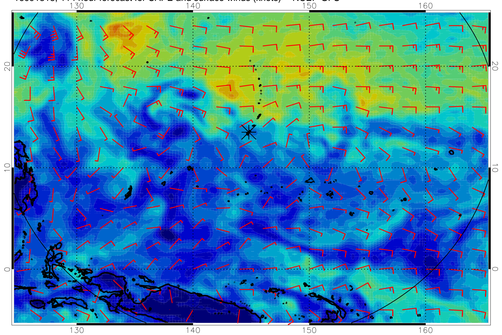
16091318, 114 hour forecast for CAPE and surface winds (knots) -- NCEP GFS
