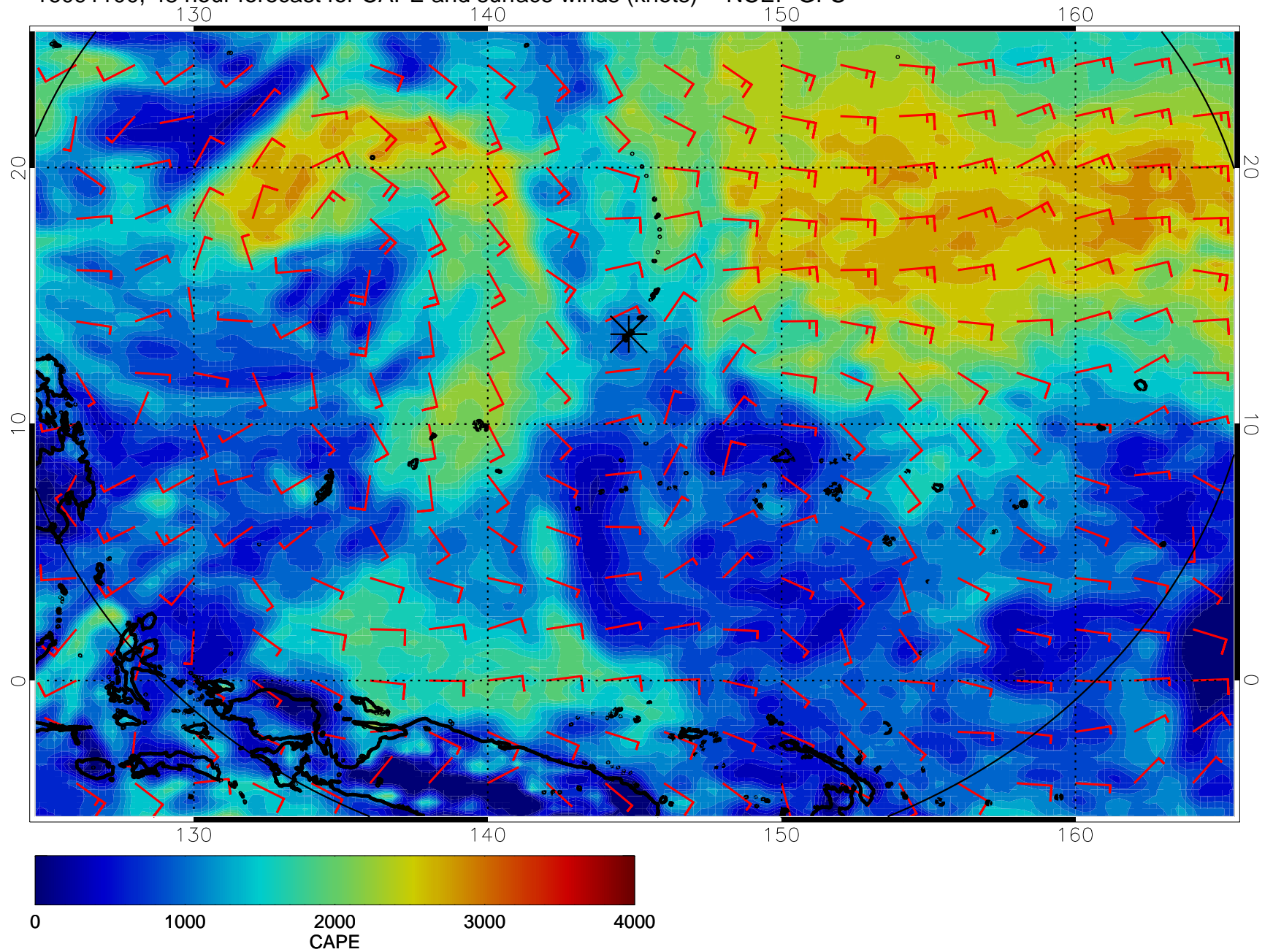
16091100, 48 hour forecast for CAPE and surface winds (knots) -- NCEP GFS
