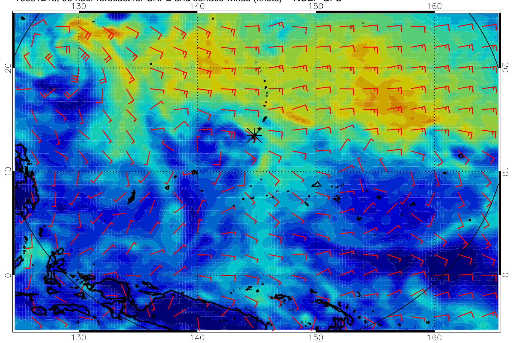
16091218, 90 hour forecast for CAPE and surface winds (knots) -- NCEP GFS
