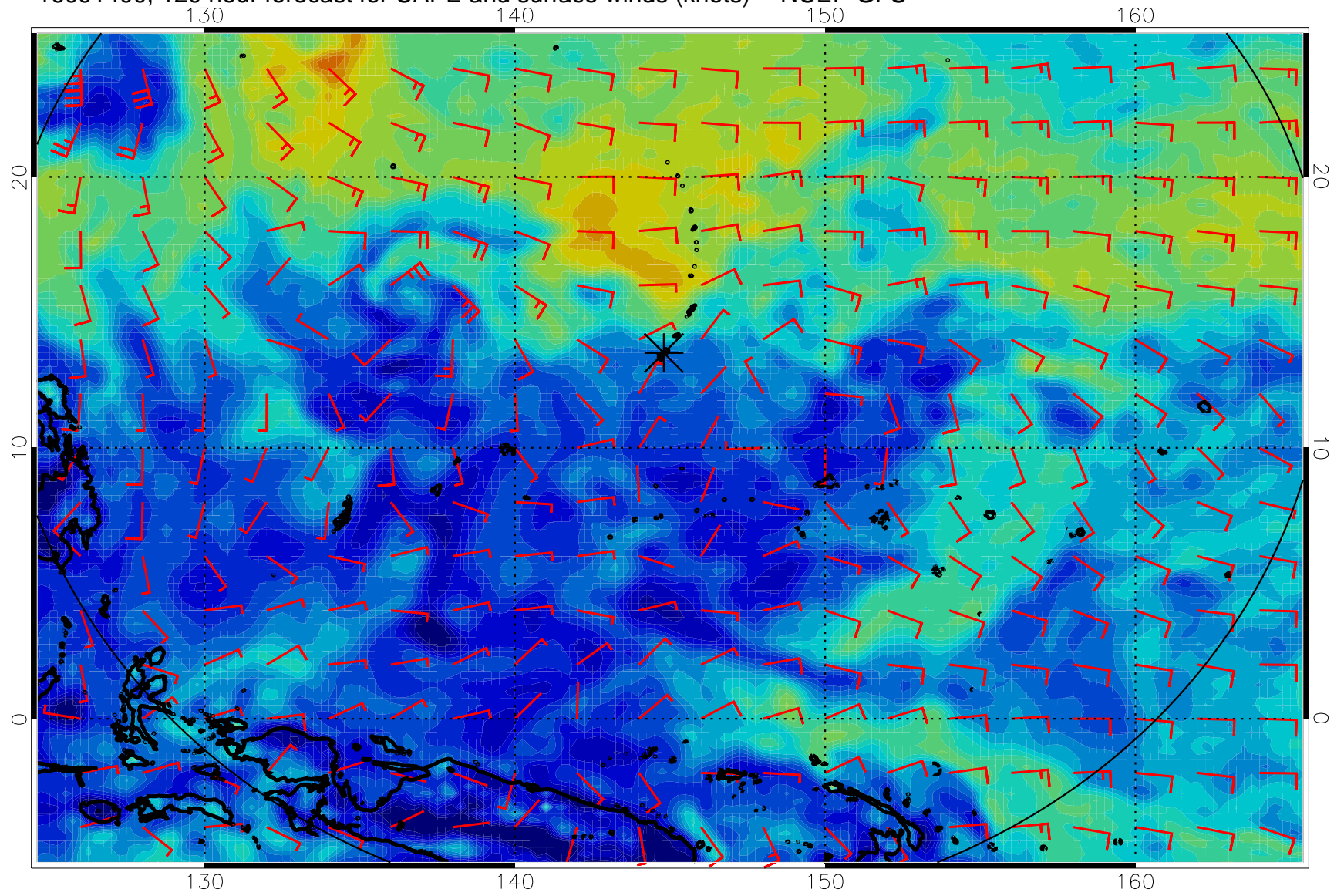
16091400, 120 hour forecast for CAPE and surface winds (knots) -- NCEP GFS
