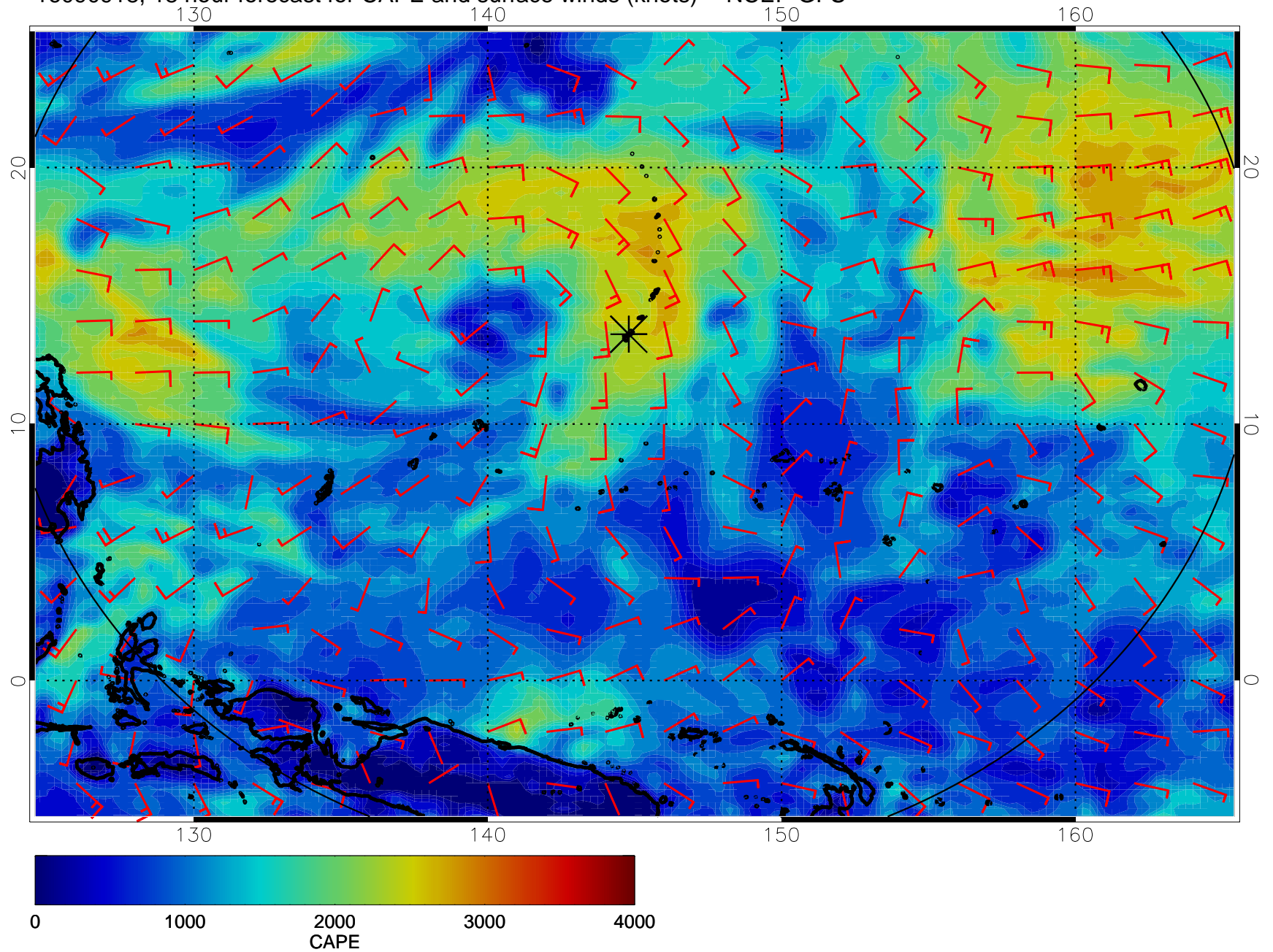
16090918, 18 hour forecast for CAPE and surface winds (knots) -- NCEP GFS
