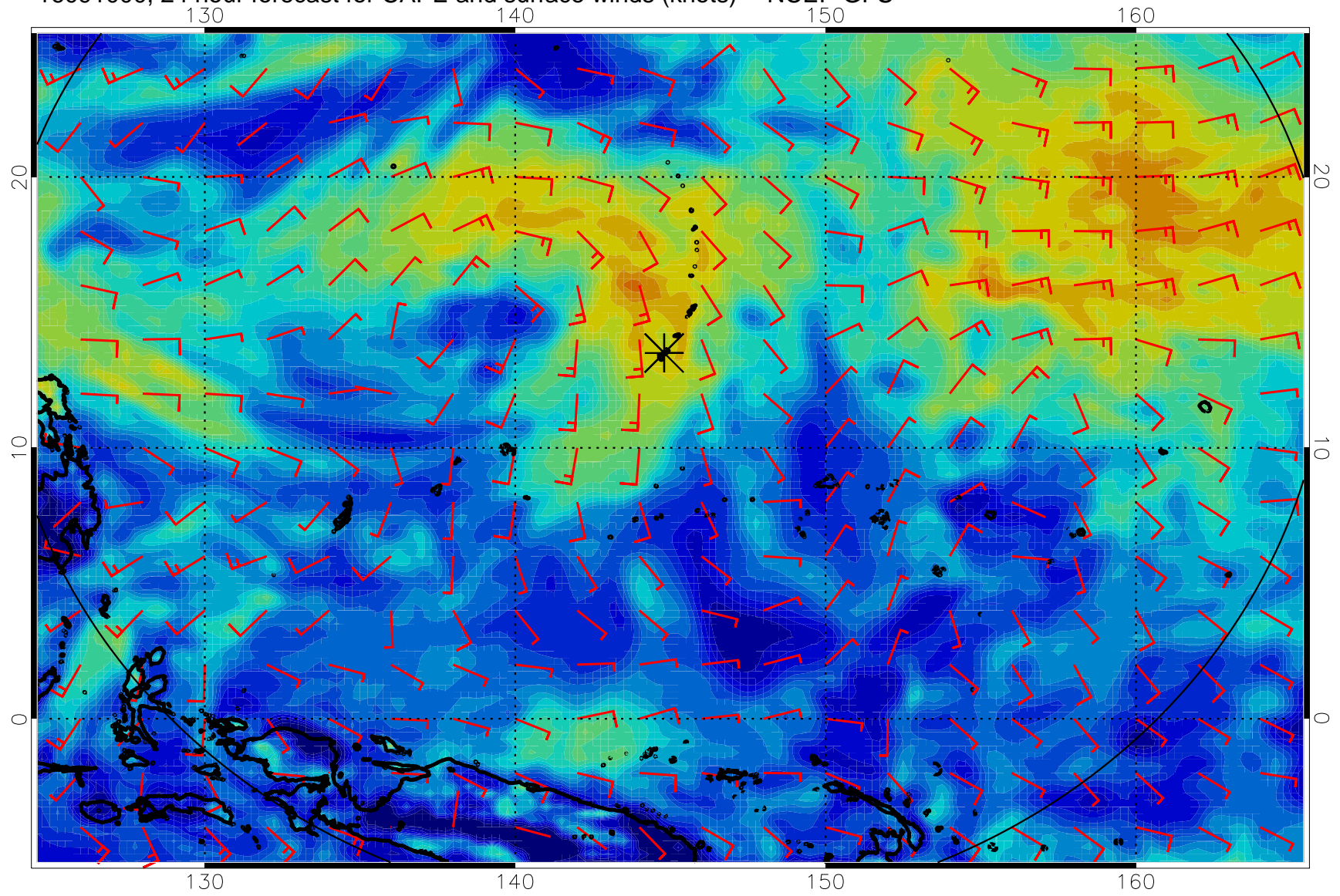
16091000, 24 hour forecast for CAPE and surface winds (knots) -- NCEP GFS
