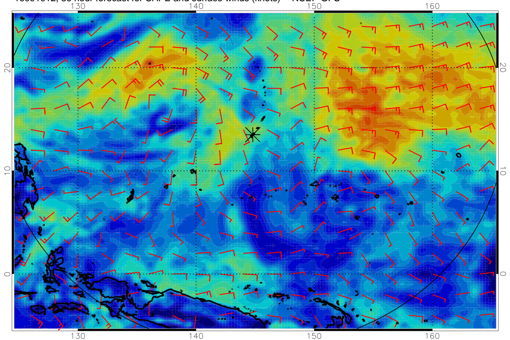
16091012, 36 hour forecast for CAPE and surface winds (knots) -- NCEP GFS
