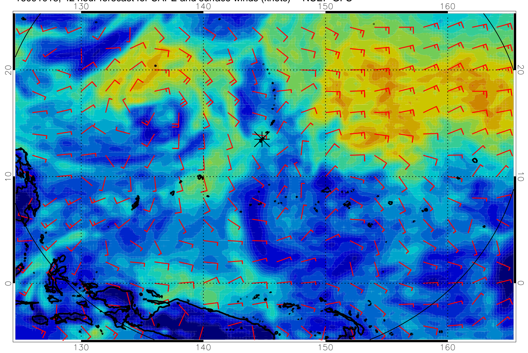
16091018, 42 hour forecast for CAPE and surface winds (knots) -- NCEP GFS
