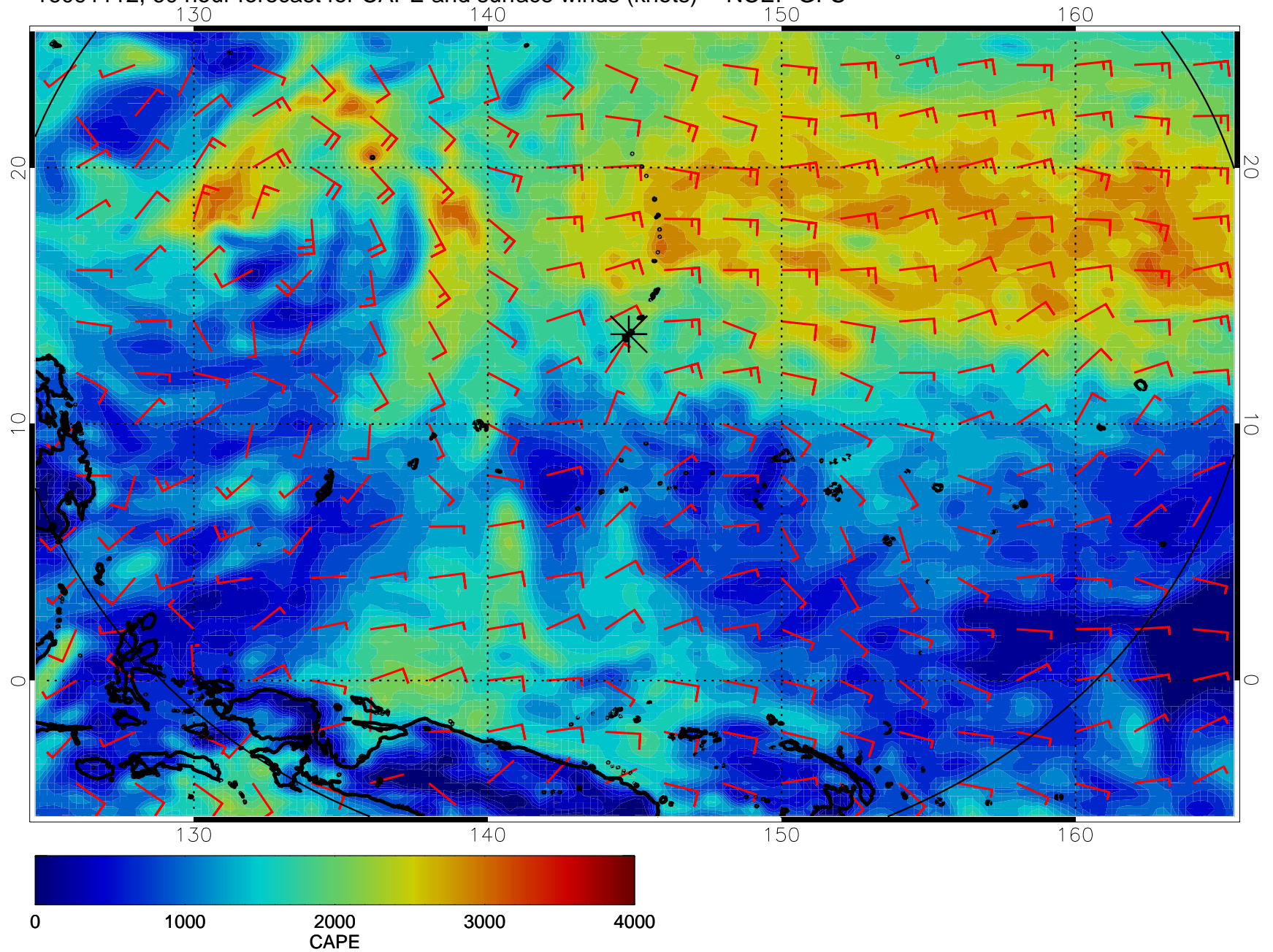
16091112, 60 hour forecast for CAPE and surface winds (knots) -- NCEP GFS
