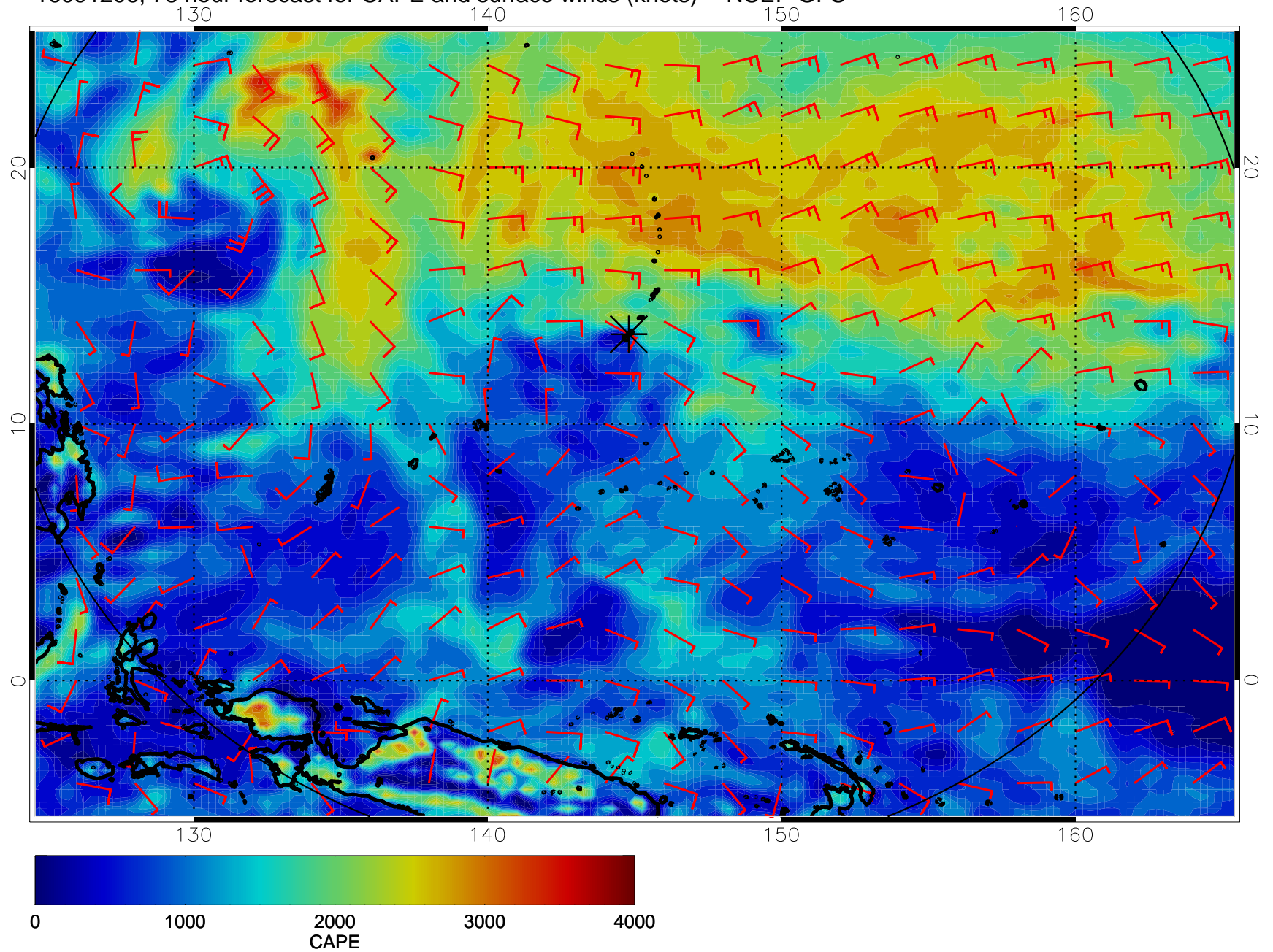
16091206, 78 hour forecast for CAPE and surface winds (knots) -- NCEP GFS
