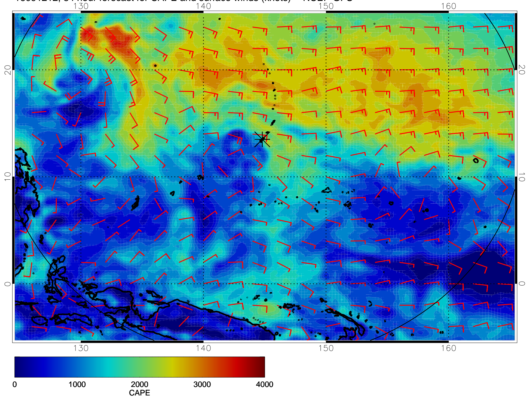
16091212, 84 hour forecast for CAPE and surface winds (knots) -- NCEP GFS
