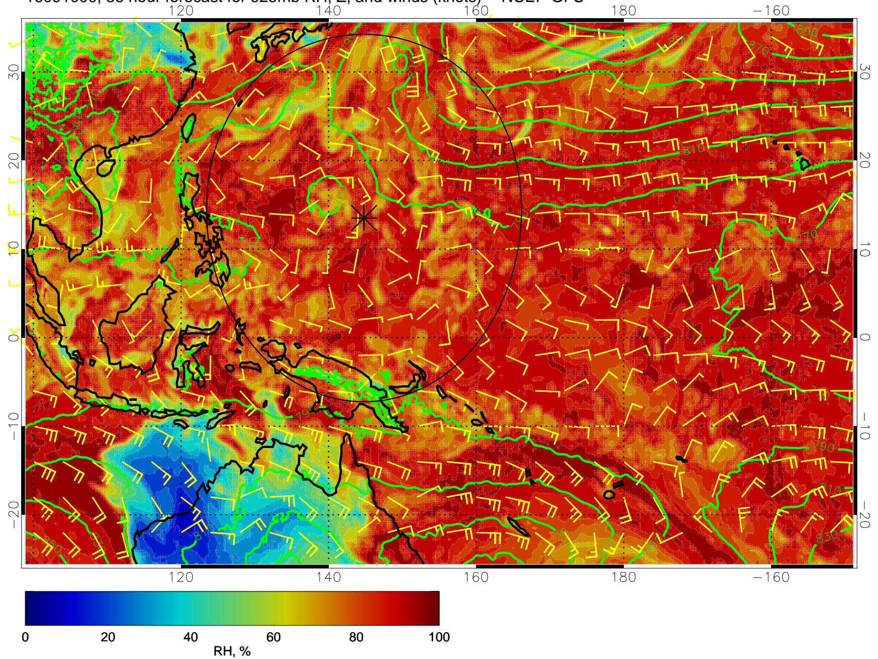
16091000, 36 hour forecast for 925mb RH, Z, and winds (knots) -- NCEP GFS
