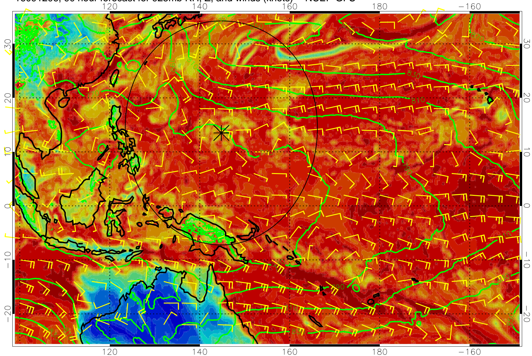
16091206, 90 hour forecast for 925mb RH, Z, and winds (knots) -- NCEP GFS
