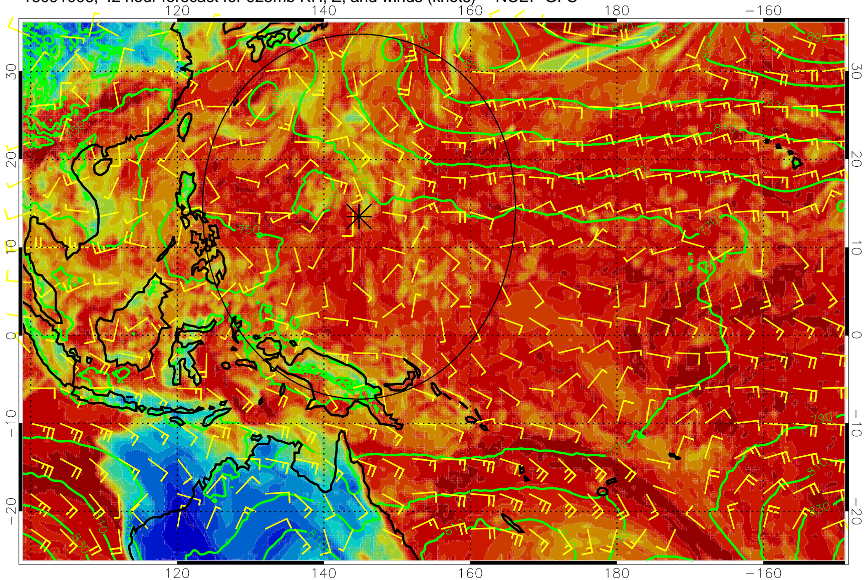
16091006, 42 hour forecast for 925mb RH, Z, and winds (knots) -- NCEP GFS
