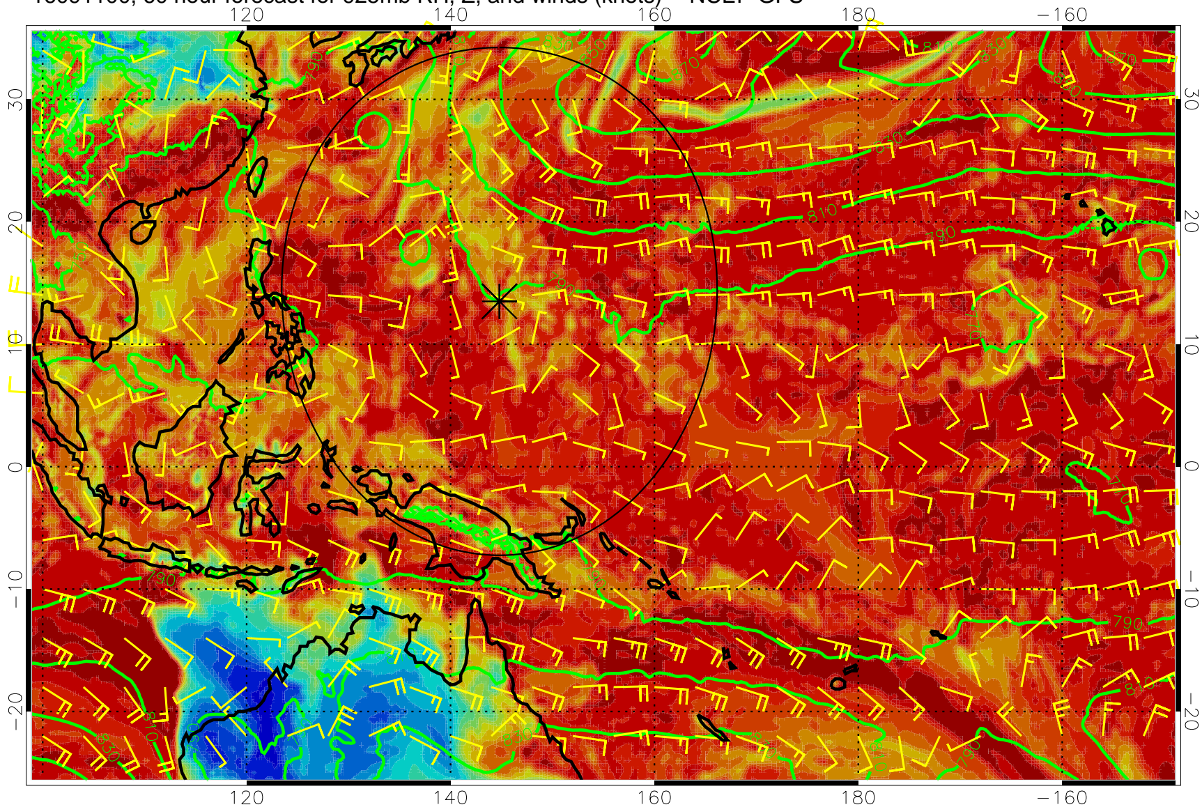
16091100, 60 hour forecast for 925mb RH, Z, and winds (knots) -- NCEP GFS
