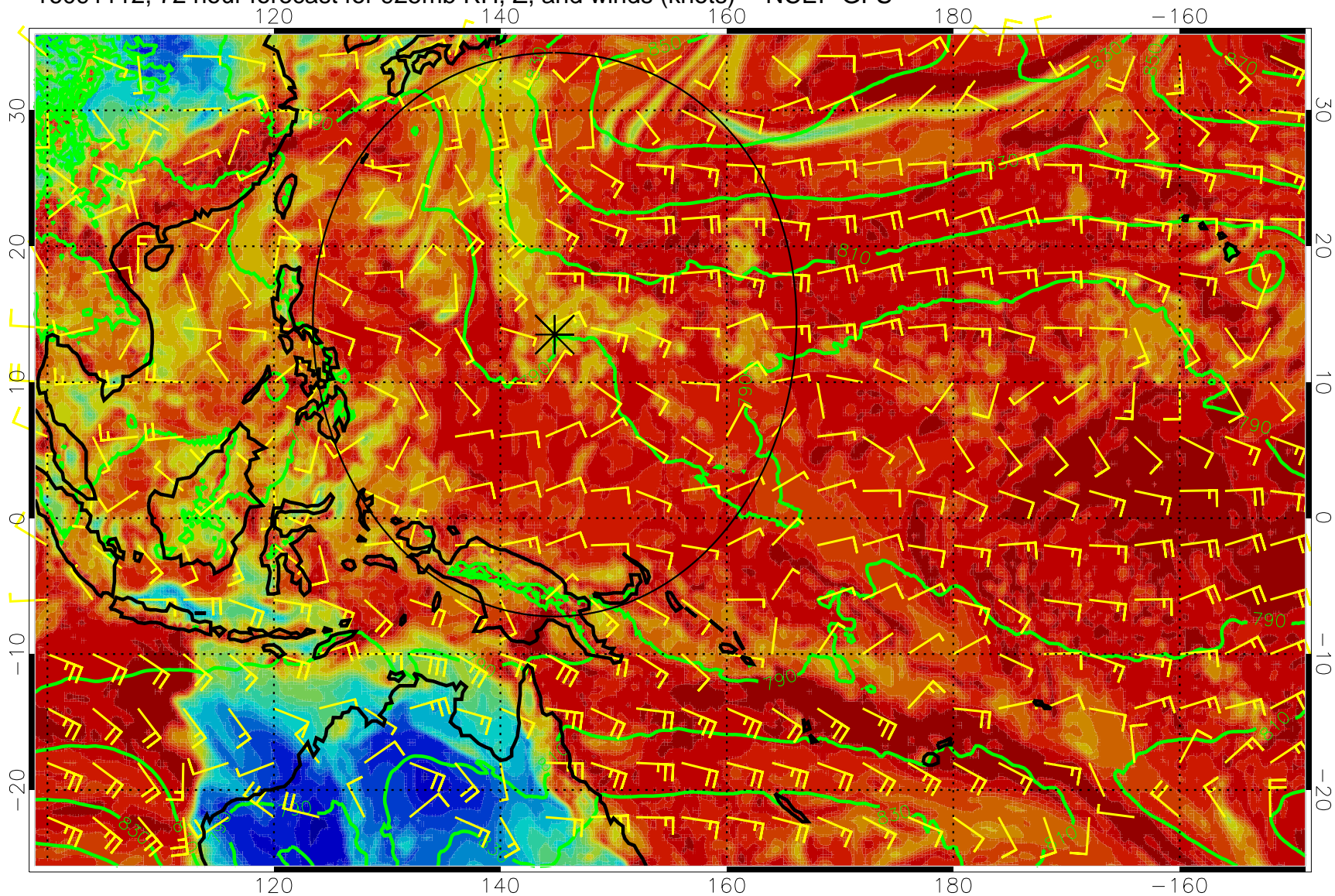
16091112, 72 hour forecast for 925mb RH, Z, and winds (knots) -- NCEP GFS
