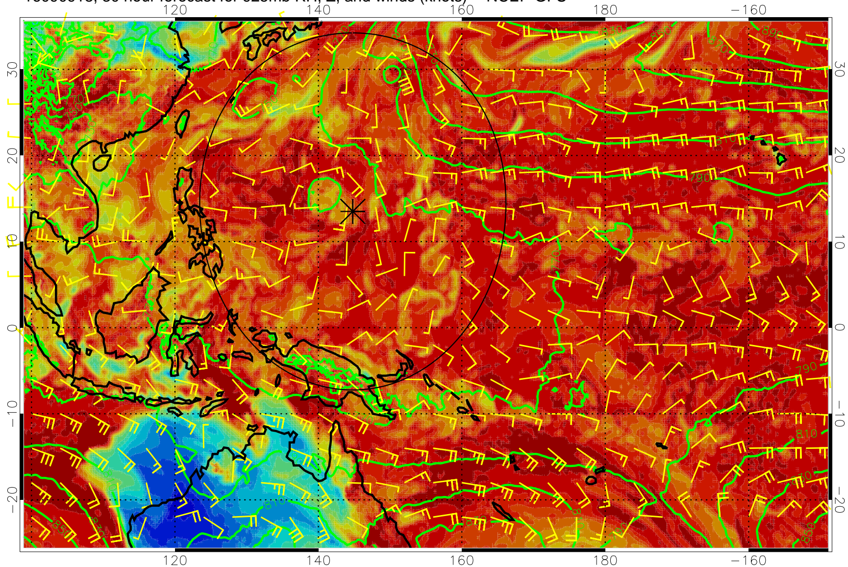
16090918, 30 hour forecast for 925mb RH, Z, and winds (knots) -- NCEP GFS
