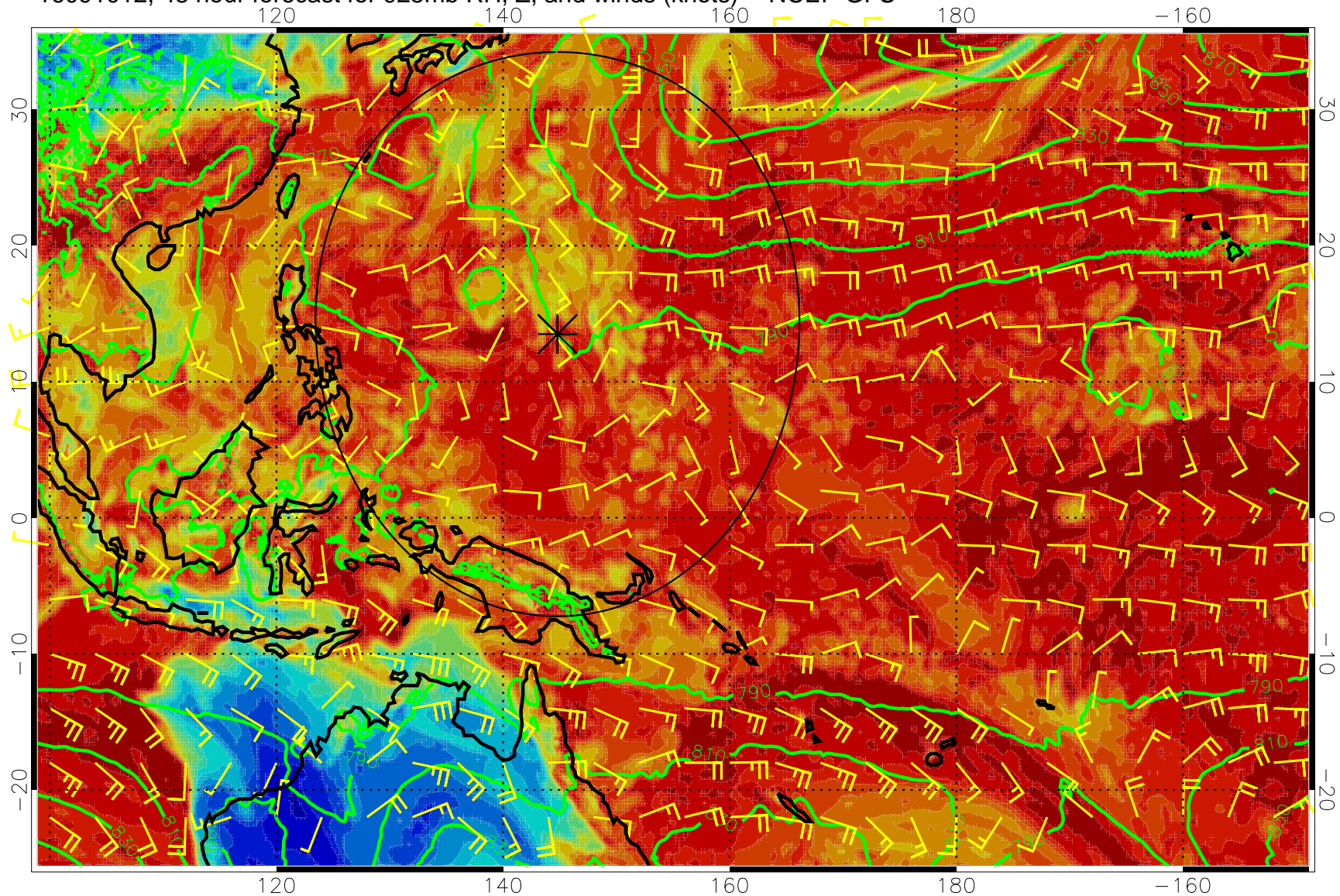
16091012, 48 hour forecast for 925mb RH, Z, and winds (knots) -- NCEP GFS
