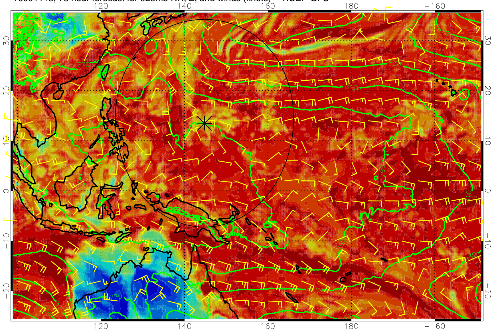
16091118, 78 hour forecast for 925mb RH, Z, and winds (knots) -- NCEP GFS
