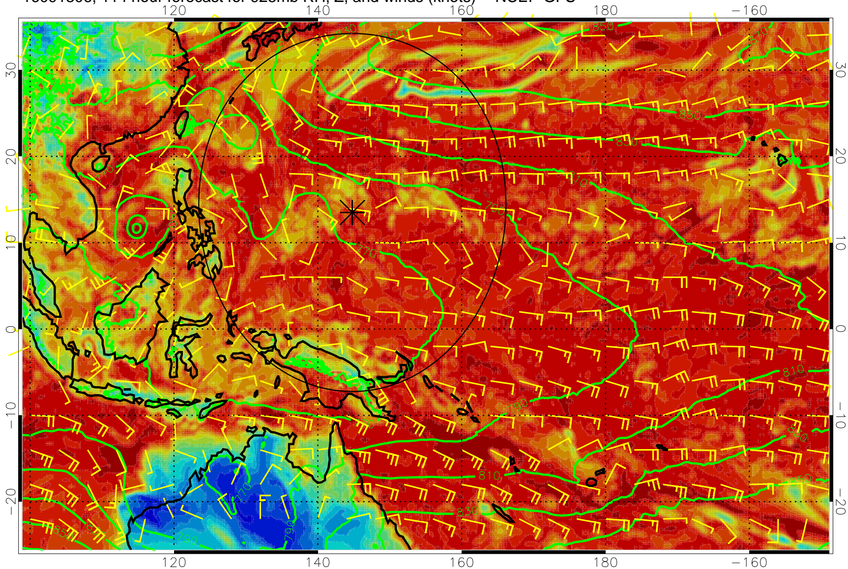
16091306, 114 hour forecast for 925mb RH, Z, and winds (knots) -- NCEP GFS
