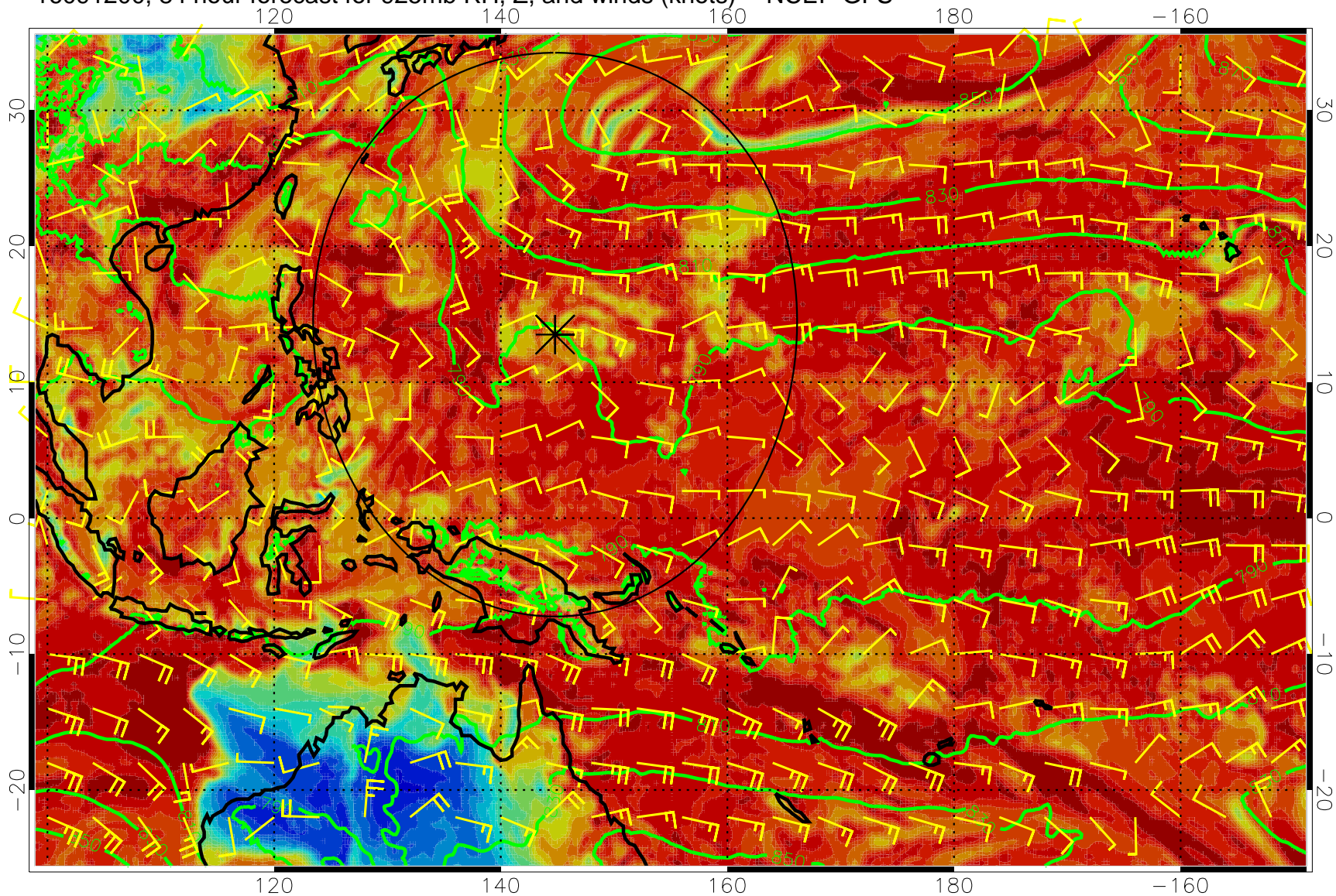
16091200, 84 hour forecast for 925mb RH, Z, and winds (knots) -- NCEP GFS
