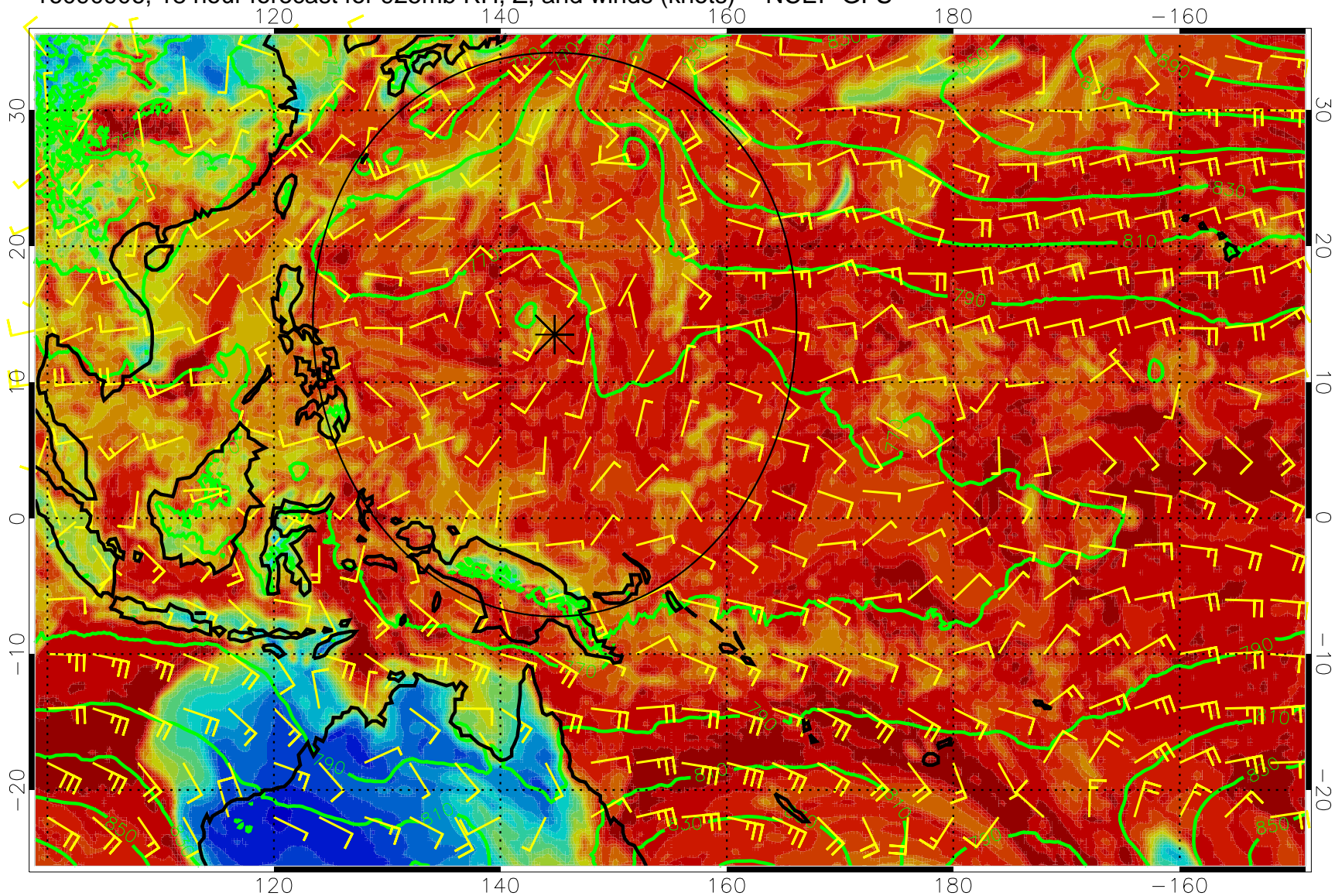
16090906, 18 hour forecast for 925mb RH, Z, and winds (knots) -- NCEP GFS
