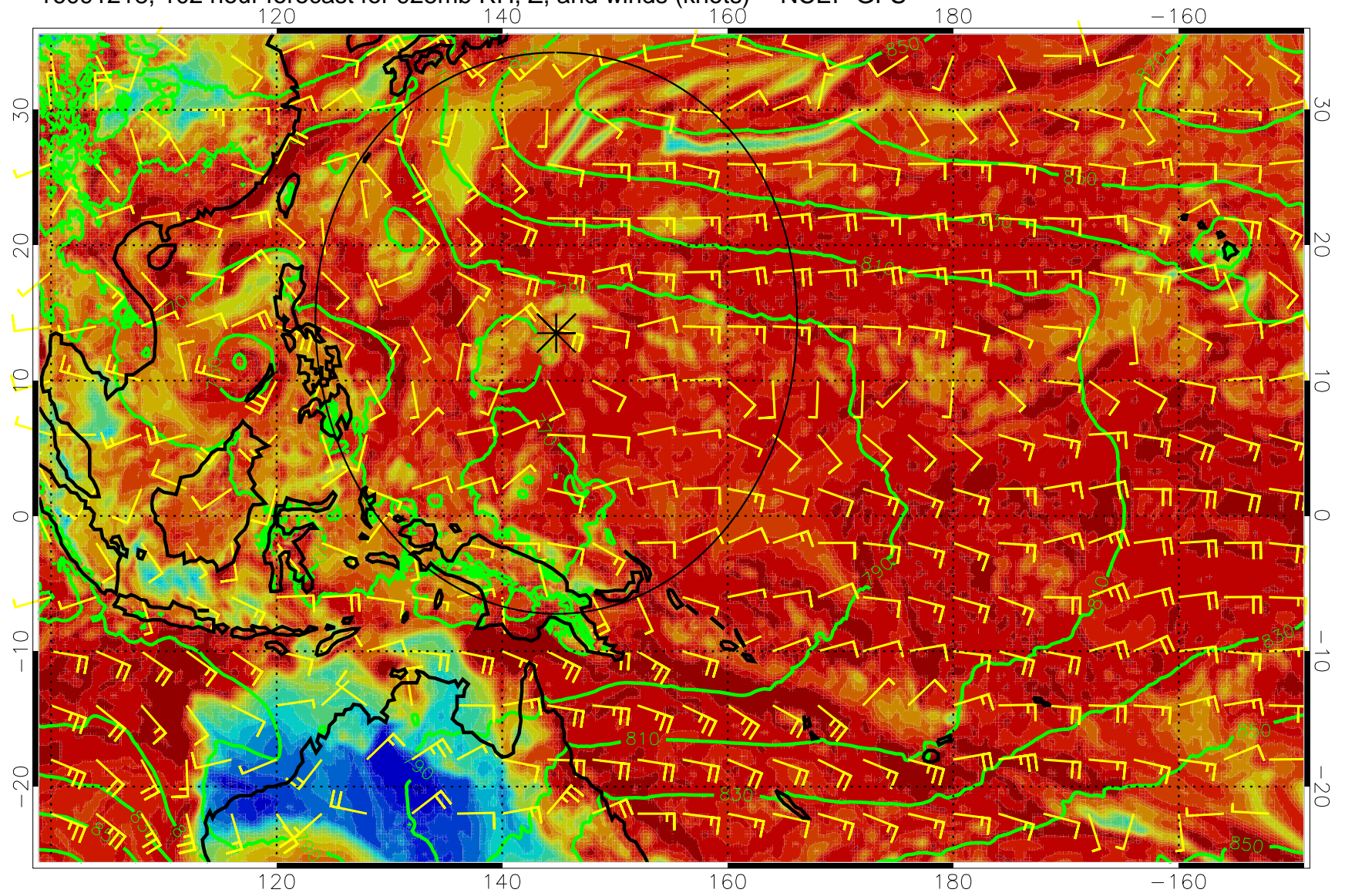
16091218, 102 hour forecast for 925mb RH, Z, and winds (knots) -- NCEP GFS
