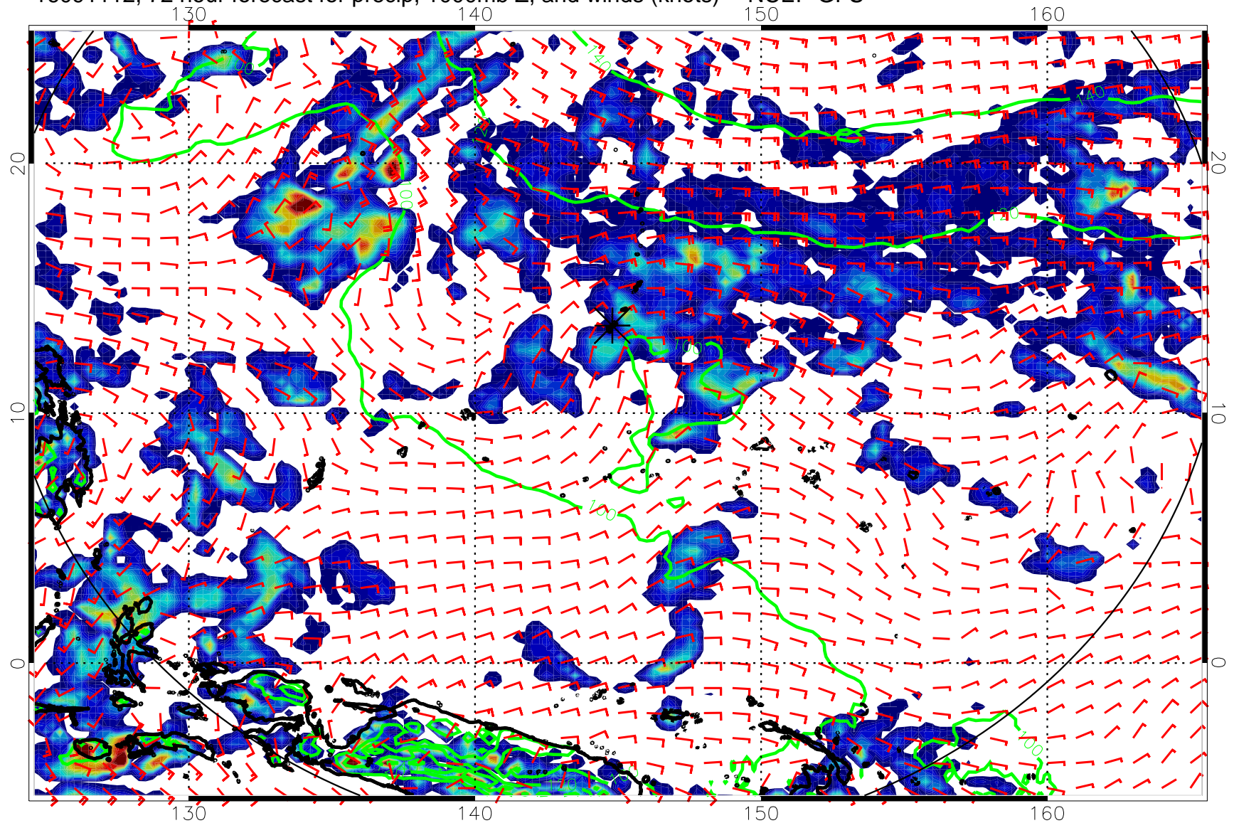
16091112, 72 hour forecast for precip, 1000mb Z, and winds (knots) -- NCEP GFS
