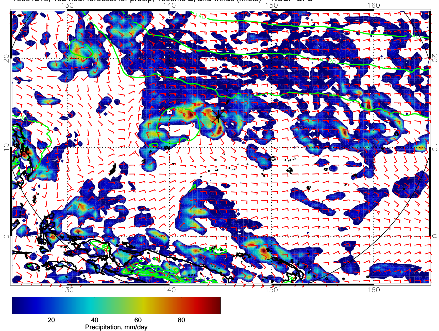
16091218, 102 hour forecast for precip, 1000mb Z, and winds (knots) -- NCEP GFS
