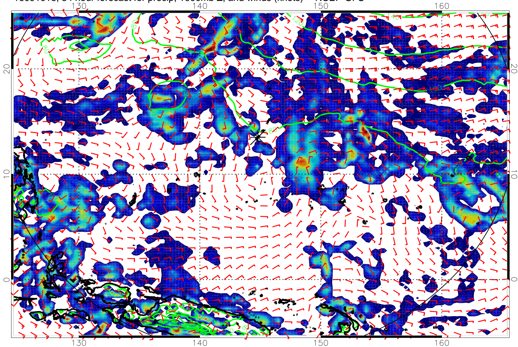
16091018, 54 hour forecast for precip, 1000mb Z, and winds (knots) -- NCEP GFS
