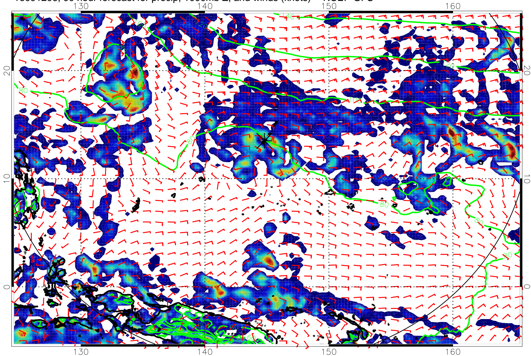
16091206, 90 hour forecast for precip, 1000mb Z, and winds (knots) -- NCEP GFS
