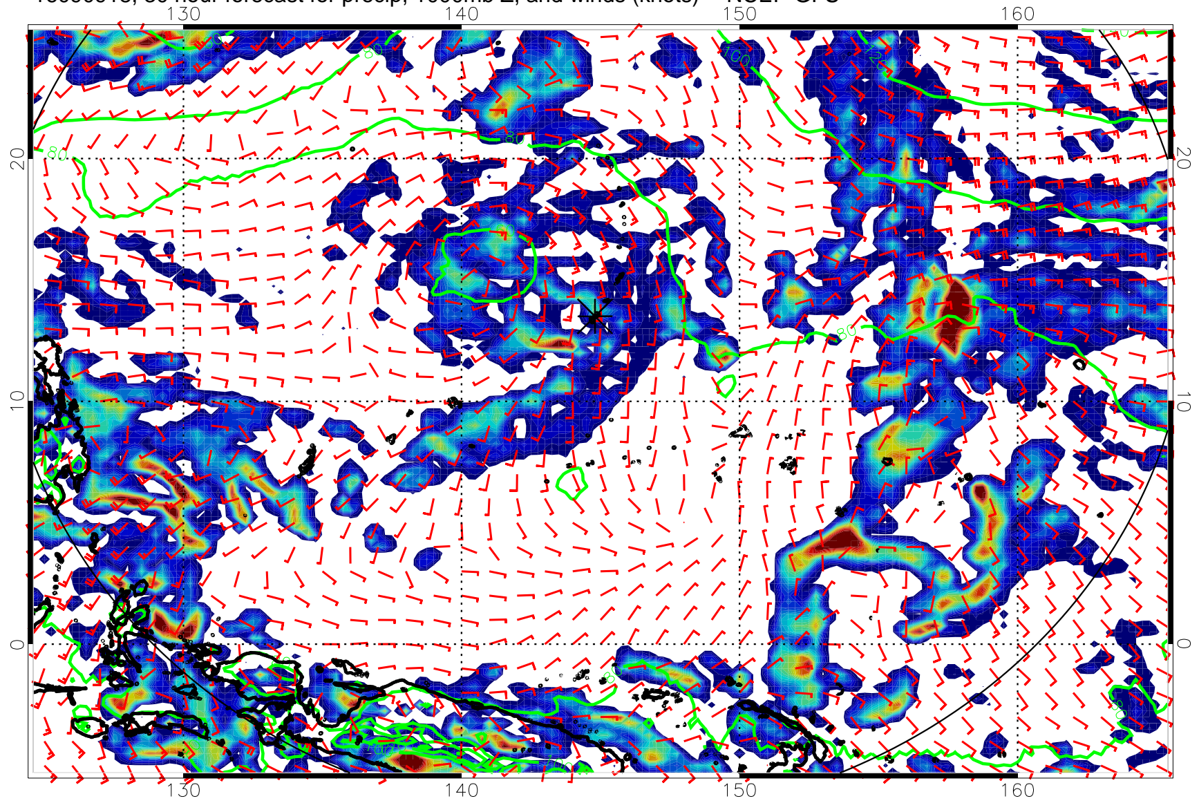
16090918, 30 hour forecast for precip, 1000mb Z, and winds (knots) -- NCEP GFS
