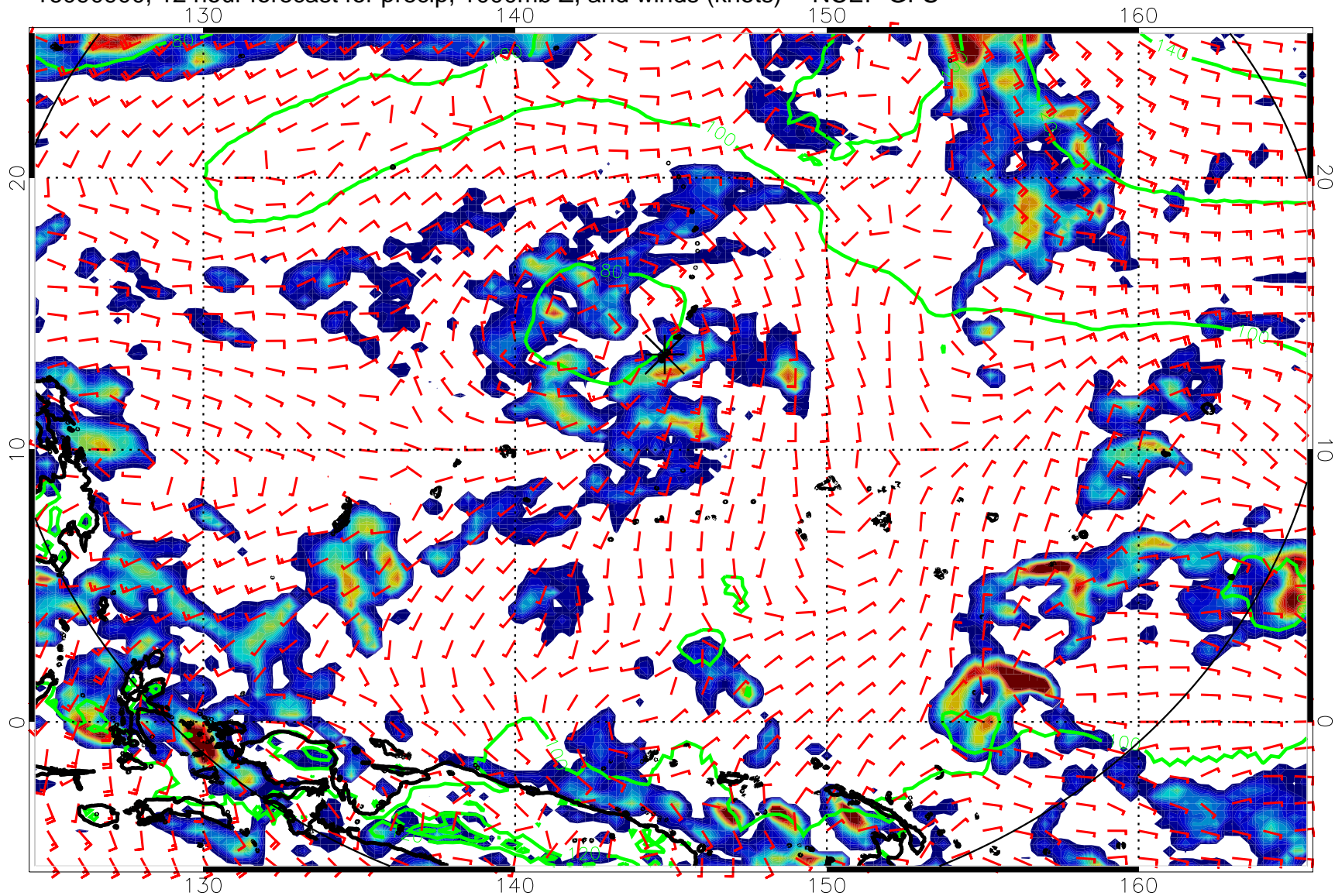
16090900, 12 hour forecast for precip, 1000mb Z, and winds (knots) -- NCEP GFS
