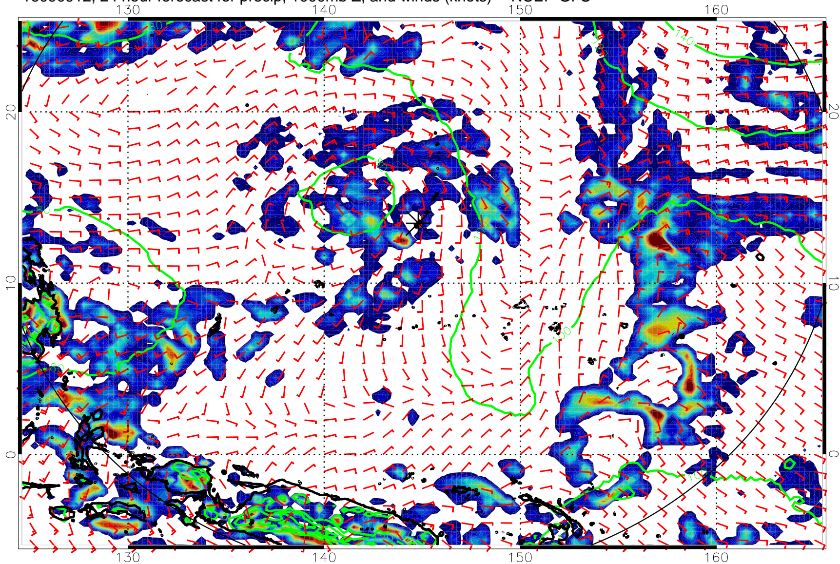
16090912, 24 hour forecast for precip, 1000mb Z, and winds (knots) -- NCEP GFS
