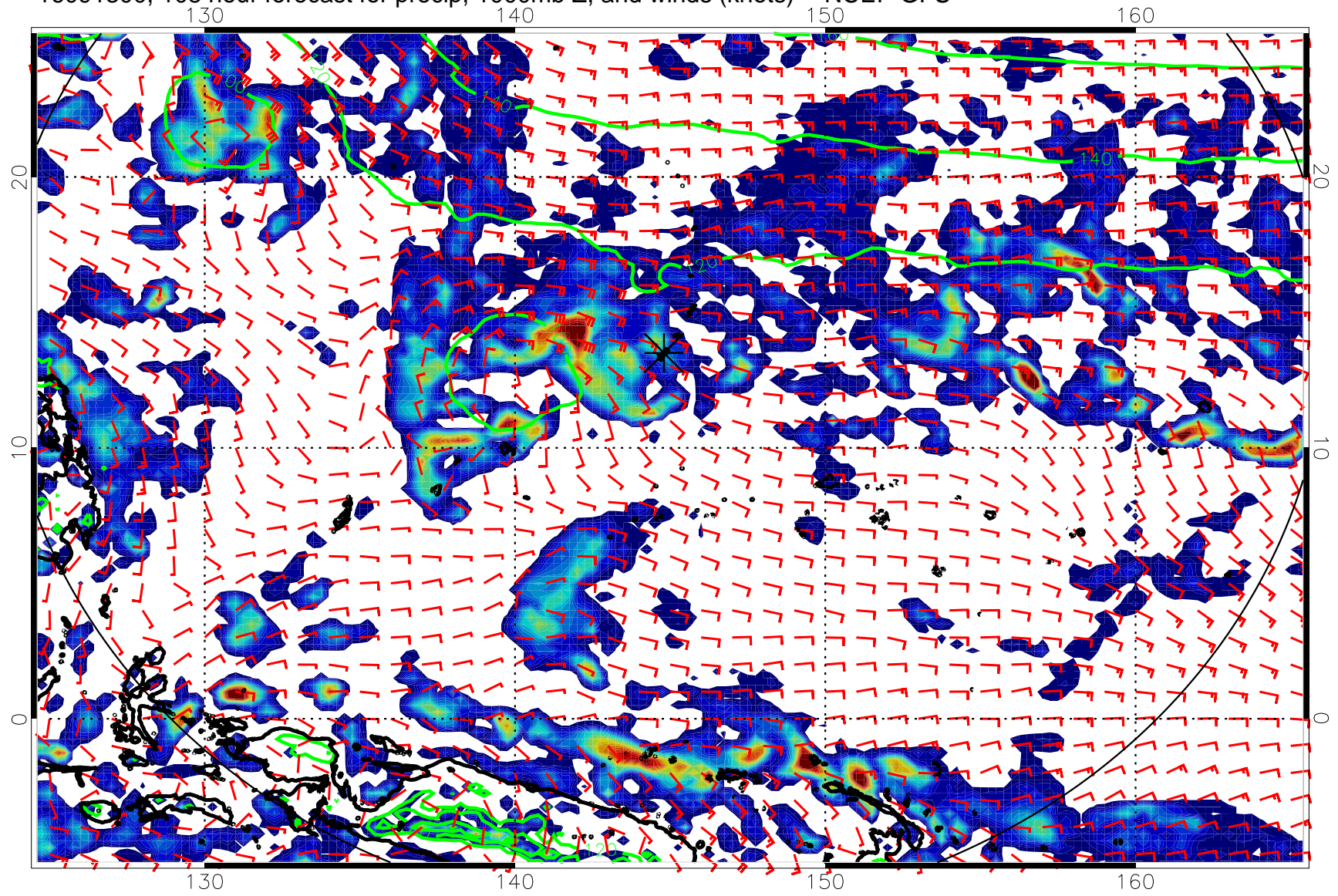
16091300, 108 hour forecast for precip, 1000mb Z, and winds (knots) -- NCEP GFS
