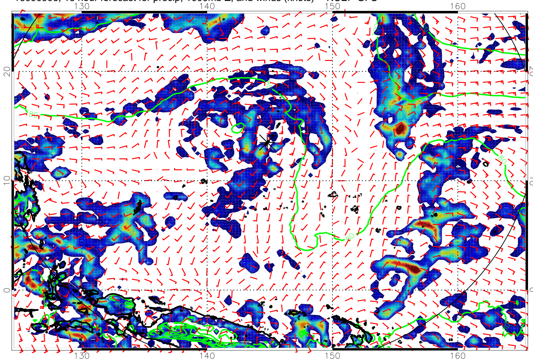
16090906, 18 hour forecast for precip, 1000mb Z, and winds (knots) -- NCEP GFS
