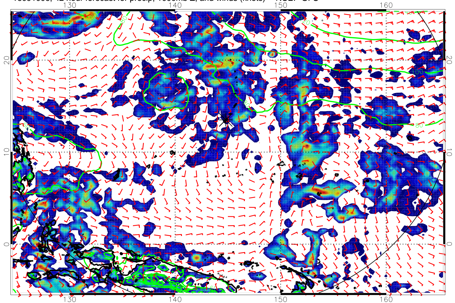
16091006, 42 hour forecast for precip, 1000mb Z, and winds (knots) -- NCEP GFS
