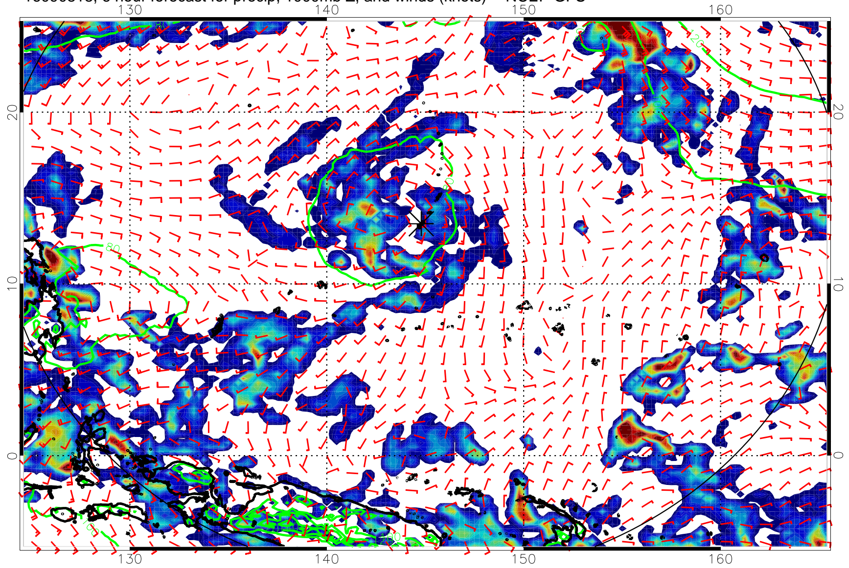
16090818, 6 hour forecast for precip, 1000mb Z, and winds (knots) -- NCEP GFS
