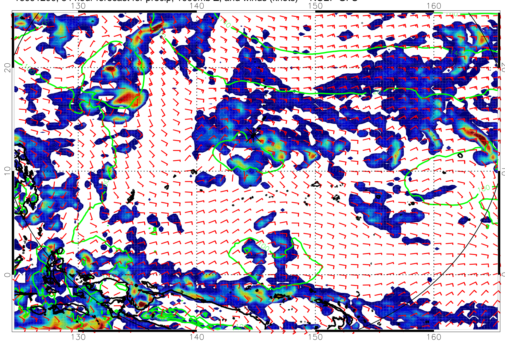
16091200, 84 hour forecast for precip, 1000mb Z, and winds (knots) -- NCEP GFS
