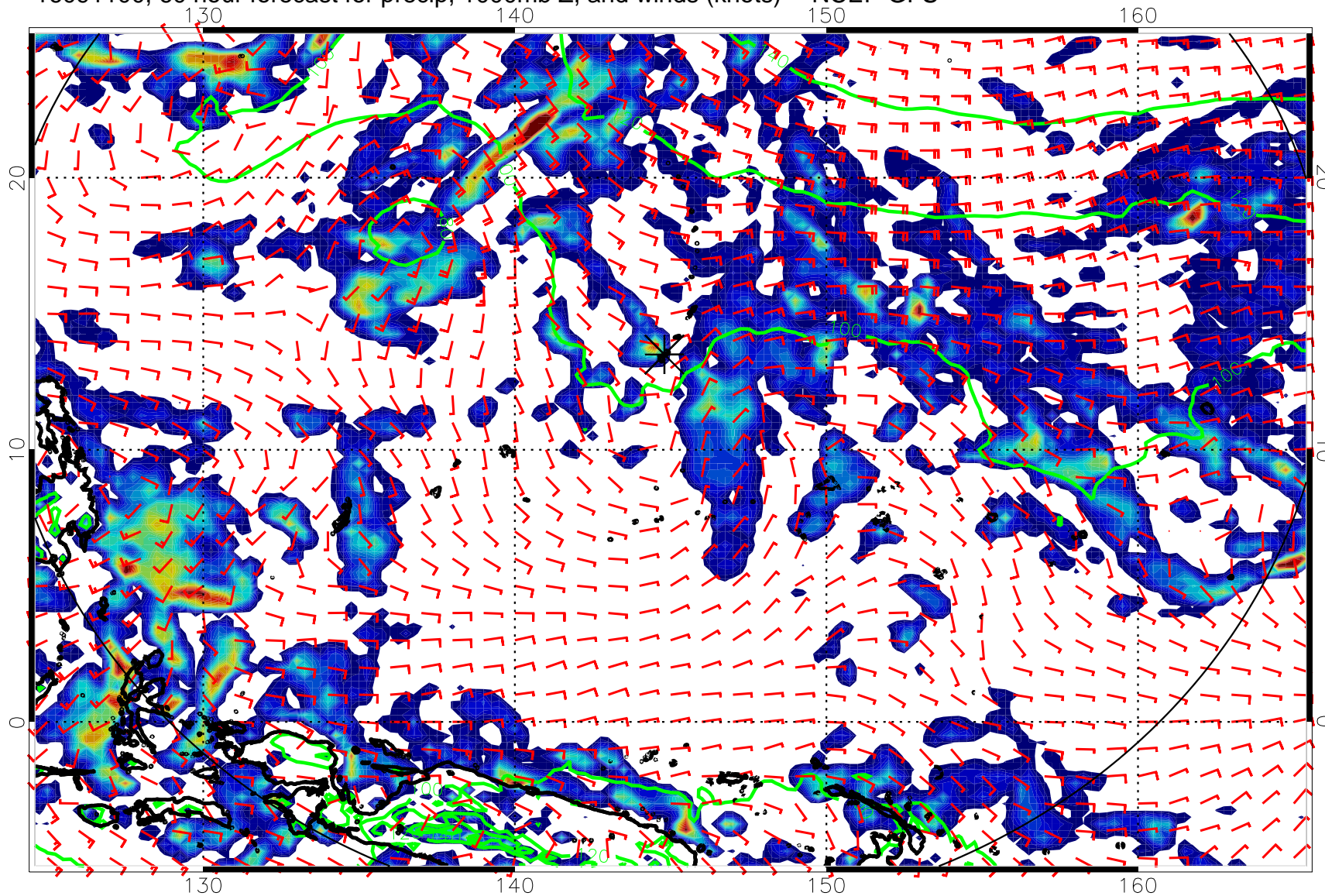
16091100, 60 hour forecast for precip, 1000mb Z, and winds (knots) -- NCEP GFS
