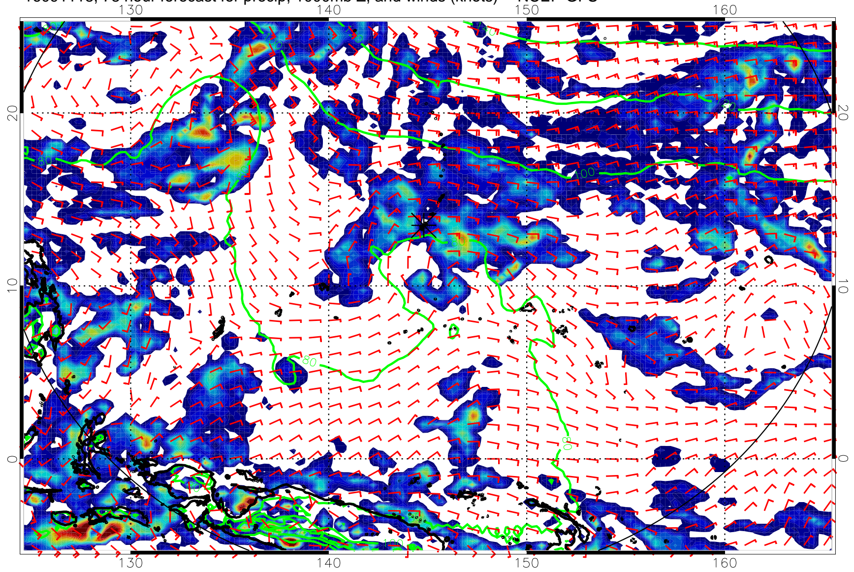
16091118, 78 hour forecast for precip, 1000mb Z, and winds (knots) -- NCEP GFS
