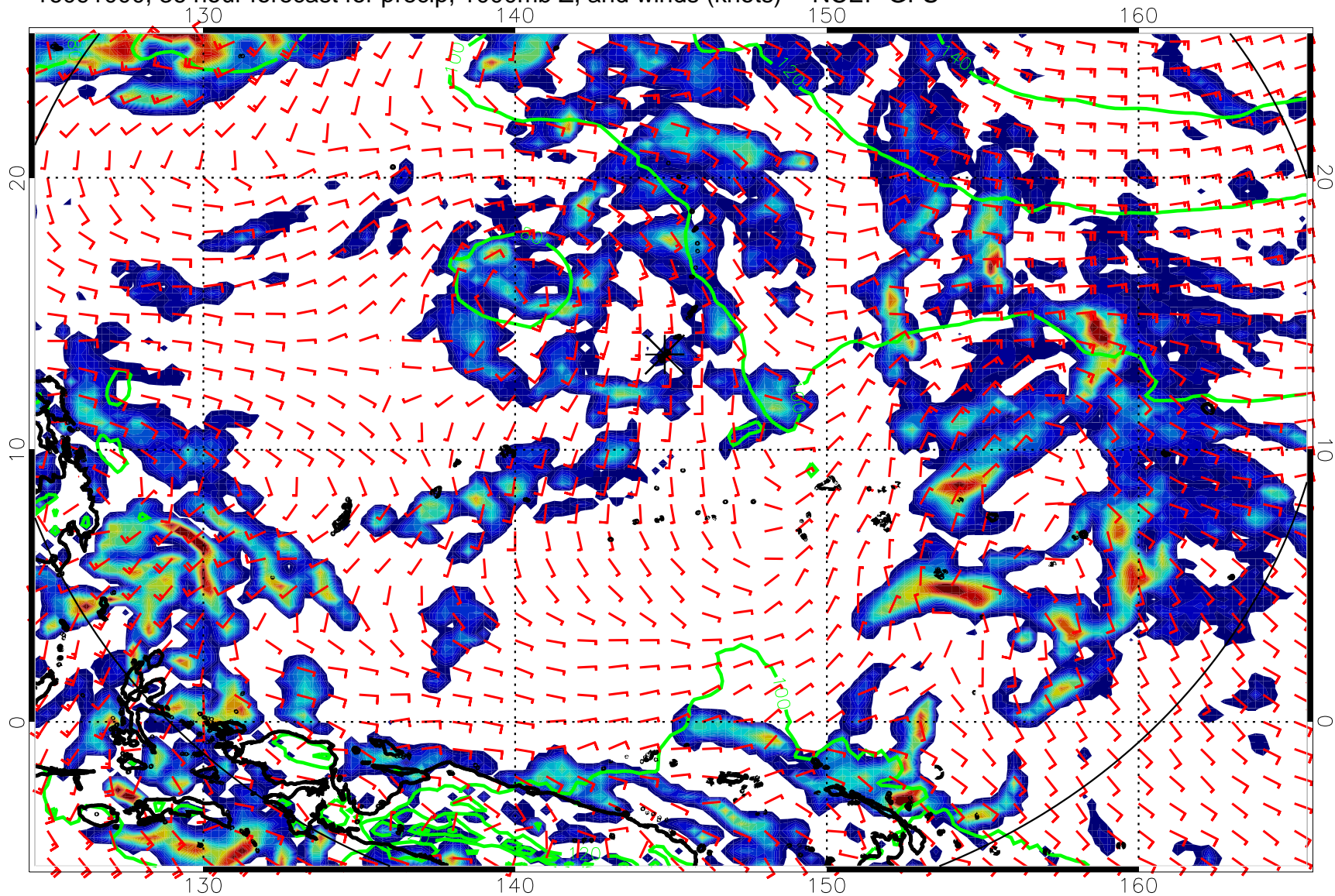
16091000, 36 hour forecast for precip, 1000mb Z, and winds (knots) -- NCEP GFS
