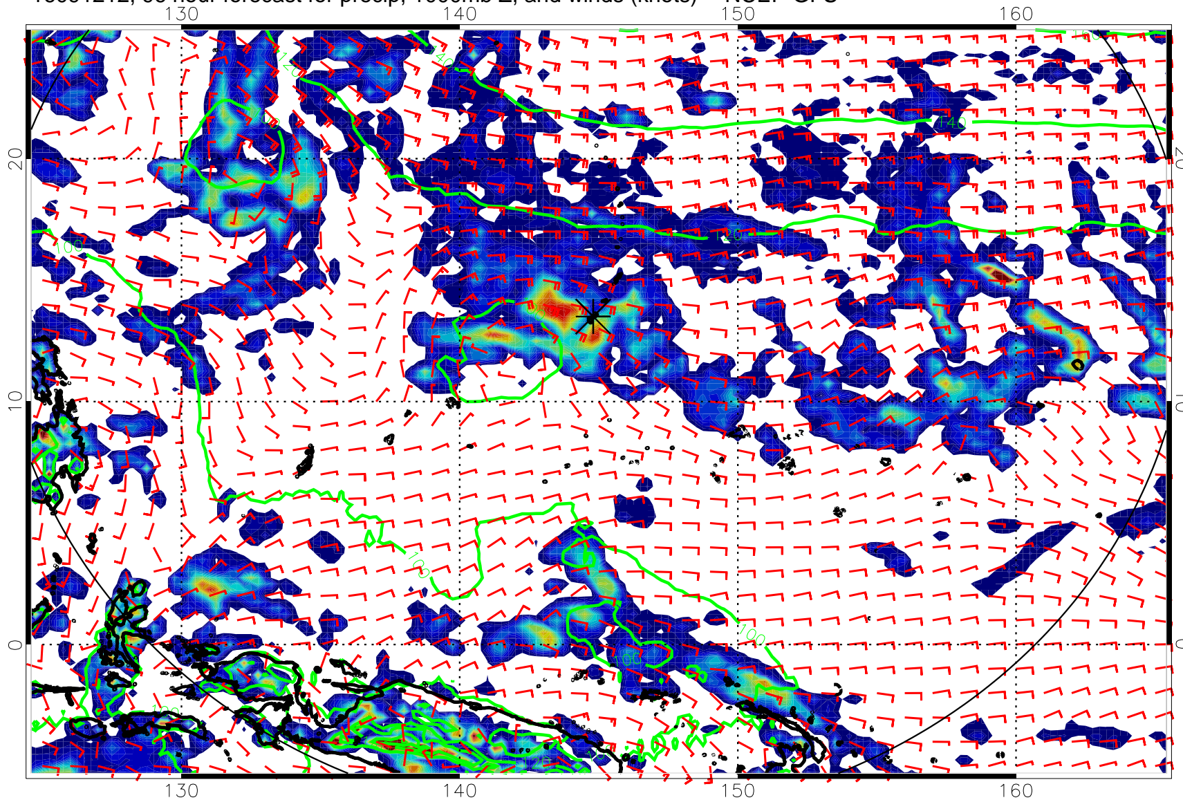
16091212, 96 hour forecast for precip, 1000mb Z, and winds (knots) -- NCEP GFS
