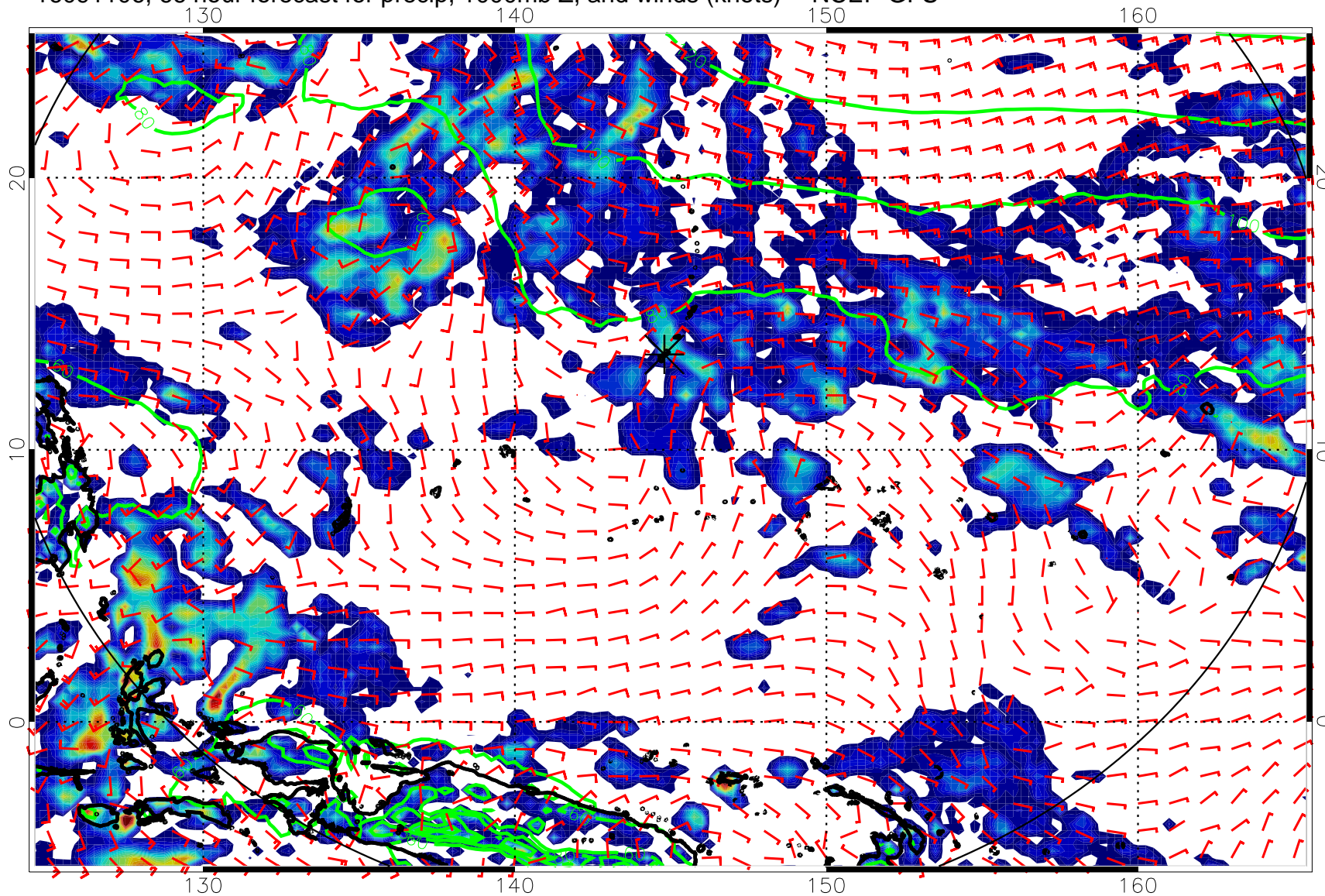
16091106, 66 hour forecast for precip, 1000mb Z, and winds (knots) -- NCEP GFS
