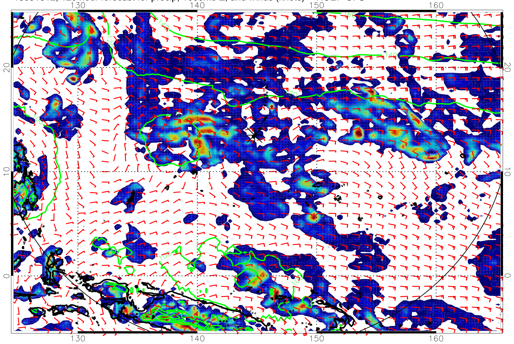
16091312, 120 hour forecast for precip, 1000mb Z, and winds (knots) -- NCEP GFS
