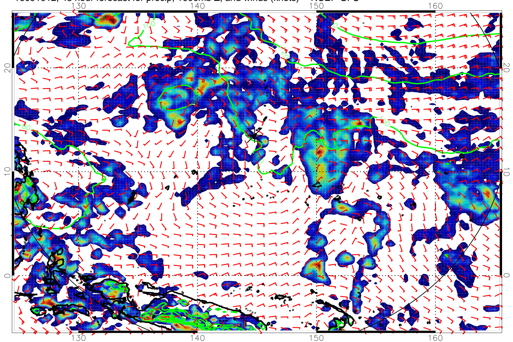
16091012, 48 hour forecast for precip, 1000mb Z, and winds (knots) -- NCEP GFS
