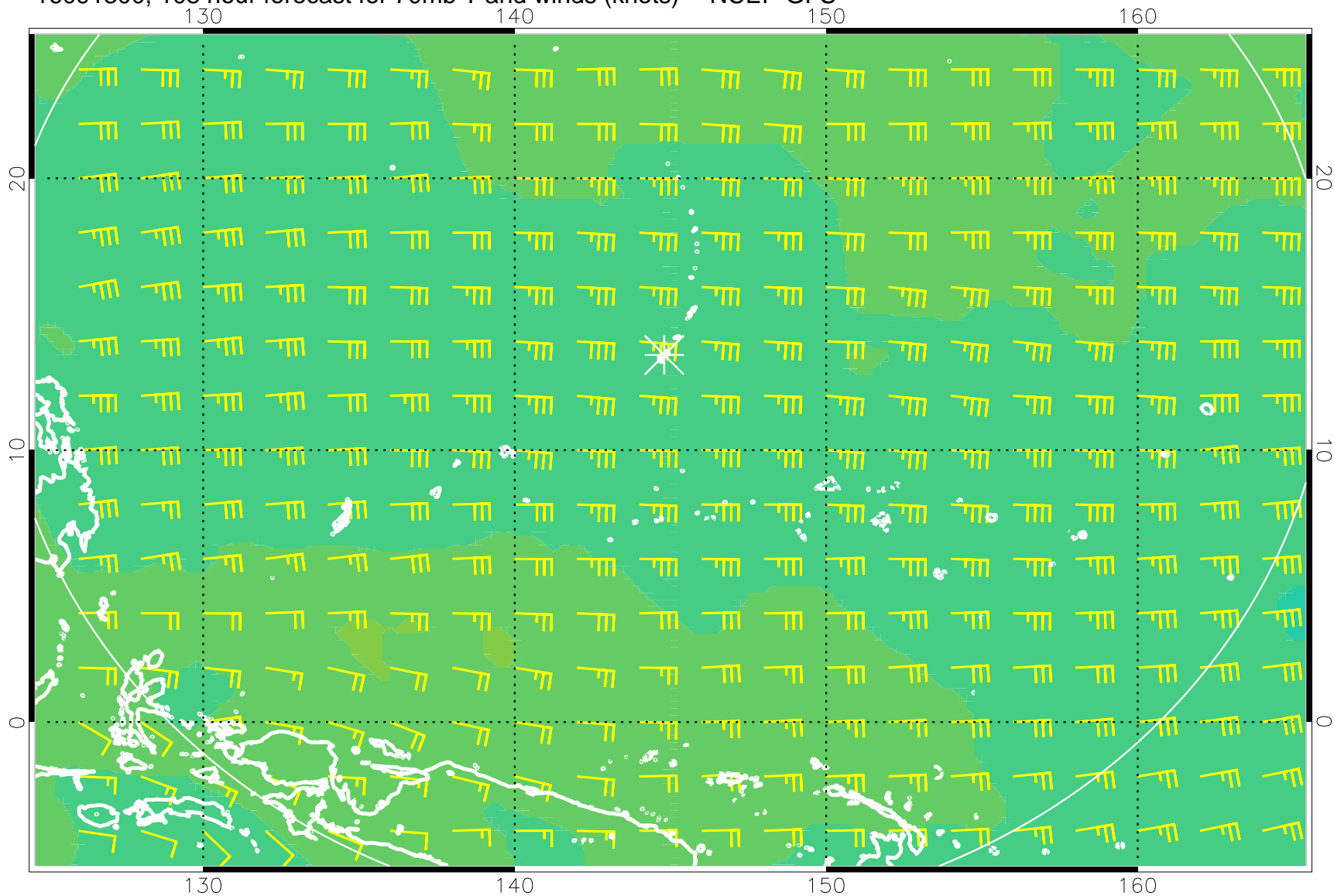
16091300, 108 hour forecast for 70mb T and winds (knots) -- NCEP GFS
