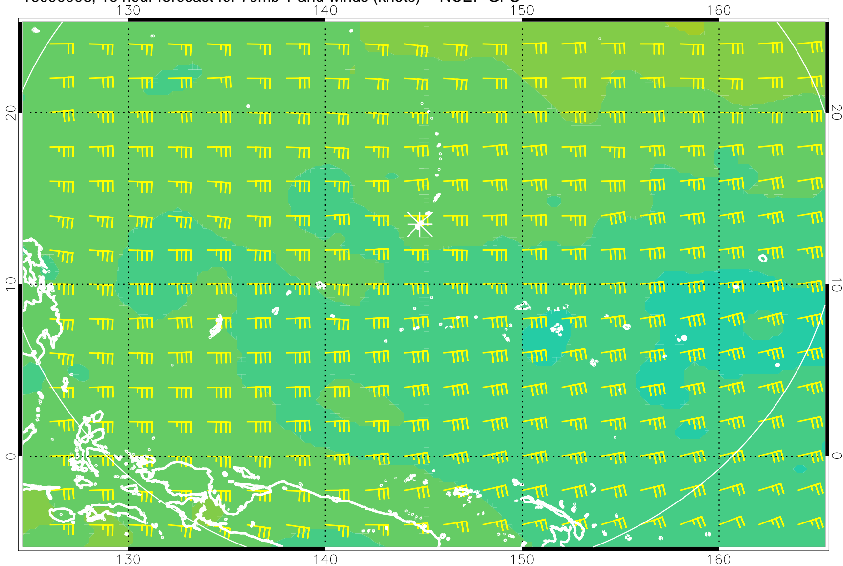
16090906, 18 hour forecast for 70mb T and winds (knots) -- NCEP GFS
