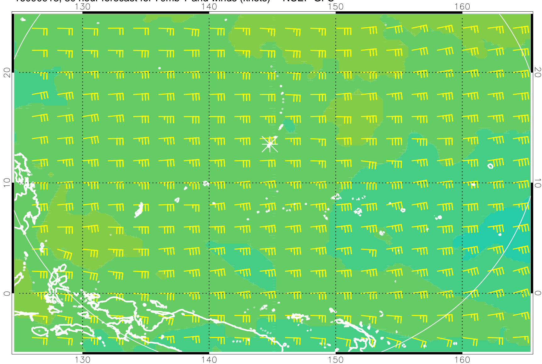
16090918, 30 hour forecast for 70mb T and winds (knots) -- NCEP GFS
