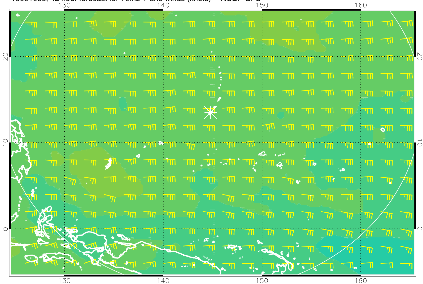
16091006, 42 hour forecast for 70mb T and winds (knots) -- NCEP GFS
