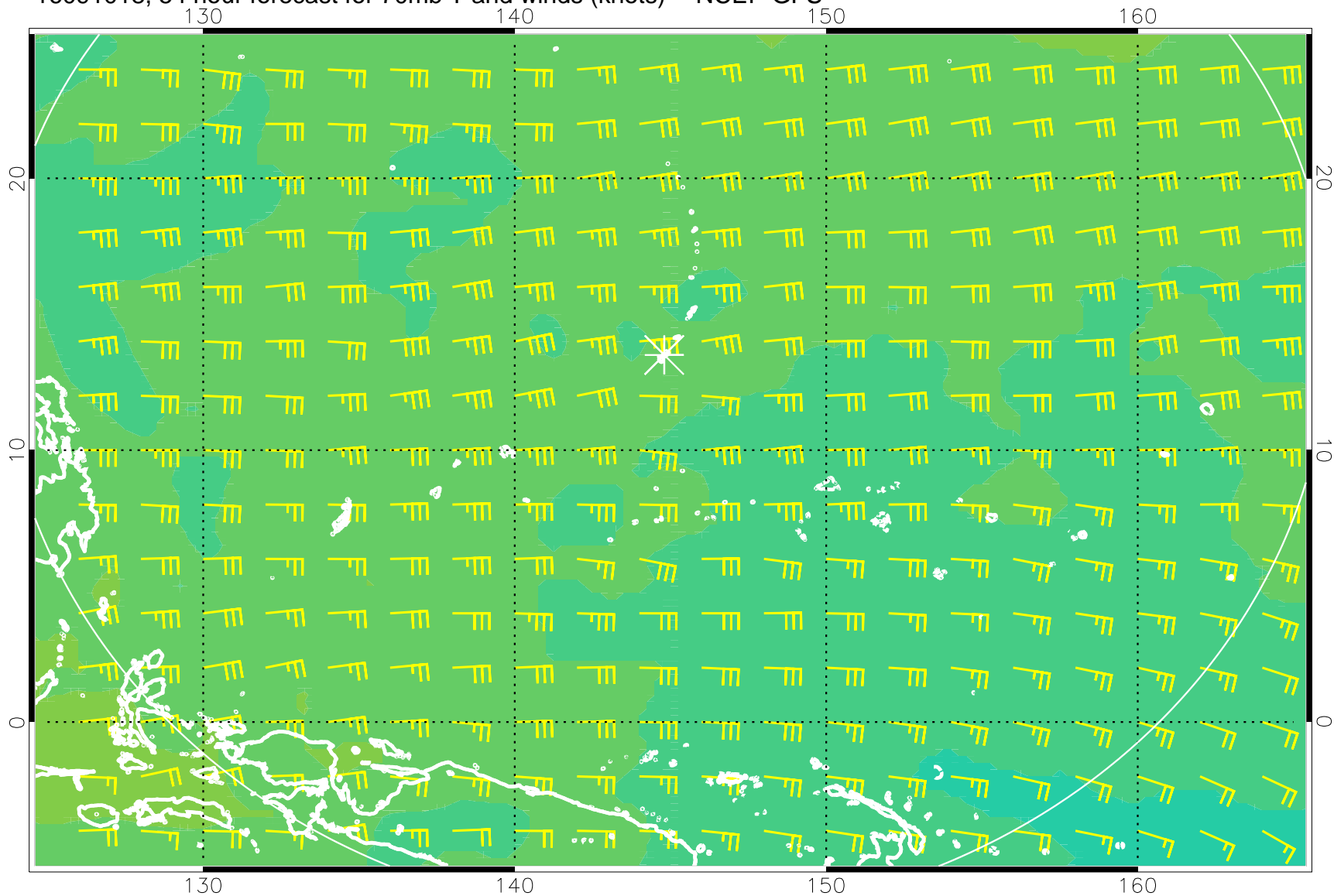
16091018, 54 hour forecast for 70mb T and winds (knots) -- NCEP GFS
