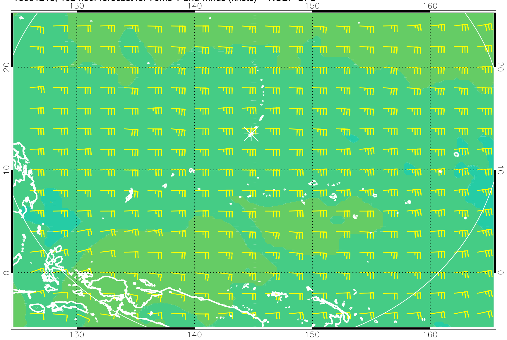
16091218, 102 hour forecast for 70mb T and winds (knots) -- NCEP GFS
