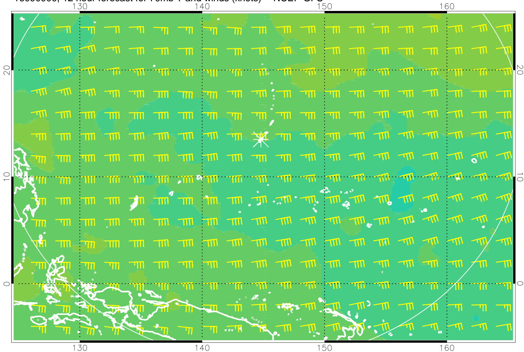
16090900, 12 hour forecast for 70mb T and winds (knots) -- NCEP GFS
