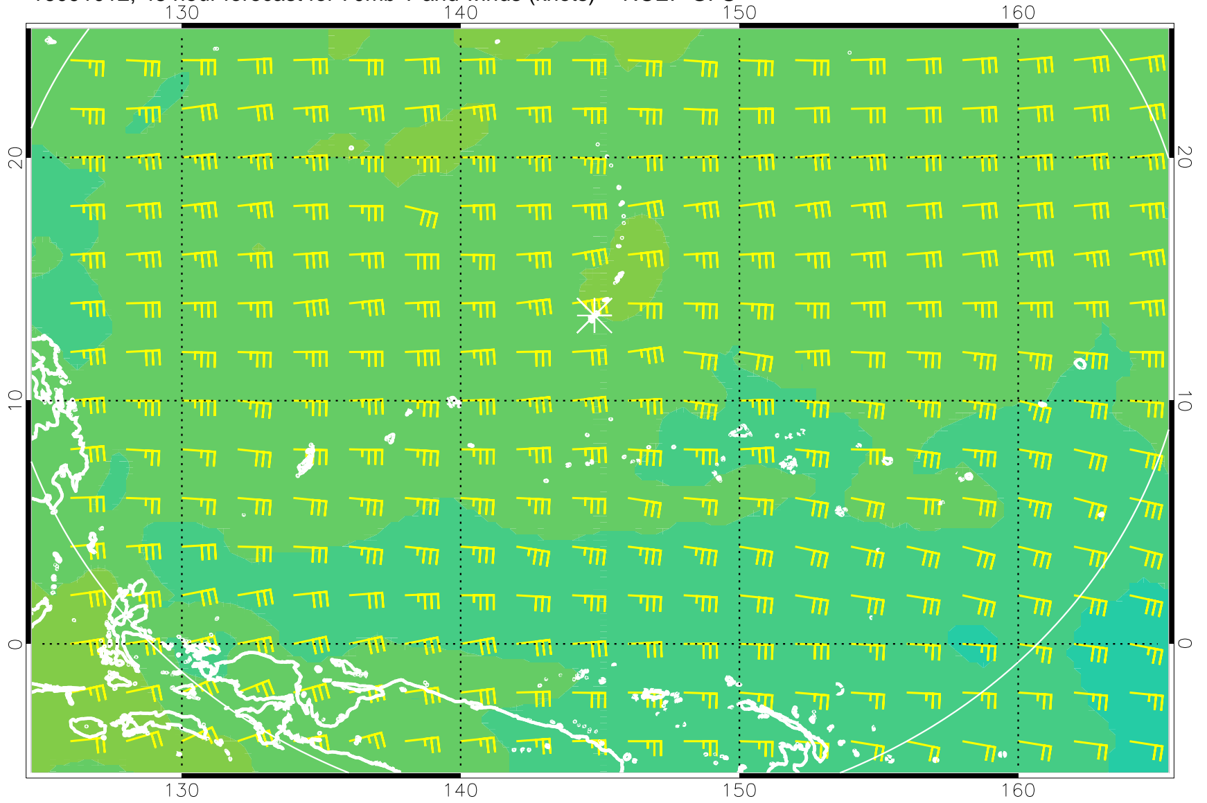
16091012, 48 hour forecast for 70mb T and winds (knots) -- NCEP GFS
