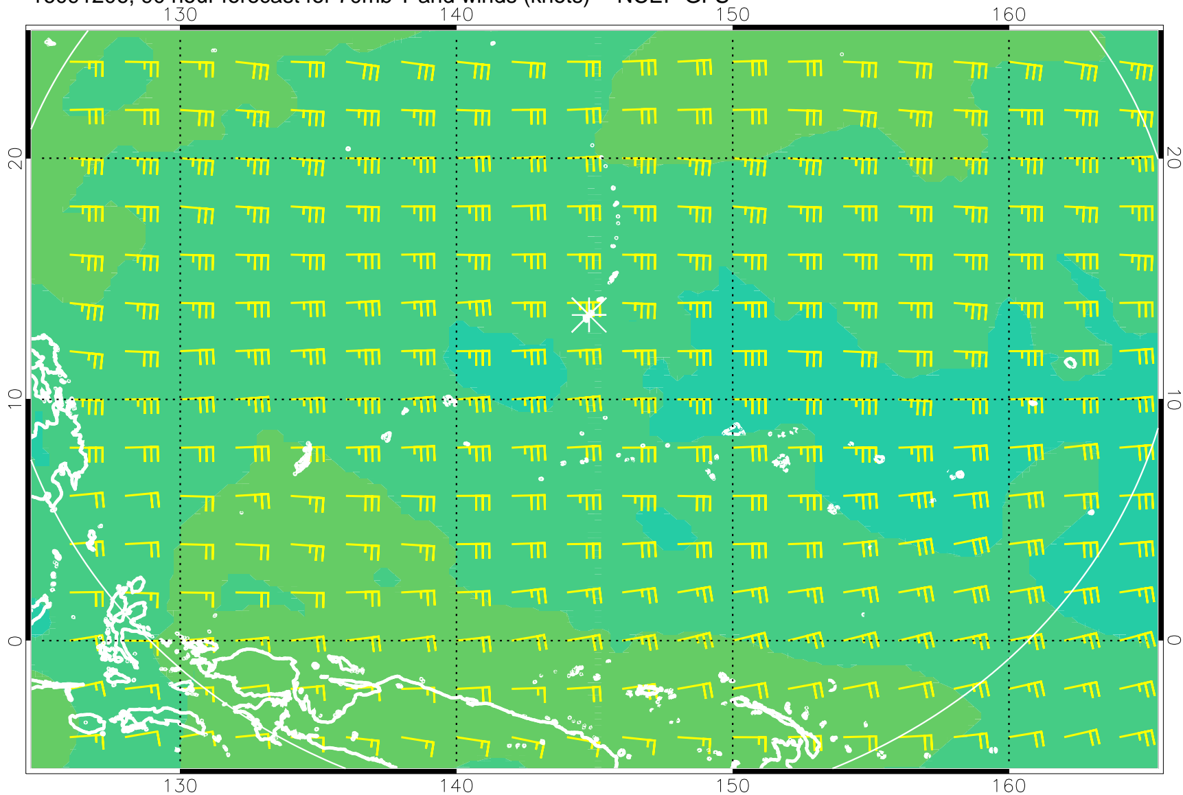
16091206, 90 hour forecast for 70mb T and winds (knots) -- NCEP GFS
