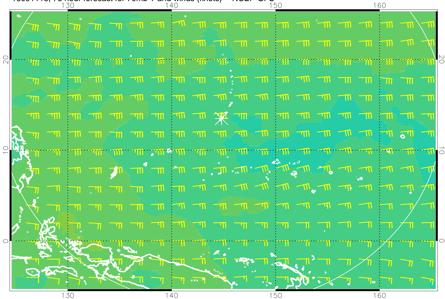
16091118, 78 hour forecast for 70mb T and winds (knots) -- NCEP GFS
