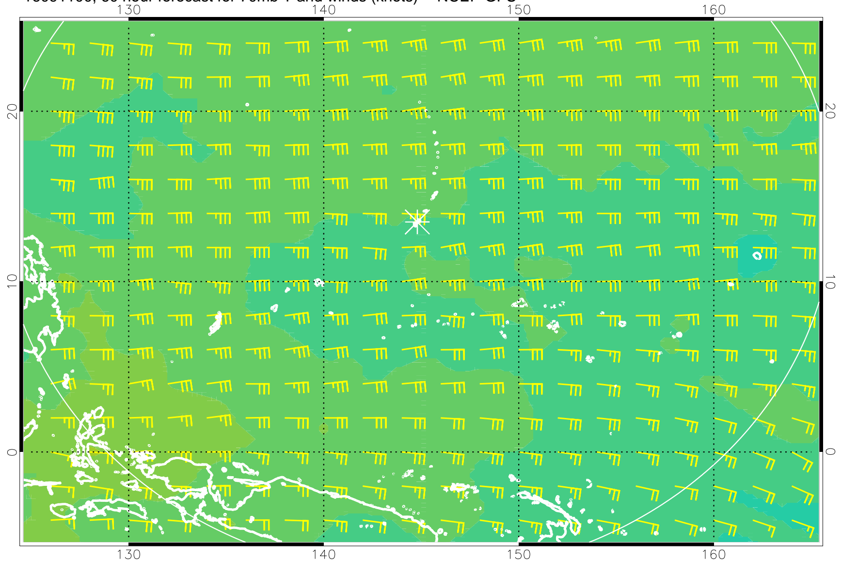
16091100, 60 hour forecast for 70mb T and winds (knots) -- NCEP GFS
