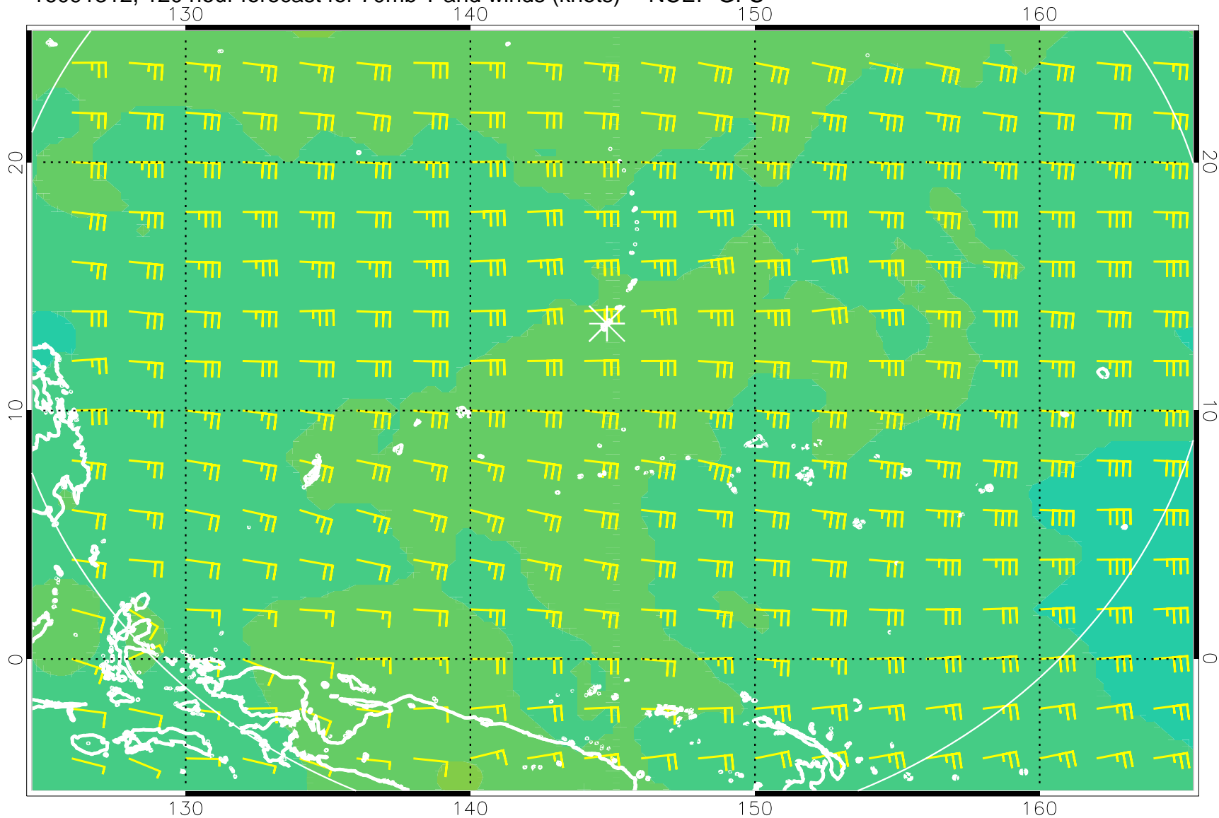
16091312, 120 hour forecast for 70mb T and winds (knots) -- NCEP GFS
