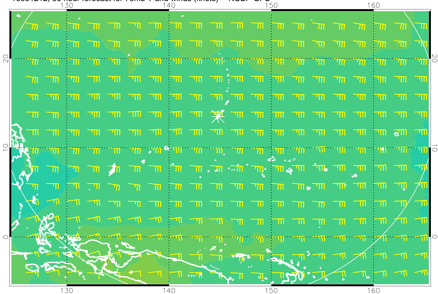
16091212, 96 hour forecast for 70mb T and winds (knots) -- NCEP GFS
