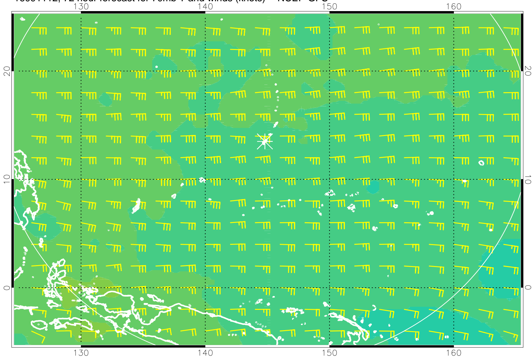
16091112, 72 hour forecast for 70mb T and winds (knots) -- NCEP GFS
