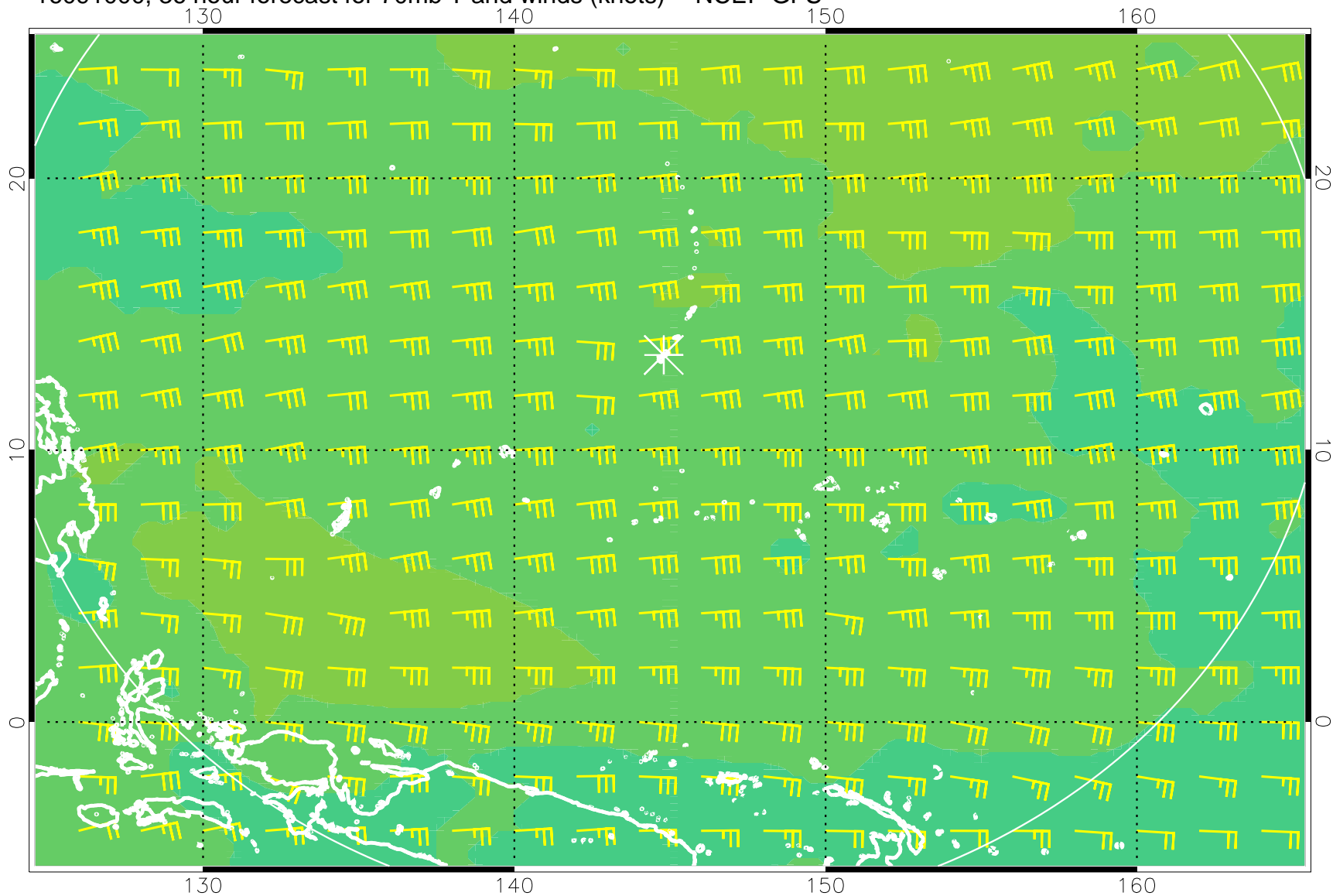
16091000, 36 hour forecast for 70mb T and winds (knots) -- NCEP GFS
