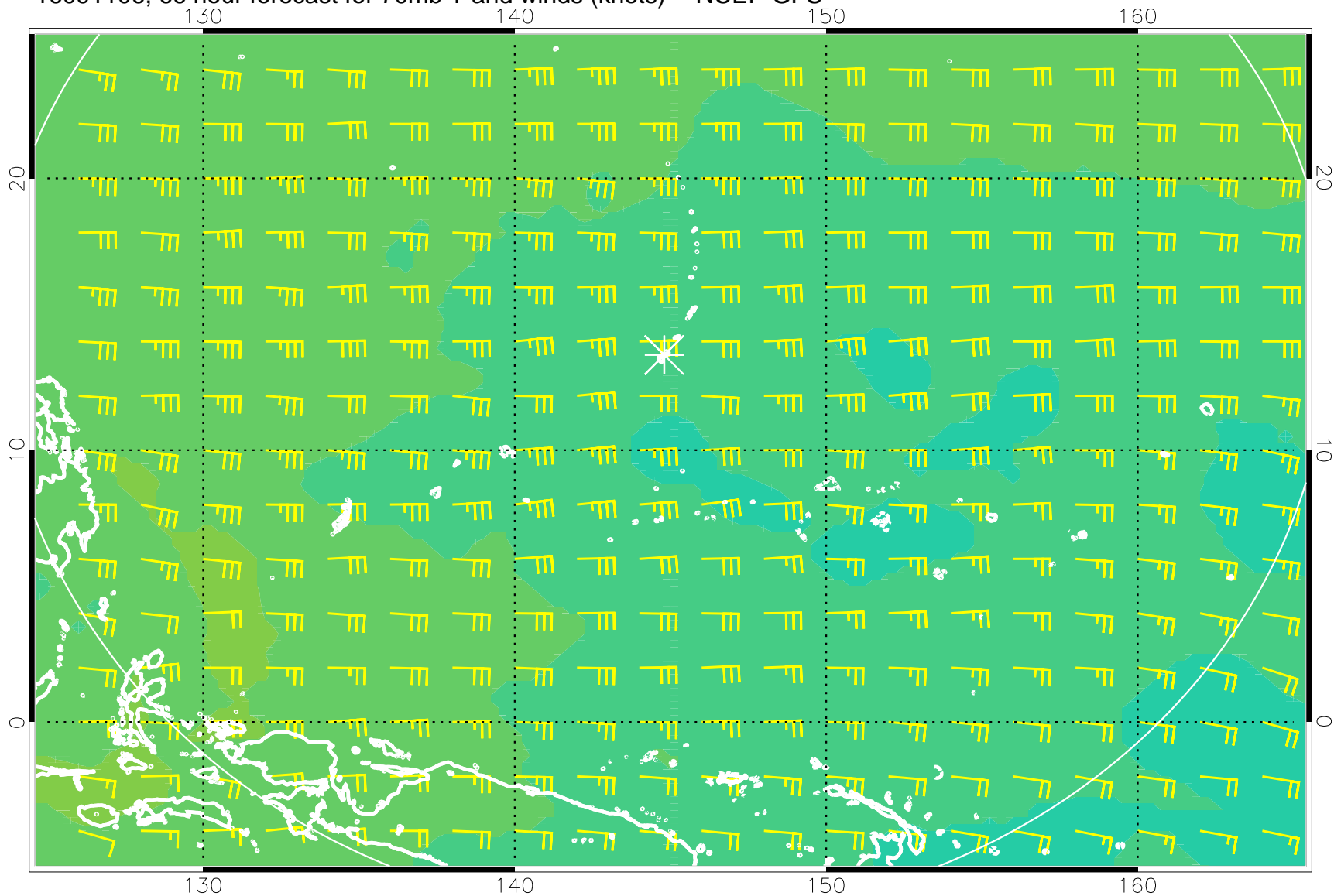
16091106, 66 hour forecast for 70mb T and winds (knots) -- NCEP GFS
