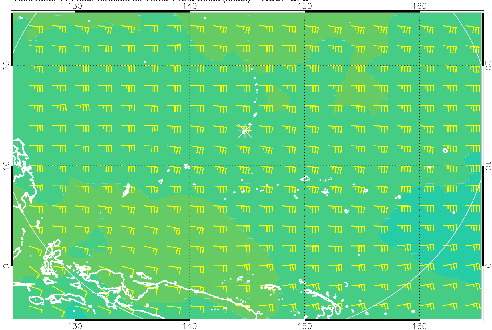
16091306, 114 hour forecast for 70mb T and winds (knots) -- NCEP GFS
