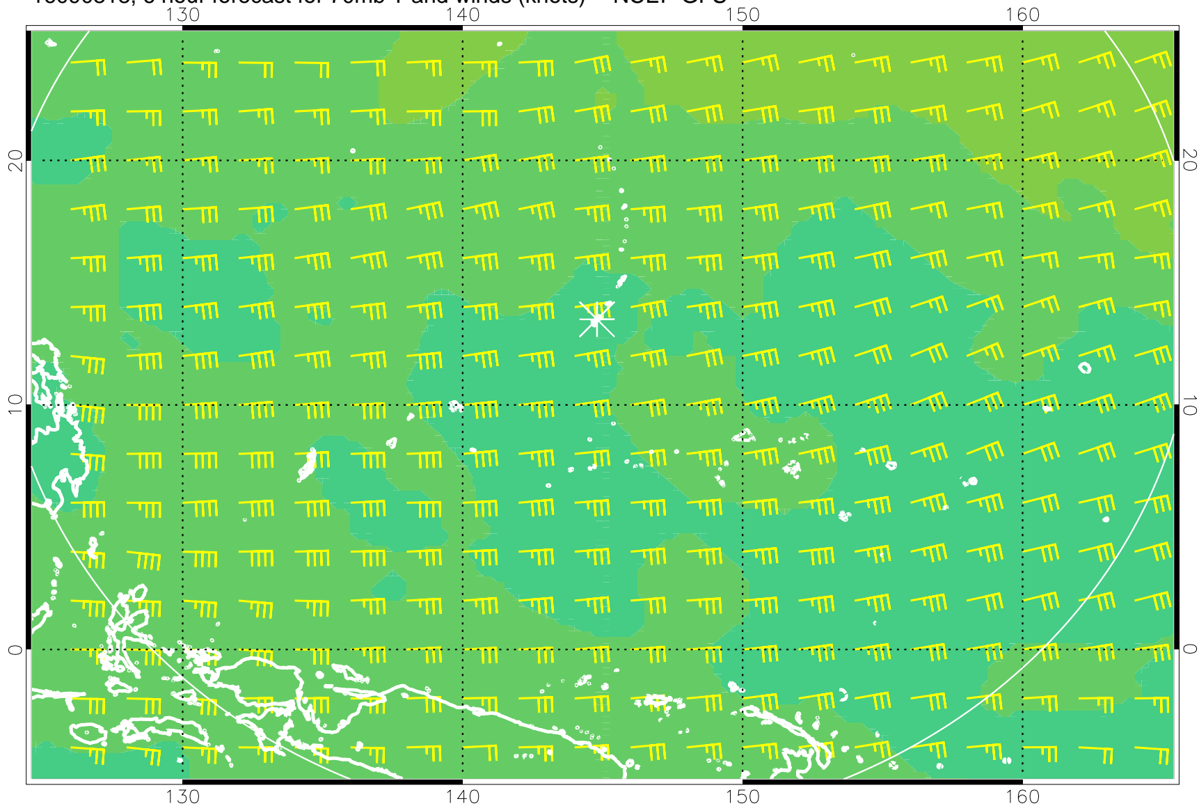
16090818, 6 hour forecast for 70mb T and winds (knots) -- NCEP GFS
