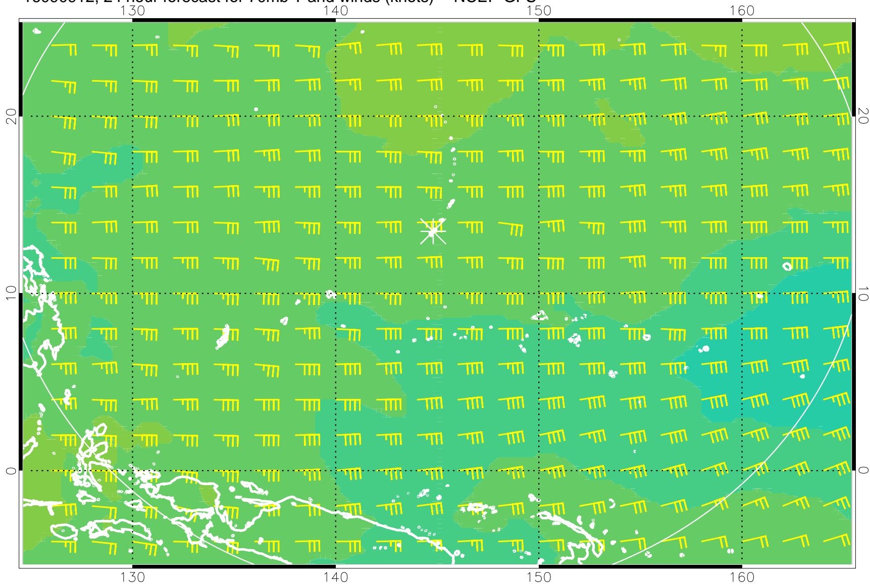
16090912, 24 hour forecast for 70mb T and winds (knots) -- NCEP GFS
