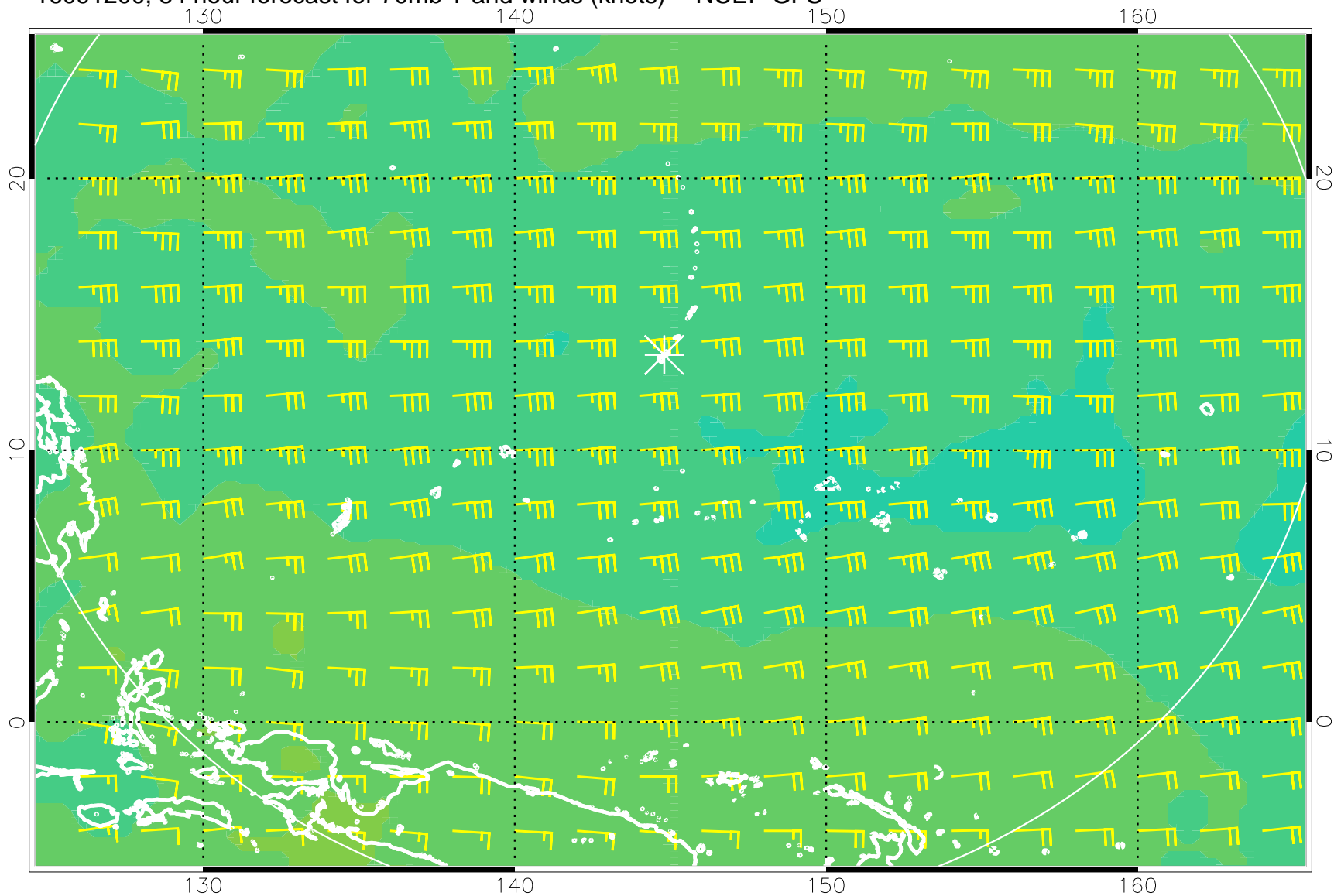
16091200, 84 hour forecast for 70mb T and winds (knots) -- NCEP GFS
