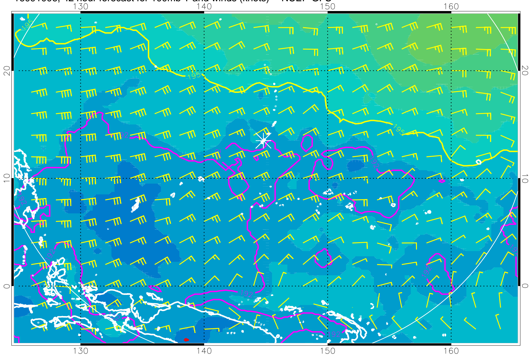
16091006, 42 hour forecast for 100mb T and winds (knots) -- NCEP GFS
