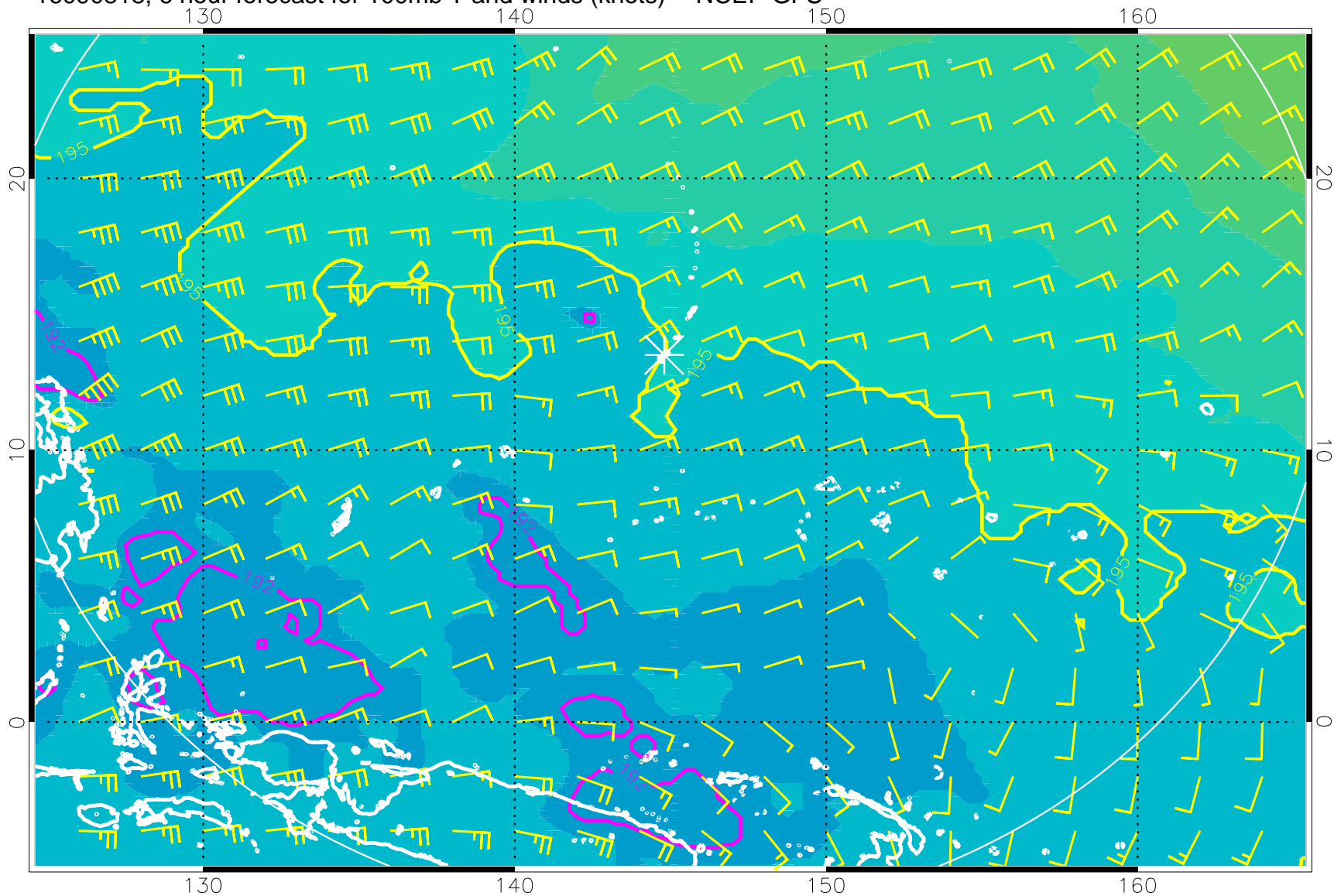
16090818, 6 hour forecast for 100mb T and winds (knots) -- NCEP GFS
