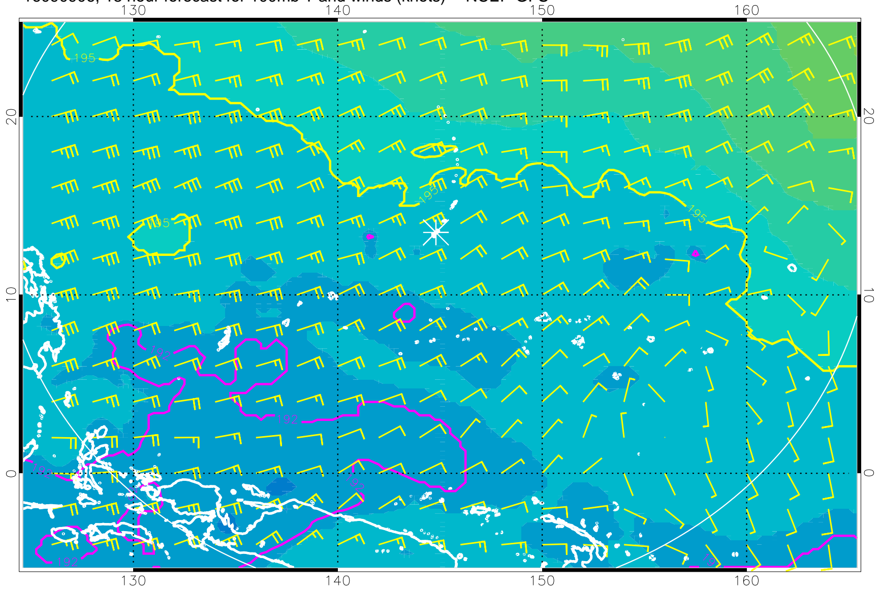
16090906, 18 hour forecast for 100mb T and winds (knots) -- NCEP GFS
