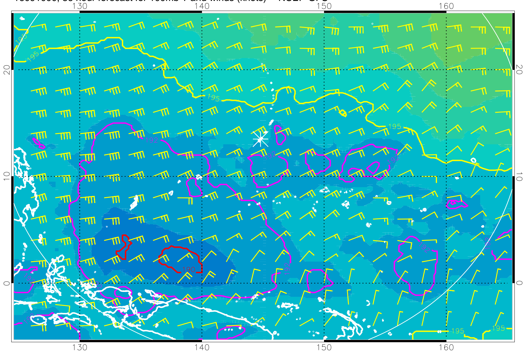
16091000, 36 hour forecast for 100mb T and winds (knots) -- NCEP GFS
