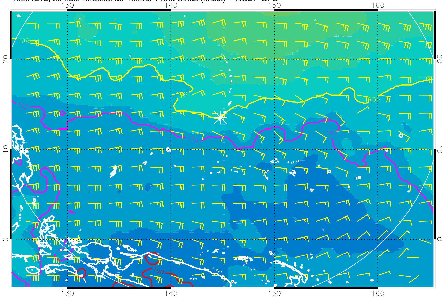
16091212, 96 hour forecast for 100mb T and winds (knots) -- NCEP GFS
