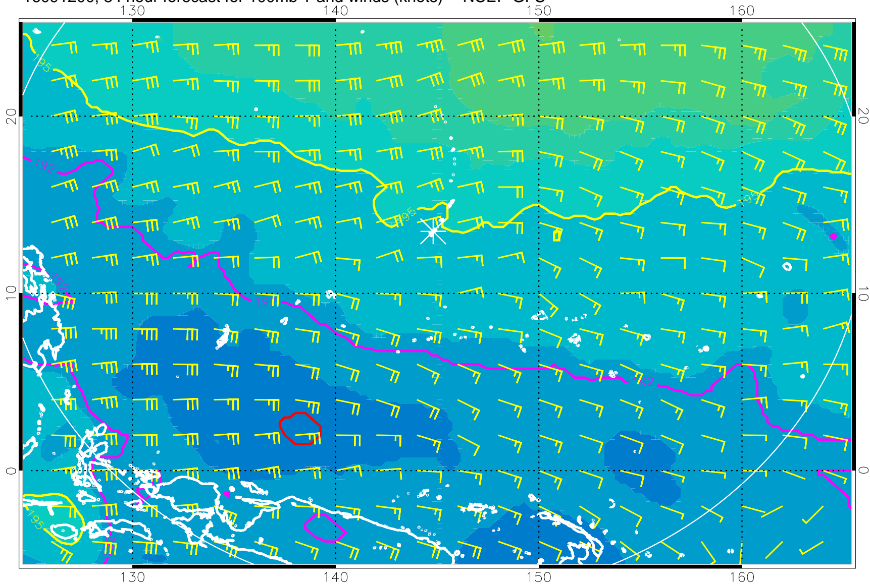
16091200, 84 hour forecast for 100mb T and winds (knots) -- NCEP GFS
