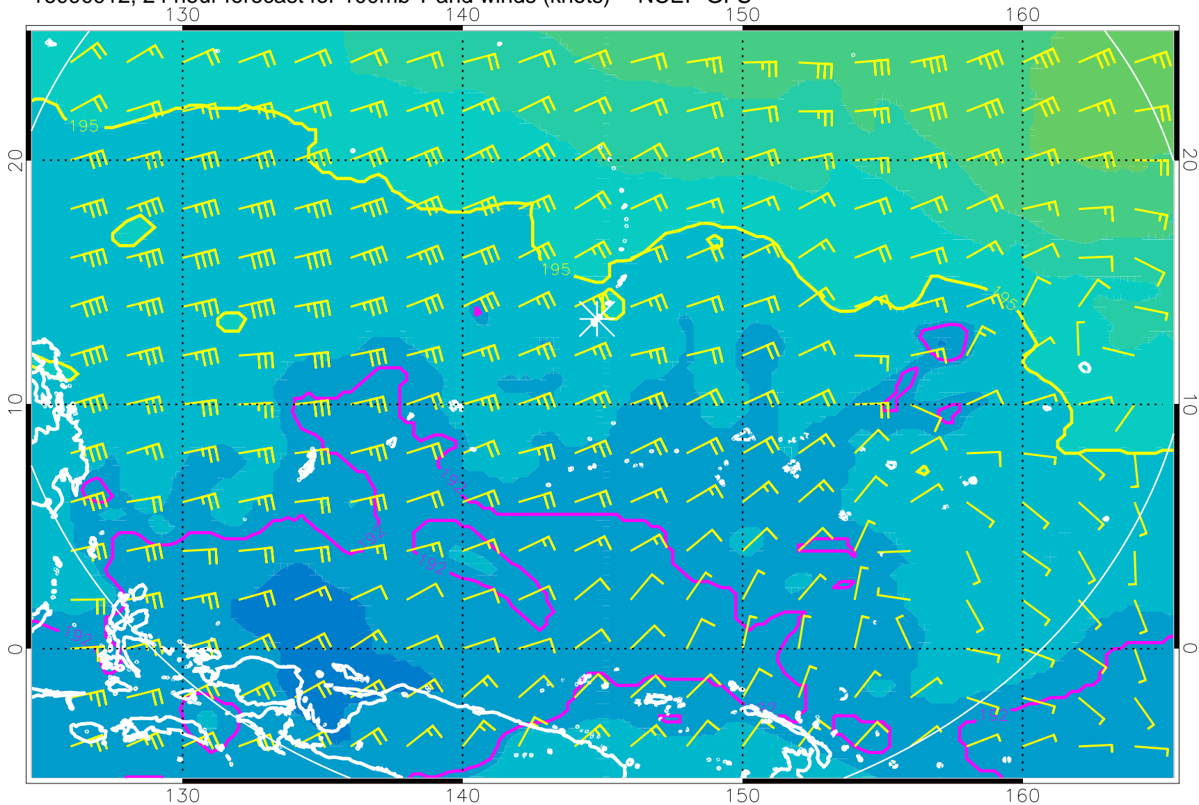
16090912, 24 hour forecast for 100mb T and winds (knots) -- NCEP GFS
