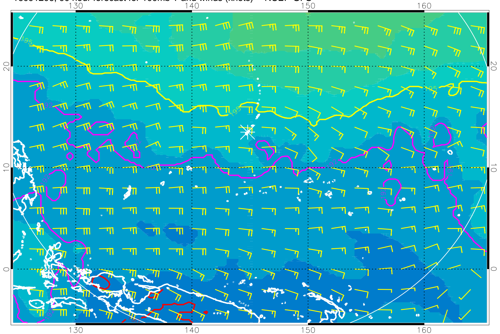
16091206, 90 hour forecast for 100mb T and winds (knots) -- NCEP GFS
