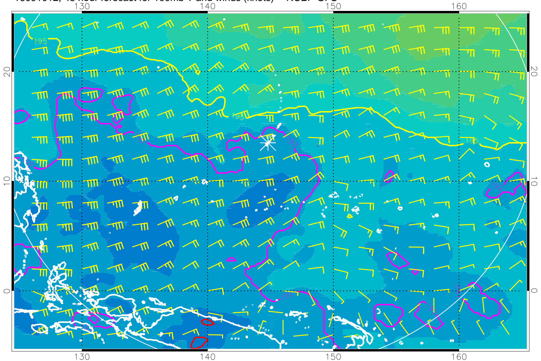
16091012, 48 hour forecast for 100mb T and winds (knots) -- NCEP GFS
