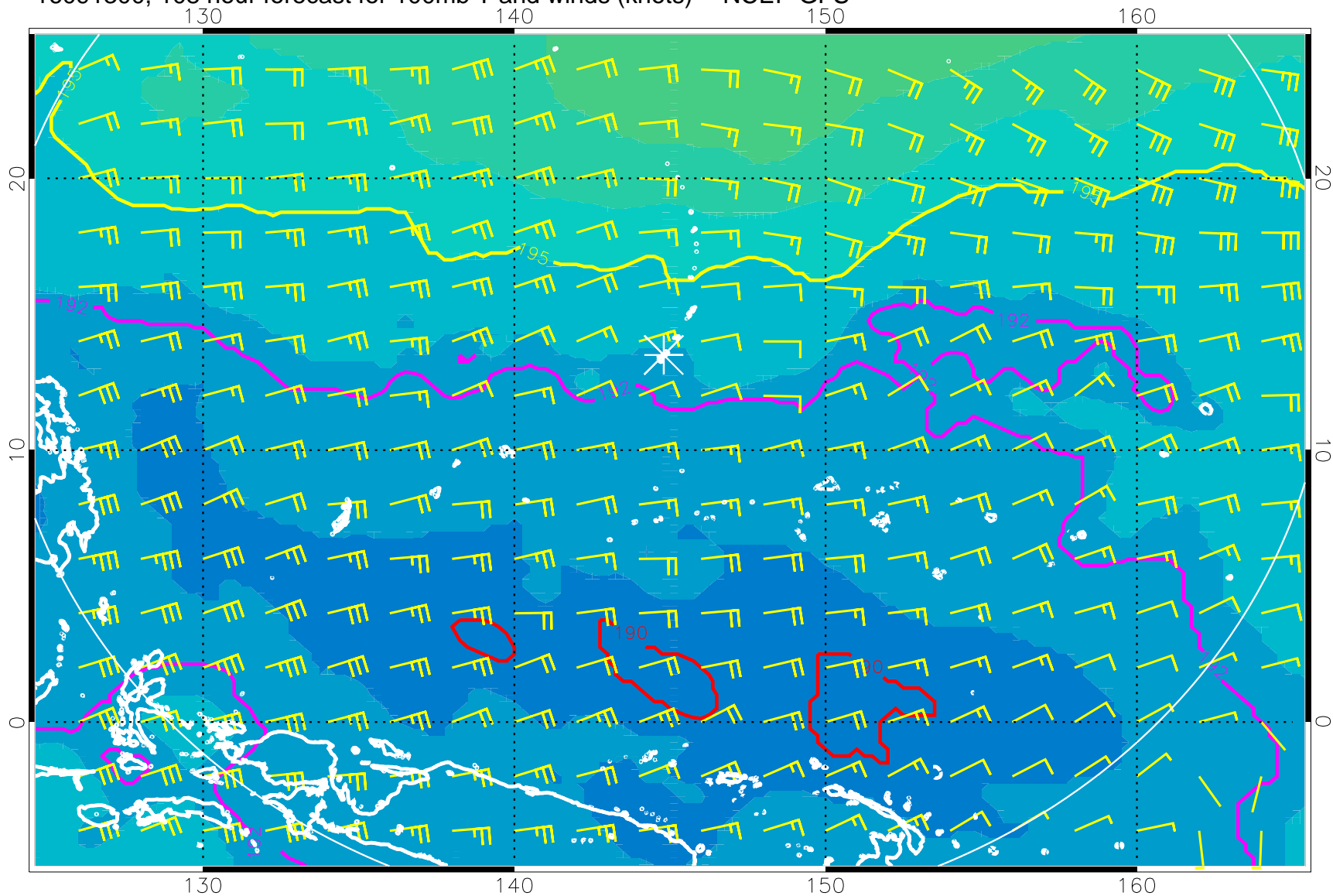
16091300, 108 hour forecast for 100mb T and winds (knots) -- NCEP GFS
