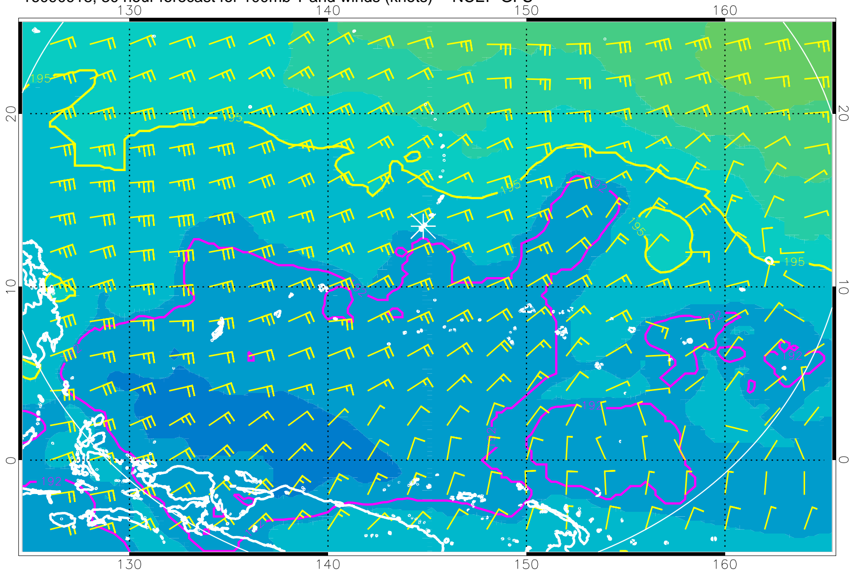
16090918, 30 hour forecast for 100mb T and winds (knots) -- NCEP GFS
