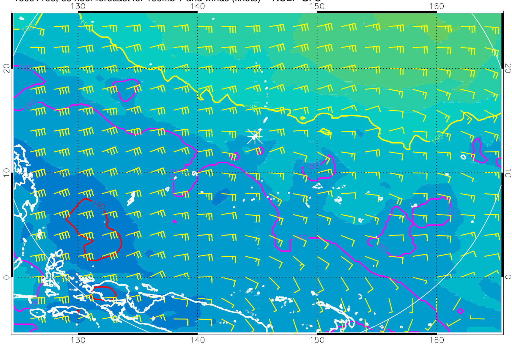
16091106, 66 hour forecast for 100mb T and winds (knots) -- NCEP GFS
