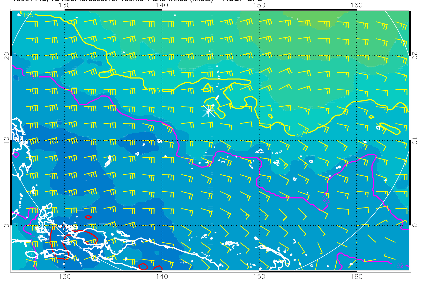
16091112, 72 hour forecast for 100mb T and winds (knots) -- NCEP GFS
