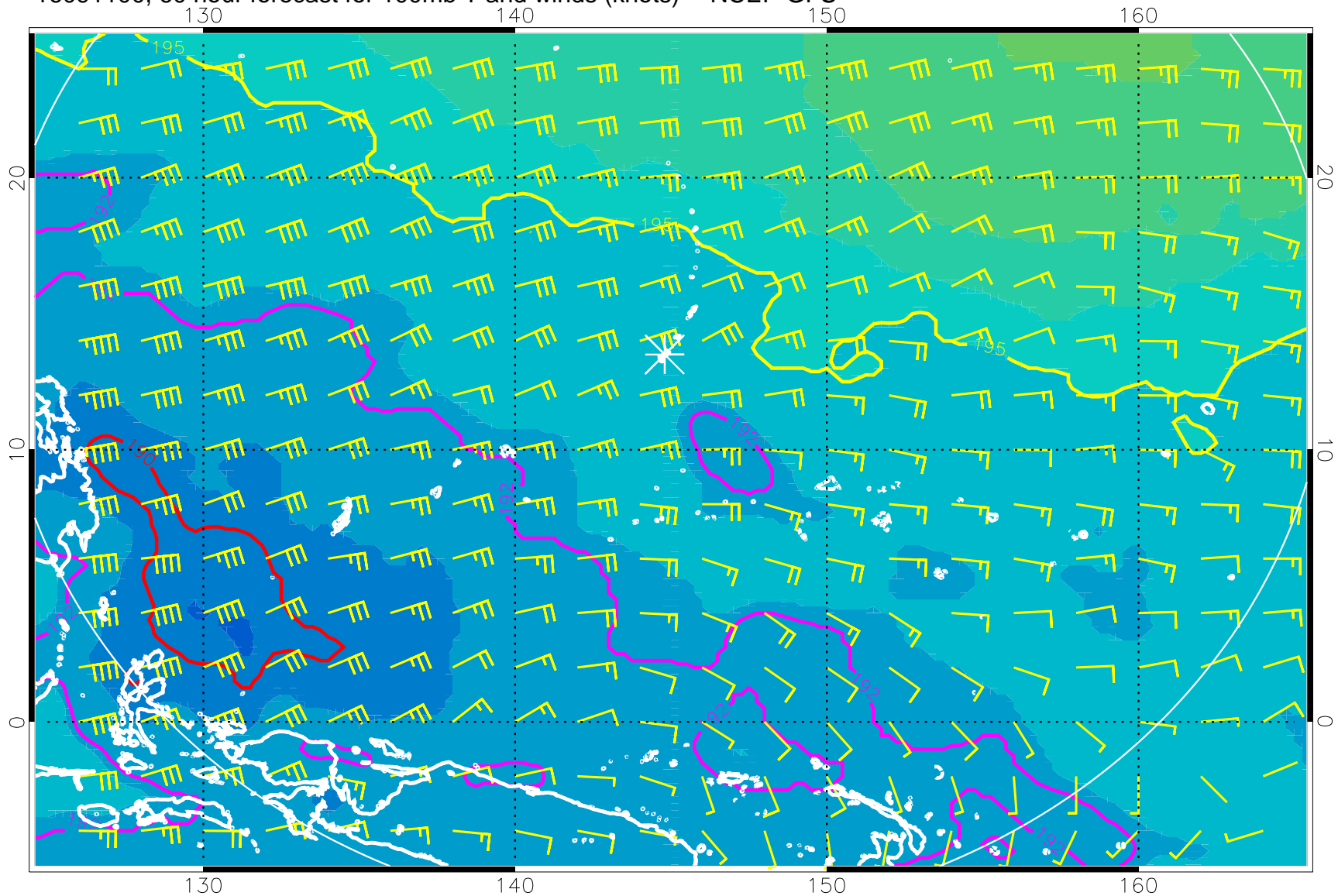
16091100, 60 hour forecast for 100mb T and winds (knots) -- NCEP GFS
