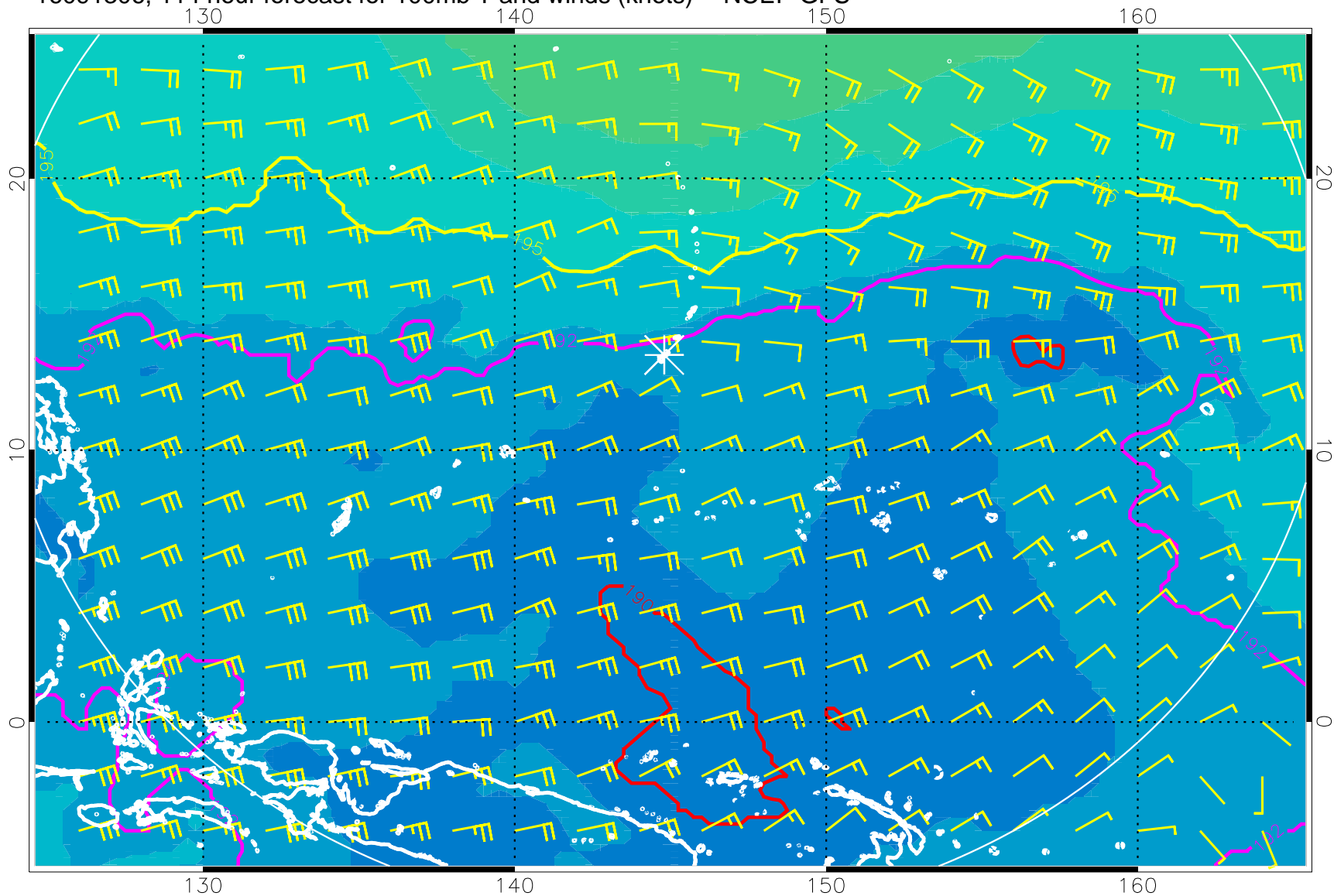
16091306, 114 hour forecast for 100mb T and winds (knots) -- NCEP GFS
