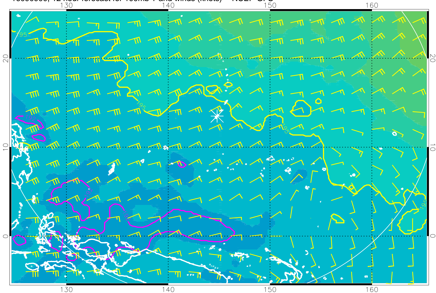
16090900, 12 hour forecast for 100mb T and winds (knots) -- NCEP GFS
