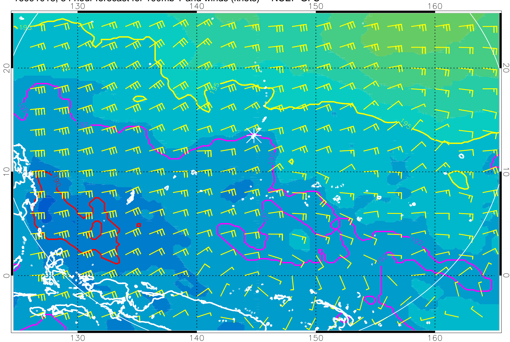
16091018, 54 hour forecast for 100mb T and winds (knots) -- NCEP GFS
