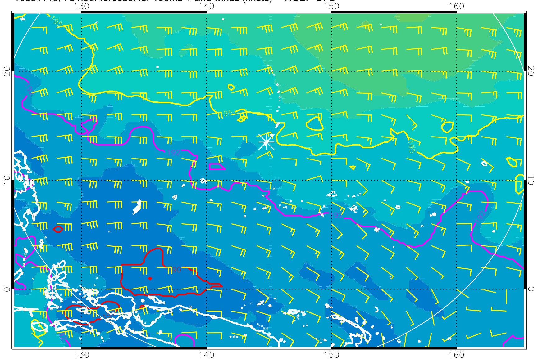
16091118, 78 hour forecast for 100mb T and winds (knots) -- NCEP GFS
