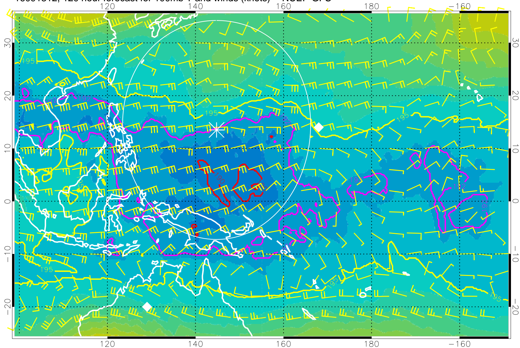
16091312, 120 hour forecast for 100mb T and winds (knots) -- NCEP GFS
