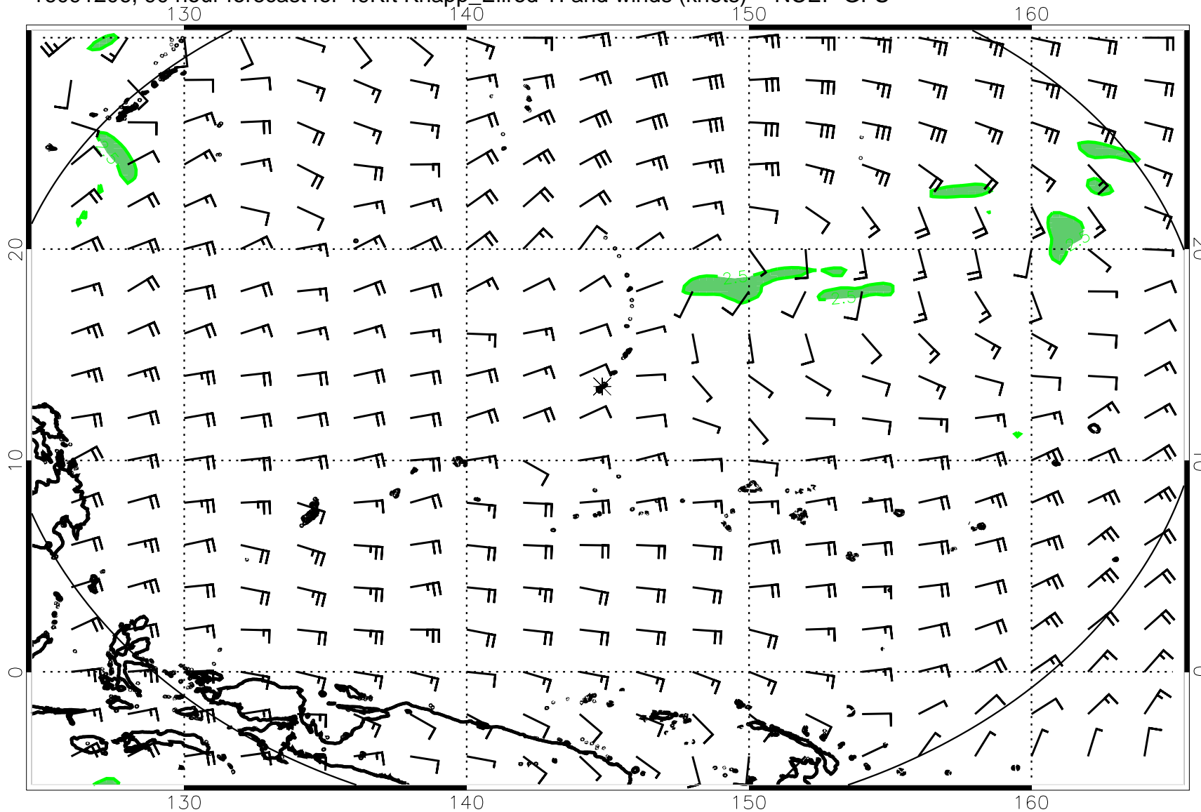
16091206, 90 hour forecast for 49Kft Knapp_Ellrod TI and winds (knots) -- NCEP GFS
