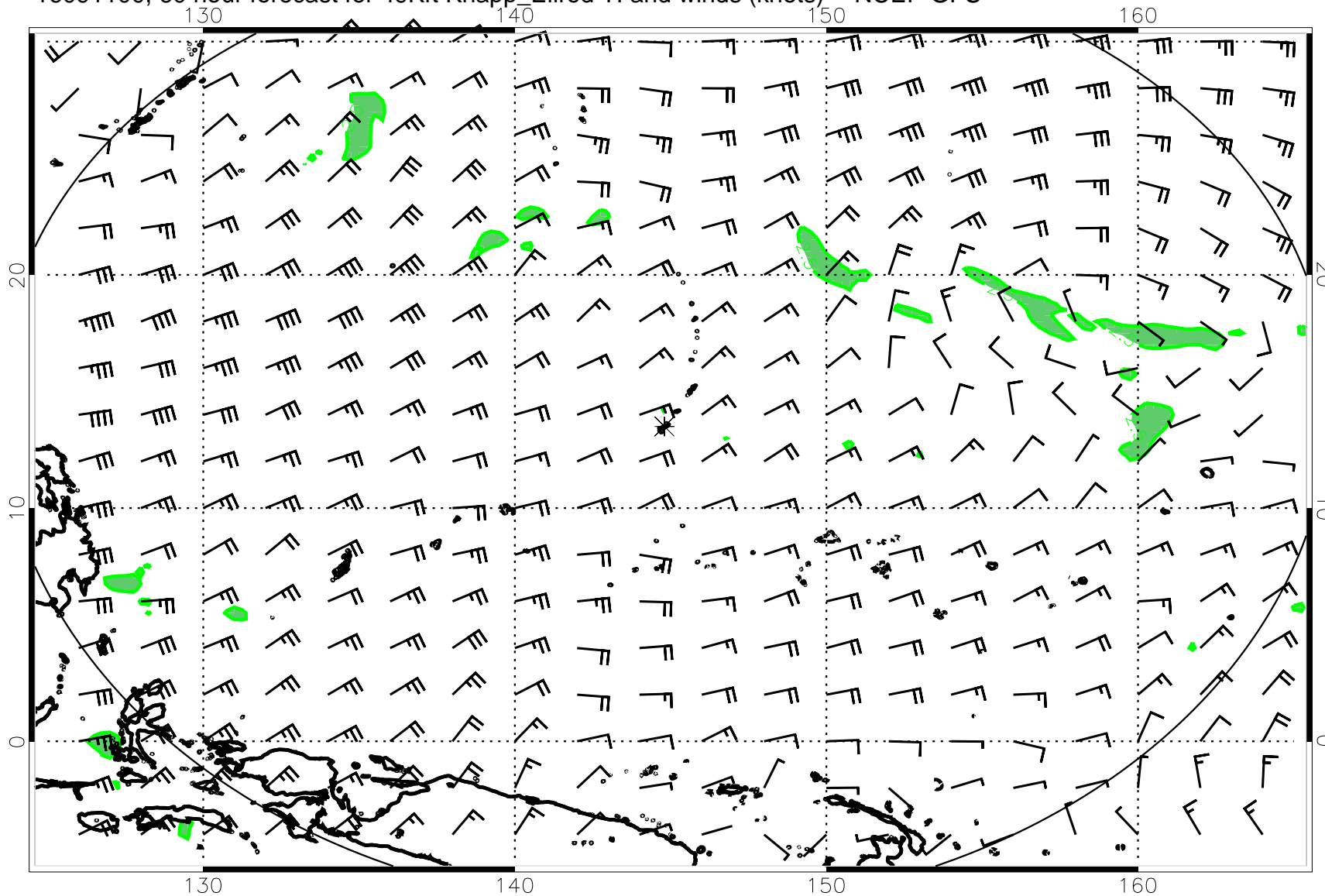
16091100, 60 hour forecast for 49Kft Knapp_Ellrod TI and winds (knots) -- NCEP GFS
