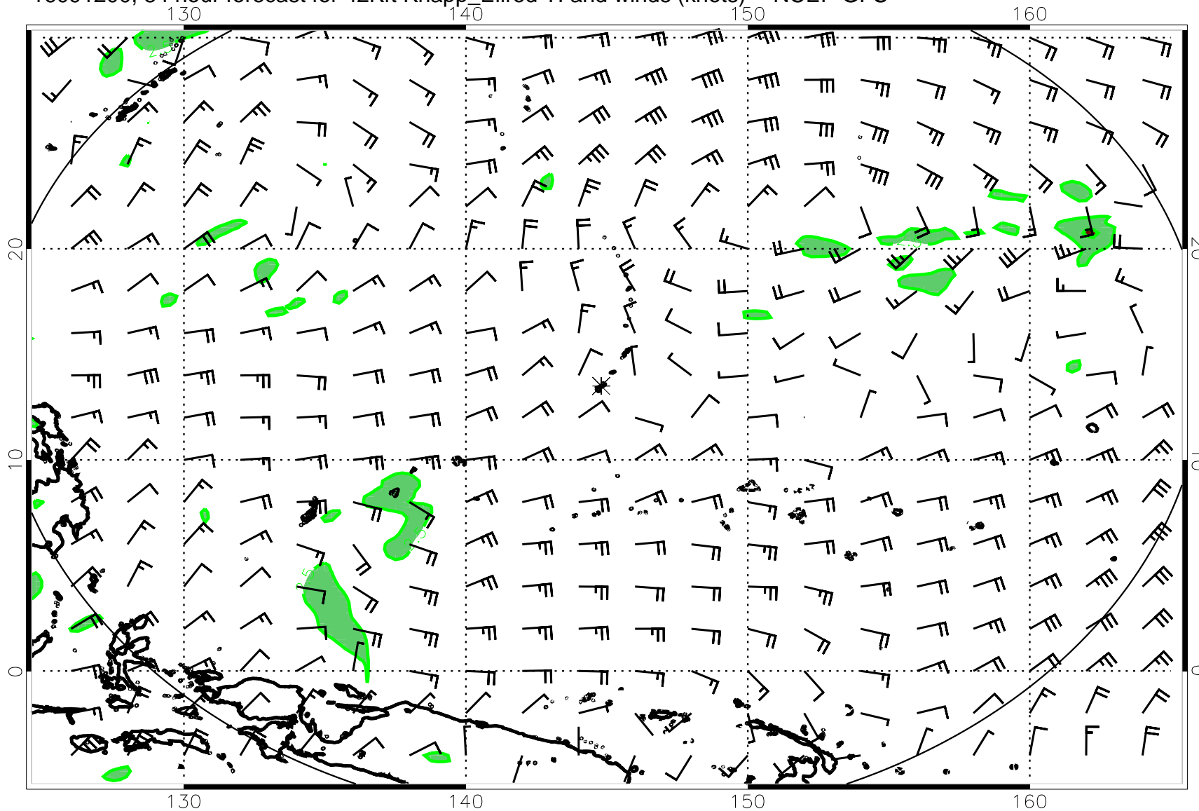
16091200, 84 hour forecast for 42Kft Knapp_Ellrod TI and winds (knots) -- NCEP GFS
