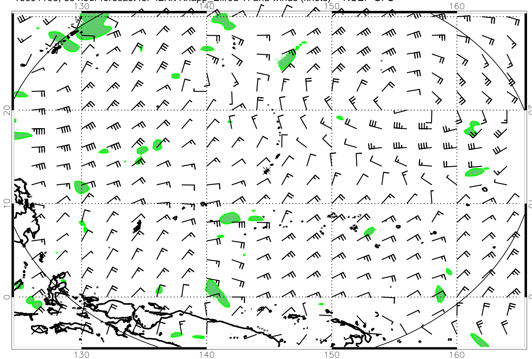
16091106, 66 hour forecast for 42Kft Knapp_Ellrod TI and winds (knots) -- NCEP GFS
