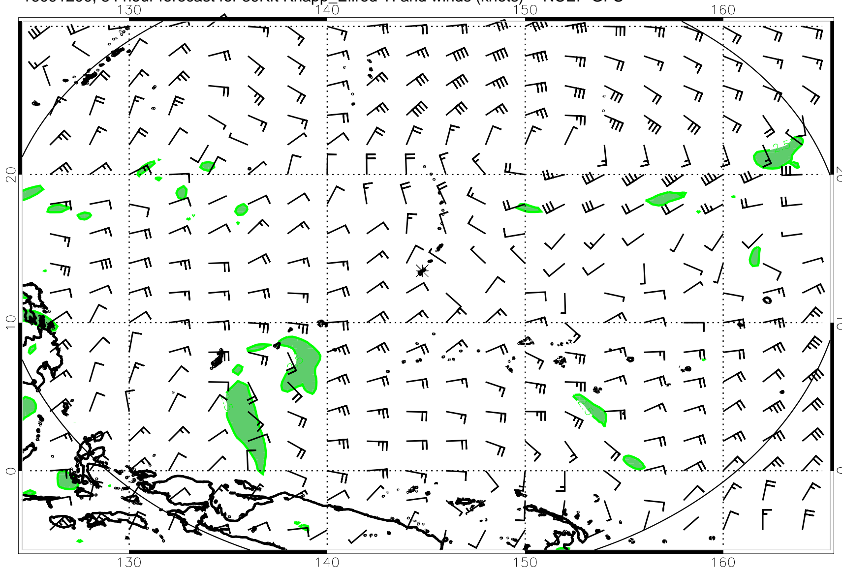
16091200, 84 hour forecast for 39Kft Knapp_Ellrod TI and winds (knots) -- NCEP GFS
