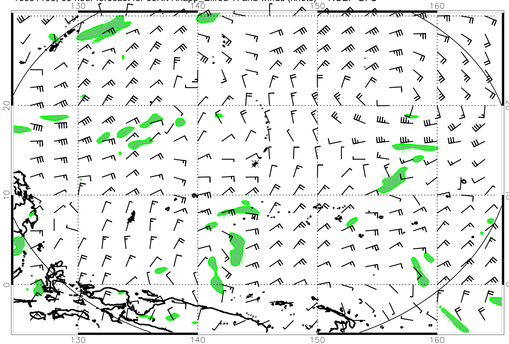
16091106, 66 hour forecast for 39Kft Knapp_Ellrod TI and winds (knots) -- NCEP GFS
