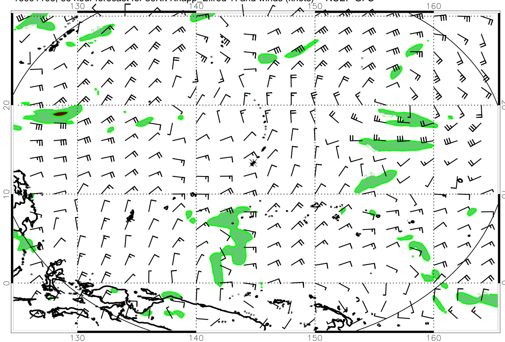
16091106, 66 hour forecast for 36Kft Knapp_Ellrod TI and winds (knots) -- NCEP GFS
