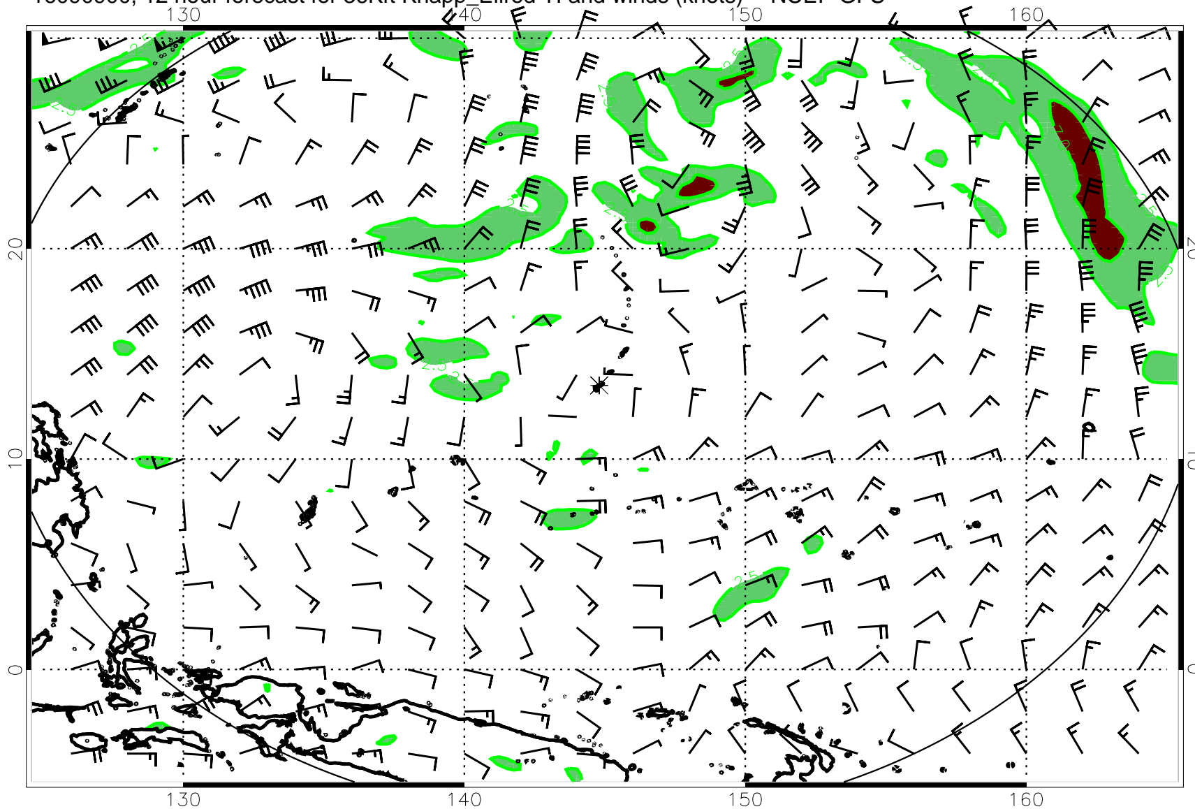
16090900, 12 hour forecast for 36Kft Knapp_Ellrod TI and winds (knots) -- NCEP GFS
