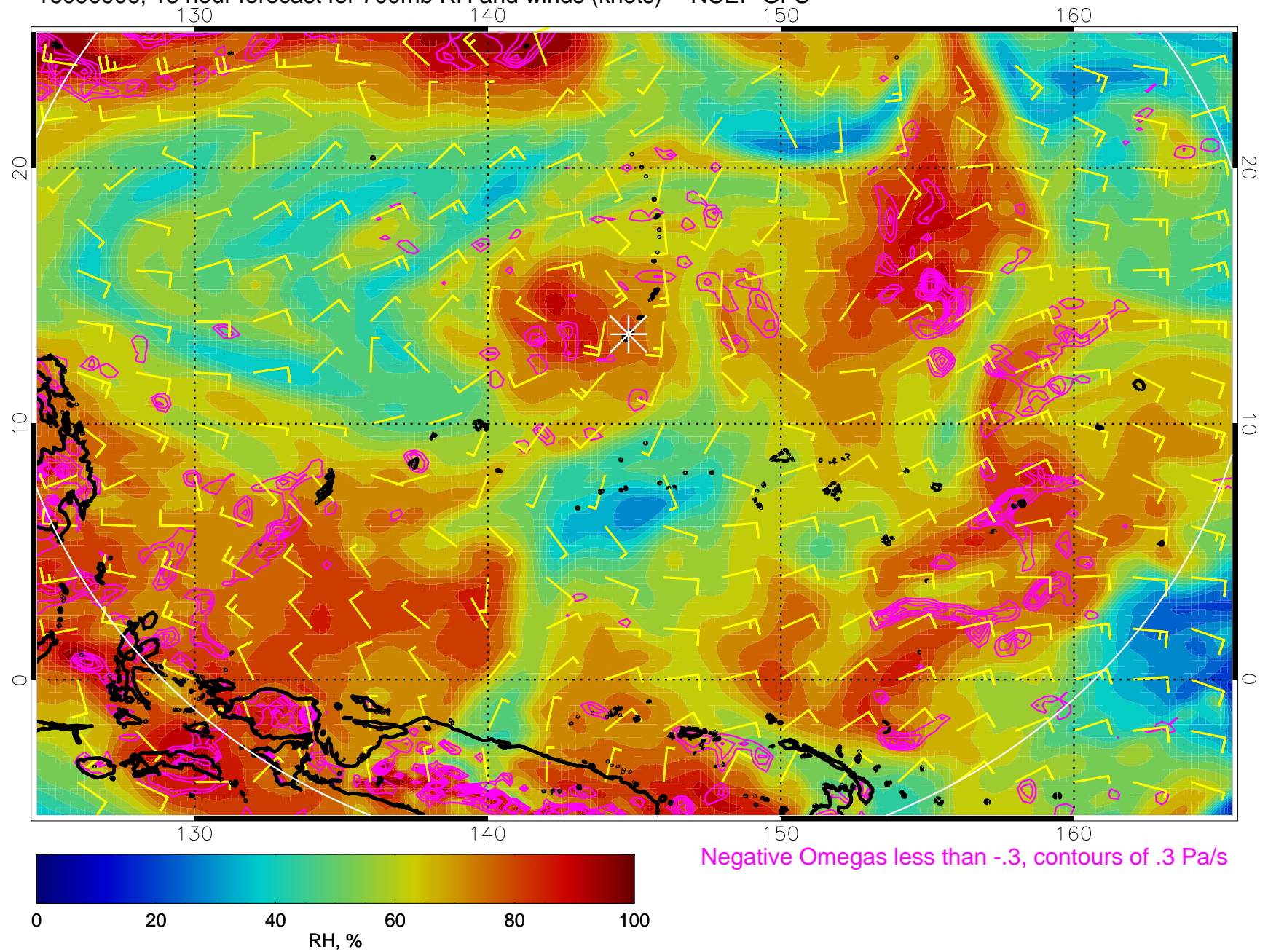
16090906, 18 hour forecast for 700mb RH and winds (knots) -- NCEP GFS
