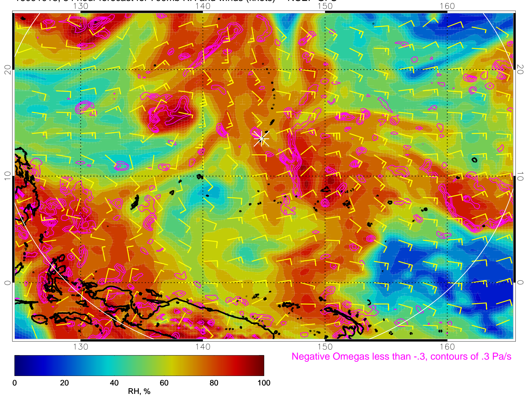
16091018, 54 hour forecast for 700mb RH and winds (knots) -- NCEP GFS
