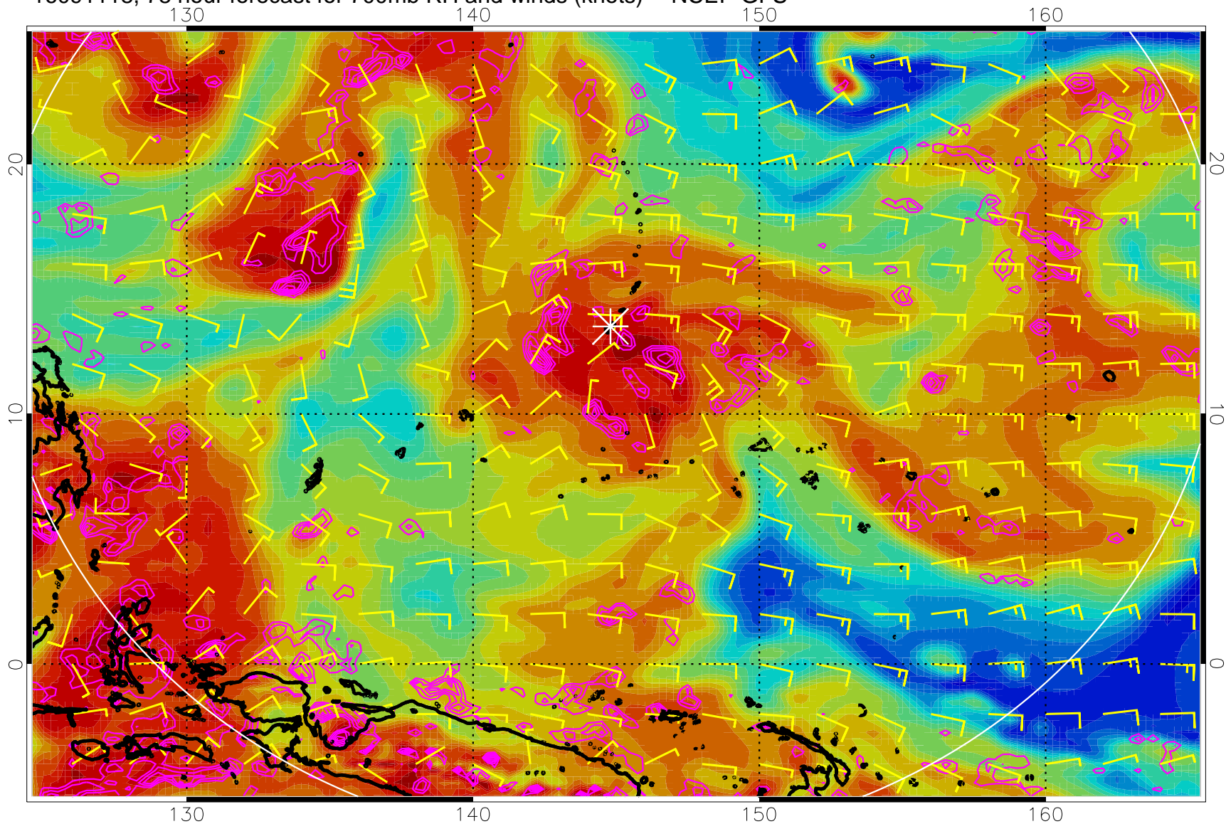
16091118, 78 hour forecast for 700mb RH and winds (knots) -- NCEP GFS
