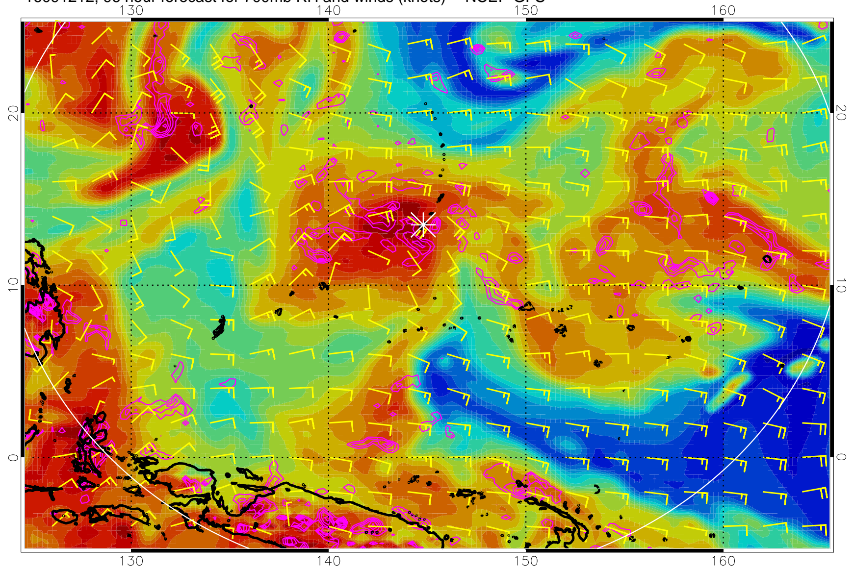
16091212, 96 hour forecast for 700mb RH and winds (knots) -- NCEP GFS
