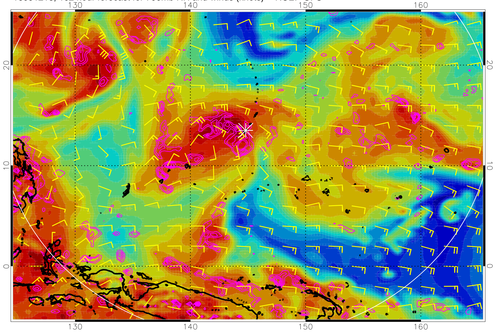
16091218, 102 hour forecast for 700mb RH and winds (knots) -- NCEP GFS
