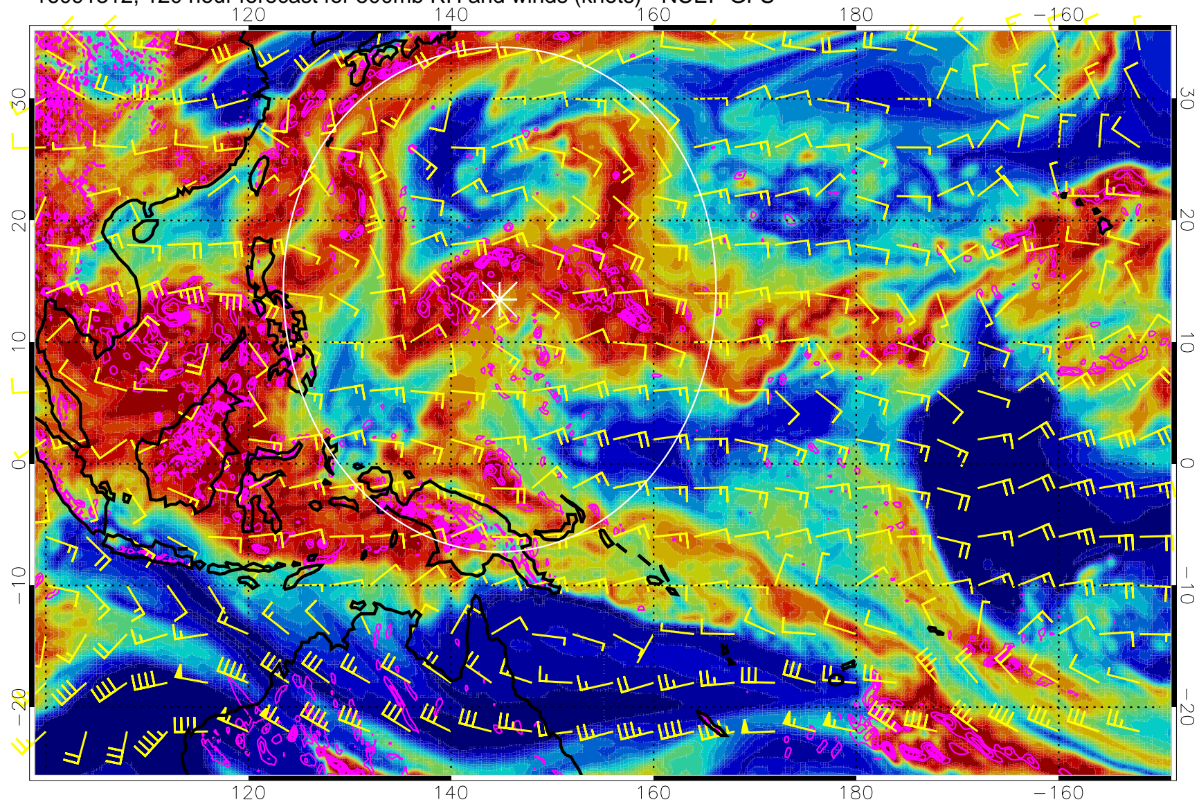
16091312, 120 hour forecast for 500mb RH and winds (knots) - NCEP GFS
