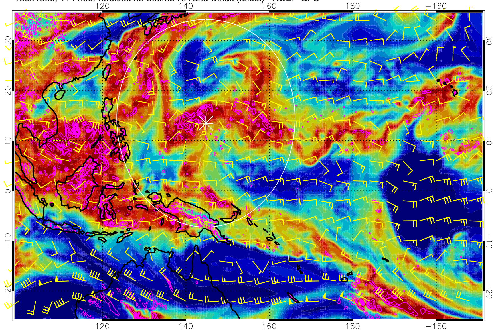
16091306, 114 hour forecast for 500mb RH and winds (knots) - NCEP GFS
