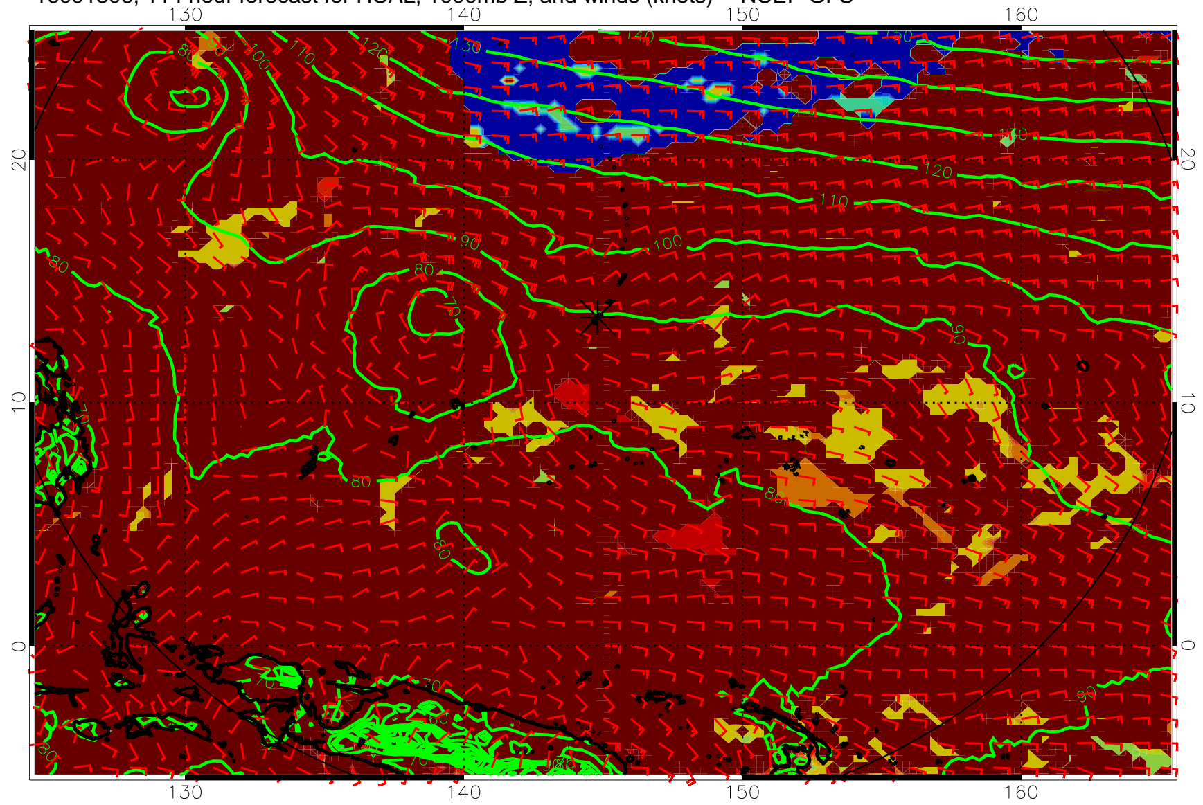
16091306, 114 hour forecast for HCAL, 1000mb Z, and winds (knots) -- NCEP GFS
