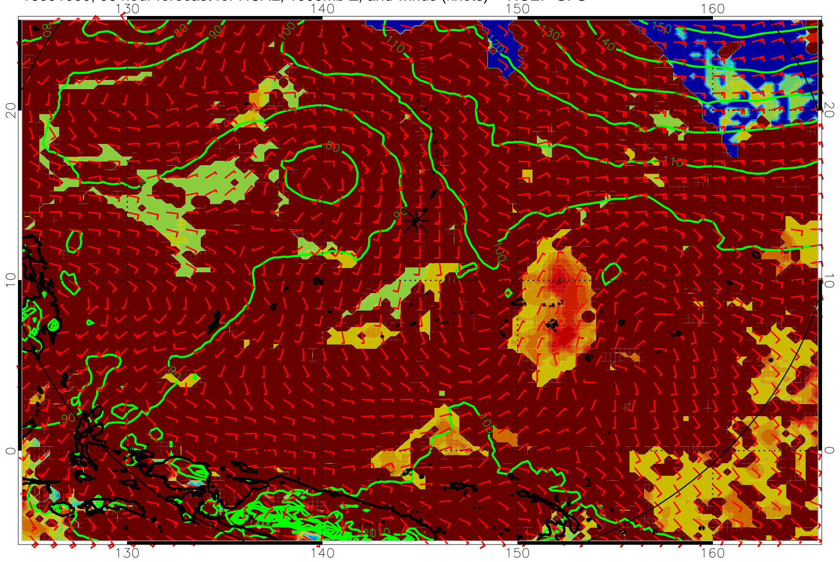
16091000, 36 hour forecast for HCAL, 1000mb Z, and winds (knots) -- NCEP GFS
