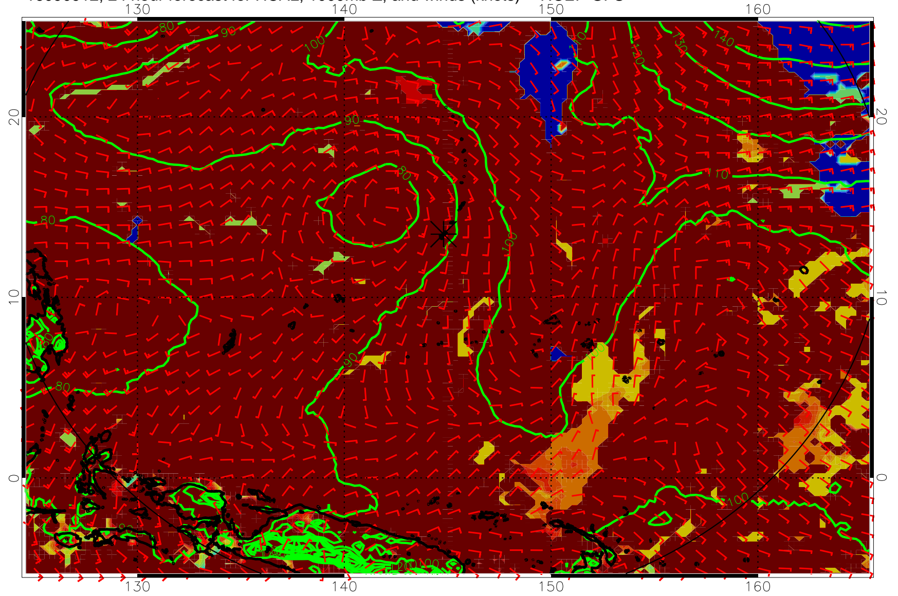
16090912, 24 hour forecast for HCAL, 1000mb Z, and winds (knots) -- NCEP GFS
