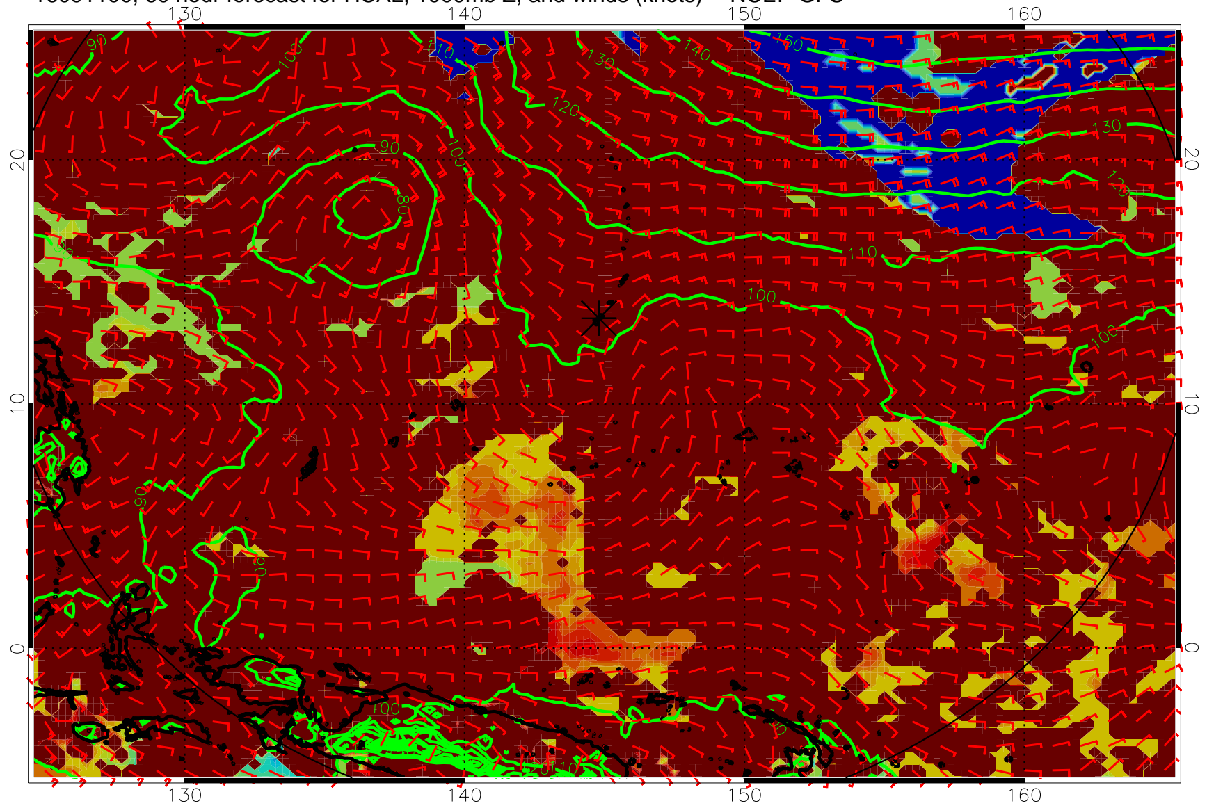
16091100, 60 hour forecast for HCAL, 1000mb Z, and winds (knots) -- NCEP GFS
