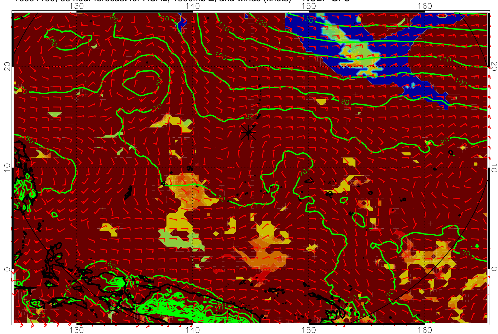
16091106, 66 hour forecast for HCAL, 1000mb Z, and winds (knots) -- NCEP GFS
