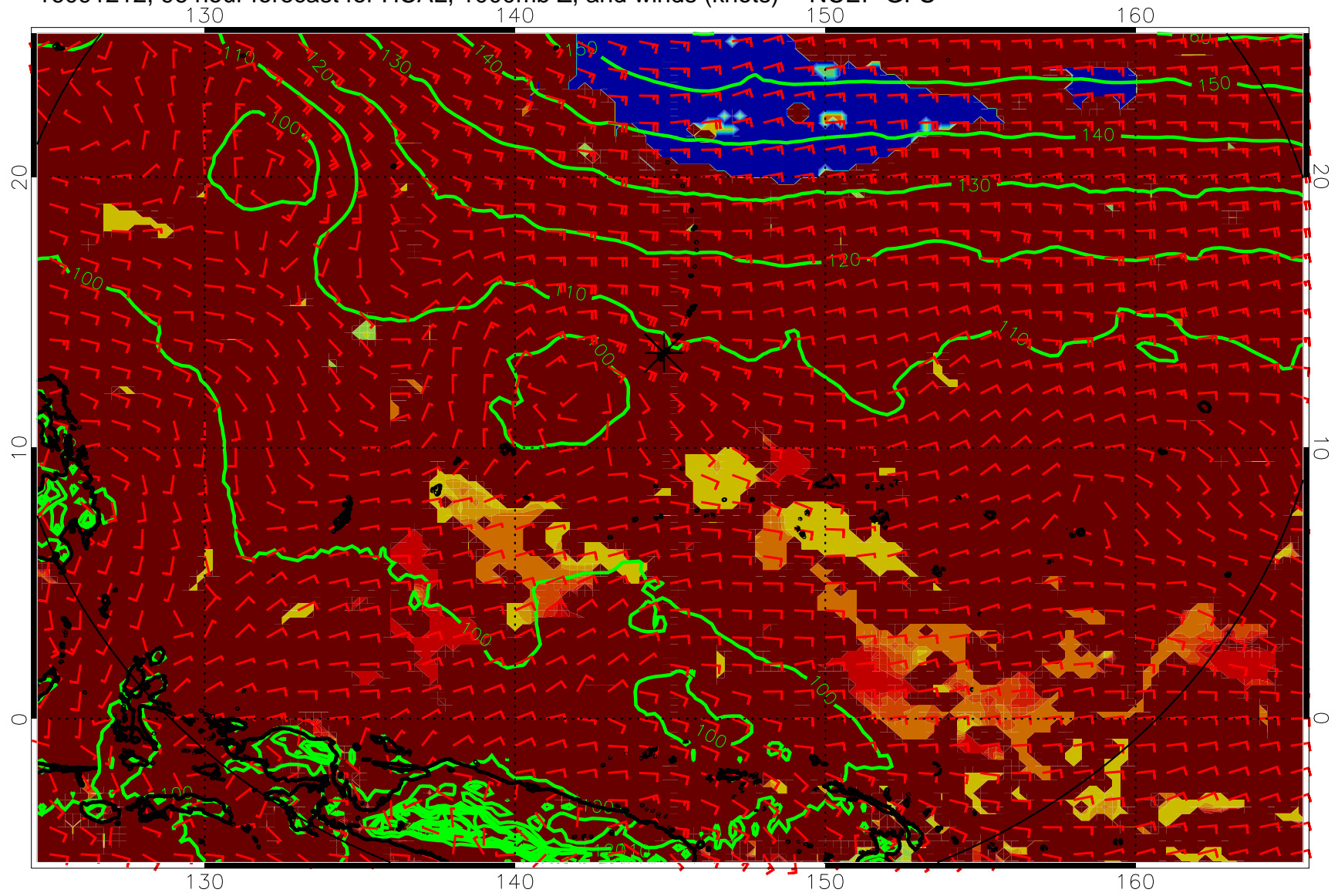
16091212, 96 hour forecast for HCAL, 1000mb Z, and winds (knots) -- NCEP GFS
