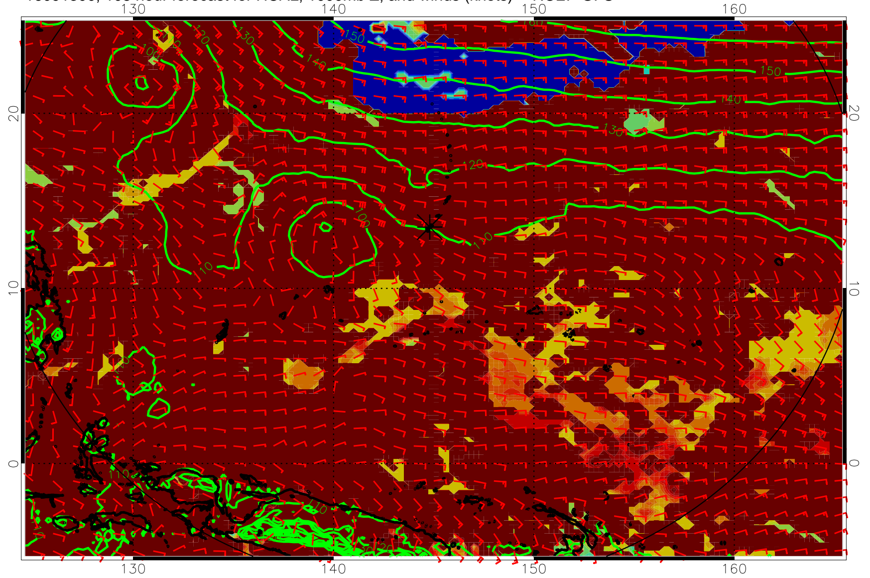
16091300, 108 hour forecast for HCAL, 1000mb Z, and winds (knots) -- NCEP GFS
