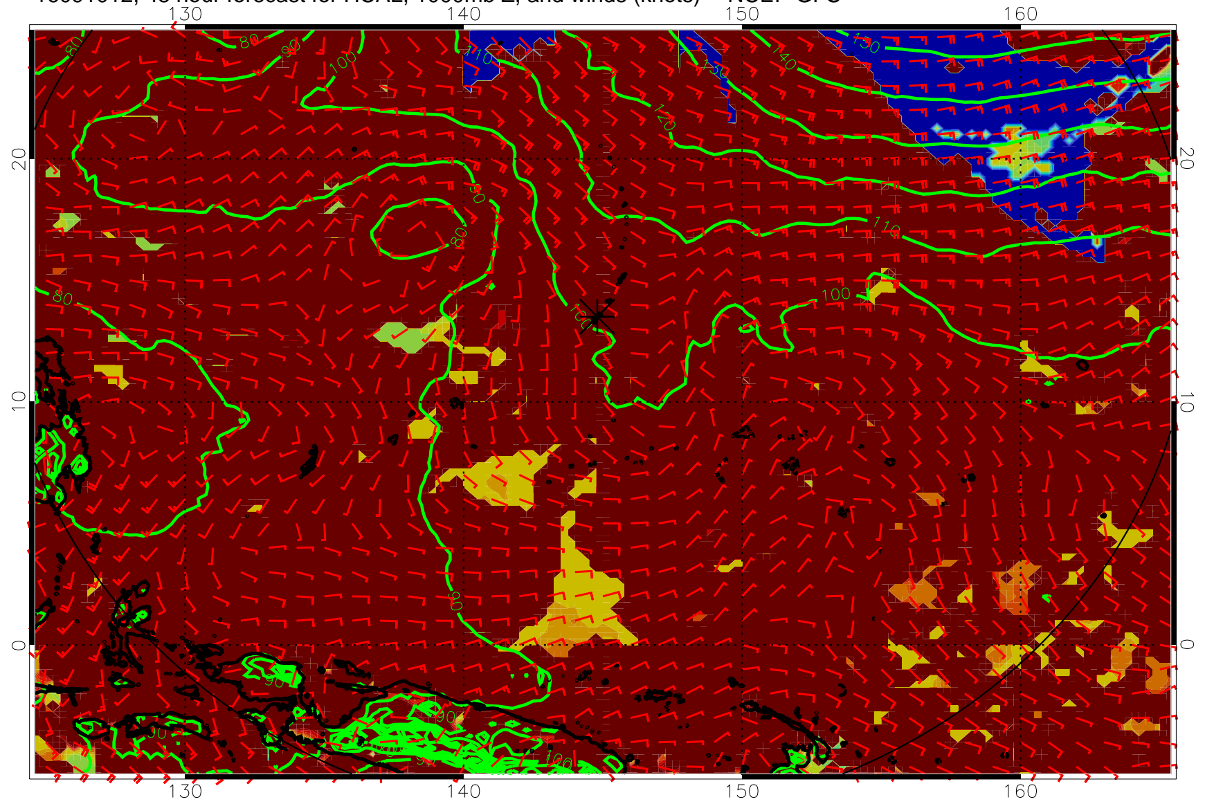
16091012, 48 hour forecast for HCAL, 1000mb Z, and winds (knots) -- NCEP GFS
