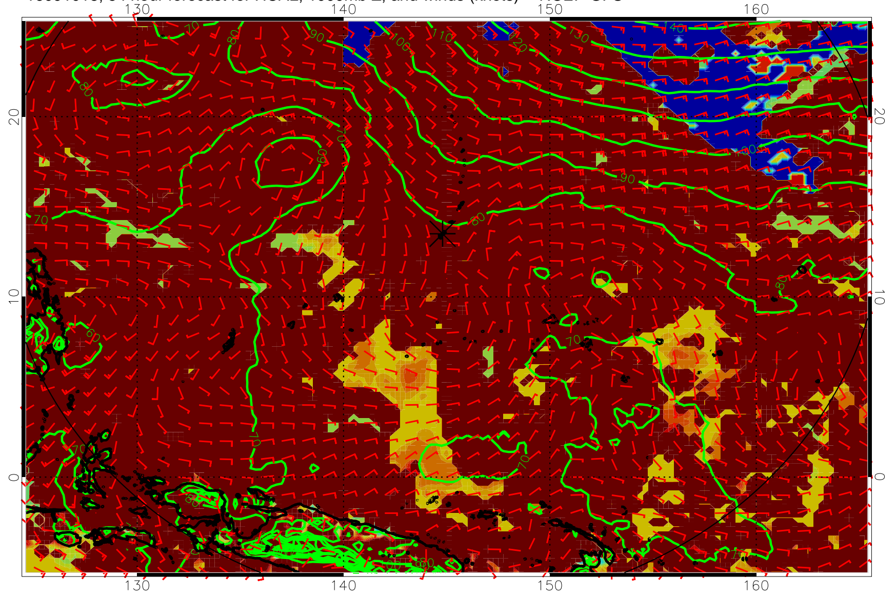
16091018, 54 hour forecast for HCAL, 1000mb Z, and winds (knots) -- NCEP GFS
