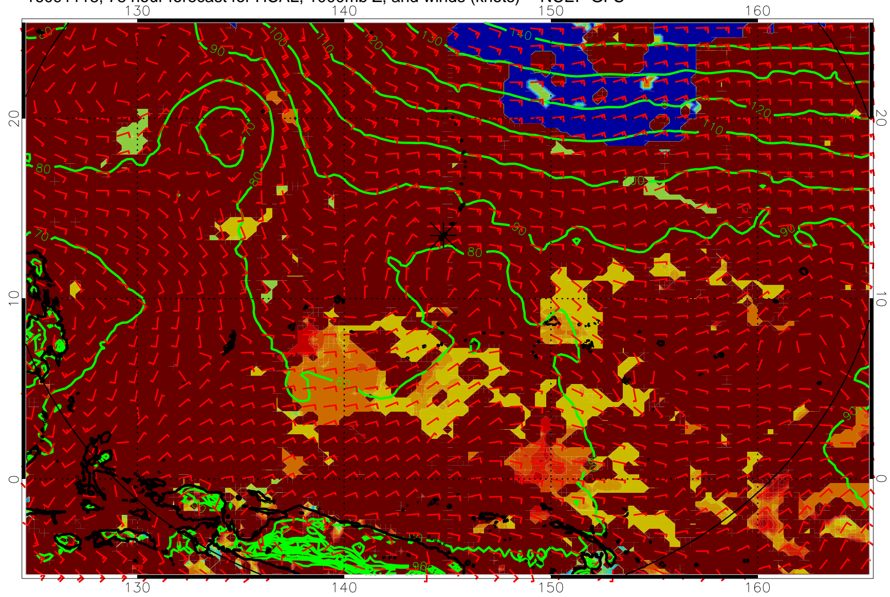
16091118, 78 hour forecast for HCAL, 1000mb Z, and winds (knots) -- NCEP GFS
