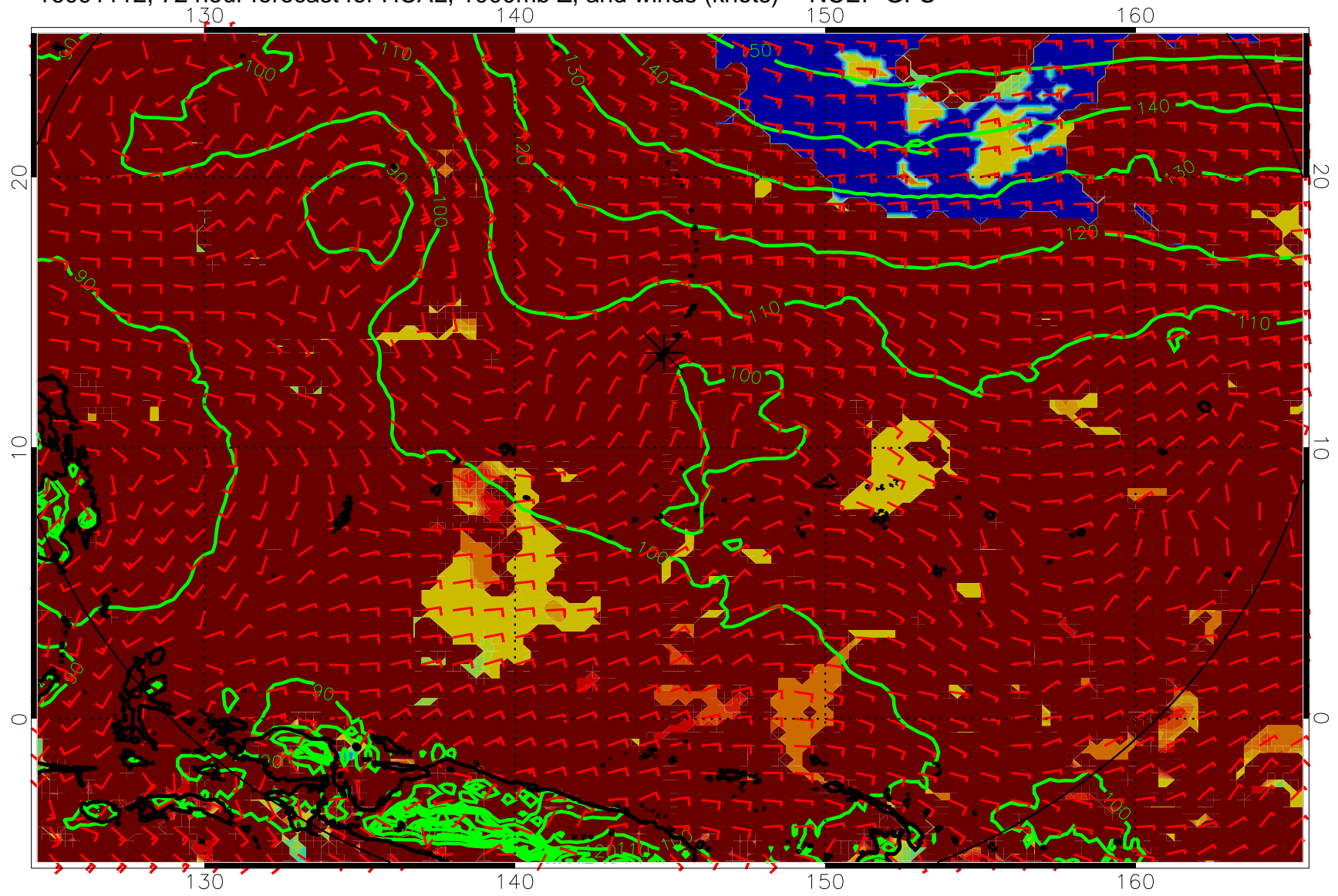
16091112, 72 hour forecast for HCAL, 1000mb Z, and winds (knots) -- NCEP GFS
