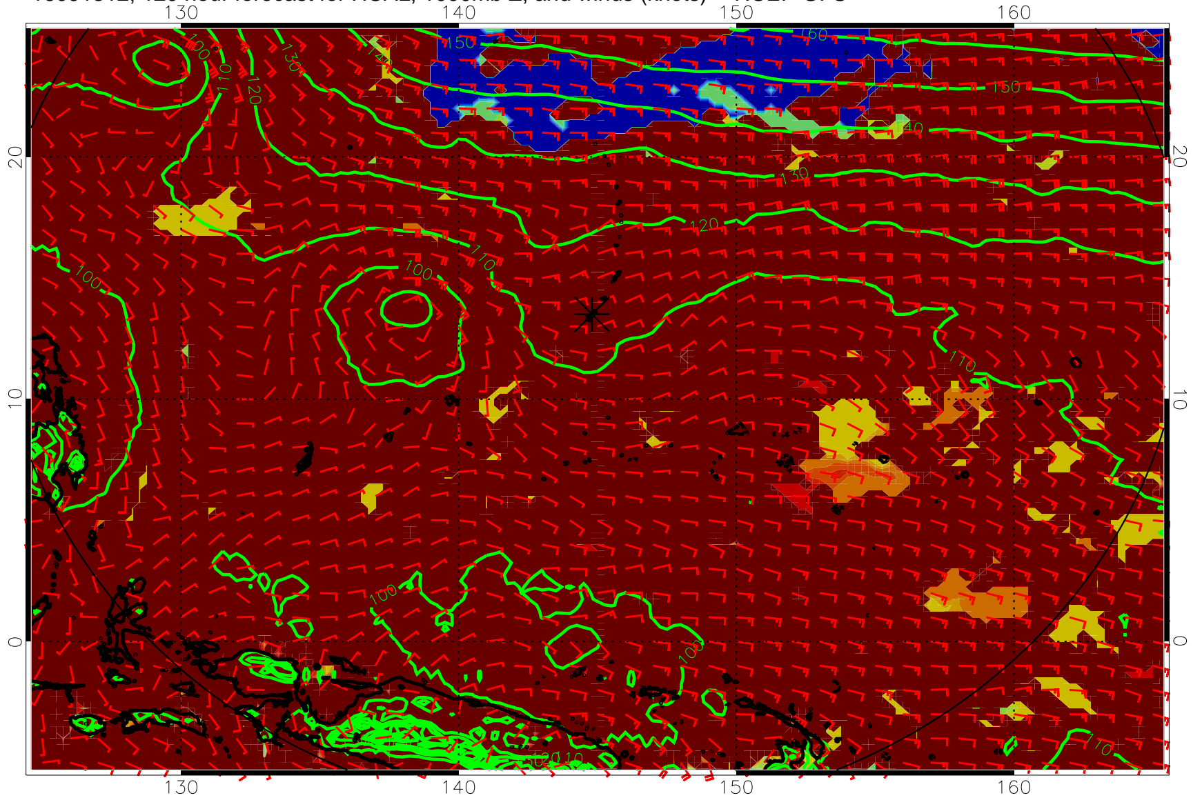
16091312, 120 hour forecast for HCAL, 1000mb Z, and winds (knots) -- NCEP GFS
