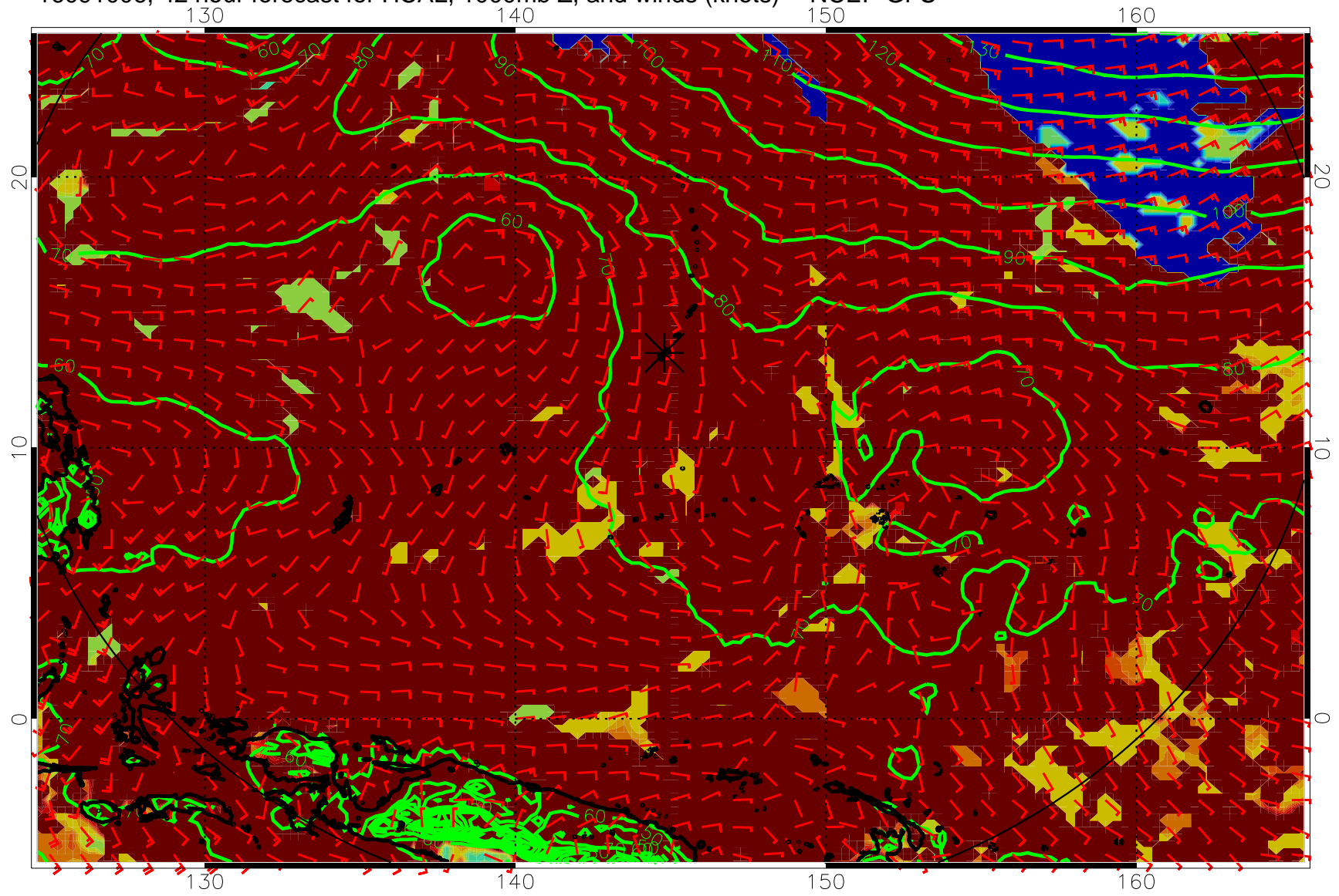
16091006, 42 hour forecast for HCAL, 1000mb Z, and winds (knots) -- NCEP GFS
