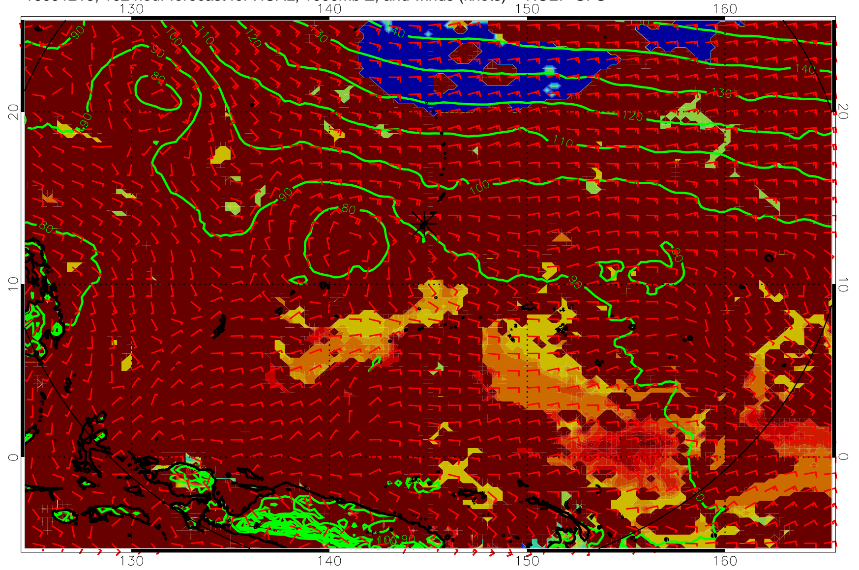
16091218, 102 hour forecast for HCAL, 1000mb Z, and winds (knots) -- NCEP GFS
