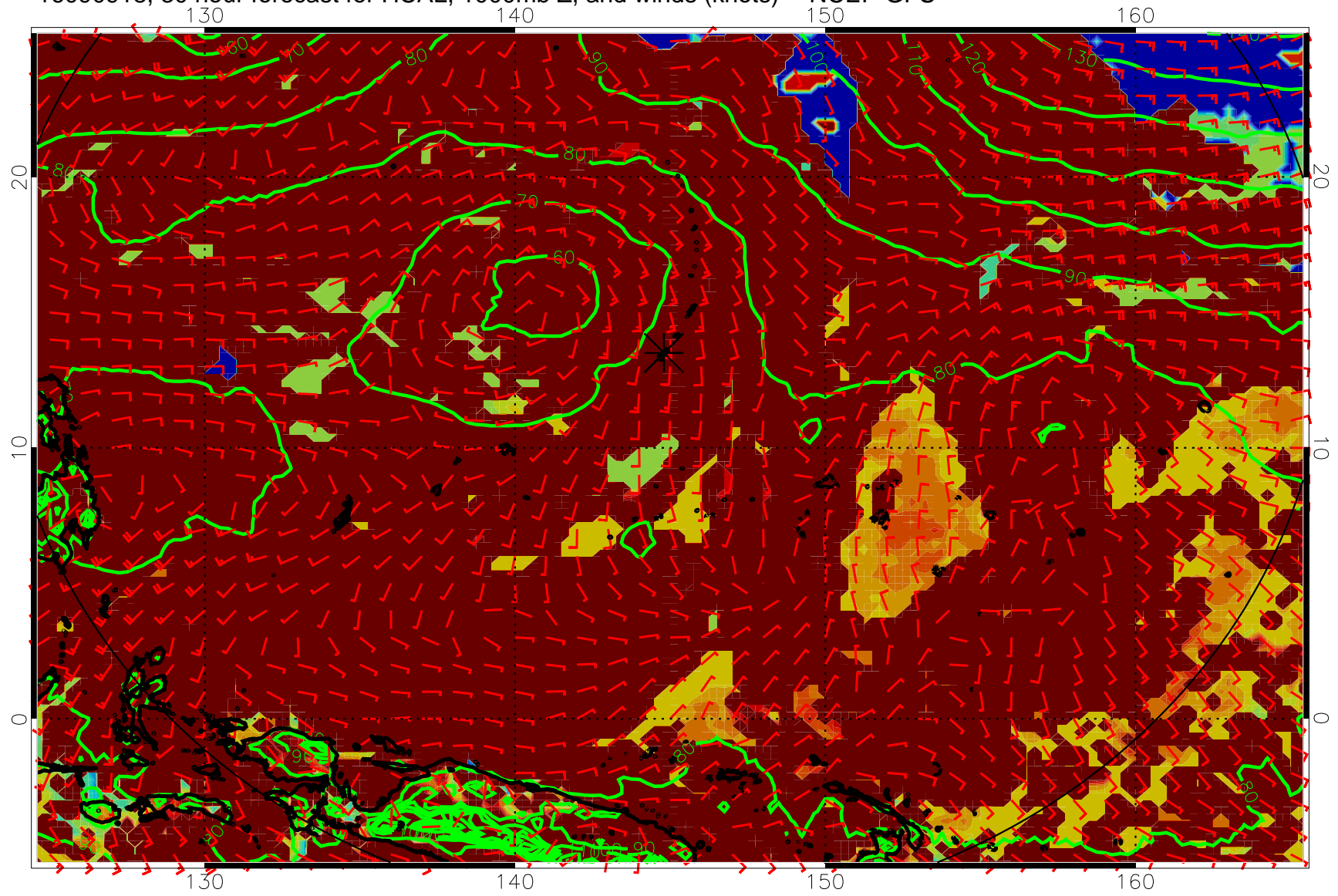
16090918, 30 hour forecast for HCAL, 1000mb Z, and winds (knots) -- NCEP GFS
