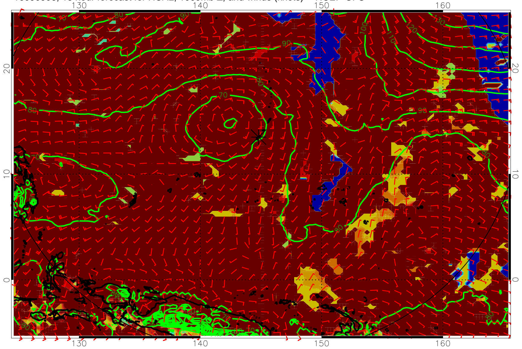
16090906, 18 hour forecast for HCAL, 1000mb Z, and winds (knots) -- NCEP GFS
