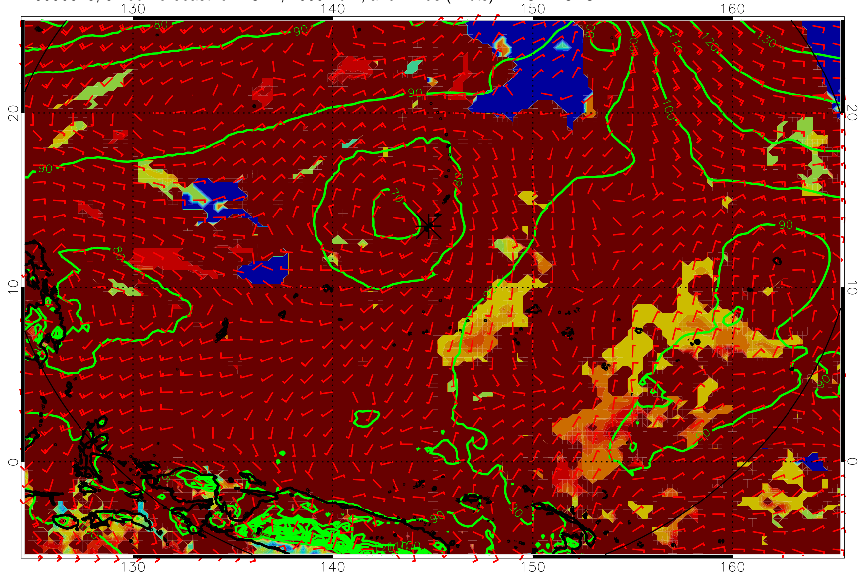
16090818, 6 hour forecast for HCAL, 1000mb Z, and winds (knots) -- NCEP GFS
