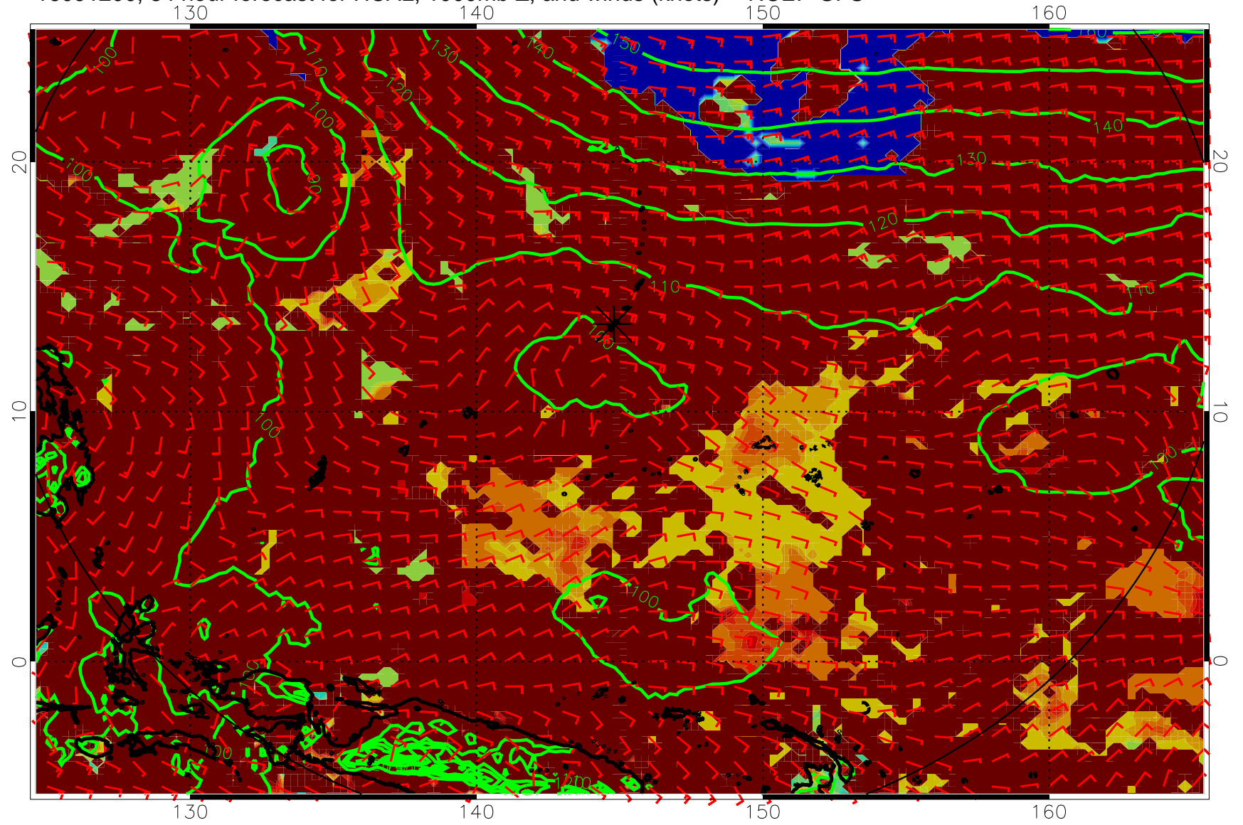
16091200, 84 hour forecast for HCAL, 1000mb Z, and winds (knots) -- NCEP GFS
