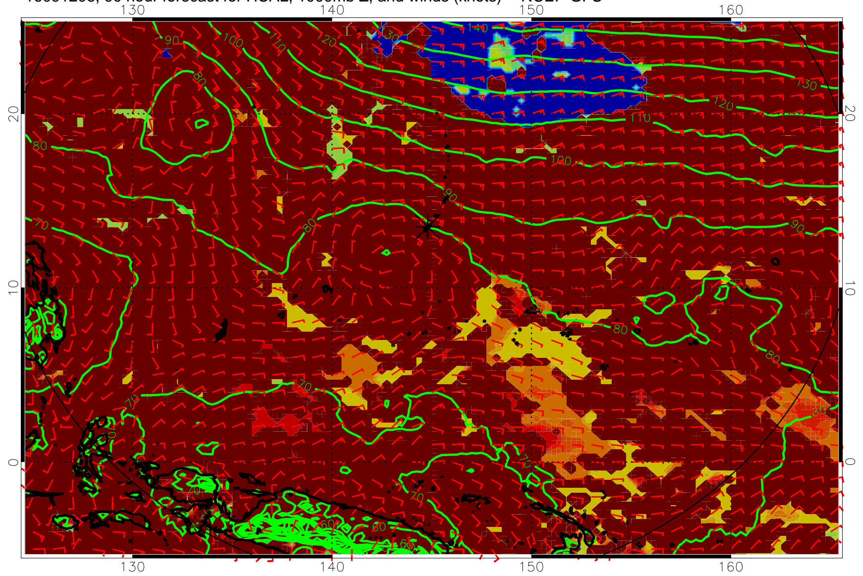
16091206, 90 hour forecast for HCAL, 1000mb Z, and winds (knots) -- NCEP GFS
