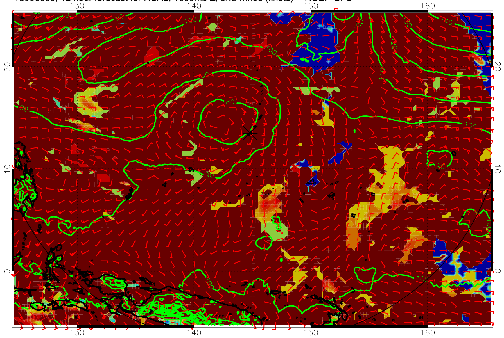
16090900, 12 hour forecast for HCAL, 1000mb Z, and winds (knots) -- NCEP GFS
