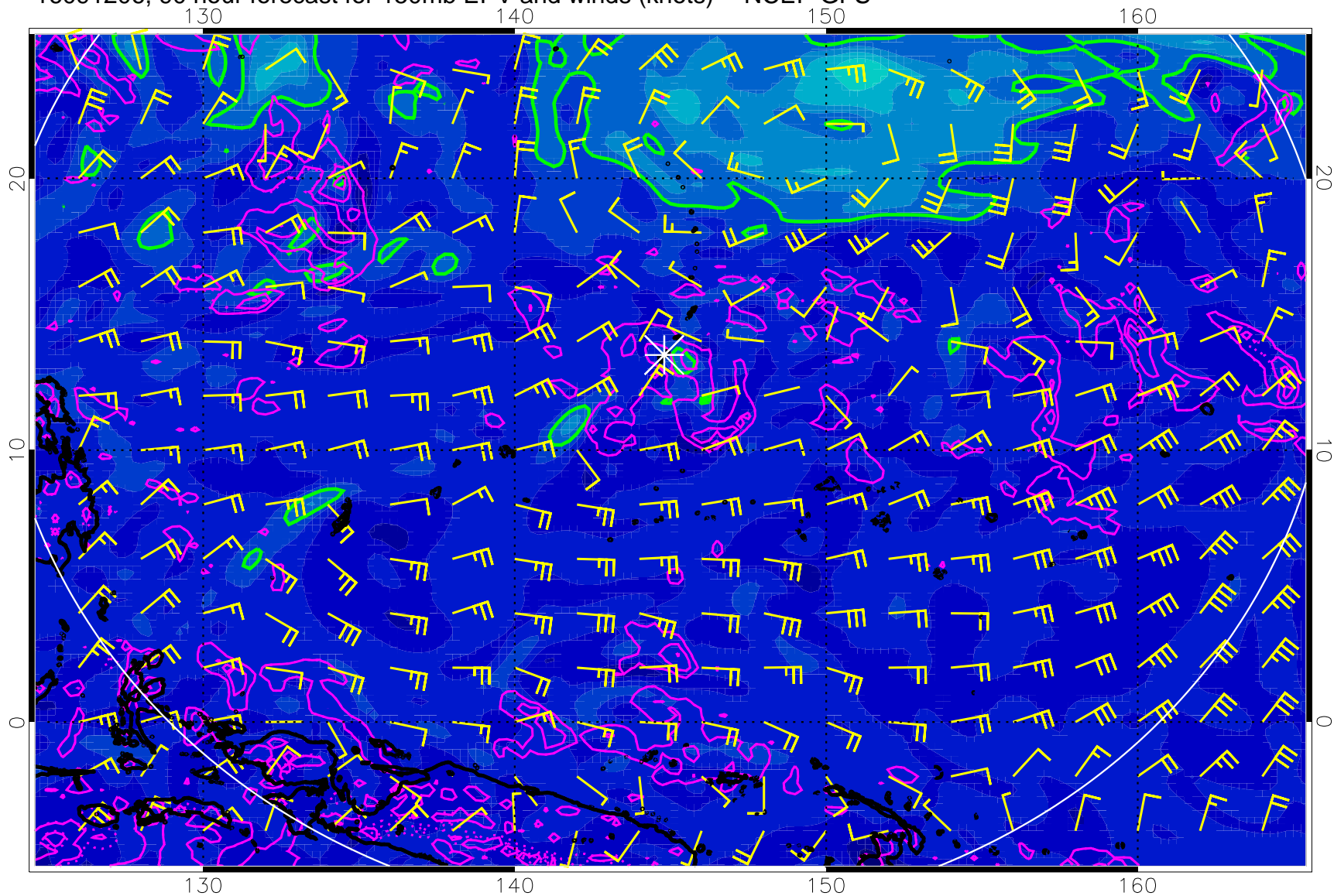
16091206, 90 hour forecast for 150mb EPV and winds (knots) -- NCEP GFS
