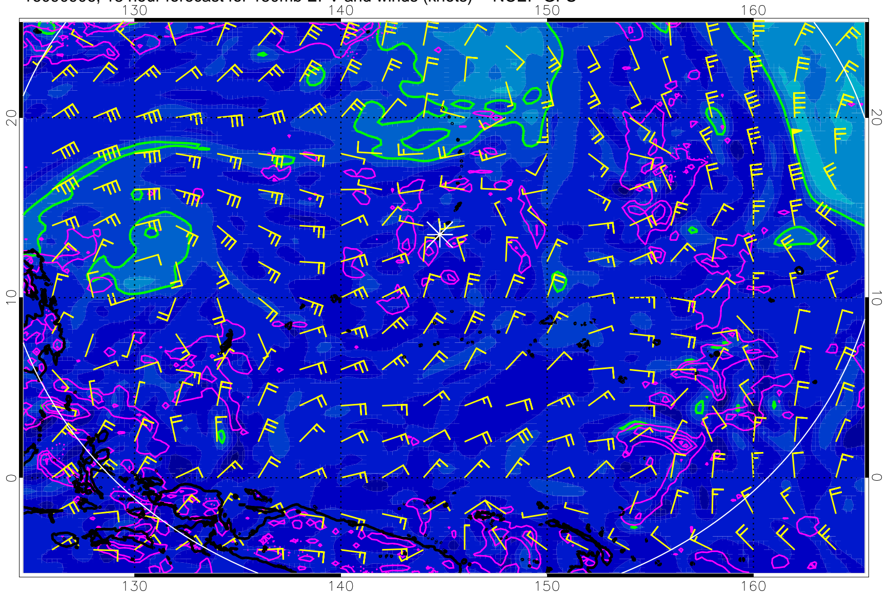
16090906, 18 hour forecast for 150mb EPV and winds (knots) -- NCEP GFS
