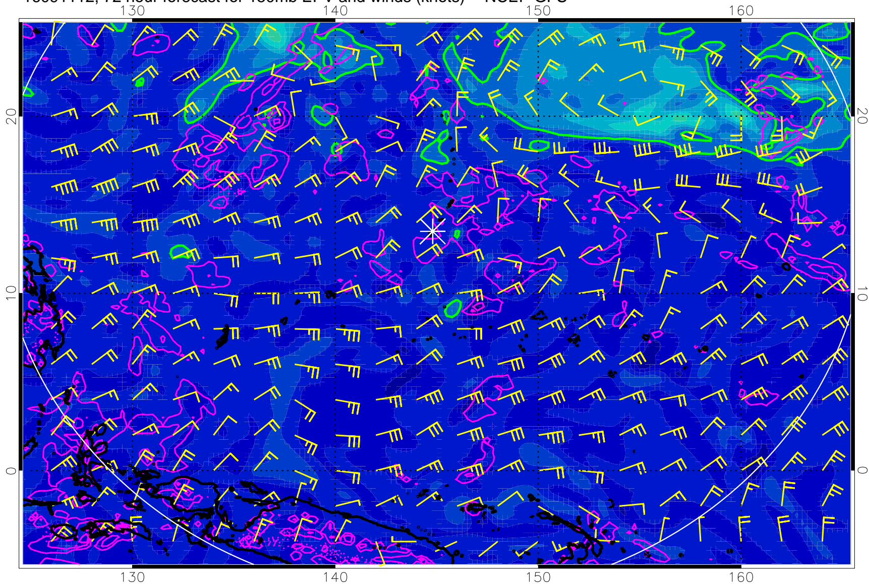
16091112, 72 hour forecast for 150mb EPV and winds (knots) -- NCEP GFS
