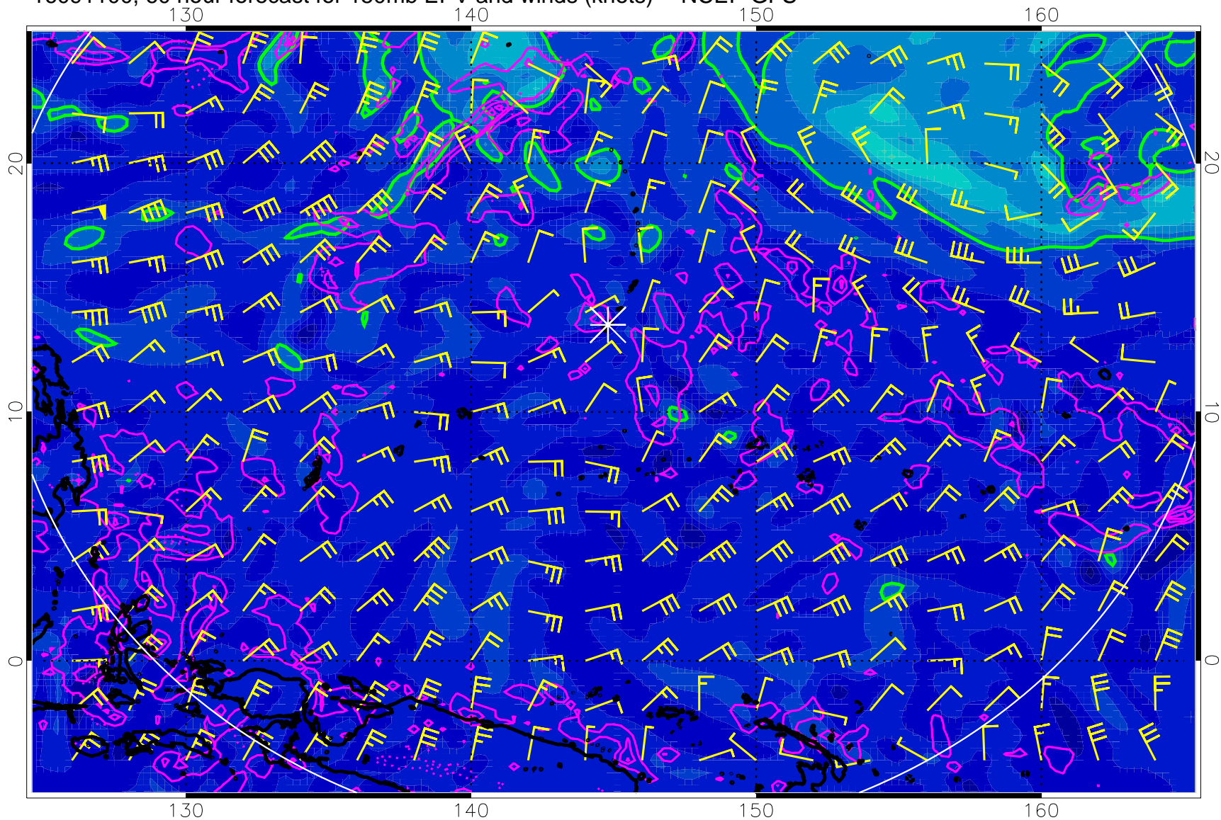
16091100, 60 hour forecast for 150mb EPV and winds (knots) -- NCEP GFS
