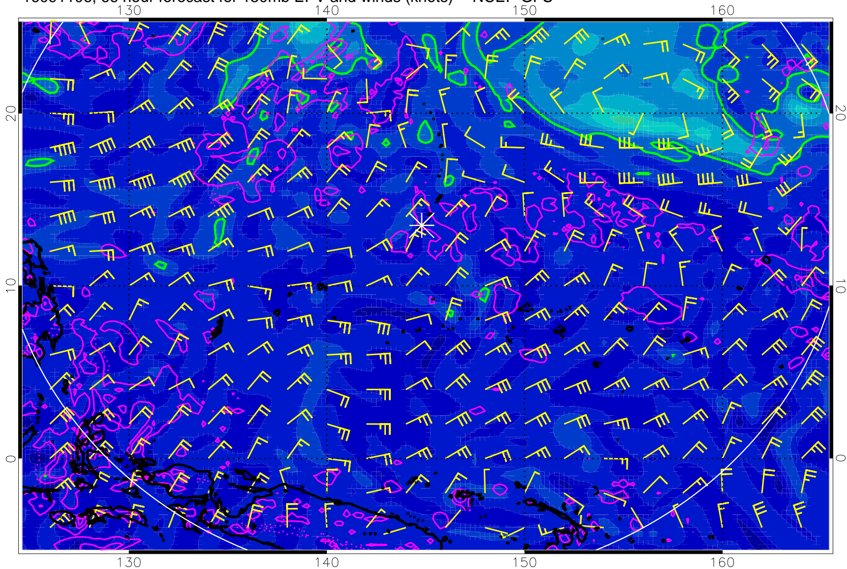
16091106, 66 hour forecast for 150mb EPV and winds (knots) -- NCEP GFS
