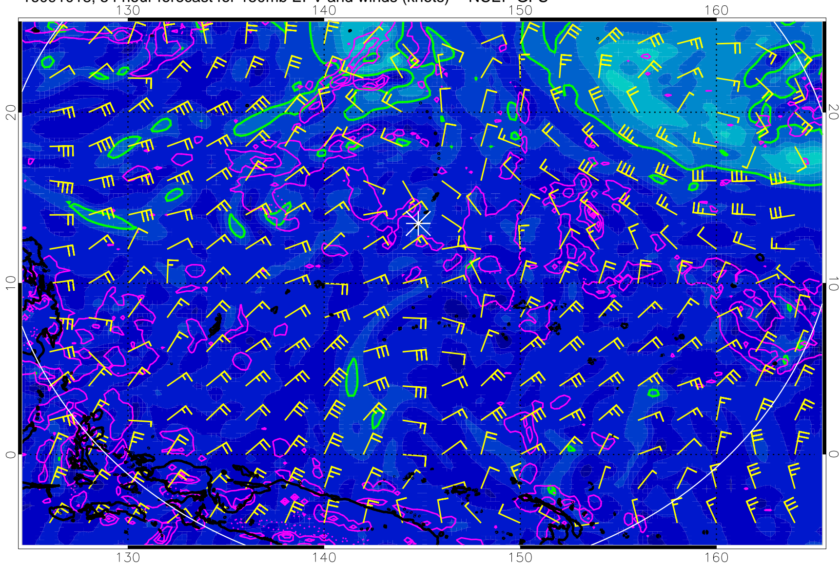
16091018, 54 hour forecast for 150mb EPV and winds (knots) -- NCEP GFS
