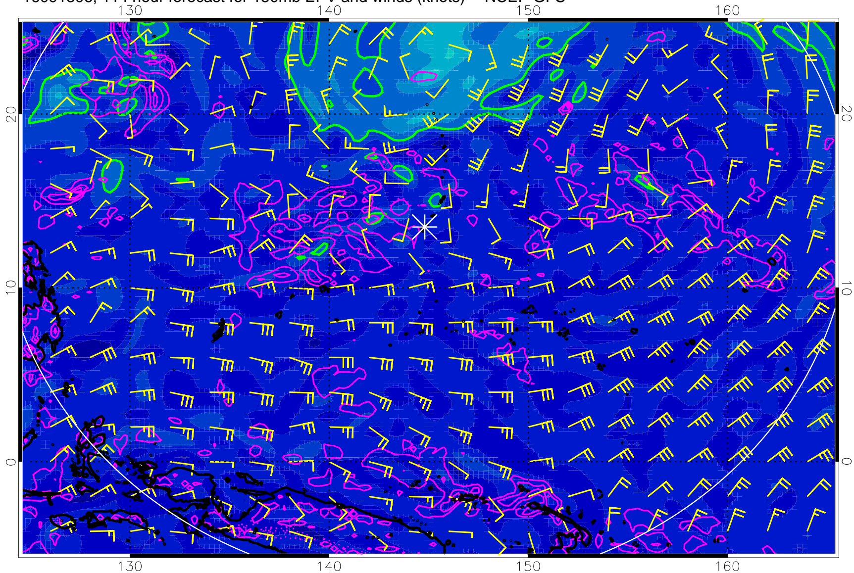
16091306, 114 hour forecast for 150mb EPV and winds (knots) -- NCEP GFS
