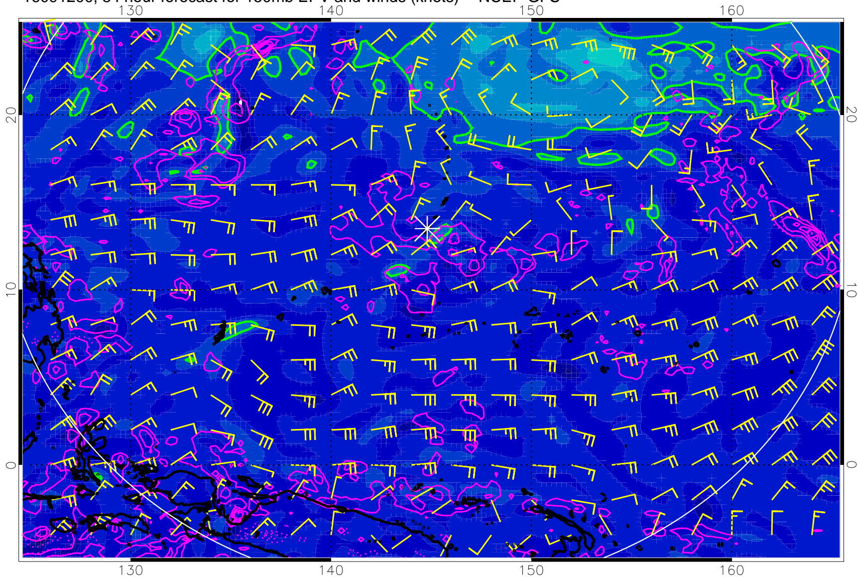
16091200, 84 hour forecast for 150mb EPV and winds (knots) -- NCEP GFS
