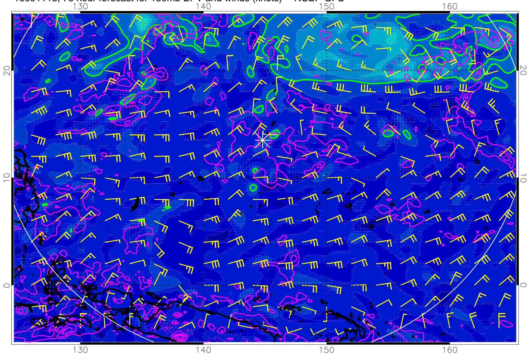
16091118, 78 hour forecast for 150mb EPV and winds (knots) -- NCEP GFS
