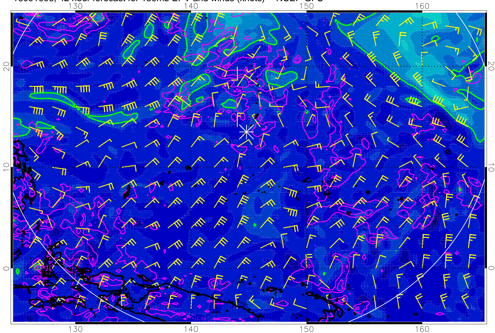
16091006, 42 hour forecast for 150mb EPV and winds (knots) -- NCEP GFS
