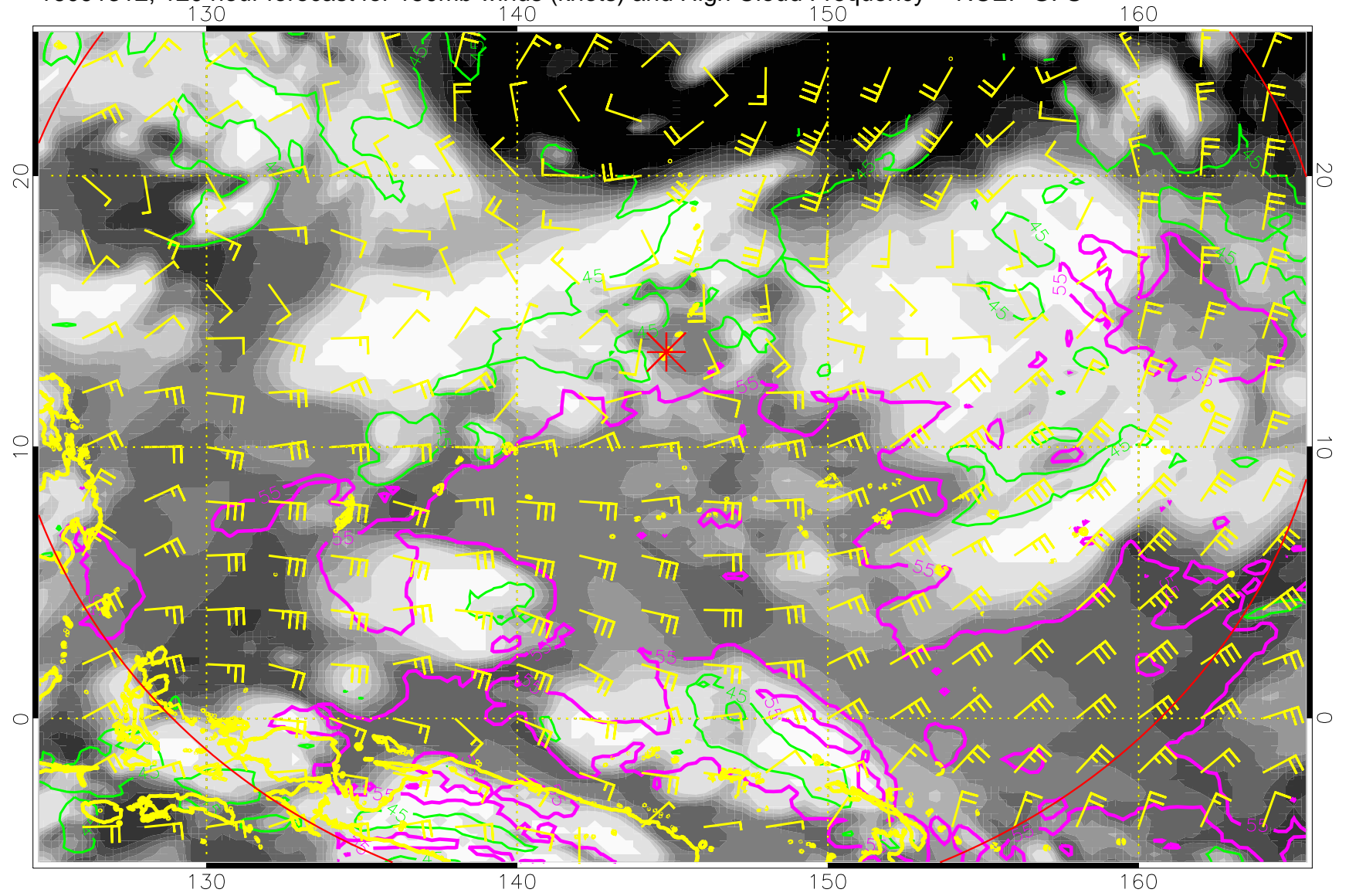
16091312, 120 hour forecast for 150mb winds (knots) and High Cloud Frequency -- NCEP GFS
