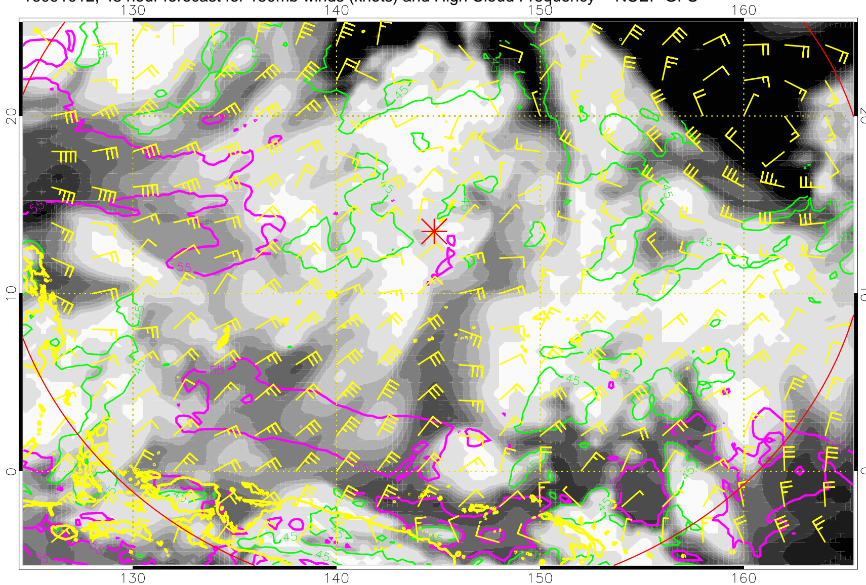
16091012, 48 hour forecast for 150mb winds (knots) and High Cloud Frequency -- NCEP GFS
