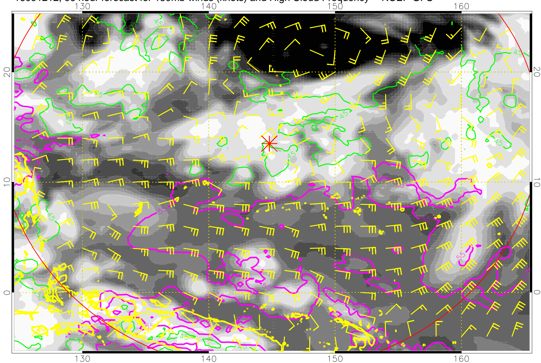
16091212, 96 hour forecast for 150mb winds (knots) and High Cloud Frequency -- NCEP GFS
