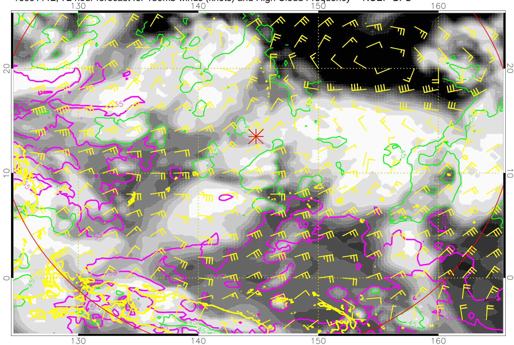
16091112, 72 hour forecast for 150mb winds (knots) and High Cloud Frequency -- NCEP GFS
