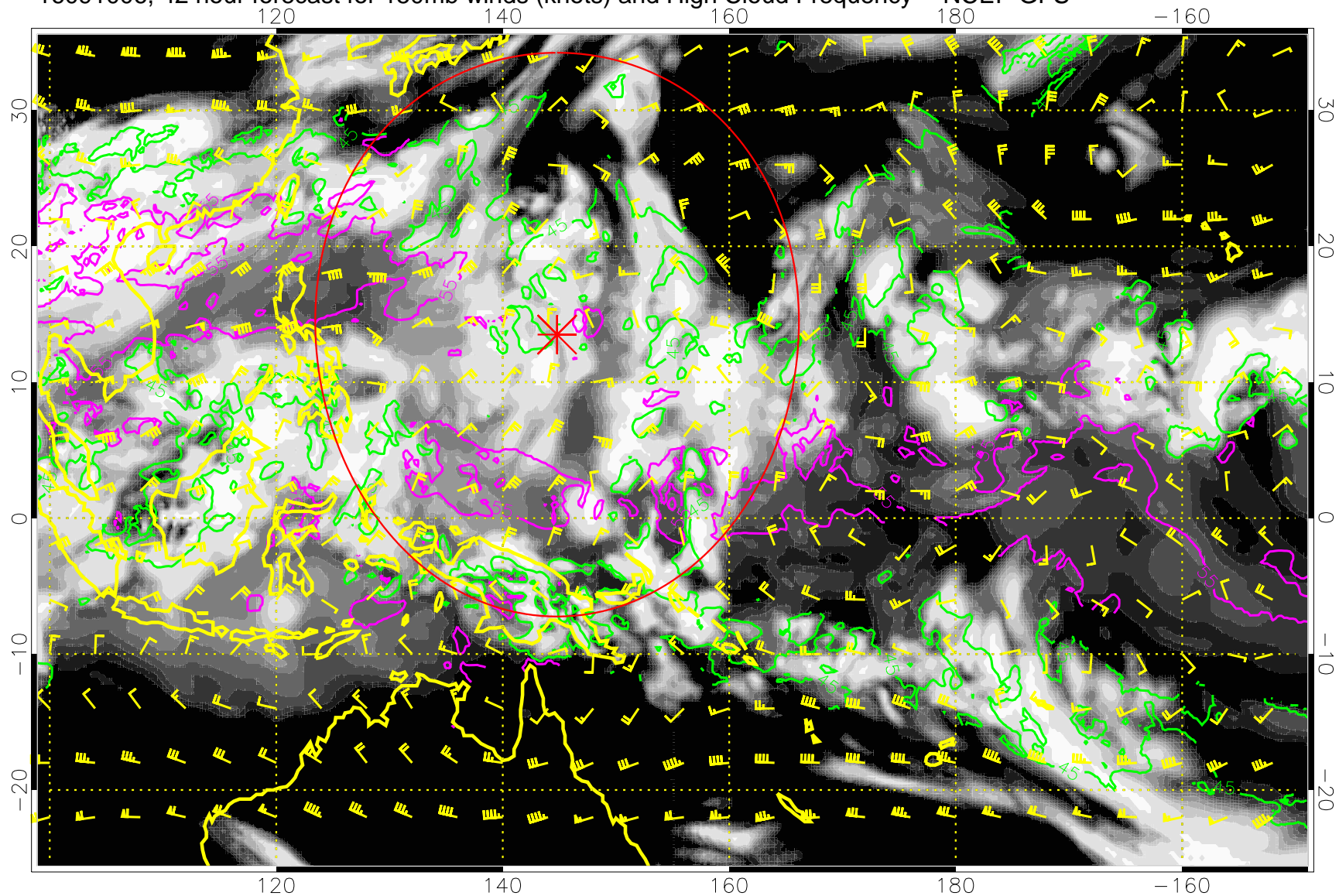
16091006, 42 hour forecast for 150mb winds (knots) and High Cloud Frequency -- NCEP GFS
