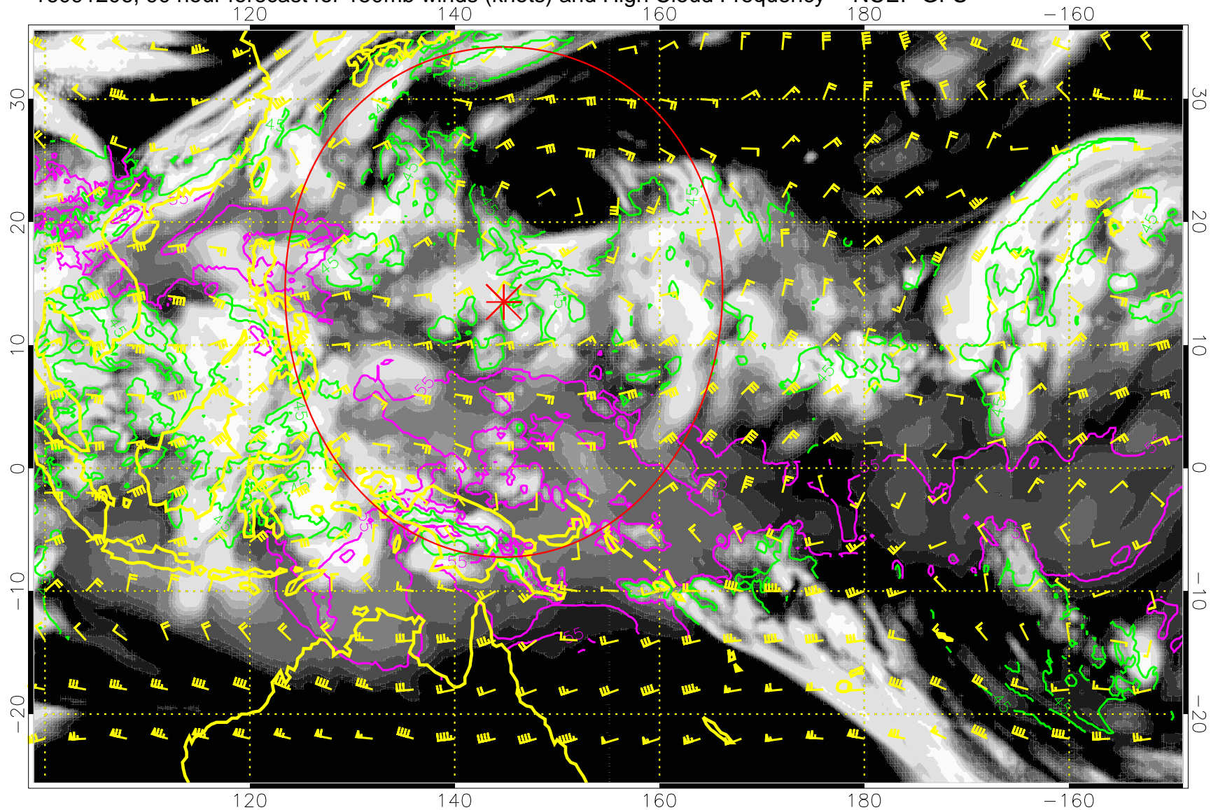
16091206, 90 hour forecast for 150mb winds (knots) and High Cloud Frequency -- NCEP GFS
