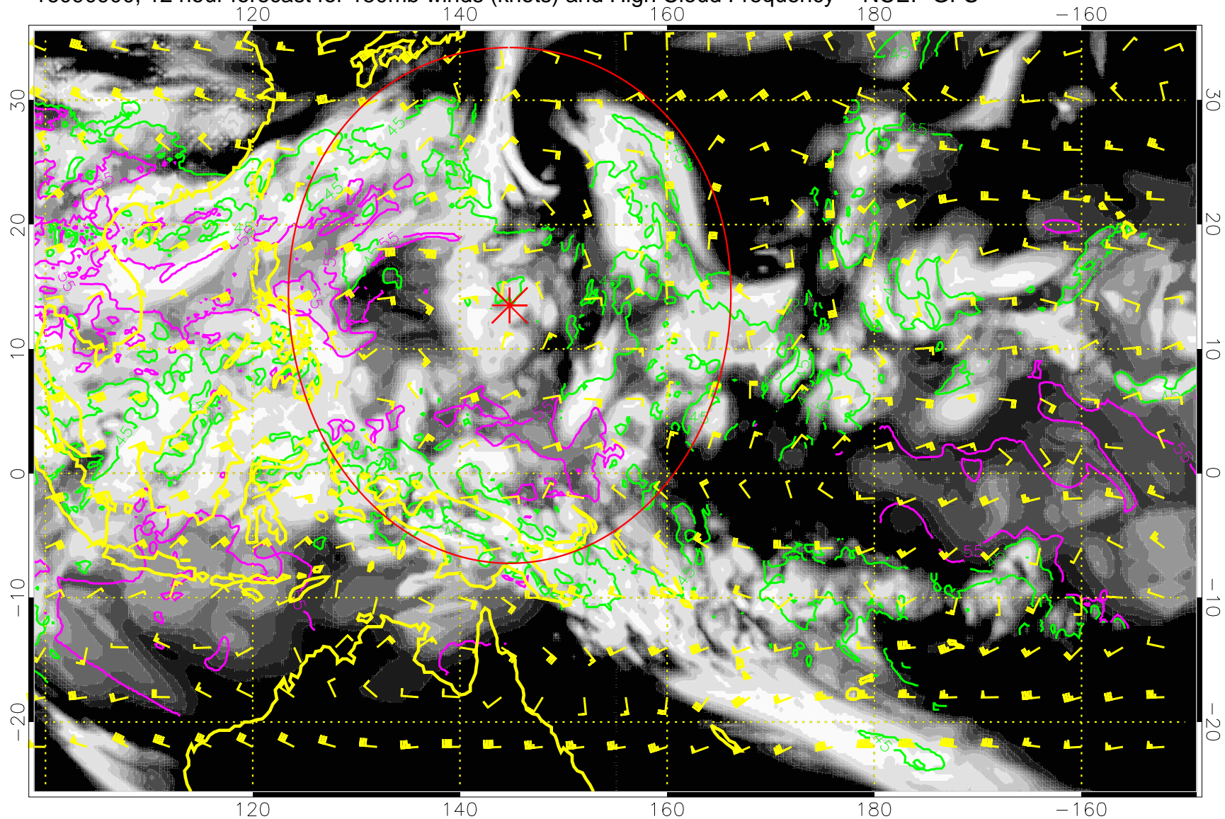
16090900, 12 hour forecast for 150mb winds (knots) and High Cloud Frequency -- NCEP GFS
