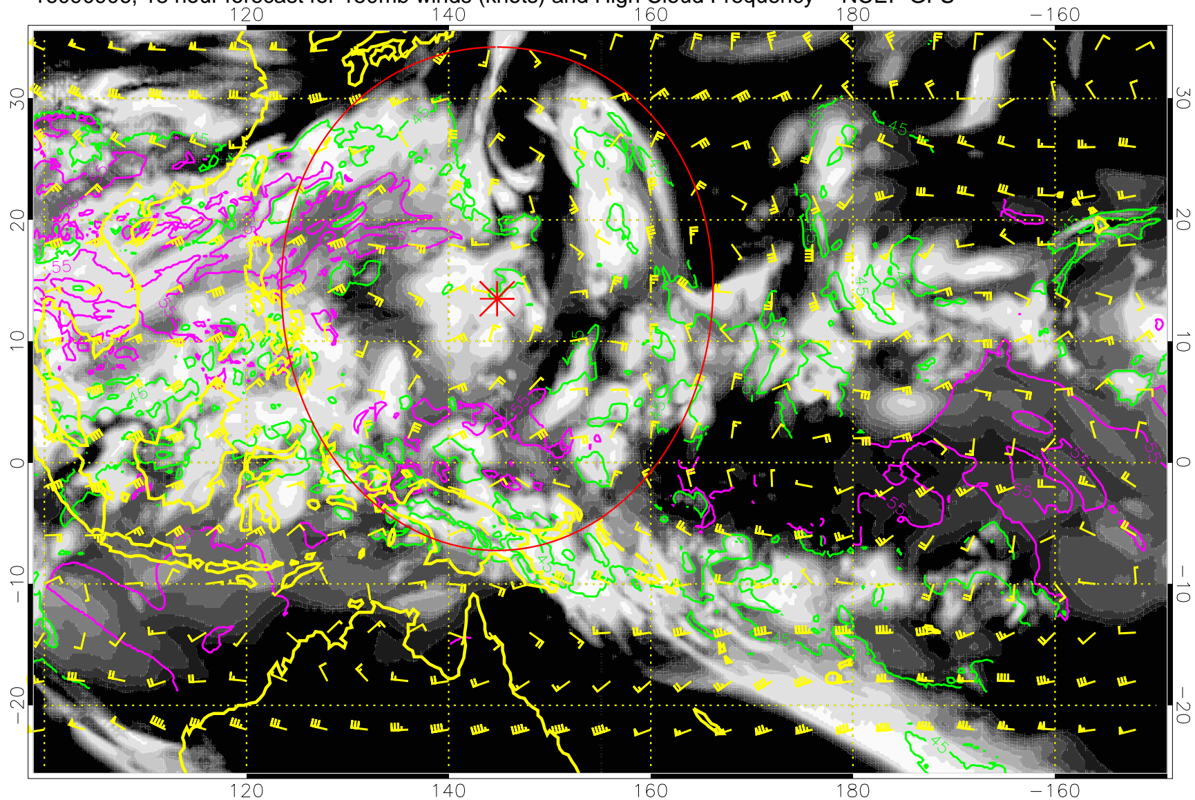
16090906, 18 hour forecast for 150mb winds (knots) and High Cloud Frequency -- NCEP GFS
