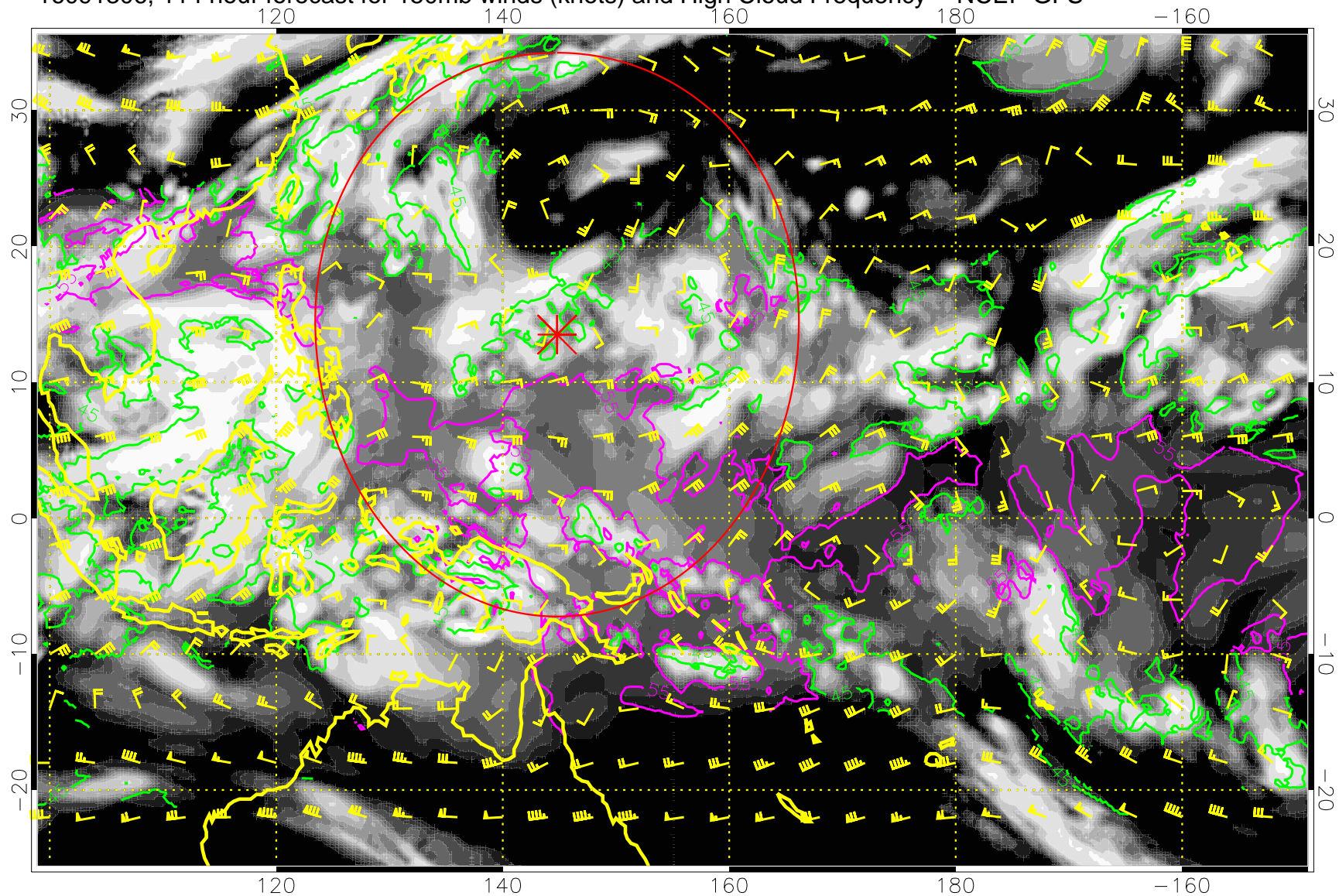
16091306, 114 hour forecast for 150mb winds (knots) and High Cloud Frequency -- NCEP GFS
