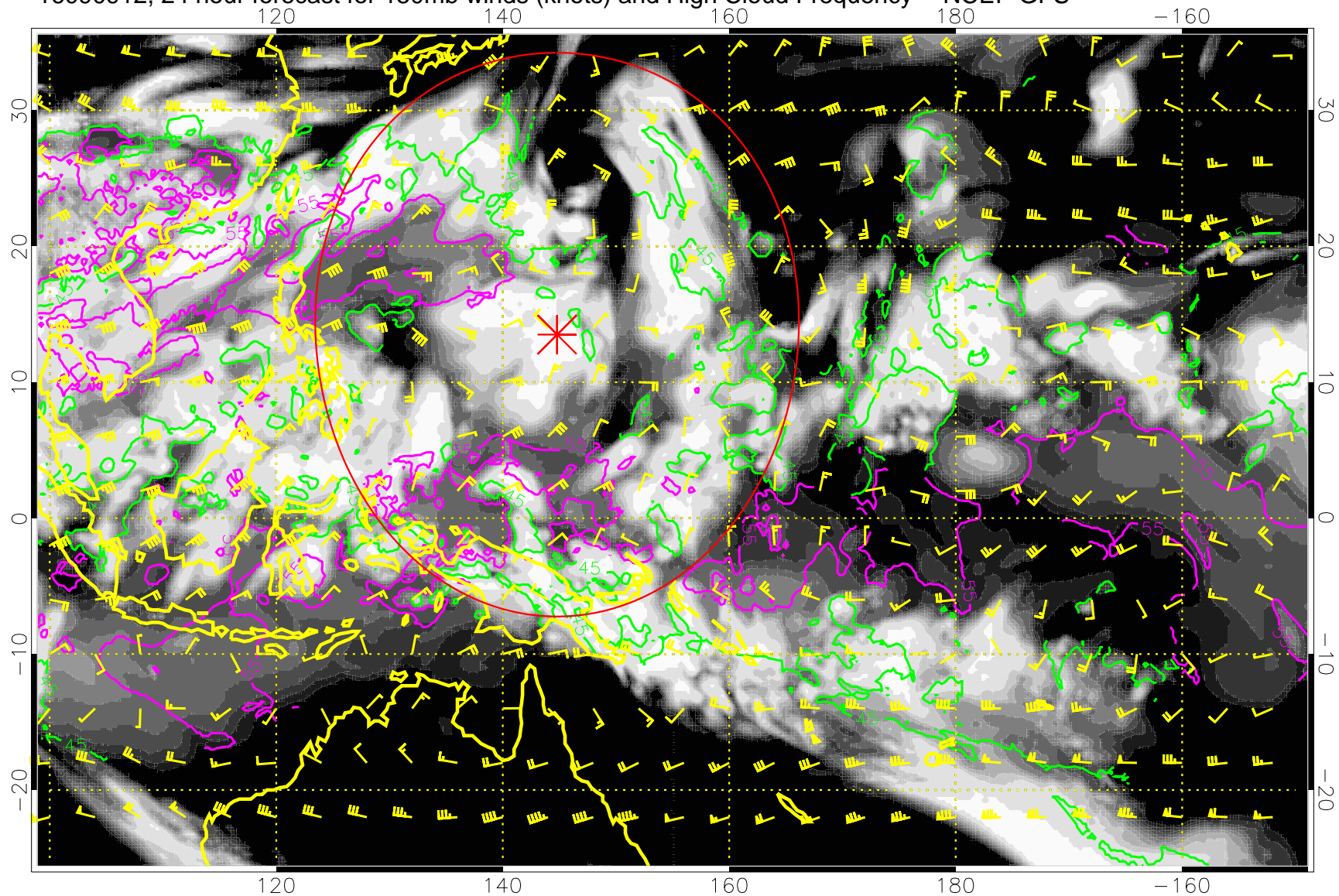
16090912, 24 hour forecast for 150mb winds (knots) and High Cloud Frequency -- NCEP GFS
