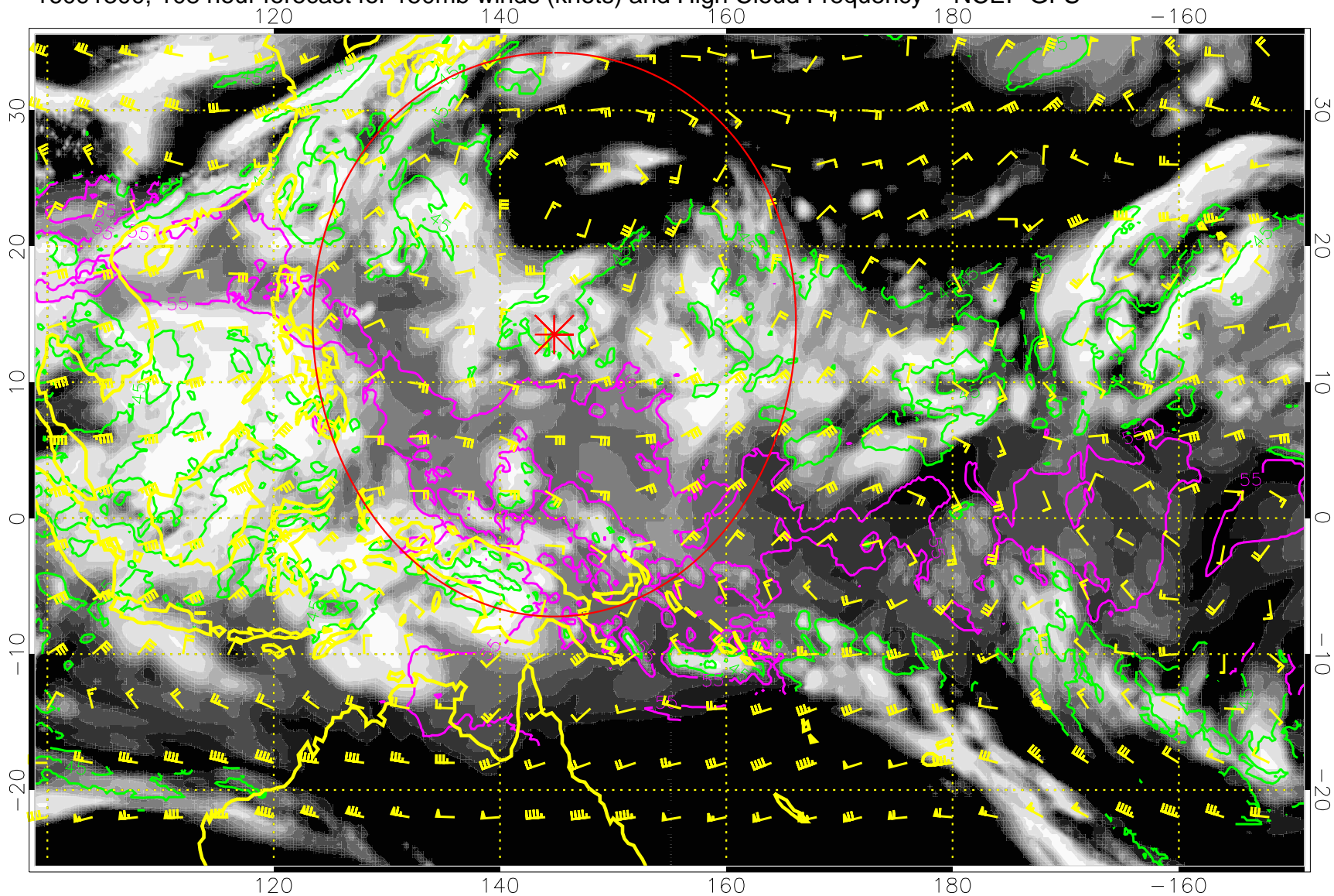
16091300, 108 hour forecast for 150mb winds (knots) and High Cloud Frequency -- NCEP GFS
