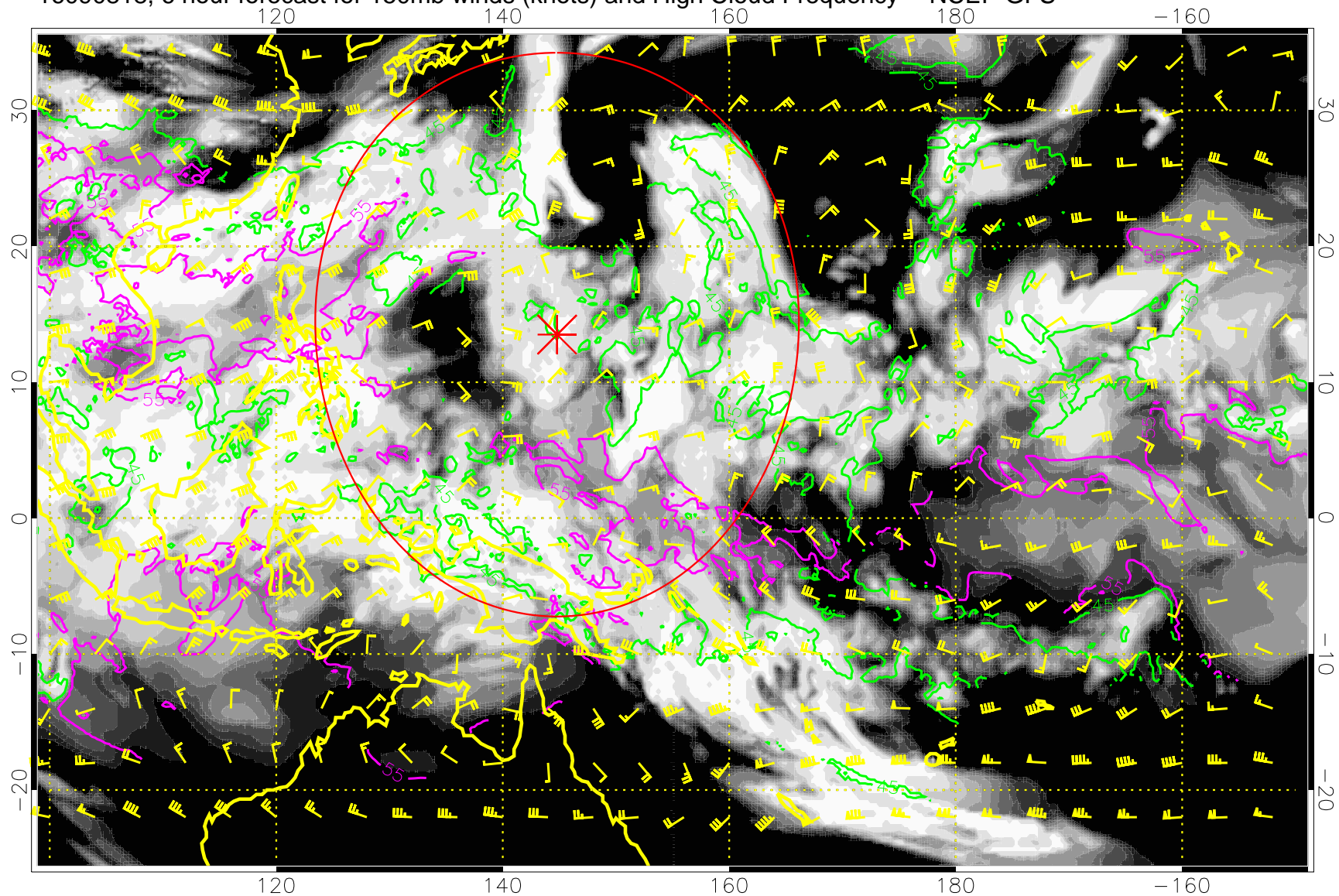
16090818, 6 hour forecast for 150mb winds (knots) and High Cloud Frequency -- NCEP GFS
