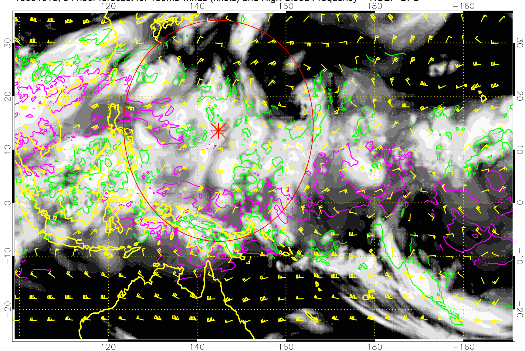
16091018, 54 hour forecast for 150mb winds (knots) and High Cloud Frequency -- NCEP GFS
