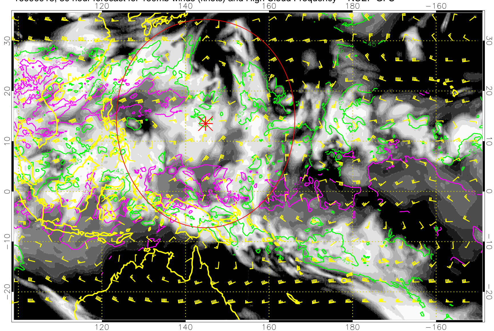
16090918, 30 hour forecast for 150mb winds (knots) and High Cloud Frequency -- NCEP GFS
