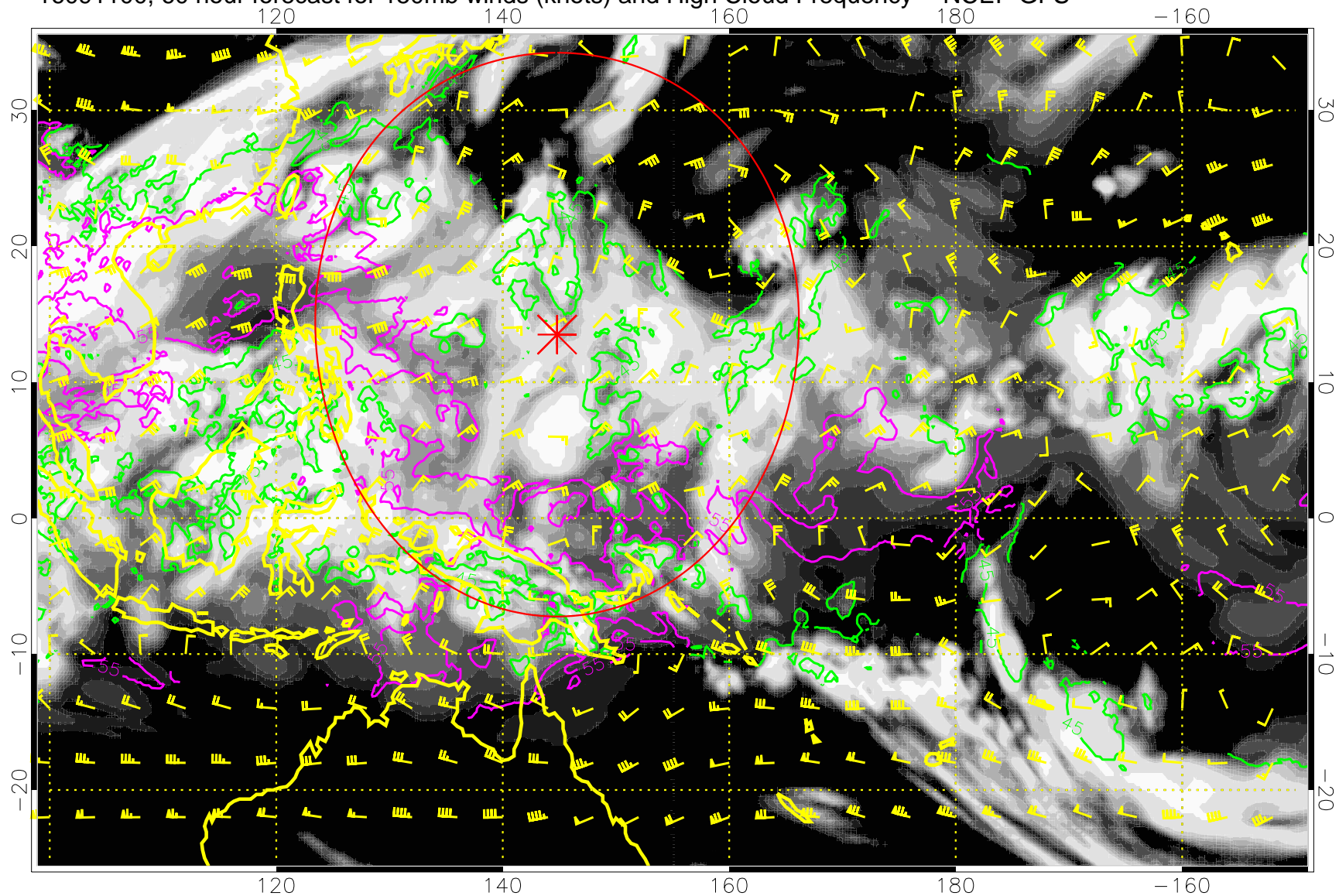
16091100, 60 hour forecast for 150mb winds (knots) and High Cloud Frequency -- NCEP GFS
