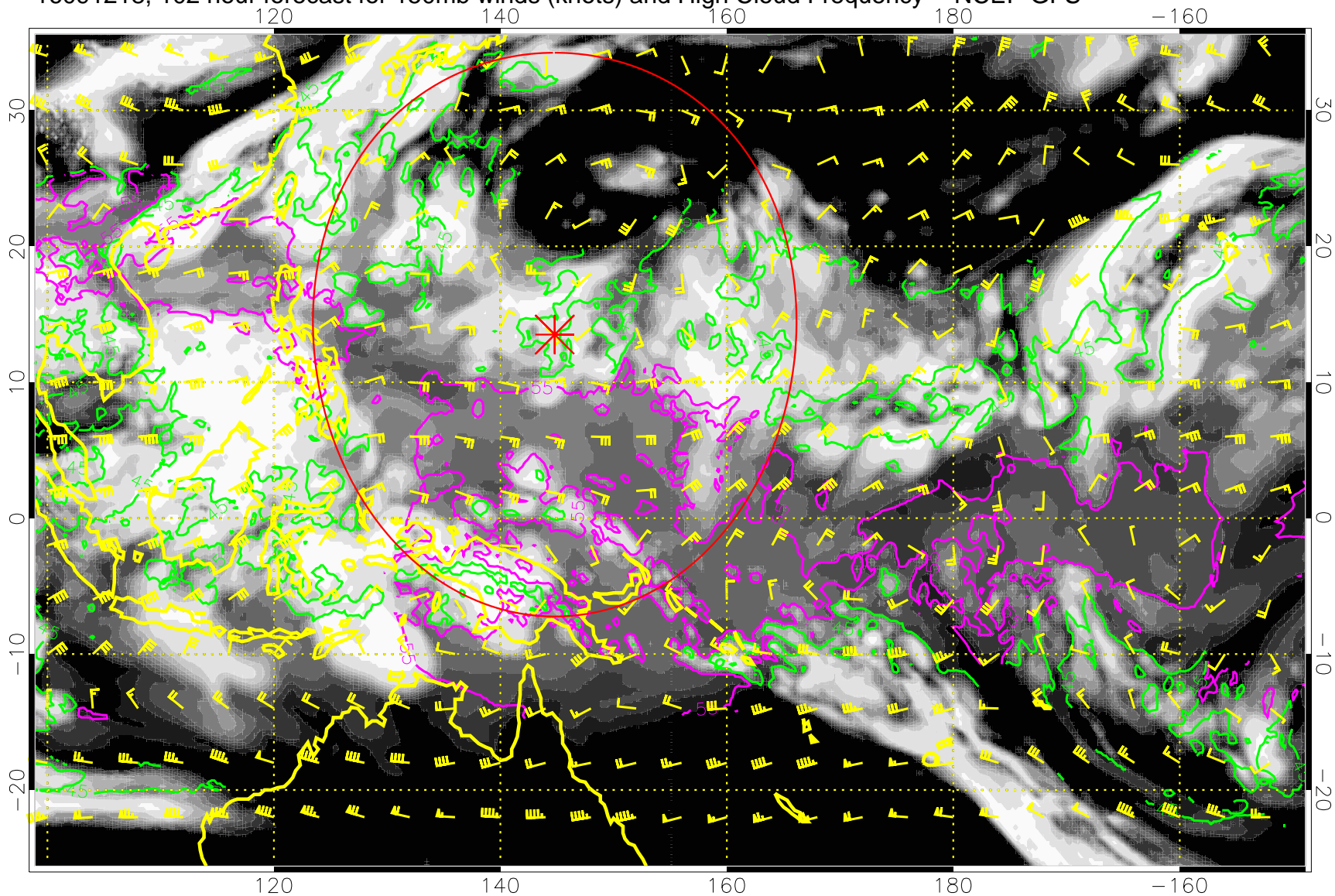
16091218, 102 hour forecast for 150mb winds (knots) and High Cloud Frequency -- NCEP GFS
