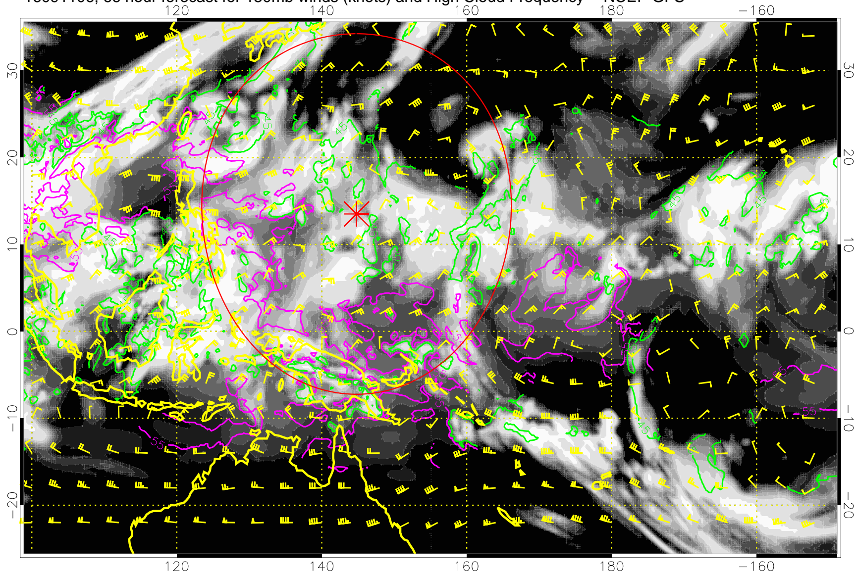
16091106, 66 hour forecast for 150mb winds (knots) and High Cloud Frequency -- NCEP GFS
