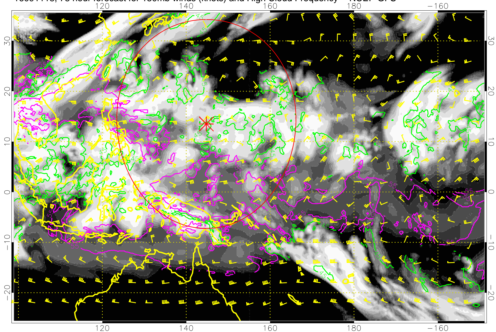
16091118, 78 hour forecast for 150mb winds (knots) and High Cloud Frequency -- NCEP GFS
