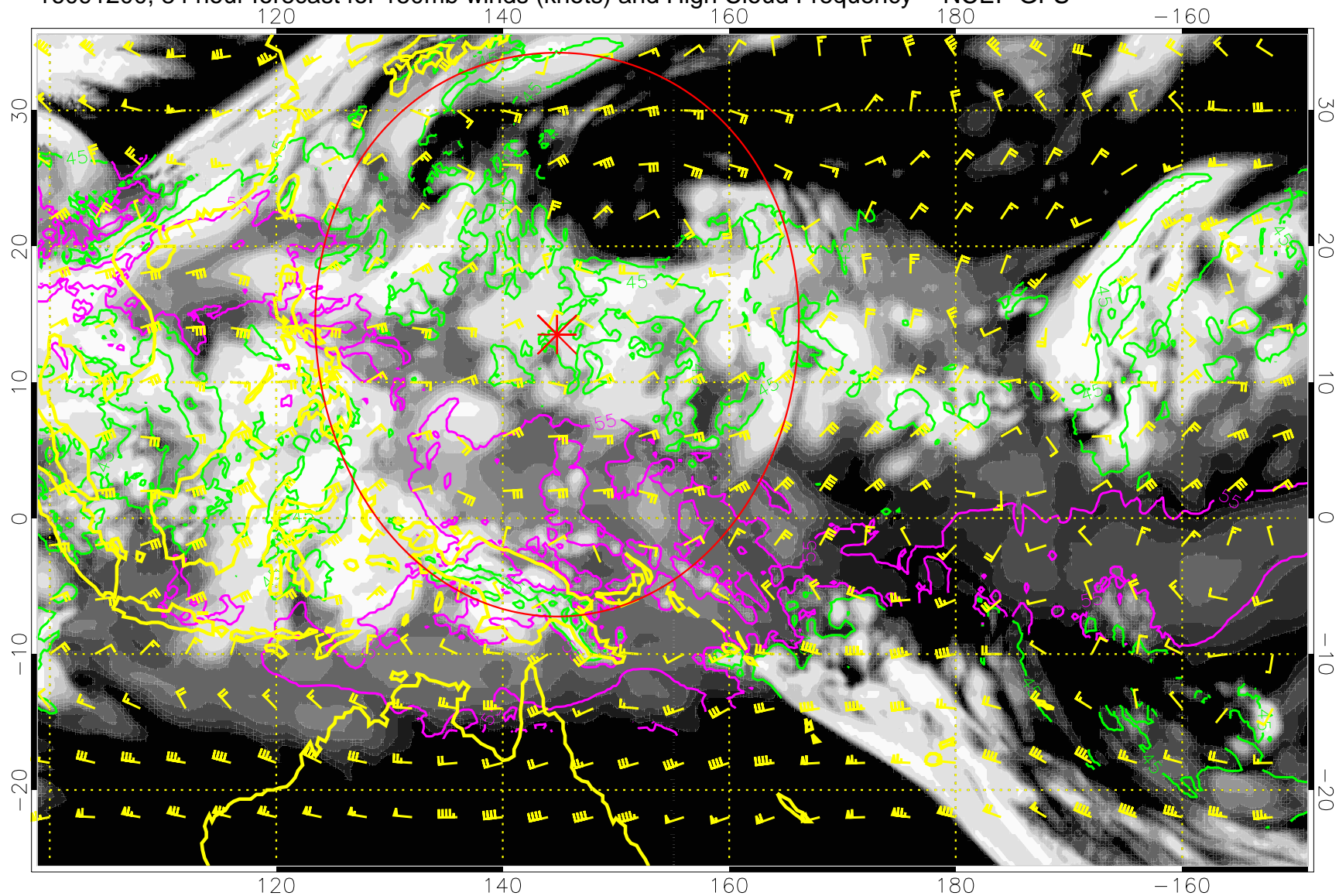
16091200, 84 hour forecast for 150mb winds (knots) and High Cloud Frequency -- NCEP GFS
