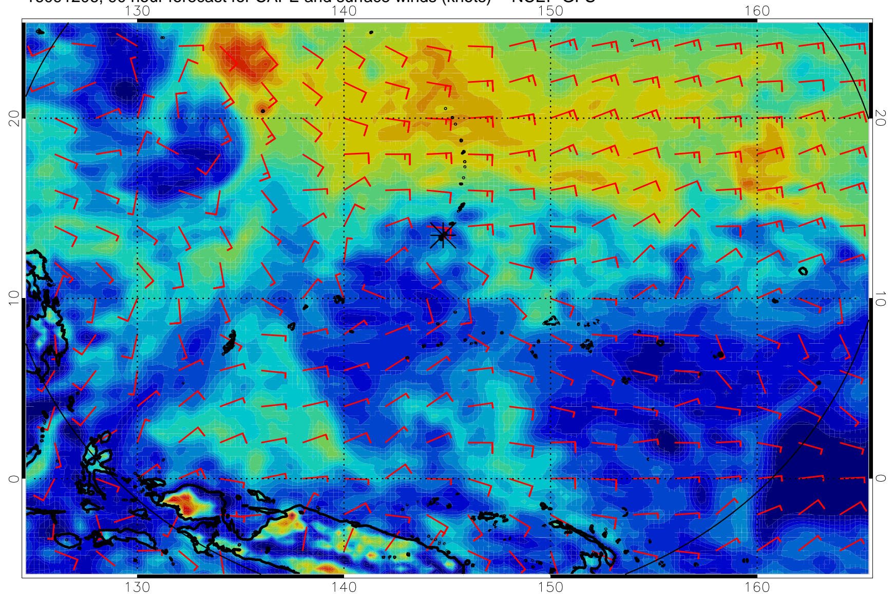
16091206, 90 hour forecast for CAPE and surface winds (knots) -- NCEP GFS
