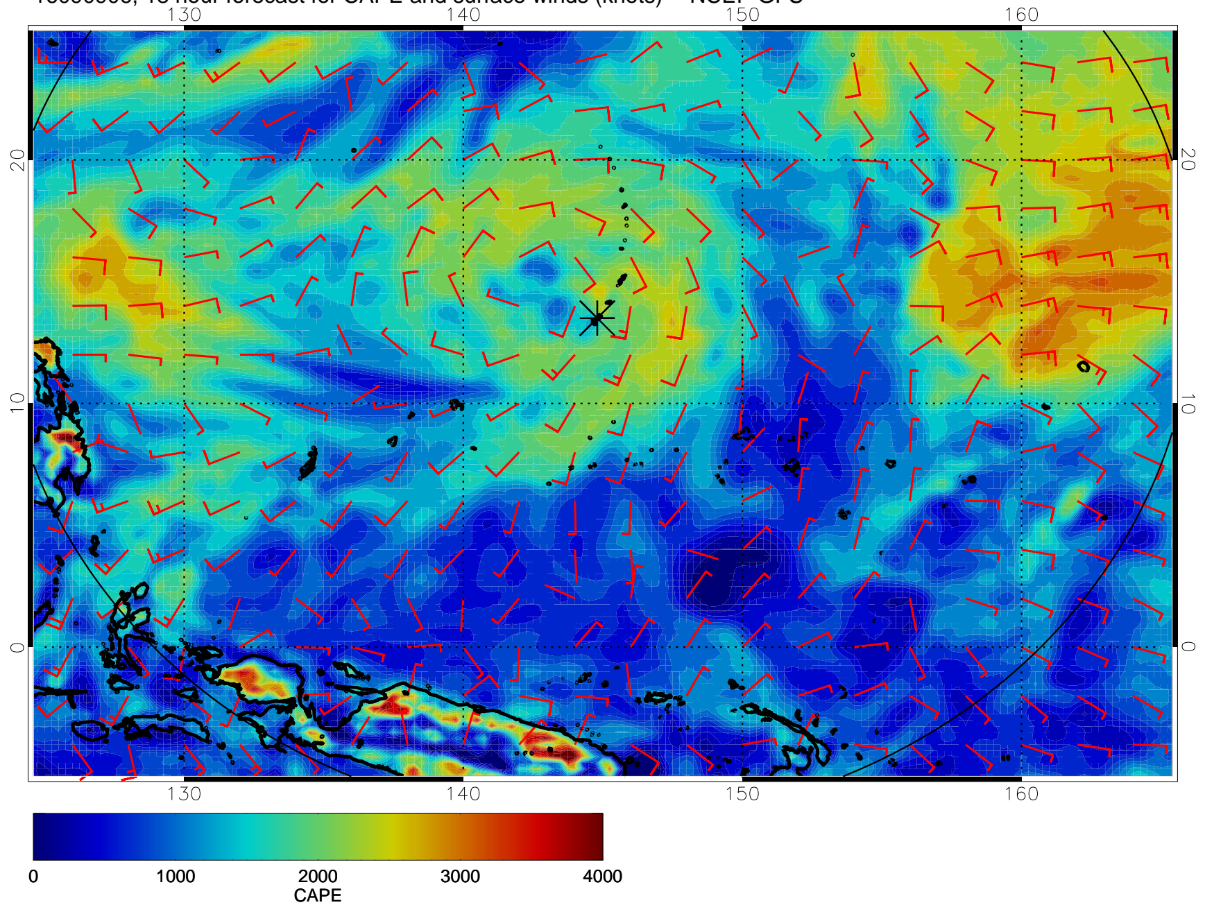
16090906, 18 hour forecast for CAPE and surface winds (knots) -- NCEP GFS
