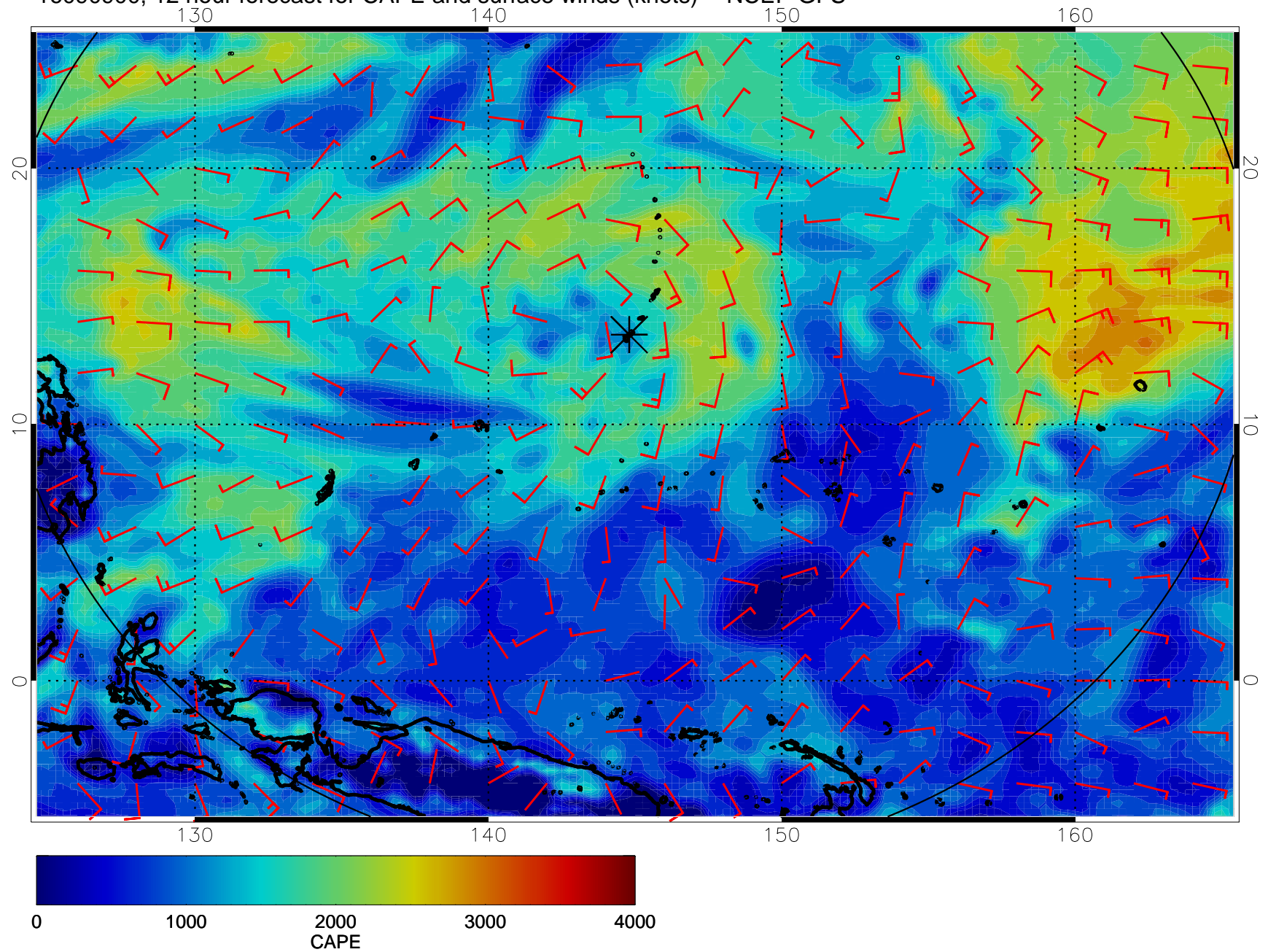
16090900, 12 hour forecast for CAPE and surface winds (knots) -- NCEP GFS
