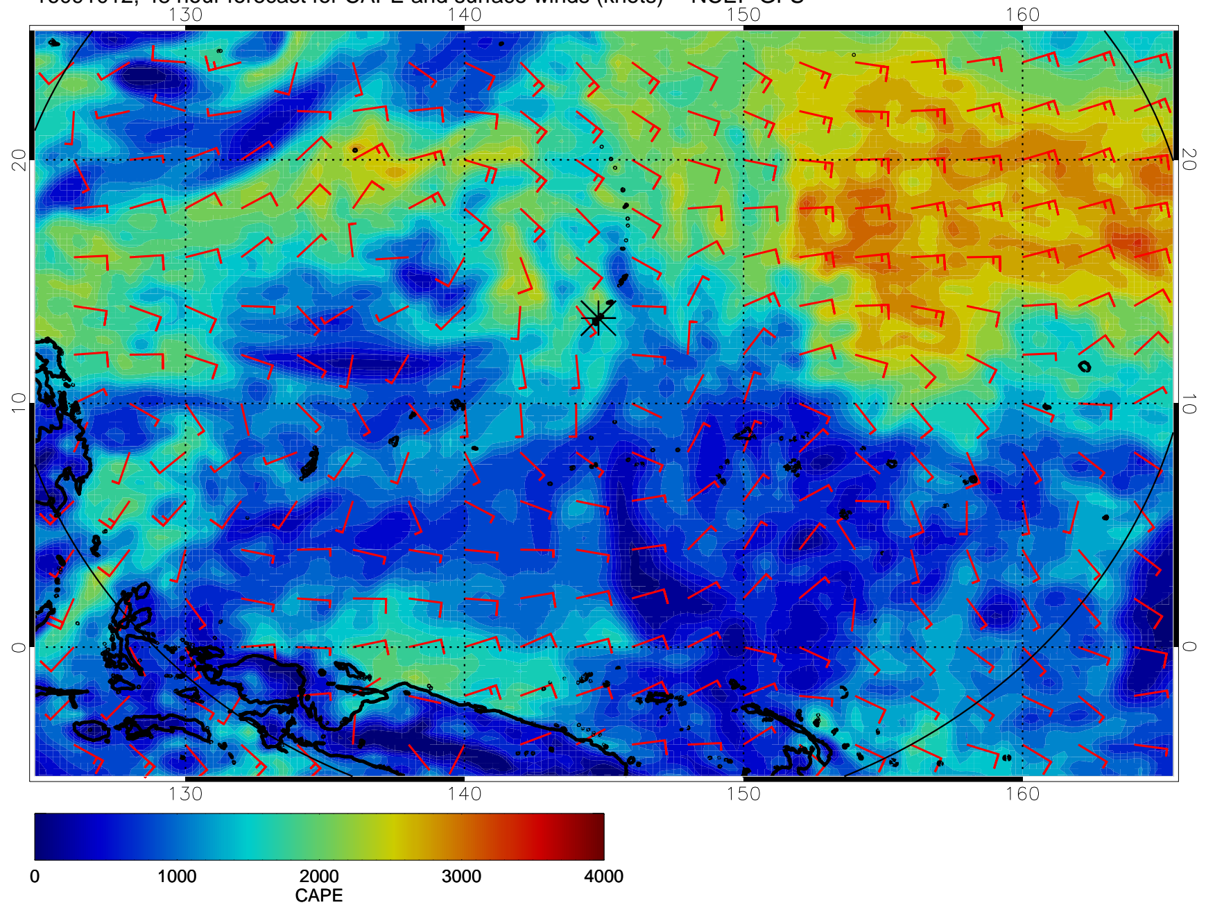
16091012, 48 hour forecast for CAPE and surface winds (knots) -- NCEP GFS
