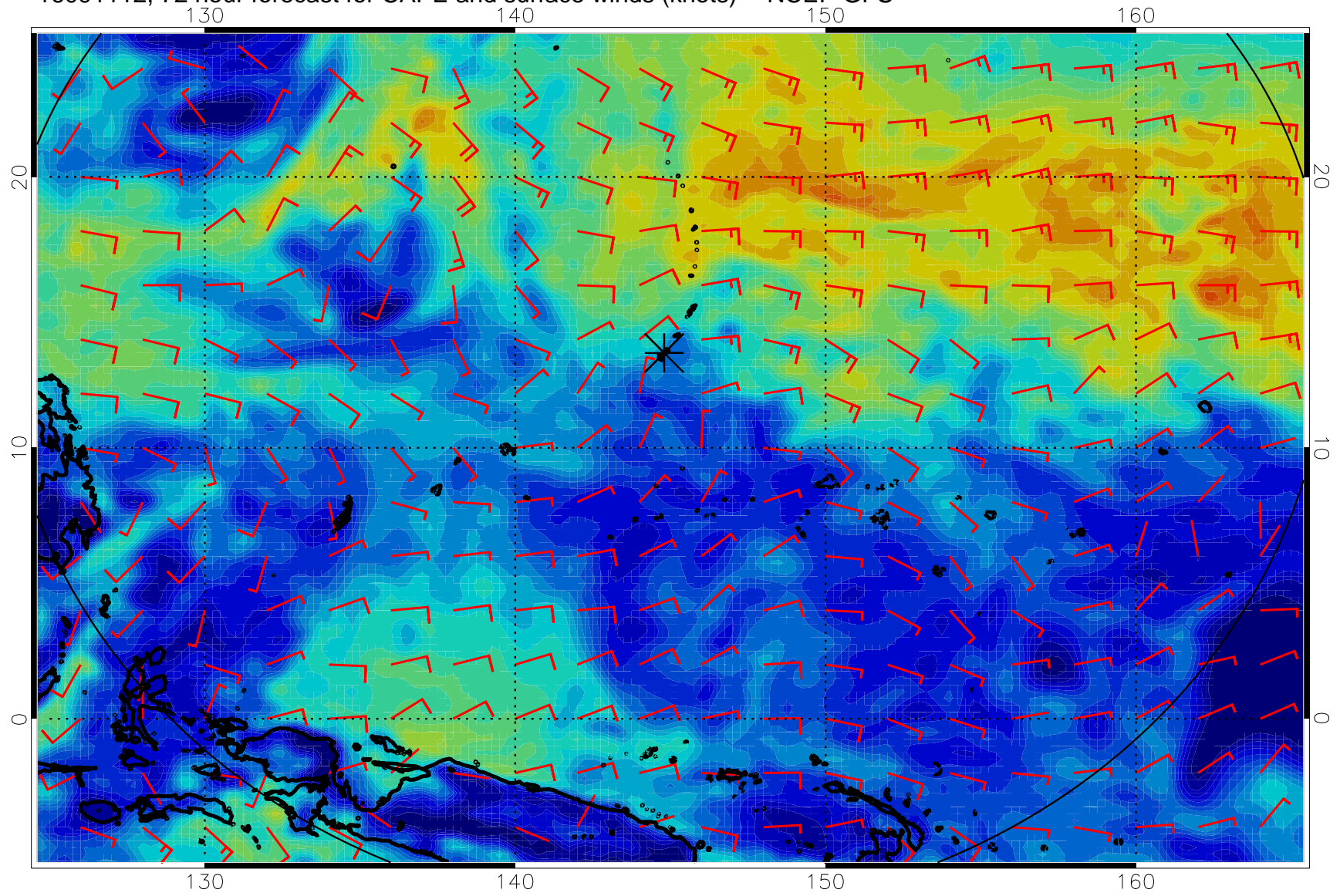
16091112, 72 hour forecast for CAPE and surface winds (knots) -- NCEP GFS
