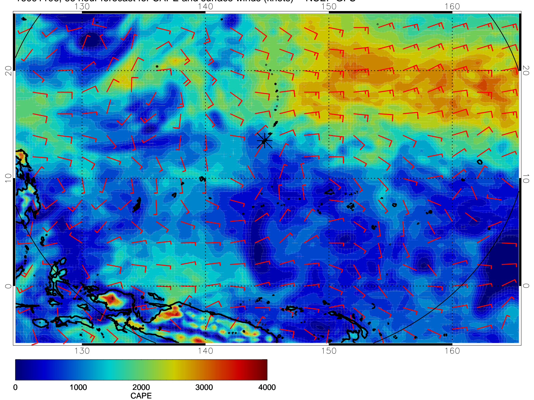
16091106, 66 hour forecast for CAPE and surface winds (knots) -- NCEP GFS
