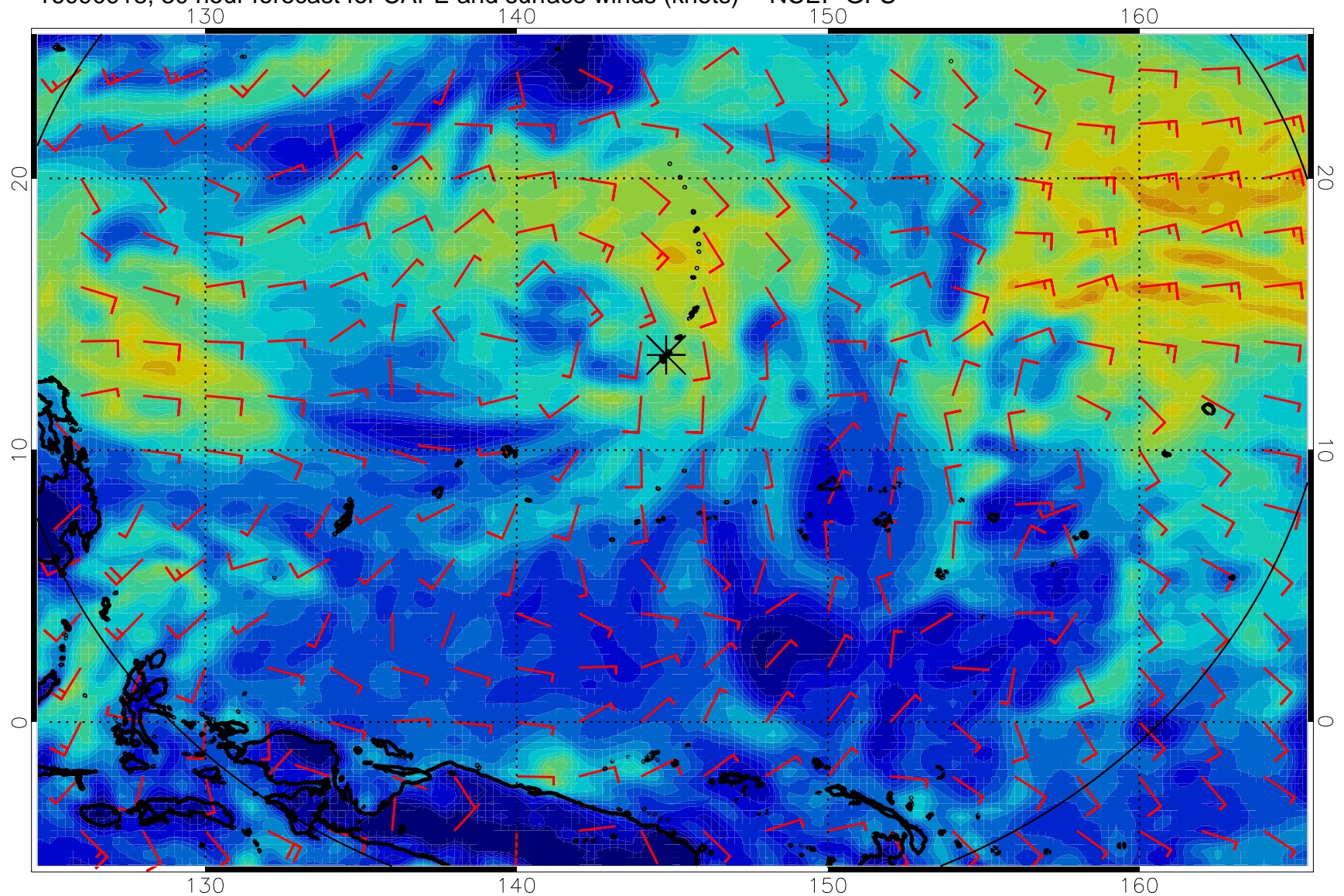
16090918, 30 hour forecast for CAPE and surface winds (knots) -- NCEP GFS
