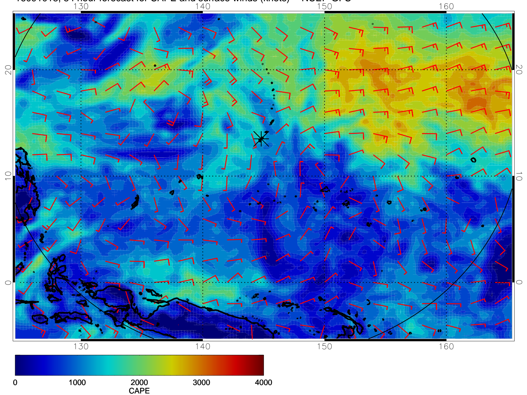
16091018, 54 hour forecast for CAPE and surface winds (knots) -- NCEP GFS
