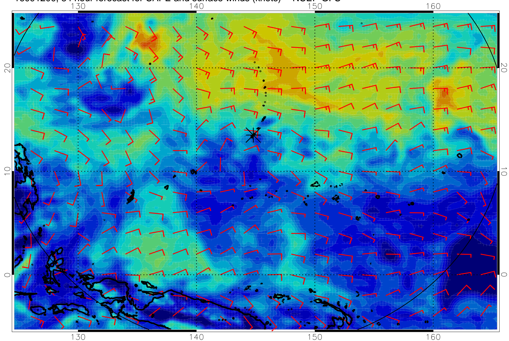
16091200, 84 hour forecast for CAPE and surface winds (knots) -- NCEP GFS
