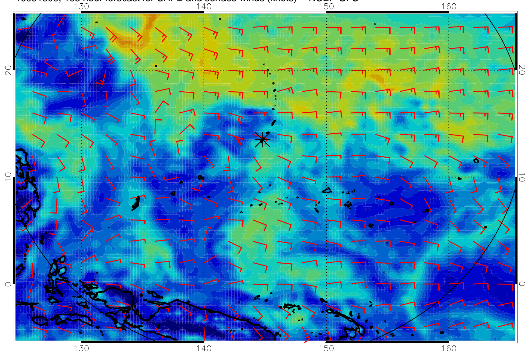
16091300, 108 hour forecast for CAPE and surface winds (knots) -- NCEP GFS
