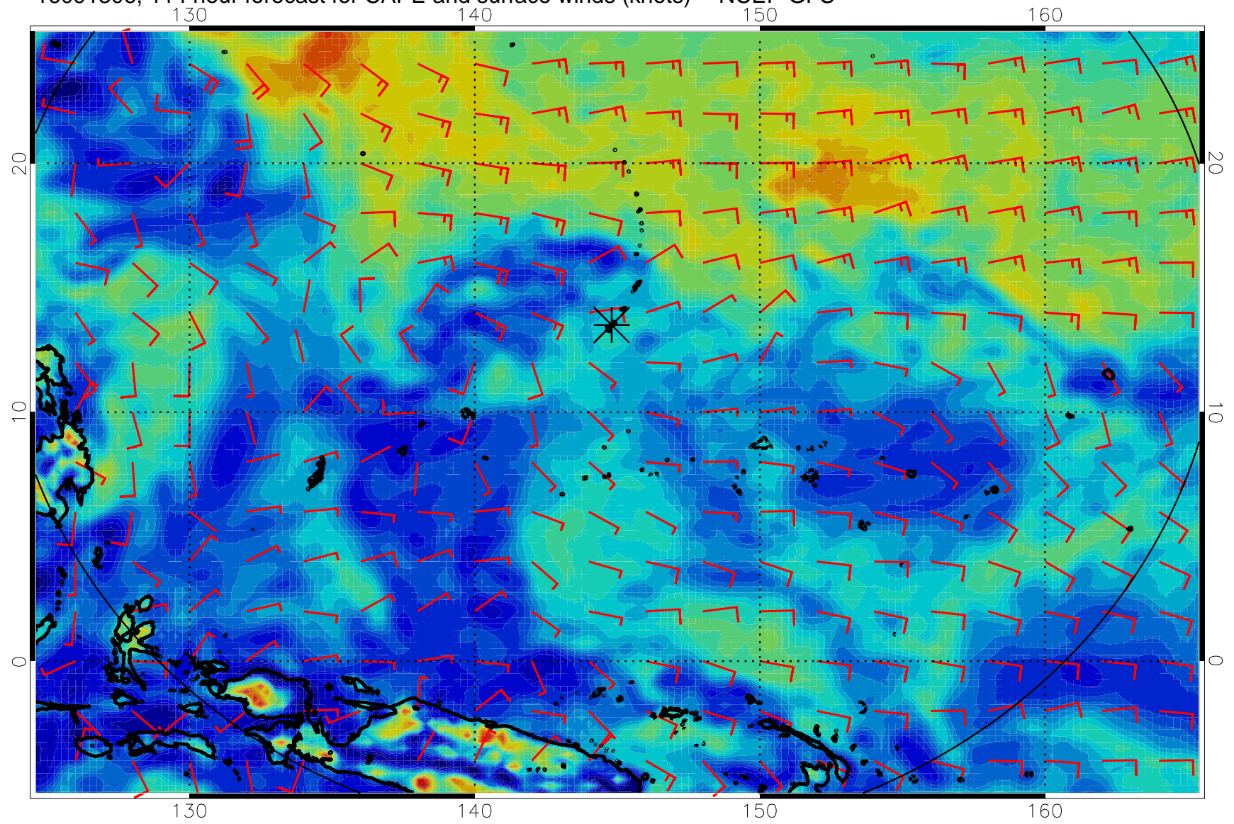
16091306, 114 hour forecast for CAPE and surface winds (knots) -- NCEP GFS
