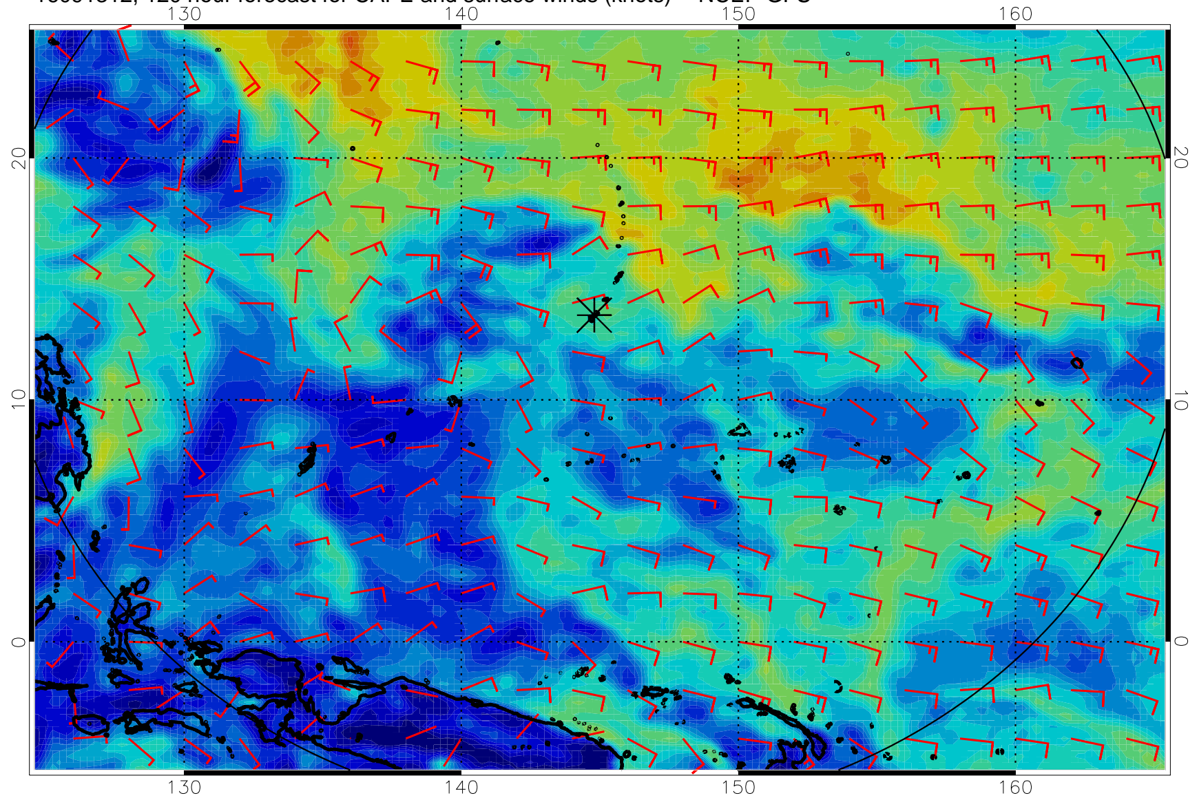
16091312, 120 hour forecast for CAPE and surface winds (knots) -- NCEP GFS
