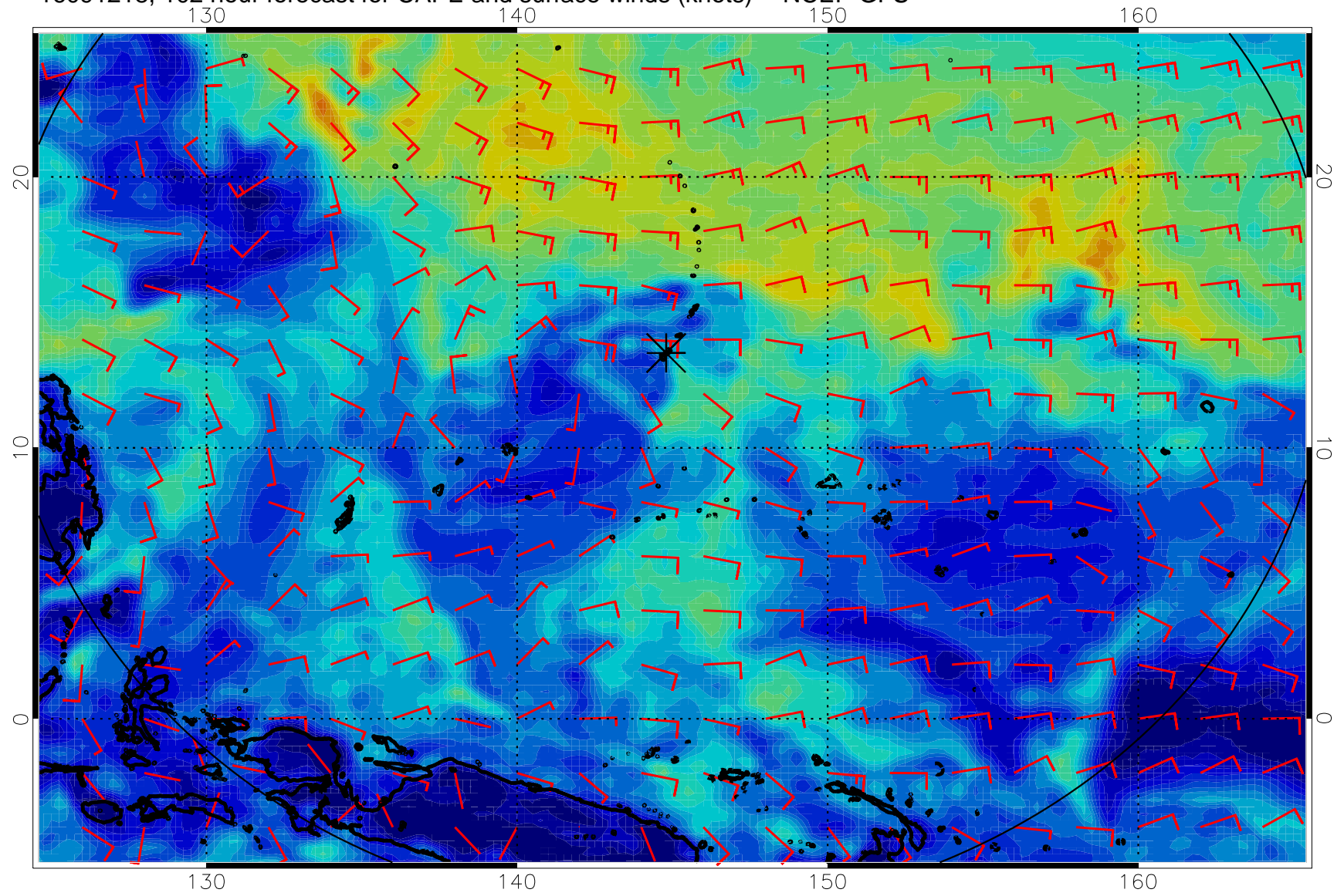
16091218, 102 hour forecast for CAPE and surface winds (knots) -- NCEP GFS
