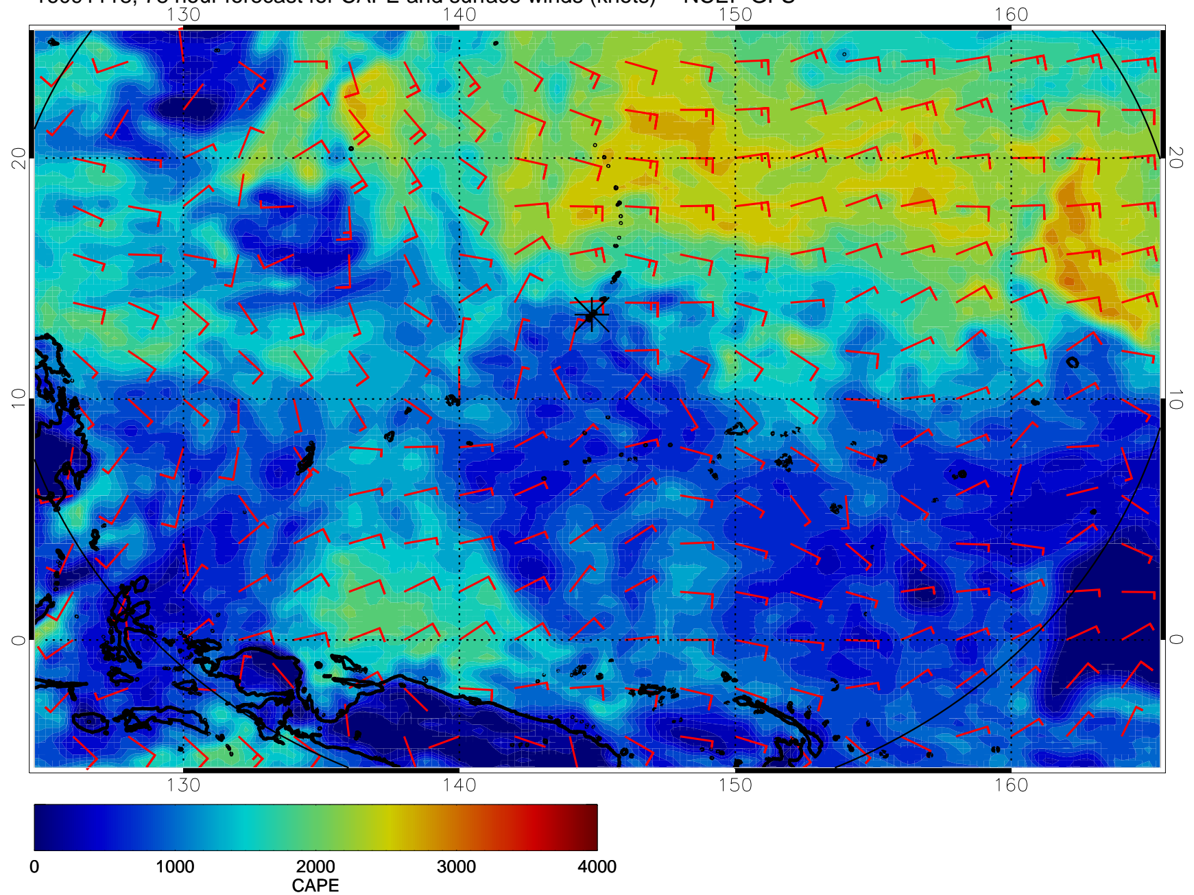
16091118, 78 hour forecast for CAPE and surface winds (knots) -- NCEP GFS
