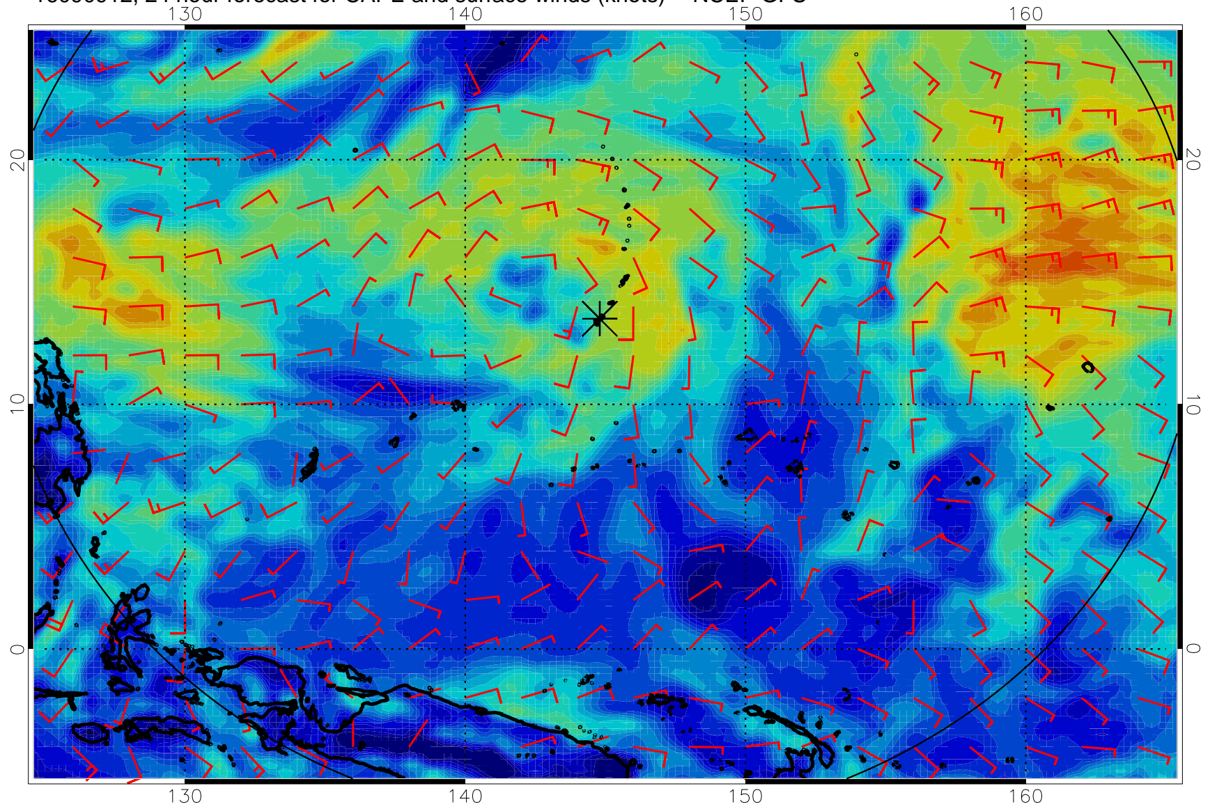
16090912, 24 hour forecast for CAPE and surface winds (knots) -- NCEP GFS
