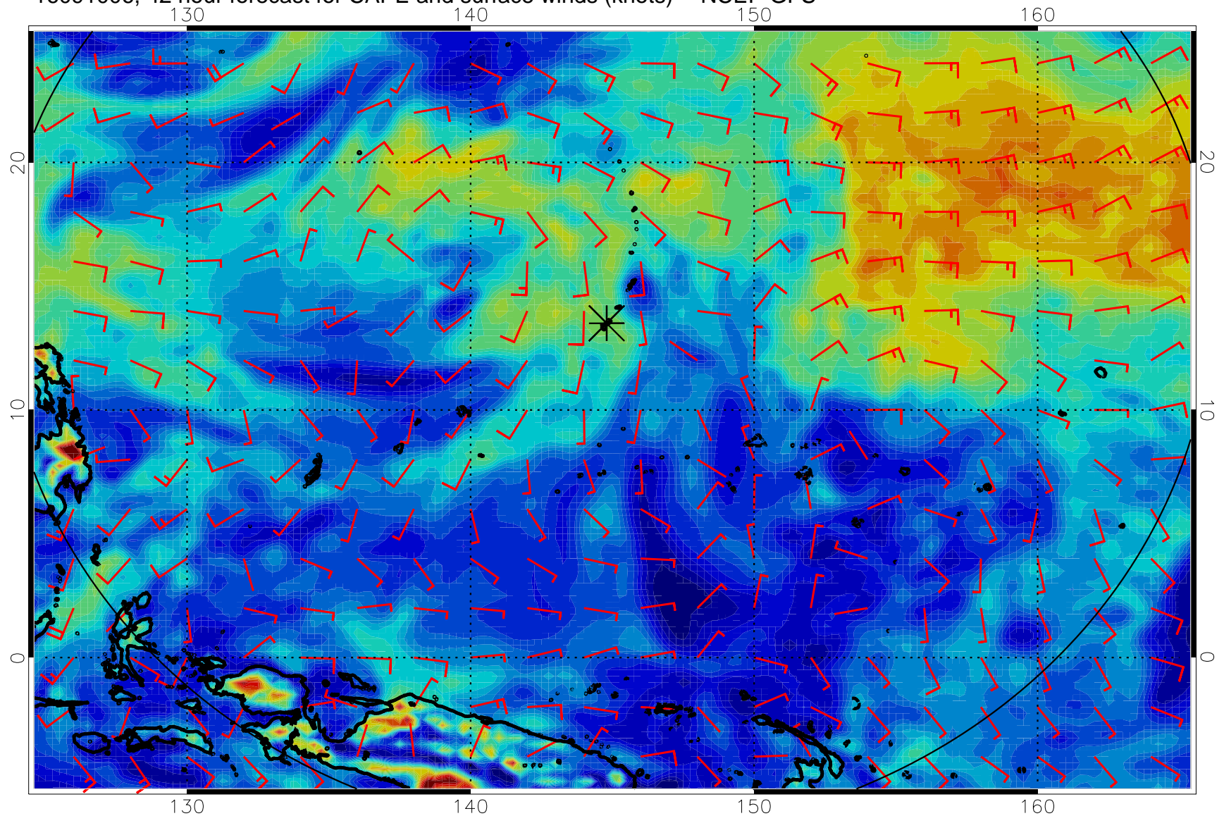
16091006, 42 hour forecast for CAPE and surface winds (knots) -- NCEP GFS
