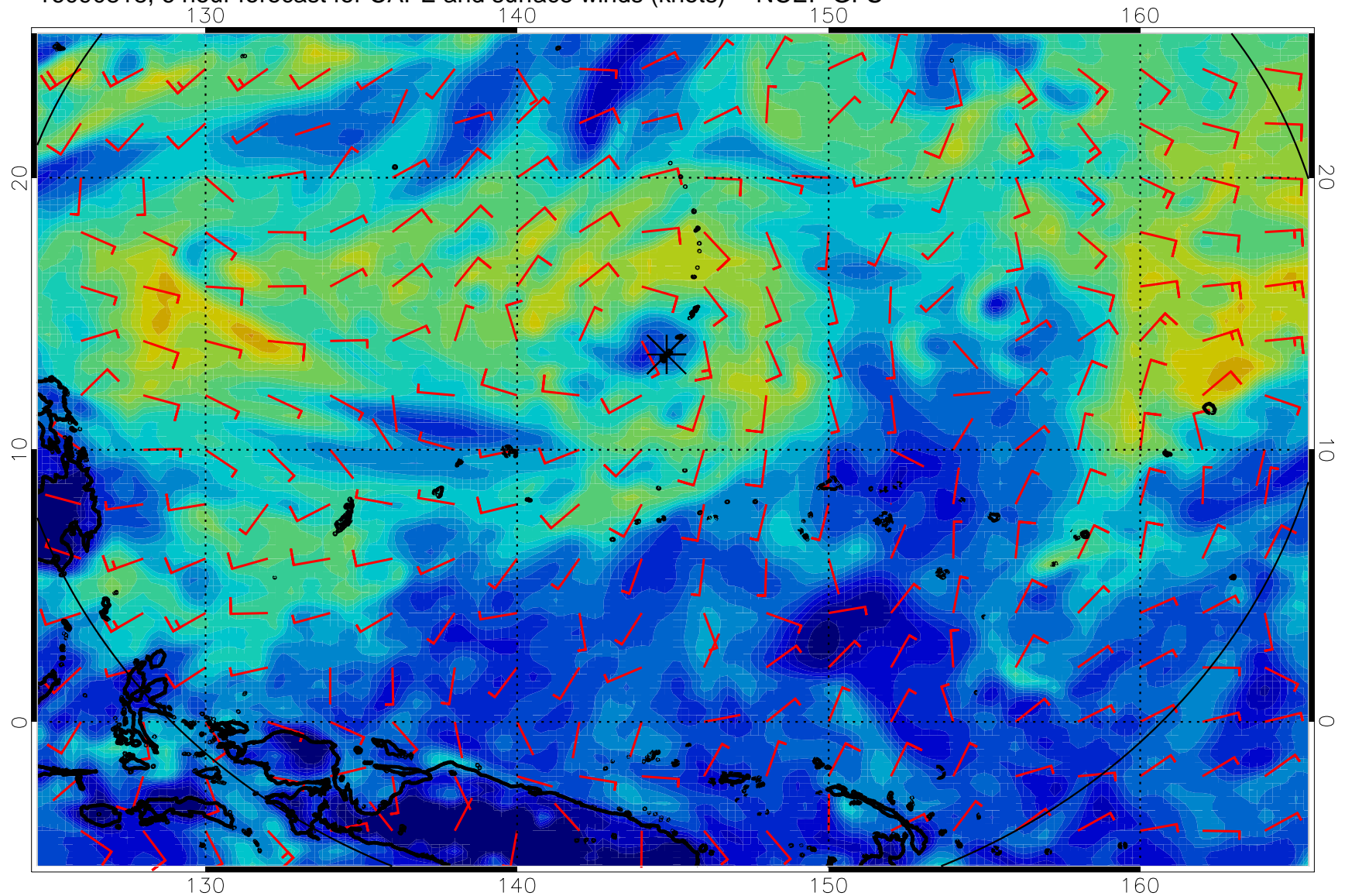
16090818, 6 hour forecast for CAPE and surface winds (knots) -- NCEP GFS
