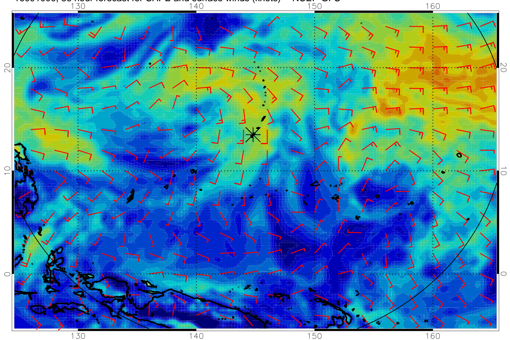
16091000, 36 hour forecast for CAPE and surface winds (knots) -- NCEP GFS
