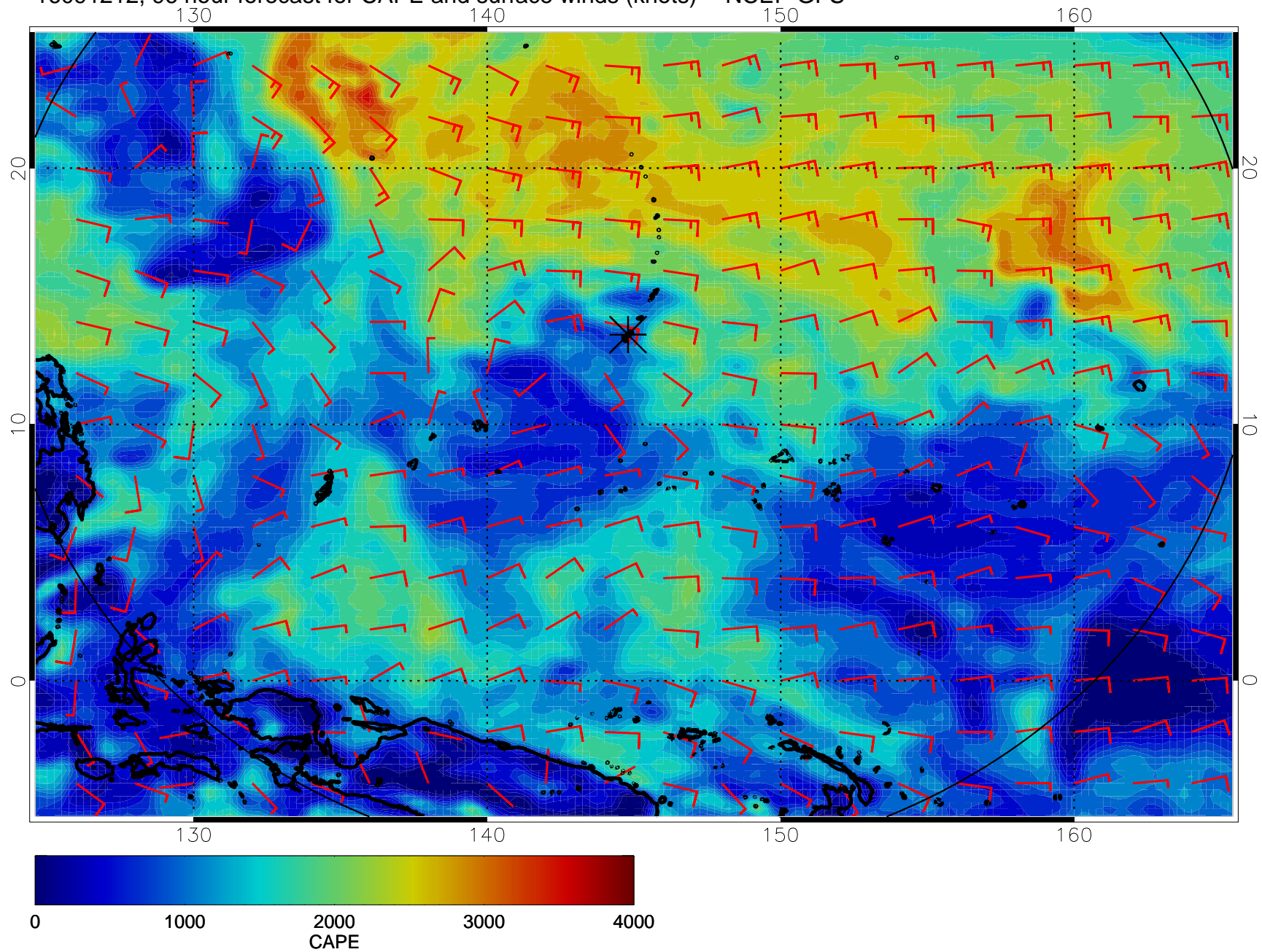
16091212, 96 hour forecast for CAPE and surface winds (knots) -- NCEP GFS
