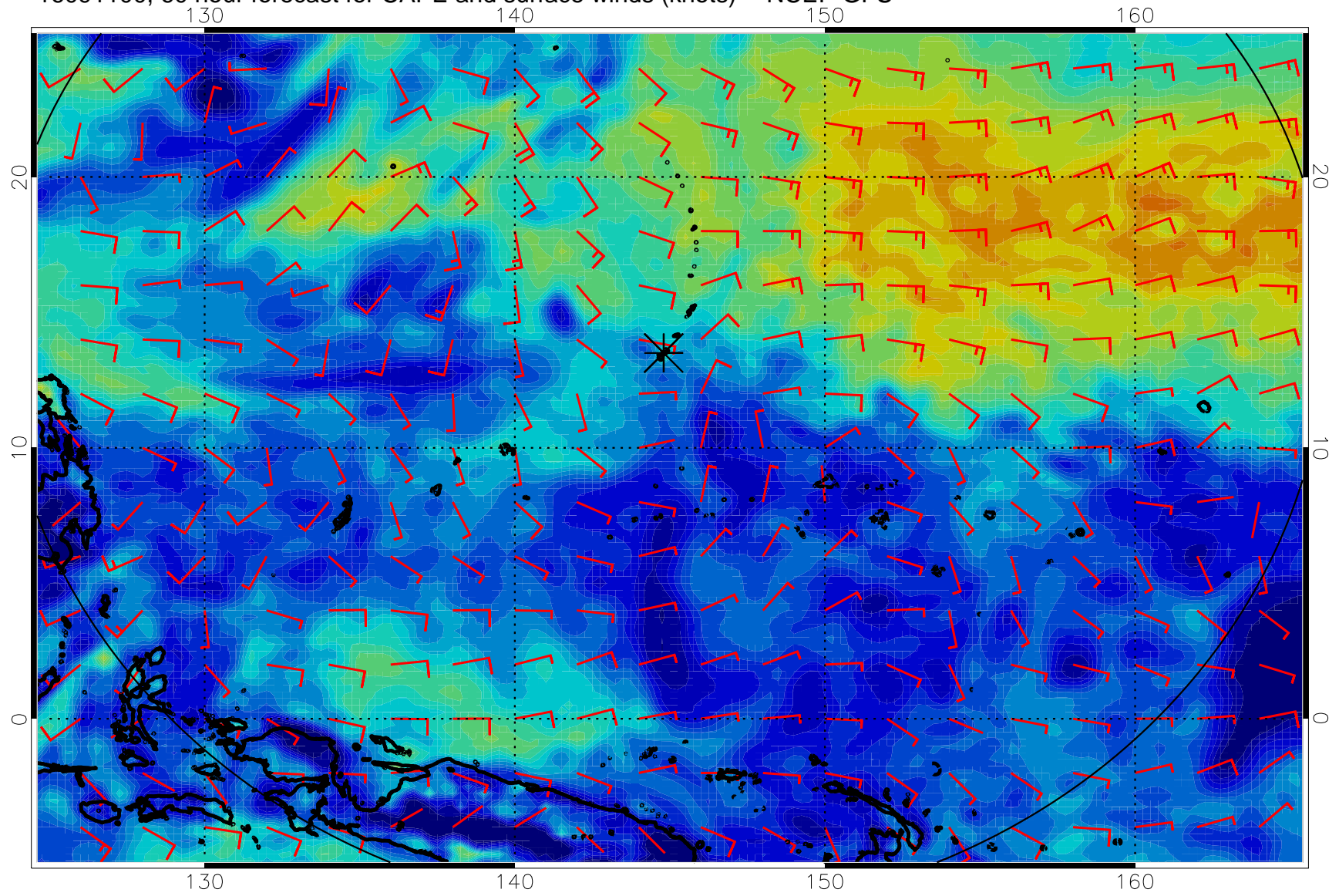
16091100, 60 hour forecast for CAPE and surface winds (knots) -- NCEP GFS
